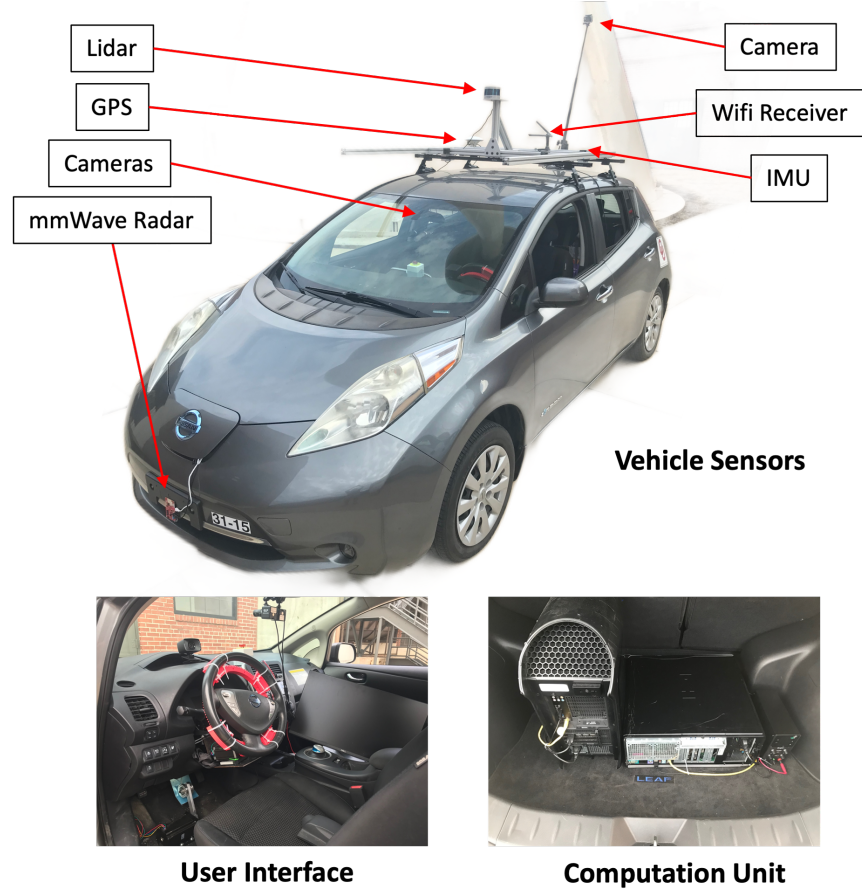
Figure 2.5: Environment perception sensors, human-machine interface and computation unit of the Nissan Leaf test car at The University of Oklahoma Mobility and Intelligence Lab
