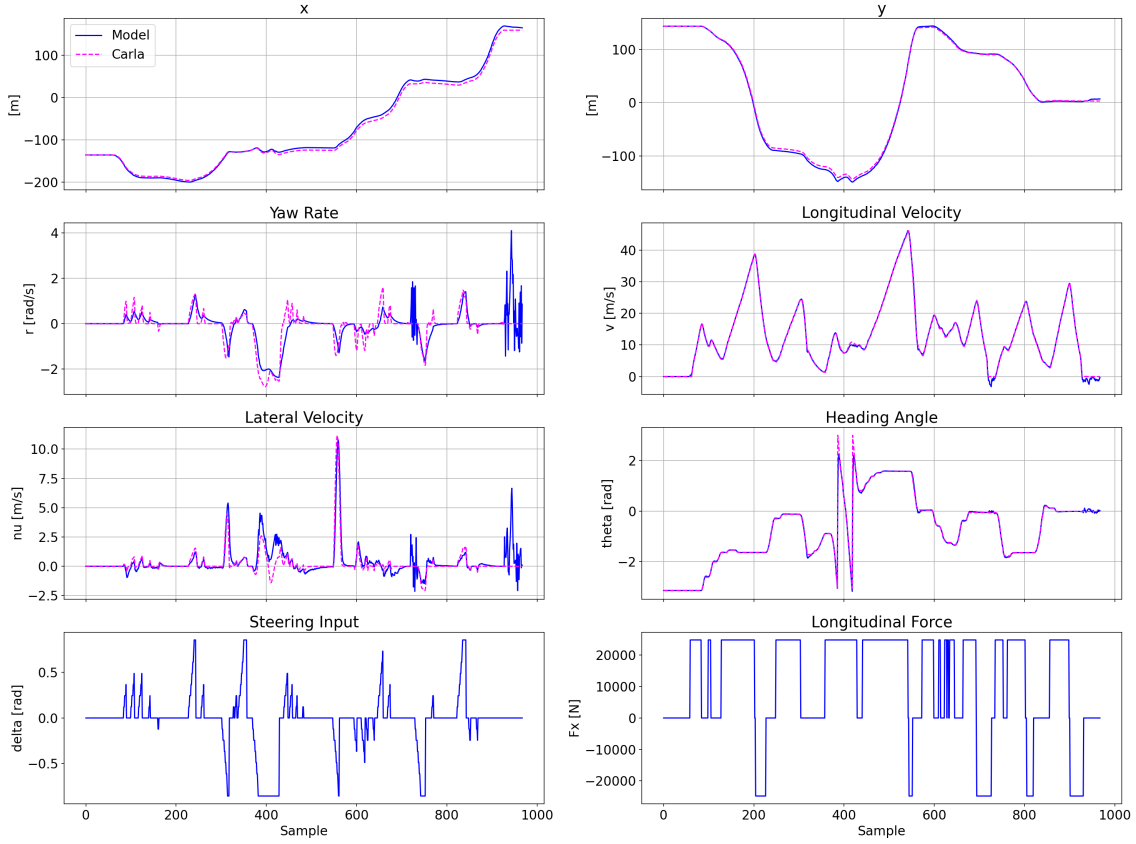
Figure 4.2: Model's output vs CARLA's data after applying EKF
