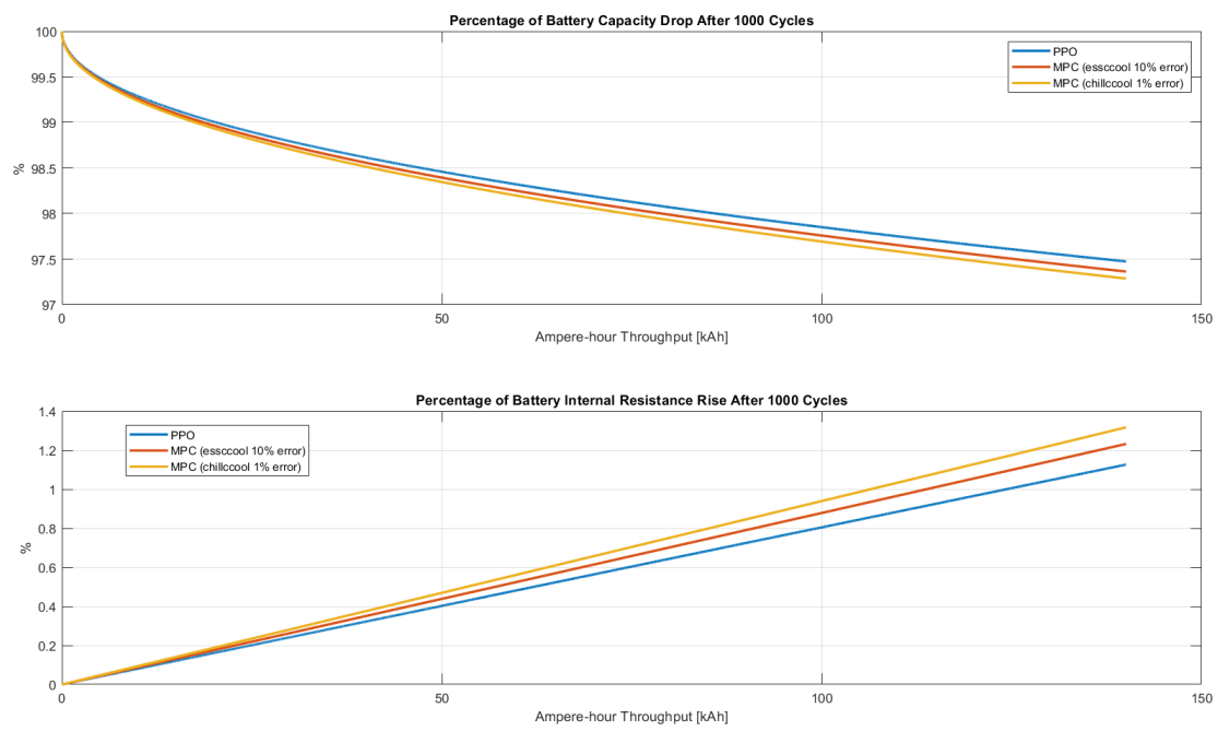
Figure 5.10: Battery aging after 1000 cycles in PPO, MPC with 10% and 1% model errors
