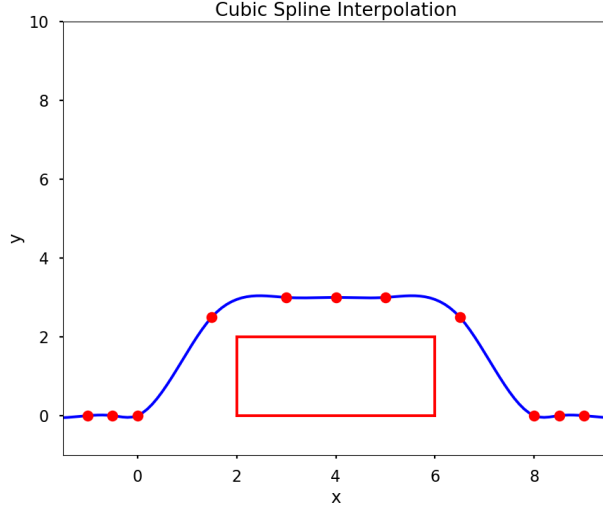
Figure 4.3: Adding the obstacle to the road boundary
