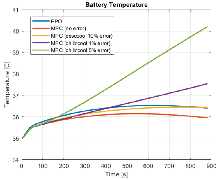
Figure 5.9: The impact of model error on MPC results
