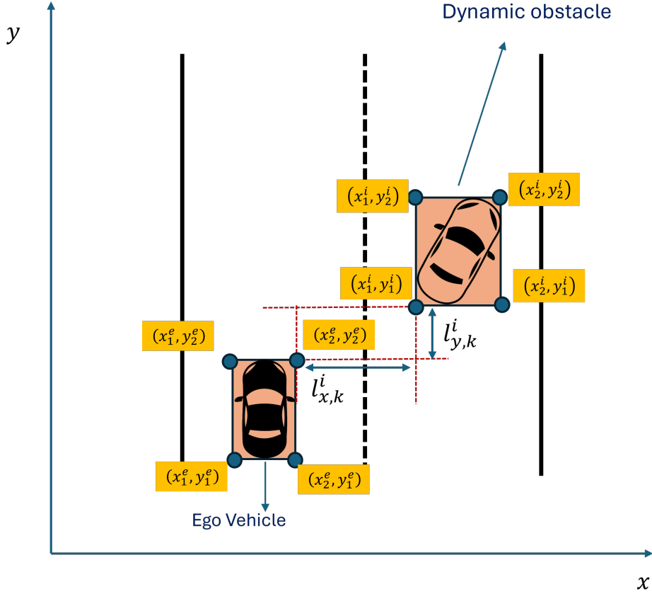
Figure 3.1: r_k components l_{x,k}^i and l_{y,k}^i
