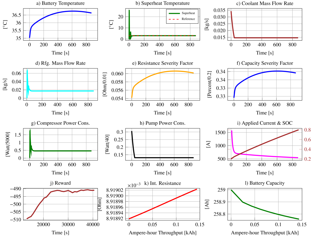
Figure 5.8: PPO results with 6C charging current
