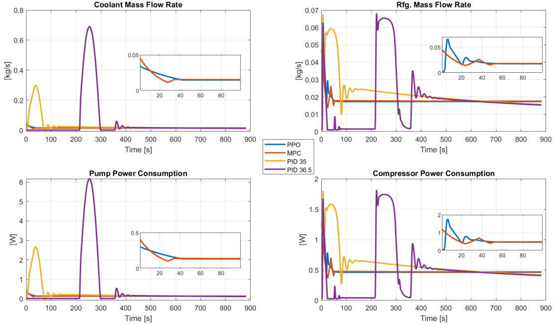
Figure 5.6: Coolant and refrigerant mass flow rates, as well as pump and compressor power consumption in all cases.
