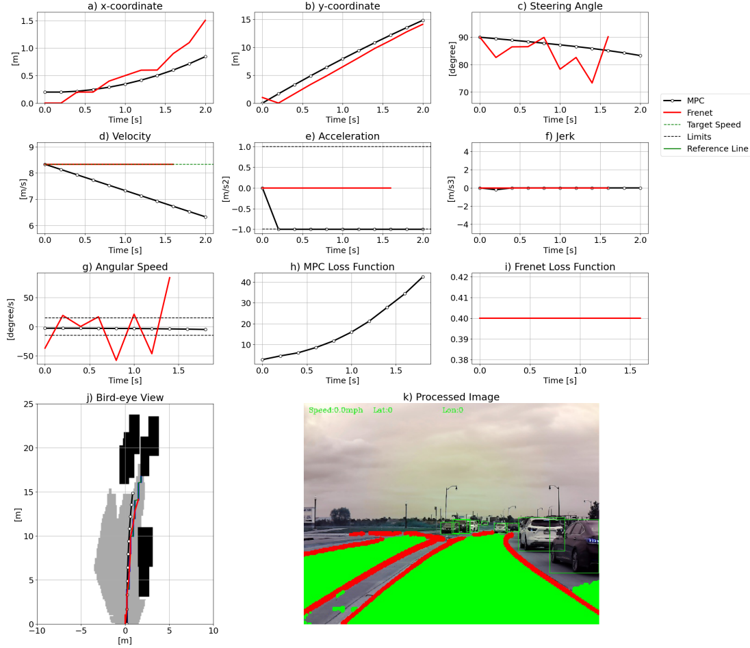
Figure 2.8: The results of scenario 3
