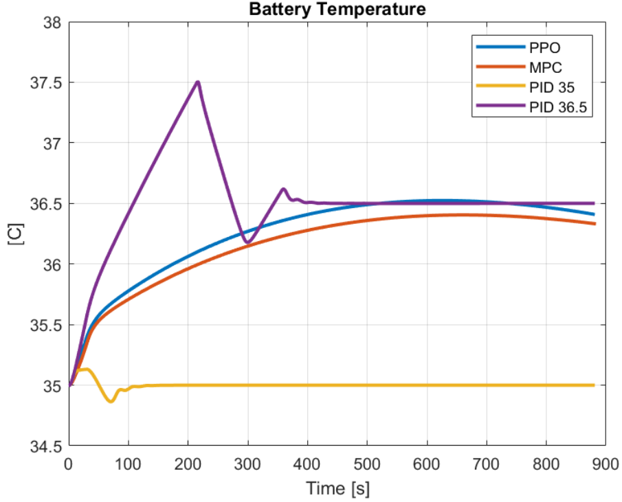
Figure 5.5: Battery Temperature Elevation.
