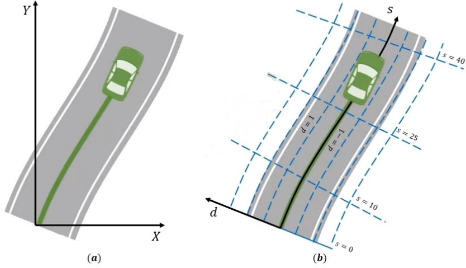
Figure 2.4: a) Cartesian coordinate, and b) Frenet coordinate
