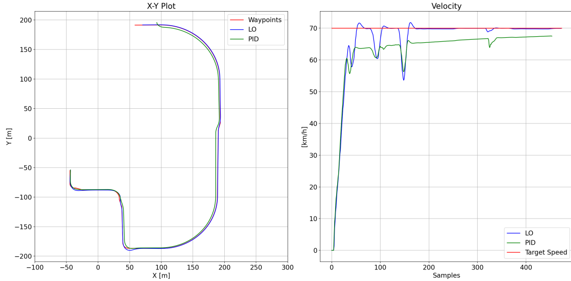
Figure 4.9: LO and PID local path planning and target speed tracking results.
