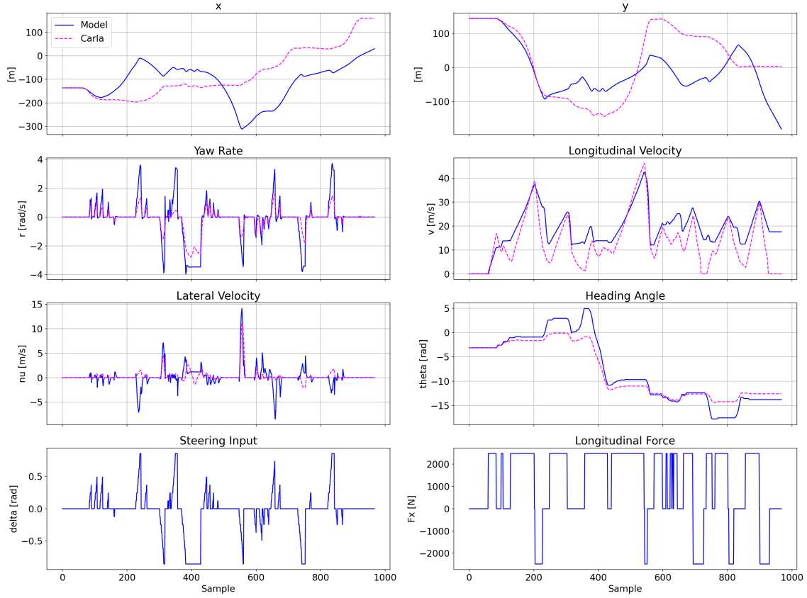
Figure 4.1: Model's output vs CARLA's data
