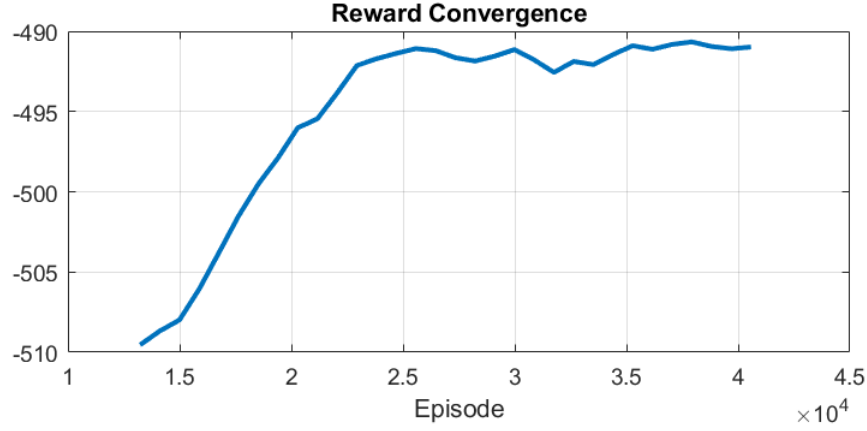
Figure 5.4: PPO reward convergence during train.
