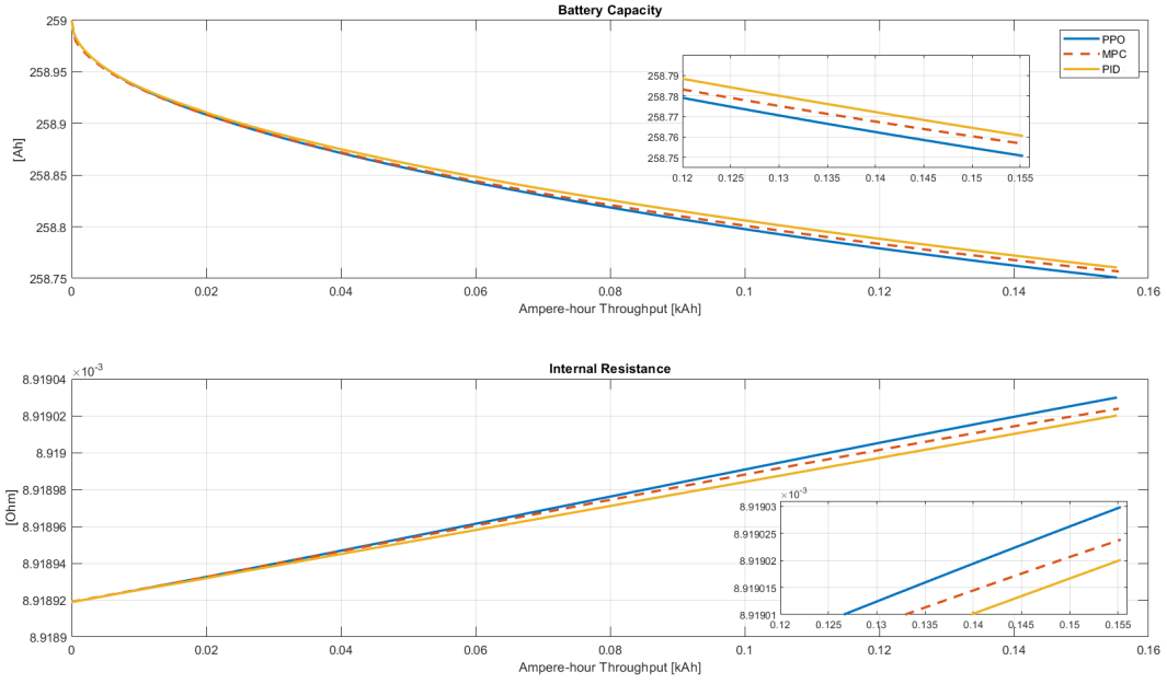
Figure 5.7: Fresh battery aging after one fast charging session in different cases
