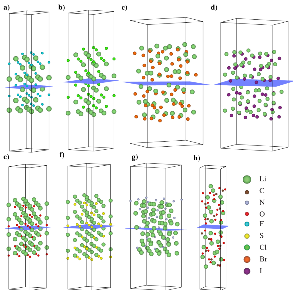
Figure 5.2: Representative homogeneous ( \Sigma 3 ) grain boundaries constructed by cleaving along the (-111) plane for (a) LiF, (b) LiCl, (c) LiBr (d) LiI, (e) \text{Li}_2\text{O} , (f) \text{Li}_2\text{S} , (g) \text{Li}_3\text{N} , and (h) \text{Li}_2\text{CO}_3 . The grain-boundary interface is highlighted in blue.
