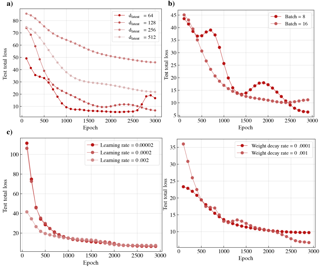
Figure C.15: Tuning of GVAE for grain boundary diffusion: a) latent dimension ( d_{latent} ), b) batch, c) learning rate and (d) weight decay rate in Adam optimizer.
