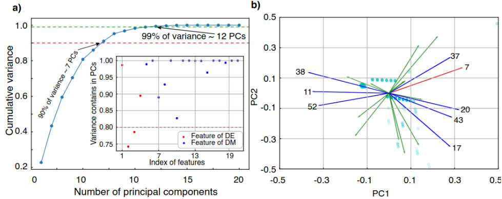
Figure 4.18: PC analysis; a) PCs that explain cumulative variance with inset graph that depicts variance of features represented by 12 PCs and b) most contributed features in PC space spanned by first two PCs. The eigenvectors of features are projected as arrows. The important features of diffusing elements are marked in red, diffusion media in blue, and other less contributing features in green color. The scatter plot in the background illustrates the scaled distribution of data points in PC space.
