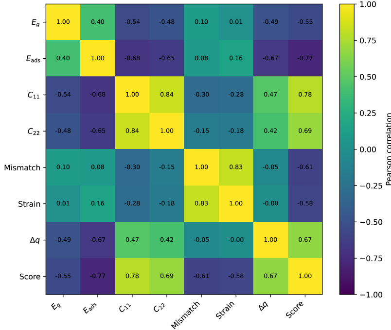
Figure 6.7: Pearson correlation coefficient between the normalized descriptors of Li-metal-MXene heterosystems.
