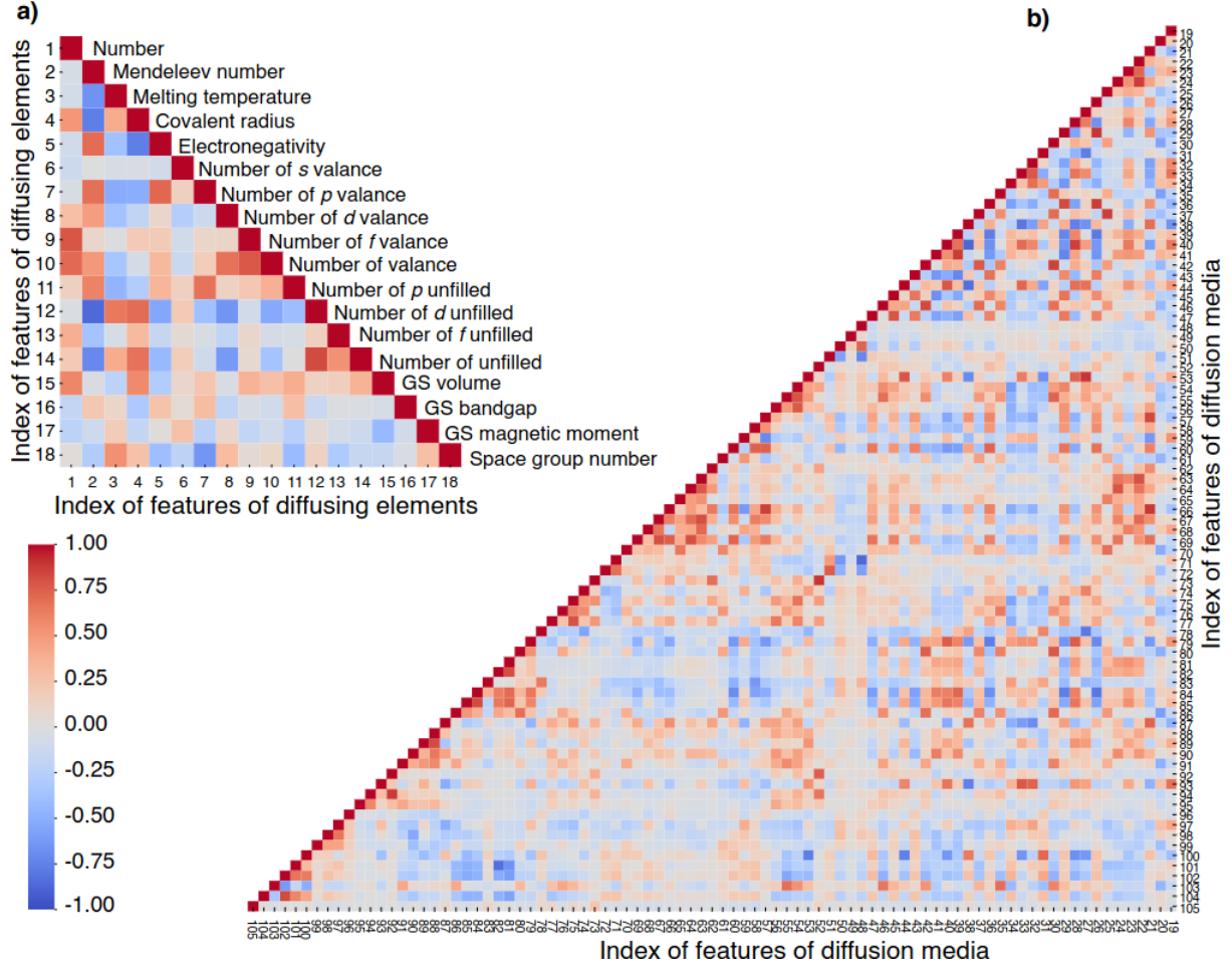
Figure C.6: Correlation values of features of a) diffusing elements and b) diffusion media for the model self diffusion in MCA media. Name of features of diffusion media with respective indices are given in Table C.2
