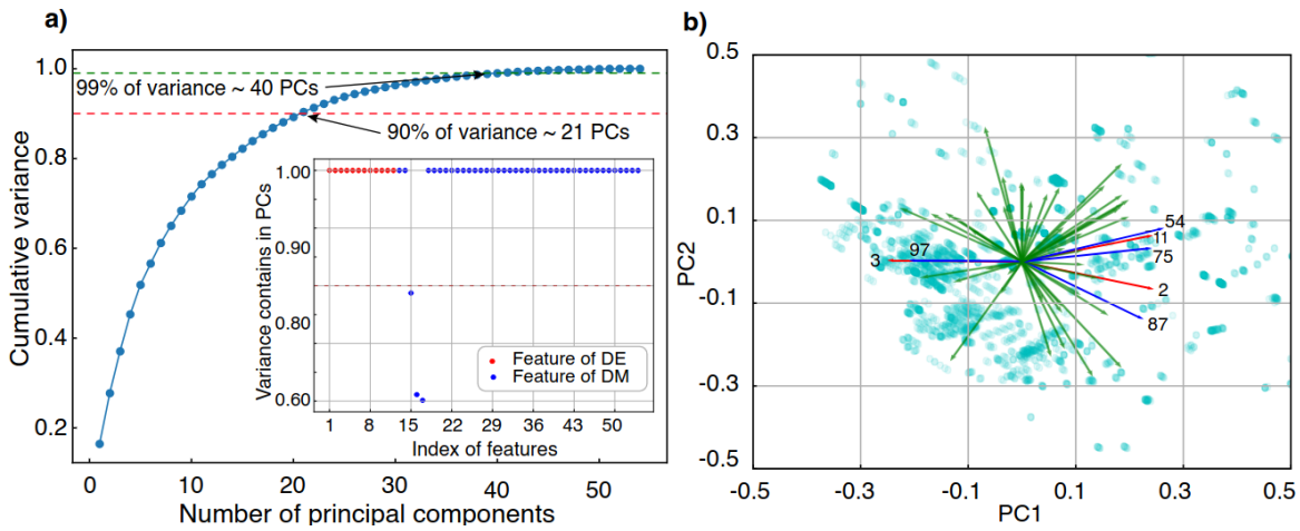
Figure 4.10: PC analysis – self diffusion in MCA media; a) PCs that explain cumulative variance with inset graph that depicts variance of features represented by 40 PCs and b) most contributed features in PC space spanned by first two PCs. The eigenvectors of features are projected as arrows. The important features of diffusing elements are marked in red, diffusion media in blue and other less contributing features in green color. The scatter plot in the background illustrates the scaled distribution of data points in PC space.
