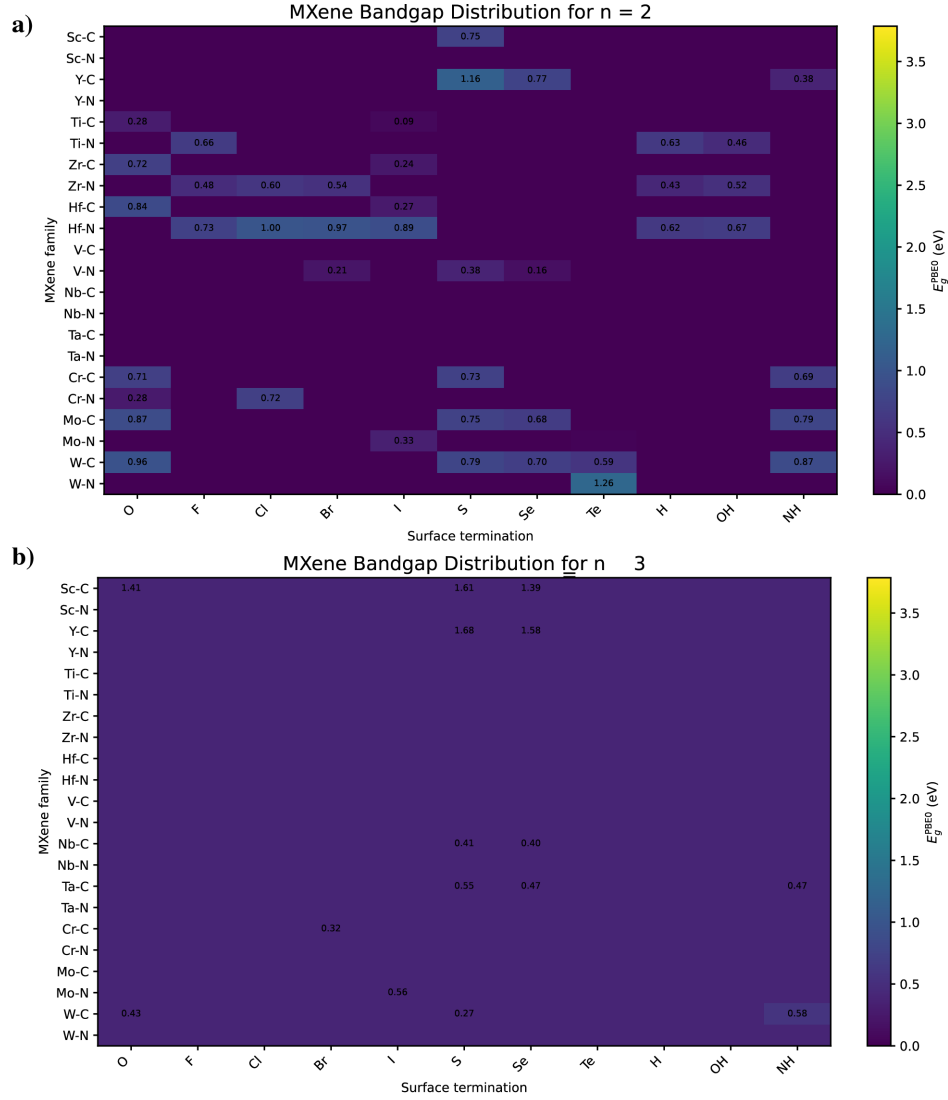
Figure C.18: PBE0 bandgap distribution of the MXene configurations with n = 2, 3 .
