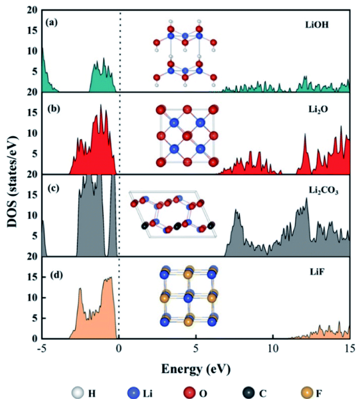
Figure 2.3: Total electronic density of states and the crystal structure of (a) LiOH, (b) Li 2 O, (c) Li 2 CO 3 , and (d) LiF. The dashed line indicates the location of the valence band maxima, which is set to zero. Reproduced with permission from reference [61]. Copyright 2021 The Royal Society of Chemistry.
