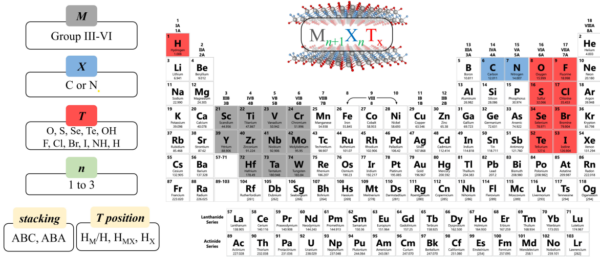
Figure 6.1: MXene phases considered for high-throughput screening for integrating into SEI. Total of 4356 different MXene structures. In the figure M stands for transition metals, X for carbides/nitrides, T for surface terminations, and n is number of the layers in MXene phase. This structure database refereed from MXgap dataset developed by Ontiveros et al. [308]
