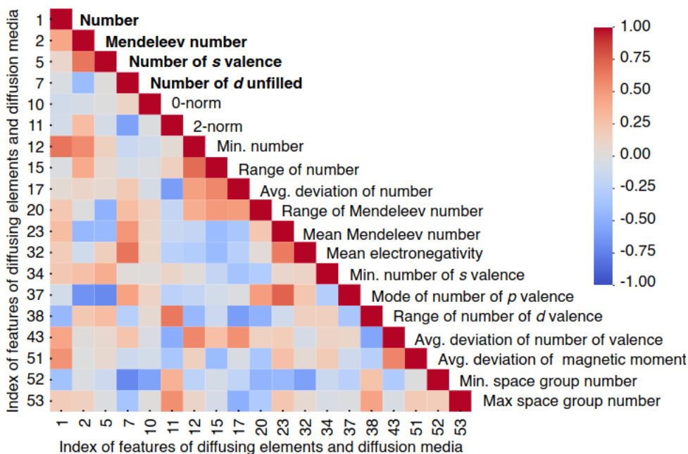
Figure 4.17: Feature space – chemical diffusion in MCA media: combined feature space used for training. Features of diffusing elements are highlighted in bold characters and diffusion media in regular fonts (Individual feature space of diffusing element and diffusion media for this model are given in Figure C.8a and b respectively). Common abbreviations such as ‘min.’ for minimum, ‘avg.’ for average, and ‘dev.’ for deviation are used.
