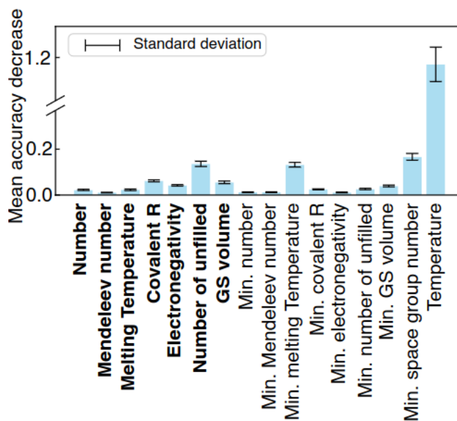
Figure 4.4: Feature importance – impurity diffusion in IM media: features of diffusing elements are highlighted in bold fonts and diffusion media are given in normal fonts.
