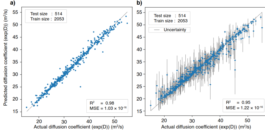
Figure 4.15: Performance of model – impurity diffusion in MCA media when trained with a) the entire feature space (dimension: 2567 \times 49 ) and b) principal components of the entire feature space (dimension: 2567 \times 43 ). The vertical gray solid lines depict the uncertainty associated with each data point.
