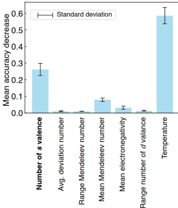
Figure 4.20: Feature importance – chemical diffusion in MCA media: Features of diffusing elements are highlighted in bold font and diffusion media are given in normal font.
