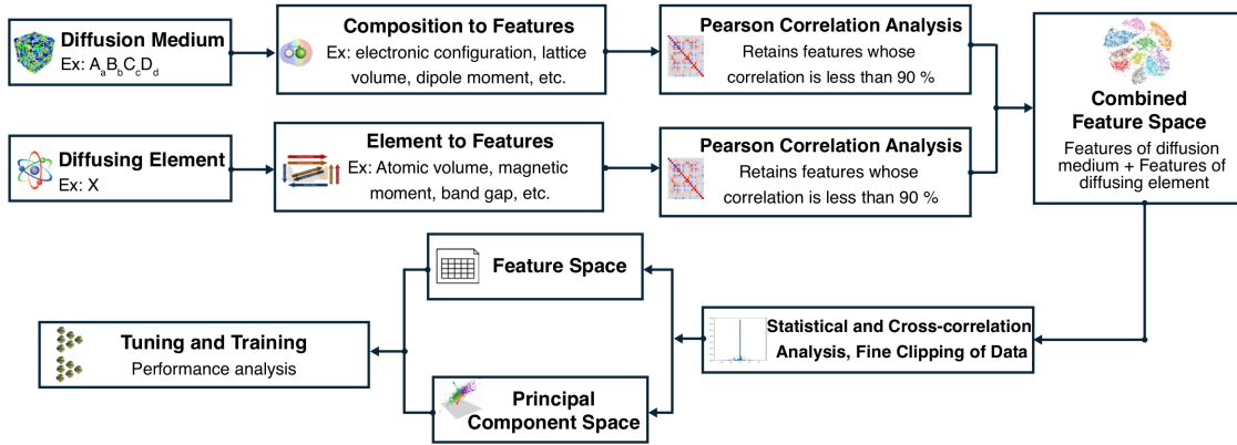
Figure 3.3: Workflow of predictive modeling of diffusion coefficient in conventional alloys.
