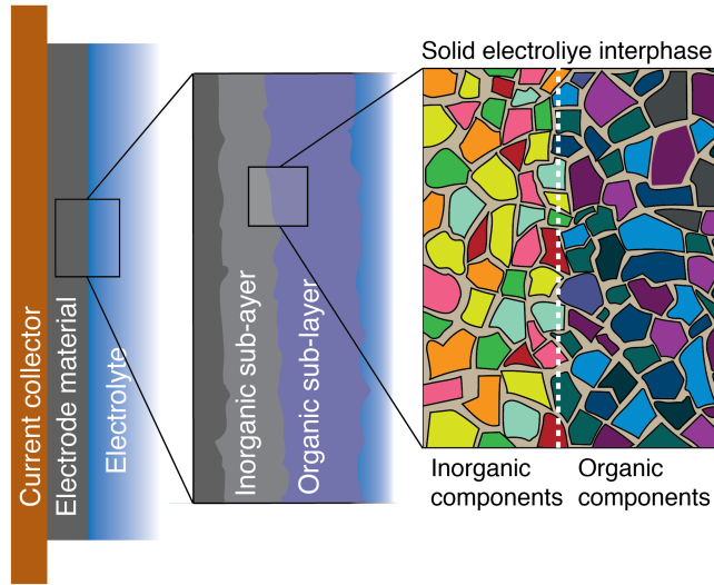
Figure 1.2: A generic illustration of multi-component, bi-layered mosaic-model of SEI. The inorganic part mostly composed of lithium halides, oxides, sulfides and carbonates while inorganic part includes short-chain alkyl carbonates, poly-sulfides and polymeric species formed from reduction products of additives and organic solvents in electrolyte[44, 45].
