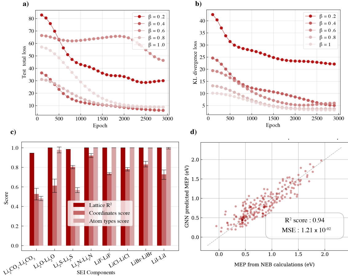
Figure 5.11: For grain boundary diffusion, performance of the GVAE model in terms of convergence of the (a) total test loss and (b) KL divergence for different values of the weighting parameter \beta ranging from 0.2 to 1.0. The reconstruction performance of the GVAE for lattice parameters, atomic coordinates, and atom types is shown in (c), and the corresponding R^2 score for migration-barrier prediction using GNN model is shown in (d).
