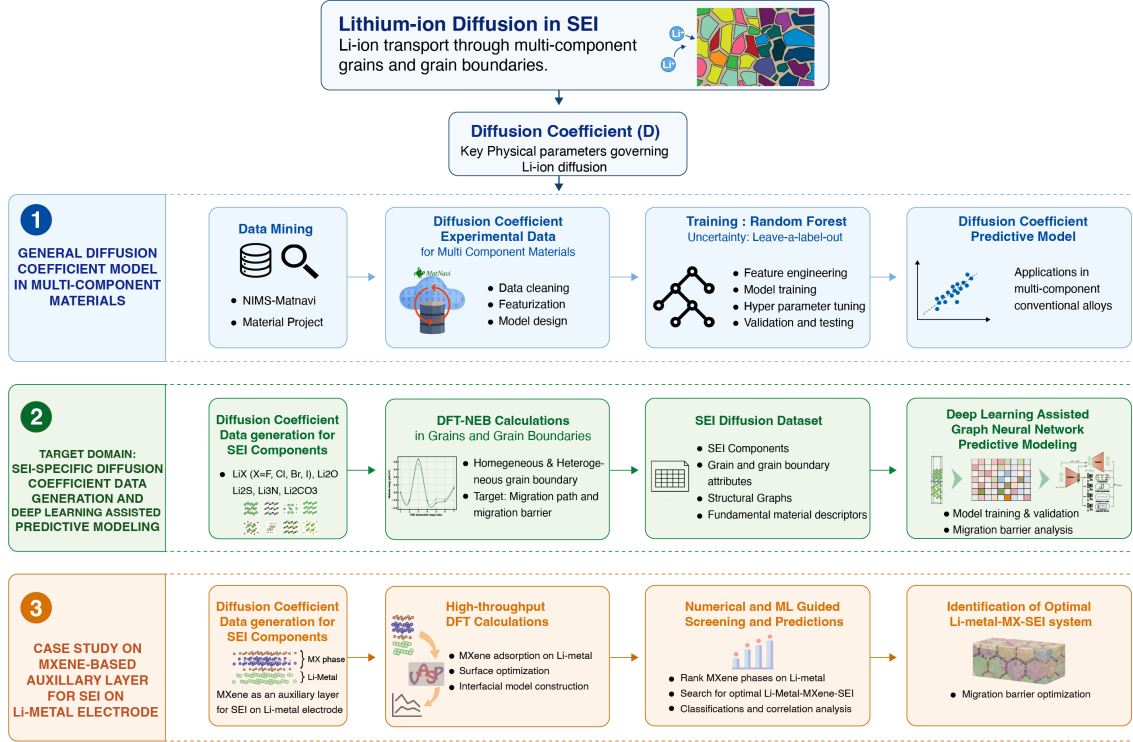
Figure 1.3: Schematic representation of the thesis workflow for understanding and engineering Li-ion diffusion in the SEI. The study begins with the development of a generalized diffusion coefficient modeling framework for multicomponent materials using curated experimental datasets and machine learning approaches. This is followed by SEI-specific diffusion modeling, involving targeted data generation, physicochemical feature engineering, and predictive modeling to capture Li-ion transport behavior within the complex SEI environment. Finally, a design-oriented case study on MXene-based interfacial coatings is conducted using combined DFT and machine learning methods to identify optimized surface terminations that promote uniform Li-ion transport and enable stable SEI formation.
