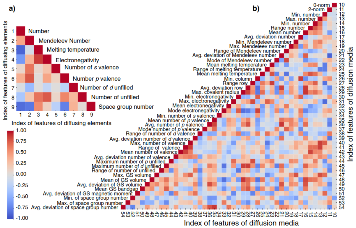
Figure C.8: Mutual correlation values of features of diffusing elements and diffusion media for the model impurity diffusion in MCA media.
