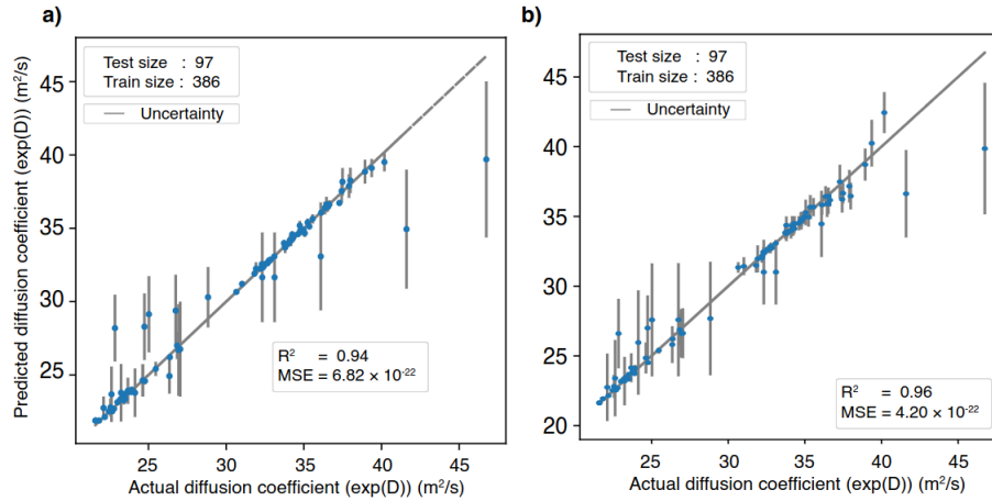
Figure 4.19: Performance of model – chemical diffusion in MCA media: a) when trained with the entire feature space (dimension: 483 \times 20 ) and b) with principal components of the entire feature space (dimension: 483 \times 12 ). The gray solid lines depict the uncertainty associated with each data point.
