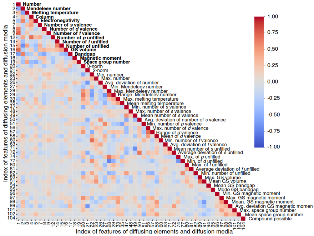
Figure 4.13: Feature space – impurity diffusion in MCA media: combined feature space used for training. Features of diffusing elements are highlighted in bold characters and diffusion media in regular fonts (Individual feature space of diffusing element and diffusion media for this model are given in Figure C.7a and b respectively). Common abbreviations such as ‘min.’ for minimum, ‘avg.’ for average, and ‘dev.’ for deviation are used.
