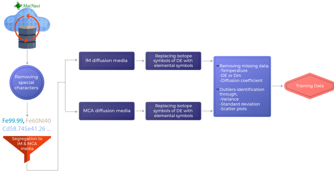
Figure C.3: Schematic diagram of material data preprocessing. The program used for preprocessing is available in GitHub repository, https://github.com/yanqingsu/ML-DiCE
