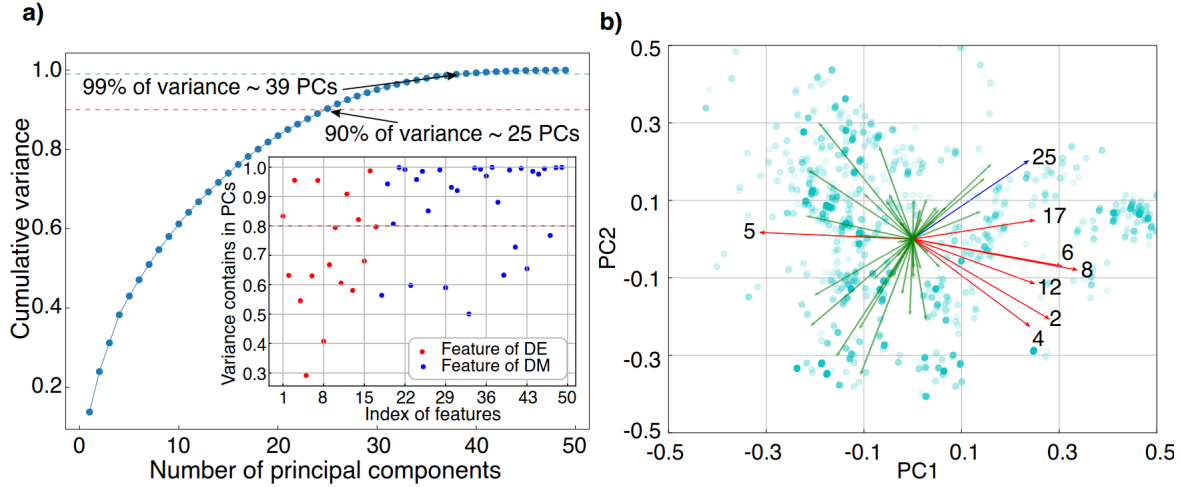
Figure 4.2: PC analysis; a) PCs that explain cumulative variance with inset graph that depicts variance of features represented by 25 PCs and b) most contributed features in PC space spanned by first two PCs. The eigenvectors of features are projected as arrows. The important features of diffusing element are marked in red, diffusion media in blue, and other less contributing features in green color. The scatter plot in the background illustrates the scaled distribution of data points in PC space.
