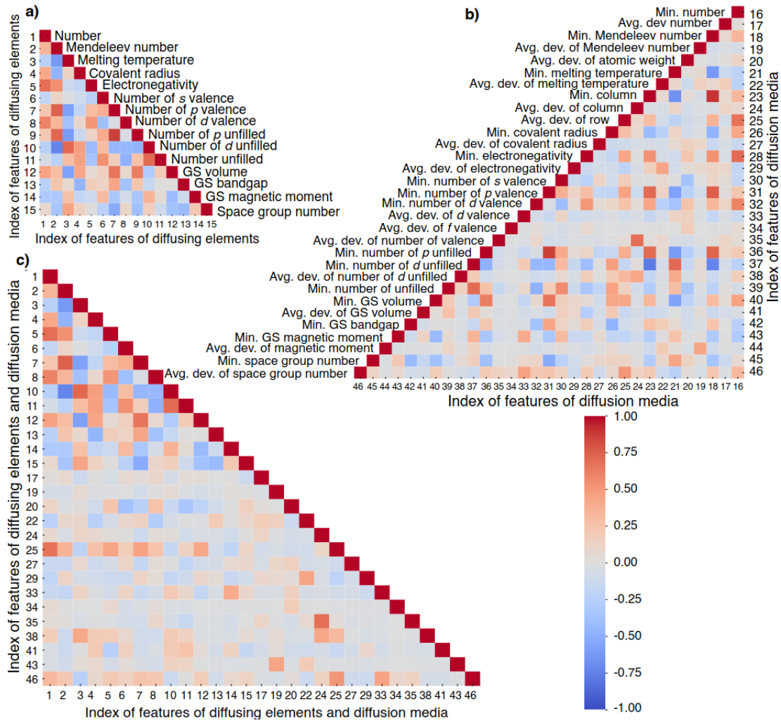
Figure 4.5: Feature spaces – self diffusion in IM media for a) diffusing elements, b) diffusion media, and c) the combined feature space used for training. Features of diffusing element and diffusion media are indexed sequentially and the respective indices are marked in the combined feature space for reference. Common abbreviations such as ‘min.’ for minimum, ‘avg.’ for average, and ‘dev.’ for deviation are used.
