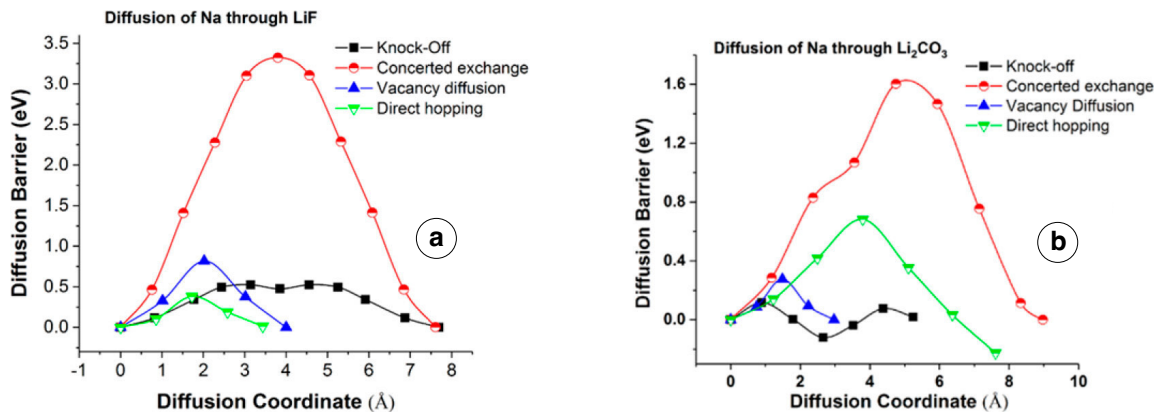
Figure 2.2: Diffusion profiles of the different ionic migration mechanisms for (a) LiF, (b) \text{Li}_2\text{CO}_3 . Adapted with permission from reference [25]. Copyright 2018 American Chemical Society.
