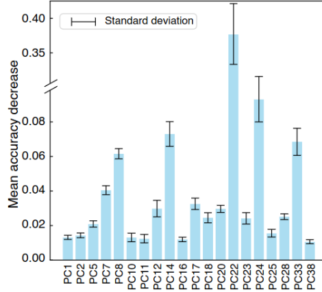
Figure 4.12: Feature importance – self diffusion in MCA media: MLPRegressor were used with feature permutation scheme. Features of diffusing elements are highlighted in bold font and diffusion media are given in normal font.
