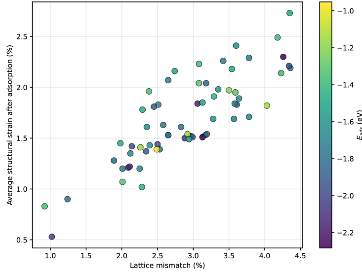
Figure 6.4: Scatter plot showing the relationship between lattice mismatch and average structural strain after MXene adsorption on Li metal. A positive correlation between the two descriptors is observed, indicating that larger lattice mismatch generally leads to increased interfacial distortion after adsorption. The color scale represents the adsorption energy of the corresponding Li–MXene heterostructures.
