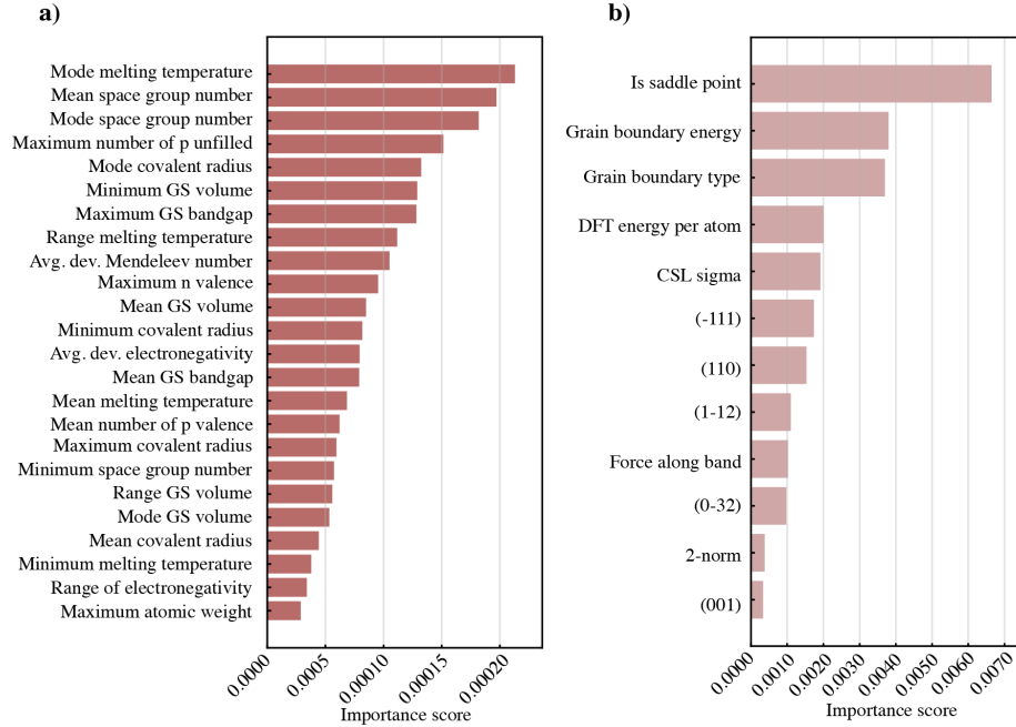
Figure 5.12: Feature importance analysis of grain boundary diffusion: important features identified from the subset of a) composition-based and b) structural features are listed based on mean accuracy decrease score. The statistical measures mentioned in the beginning of each composition-derived descriptors is attributed to the elements present in SEI component. A close examination on feature importance can tell that grain boundary diffusion is strongly governed by localized structural descriptors (saddle point and grain boundary energetics) showing a sharper and strong feature importance distribution compared to grain diffusion, where structural effects are more distributed across surface-related features.
