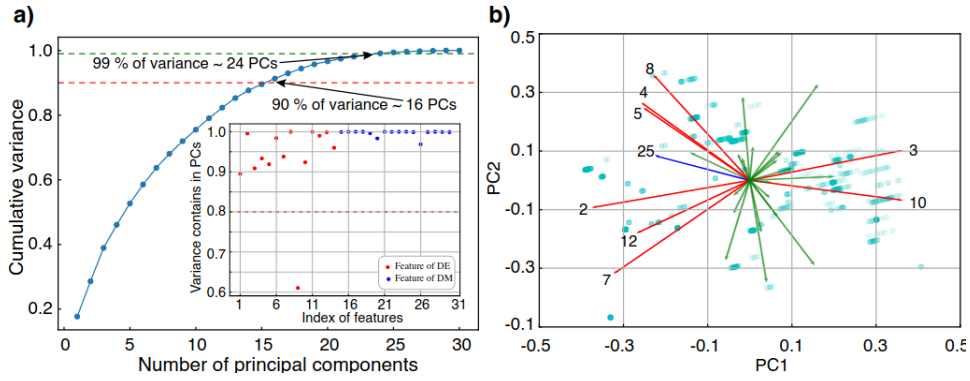
Figure 4.6: PC analysis; a) PCs that explain cumulative variance with inset graph that depicts variance of features represented by 24 PCs and b) most contributed features in PC space spanned by first two PCs. The eigenvectors of features are projected as arrows. The important features of diffusing elements are marked in red, diffusion media in blue, and other less contributing features in green color. The scatter plot in the background illustrates the scaled distribution of data points in PC space.
