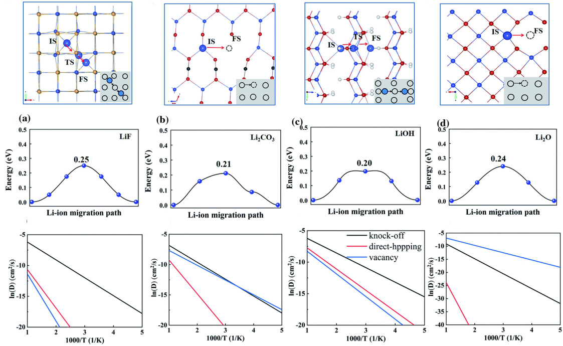
Figure 2.1: Diffusion profiles of the different ionic migration mechanisms for bulk (a) LiF, (b) Li 2 CO 3 (c) LiOH, and (d) Li 2 O. Respective models used for the calculation have been given in the first row where the circles represent the lithium vacancies. Reproduced with permission from reference [61] . Copyright 2021 The Royal Society of Chemistry.
