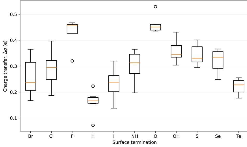
Figure 6.5: A comparative overview of charge transfer between MXene and Li-metal illustrated as box-plots. As expected, MXene with oxygen and fluorine surface terminations exhibits elevated charge transfer that point towards the comparatively better stability of adsorbed MXene.
