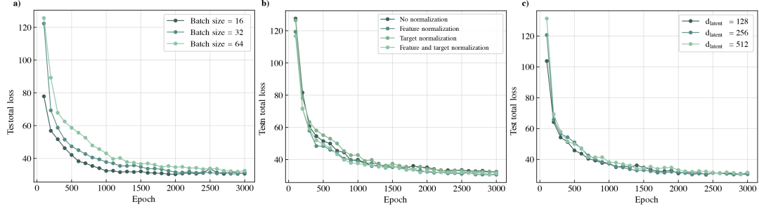
Figure C.10: Results of GVAE model tuning; a) total loss of test with varying batch sizes, b) normalization among feature/target, and latent dimension.
