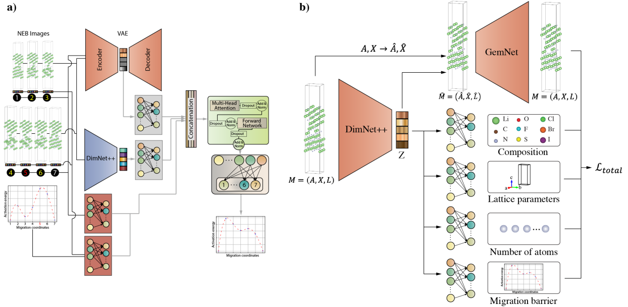
Figure 5.6: Schematic illustration of the (a) predictive GNN model architecture. A grain-boundary NEB data point for LiF is shown as an illustrative example. The NEB images marked in white indices represent the initial and final structures, those in yellow indicate intermediate structures, and marked in red corresponds to the saddle point. The representative boxes illustrated beneath each structure denote the compositional features. Black connecting lines represent pre-processing operations, while gray lines depict the on-the-fly training and testing pathway of the model. Panel (b) depicts architecture of of GVAE model where M is the ground truth structure and \hat{M} is the noised counterpart. A , X , and L denotes atom types, atom positions and lattice parameters. Role of GVAE in this design is to provide embedded representation of a complete NEB calculation (include all images and their features) to the GNN.
