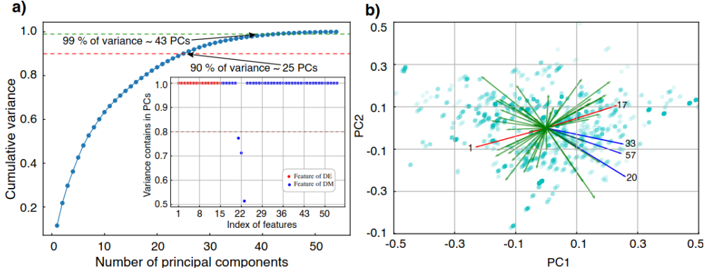
Figure 4.14: PC analysis – impurity diffusion in MCA media; a) PCs that explain cumulative variance with inset graph that depicts variance of features represented by 43 PCs and b) most contributed features in PC space spanned by first two PCs. The eigenvectors of features are projected as arrows. The important features of diffusing elements are marked in red, diffusion media in blue, and other less contributing features in green color. The scatter plot in the background illustrates the scaled distribution of data points in PC space.
