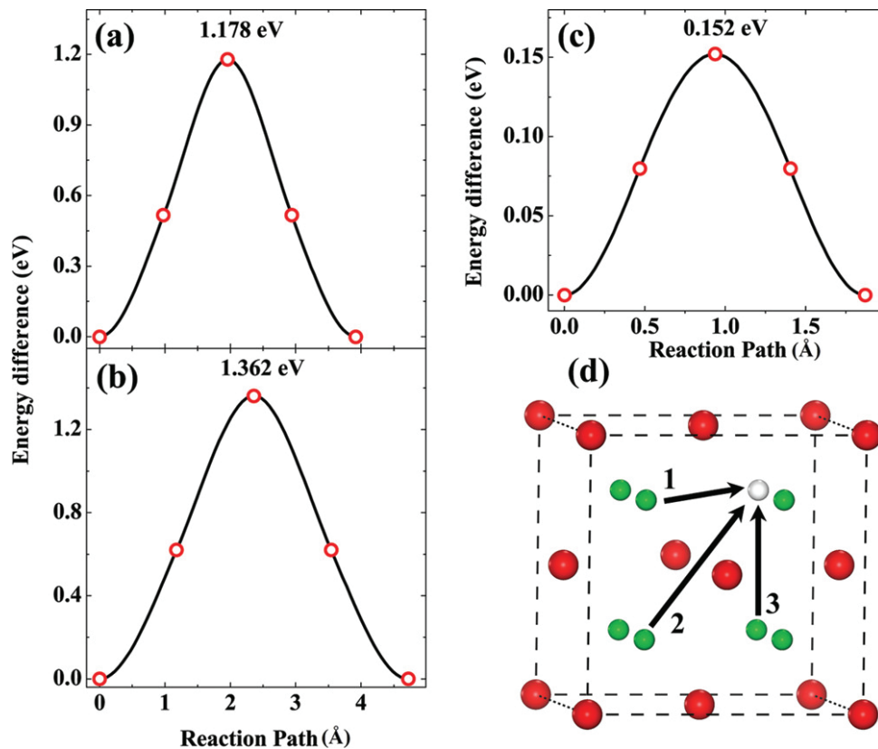
Figure 2.4: (a–c) are energy profiles of different migration pathways of single lithium-ion migration in \text{Li}_2\text{O} . (d) illustrates the cubic structure and migration pathways, marked with arrows. Red and green spheres are O and Li atoms, respectively, and the white sphere indicates the Li vacancy position. Adapted with permission from reference [111]. Copyright 2011 American Chemical Society.
