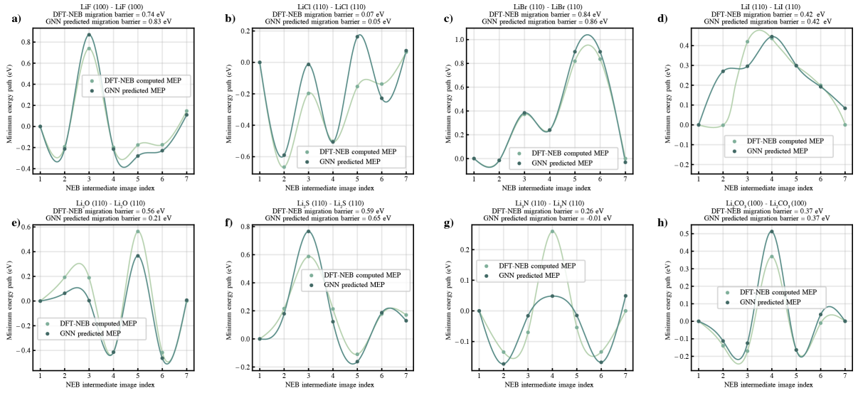
Figure 5.8: Comparison between the MEPs predicted by the GNN model and those obtained from NEB calculations for grain diffusion of (a) LiF (100), (b) LiCl (110), (c) LiBr (110), (d) LiI (110), (e) Li 2 O (110), (f) Li 2 S (110), (g) Li 3 N (110), and (h) Li 2 CO 3 (100). The exposed surface corresponding to each grain is indicated in the brackets. The model achieves a point-wise MEP MAE of approximately 0.05 – 0.08 eV and a migration barrier MAE of about 0.10 eV, which reduces to a range of 0.04 – 0.05 eV when clear outliers reported in the case of Li 2 O and Li 3 N are excluded.
