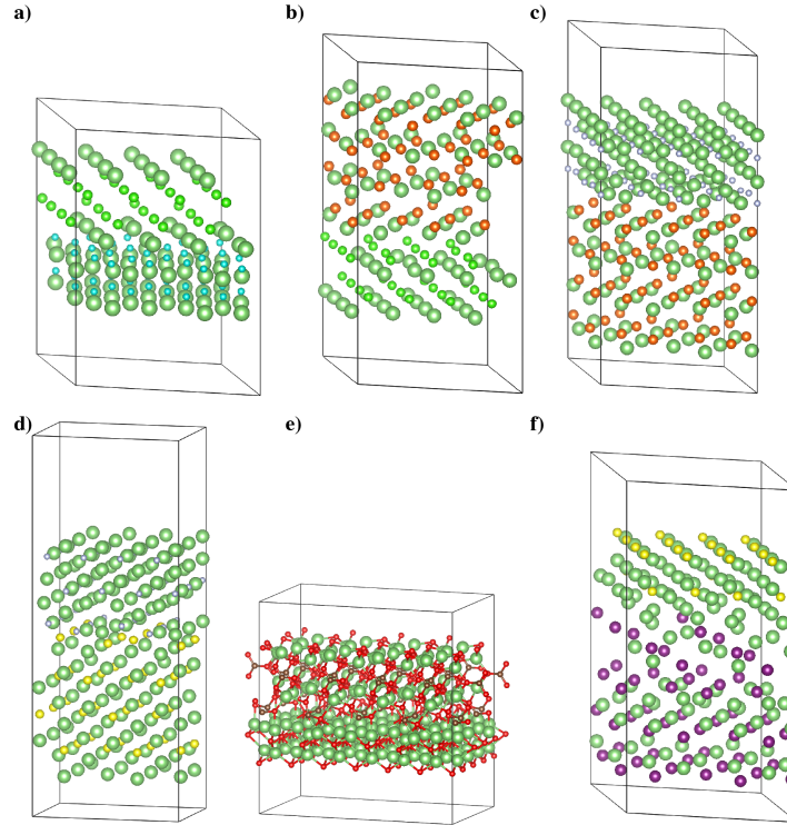
Figure C.9: Representative heterogeneous grain boundaries built using Zur–McGill algorithm for (a) LiF(111)-LiCl(111), (b) LiCl(111)-LiBr(001), (c) LiBr(110)-Li 3 N(100) (d) Li 2 S(001) -Li 3 N(100), (e) Li 2 O(001)-Li 2 CO 3 (100), and (f) LiI(001)-Li 2 S(111).
