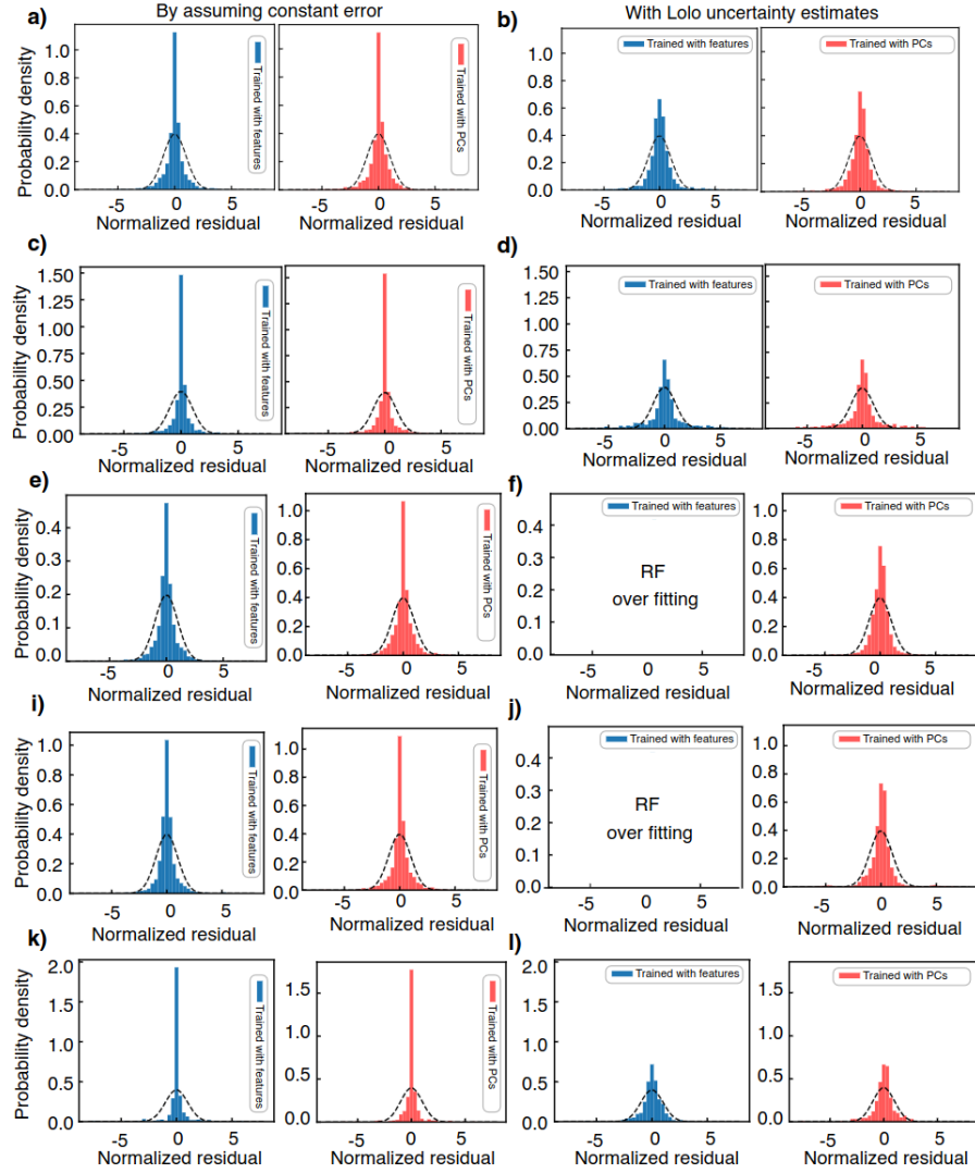
Figure C.5: Probability density distributions of normalized residuals, calculated through eight-fold cross-validation. Each graph set consists of two figures: on the left, it is assumed that all entries have constant error (out-of-bag errors), while on the right, the error distribution is depicted using Lolo uncertainty estimates calculated based on variability and correlation with inclusion of points in their randomly drawn training set. Graph sets a – d illustrate the uncertainty behavior of the impurity and self diffusion models in an IM media, while, graph sets c up to l present the uncertainty behavior of the self, impurity, and chemical diffusion in MCA media.
