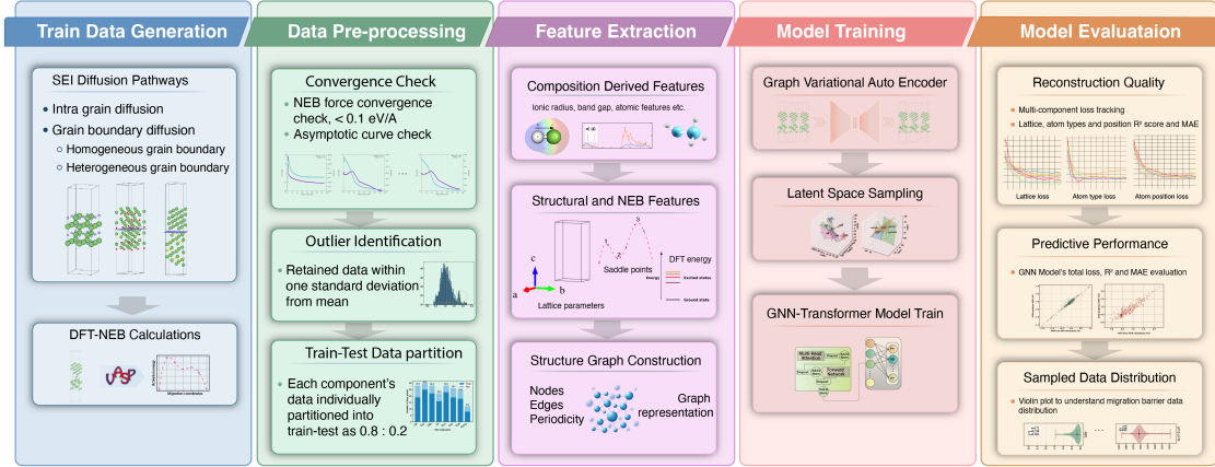
Figure 5.1: Workflow of modeling Li-ion transport in SEI. Diffusion minimum energy path and migration barrier estimated using nudged elastic band method implemented in DFT computational code. Graph variational autoencoder used to augment data and GNN transformer model for predictive modeling.
