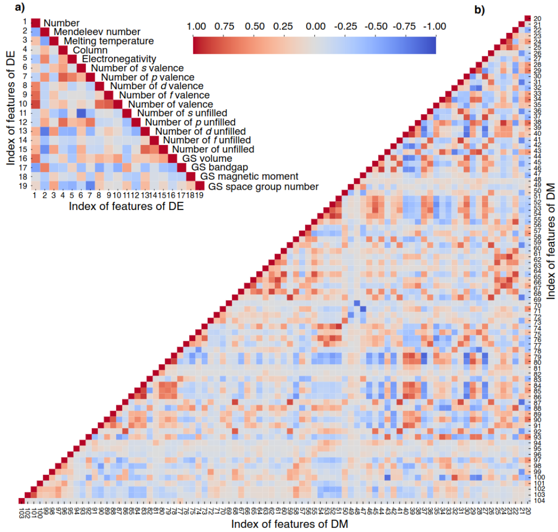
Figure C.7: Correlation values of features of a) diffusing elements and b) diffusion media for the model impurity diffusion in MCA media. Name of features with respective indices are given in Table C.3
