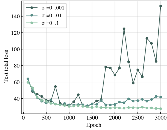
Figure C.12: Latent diffusion noise conditioning: Three trials with noise range 0.1 – 0.001 that used to perturb atomic positions.
