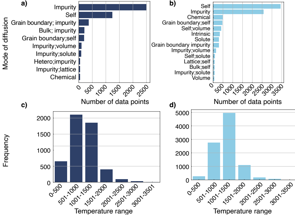
Figure 3.2: Dataset overview: a) diffusion mode present in dataset for IM media and b) MCA media. Frequency of temperature range of diffusion for c) IM media and d) MCA media.
