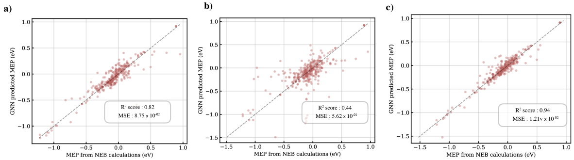
Figure C.16: Comparison of GNN model performance with three training schemes: R^2 scatter plots of training with a) composition derived features, b) GVAE latent embeddings, and c) combined features.
