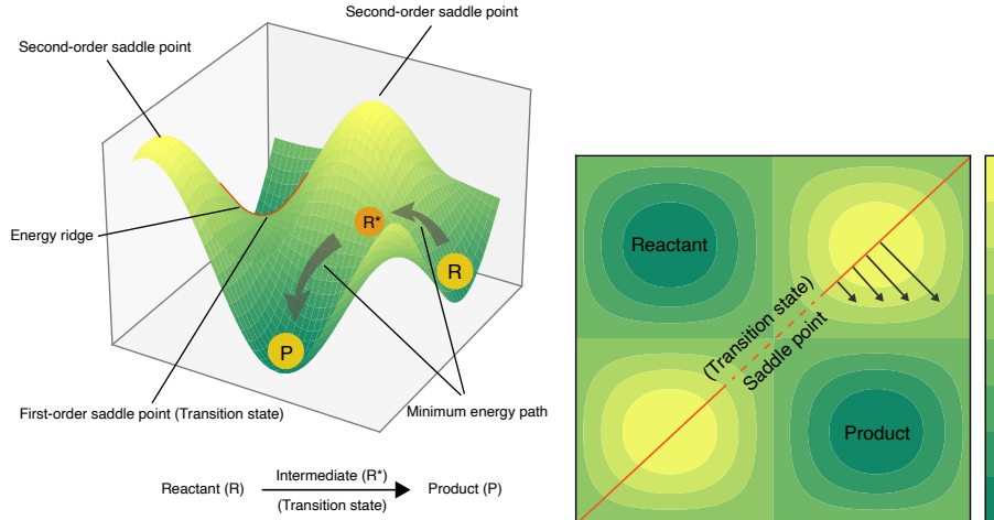
Figure 3.1: Potential energy terrain of a MEP for a chemical reaction[44, 45].
