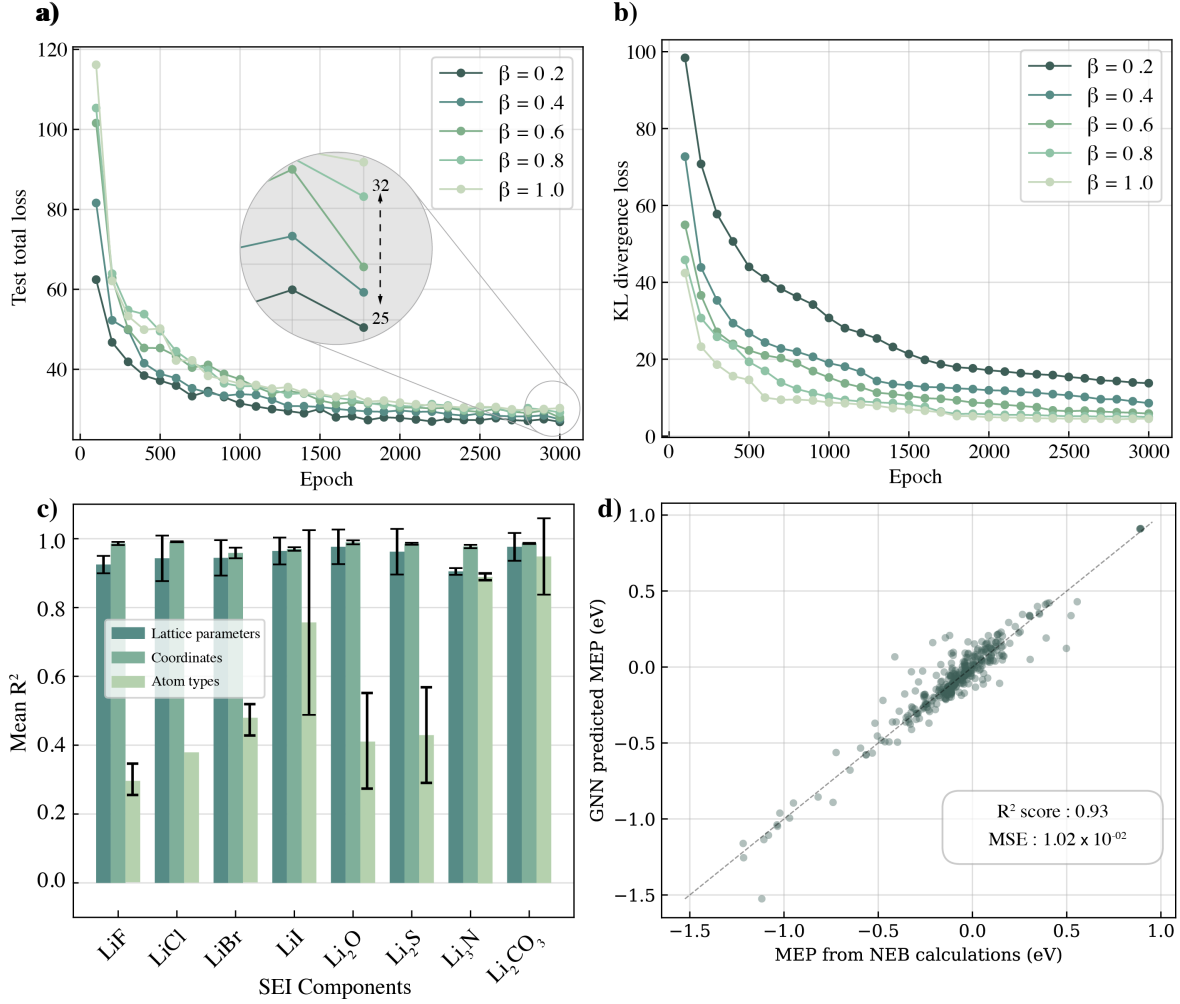
Figure 5.7: For grain diffusion, performance of the GVAE model in terms of convergence of the (a) total test loss and (b) KL divergence for different values of the weighting parameter \beta ranging from 0.2 to 1.0. The reconstruction performance of the GVAE for lattice parameters, atomic coordinates, and atom types is shown in (c), and the corresponding R^2 score for predicting MEP using GNN model is shown in (d).
