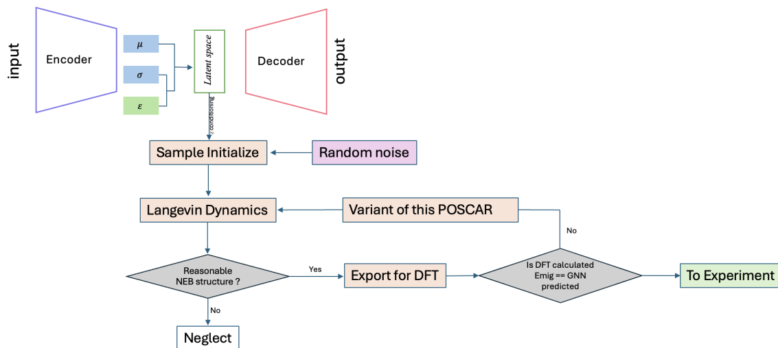
Figure 3.4: Proposed generative modeling workflow for SEI structure generation and Li-ion migration barrier screening. An input structure is encoded into a latent space using a variational autoencoder-based model, followed by random sampling and decoding to generate new POSCAR variants. The generated structures are filtered based on their suitability for NEB calculations, exported for DFT validation, and compared with GNN-predicted migration barriers before being considered for experimental relevance.
