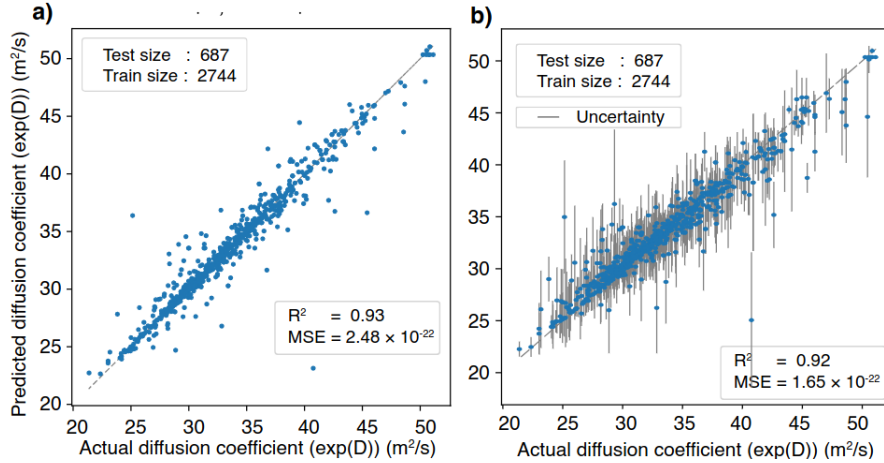
Figure 4.11: Performance of model – self diffusion in MCA media when trained with a) the entire feature space (dimension: 3431 \times 54 ) and with b) the principal components of the entire feature space (dimension: 3431 \times 40 ). The gray solid lines depict the uncertainty associated with each test data point.
