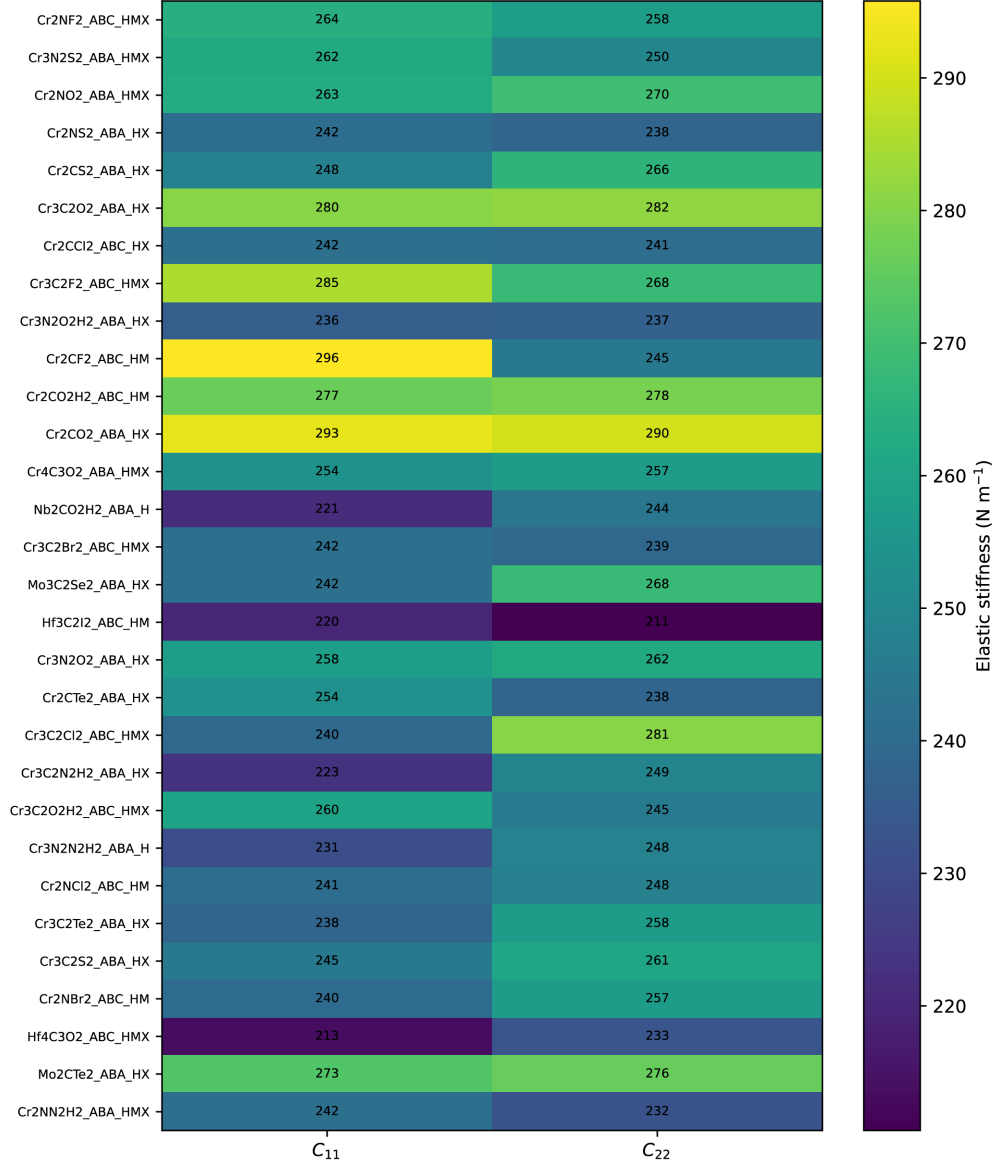
Figure 6.3: C_{11} and C_{22} of top 30 MXene phases along with their stacking orientation (ABA and ABC) and termination hollow-site configurations (H, HM, and HMX).
