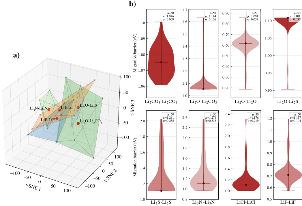
Figure 5.13: Data sampling scheme in latent space: (a) distribution of grain boundary diffusion data for different SEI components in the GVAE latent space, visualized in a 3-D Cartesian basis after t-SNE dimensionality reduction; (b) violin plots of the data generated from the hulls of the respective SEI components. The red dot in each hull indicates the hull center. A few clusters have been illustrated here for a better visualization. Panel (b) shows that grain boundary diffusion generally exhibits higher and more broadly distributed migration barriers compared to bulk, with more variability depending on the specific interface chemistry, particularly for mixed-component boundaries. Due to numerous grain boundary structures involved in the analysis, only important one selected based on migration energy barrier is included in the illustration.
