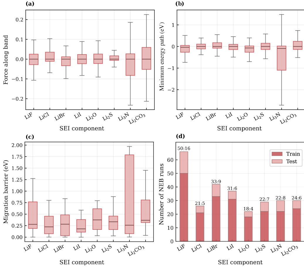
Figure 5.3: Overview of Li-ion grain diffusion through SEI components; a) box plot of average nudged elastic force b) energies of intermediate images in minimum energy path, c) migration barrier and number of NEB runs and their test–train partition in SEI components. Prima facie, lithium halides exhibit comparatively lower migration barriers for grain-boundary diffusion than other SEI components.
