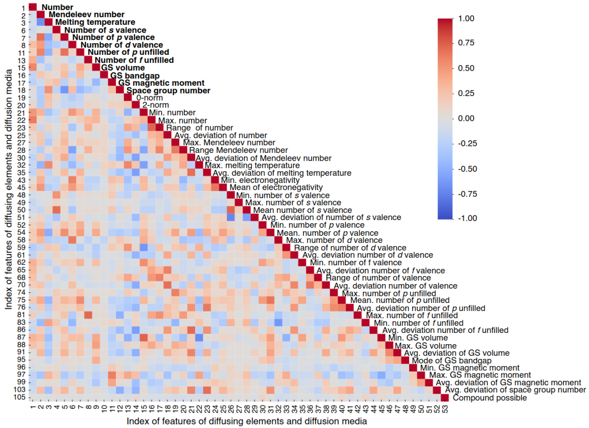
Figure 4.9: Feature space – self diffusion in MCA media: combined feature space of diffusing element and diffusion media used for training. Features of diffusing elements are highlighted in bold fonts and diffusion media in regular fonts (Individual feature space of diffusing element and diffusion media for this model are given in Figure C.6a and b respectively). Common abbreviations such as ‘min.’ for minimum, ‘avg.’ for average, and ‘dev.’ for deviation are used.
