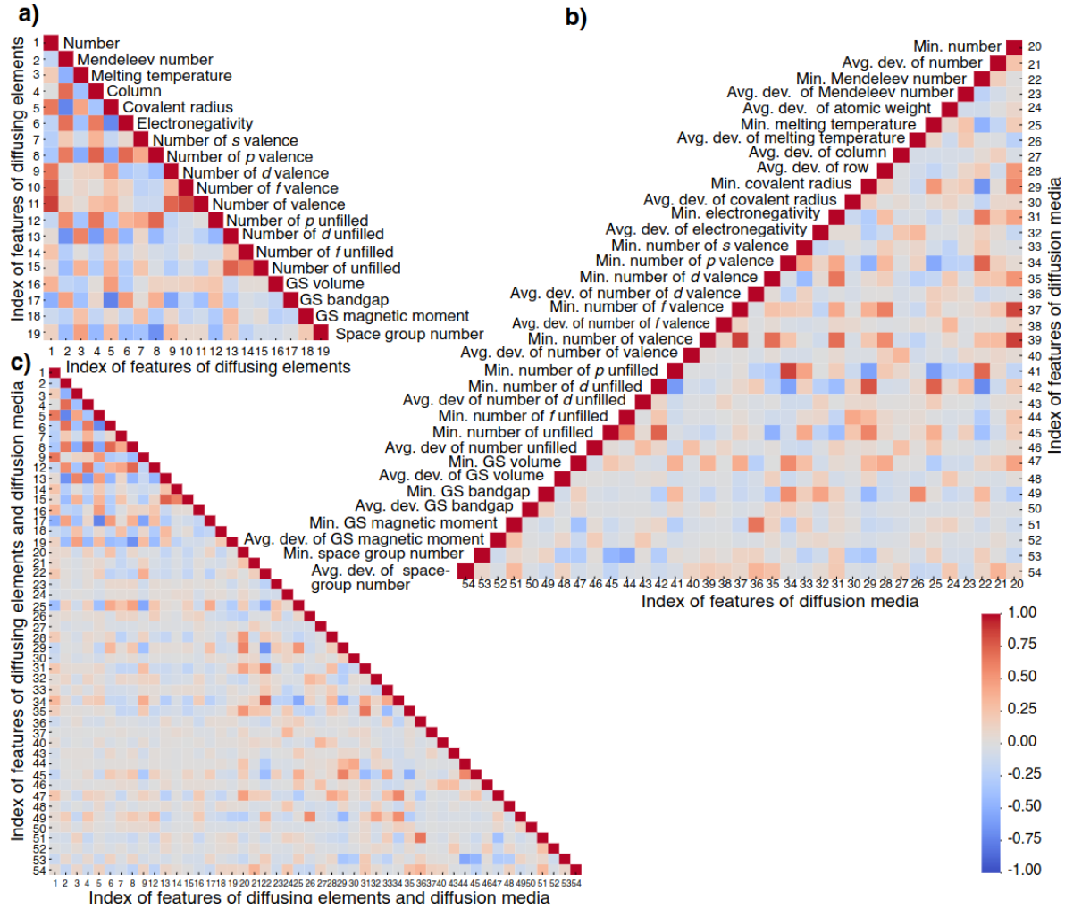
Figure 4.1: Feature spaces – impurity diffusion in IM media for a) diffusing elements, b) diffusion media, and c) the combined feature space used for training. Features of diffusing elements and diffusion media are indexed sequentially and the respective indices are marked in the combined feature space for reference. Common abbreviations such as ‘min.’ for minimum, ‘avg.’ for average, and ‘dev.’ for deviation are used.
