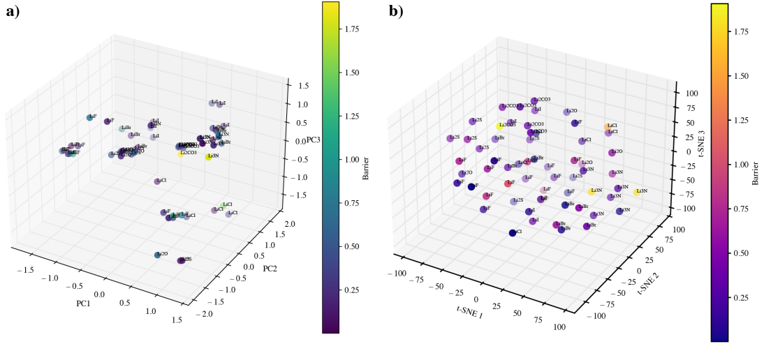
Figure C.14: Visualization of latent space clustering of SEI components using (a) PCA and (b) t-SNE based dimensionality reduction. A clear clustering can be observed in PC space three PCs compared to t-SNE based cluster classification.
