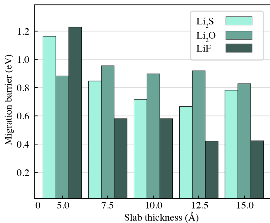
Figure C.17: Convergence test on slab thickness vs migration barrier in Li 2 S, Li 2 O and LiF.
