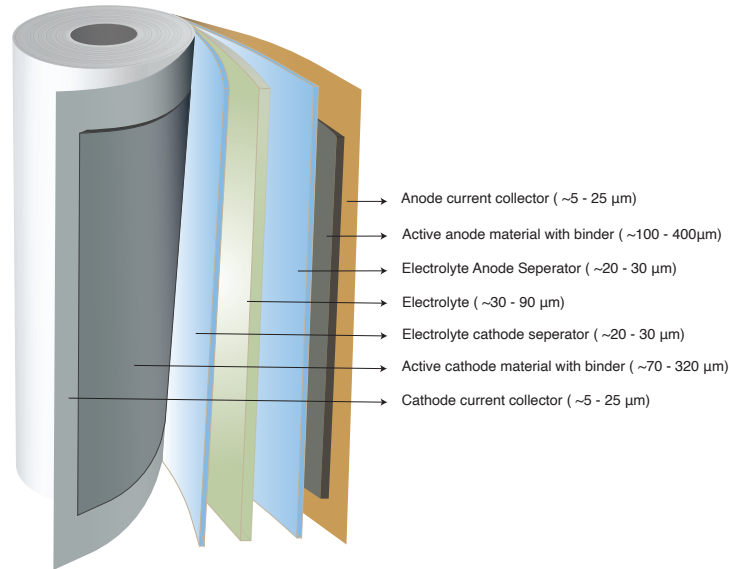
Figure 1.1: An illustration of different layers of a typical Lithium-based battery pack with their relative thickness.
