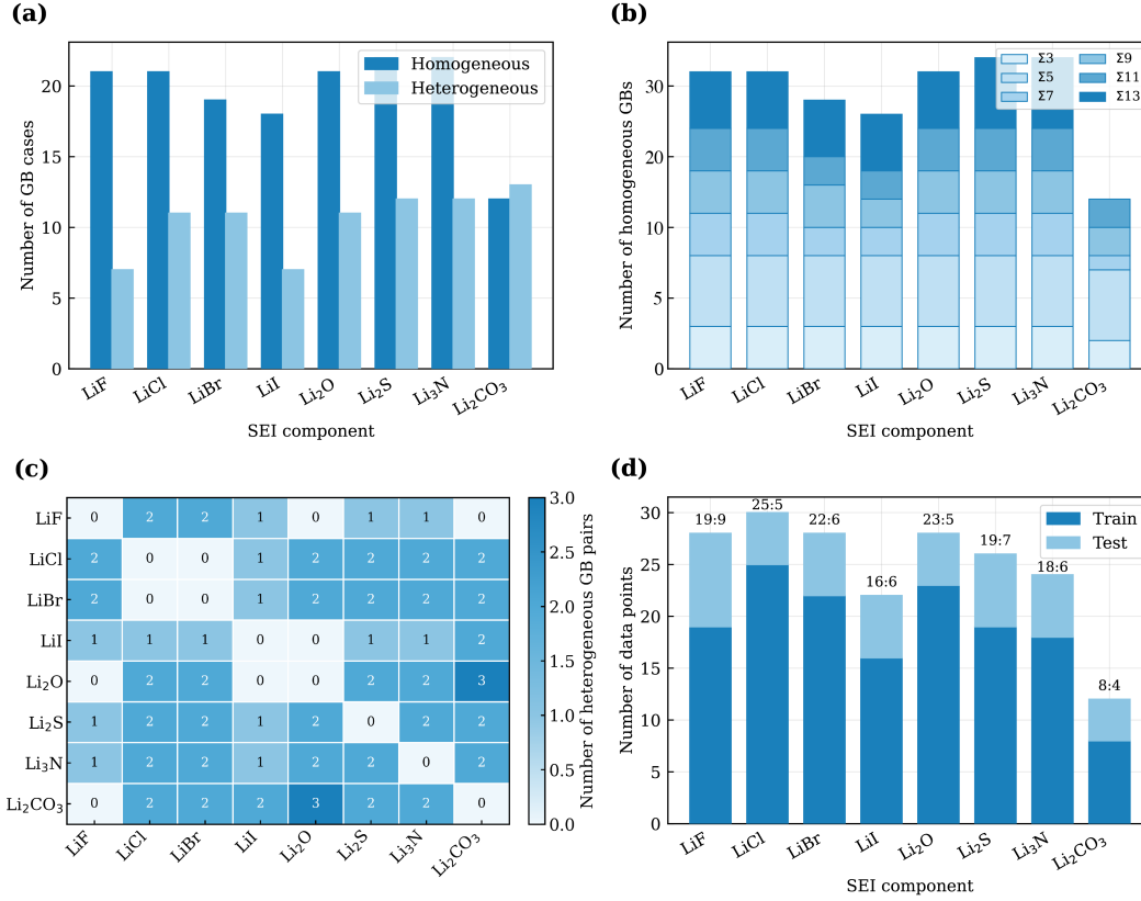
Figure 5.4: Summary of the diffusion dataset generated from grain boundaries formed between SEI components: (a) Numbers of homogeneous and heterogeneous grain boundary diffusion cases for each SEI component, (b) homogeneous grain-boundary structures according to the CSL parameter \Sigma , (c) heterogeneous grain-boundary pairs formed between different SEI components, and (d) train–test split of the total dataset for each SEI component, with the numbers above the bars indicating the corresponding counts of train and test samples used.
