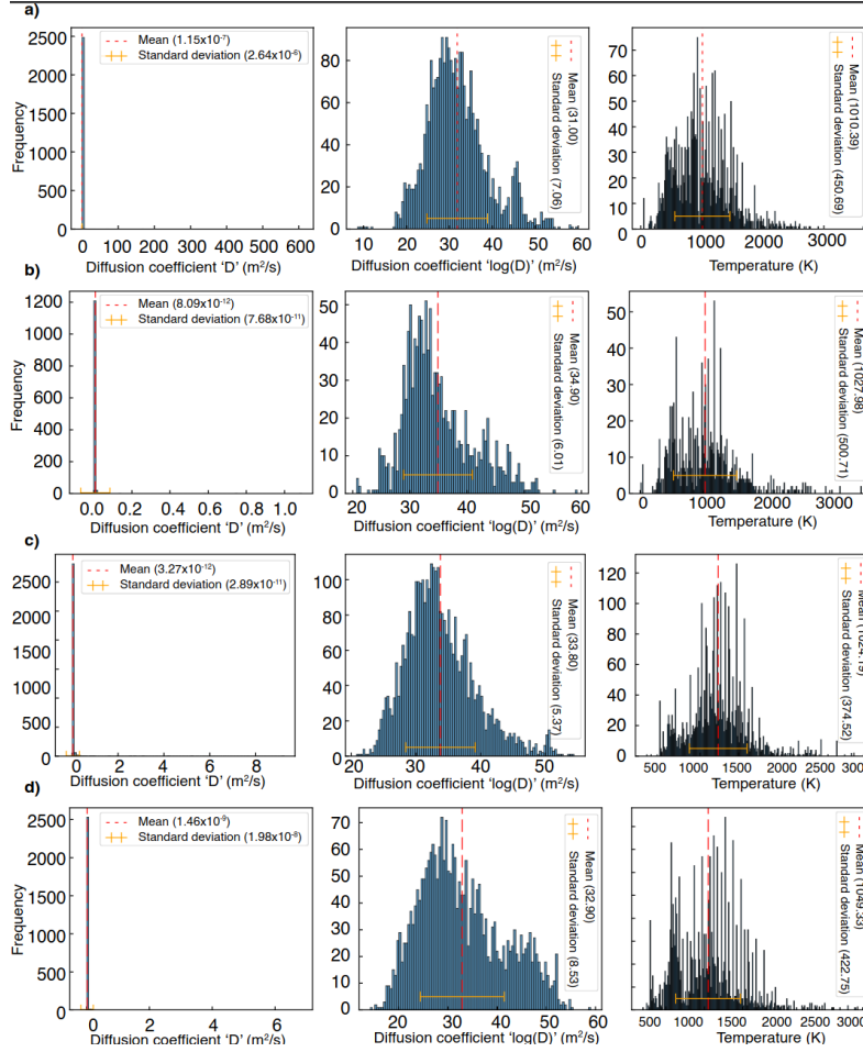
Figure C.4: In each graph set, the leftmost figure represents the standard deviation of the diffusion coefficient, the middle figure illustrates the standard deviation of the diffusion coefficient after taking the logarithm, and the rightmost figure displays the standard deviation of temperature. The data for a) impurity and b) self-diffusion modes in IM media, and impurity, self, and chemical diffusion in MCA media are represented by c), d), and e), respectively.
