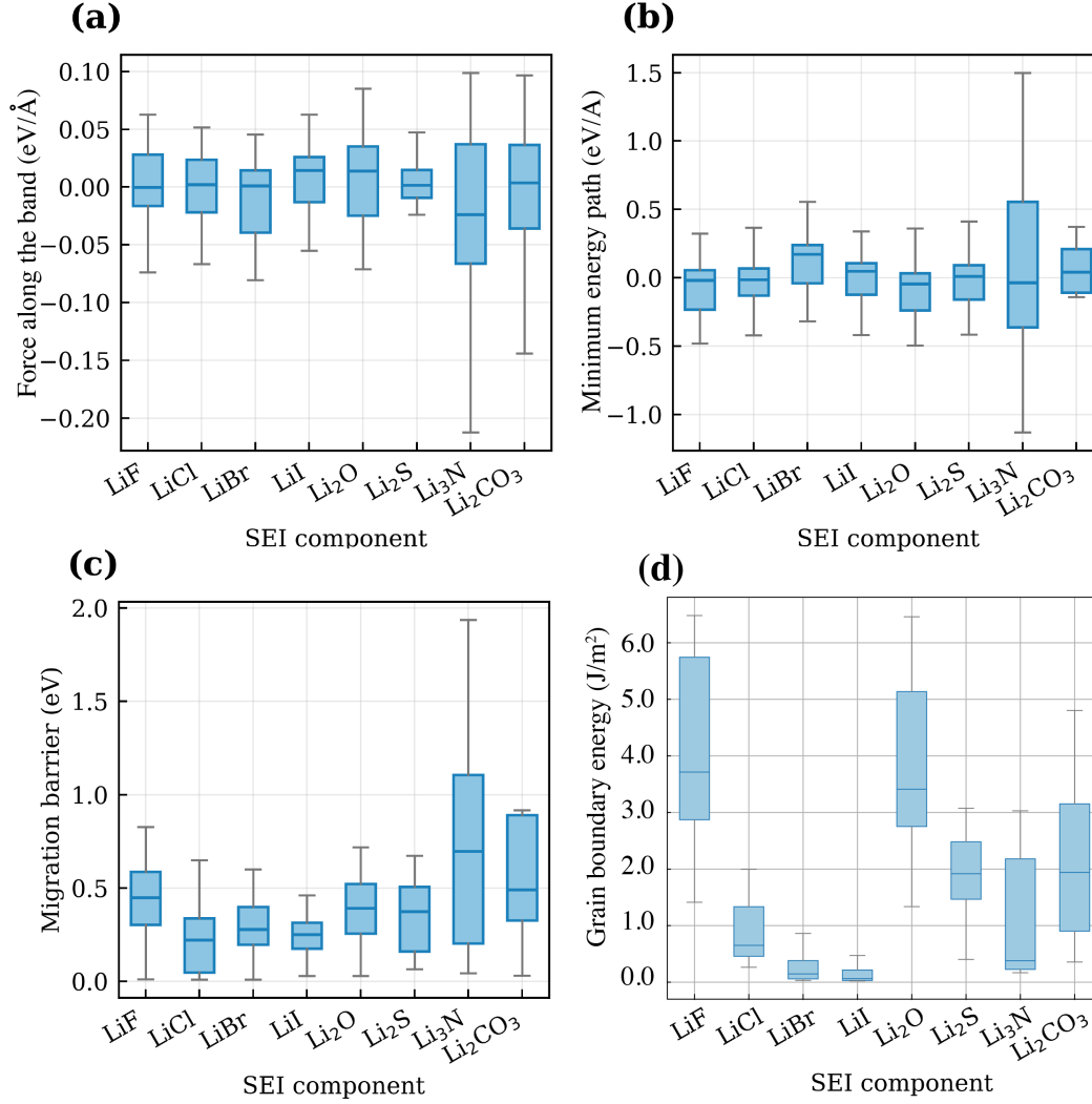
Figure 5.5: Statistical overview of NEB dataset for grain boundary diffusion: Boxplots of the (a) NEB force values along the diffusion pathway for converged NEB images, (b) energies of intermediate images in minimum energy path, (c) Li-ion migration barriers and (d) grain boundary energy. A lower migration barrier in grain boundaries composed lithium halides can be observable, wherein especially LiCl based grain boundary exhibit lower among all other lithium halides.
