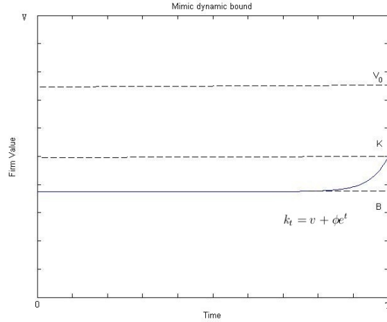
Figure 6.2: Mimic Dynamic bound
