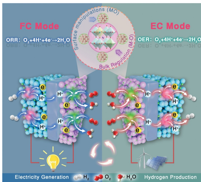
Figure 2.1. Schematic diagram of R-PCEC in fuel cell (FC) and electrolysis cell (EC) operation modes along with the bulk and in-situ surface modification strategy for air electrode [11] .
