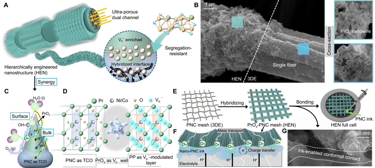
Figure 6.2. Structure, morphology, and oxygen-vacancy-induced lattice structure evolution of the hybrid interface in PrO x -PNC hierarchical structure. (A) Synergistic interaction between PrO x and PNC on the HEN electrode, illustrating the regulation of oxygen vacancy enrichment and its benefit for suppressing segregation. (B) Structure morphology depicting a single fiber in the mesh, showing the pristine part and the hierarchical pre-treatment part (side view and cross-section view). (C) Schematic of the oxygen evolution pathway facilitated by PrO x -decorated PNC functioning as a triple-conducting oxide (TCO). (D) Spatial engineering of V_O distribution across PrO x -PNC heterostructure. PP denotes the PrO x -PNC coupled region. (E) Schematic representation of the fabrication process for the HEN electrode onto the as-prepared half-cell ( \text{BaCe}_{0.7}\text{Zr}_{0.1}\text{Y}_{0.1}\text{Yb}_{0.1}\text{O}_{3-\delta} -BCZYYb7111 [177,226,255] /BCZYYb7111-NiO), employing a two-step approach involving hybridization and bonding. (F) Schematic of coupled charge-mass transfer pathway. The conformal coating of nano-PNC “glue ink” on the inner wall preserves the ultraporous channels for rapid gas/steam diffusion while creating a continuous electronic pathway along the PNC backbone. (G) Micrograph of the HEN steam-electrode showing an ink-enabled
