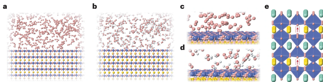
Figure 2.3. Illustrative comparison of oxygen electrode operating conditions in SOECs and PCECs. (a) Surface of the oxygen electrode material exposed to O_2 in SOECs. (b) Surface of the oxygen electrode material exposed to a H_2O/O_2 mixture with a high steam concentration in PCECs. (c-d) Enlarged views of the surface areas from a (c) and b (d), showing interactions between the surface of the oxygen electrode material and O_2 or H_2O molecules. In a–d, red and white spheres represent oxygen and hydrogen atoms, respectively, whereas yellow and blue spheres denote cations in the oxygen electrode materials. (e) Lattice structure of a layered double perovskite AA'BO_{5+\delta} with oxygen migration channels indicated by the red arrows. Atoms on A and A' sites are depicted by yellow and green spheres, respectively; cations on B sites are represented by the blue polyhedral units; oxygen atoms are shown as red spheres [20] .
