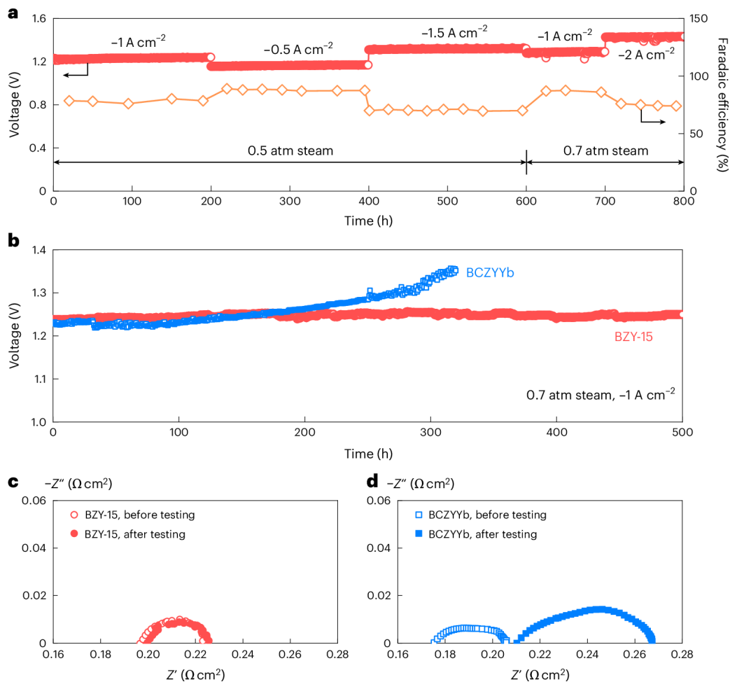
Figure 2.25. Stability under high-steam pressure electrolysis. (a) Cell voltage and Faradaic efficiency during long-term PCEC operations of BZY-15 cell at 600 °C. Feedstock for fuel electrode: pure \text{H}_2 . Other testing conditions are specified in the main text. (b) Cell voltage during long-term PCEC operations of BZY-15 and BCZYYb cells at -1 \text{ A cm}^{-2} and 0.7 atm steam at 600 °C. Feedstock for fuel electrode: pure \text{H}_2 . (c) EIS measured at a d.c. bias of -1 \text{ A cm}^{-2} before and after 500 h of testing of the BZY-15 cell in (b). (d) EIS measured at a d.c. bias of -1 \text{ A cm}^{-2} before and after 320 h of testing of the BCZYYb cell in (b) [139] .
