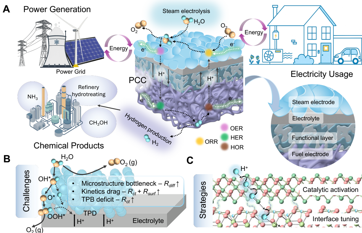
Figure 6.1. PCCs energy pathway: from grid electricity to hydrogen and chemicals. (A) Integrated schematic of reversible PCCs operation with its applications on power grid and chemical production. (B) Challenges at the steam-electrode/electrolyte interface in terms of microstructure, kinetics and TPB. (C) Strategies to boost PCCs' performance. Catalytic activation accelerates surface reactions; interface tuning engineers defect coherence to widen TPB contact and facilitate proton migration, as indicated by the dashed pathway.
