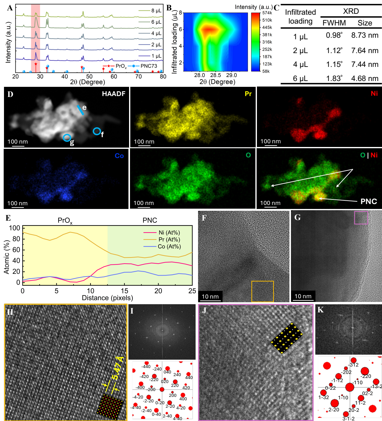
Figure 4.3. In-depth characterization of the hybrid Type VI electrode through XRD and TEM analysis. (A) XRD of hybridized electrode powders with different infiltrated loadings. (B) Selected XRD range to indicate (111) crystalline plane of as-infiltrated \text{PrO}_x on different loaded
