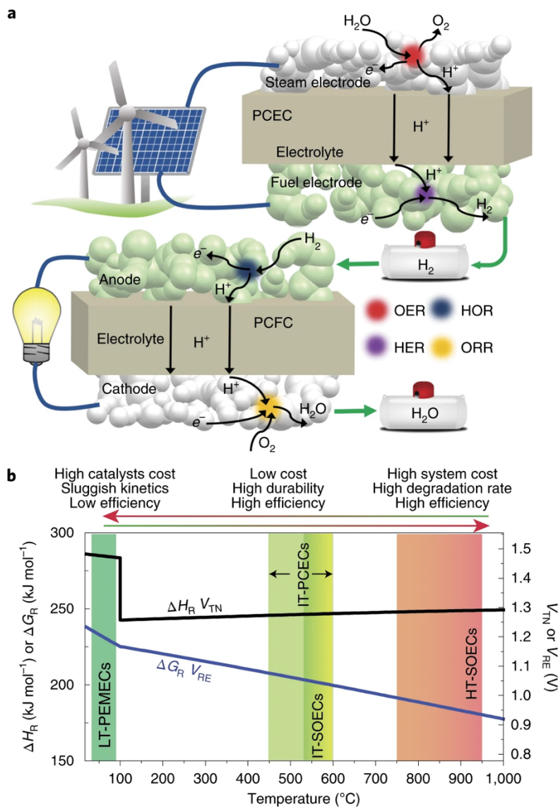
Figure 2.2. Schematic of RePCECs and comparison with low-temperature proton exchange membrane electrolysis cells, intermediate-temperature solid oxide electrolysis cells and high-temperature solid oxide electrolysis cells. (a) Schematic of the RePCEC: a reversible energy storage device that can operate in both fuel cell and electrolysis modes. OER, oxygen evolution reaction; ORR, oxygen reduction reaction; HOR, hydrogen oxidation reaction; HER, hydrogen evolution reaction. (b) Thermodynamics of water electrolysis as a function of temperature. \Delta G_R is correlated with the reversible voltage ( V_{RE} ) while \Delta H_R is correlated with thermal neutral voltage ( V_{TN} ) in electrolysis mode. \Delta G_R and V_{RE} share the same plot and different y axes. \Delta H_R and V_{TN} share the same plot and different y axes. PEMECs, proton exchange membrane
