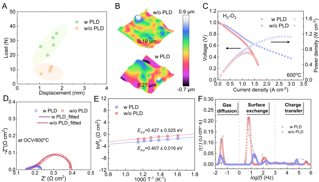
Figure 5.4. Interfacial reinforcement and polarization reduction enabled by PLD. (A) Shear-force measurements of cells without and with PLD, showing a ~3-fold increase in interfacial mechanical robustness after PLD interlayer formation. (B) AFM surface topography of cells without and with PLD, illustrating increased surface roughness and enhanced contact area. (C) I–V and power-density curves at 600 °C in H 2 –O 2 . (D) Nyquist plots measured at OCV and 600 °C in H 2 –O 2 , showing reduced polarization with PLD. (E) Arrhenius plots of R_p with linear fits, from which apparent activation energies are extracted, revealing lower effective kinetic barriers. (F) DRT spectra derived from EIS at 600 °C, deconvoluting gas diffusion, surface exchange, and charge-transfer contributions, and highlighting suppression of dominant interfacial kinetic losses.
