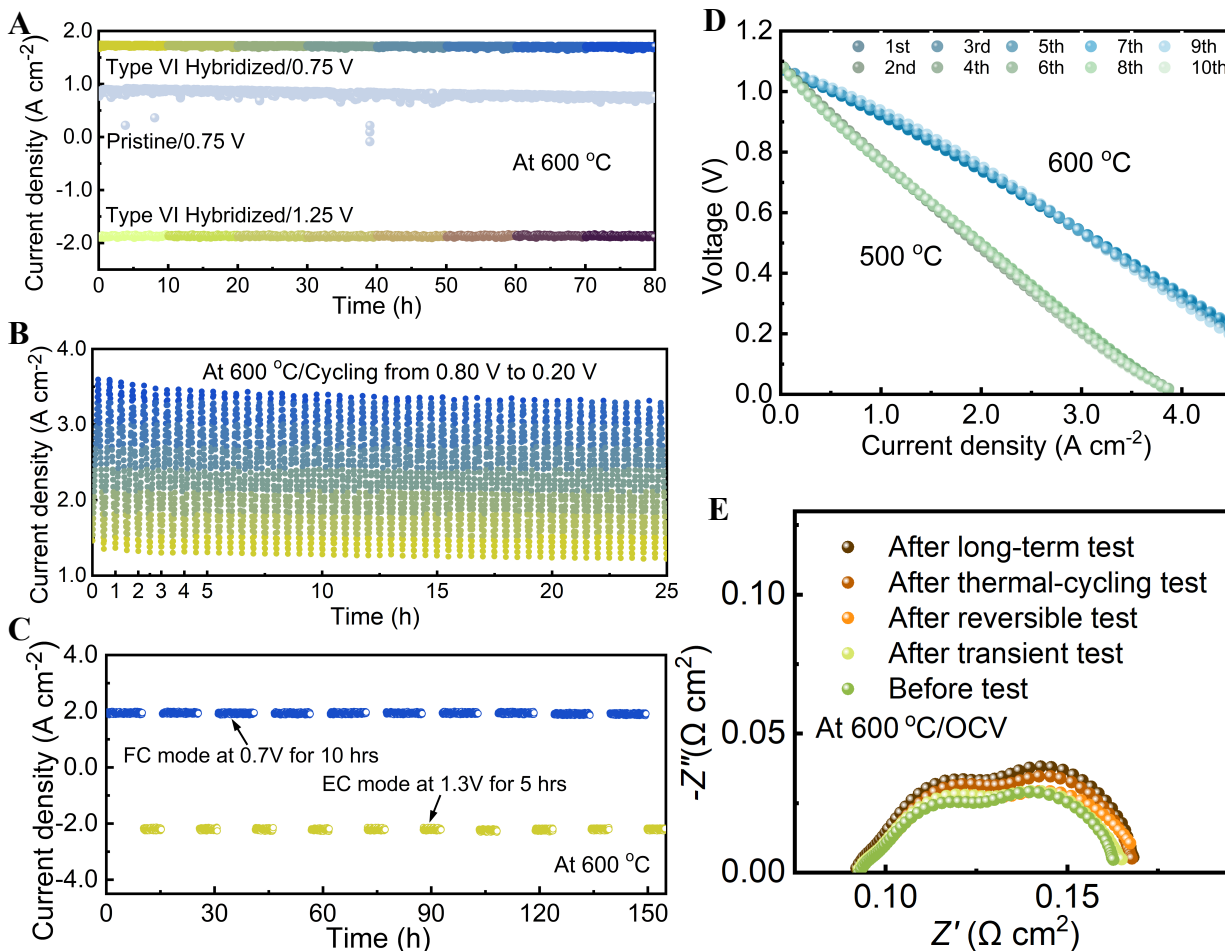
Figure 4.6. Exceptional stability and durability of the hybrid Type VI electrode full cells in both fuel cell and electrolysis modes. (A) Long-term stability tests for 80 hours at 0.75 V for full cell mode and at 1.25 V for 20% steam electrolysis at 600°C, with contrast to the pristine PNC full cells under identical test conditions of full cell mode. (B) Transient tests (time-interval based) under fuel cell mode between 0.80 V and 0.20 V. A cycle (from 0.8 V to 0.2 V, and then back to 0.8 V) lasted for 0.5 hour. (C) Reversible tests between fuel cell mode at 0.70 V and electrolysis mode at 1.30 V for 10 cycles. Each cycle consisted of operating in fuel cell mode for 10 hours, followed by 5 hours in 20% steam electrolysis mode, with a 15-minute transition between the two modes. (D) I - V curves of fast-changing thermal cycling tests at 600 and 500°C for 5 cycles. (E) Corresponding EIS spectra collected before any test and after multiple durability tests.
