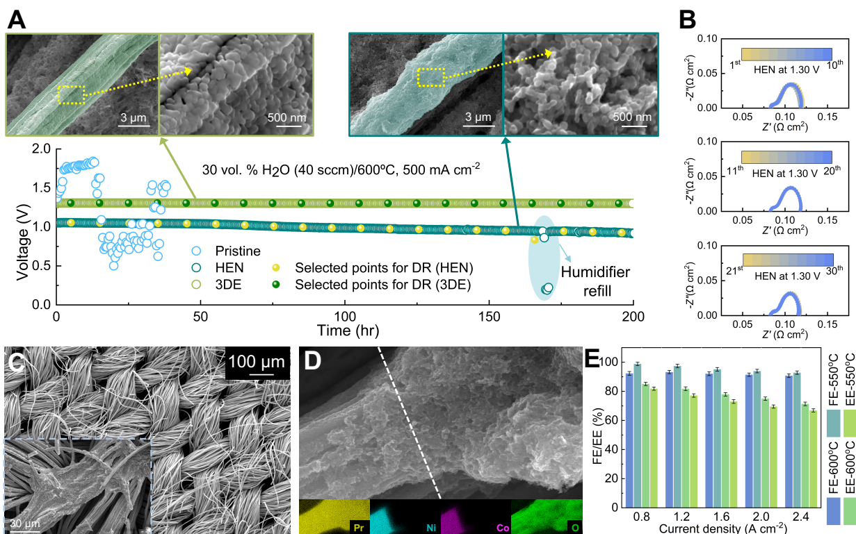
Figure 6.4. Electrochemical performance and structural stability of a PCC incorporating the HEN electrode. (A) Long-term galvanostatic durability, showing superior stability of the HEN architecture compared to pristine and 3DE counterparts, attributed to its optimized morphology (inset: corresponding SEM images). (B) Impedance spectra measured at 1.30 V over 30 cycles, indicating consistent interfacial properties over extended operation. (C) SEM image of interwoven mesh fibers in 3DE electrode, illustrating mass and charge transport pathways; inset shows the region after hierarchical hybridization. (D) SEM images of a single 3DE mesh fiber before (left) and after (right) hierarchical pretreatment with corresponding elemental EDX mapping. (E) Faradaic and energy efficiencies of HEN cells across different temperatures, highlighting enhanced catalytic effectiveness.
