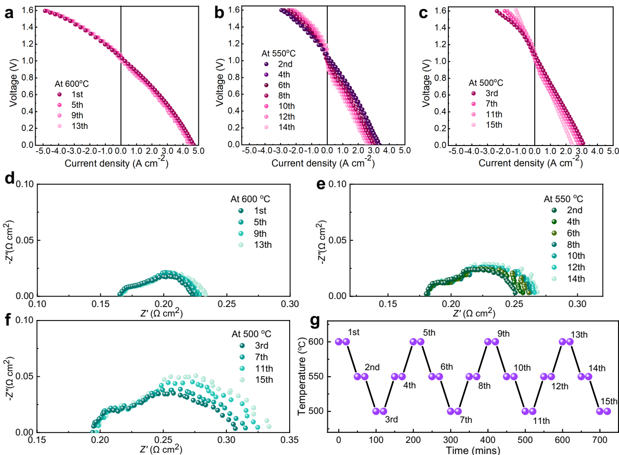
Figure 3.7. Thermal cycle stability evaluation of NAUP-PNC electrode under both fuel cell and electrolysis modes, explicated by dynamically operation across different temperatures. (a-c) I-V curves of fast-changing thermal cycling tests at 600, 550, 500 °C respectively. (d-f) Corresponding EIS curves at 1.30 V of fast-changing thermal cycling tests at 600, 550, 500 °C respectively. H 2 (20 sccm) was used for the anode and O 2 (40 sccm) for the electrode in fuel cell mode. Electrolysis mode was implemented for the anode using H 2 (20 sccm) and the electrode using 20 vol.% H 2 O + 80 vol.% O 2 (40 sccm). (g) Illustration of the complete thermal cycling
