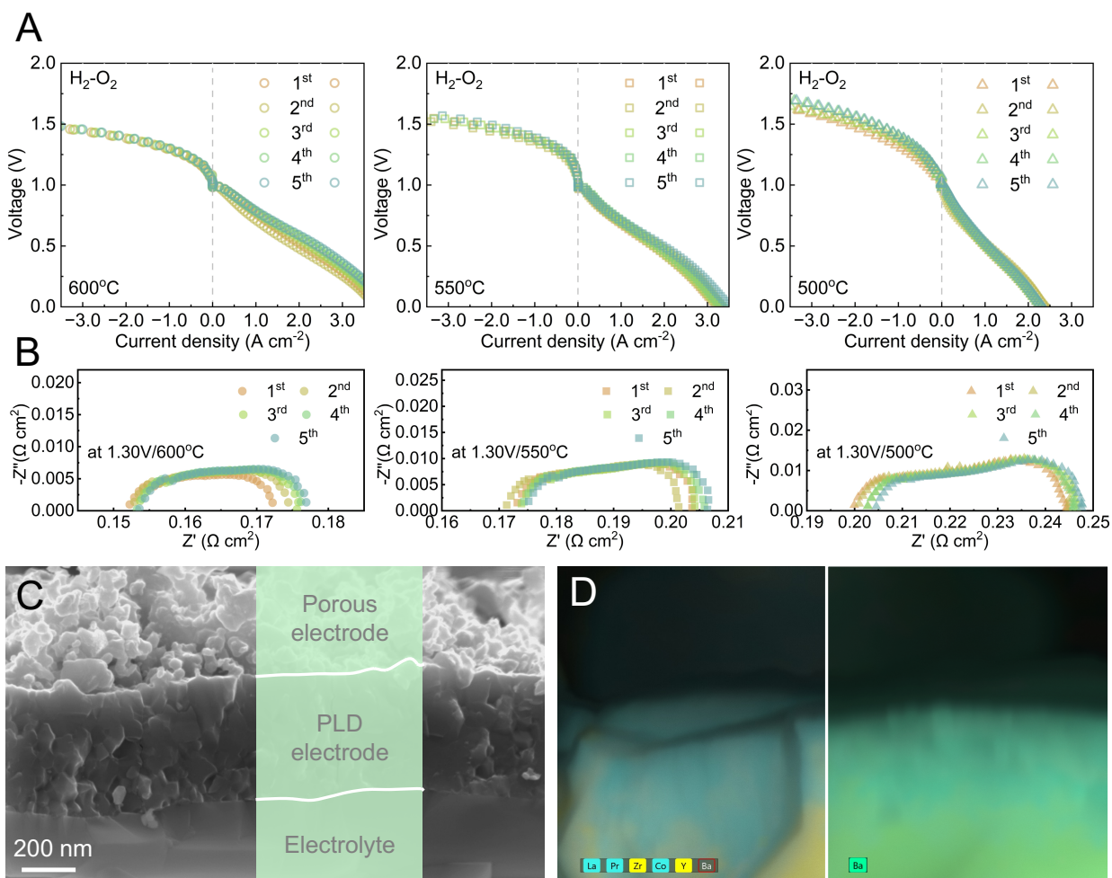
Figure 5.7. Stable reversible performance enabled by a robust bilayer interface under steam and repeated thermal cycling. (A) Polarization curves collected in \text{H}_2\text{-O}_2 for repeated thermal
