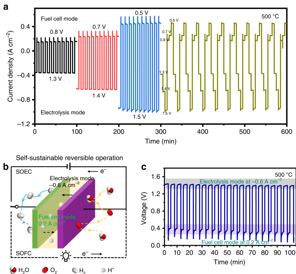
Figure 2.24. Reversible operation and analysis in hydrogen and power generation. The cycling reversible operation of the electrochemical cell between electrolysis mode (hydrogen production) and fuel cell mode (electricity generation) at different current densities to examine the capability of converting hydrogen generated by electrolysis into electricity. (a) Reversible operation with external hydrogen supply: current density responses as working mode transiently changing between electrolysis and fuel cell at 500 °C. (b) Schematic of self-
