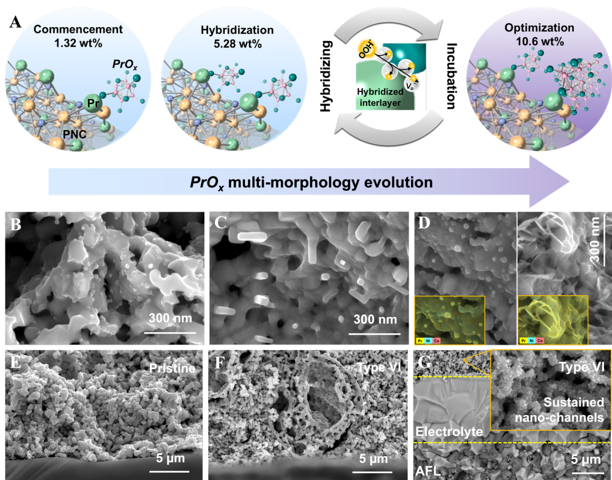
Figure 4.2. Schematic of the readily hybridized electrode and its characterizations. (A) Procedures for the incubation and hybridization of the PNC- \text{PrO}_x electrode. (B-D) Evolution of \text{PrO}_x morphology: (B) commencement with nanoparticles, (C) hybridization with nanobars, and (D) optimization with coexisting nanoparticles and nanowires (with inset showing compositional distribution; yellow for Pr, sky blue for Ni and peachy pink for Co). (E) Electrode/electrolyte interface of pristine PNC backbone. (F) Electrode/electrolyte interface of the hybridized electrode (Type VI, 6 \mu\text{L} ), showing the porous structure. (G) Cross-section of the post-stability test single cell, highlighting sustained nano-channels on the hybridized electrode.
