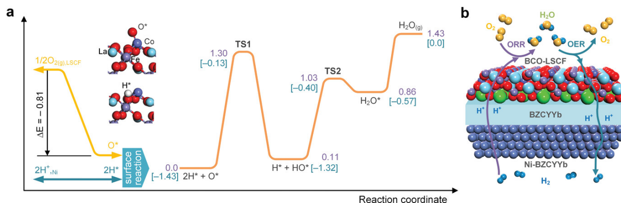
Figure 2.17. (a) Schematic of the energy profile for the fuel cell and water electrolysis modes on LSCF (001). “*” denotes an adsorbed species on the surface. TS1 and TS2 are transition states. The energies in brackets are for the water electrolysis mode. In this reaction scheme, a Co ion on
