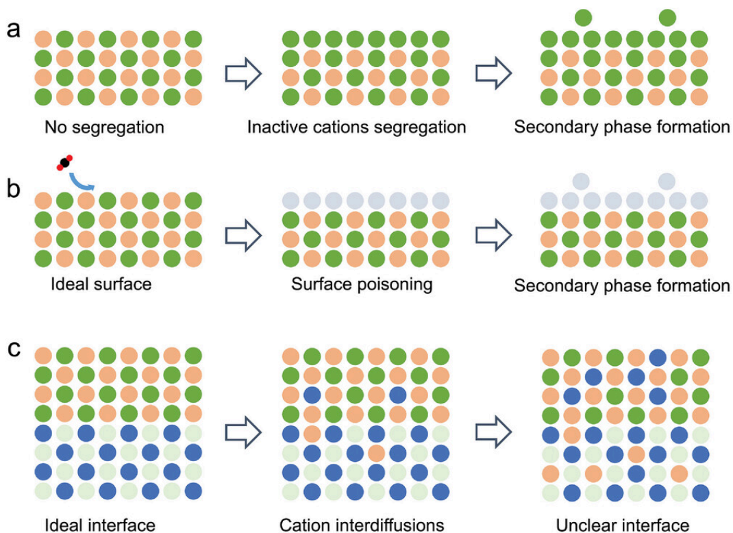
Figure 2.8. Schematic illustration of (a) inactive cation surface segregation, (b) surface poisoning, and (c) cation interdiffusions [51] .
