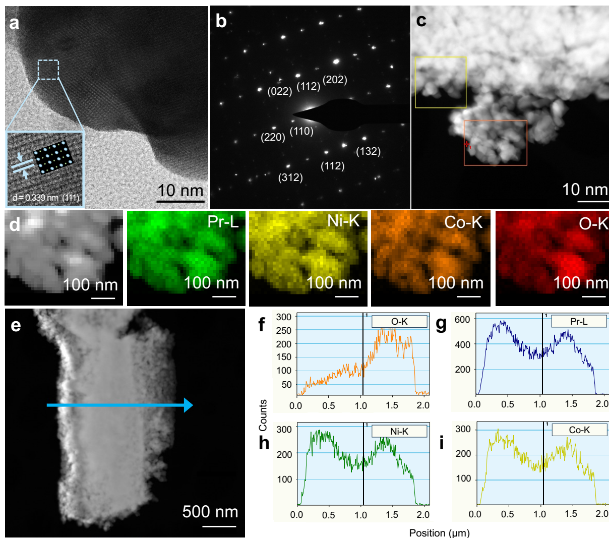
Figure 3.2. TEM characterization of NAUP-PNC oxygen electrode. (a) HRTEM image of NAUP-PNC nanoparticles. The inset contains magnified view of the marked region with a simulated atomic model of the PNC phase (orthorhombic perovskite structure, Pnma space group). (b) SAED pattern of NAUP-PNC nanoparticles. (c) HAADF image of NAUP-PNC nanoparticles; the representative areas are squared. (d) EDS elemental maps of the NAUP-PNC electrode confirm the presence of the PNC phase. From left to right, the selected area for EDS (orange rectangle in Fig. 3C) shows praseodymium as a green pattern, nickel as a yellow pattern, cobalt as an orange pattern, and oxygen as a red pattern, arranged in order. (e) EDS line scan (blue arrow) of a single NAUP-PNC electrode fiber. (f-i) Elemental information of line scan, oxygen-orange (f); praseodymium-blue (g); nickel-green (h) and cobalt-yellow (i).
