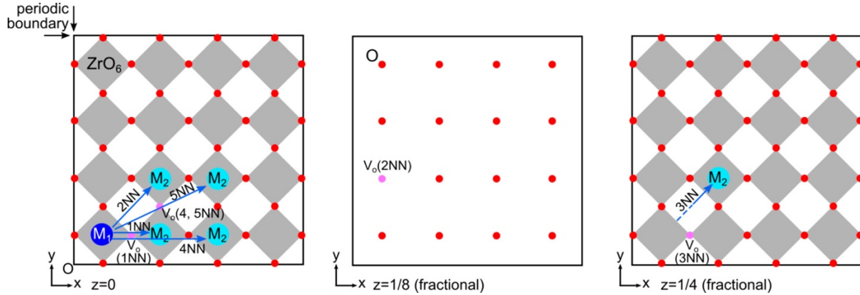
Figure 2.4. Schematic representation of (2MZr', VO^{\bullet\bullet}) configuration for the calculation of total energy. M1 and M2 denote two doped trivalent cations. The VO^{\bullet\bullet} site is equidistant and the nearest from the two M cations in each M–M configuration (1–5NN). 2NN and 3NN sites locate on a plane with different z-coordinates of 1/8 and 1/4, respectively [33] .
