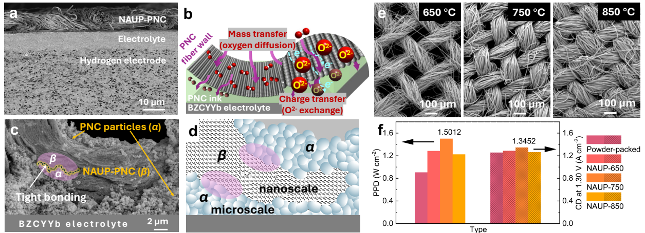
Figure 3.4. Illustration of the integrated NAUP PNC electrode and hybrid structure for optimal dual mass/charge transfer and interfacial strength in PCEC. (a) SEM image of cross section of as-fabricated NAUP-PNC/BZCYYb4411/BZCYYb4411-NiO “sandwiched” structure. Despite the use of a mesh-structured electrode, a strong and secure bonding between the electrode layer and electrolyte is still seen, with no evident signs of delamination. (b) Schematic illustration of occurrence of charge and mass dual-transfer through the single NAUP-PNC fiber inner wall to slight loading of PNC glue ink, ultimately to the electrode/electrolyte interface under the fuel cell mode. During the former fabrication, 10 μl PNC73 ink for certain electrode area (0.178 cm 2 ) was used to achieve refined bonding (Figure 3.1a, Step 3). (c) SEM image of single mesh fiber section, verifying the tight bonding between PNC73 particles (α) and NAUP-PNC structure (β). (d) Schematic illustration of enhanced bonding existing between α (microscale) and β (nanoscale). (e) SEM images of mesh calcinated at 650°C, 750°C and 850°C. (f) Bar chart of the comparison on the PPD and CD at 1.30 V at 600°C for different meshes.
