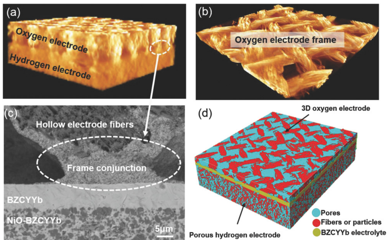
Figure 2.12. (a) 3D X-ray microscopic image for the cell consisting of hydrogen electrode (bottom layer), electrolyte (invisible) and 3D steam electrode (top layer). (b) The bulk electrode frame with hierarchical gaps, which would facilitate fast mass transfer; (c) SEM image for the cross section of the cell shows the contact area between steam electrode frame and electrolyte and (d) reconstructed 3D image for the cell with dimension of 0.4 \times 0.4 \times 0.1 \text{ mm}^3 . Three layers of cell components, that is, fibrous PBSCF electrode with a porosity of 57.7%, dense BZCYYb electrolyte, and sponge-like pore Ni-BZCYYb hydrogen electrode support, are obviously distinguished [78] .
