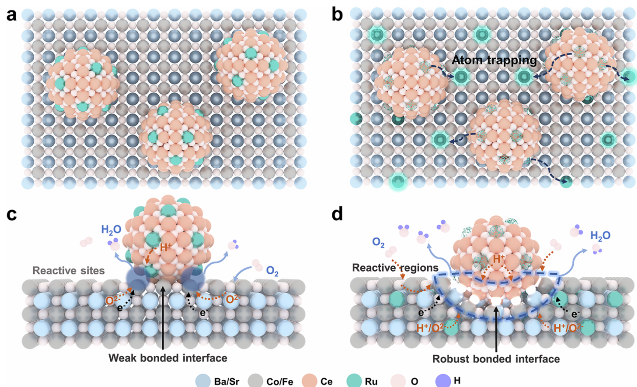
Figure 2.13. Schematic illustration of atom trapping. (a, b) Distribution of Ru element in heterogeneous catalyst before and after heat treatment. (c, d) Heterogeneous interface structure before and after atom trapping [79] .
