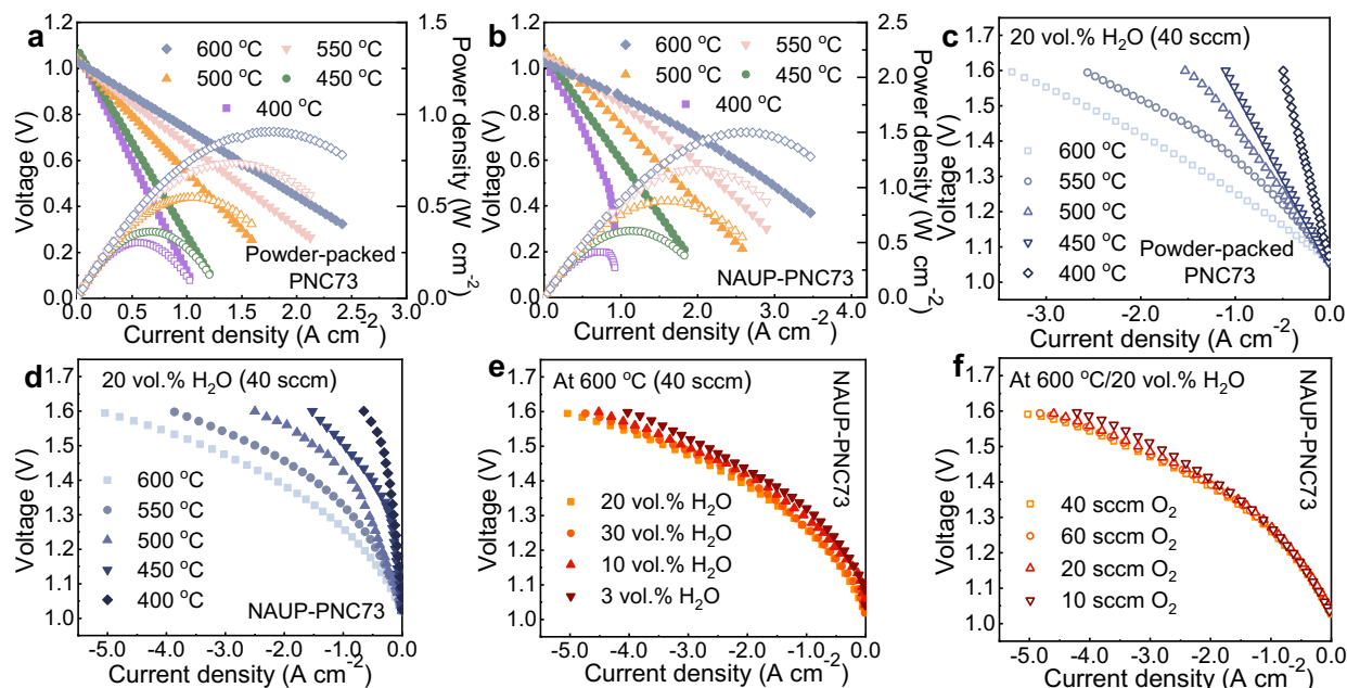
Figure 3.5. Electrochemical performances of NAUP-PNC73 full cells in both fuel-cell and electrolysis modes as compared to full cells with conventional powder-packed electrodes. (a) I - V - P curves of the cell with a conventional powder-packed PNC73 electrode measured at 400-600 °C. (b) I - V - P curves of a representative NAUP-PNC73 cell at 400-600 °C. (c) Polarization curves of a powder-packed PNC73 cell in electrolysis mode at 400-600 °C. H 2 (20 sccm) and 20 vol.% H 2 O + 80 vol.% O 2 (40 sccm) was fed to the electrode. The applied voltage for all tests ranged from 1.60 V to OCV. (d) Polarization curves of a NAUP-PNC73 cell in electrolysis mode at 400-600 °C. (e) Comparison of electrolysis performance of NAUP-PNC73 in terms of different vol.% H 2 O in O 2 at the flow rate of 40 sccm and 600 °C. (f) Comparison of electrolysis performance of NAUP-PNC73 in terms of different flow rate of O 2 at 600 °C. All tests conducted were under the same relative humidity of O 2 , which was 20 vol.% H 2 O in O 2 .
