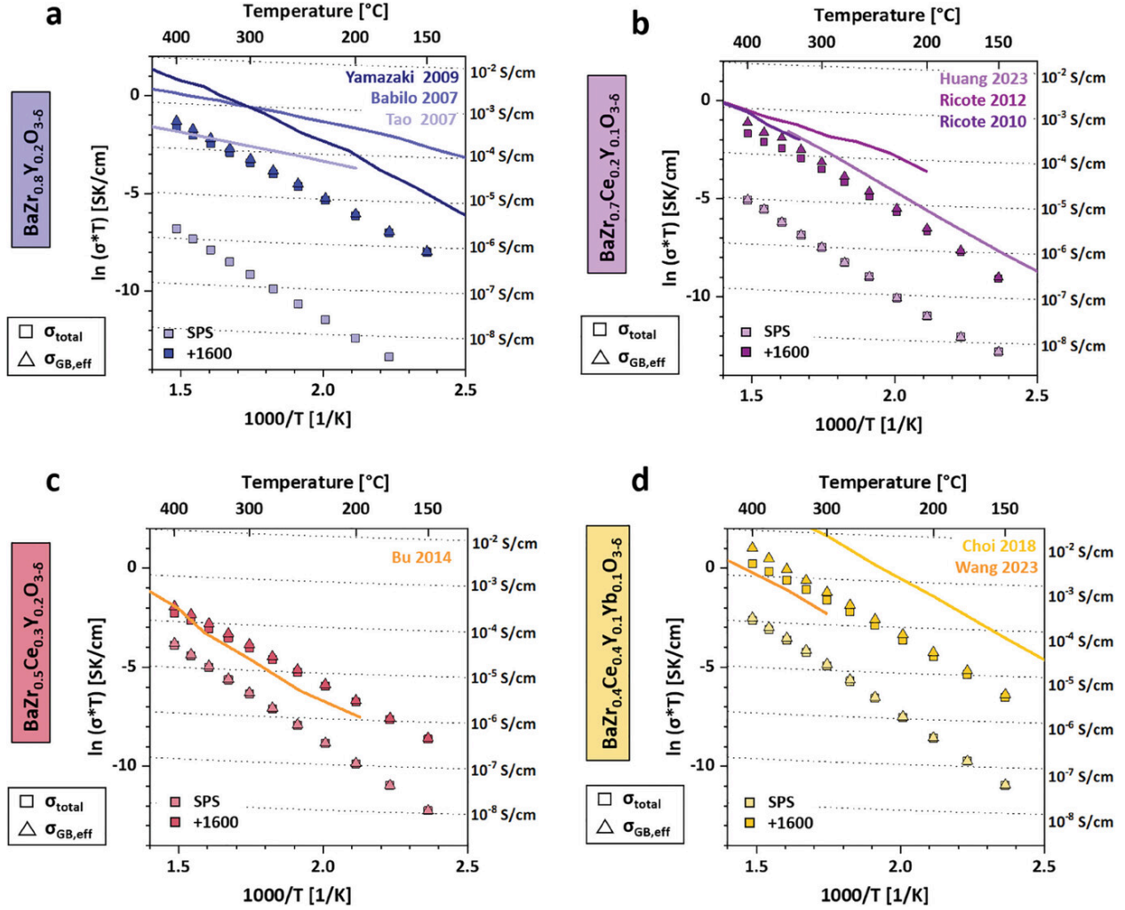
Figure 2.26. Segregation-controlled conductivity changes in different scientifically important BaZrO 3 based proton conductors. a–d) Electrochemical impedance spectroscopy in wet Ar/H 2 of BaZr 0.8 Y 0.2 O 3-δ (BZY20) (a) BaZr 0.7 Ce 0.2 Y 0.1 O 3-δ (BZCY721) (b) BaZr 0.5 Ce 0.3 Y 0.2 O 3-δ (BZCY532) (c) and BaZr 0.4 Ce 0.4 Y 0.1 Yb 0.1 O 3-δ (BZCYB4411) (d) samples after SPS and post thermally treated for 5 h at 1600 °C in air. Total and effective grain boundary conductivity are represented by squares and triangles, respectively. Literature data in all plots is visualized by lines [147] .
