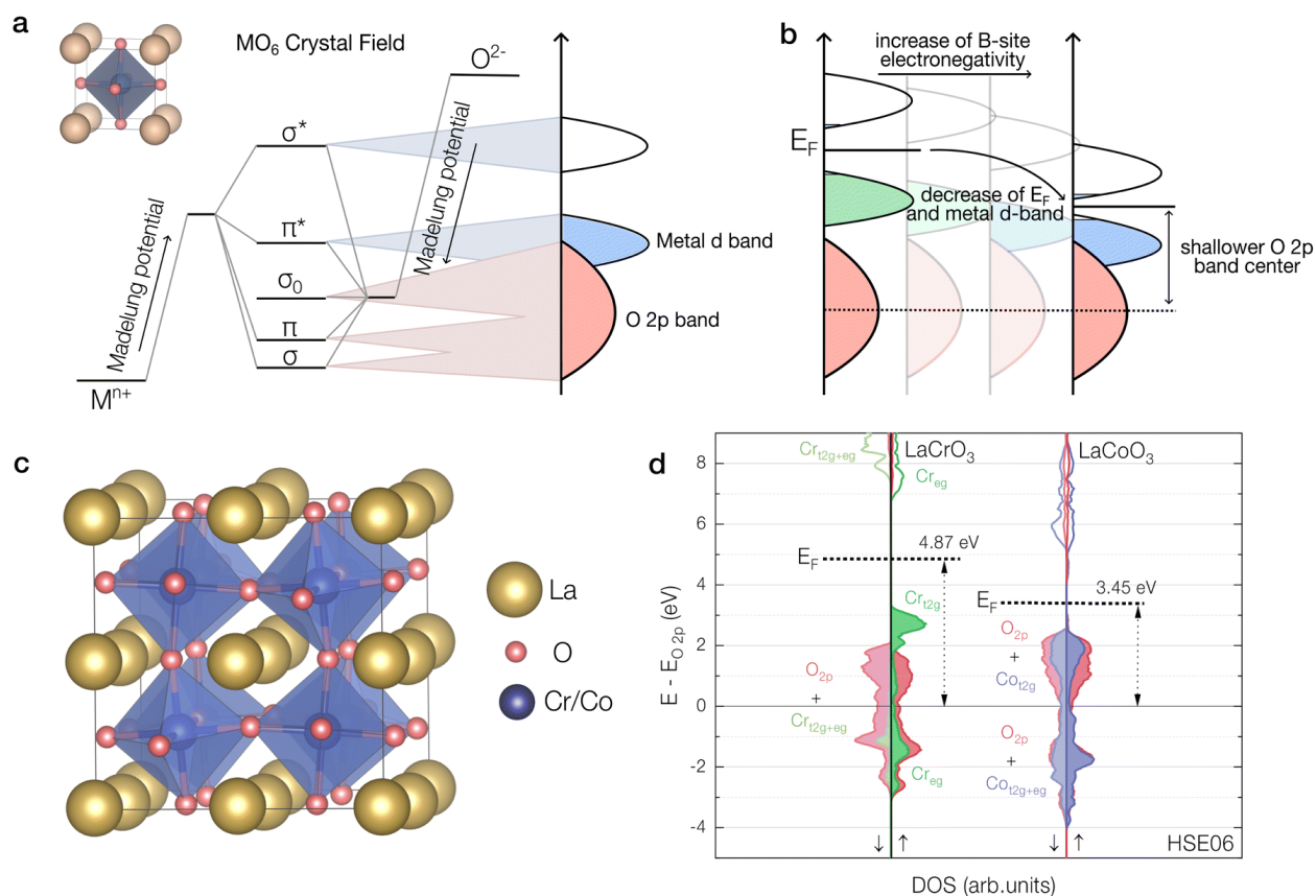
Figure 2.15. (a) Simplified evolution of an exemplary transition metal perovskite oxide band structure from the molecular orbital diagram for octahedral MO 6 . (b) Qualitative change of the electronic structure with increasing B-site cation electronegativity. E F and the metal d-band shift down, leading to a shallower O 2p band center. (c) Model of a 2 × 2 × 2 perovskite unit cell used for hybrid calculations (tilting angles slightly differ between LaCoO 3 and LaCrO 3 ). (d) Projected
