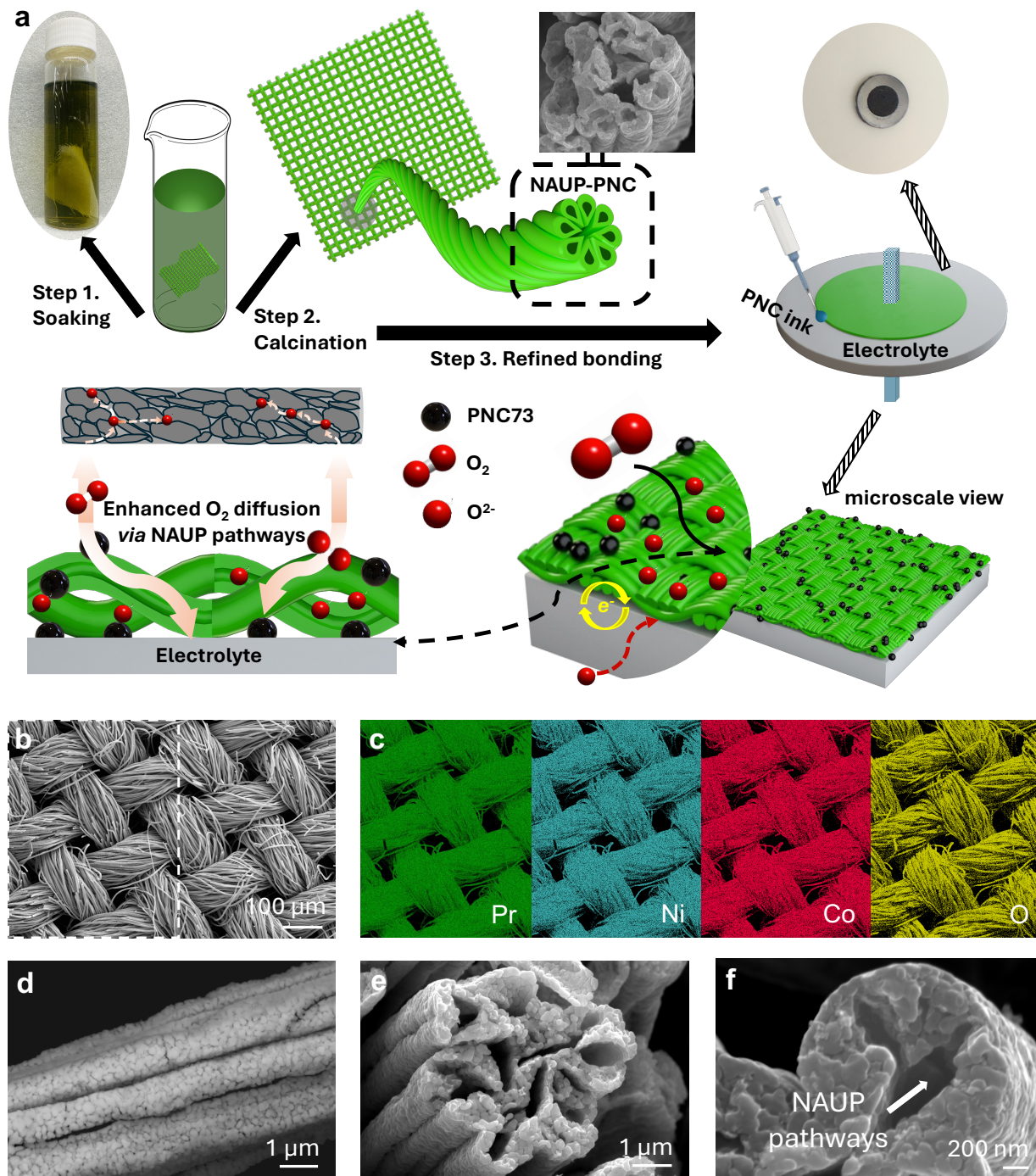
Figure 3.1. Scalable fabrication and characterization of nano-structured ultra-porous PNC73 oxygen electrode. (a) Schematic illustration of the process to fabricate NAUP-PNC73
