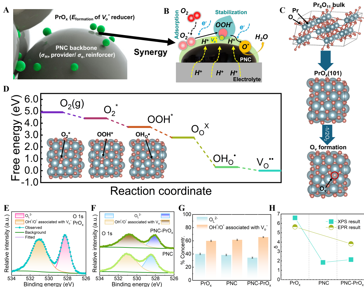
Figure 4.7. DFT analysis. (A) Schematic illustration of the reconstructed hetero interlayer between the \text{PrO}_x coating and PNC bulk. (B) Synergistic effect of the \text{PrO}_x coating and PNC bulk, facilitating the stabilization of the \text{OOH}^* intermediate. (C) The optimized lattice of monoclinic \text{Pr}_6\text{O}_{11} bulk with slab models representing \text{PrO}_x (101) and the V_{\text{O}}^{\bullet\bullet} site in the top layer. (D) free energy diagram depicting ORR on \text{PrO}_x in the presence of V_{\text{O}}^{\bullet\bullet} at 600^\circ\text{C} and 1 atm. The optimized ORR intermediate species ( \text{O}_2^* , \text{OOH}^* , and \text{OH}_o^* ) at the V_{\text{O}}^{\bullet\bullet} site is depicted in the inset of D). (E) Deconvoluted O 1s spectrum of \text{PrO}_x showing two main components attributed to lattice oxygen ( \text{O}_L^{2-} ) and surface V_{\text{O}}^{\bullet\bullet} . (F) Comparative O 1s spectra for PNC- \text{PrO}_x and PNC samples, illustrating enhanced intensity of surface V_{\text{O}}^{\bullet\bullet} sites in the hybrid. (G) Quantified relative concentrations of \text{O}_L^{2-} and surface V_{\text{O}}^{\bullet\bullet} across the three materials. (H) Surface oxygen vacancy concentration \delta determined by XPS and EPR for \text{PrO}_x , PNC, and PNC- \text{PrO}_x .
