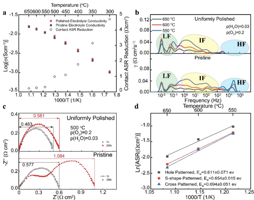
Figure 2.22. EIS characterization results of the symmetrical cells with thick BCZYYb7111 electrolyte pellets (pristine and homogeneously laser-polished electrolyte surfaces) sandwiched between two identical porous BCFZY0.1 cathode films. (a) comparison of the apparent conductivities and the contact ASR reduction caused by laser polishing, (b) DRT spectra of the uniformly polished and pristine symmetrical cells, (c) ASR degradation of the uniformly polished and pristine symmetrical cells, and (d) activation energies of the patterned symmetrical cells [129] .
