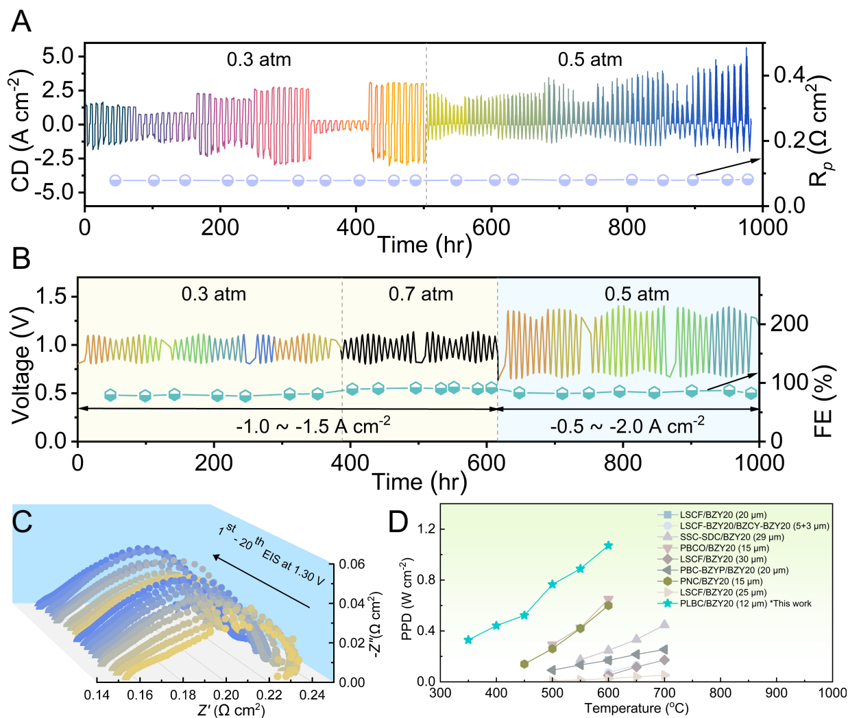
Figure 5.6. Long-term reversible operation and benchmarked performance of the PLD-enabled protonic ceramic cell under thermal cycling test. (A) Current-density (CD) cycling stability over \sim 1000 h under pressurized steam electrolysis, with the corresponding R_p tracked continuously throughout the test. (B) Voltage response during dynamic current-density cycling under varying steam pressures (0.3, 0.7, and 0.5 atm), together with the evolution of FE over time. (C) Operando EIS collected at 1.30 V, demonstrating impedance stability during sustained electrolysis operation. (D) Literature benchmark of PPD as function of temperature for representative cells, highlighting the performance achieved in this work [139,288–294] .
