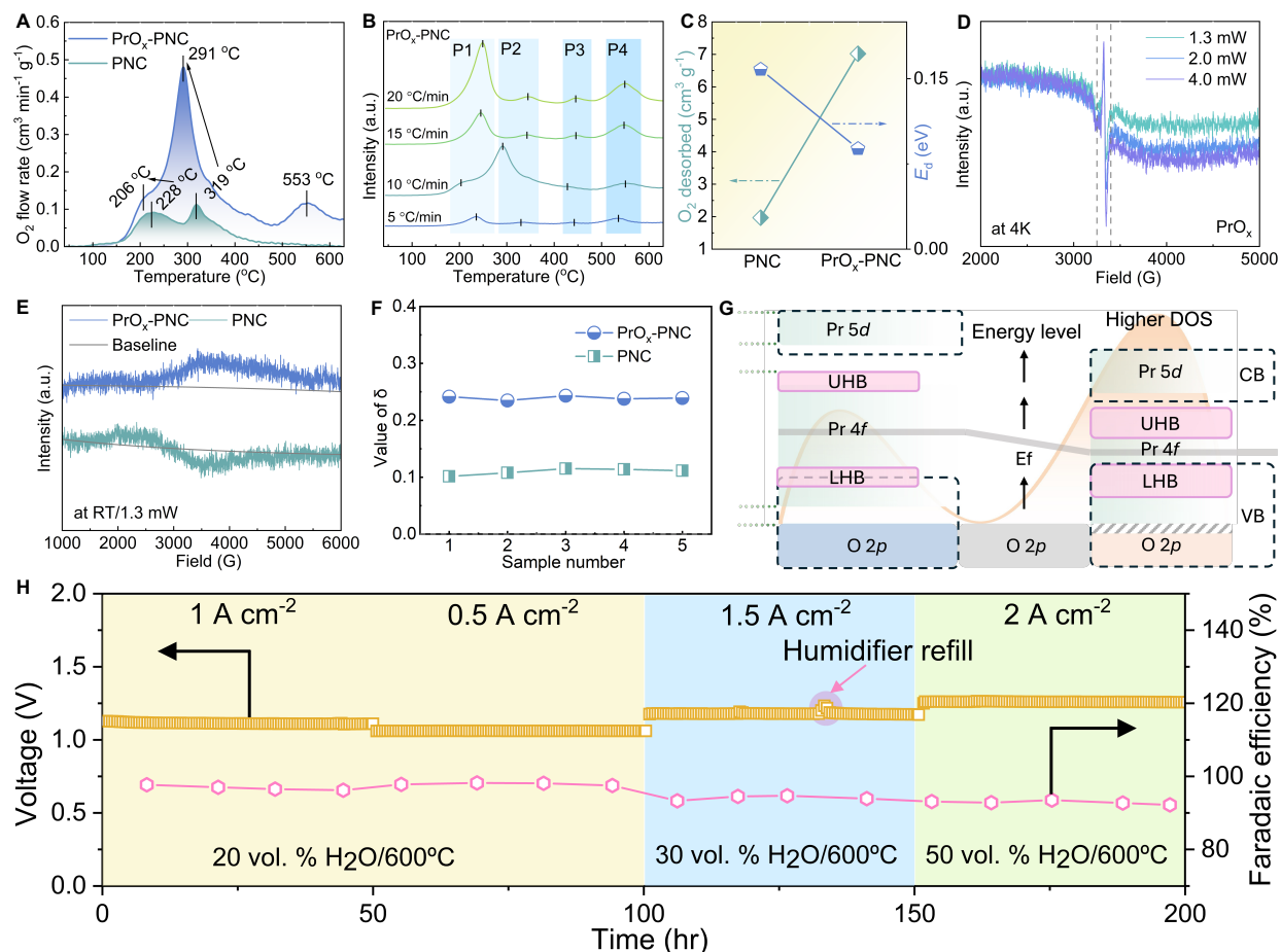
Figure 6.6. Comprehensive investigation of oxygen vacancy behavior and mobility for understanding the mechanism related with the hybrid interfaces. (A) \text{O}_2 -TPD profiles collected at 10^\circ\text{C min}^{-1} . (B) \text{O}_2 -TPD spectra under various heating rates ( 5\text{--}20^\circ\text{C min}^{-1} ) exhibit four resolved peaks (P1–P4), corresponding to surface adsorbed, lattice, subsurface, and bulk oxygen species. (C) Comparison of total desorbed \text{O}_2 and activation energy. (D) Low-temperature (4 K) EPR spectra of \text{PrO}_x under 1.3–4.0 mW reveals strong paramagnetic signals, validating oxygen defect centers. (E) Room-temperature EPR spectra at 1.3 mW show the stronger signal in \text{PrO}_x\text{--PNC} compared to PNC, confirming higher surface vacancy concentration. (F) Iodometric titration results show consistently higher bulk oxygen non-stoichiometry ( \delta ) in \text{PrO}_x\text{--PNC} across five samples. (G) Schematic of the proposed band structure modulation mechanism at the \text{PrO}_x\text{--PNC} interface showing enhanced orbital hybridization and increased density of states (DOS) near the Fermi level ( E_f ). (H) Electrolysis performance at 600^\circ\text{C} under varied \text{H}_2\text{O} partial pressure and current densities ( 0.5\text{--}2\text{ A cm}^{-2} ) demonstrates excellent Faradaic efficiency and voltage stability, confirming robust oxygen vacancy modulation.
