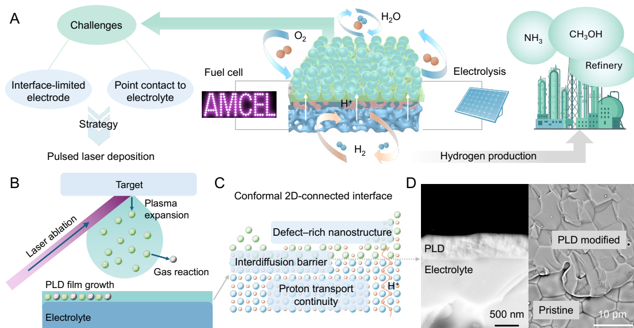
Figure 5.1. PLD-enabled interfacial nanostructuring strategy for protonic ceramic cells. (A) Schematic overview of targeted applications, persistent oxygen electrode–electrolyte interfacial limitations, and the PLD-based strategy to overcome them. (B) Illustration of the PLD process, highlighting the formation of thin, dense, and adherent ceramic layers with controlled composition and thickness. (C) Conceptual depiction of a conformal electrode–electrolyte interface that enhances interfacial bonding, transport continuity, and reaction-zone accessibility. (D) Representative electrode layer directly deposited on the electrolyte, shown in cross-sectional (left) and top-view (right) configurations.
