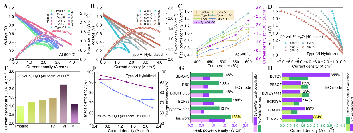
Figure 4.5. Electrochemical performance of the hybrid Type VI electrode full cells in both fuel cell and electrolysis modes. (A) I - V - P curves of different loaded hybrid electrode full cells at 600^\circ\text{C} . (B) I - V - P curves of the hybrid Type VI electrode full cells at 400 - 600^\circ\text{C} . (C) Comparisons of peak power density and current density of different loaded hybrid electrode full cells at 400 - 600^\circ\text{C} . (D) Polarization curves of the hybrid Type VI electrode full cells in electrolysis mode at 400 - 600^\circ\text{C} . \text{H}_2 (20 sccm) and 20 vol.% \text{H}_2\text{O} + 80 vol.% \text{O}_2 (40 sccm) were fed to the electrode. The applied voltage for all tests ranged from 1.60 V to OCV. (E) Comparisons of current density at 1.30 V of different loaded hybrid electrode full cells at 600^\circ\text{C} for steam electrolysis. (F) Faradaic efficiency of hybrid Type VI electrode full cells. G) and H) Comparison of the hybrid Type VI electrode full cell performances in both fuel cell and electrolysis at 1.30 V with some recent literatures. \text{Ba}(\text{Co}_{0.4}\text{Fe}_{0.4}\text{Zr}_{0.1}\text{Y}_{0.1})_{0.95}\text{O}_{3-\delta} (BCFZY-0.95); \text{BaCe}_{0.36}\text{Fe}_{0.64}\text{O}_{3-\delta} (BCF36); \text{Ba}_{0.5}\text{Sr}_{0.5}(\text{Co}_{0.8}\text{Fe}_{0.2})_{0.95}\text{P}_{0.05}\text{O}_{3-\delta} (BSCFP0.05); \text{PrBaCo}_2\text{O}_{5+\delta} (PBC); \text{Ba}_{0.5}\text{Sr}_{0.5}\text{Co}_{0.7}\text{Fe}_{0.2}\text{Ni}_{0.1}\text{O}_{3-\delta} / \text{BaZr}_{0.1}\text{Ce}_{0.7}\text{Y}_{0.1}\text{Yb}_{0.1}\text{O}_{3-\delta} (BB-OPS); \text{Ba}(\text{Co}_{0.4}\text{Fe}_{0.4}\text{Zr}_{0.1}\text{Y}_{0.1})_{0.95}\text{Mg}_{0.05}\text{O}_{3-\delta} (BCFZYM);
