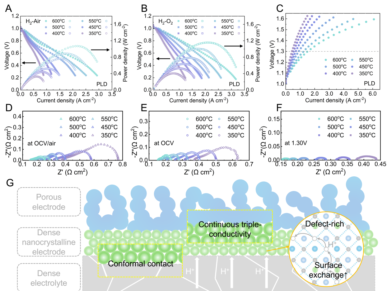
Figure 5.5. Performance enhancement enabled by interfacial nanostructuring in PCCs. (A) Temperature-dependent I–V and corresponding power-density curves of the PLD cell measured in H_2 –air from 350 to 600 °C. (B) Temperature-dependent I–V and power-density curves in H_2 – O_2 (350–600 °C), highlighting enhanced intrinsic oxygen-electrode kinetics. (C) Polarization behavior of the PLD cell under 0.3 atm steam. (D) Temperature-dependent EIS collected at OCV in H_2 –air, showing the evolution of polarization resistance with temperature. (E) Temperature-dependent EIS collected at OCV in H_2 – O_2 . (F) EIS measured under electrolysis operation at 1.30 V and 0.3 atm steam, revealing markedly reduced impedance under operating bias. (G) Mechanistic schematic illustrating how a dense nanocrystalline PLD-derived layer creates conformational contact and continuous triple-conducting pathways, while a defect-rich interfacial region promotes oxygen surface exchange and interfacial charge transfer.
