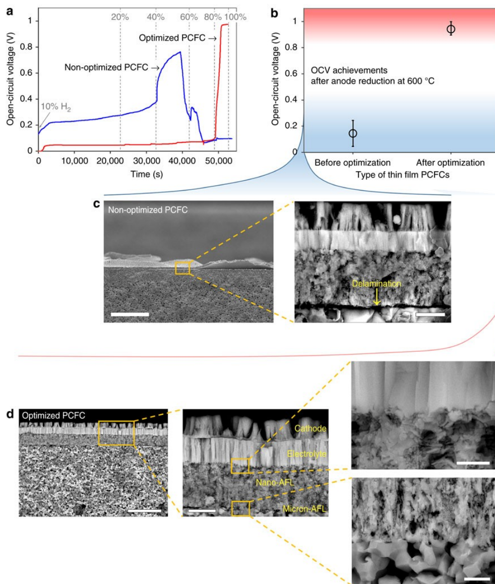
Figure 2.27. Comparison between PCFCs with optimized and non-optimized nano-AFLs. The optimized nano-AFL was fabricated by post annealing at 1300^\circ\text{C} for 1 h after PLD with
