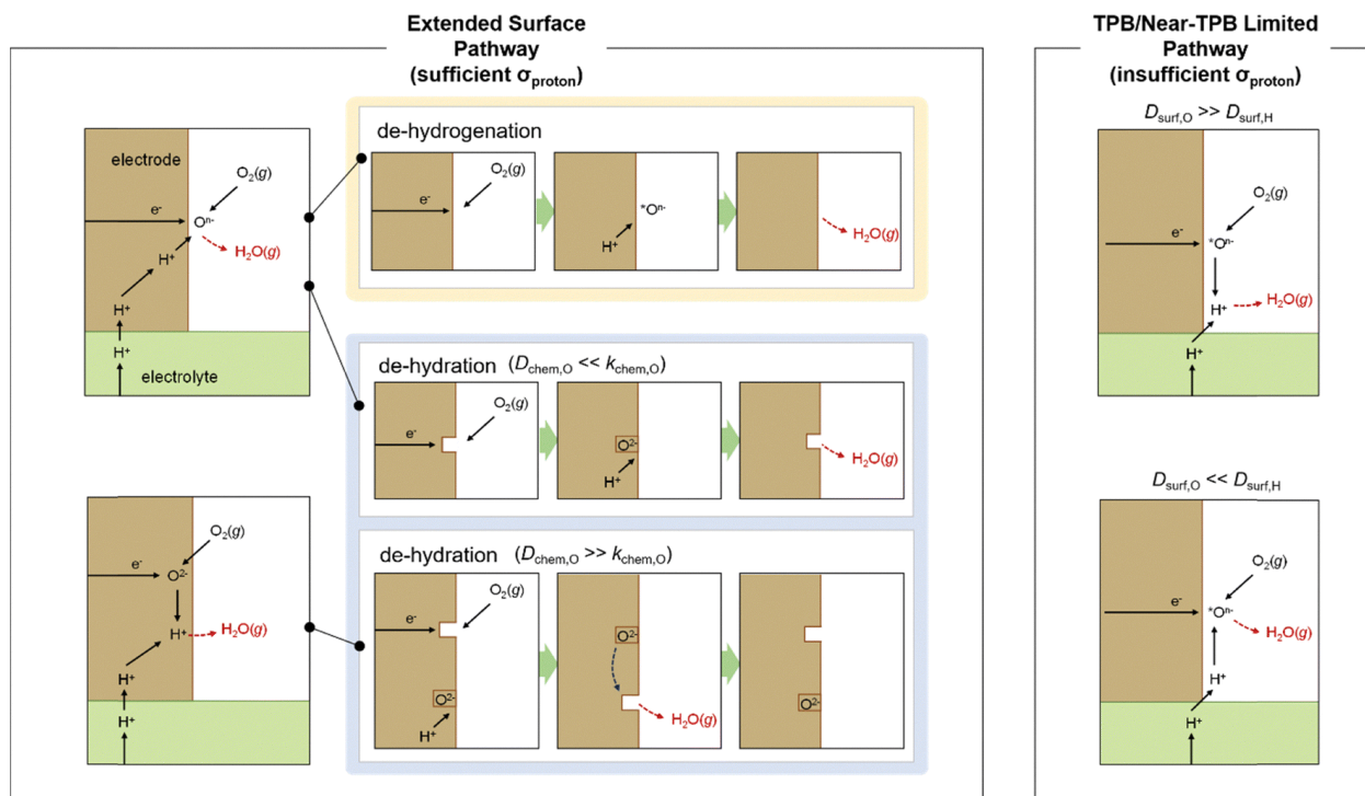
Figure 2.14. Five representative reaction pathways for proton-coupled oxygen reduction reaction in PCFC cathodes are governed by the proton conductivity of the cathode material. In the TPB/Near-TPB limited pathway (insufficient \sigma_{\text{proton}} ), the dominant route depends on the relative diffusivity of protons and oxygen species at the cathode surface. In the extended surface pathway (sufficient \sigma_{\text{proton}} ), proton release occurs via either a dehydrogenation mechanism (not involving oxygen vacancies) or a dehydration mechanism (involving oxygen vacancies), the latter of which is further classified based on the relative rates of bulk oxygen diffusion ( D_{\text{chem,O}} ) and surface oxygen exchange ( k_{\text{chem,O}} ) [84] .
