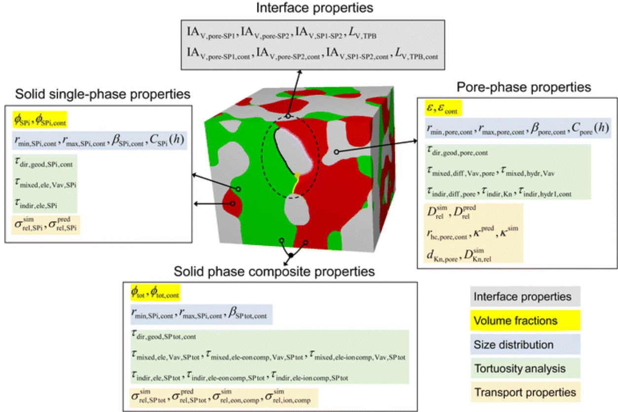
Figure 2.10. Overview of the characterized microstructure properties for the two solid-phases SP1 and SP2 (summarized as SPi, where i denotes 1 or 2), the total composite solid-phase SP tot, the pore-phase and the interface properties. The used variables are explained in the following sections [63] .
