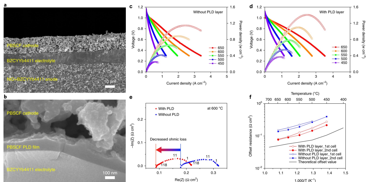
Figure 2.21. Electrochemical properties of the PBSCF cathode based on BZCYYb4411 proton conducting electrolyte using humidified (3% H 2 O) H 2 as fuel and dry air as oxidant at various temperatures. (a) Cross-section. (b) Expanded view of cross-section showing PLD layer at the cathode of electrolyte–cathode interface. (c) Polarization and power density curves of a representative cell without a PLD layer. (d) Polarization and power density curves of a representative cell with a PLD layer. (e) Impedance spectra collected at 600 °C, showing dramatic decrease in offset resistance on introduction of the cathode PLD layer. (f) Offset (ohmic) resistance under OCV [117] .
