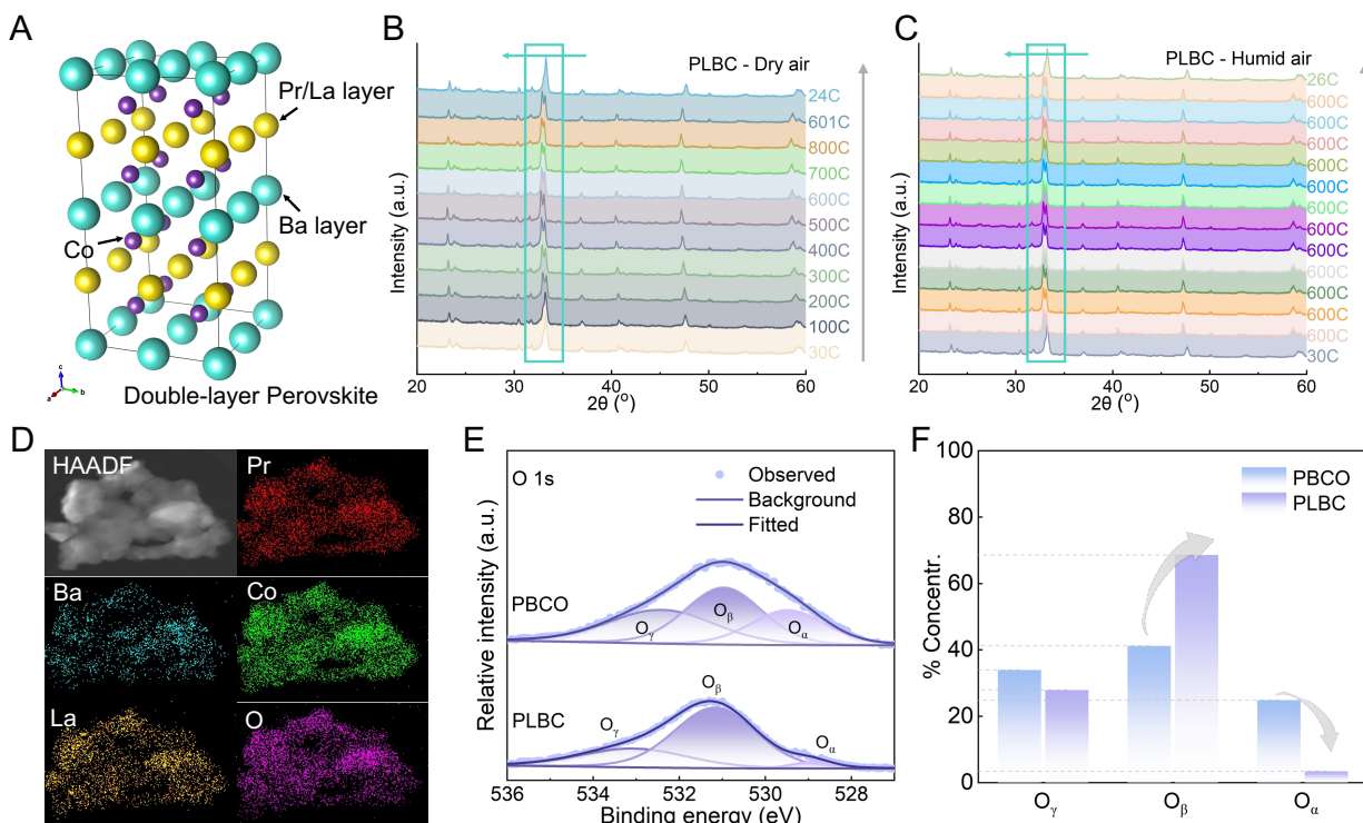
Figure 5.2. Structural stability, chemical expansion, and defect chemistry of PLBC. (A) Crystal structure of the double-layer perovskite PLBC. (B, C) High-temperature X-ray diffraction (HT-XRD) patterns of PLBC powder collected in (B) dry air (100 sccm) and (C) humid air (2.9–3.1 vol% H_2O in air, 100 sccm), revealing atmosphere-dependent chemical expansion. (D) STEM-EDS elemental mapping of PLBC powder confirming spatially uniform cation distribution. (E) XPS O 1s spectra comparing PBCO and PLBC powders, where O_\alpha , O_\beta , and O_\gamma denote lattice oxygen, hydroxyl-related species, and surface adsorbates, respectively. (F) Quantitative distribution of the resolved oxygen species shown in (E).
