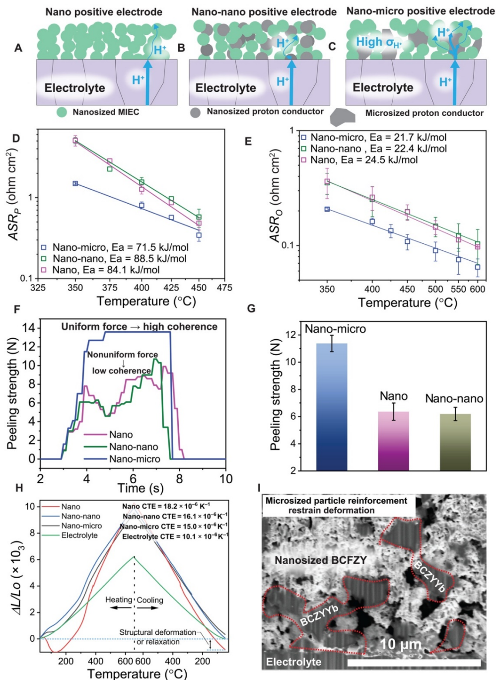
Figure 2.23. Redesigned nano-micro positive electrode simultaneously reducing ASRO and ASRP. The errors bars in these figures correspond to SDs from the averaging across all measurements. (A) Illustration of the nano positive electrode, which is a nanosized BaCo_{0.4}Fe_{0.4}Zr_{0.1}Y_{0.1}O_{3-\delta} (BCFZY). (B) Illustration of the nano-nano positive electrode, which is a composite of a nanosized BCFZY and a nanosized BaCe_{0.4}Zr_{0.4}Y_{0.1}Yb_{0.1}O_{3-\delta} (BCZYyb). (C) Illustration of the nano-micro positive electrode, which is a composite of a nanosized BCFZY and
