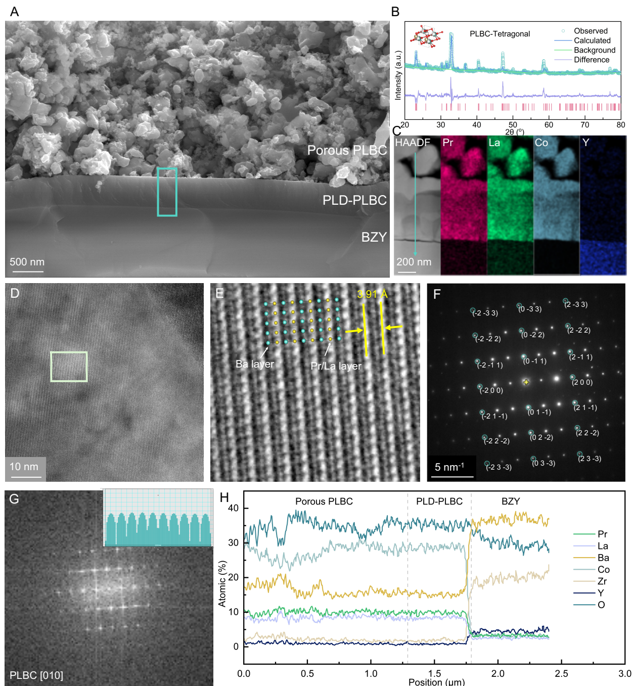
Figure 5.3. PLD-derived nanocrystalline PLBC interlayer with compositional continuity stabilizes the PLBC | BZY interface. (A) Cross-sectional SEM image of a PLD-PLBC full cell, showing the porous PLBC electrode supported by a dense PLD-derived interlayer on the BZY
