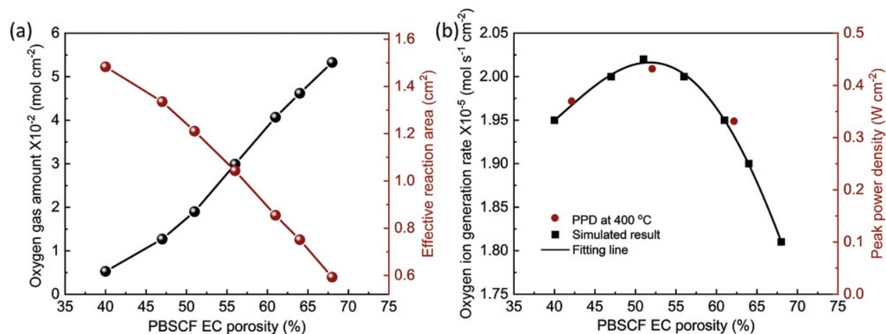
Figure 2.9. Phase field simulation of 3DEC with different porosities. (a) Oxygen gas absorption and effective reaction area in cathode bulk. (b) Oxygen ion generation rate and experimental PPD at 400 °C versus cathode porosity [59] .
