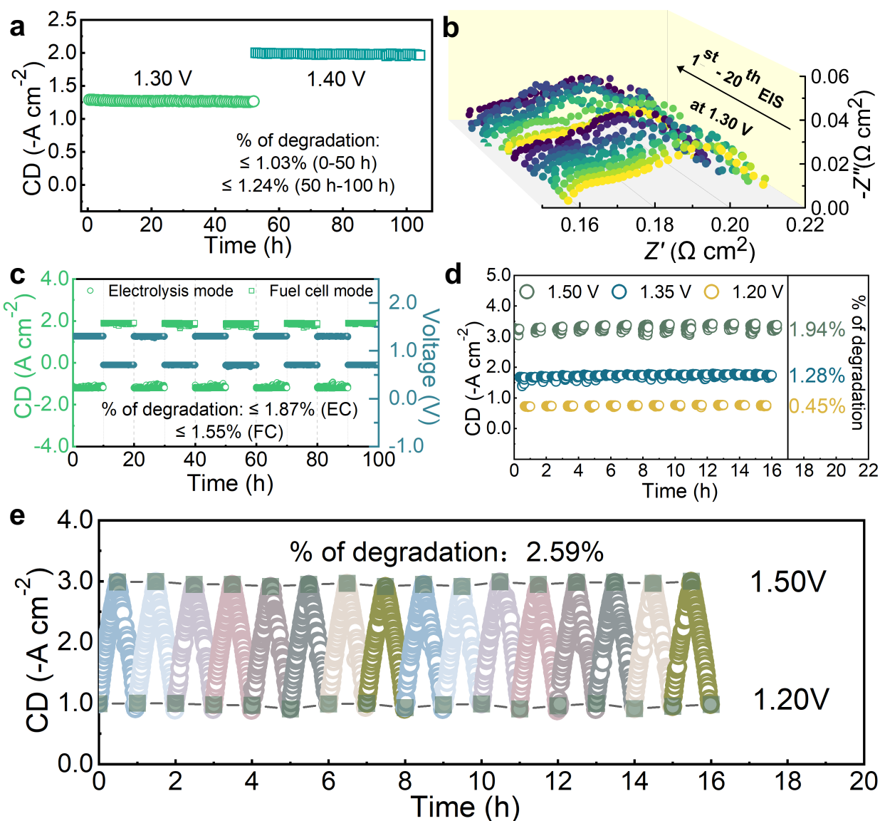
Figure 3.6. Extraordinary stability and durability on accelerated stress tests of NAUP-PNC full cells under both fuel cell and electrolysis modes. (a) Long-term stability tests for 100 hours,
