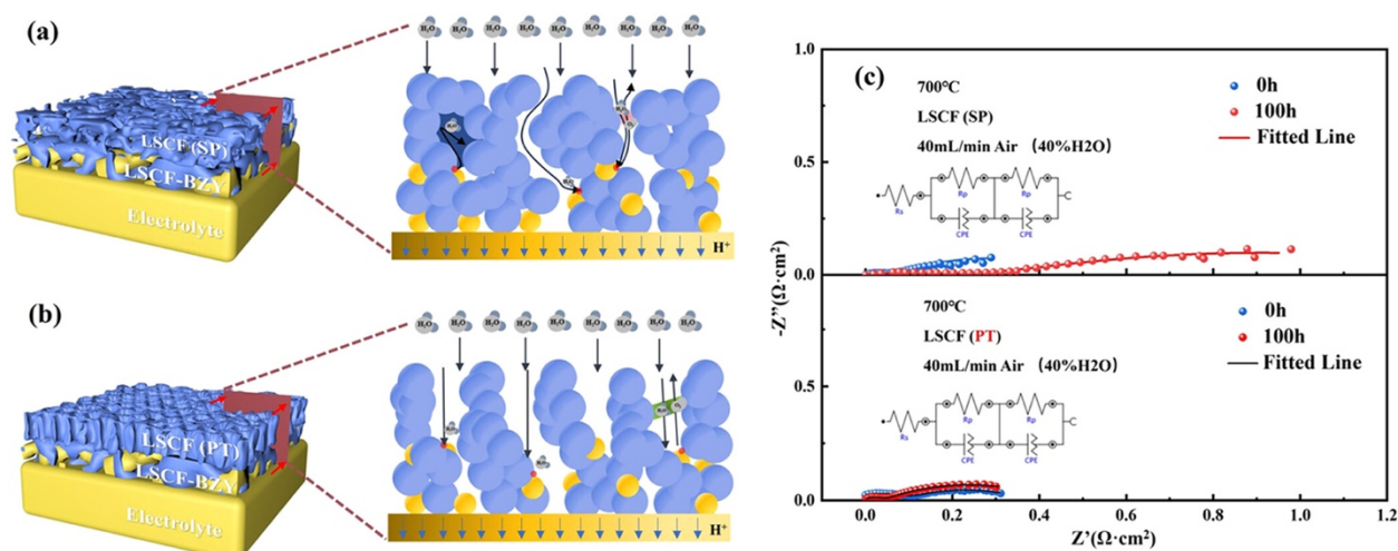
Figure 2.11. Schematic diagram of steam transport pathways in LSCF(SP)/LSCF – BZY (a) and LSCF(PT)/LSCF – BZY (b) air electrodes. EIS (Ohmic impedance removed) of the electrodes before and after 100 h of operation in 40% H 2 O–air (c) [71] .
