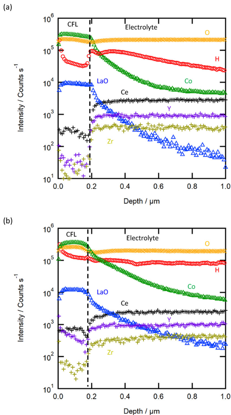
Figure 2.20. SIMS depth profiles of the LSCF-CFL cells (a) before and (b) after fuel cell measurements. The assignment is as follows: O (orange, cross), H (red, open circle), LaO (blue, open triangle), Co (green, open triangle), Ce (black, plus), Y (purple, plus), and Zr (yellow, plus). The dashed lines at a 0.2 \mu\text{m} depth indicate the border between CFL and the electrolyte. For SIMS measurements, the LSCF cathode was removed by scratching and sonication [114] .
