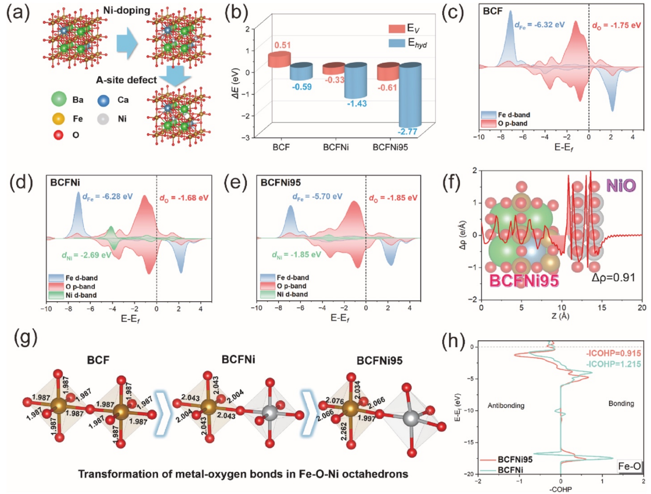
Figure 2.18. (a) Schematic diagram of BCFNi95 ( \text{Ba}_5\text{Ca}_2\text{Fe}_6\text{NiO}_{23} ), BCFNi ( \text{Ba}_6\text{Ca}_2\text{Fe}_6\text{Ni}_2\text{O}_{24} ), and BCF ( \text{Ba}_8\text{Fe}_8\text{O}_{24} ); (b) Calculated oxygen vacancy formation energies and hydrations energies for BCFNi95, BCFNi and BCF perovskites; Electronic DOS for (c) BCF, (d) BCFNi and (e) BCFNi95; (f) Planar average charge density difference plots of NiO|BCFNi95; (g) Comparison of Fe-O bonds in BCF, BCFNi and BCFNi95; (h) -ICOHP calculations results of Fe-O bonds in BCFNi and BCFNi95 [23] .
