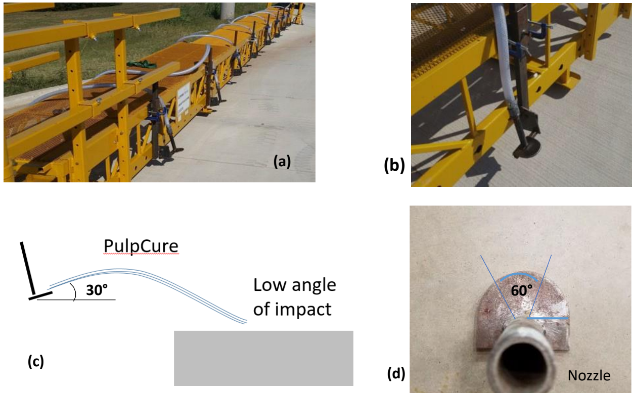
Figure 4-2 shows (a) entire work bridge with nozzles, (b) close-up of a nozzle, (c) diagram of pulp cure during placement, and (d) angle of nozzle.
