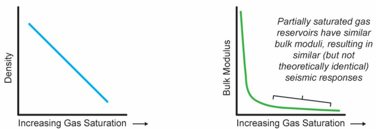
Figure 3-1: Change in rock properties with increasing gas saturation. The bulk modulus quickly decreases with a relatively small amount of gas saturation. This bulk modulus similarity between low and high gas saturation is the crux of the LSG gas differentiation problem.
