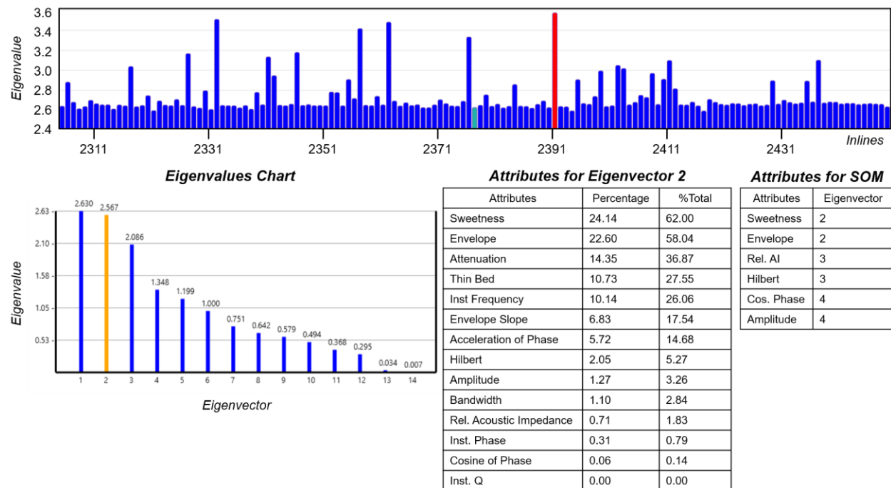
Figure 3-7: PCA results for Inline 2391 of the KKLA 3D seismic survey. The highest-ranking attributes from the first few eigenvectors were chosen to be incorporated into the SOM analysis over the entire dataset. These attributes were envelope, hilbert, the cosine of instantaneous phase, relative acoustic impedance, and sweetness. These attributes were also combined with the full-stack amplitude.
