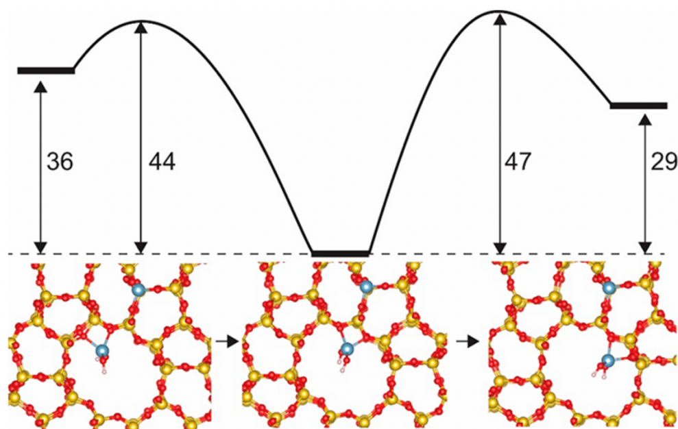
Figure 18. DFT calculations of migration of \text{Al}(\text{OH})_2^+ at the intersection. The colors blue, yellow, red, and white represent Al, Si, O, and H atoms, respectively. The energy units are given in kJ/mol. 25
