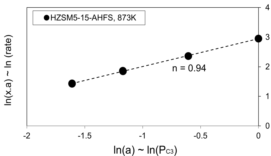
Figure 37. Estimation of the order of propane cracking on HZSM5-15-AHFS. In which x is the reaction conversion, a is the mole percent of propane in the loop.
