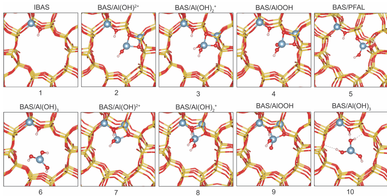
Figure 24. Calculated structures of proposed active sites in H-ZSM5 zeolite.
