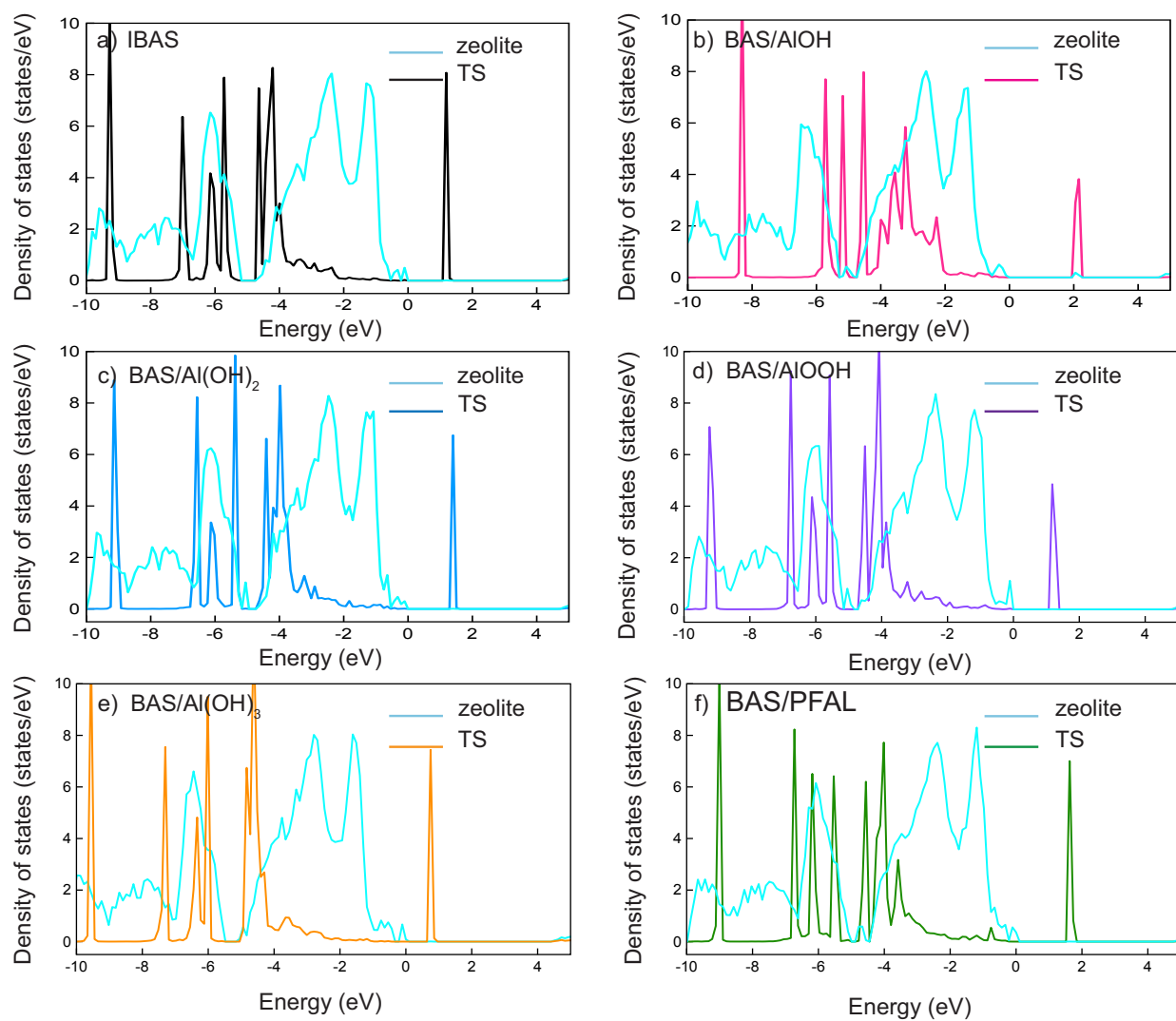
Figure 33. Density of state at the TSs of hydrogenation reactions.
