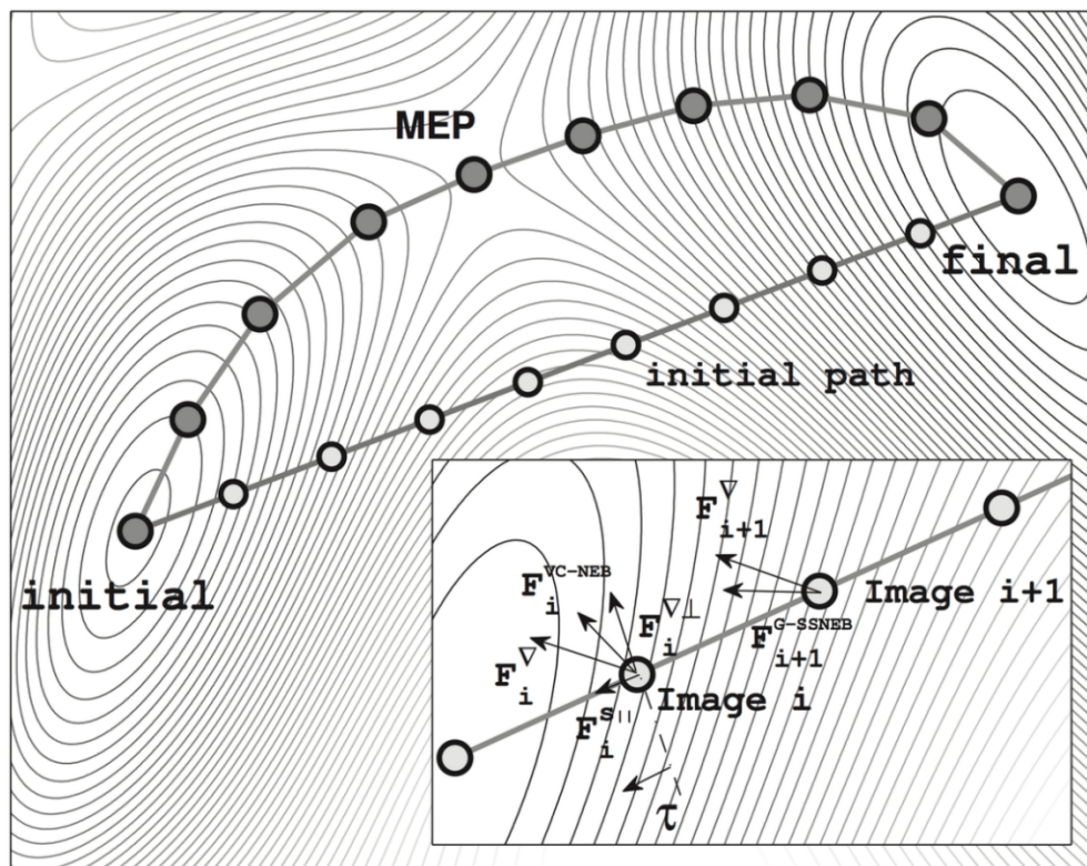
Figure 15. This figure from Jonsson et. al. illustrates an example NEB simulation that shows the creation of initial images (represented by a line with white circles) along a direct reaction path from the initial state to the final state, and the optimized final path (represented by a line with gray circles) passing through the MEP of that specific reaction. 63
