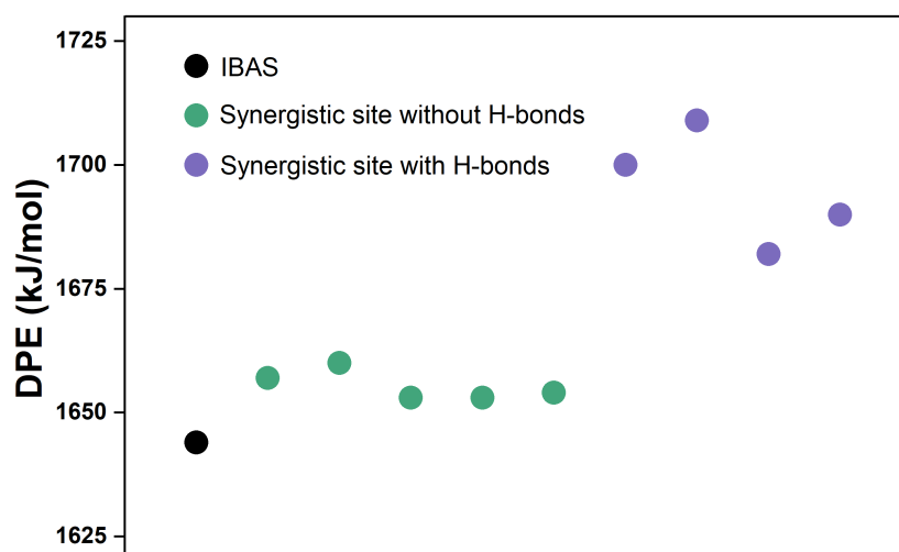
Figure 26. DPE for various proposed active site in HZSM-5 zeolite.
