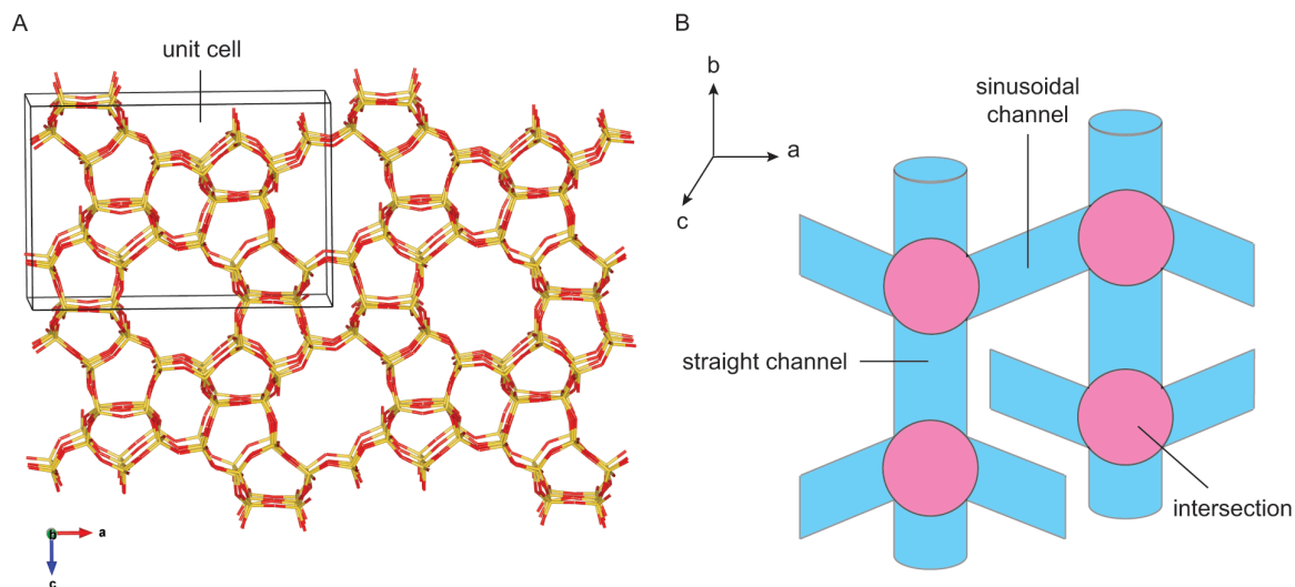
Figure 5. A) Calculated H-ZSM5 zeolite structure; B) Schematic diagram of three-dimensional channel system of H-ZSM5 zeolite morphology comprising of the straight and the sinusoidal channel.
