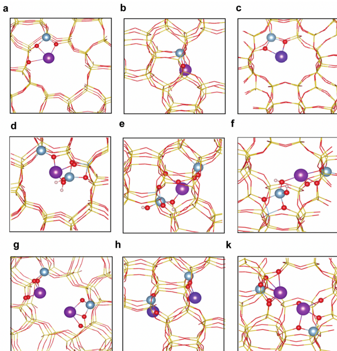
Figure 20. Calculated structures of Na + titrated to (a) IBAS at the intersection, (b) IBAS in the straight channel, (c) IBAS in the sinusoidal channel, (d) BAS/EFAL at the intersection, (e) BAS/EFAL at the straight channel, and (f) BAS/EFAL in the sinusoidal channel; calculated structures of Na + titrated to (g) paired BAS at the intersection (h) paired BAS in the straight channel and (k) paired BAS at the sinusoidal channel. Na, Al, O, Si, and H atoms are colored purple, cyan, red, yellow, and white, respectively. 31
