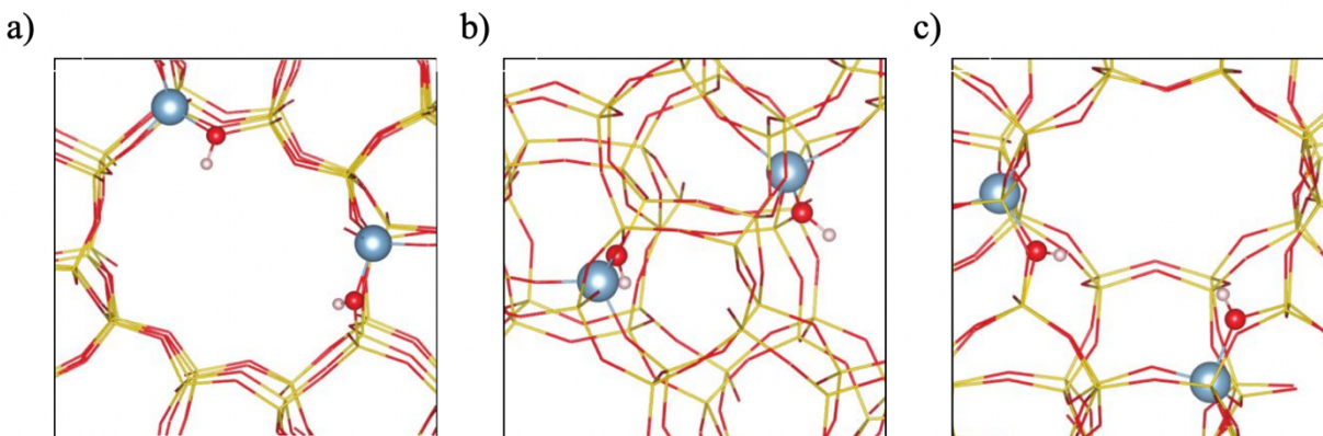
Figure 21. The optimized structures of paired BAS at a) intersection, b) straight channel, c) sinusoidal channel. 31
