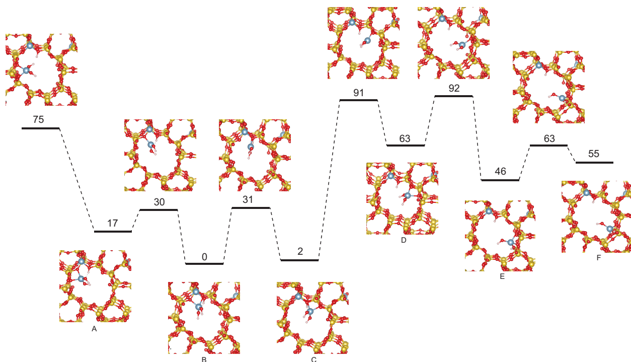
Figure 19. The role of BAS in stabilizing the EFAL species.
