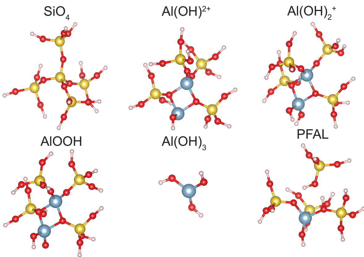
Figure 23. Calculated structures used in polarizability calculations.
