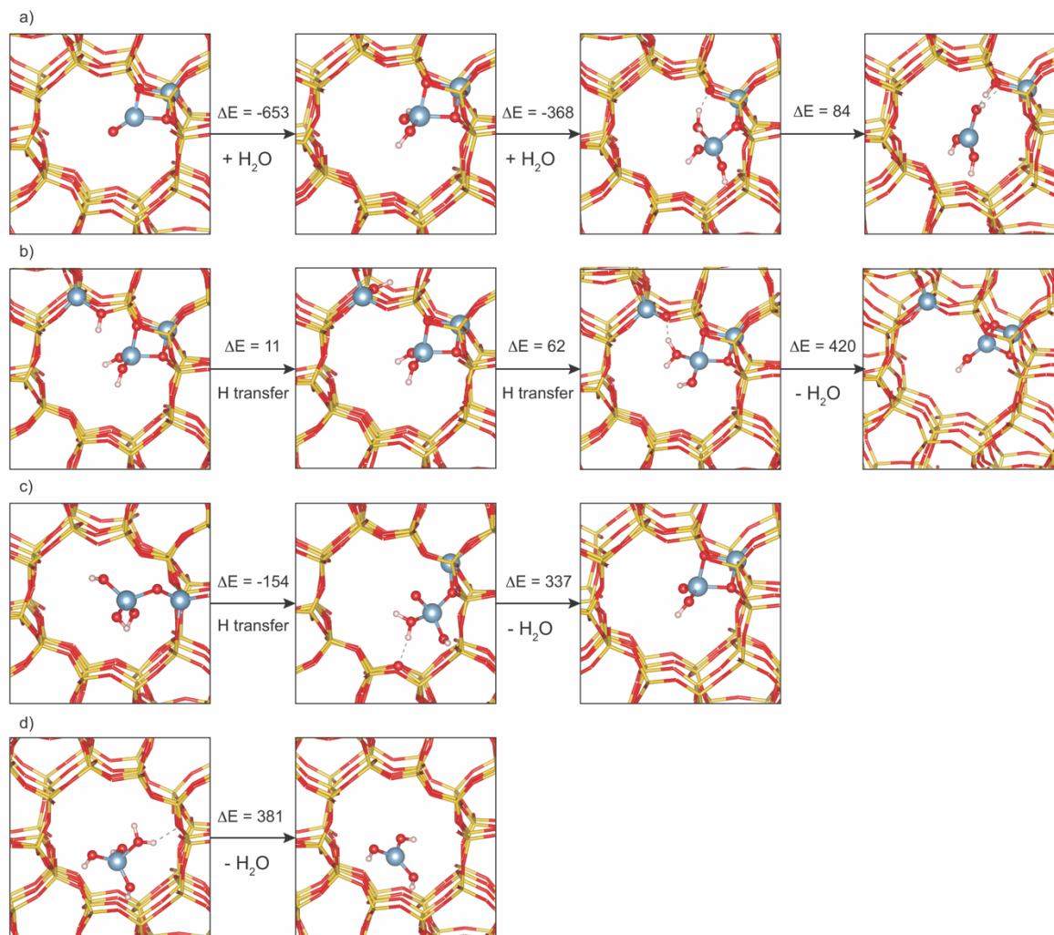
Figure 22. Transformation of EFAL species in ZSM-5.
