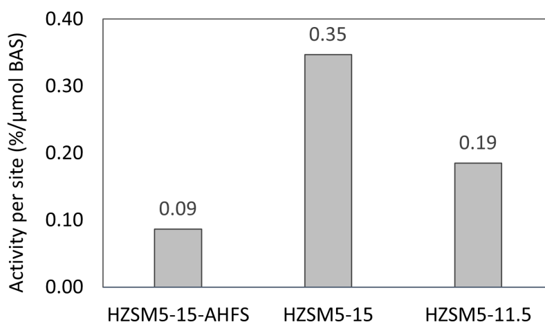
Figure 36. Activity per site of propane conversion in HZSM5-X zeolites, X is Si/Al ratio. 500 \mu l pulses of pure propane (>99%) are injected at temperature as 823 K. The BAS densities of HZSM5-15-AHFS, HZSM5-15 and HZSM5-11.5 are 0.45, 0.73 and 1.08 mmol/g, respectively.
