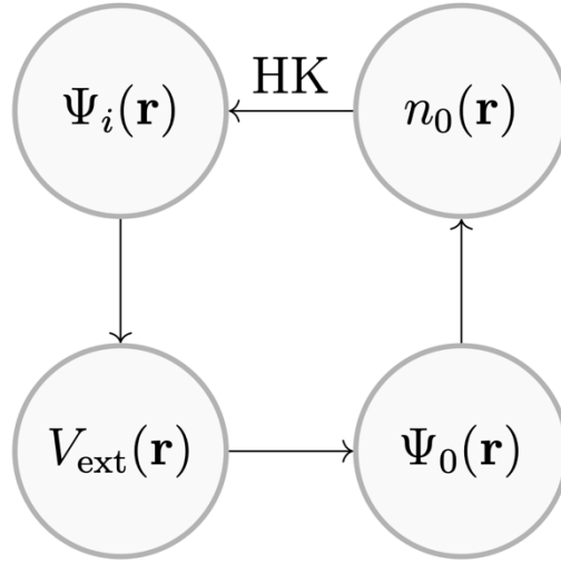
Figure 3. This process allows for the iterative determination of the ground state density of a given system, by utilizing the principle outlined in the Hohenberg-Kohn theorems, taken from ref. 23
