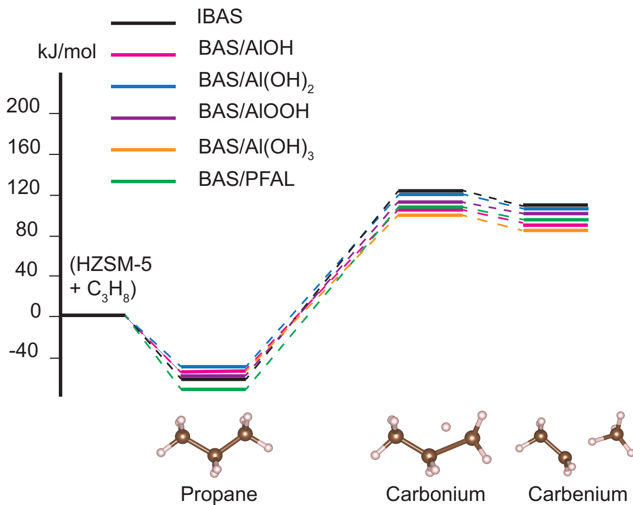
Figure 27. Enthalpy profiles of propane cracking on different active sites.
