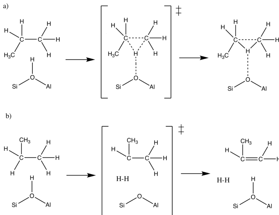
Scheme 3. Reaction mechanism of propane a) cracking and b) dehydrogenation of methylene group.
