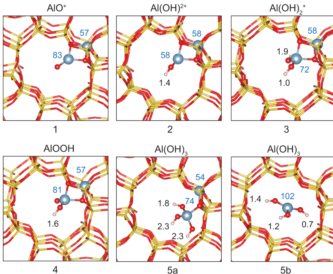
Figure 7. Optimized structures of various EFAl species stabilized at the intersection and their DFT-calculated ^1\text{H} NMR and ^{27}\text{Al} NMR.
