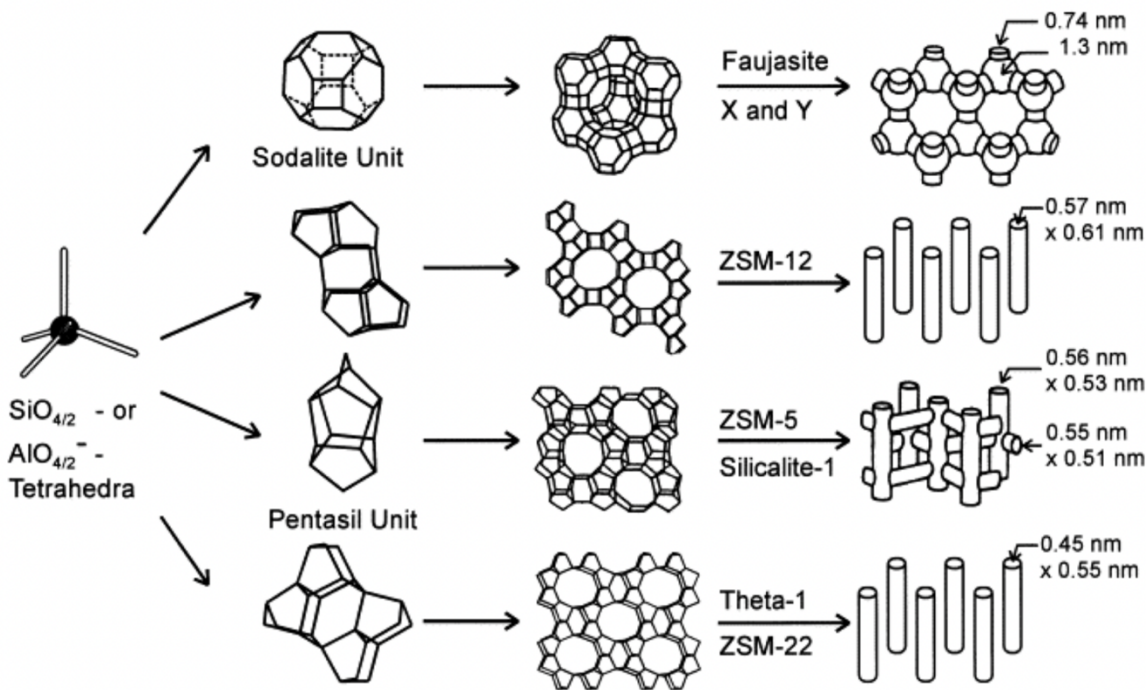
Figure 1. The configuration of four chosen zeolites along with their respective micro-pore system and measurements. This figure is taken from ref. 5
