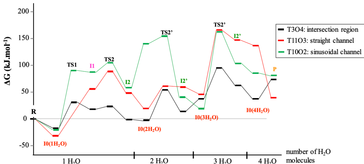
Figure 13. The free energy profiles for the favored dealumination route of T3O4, T10O2, and T11O3 sites in H-MFI, which involved four water molecules and resulted in the formation of EFAL \text{Al}(\text{OH})_3\text{H}_2\text{O} , were analyzed at a temperature of 450 K. The calculation of free energy utilized a physisorbed water reference. 17
