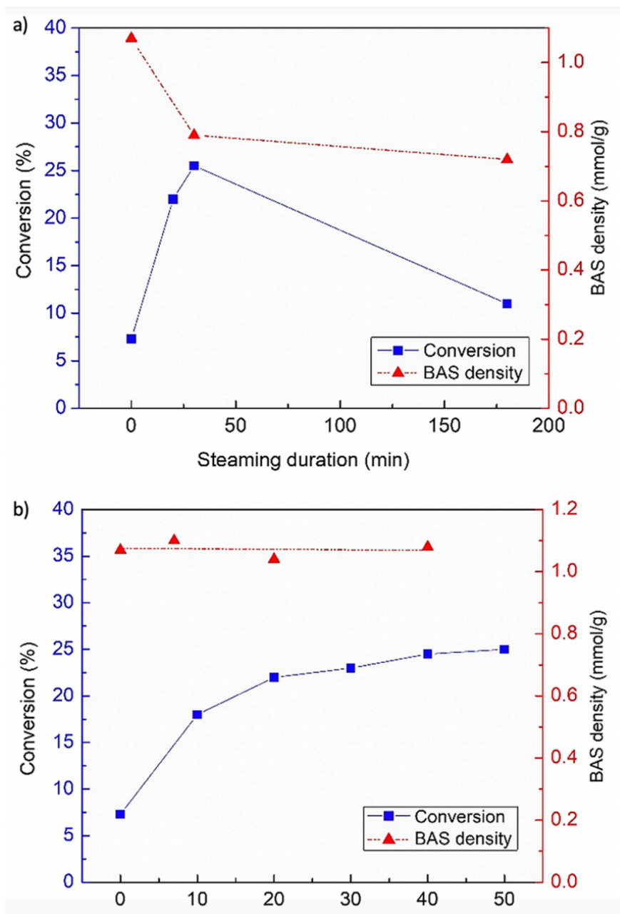
Figure 14. Conversion of n-hexane cracking on HZSM5-11.5 catalyst and BAS density (determined by IPA-TPD) as a function of (a) steaming duration (catalyst was treated by steaming) and (b) number of pulses of water (catalyst was treated by pulsing water). The steam treatment was at 480 °C in both cases, with a water partial pressure of 18.6 kPa either in a continuous manner or in pulses. Reaction conditions: T = 480 °C, P nC6 = 4.5 kPa with 0.48 μmol of n-hexane injected in each pulse, 5 mg amount
