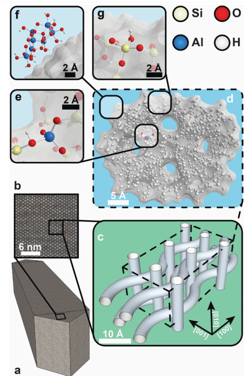
Figure 2. Overview of H-ZSM5 at various dimensional scale. a) a micro-sized coffin-shaped H-ZSM-5 crystal. b) straight pores [001] [100] planes. c) three-dimensional channel system. d) MFI framework comprises of silica and aluminum tetrahedra. e) BAS. f) extra-framework aluminum from dealumination. g) terminal silanol group.
