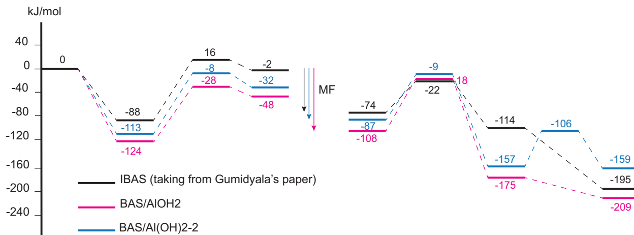
Figure 43. Energy profile of acylation of 2-MF with acetic acid on BAS with the presence of EFAL Al(OH) 2 + in proximity.
