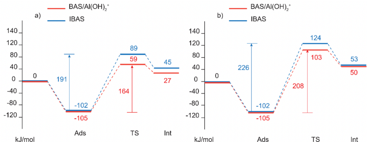
Figure 39. Reaction energy diagram of n-hexane (a) central cracking and (b) dehydrogenation of the methylene group. This figure was taken from ref. 31
