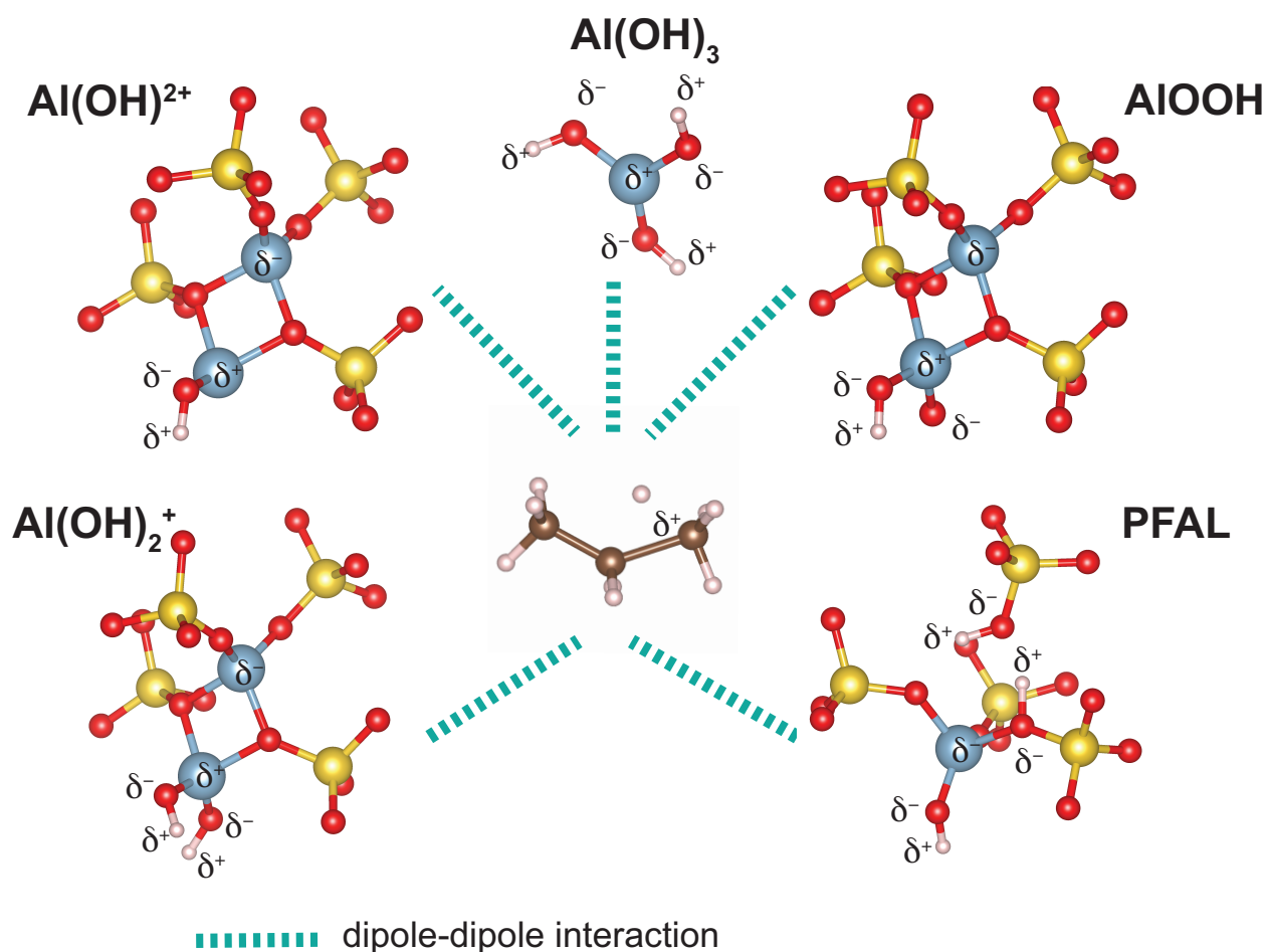
Figure 30. Electrostatic interaction between carbonium \text{C}_3\text{H}_9^+ and different EFAL and PFAL species.
