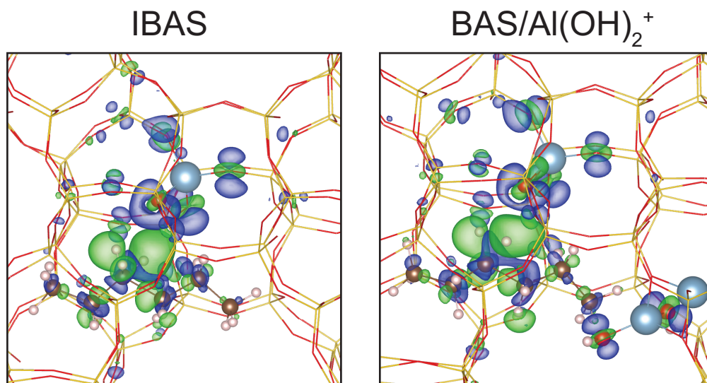
Figure 40. Electron density difference charge of TS of hexane cracking reactions on various active sites, the value of isosurface is 0.002 au. The blue color represents accumulation of charge and the green color represents depletion of charge.
