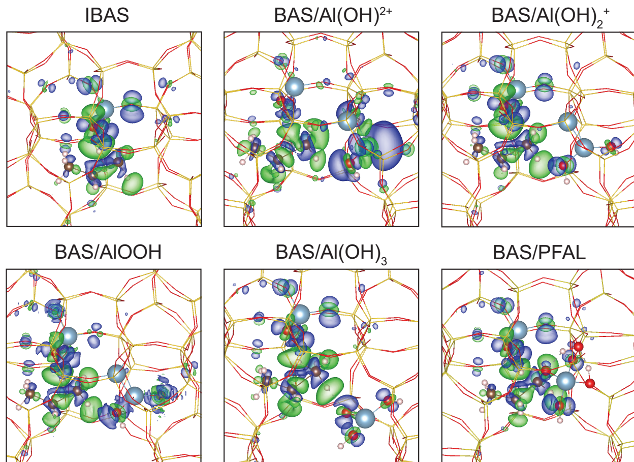
Figure 29. Electron density difference charge of TS of propane cracking reactions on various active sites, the value of isosurface is 0.002 au. The blue color represents accumulation of charge and the green color represents depletion of charge.
