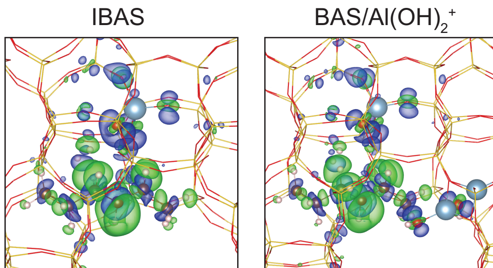
Figure 41. Electron density difference charge of TS of hexane dehydrogenation reactions on various active sites, the value of isosurface is 0.002 au. The blue color represents accumulation of charge and the green color represents depletion of charge.
