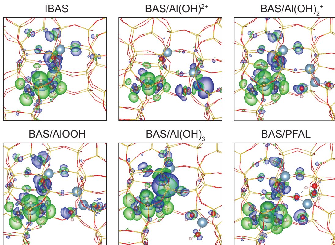
Figure 34. Electron density difference charge of TS of propane dehydrogenation reactions on various active sites, the value of isosurface is 0.002 au. The blue color represents accumulation of charge and the green color represents depletion of charge.
