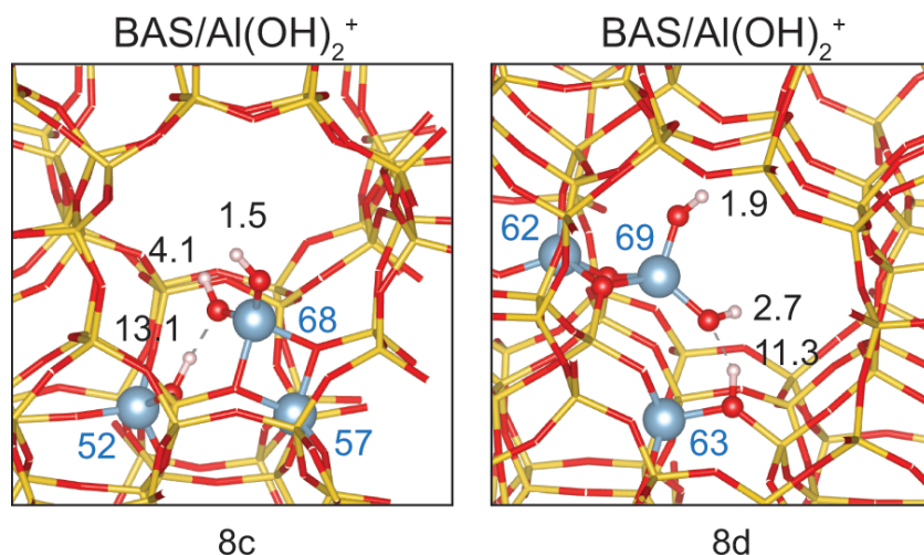
Figure 10. Optimized structures of synergistic sites \text{BAS}/\text{Al}(\text{OH})_2^+ and their DFT-calculated ^1\text{H} NMR and ^{27}\text{Al} NMR stabilized at 8c) sinusoidal channel; 8d) straight channel.
