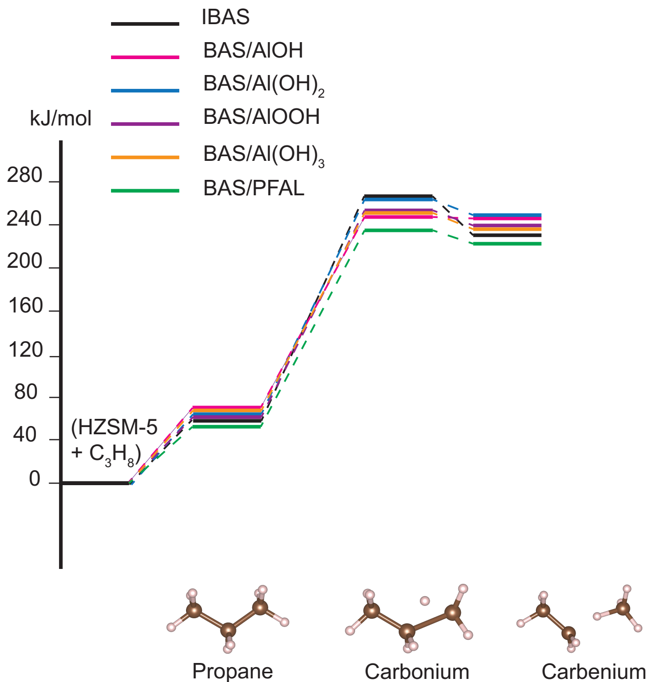
Figure 31. Free energy profiles of propane cracking on different active sites, calculated at 773 K.
