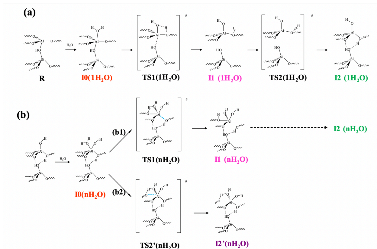
Scheme 1. Mechanism of framework atoms' hydrolysis, taken from ref. 17
