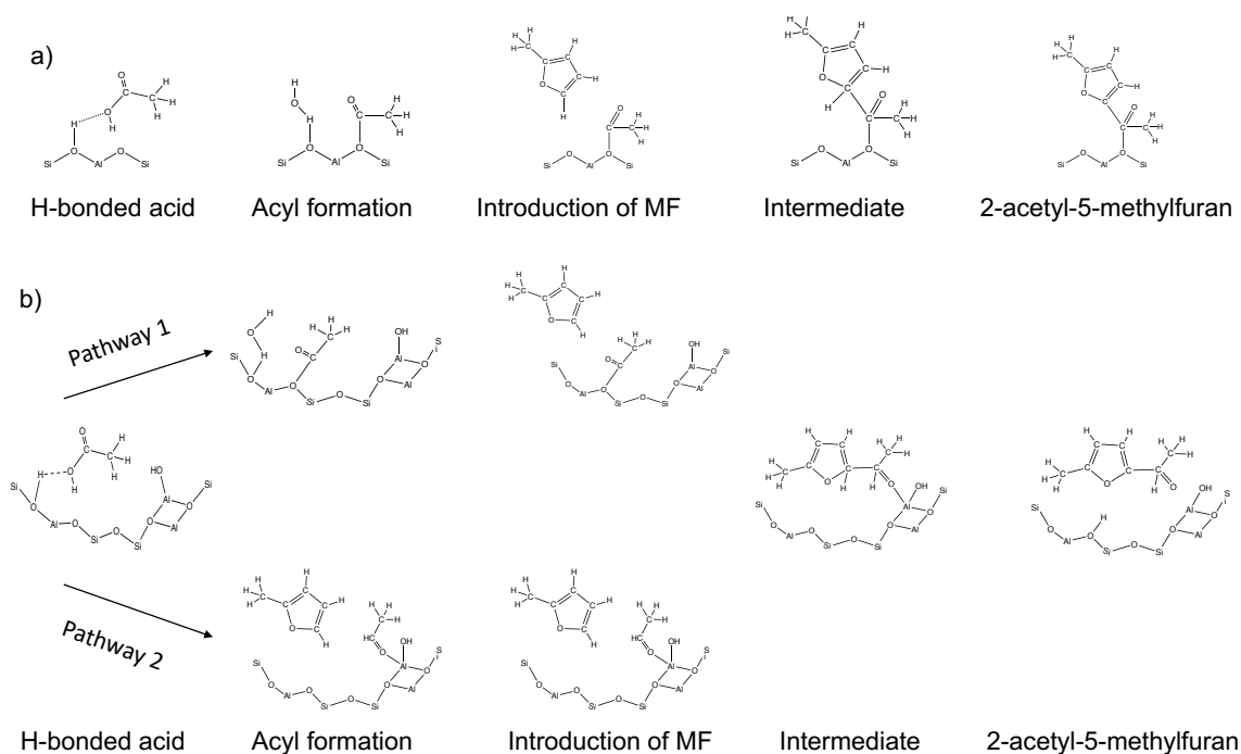
Scheme 4. Reaction pathways of acylation reaction of 2-Methylfuran with acetic acid
