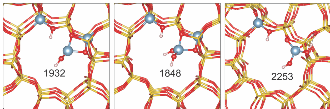
Figure 25. The numbers present the DPE of hydroxyl group in each structure. Units are kJ/mol.
