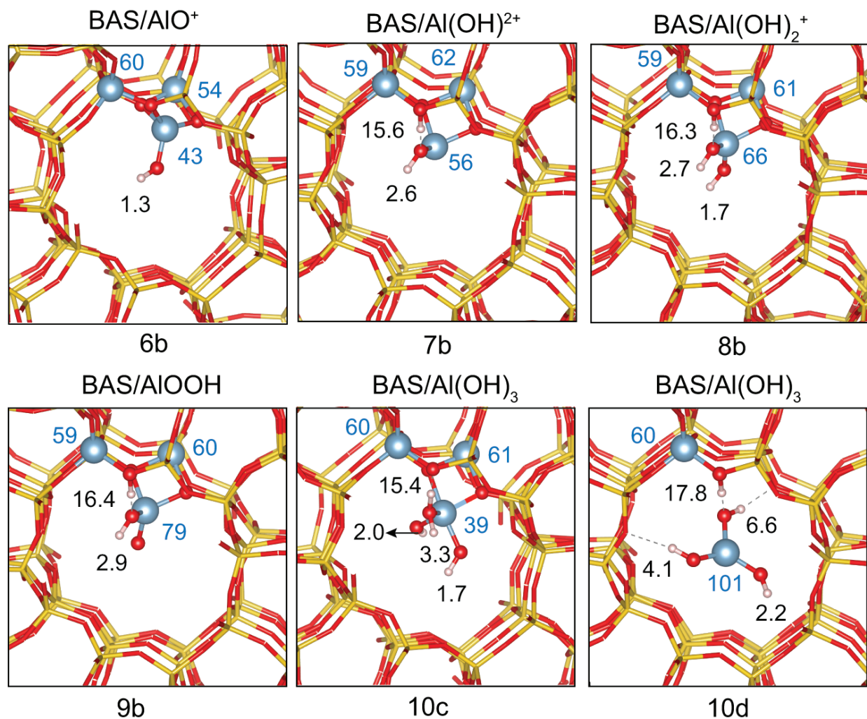
Figure 9. Optimized structures of a variety of synergistic sites BAS/EFAL species stabilized at the intersection and their DFT-calculated 1 H NMR and 27 Al NMR. In these synergistic sites, BASs form hydrogen bonds with EFAL. Black numbers: 1 H NMR and blue numbers: 27 Al NMR.
