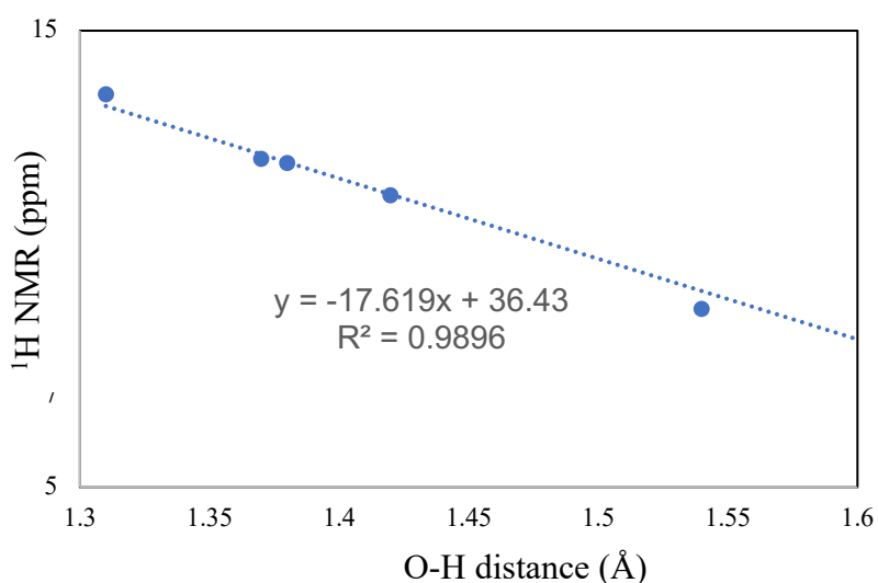
Figure 11. Linear relationship between the O-H bond distance and ^1\text{H} NMR of proton in synergistic sites.
