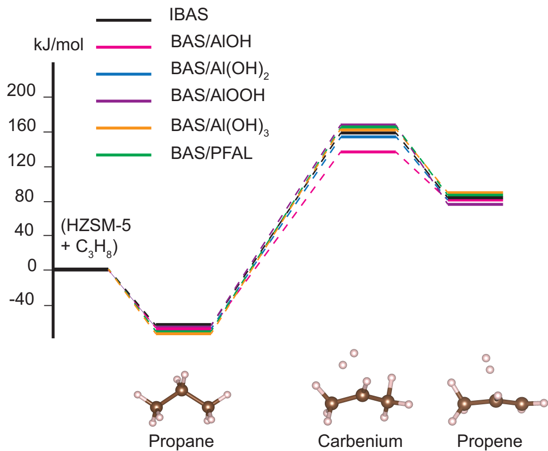
Figure 32. Energy profiles of the propane dehydrogenation reaction on different active sites.
