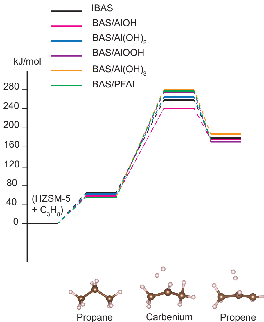
Figure 35. Free energy profiles of propane dehydrogenation reaction on different active sites, calculated at 775 K.
