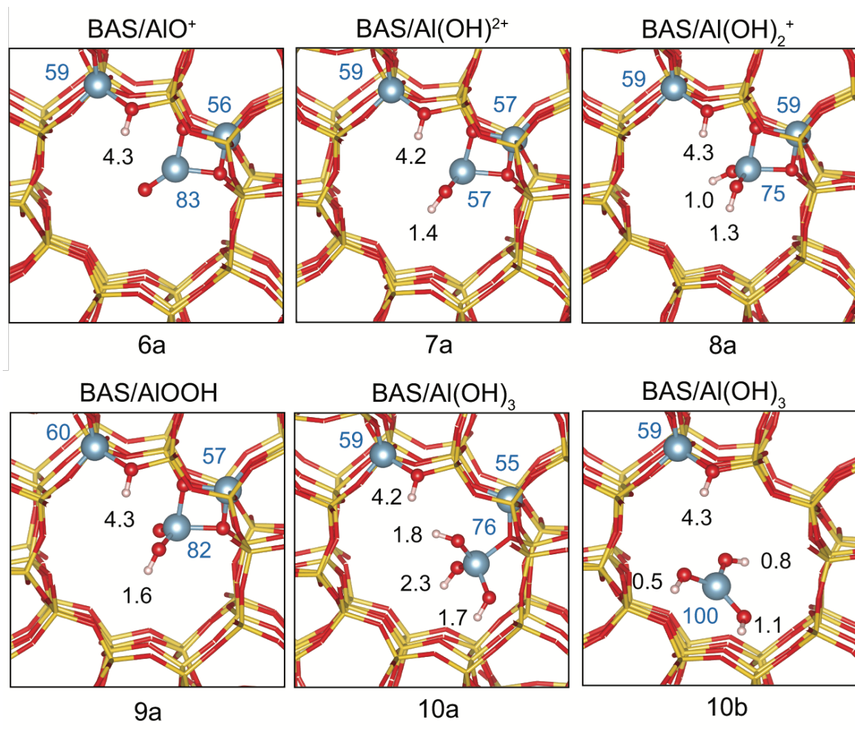
Figure 8. Optimized structures of a variety of synergistic sites BAS/EFAL species stabilized at the intersection and their DFT-calculated ^1\text{H} NMR and ^{27}\text{Al} NMR. In these synergistic sites, EFAL and BAS do not form hydrogen bonds. Black numbers: ^1\text{H} NMR and blue numbers: ^{27}\text{Al} NMR.
