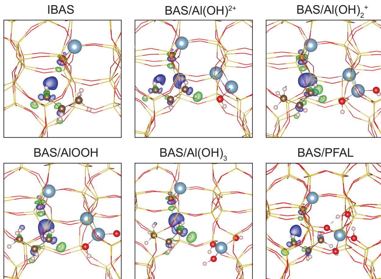
Figure 28. Electron density difference charge of propane at adsorption state on various active sites, the value of isosurface is 0.002 au. The blue color represents accumulation of charge and the green color represents depletion of charge.
