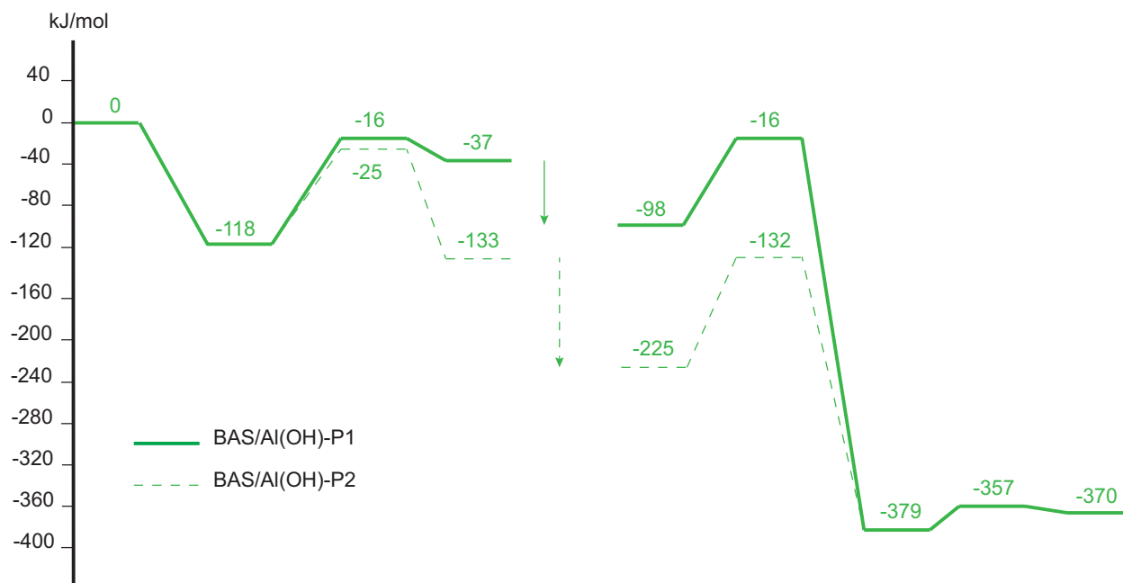
Figure 44. Energy profile of acylation of 2-MF with acetic acid on BAS with the presence of EFAL \text{Al}(\text{OH})_2^+ in proximity. The solid line represents reaction pathway 1 and dash line represents reaction pathway 2.
