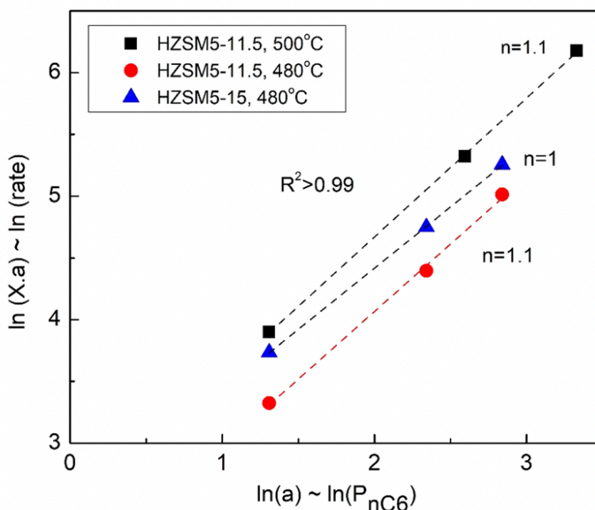
Figure 42. Determination of order of n-hexane cracking reaction, where a is the mole percent of n-hexane in the loop and X is the conversion of the reaction, taking from ref. 25
