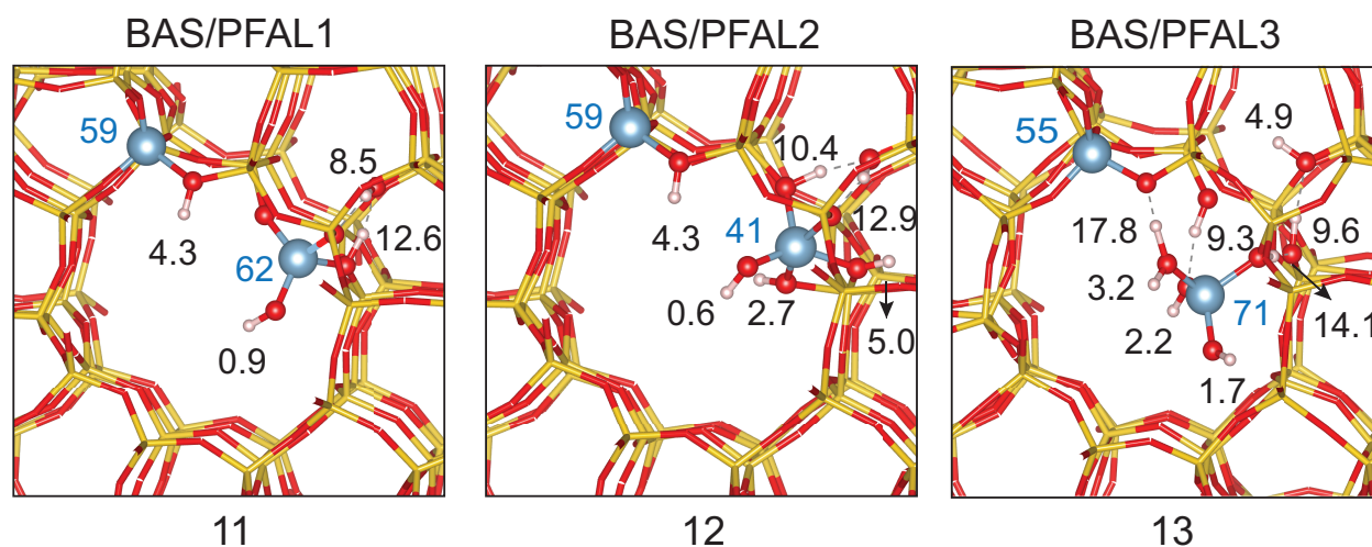
Figure 12. Optimized structures of synergistic sites BAS/PFAL species stabilized at the intersection and their DFT-calculated ^1\text{H} NMR and ^{27}\text{Al} NMR.
