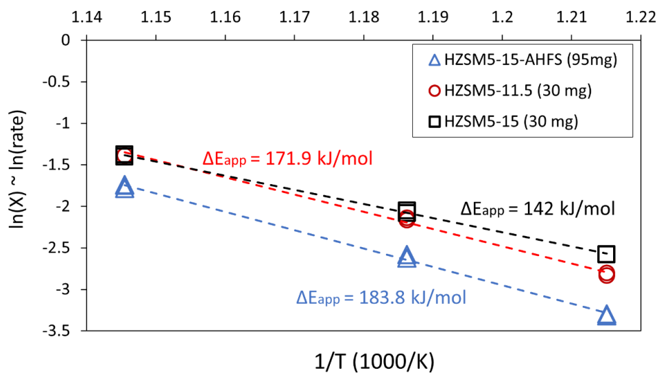
Figure 38. Estimation of apparent activation enthalpy of propane reactions on MFI zeolites.
