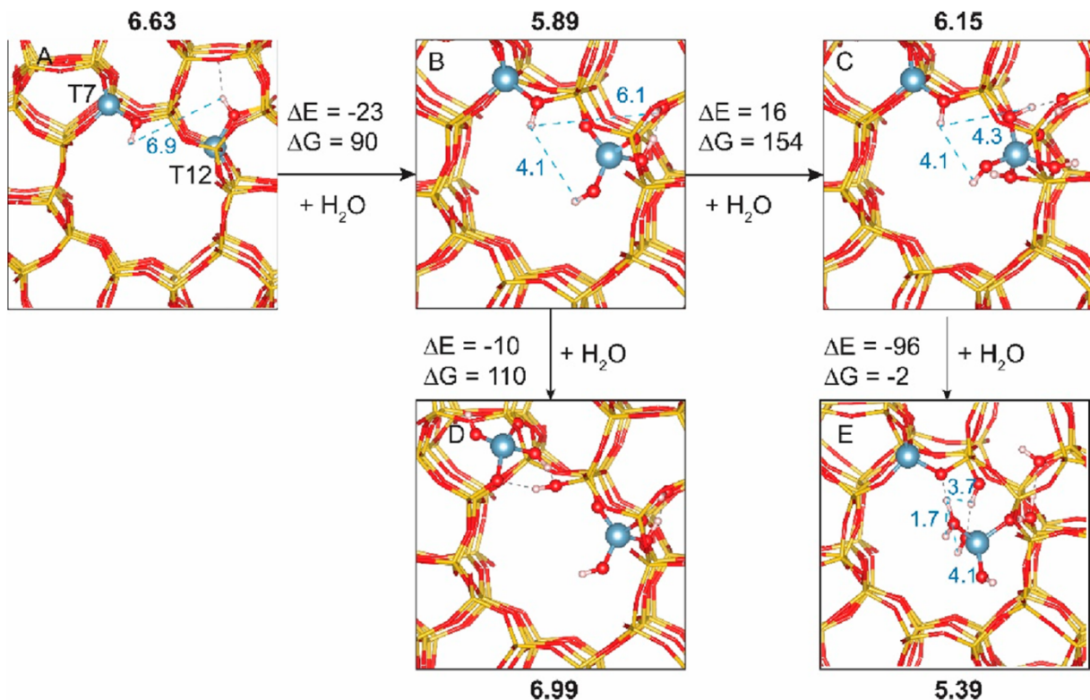
Figure 16. DFT calculations for model hydrolysis of (a) an Al(IV)-1/Al(IV)-1 pair, resulting in (b) an Al(IV)-1/Al(IV)-2 framework pair. Possible structures resulting from additional hydrolysis are shown in (c-e). Total energies and free energies are calculated with an ideal gas reference for water. The Al-Al internuclear distances (in Å) are shown in bold text above or below each structure, and H-H distances are shown in blue within each figure. 36
