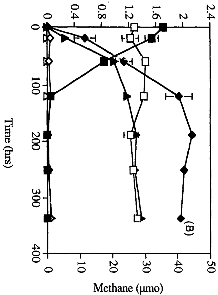
Cyclohex-1-ene carboxylate, acetate/3 (mM)
