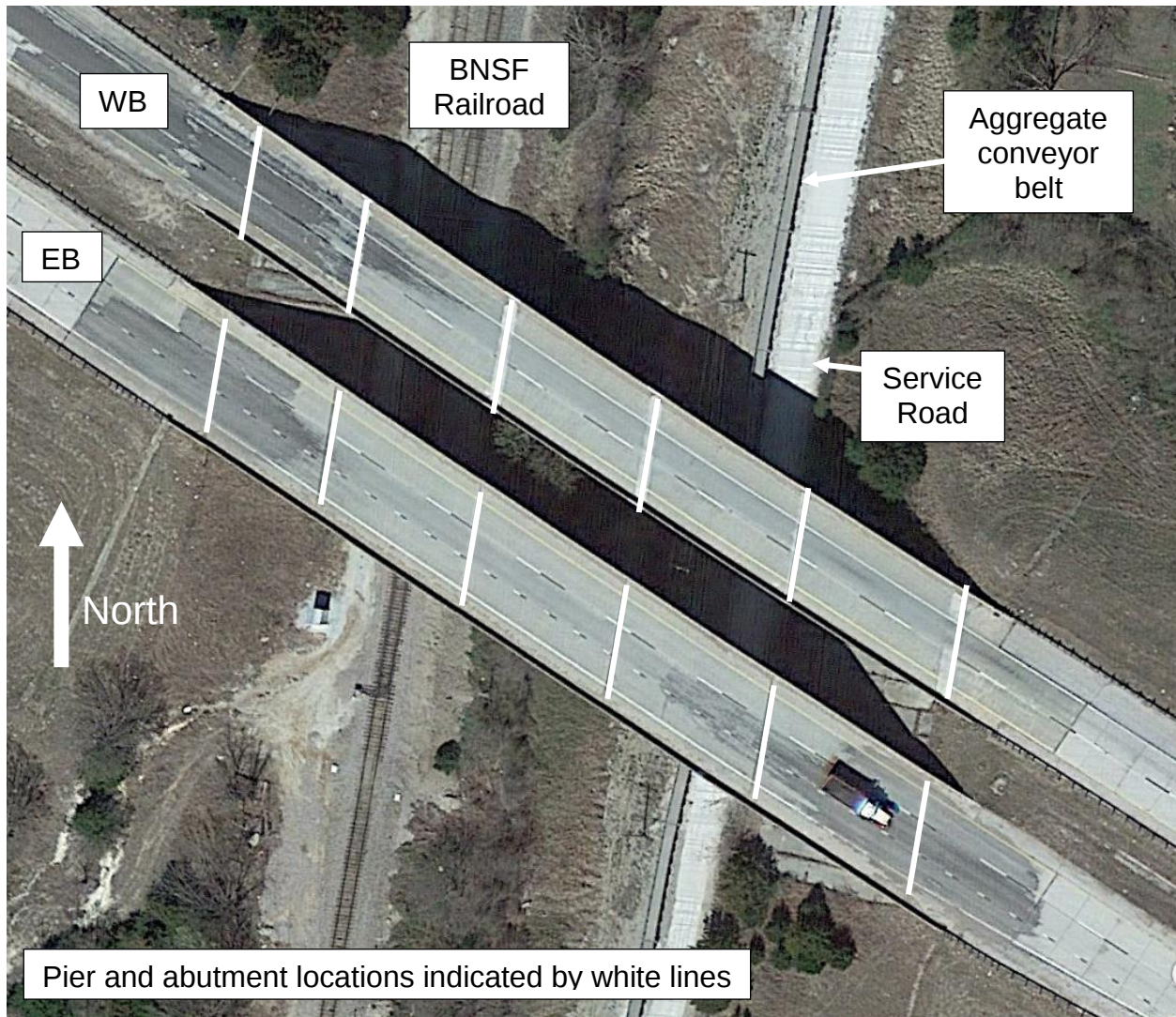
Figure 100. SH-3 over BNSF Railroad; aerial overview
