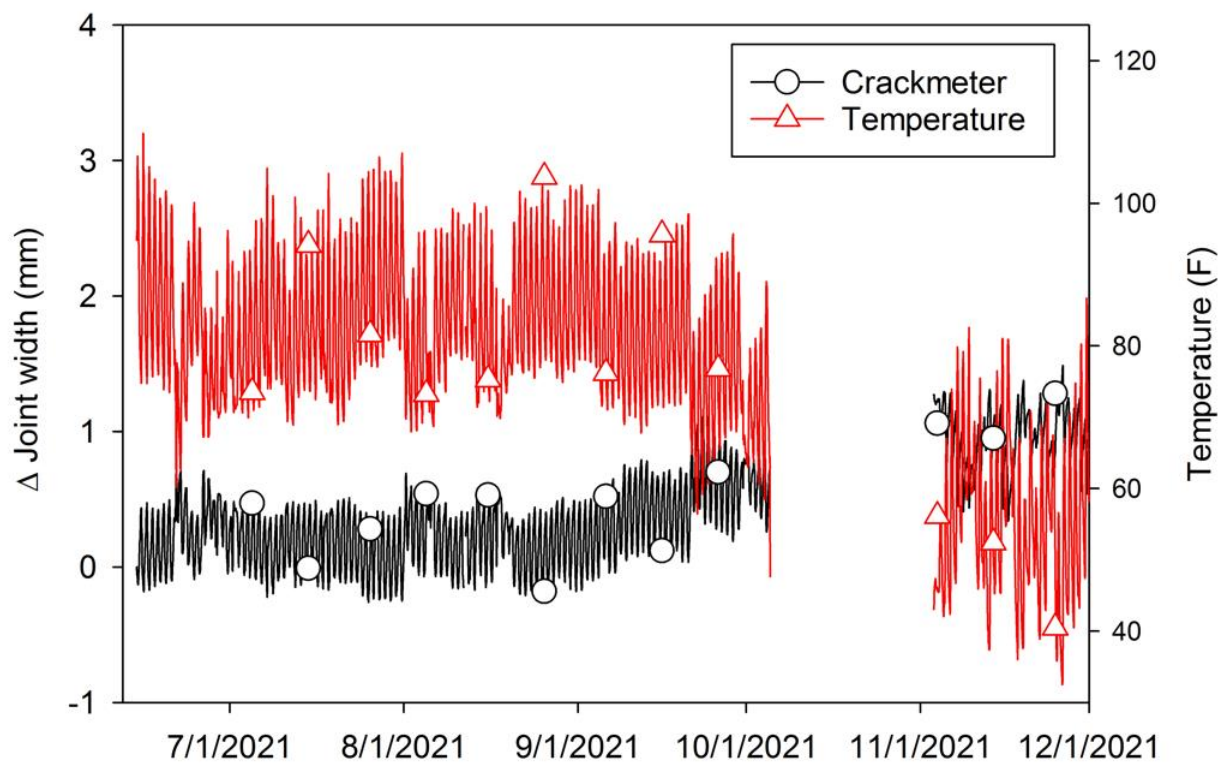
Figure 59. 19th Street over I-35 pressure relief joint width: East approach south doweled joint
