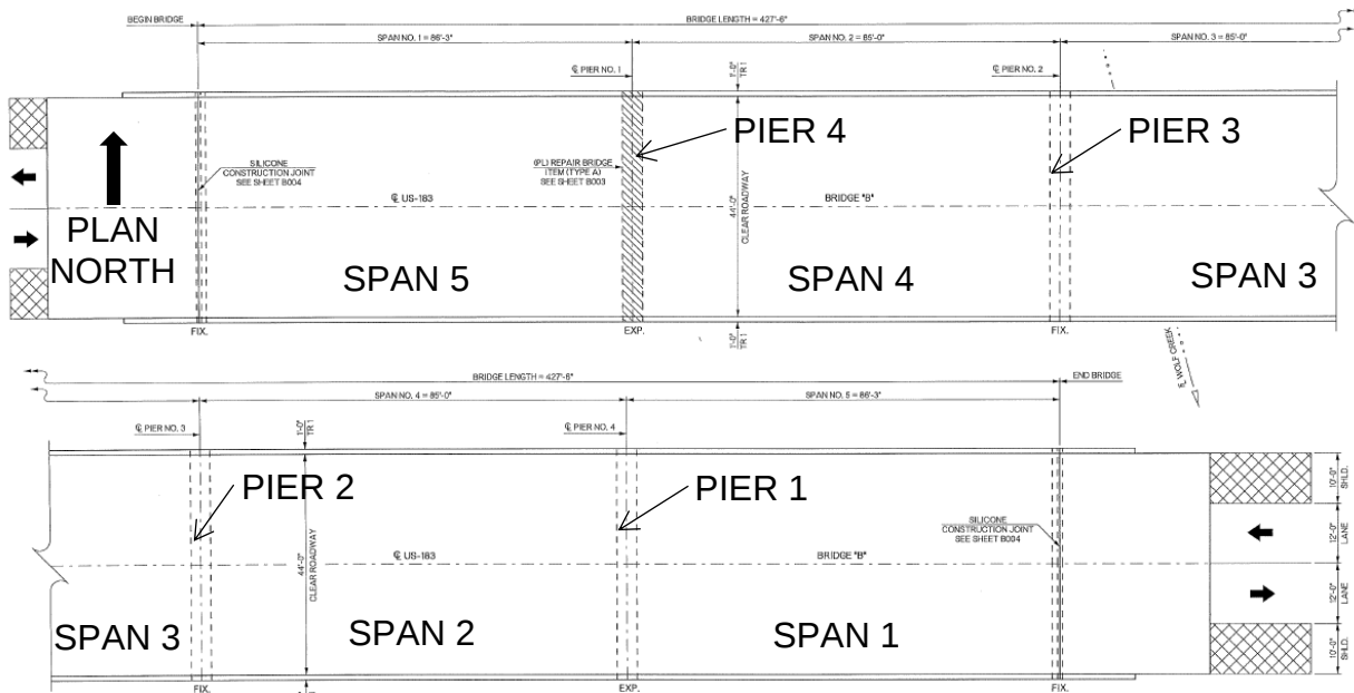
Figure 83. Plan view of U.S. 183/412 over Wolf Creek bridge
