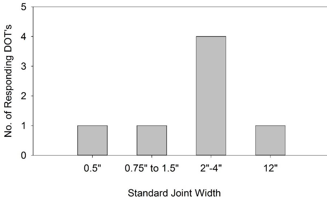
Figure 16. Pressure Relief Joint Width – Rehabilitation
