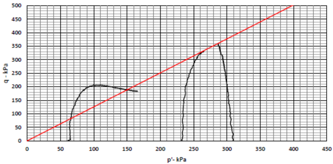
p'-q Diagram
