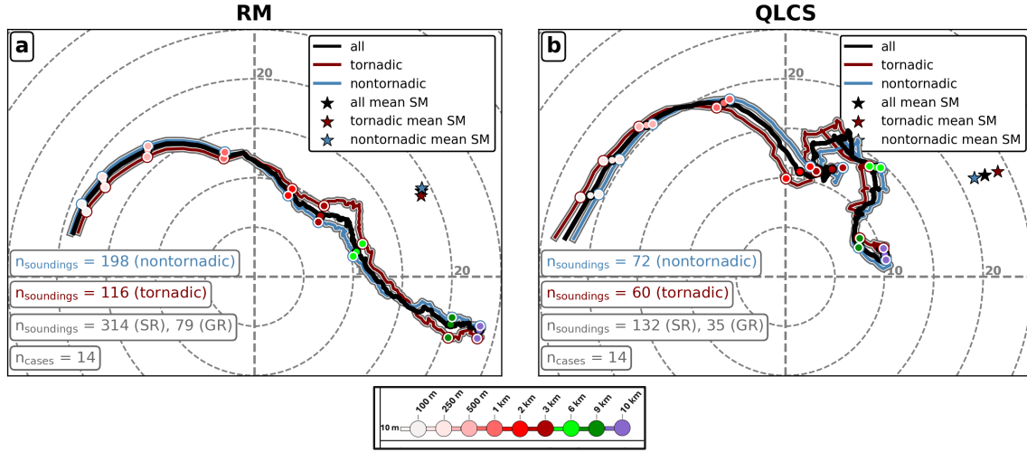
Figure 3.9: Composite SR hodographs of (a) RM and (b) QLCS environments where both a tornadic and nontornadic mesocyclone are present in the inflow of the sounding. The RM and QLCS mode classifications are the same as in Fig. 3.1. The solid black line “all” is the composite SR hodograph using all mesocyclones present in the mixed tornadic and nontornadic environment. The blue hodograph is created using the nontornadic mesocyclones and the red hodograph is for the tornadic mesocyclones. The colored dots to represent the height levels are the same as in Fig.3.1 and shown in the legend, with all mesocyclones having a black outline, tornadic having a red outline, and nontornadic having a blue outline. The mean storm motion (SM) is plotted on the hodograph with a star and color coded as the hodographs are. The n_{\text{cases}} and n_{\text{soundings}} (GR) will remain the same, as each sounding is required to have both a tornadic and nontornadic mesocyclone. The n_{\text{soundings}} (SR) varies because there may be multiple tornadic and/or nontornadic mesocyclones associated with one sounding. The SR n_{\text{soundings}} included in the tornadic composite is shown in red and the n_{\text{soundings}} included in the nontornadic composite is shown in blue.
