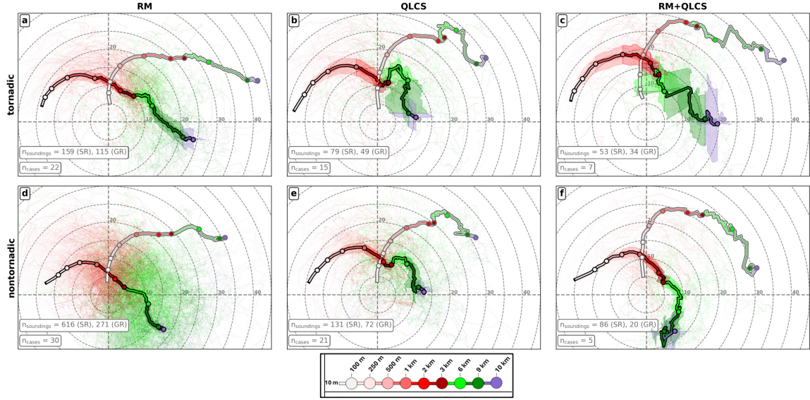
Figure 3.1: Composite hodographs of (a, d) RM, (b, e) QLCS, and (c, f) RM+QLCS for (a-c) tornadic and (d-f) nontornadic mesocyclones. The soundings included in the RM composite requires only RM modes present within the search radius and inflow of the sounding, the QLCS composite requires only QLCS modes present, and the RM+QLCS composite required at least one mesocyclone of a RM mode and QLCS mode to be present. The modes in RM consist of storm modes 4-1, 5-1, 4-2, 5-2, 2-2, 4-3, and 5-3 (see Fig. 2.2) and modes in QLCS consist of storm modes 1-1, 1-2, and 2-1 (see Fig. 2.2). The n_{\text{soundings}} is displayed for both ground-relative (GR) and storm-relative (SR) composites while n_{\text{cases}} remains the same for both. The thin lines on each individual plot are all individual SR hodographs included in the composite, and the thicker lines are the composite (mean) of all individual hodographs, where the color-filled line with a white line on top and outlined in grey is the GR composite hodograph and the color-filled line with a black outline is the SR composite hodograph. The number of hodographs making up each composite is found in grey text in the bottom left corner of each plot. The hodograph coloring follows the standard National Weather Service (NWS) colors, where 0–3-km is red, 3–6-km is lime green, 6–9-km is dark green, and 10-km and greater is purple, with additional resolution within the red 0–3-km layer due to its relevance for tornado-related processes and forecasting.
