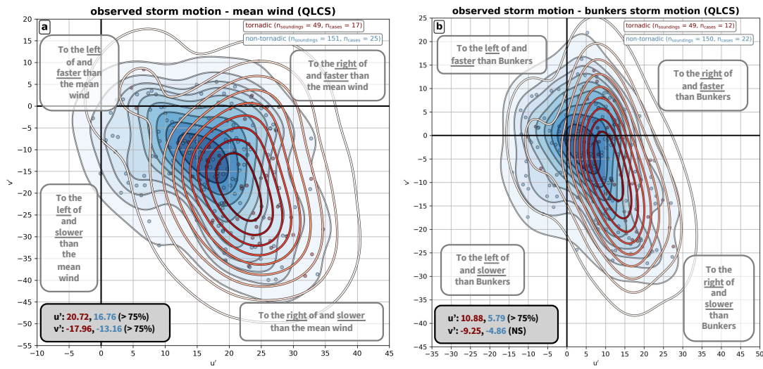
Figure 3.11: KDE plots of tornadic (reds with no fill) and nontornadic (color-filled blues) observed storm motion deviation from the a) mean wind (SH6km) and from b) Bunkers right storm motion for all QLCS modes (modes 1-1, 1-2, and 2-1, see Fig. 2.2). The other aspects of the plot are the same as the panels described in Fig. 3.10.
