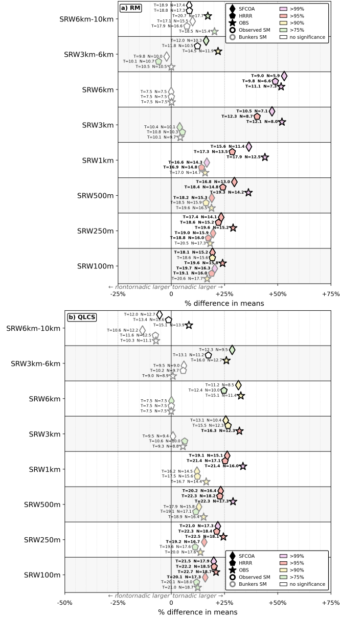
Figure 4.16: The same as in Fig. 4.6, but for SRW. The SRW parameters included are (from bottom to top): SRW100m, SRW250m, SRW500m, SRW1km, SRW3km, SRW6km, SRW3km-6km, and SRW6km-10km. The one addition here from the contents in Fig. 4.6 is an additional set of symbols representing the means using Bunkers storm motion since SRW is a storm-relative parameter. Black edge coloring on the symbol represents the tornadic vs. nontornadic comparisons when observed storm motion is used and gray edge coloring represents the tornadic vs. nontornadic comparisons when Bunkers storm motion is used.
