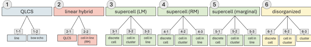
Figure 2.2: Flowchart of storm mode based on Fig. 2 of Smith et al. (2012).
