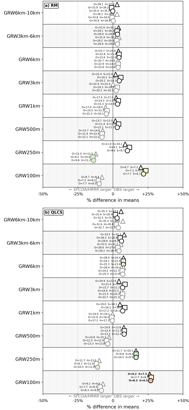
Figure 4.8: The same as in Fig. 4.5, but for GRW. The GRW parameters included are (from bottom to top): GRW100m, GRW250m, GRW500m, GRW1km, GRW3km, GRW6km, GRW3km-6km, and GRW6km-10km.
