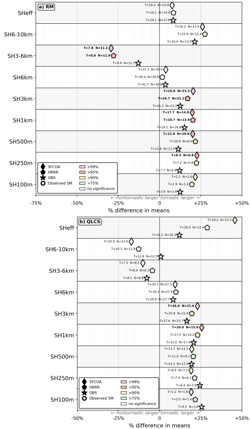
Figure 4.11: The same as in Fig. 4.6, but for shear. The shear parameters included are (from bottom to top): SH100m, SH250m, SH500m, SH1km, SH3km, SH6km, SH3km-6km, SH6km-10km, and SHEff.
