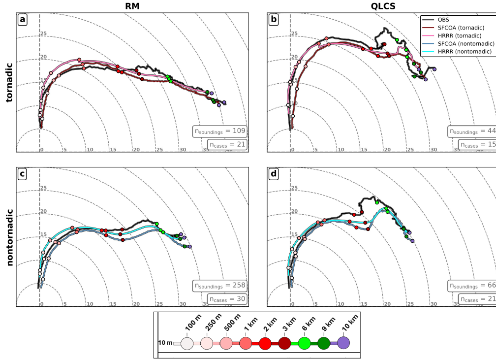
Figure 4.2: Composite ground-relative (GR) hodographs of (a) RM tornadic, (b) QLCS tornadic, (c) RM nontornadic, and (d) QLCS nontornadic mesocyclones. The soundings included in the RM composite requires only RM modes present within the search radius and inflow of the sounding and the QLCS composite requires only QLCS modes present. The modes in RM consist of storm modes 4-1, 5-1, 4-2, 5-2, 2-2, 4-3, and 5-3 and modes in QLCS consist of storm modes 1-1, 1-2, and 2-1 (see Fig. 2.2 and the associated text in Chapter 2 for more information on each storm mode). The number of hodographs making up each composite is found in gray text in the bottom left corner of each plot. The colored-coded circles indicate certain height levels, as shown in the legend.
