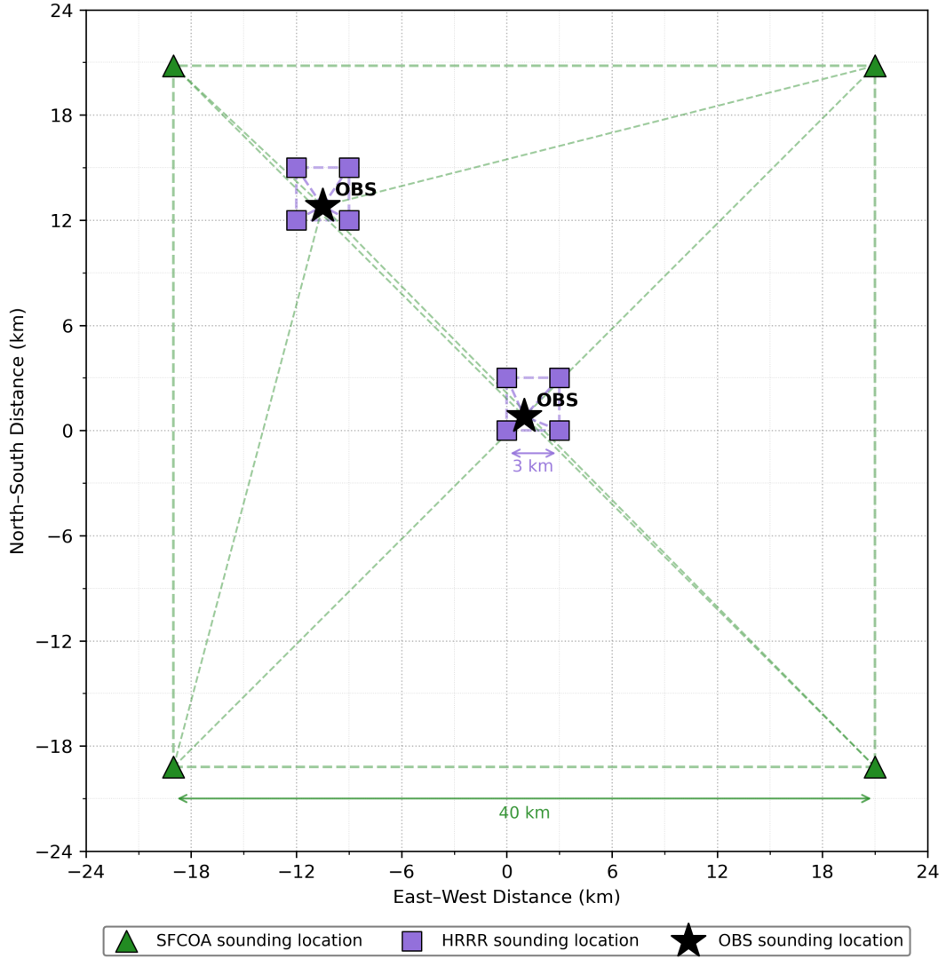
Figure 4.1: Schematic illustrating the grid point selection method for HRRR (purple squares, 3-km grid) and SFCOA (green triangles, 40-km grid) model profiles relative to two example OBS sounding locations (black stars). For each OBS sounding, profiles at the four surrounding model grid points are extracted at the hour before and after the OBS time. Dashed lines connect each sounding location to its four surrounding model grid points.
