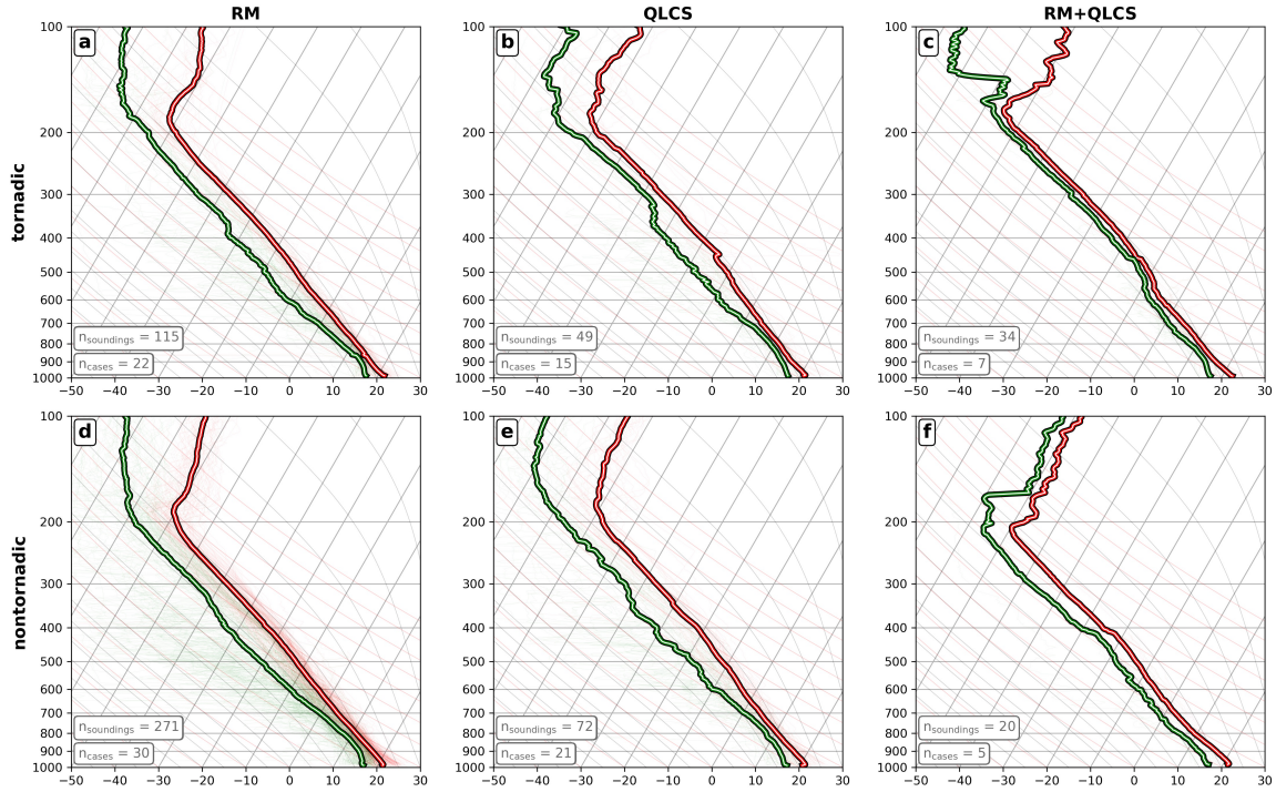
Figure 3.2: Composite skew-Ts of (a, d) RM, (b, e) QLCS, and (c, f) RM+QLCS for (a-c) tornadic and (d-f) nontornadic mesocyclones. The mode classifications are the same as in Fig.3.1. The thin red and green lines are each temperature and dew point profile, respectively, included in the composite. The thicker red and green lines with a black outline and a white line through the middle are the composite temperature and dew point profile, respectively.
