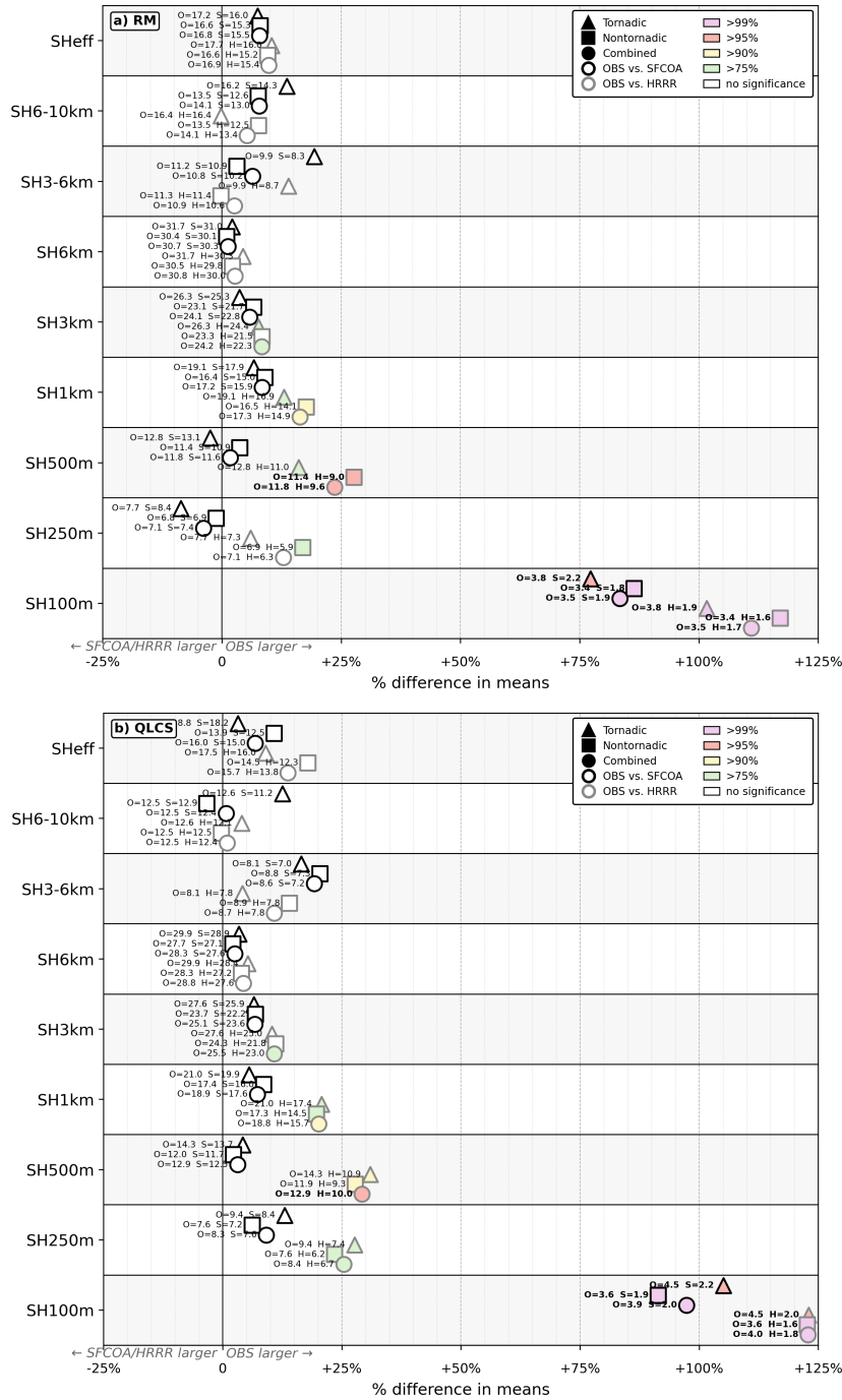
Figure 4.10: The same as in Fig. 4.5, but for shear. The shear parameters included are (from bottom to top): SH100m, SH250m, SH500m, SH1km, SH3km, SH6km, SH3km-6km, SH6km-10km, and SHEff.
