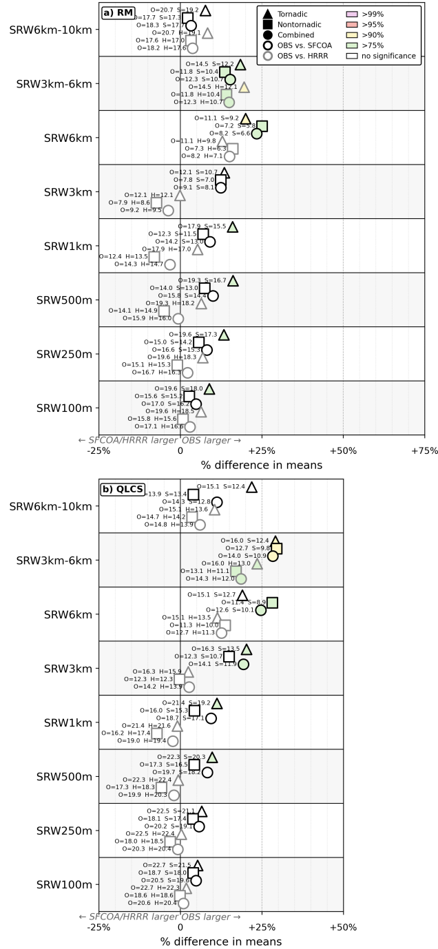
Figure 4.15: The same as in Fig. 4.5, but for SRW. The SRW parameters included are (from bottom to top): SRW100m, SRW250m, SRW500m, SRW1km, SRW3km, SRW6km, SRW3km-6km, and SRW6km-10km.
