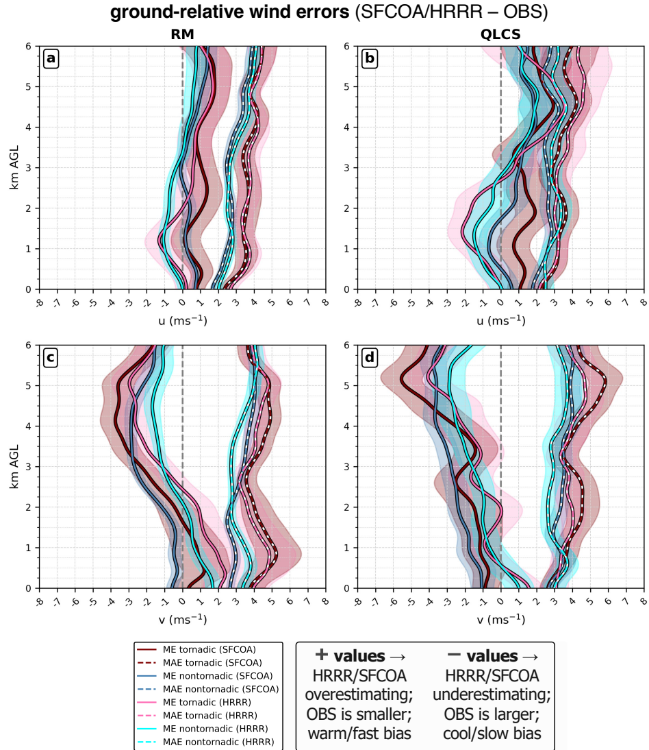
Figure 4.7: Same as Fig. 4.4, but for the errors in the ground-relative a-b) u component of the wind ( \text{ms}^{-1} ) and c-d) v component of the wind ( \text{ms}^{-1} ).
