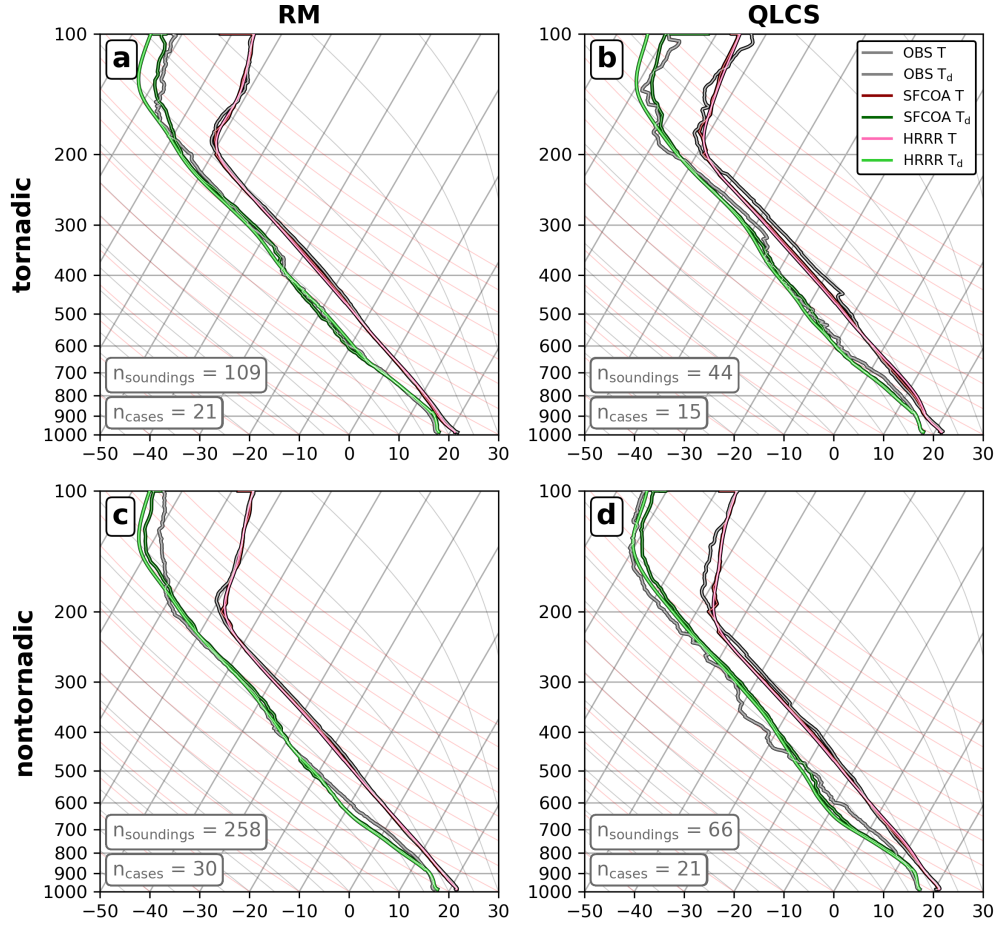
Figure 4.3: Composite skew-Ts of (a) RM tornadic, (b) QLCS tornadic, (c) RM nontornadic, and (d) QLCS nontornadic mesocyclones. The soundings included in the RM and QLCS modes are as described in Fig. 4.2. Since there are no SR thermodynamic parameters, the n_{\text{soundings}} and n_{\text{cases}} will match the GR values in Fig. 4.2. The grey outlined lines are the temperature (T) and dew point ( T_d ) for OBS. The SFCOA T is shown in maroon while HRRR T is shown in pink. The SFCOA T_d is shown in dark green while HRRR T_d is shown in lime green.
