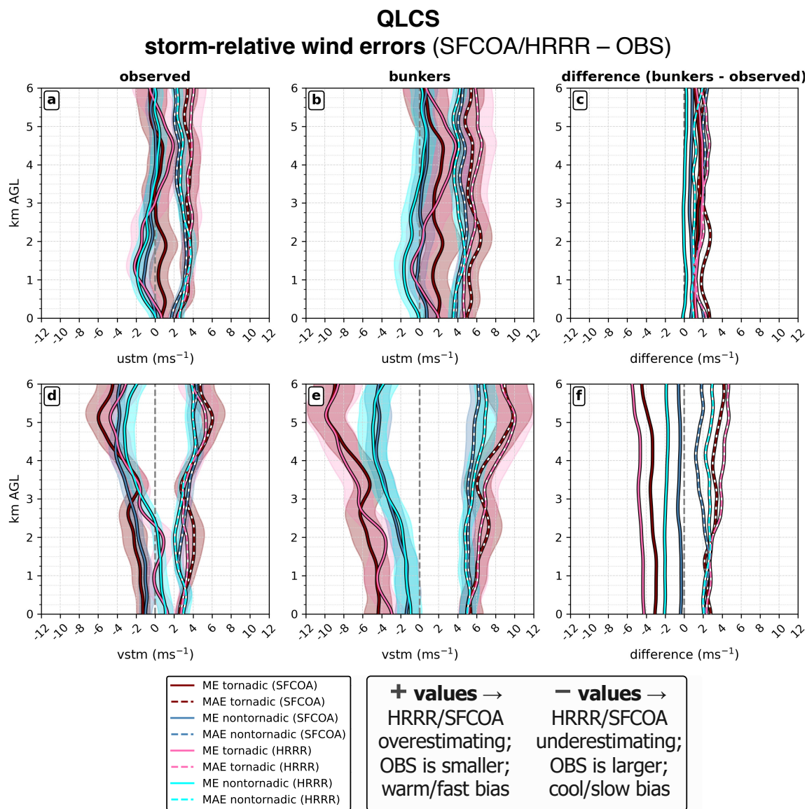
Figure 4.14: The same as in Fig. 4.13, but for QLCS.
