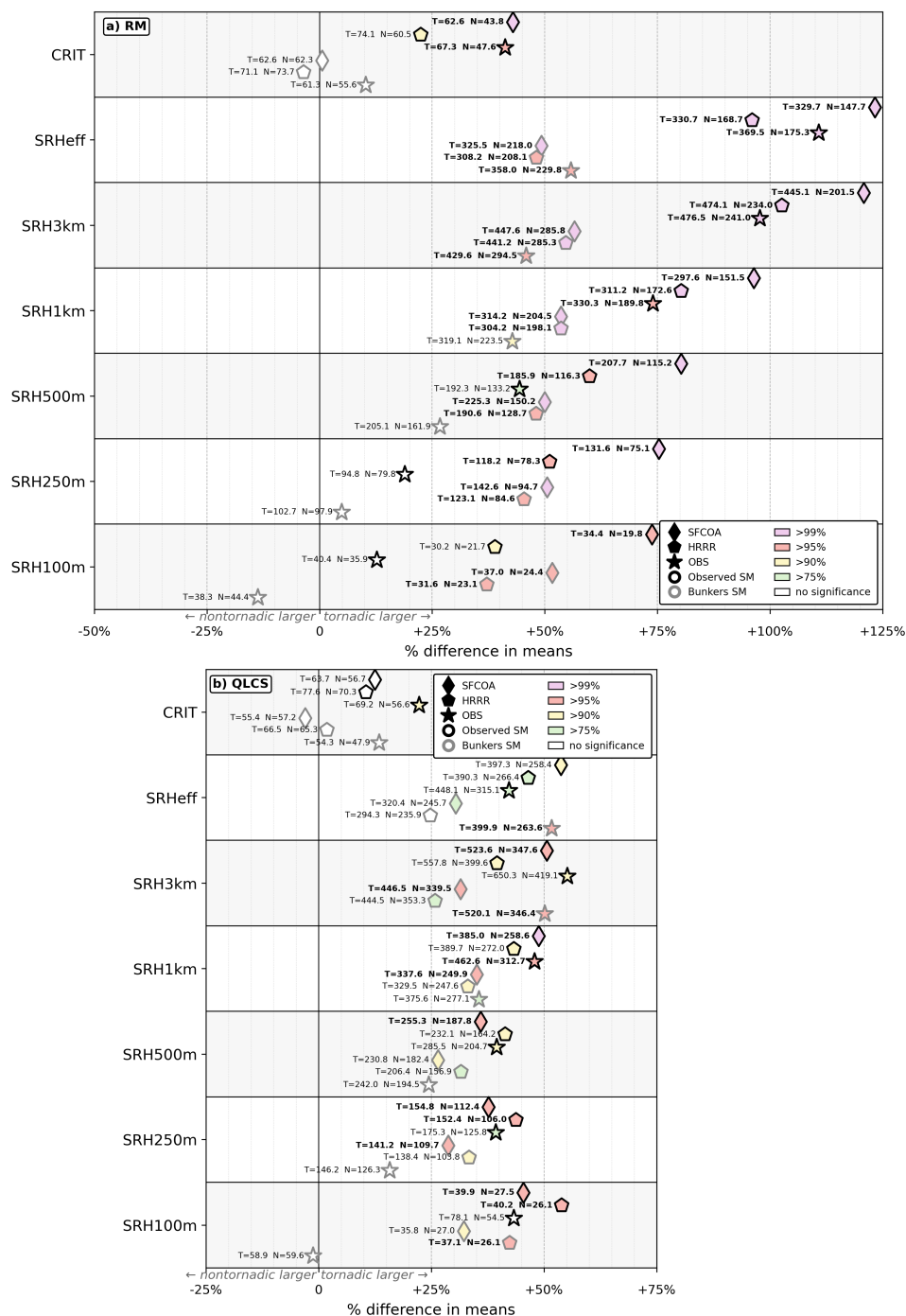
Figure 4.18: The same as in Fig. 4.6, but for SRH. The SRH parameters included are (from bottom to top): SRH100m, SRH250m, SRH500m, SRH1km, SRH3km, SRHeff, and CRIT. Both Bunkers storm motion and observed storm motion mean calculations are included as in Fig. 4.16.
