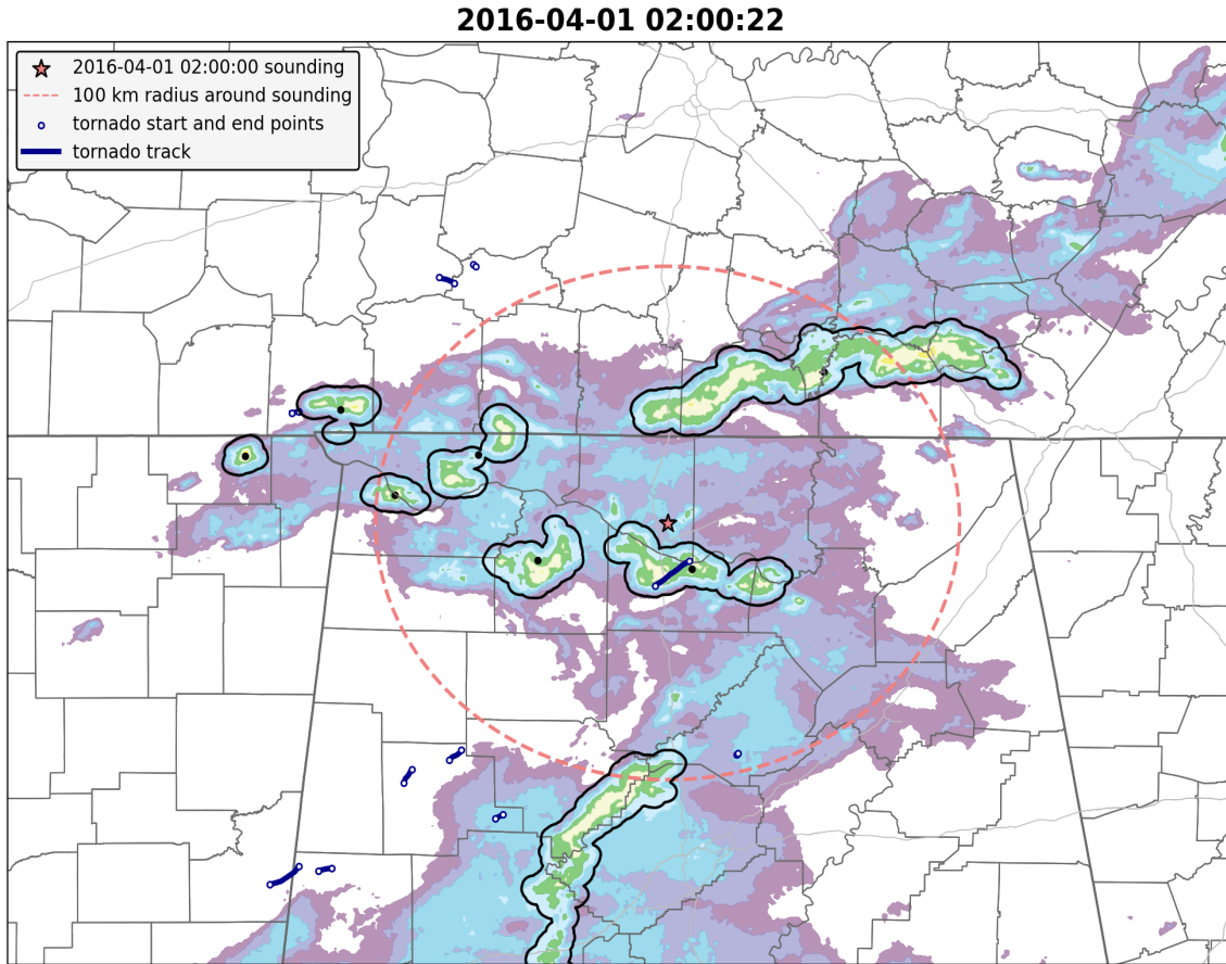
Figure 2.3: MRMS composite reflectivity at 02:00:00 UTC and the associated 02:00:00 UTC sounding from Huntsville, AL (indicated by the red star) on 1 April 2016. The red dotted ring surrounding the sounding represents the 100-km radius where storm objects are considered for the analysis. The black outline surrounding each storm is the objectively identified storm object and the black dot at the center is the center point of the object. The blue lines represent the tornadoes that occurred on the event day with a white circle marking their start and end points.
