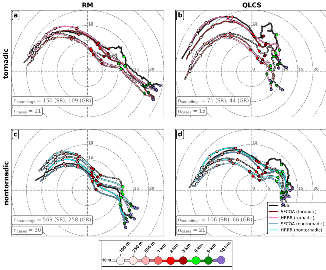
Figure 4.12: Same as in Fig. 4.2, but for SR hodographs, using both observed storm motion and Bunkers storm motion. The n_{\text{soundings}} is displayed for both ground-relative (GR) and storm-relative (SR) while n_{\text{cases}} remains the same for both. While there is no GR hodograph plotted, this number tells us the number of unique hodographs in each composite. The SR n_{\text{soundings}} minus the SR n_{\text{soundings}} gives the number of hodographs that are used more than once, but for a different mesocyclone (with a different storm motion). The solid colored lines represent the composite mean SR hodographs using observed storm motion, and the colored hodographs with white dashes overlaid are the SR hodographs using Bunker storm motion.
