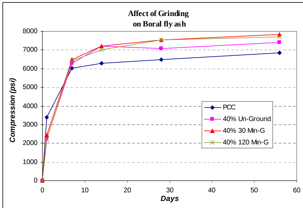
Figure 5.24 Effect of grinding duration on 40% Boral fly ash concrete
