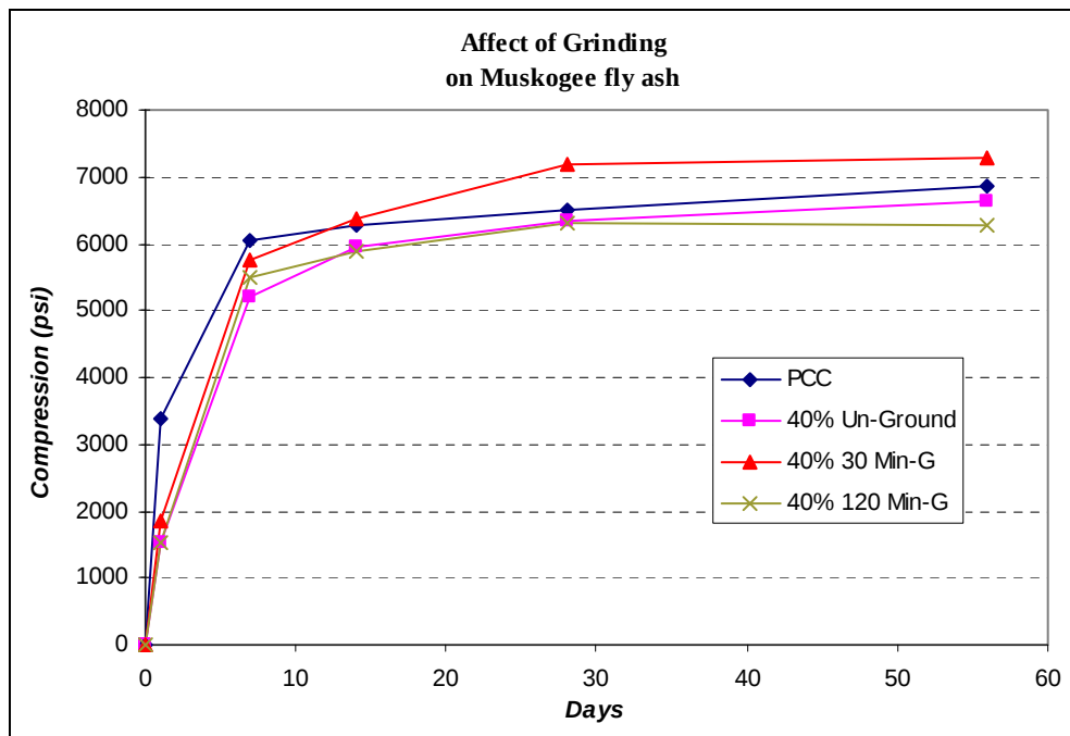
Figure 5.21 Effect of grinding duration on 40% Muskogee fly ash concrete
