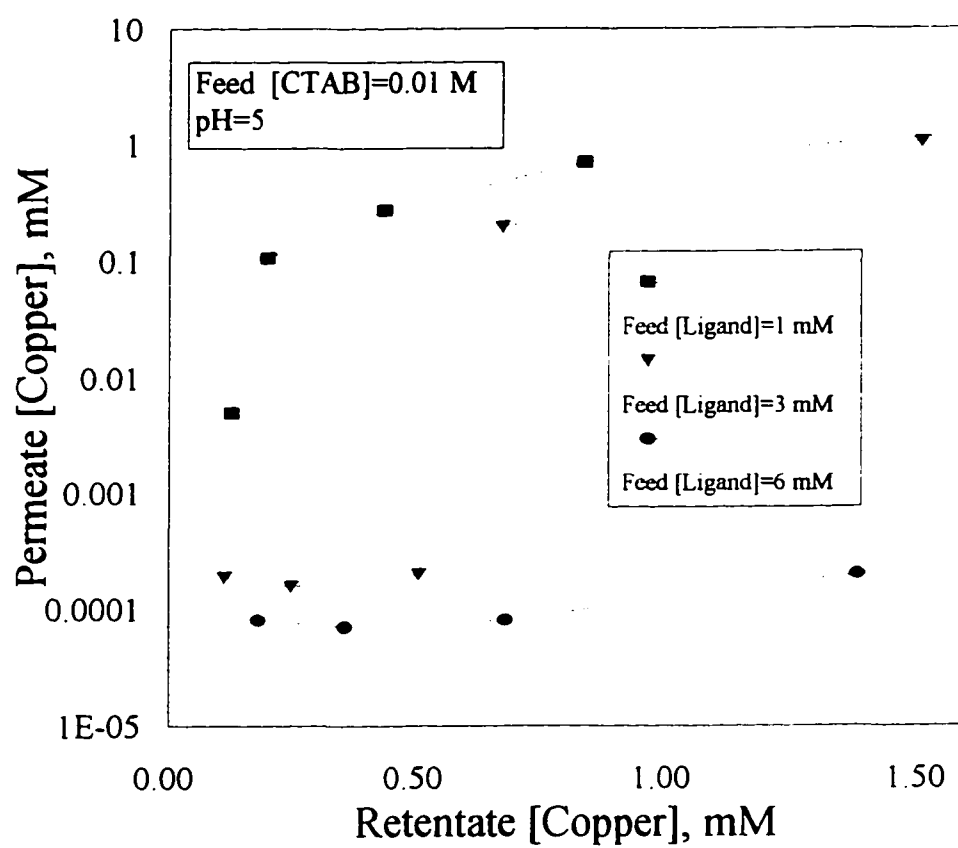
Figure I.5 Permeate [Copper] as a Function of Retentate [Copper]
