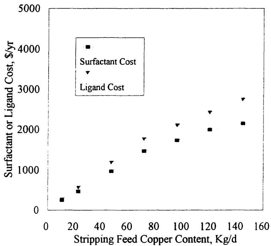
Figure II.17 Annual Cost of Surfactant and Ligand vs. Stripping Feed Copper Content, Single Stage Stripping Ultrafiltration Unit
