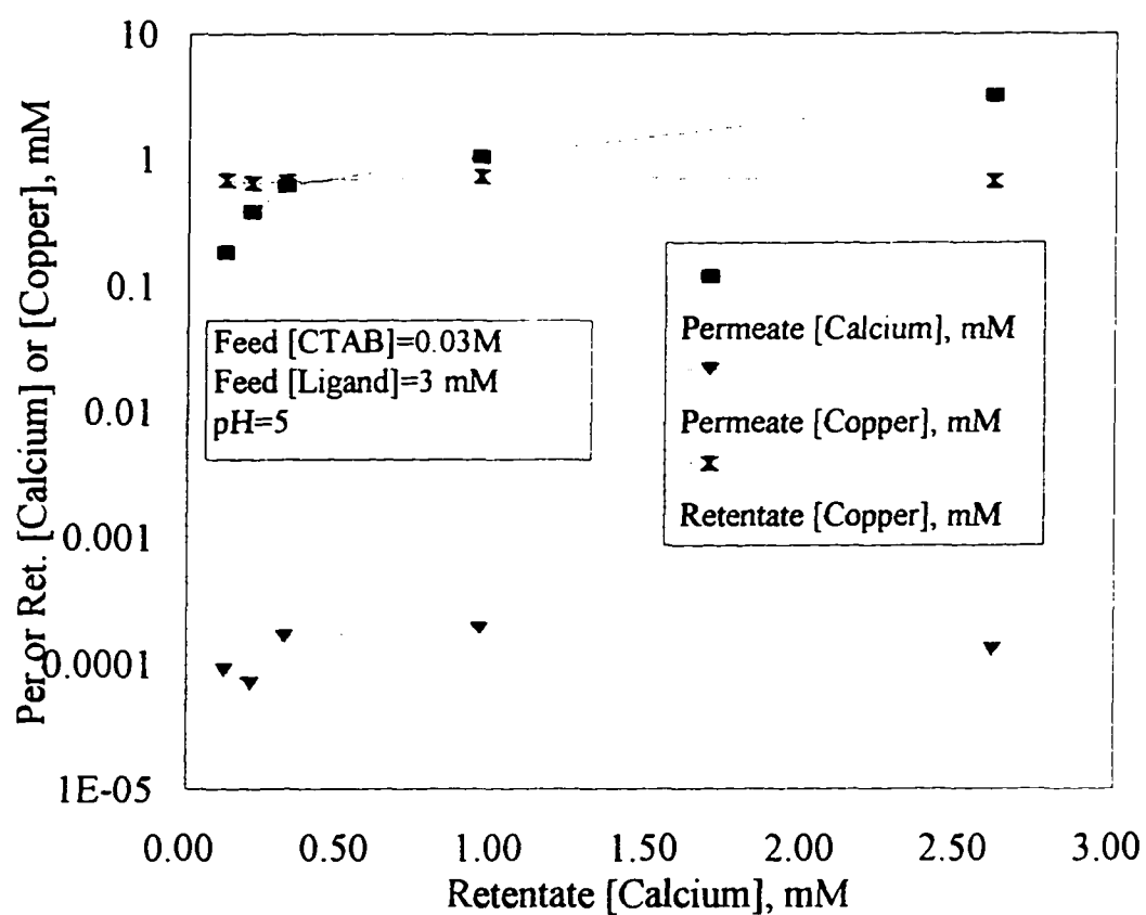
Figure I.11 Permeate or Retentate [Calcium] and [Copper] vs. Retentate [Calcium]
