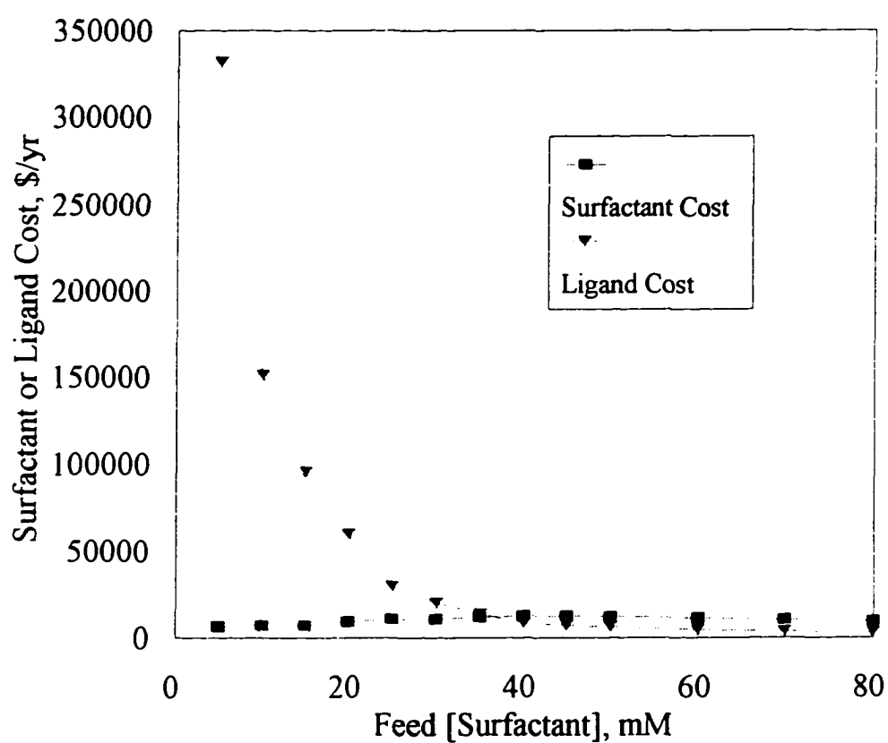
Figure II.5 Annual Cost of Surfactant or Ligand vs. Feed [Surfactant], Constant Feed [Ligand] and [Copper], Single Stage Ultrafiltration Unit
