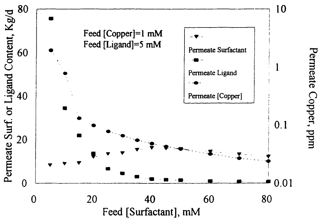
Figure II. 4 Surfactant and Ligand Losses in Permeate vs. Feed [Surfactant], Constant Feed [Ligand] and [Copper], Single Stage Ultrafiltration Unit
