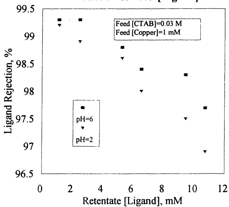
Figure I.12 Ligand Rejection as a Function of Feed [Ligand]
