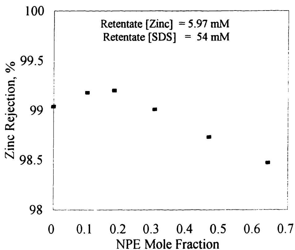
Figure III.14 Zinc Rejection vs. Mole Fraction NPE
