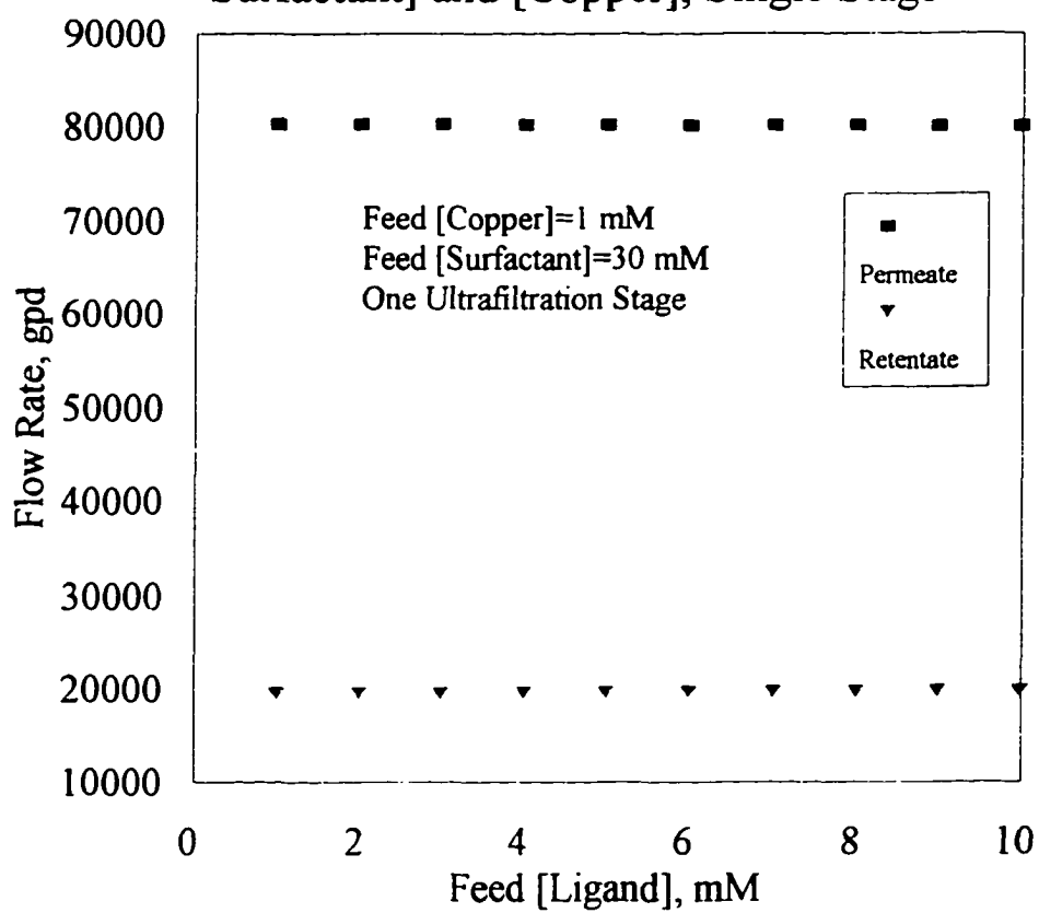
Figure II.6 Permeate or Retentate Flow Rate vs. Feed [Ligand], Constant Feed [ Surfactant] and [Copper], Single Stage
