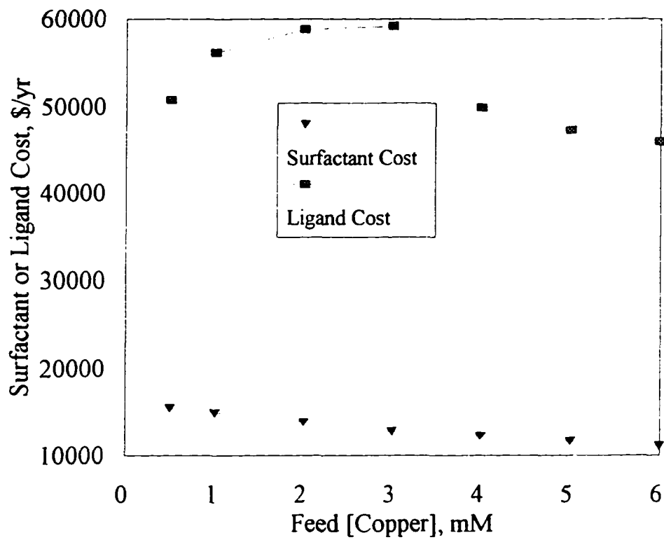
Figure II.14 Annual Cost of Surfactant and Ligand vs. Feed [Copper] with Variable Feed [Surfactant] and [Ligand] to maintain a Permeate [Copper]=4 ppm, Multistage Ultrafiltration Unit.
