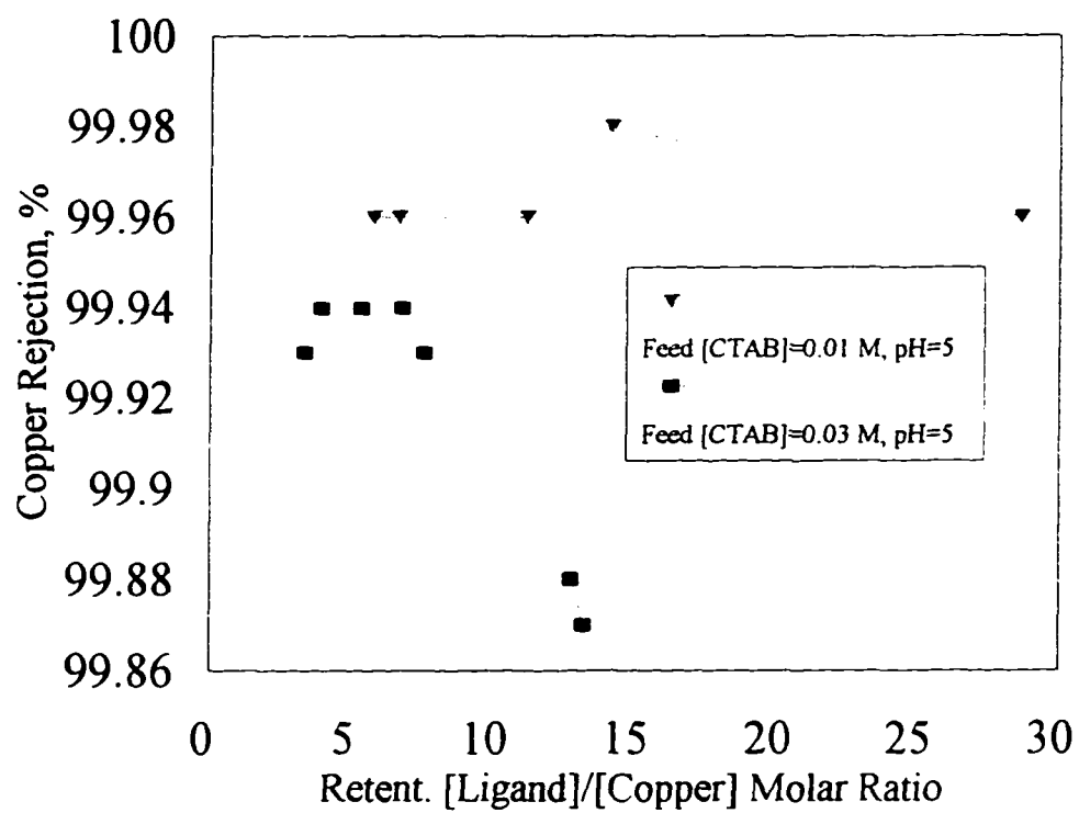
Figure I.9 Copper Rejection as a Function of Ligand/Copper Molar Ratio
