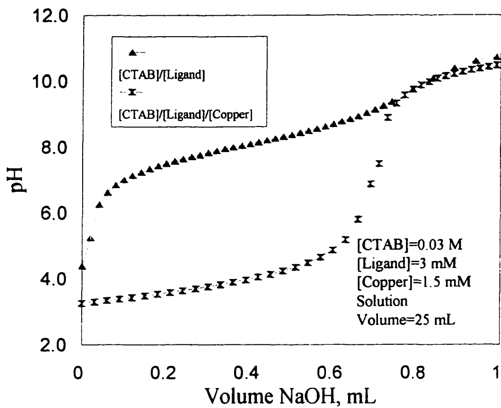
Figure I.4 Titration Results for CTAB/Ligand/Copper, 0.1 M NaOH
