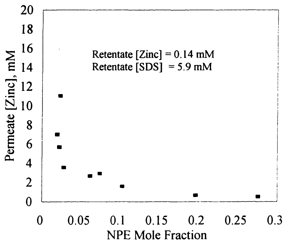
Figure III.17 Permeate Zinc vs. Mole Fraction NPE
