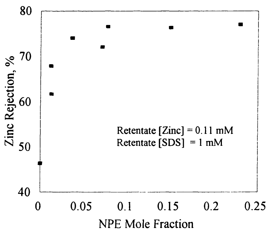
Figure III.8 Zinc Rejection vs. NPE Mole Fraction
