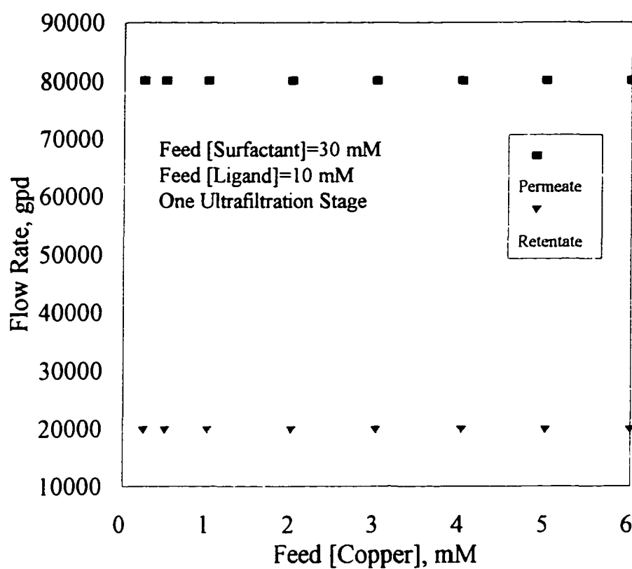
Figure II. 9 Permeate or Retentate Flow Rate vs. Feed [Copper], Constant Feed [Surfactant] and [Ligand], Single Stage Ultrafiltration Unit
