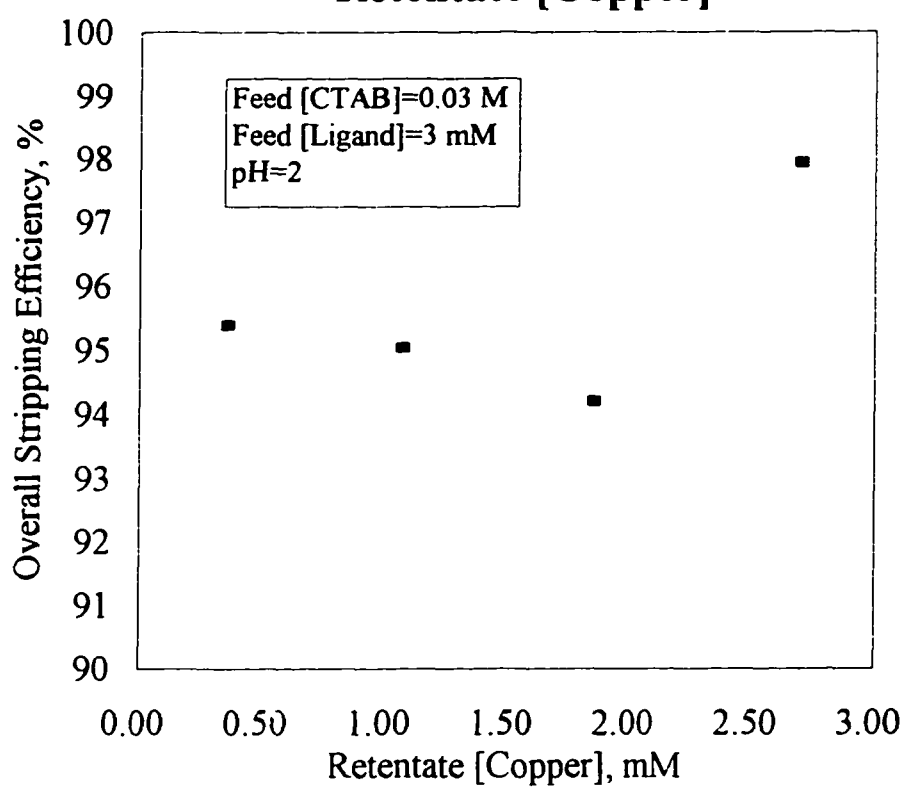
Figure I.15 Overall Stripping Efficiency vs. Retentate [Copper]
