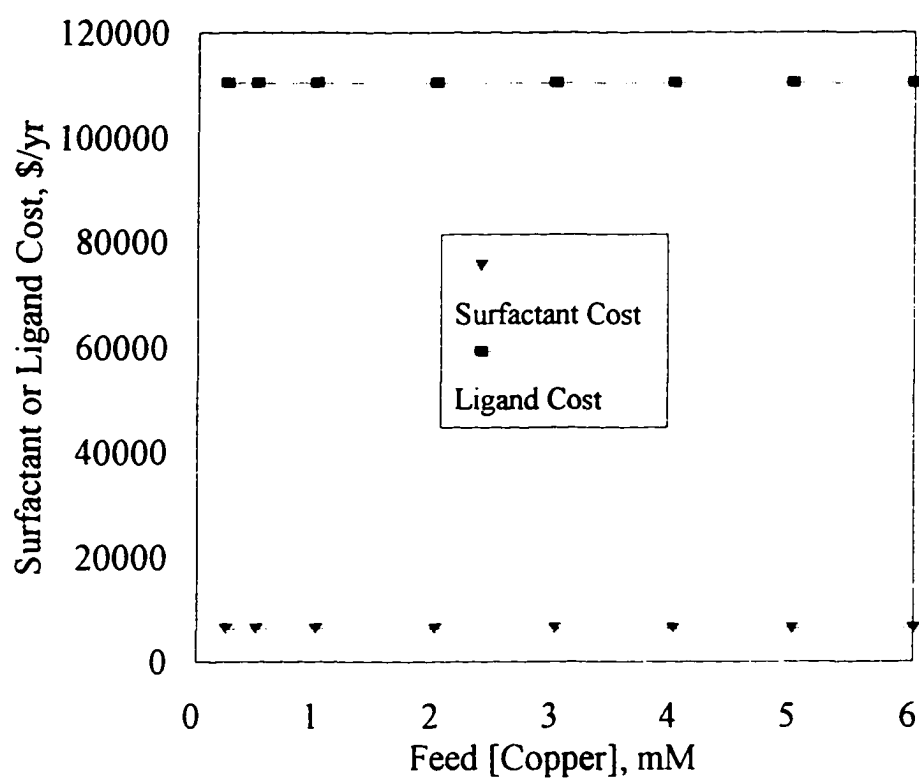
Figure II. 11 Annual Cost of Surfactant and Ligand vs. Feed [Copper], Single Stage Extraction Ultrafiltration Constant Feed [Surfactant] and [Ligand]
