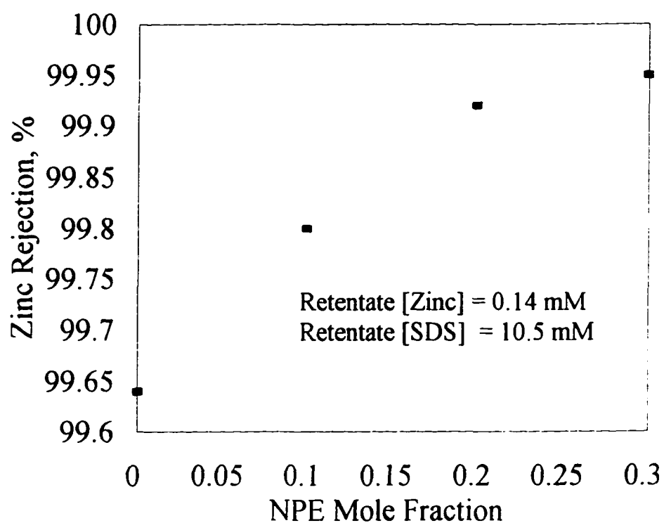
Figure III.13 Zinc Rejection vs. Mole Fraction NPE
