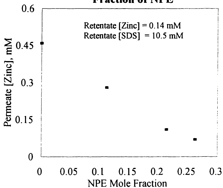
Figure III.18 Permeate Zinc vs. Mole Fraction of NPE
