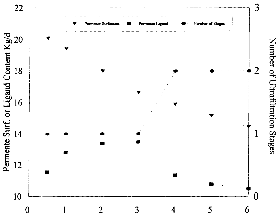
Figure II. 13 Surfactant and Ligand Losses in Permeate vs. Feed [Copper] to Maintain a Permeate [Copper]= 4 ppm, Multistage Ultrafiltration Unit
