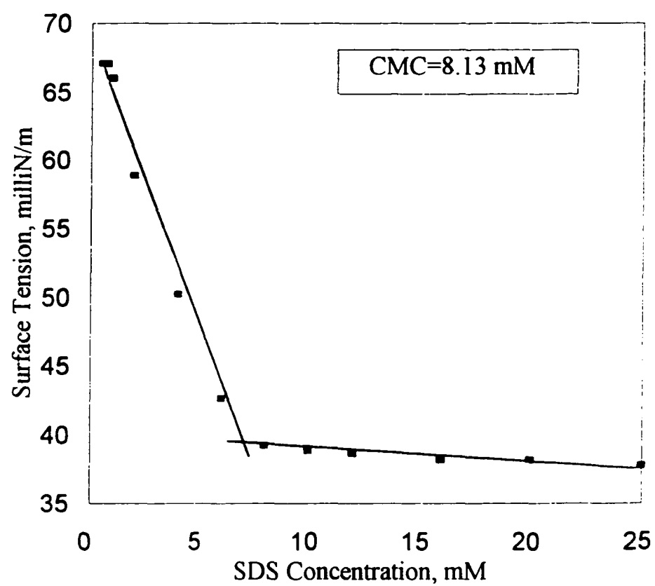
Figure III.2 Surface Tension of Pure SDS
