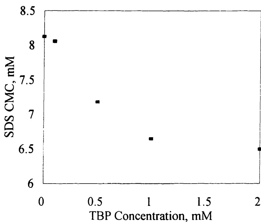
Figure III.4 Surface Tension of SDS with Added TBP
