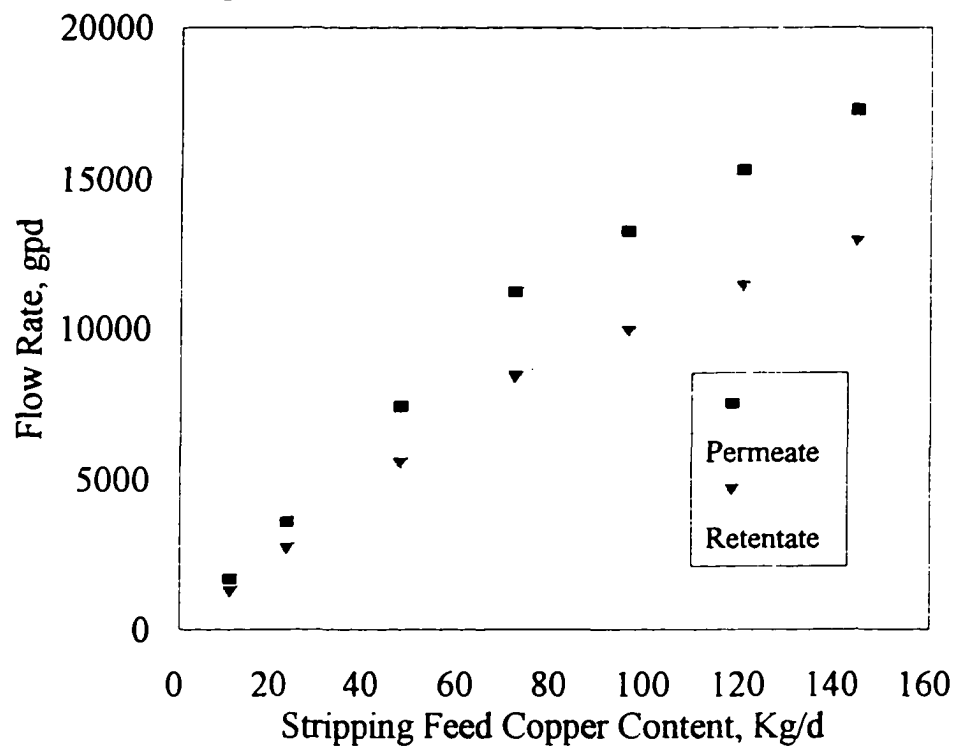
Figure II.15 Stripping Permeate or Retentate Flow Rate vs. Stripping Feed Copper Content, Single Stage Ultrafiltration Unit
