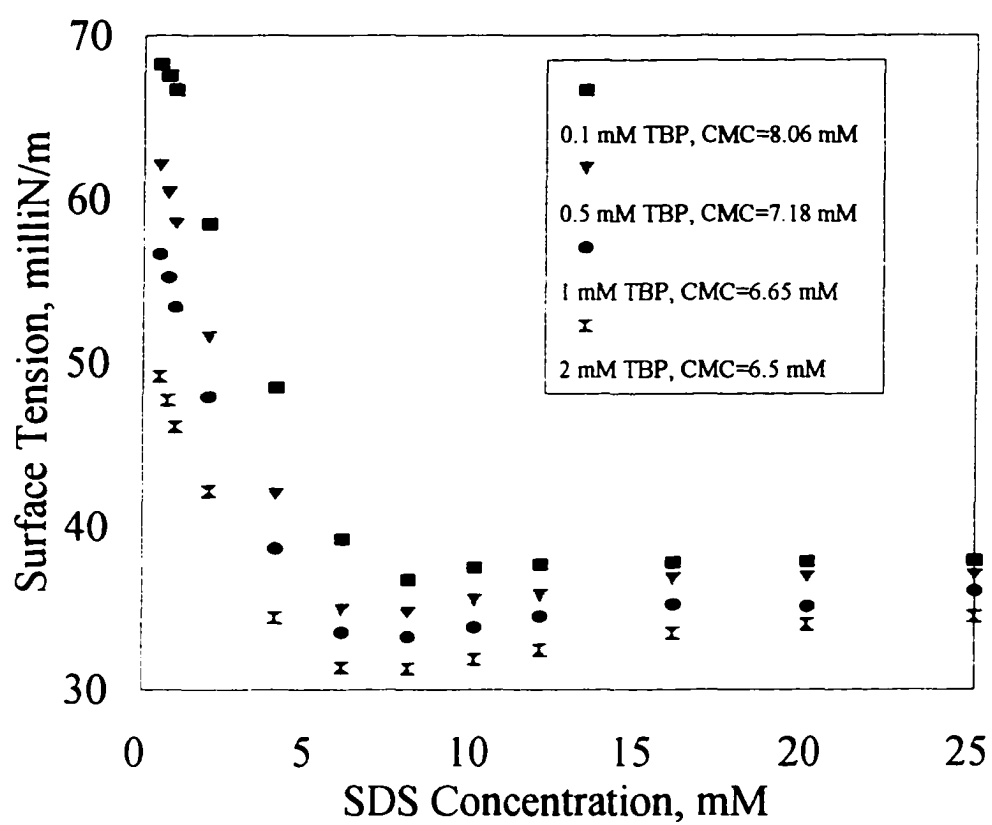
Figure III.3 SDS CMC as a Function of [TBP]
