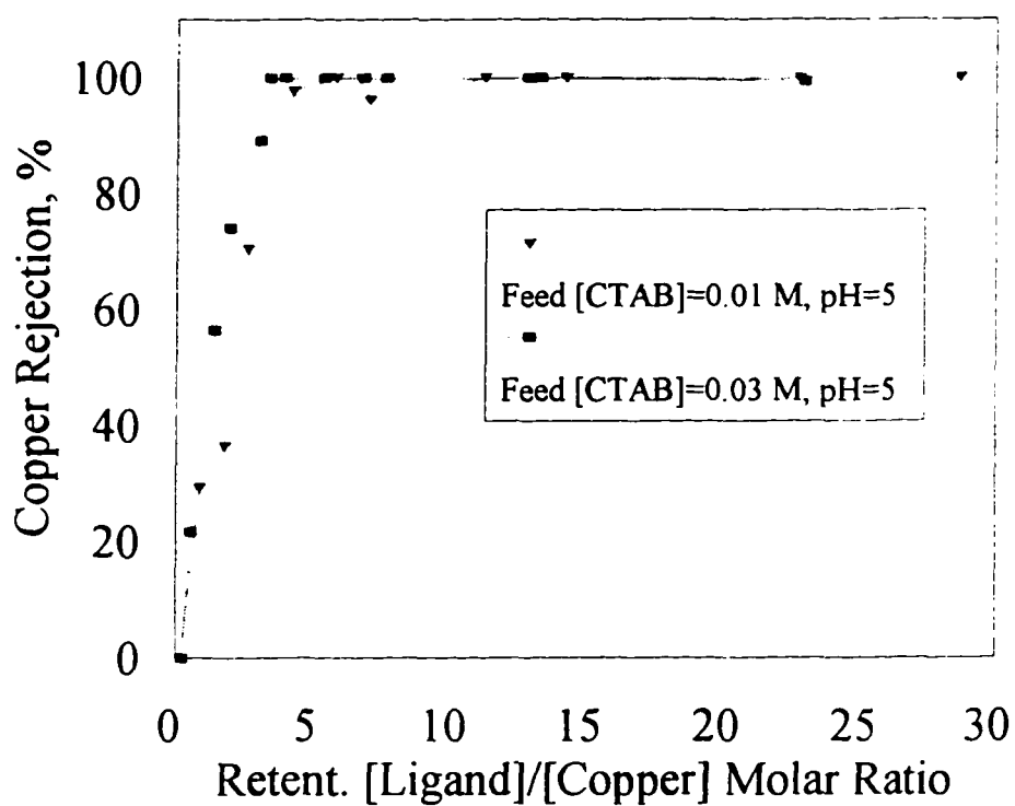
Figure I.8 Copper Rejection as a Function of Ligand/Copper Molar Ratio
