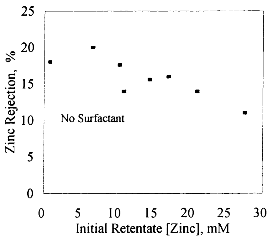
Figure III.7 Zinc Rejection vs. Initial Retentate [Zinc] in Pure Water
