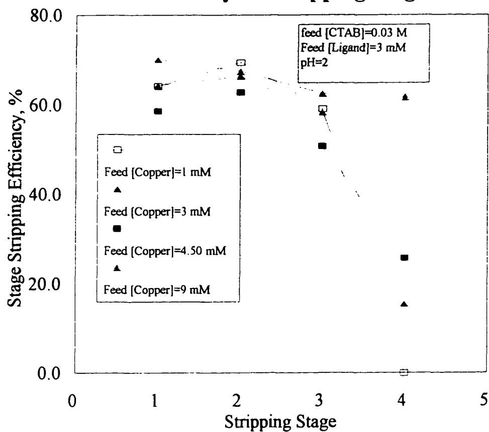
Figure I.14 Stage Stripping Efficiency vs. Stripping Stage
