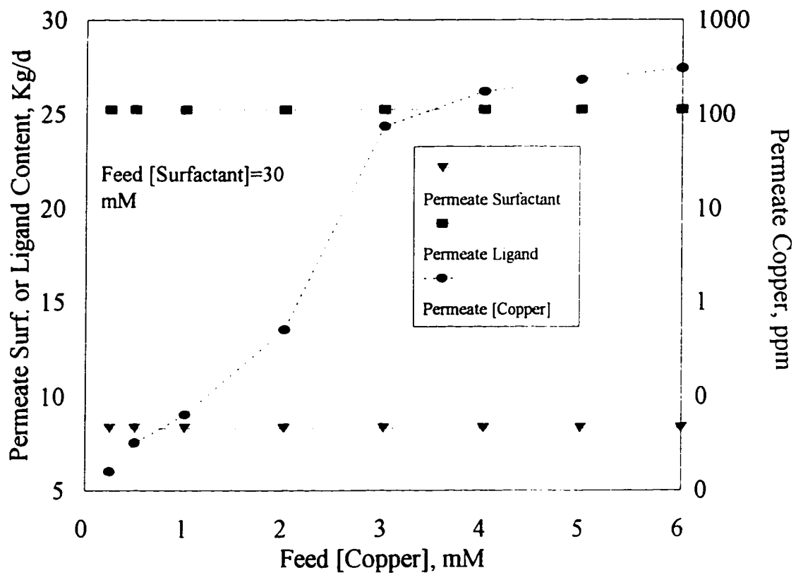
Figure II.10 Surfactant and Ligand Losses in Permeate vs. Feed [Copper], Constant Feed [Surfactant] and [Ligand], Single Stage Ultrafiltration Unit
