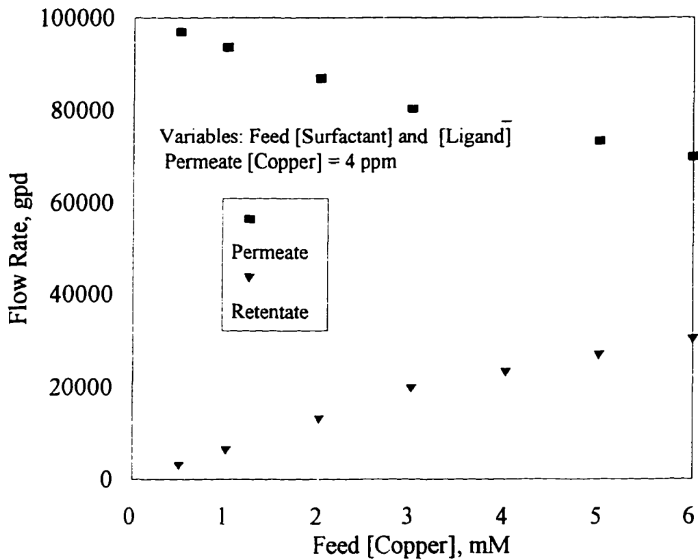
Figure II.12 Permeate or Retentate Flow Rate vs. Feed [Copper] with Variable Feed [Surfactant] and [Ligand] to Maintain a Permeate [Copper]=4 ppm, Multistage Ultrafiltration Unit
