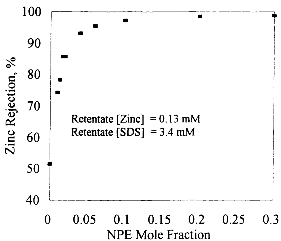
Figure III.9 Zinc Rejection vs. NPE Mole Fraction
