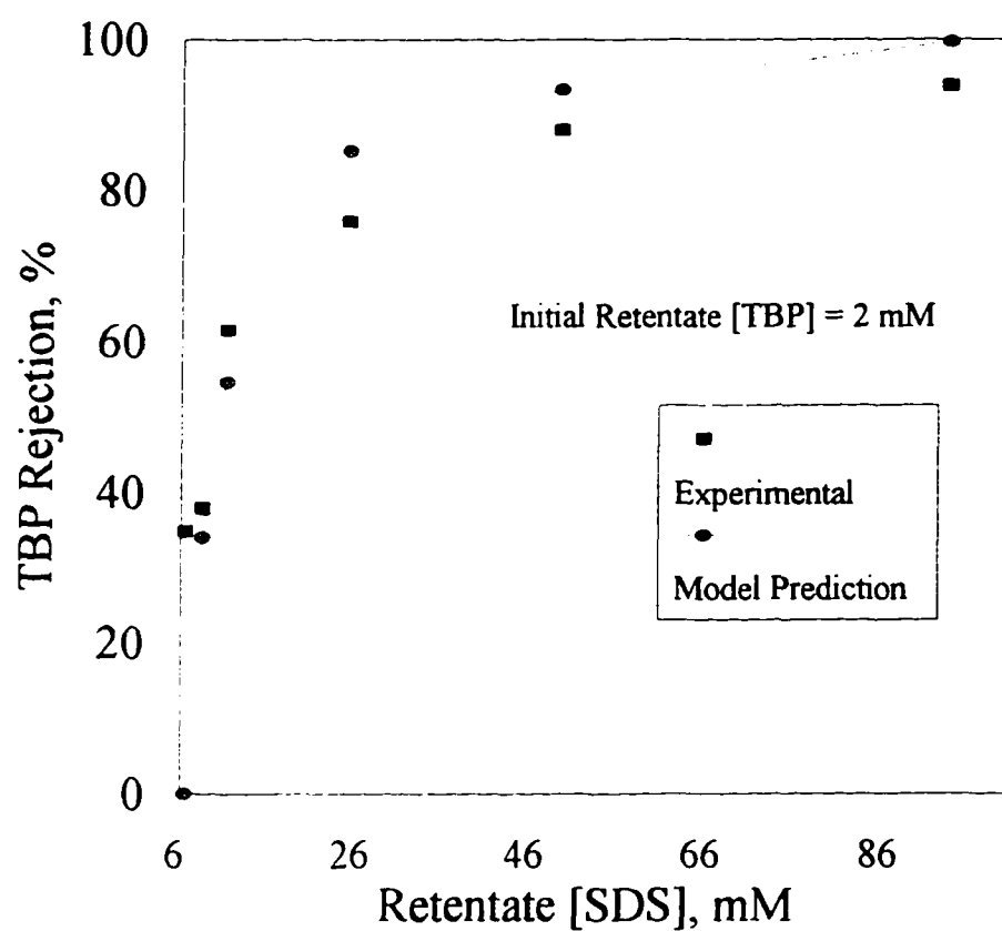
Figure III.11 TBP Rejection vs. Retentate [SDS], Above CMC
