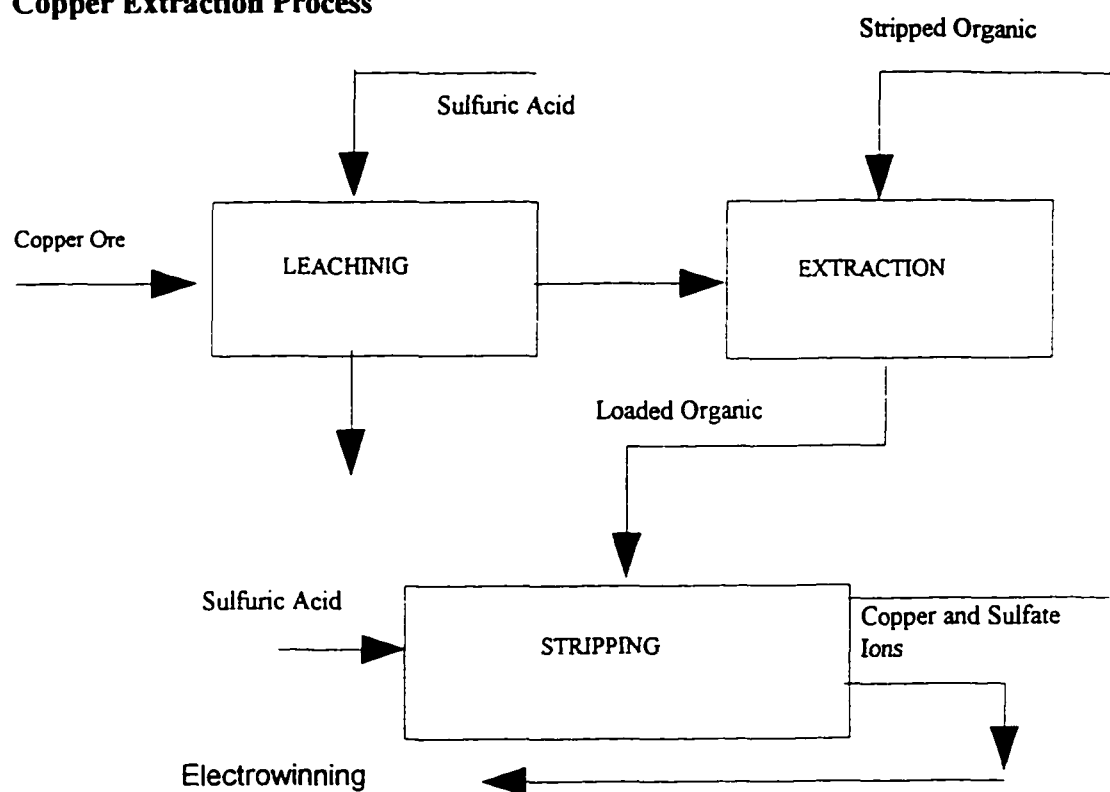
Figure I.1 Schematic of Traditional Copper Extraction Process
