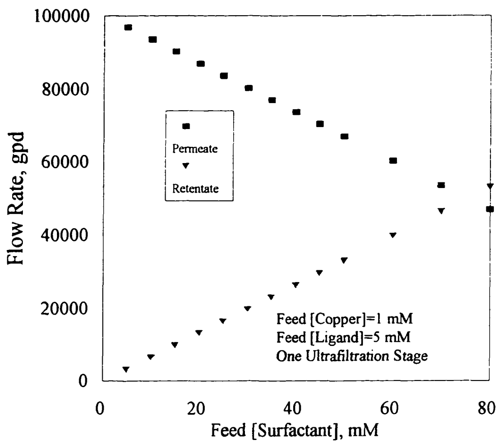
Figure II.3 Permeate or Retentate Flow Rate vs. Feed [Surfactant], Constant Feed [Ligand] and [Copper], Single Stage Ultrafiltration Unit
