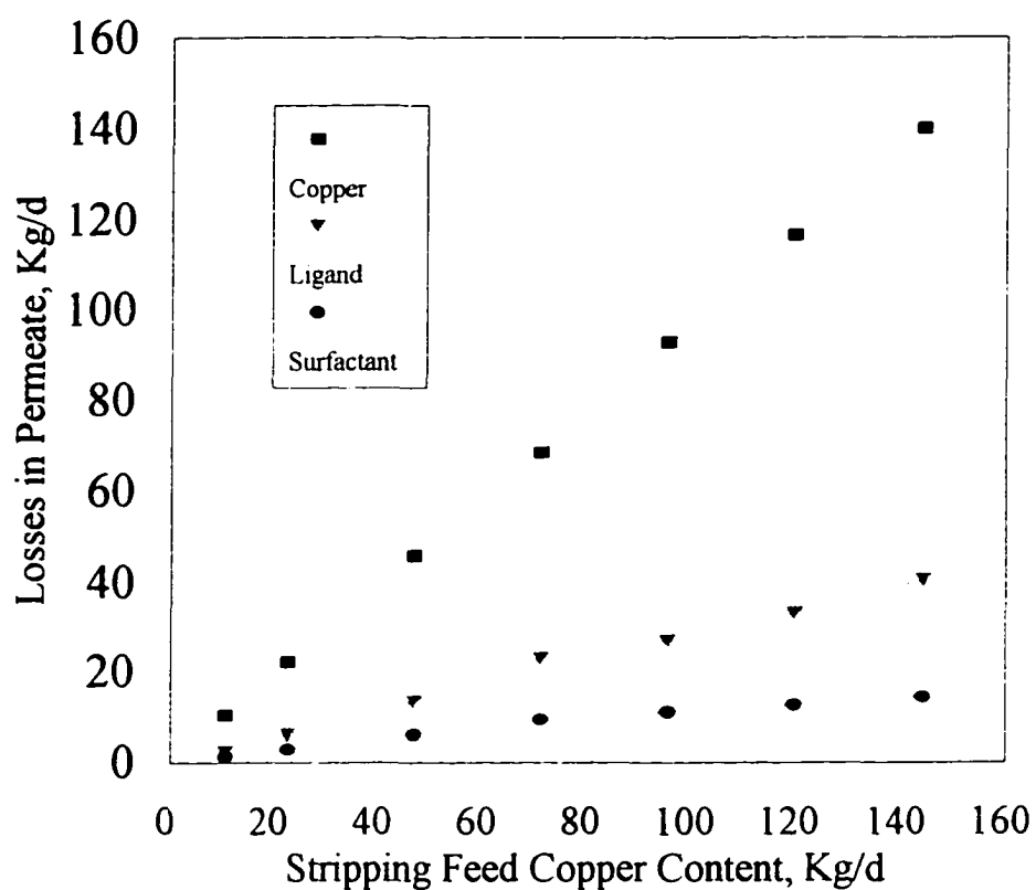
Figure II.16 Surfactant and Ligand Losses in Stripping Permeate vs. Stripping Feed Copper Content, Single Stage Stripping Ultrafiltration Unit
