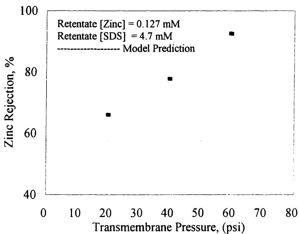
Figure III.10 Zinc Rejection as a Function of Transmembrane Pressure
