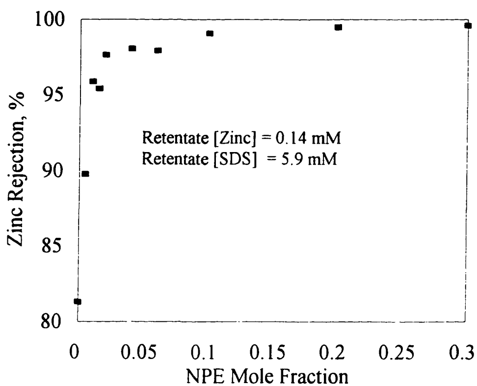
Figure III.12 Zinc Rejection vs. Mole Fraction NPE
