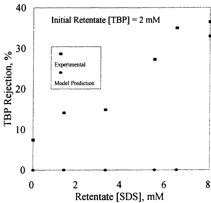
Figure III.5 TBP Rejection vs. Retentate [SDS], Below CMC
