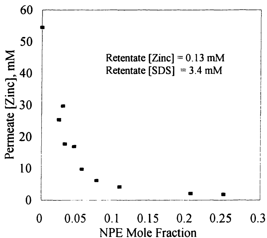
Figure III.16 Permeate Zinc vs. Mole Fraction NPE
