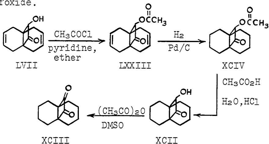
Scheme IX
