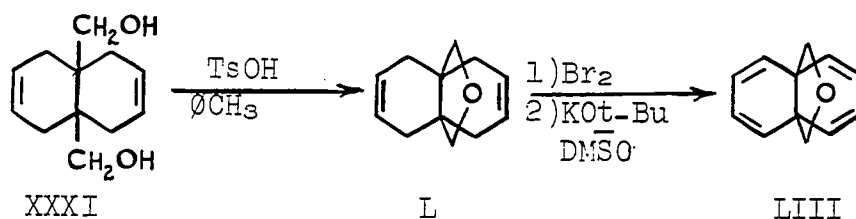
Scheme III
