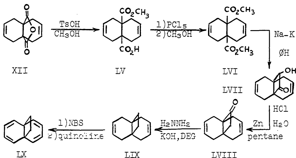
Scheme IV
