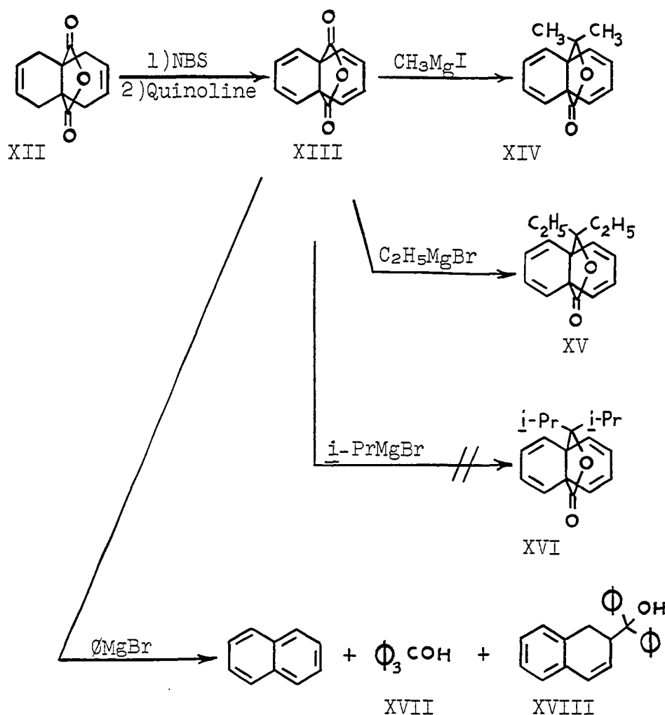
Scheme I
