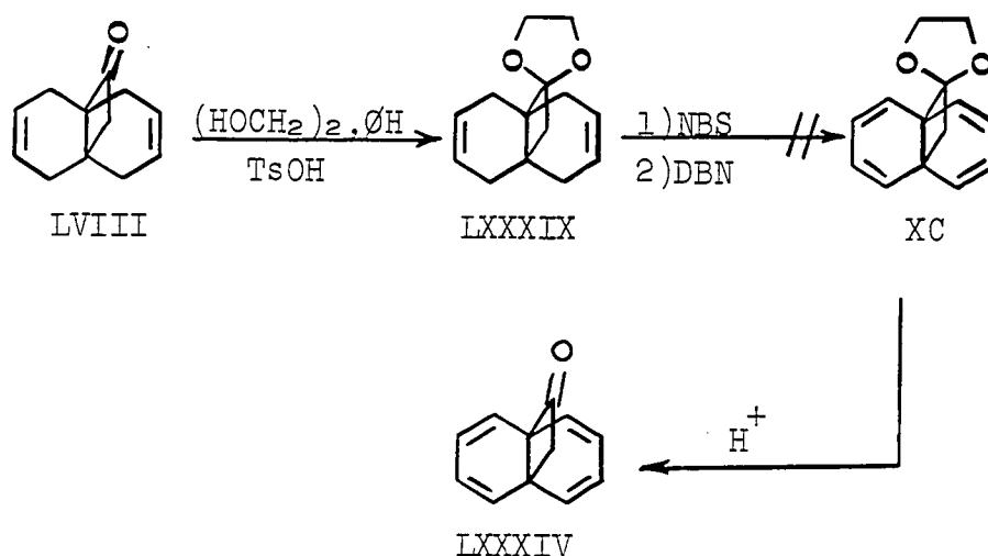
Scheme VIII
