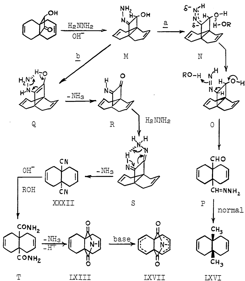
Scheme V
