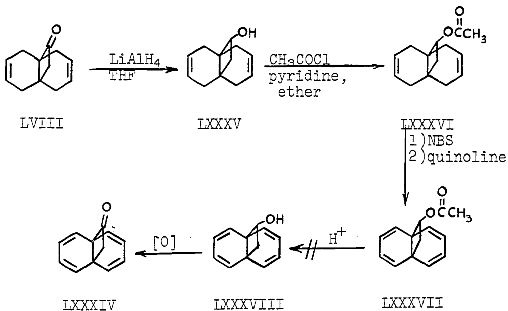
Scheme VII
