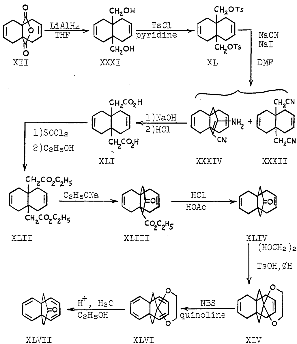
Scheme II
