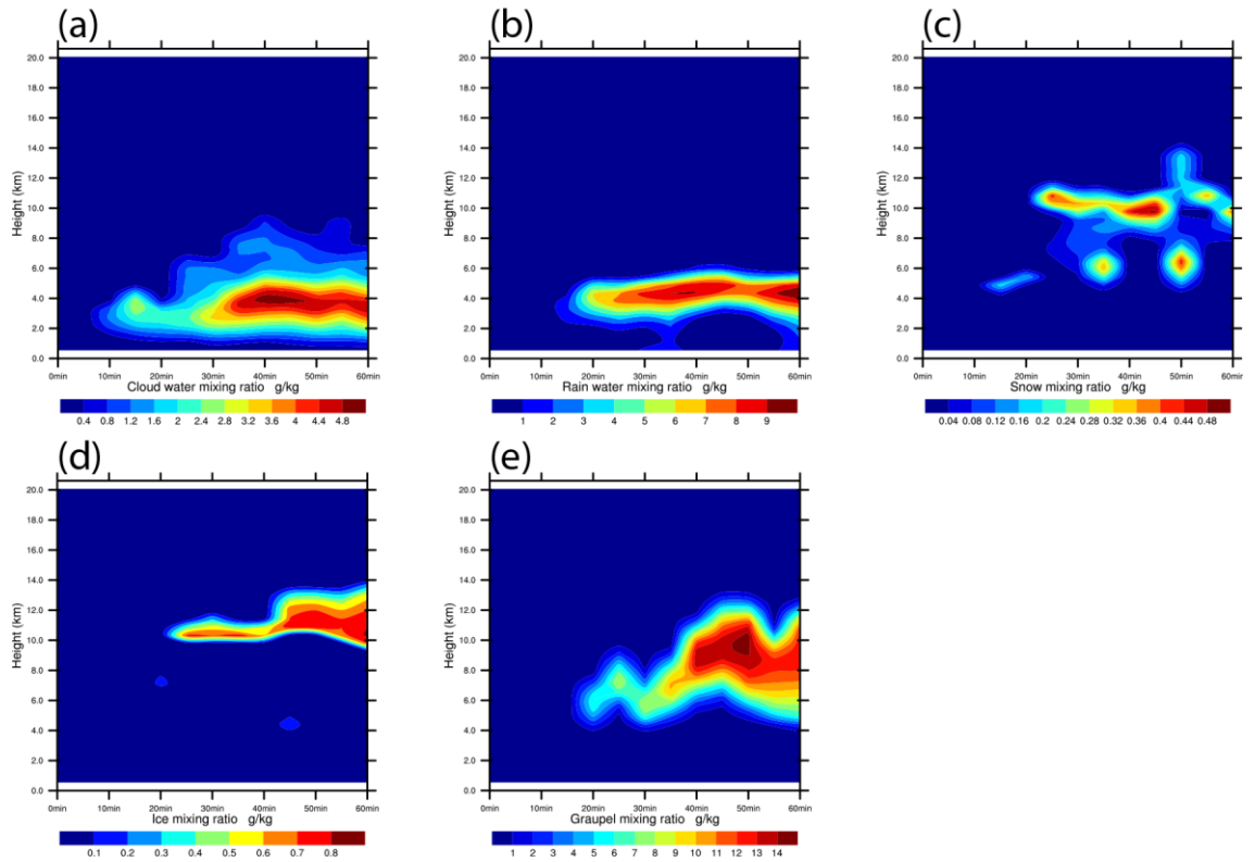
Figure 3. Time-Height composites of maximum hydrometeor mixing ratios (g kg -1 ) for truth simulation. (a) Cloud water; (b) Rain water; (c) Snow; (d) Ice; and (e) Graupel.
