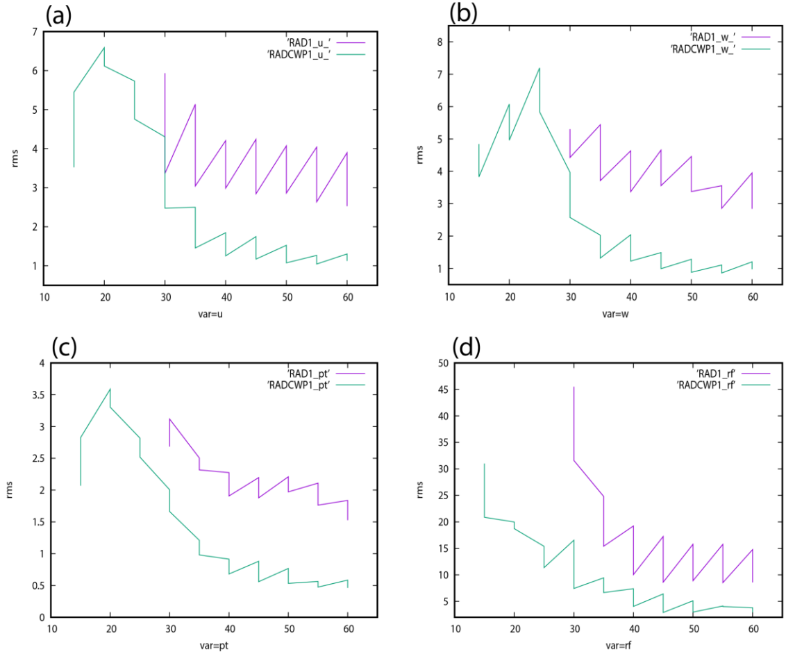
Figure 8. The rms error of the 3DENVar analysis and forecast for RAD1 (purple) and RADCWP1 (green) experiments. (a) Horizontal wind component u ( \text{m s}^{-1} ); (b) vertical wind component w ( \text{m s}^{-1} ); (c) perturbation potential temperature pt (K); and (d) simulated reflectivity rf (dBZ).
