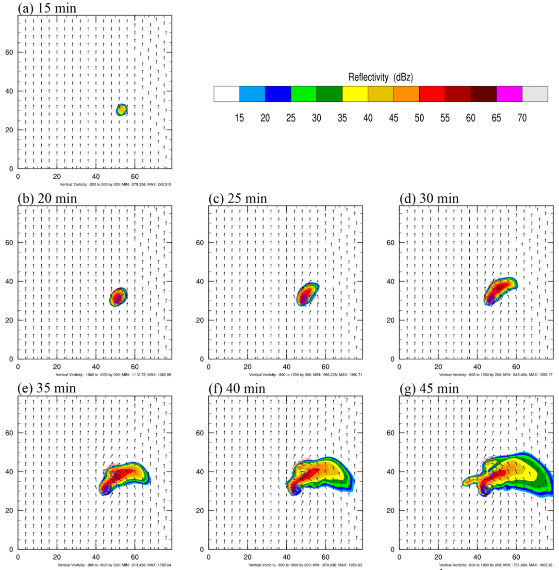
Figure 2. Simulated reflectivity (dBZ, shaded), wind field ( \text{m s}^{-1} , arrows) and relative vorticity ( 10^{-5} \text{ s}^{-1} , contours) at 4 km AGL from 15 min to 45 min as reference truth. Blue solid lines represent positive vorticities and red dashed lines are negative vorticities.
