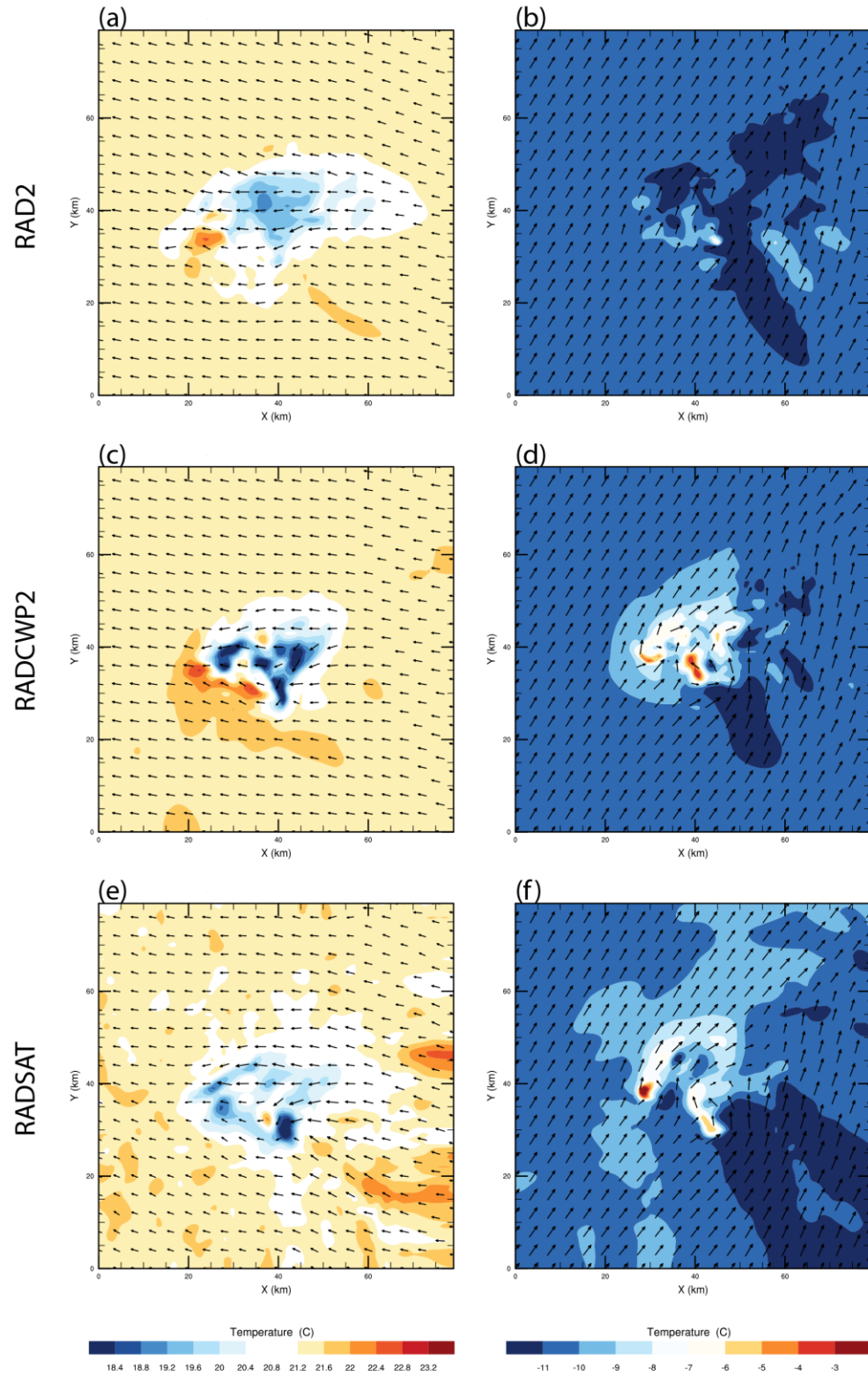
Figure 14. As in Fig. 6, but for experiment RAD2, RADCWP2 and RADSAT.
