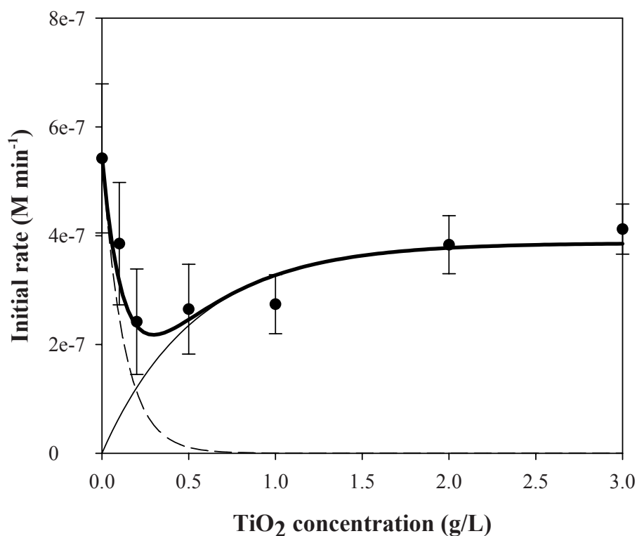
Figure 2.2. Initial rate of \text{NH}_4^+/\text{NH}_3 degradation versus \text{TiO}_2 concentration, initial pH: 10.2; [\text{NH}_3]_{\text{T},0} ranged from 9.38 \times 10^{-5} to 9.76 \times 10^{-5} M; error bars are 95% confidence intervals. Dashed and solid lines are schematic lines of homogeneous and heterogeneous degradation of \text{NH}_4^+/\text{NH}_3 that may occur in parallel, and the thicker line is the sum of these two processes.
