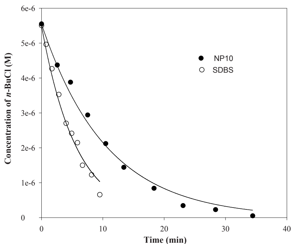
Figure 4.4. Photodegradation of n -BuCl by UV/ \text{H}_2\text{O}_2 at pH \sim 10.1 with initial addition of surfactants. A Vycor filter was used; [Surfactant]: 2 \times 10^{-5} M; [\text{NH}_3]_{\text{T},0} ( [\text{NH}_4^+] + [\text{NH}_3] ): (1.06 \pm 0.14) \times 10^{-4} M; [\text{NaCl}] : 0.001 M; lines are pseudo-first order reaction model fits of the concentration of n -BuCl versus time.
