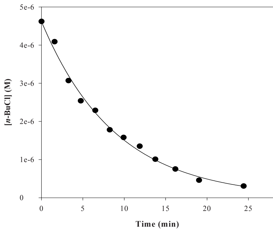
Figure D2. Photodegradation of n -BuCl with 2 × 10 -5 M cetylpyridinium chloride
