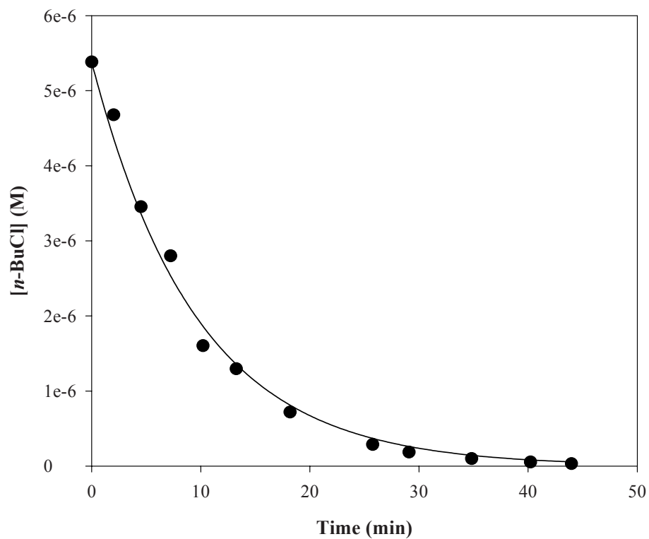
Figure D9. Photodegradation of n -BuCl with 1.2 \times 10^{-5} M Brij® 23 lauryl ether and 0.01 M \text{H}_2\text{O}_2
