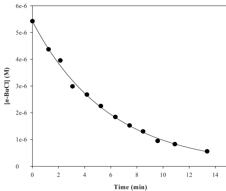
Figure D11. Photodegradation of n -BuCl with 2 \times 10^{-5} ally-tetra-O-acetyl - \beta -D-glucopyranoside
