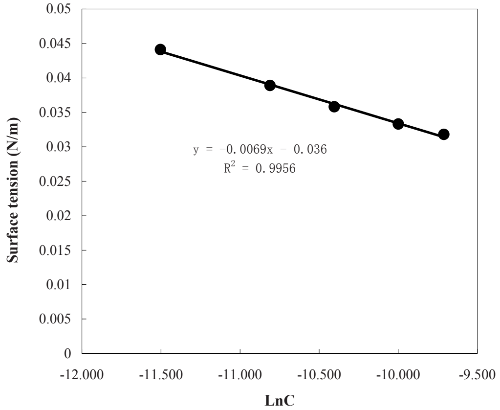
Figure F4. Surface tension as function of natural logarithm of NP10 concentrations
