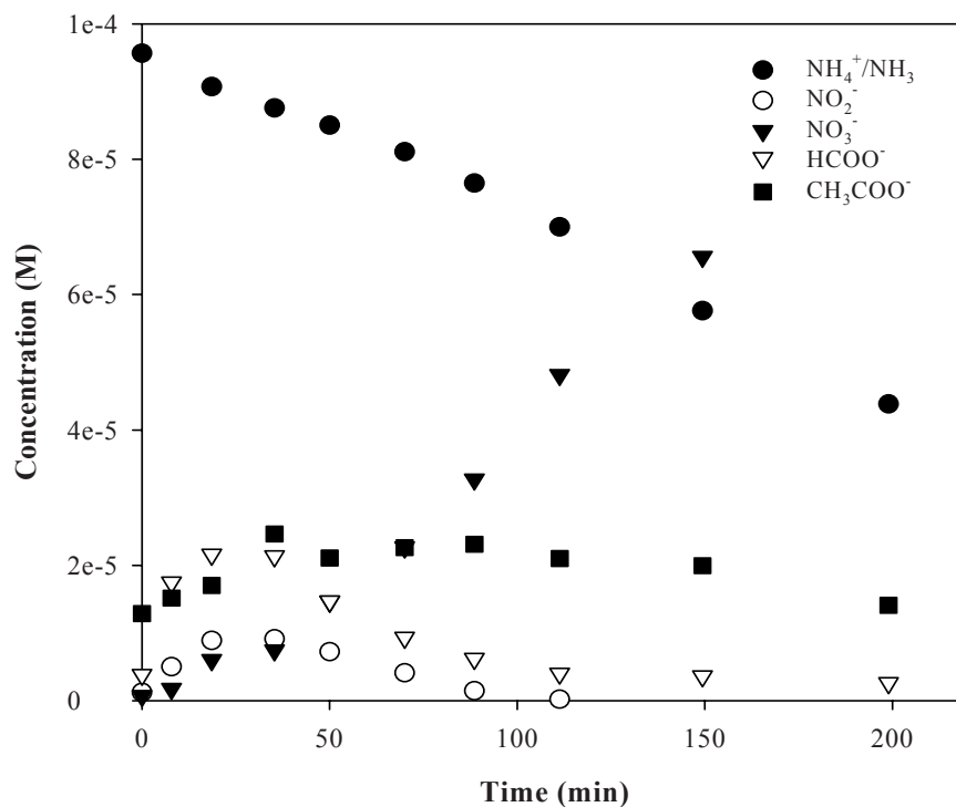
Figure E8. \text{NH}_4^+/\text{NH}_3 degradation with 2 \times 10^{-5} M cetyltrimethylammonium chloride
