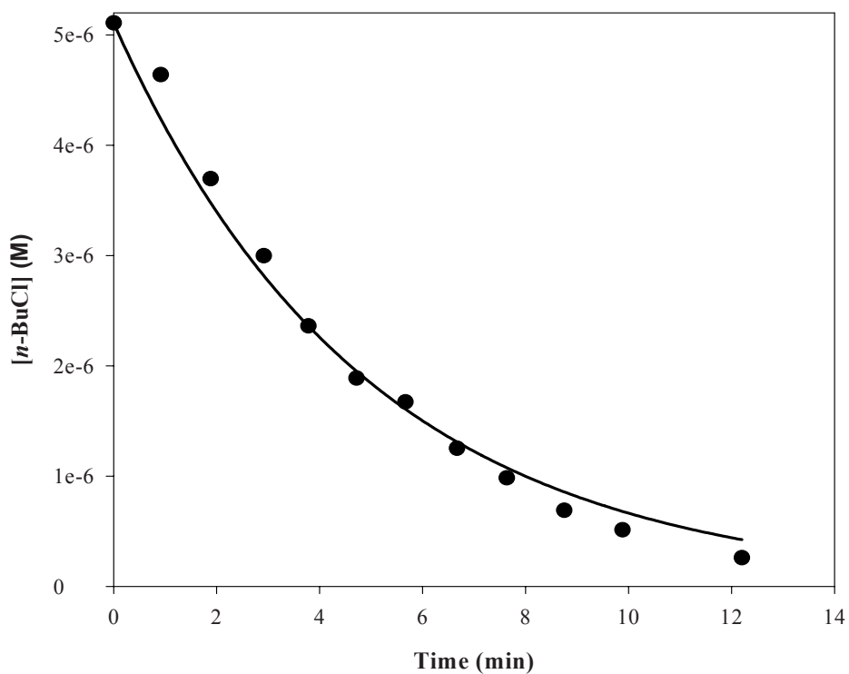
Figure D6. Photodegradation of n -BuCl with 2 \times 10^{-5} M sodium dodecylsulfate
