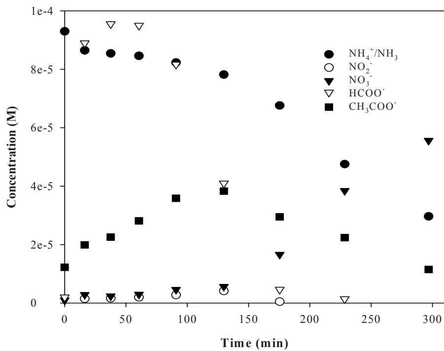
Figure E11. \text{NH}_4^+/\text{NH}_3 degradation with 1.2 \times 10^{-5} M Brij@35
