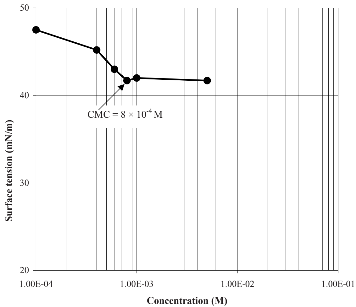
Figure F2. Surface tension versus concentration of CPC
