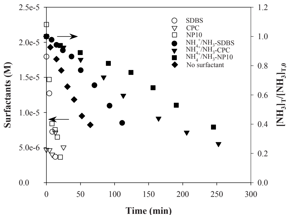
Figure 4.1. Photocatalytic degradation of \text{NH}_4^+/\text{NH}_3 and surfactants at pH \sim 10.1 . Open symbols are for the concentrations of surfactants and closed symbols are for \text{NH}_4^+/\text{NH}_3 degradation. [Surfactant]: 2 \times 10^{-5} M; [NaCl]: 0.001 M; [\text{NH}_3]_{\text{T},0} ( [\text{NH}_4^+] + [\text{NH}_3] ): (1.06 \pm 0.14) \times 10^{-4} M.
