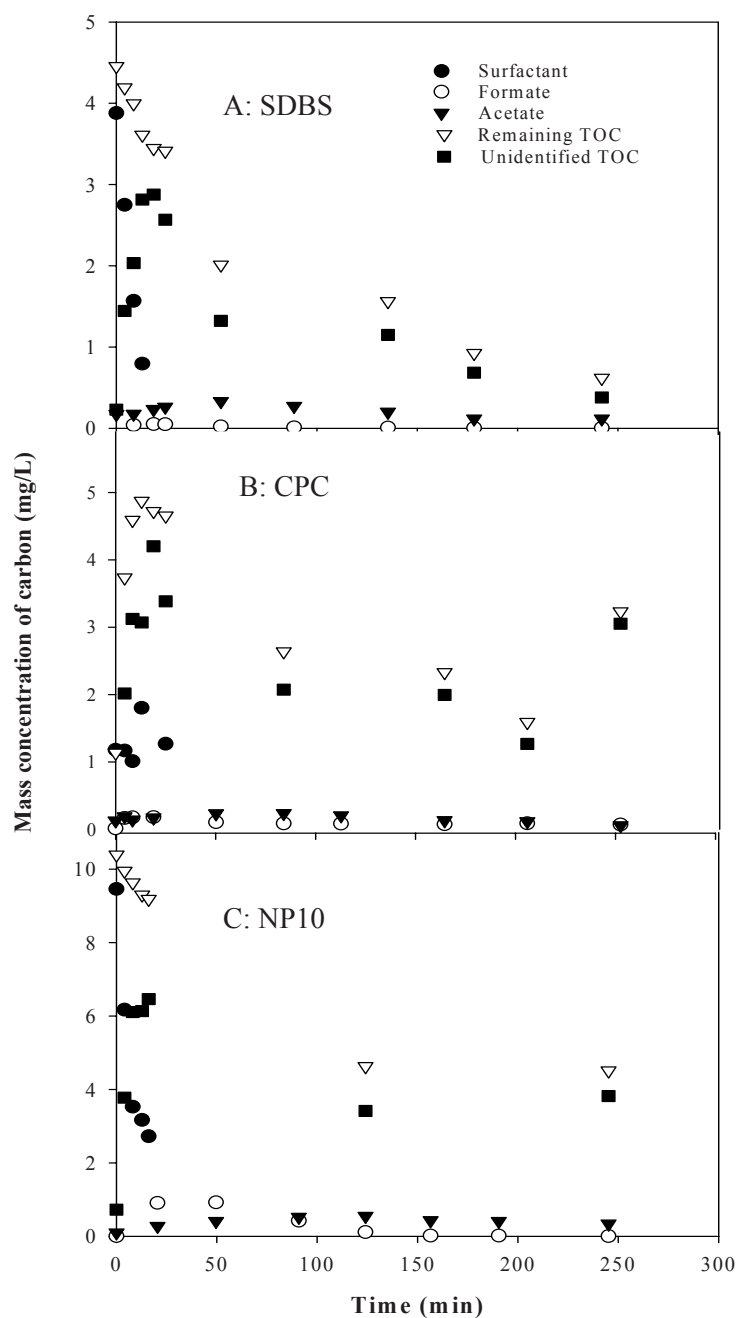
Figure 4.3. Mass concentration of surfactants and selected products during the photocatalytic degradation of \text{NH}_4^+/\text{NH}_3 and surfactants at pH \sim 10.1 . [\text{NH}_3]_{\text{T},0} : (1.06 \pm 0.14) \times 10^{-4} M; [\text{surfactant}] : 2 \times 10^{-5} M. [\text{unidentified TOC}] = [\text{Remaining TOC}] - C_{\text{formate}} - C_{\text{acetate}} - C_{\text{surfactant}} , where C is the mass concentration of carbon; Data for panel A was obtained from an experiment where [\text{NH}_3]_{\text{T},0} was 1.5 \times 10^{-4} M.
