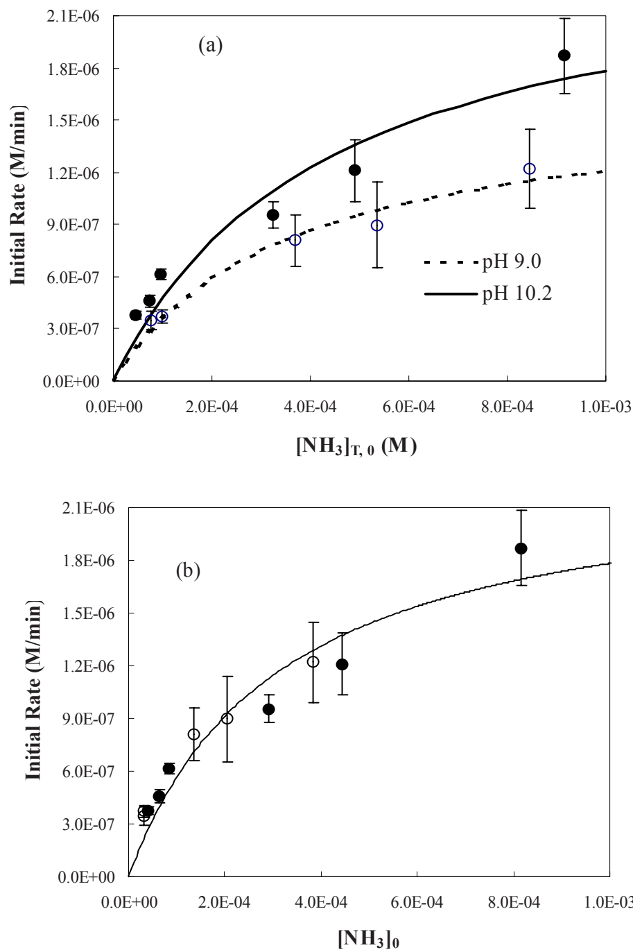
Figure 2.5* . Initial rate of \text{NH}_4^+/\text{NH}_3 photocatalytic oxidation versus (a) [\text{NH}_3]_{\text{T},0} at pH \sim 9 ( \circ ), and pH \sim 10.2 ( \bullet ), and (b) [\text{NH}_3]_0 . [\text{NH}_3]_0 = K_a \times [\text{NH}_3]_{\text{T},0} / ([\text{H}^+] + K_a) . [\text{NH}_3]_{\text{T},0} was measured by the ammonia gas-sensing electrode, \text{p}K_a = 9.3 (Stumm and Morgan 1996); \text{TiO}_2 : 3 g/L; [\text{NH}_3]_{\text{T},0} : 4.4 \times 10^{-5} to 9.2 \times 10^{-4} M; error bars are 95% confidence intervals; lines are the Langmuir-Hinshelwood model fits.
