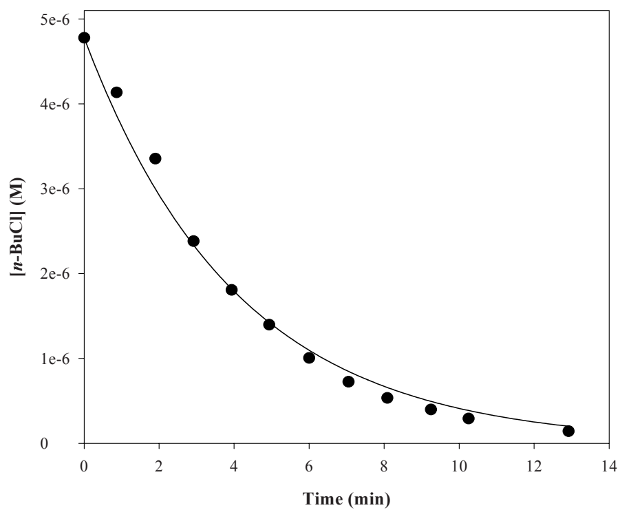
Figure D4. Photodegradation of n -BuCl with 2 \times 10^{-5} M 1-octanesulfonic acid sodium
