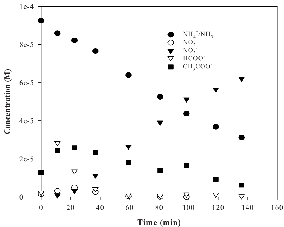
Figure E10. \text{NH}_4^+/\text{NH}_3 degradation with 2 \times 10^{-5} M hexyl- \beta -D-glucoside
