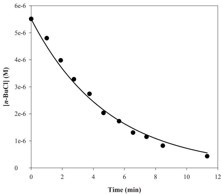
Figure D3. Photodegradation of n -BuCl with 2 \times 10^{-5} M hexyl- \beta -D-glucoside
