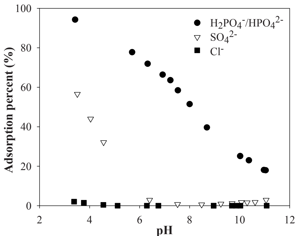
Figure 3.3. Adsorption of chloride ( \text{Cl}^- ), sulfate ( \text{SO}_4^{2-} ) and phosphate ( \text{H}_2\text{PO}_4^-/\text{HPO}_4^{2-} ). [anion]: 2 \times 10^{-4} M; [\text{NaClO}_4] : 0.01 M; [\text{TiO}_2] : 3 g/L; adsorption equilibrium time: 24 hours. \text{pH}_{\text{pzc}} of the Degussa \text{TiO}_2 is 6.2-7.5 (Hoffmann et al., 1995; Fernández-Nieves et al., 1998).
