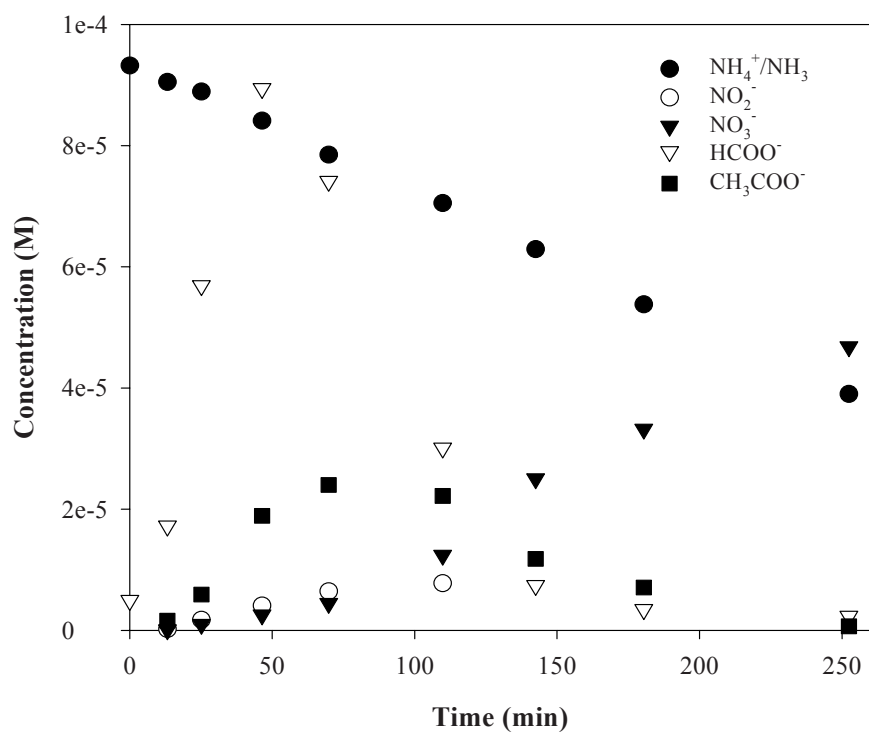
Figure E12. \text{NH}_4^+/\text{NH}_3 degradation with 1.2 \times 10^{-5} M Brij® 35 and 0.01 M \text{H}_2\text{O}_2
