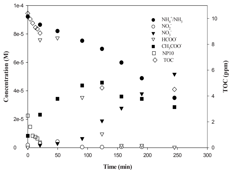
Figure E9. \text{NH}_4^+/\text{NH}_3 degradation with 2 \times 10^{-5} M NP10
