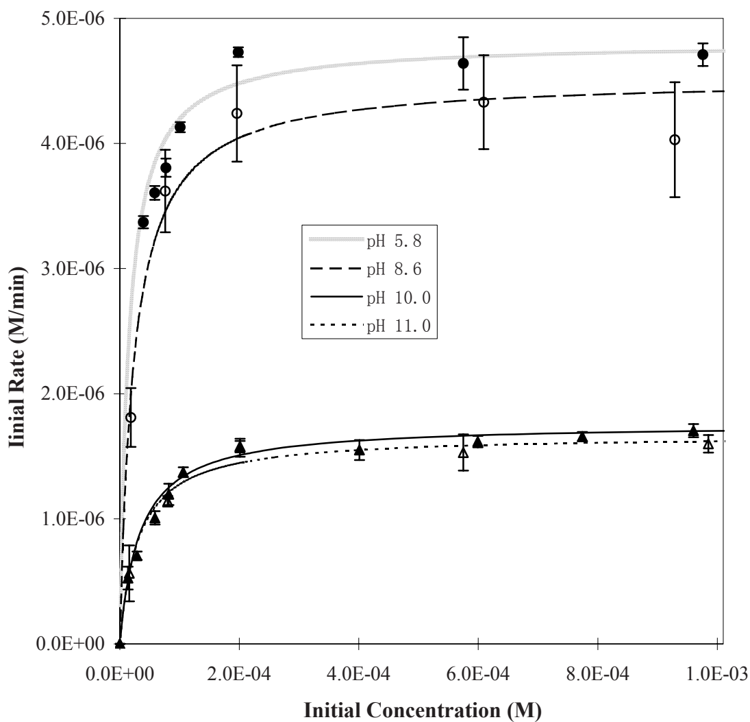
Figure 2.7. Initial rate of \text{NO}_2^- photocatalytic oxidation versus initial concentration at different initial pH values, the symbols represent the initial rates at different pH, pH \sim 5.8 ( \bullet ), pH \sim 8.6 ( \circ ), pH \sim 10.0 ( \blacktriangle ), pH \sim 11.0 ( \Delta ); [\text{NO}_2^-]_0 : 1.37 \times 10^{-5} - 9.85 \times 10^{-4} M; error bars are 95% confidence intervals; lines are the Langmuir-Hinshelwood model fits.
