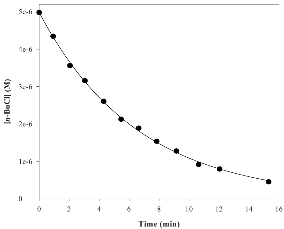
Figure D5. Photodegradation of n -BuCl with 2 \times 10^{-5} M dihexyl sulfosuccinate sodium
