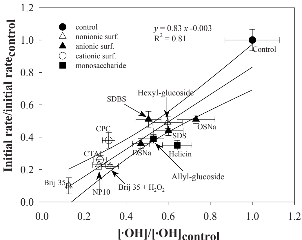
Figure 4.5. Relative initial rate of \text{NH}_4^+/\text{NH}_3 degradation versus relative concentration of \cdot\text{OH} in the presence of surfactants/monosaccharides. [\text{NH}_3]_{\text{T},0} : (1.06 \pm 0.14) \times 10^{-4} M, [surfactants/monosaccharides]: 2 \times 10^{-5} M except for Brij® 35 ( 1.2 \times 10^{-5} M); pH: \sim 10.1 . Error bars are 95% confidence intervals of initial rates of \text{NH}_4^+/\text{NH}_3 degradation and [\cdot\text{OH}] (calculated from propagation of error, as described in Appendix D). The straight line is the linear regression line. The curved lines represent upper and lower bounds of the 95% confidence interval.
