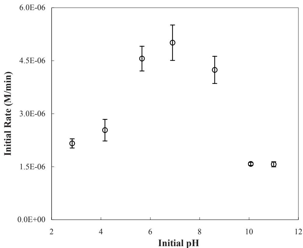
Figure 2.6. (a) Initial rate of \text{NO}_2^- photocatalytic oxidation versus initial pH; [\text{NO}_2^-]_0 : (1.8 \pm 0.2) \times 10^{-4} \text{ M} ; \text{TiO}_2 : 3 g/L; uncertainties are 95% confidence intervals. pH values (from left to right) are 2.8, 4.2, 5.7, 6.9, 8.6, 10.1, and 11.0.
