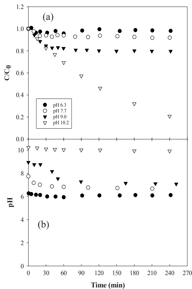
Figure 2.4. (a) [\text{NH}_3]_{\text{T}} disappearance and (b) pH variation during \text{NH}_4^+/\text{NH}_3 photocatalytic oxidation versus initial pH. [\text{NH}_3]_{\text{T},0} : 9.45 \times 10^{-5} to 9.98 \times 10^{-5} M, \text{TiO}_2 concentration: 3 g/L.
