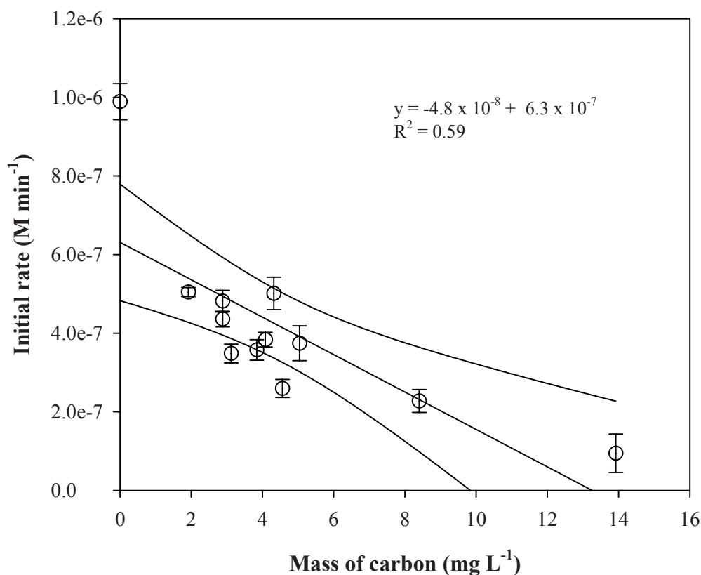
Figure 4.7. Initial rate of \text{NH}_4^+/\text{NH}_3 degradation at pH 10.1 vs. the mass concentration of carbon. [\text{NH}_3]_{\text{T},0} : (1.06 \pm 0.14) \times 10^{-4} M, [surfactant]/[monosaccharide]: 2 \times 10^{-5} M, except for Brij® 35 ( 1.2 \times 10^{-5} M). Error bars are 95% confidence intervals of initial rates of \text{NH}_4^+/\text{NH}_3 degradation. The straight line is the linear regression line. The curved lines represent upper and lower bounds of the 95% confidence interval.
