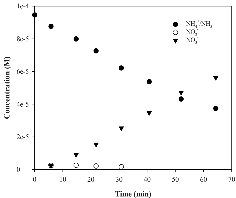
Figure E2. Photocatalytic degradation of \text{NH}_4^+/\text{NH}_3 without surfactants (control)
