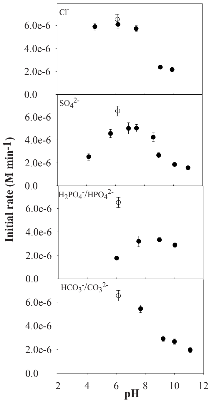
Figure 3.4. Effect of inorganic anions on \text{NO}_2^- photocatalytic oxidation between pH 4 and 11. [\text{NO}_2^-] : (1.9 \pm 0.1) \times 10^{-4} M; [\text{anion}] : 1 \times 10^{-3} M; [\text{TiO}_2] : 3 g/L; error bars are 95% confidence intervals. Some data for the \text{SO}_4^{2-} panel were previously reported in chapter 2. Open circles represent the initial rate of \text{NO}_2^- photocatalytic oxidation at pH ~ 6 when no anions were added.
