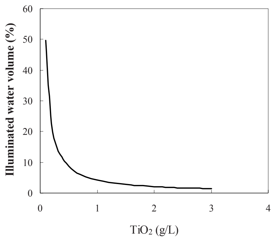
Figure B2. Percentage of illuminated water volume versus TiO 2 concentration at the light intensity ( I/I_0 ) of 0.01 at a wavelength of 388 nm.
