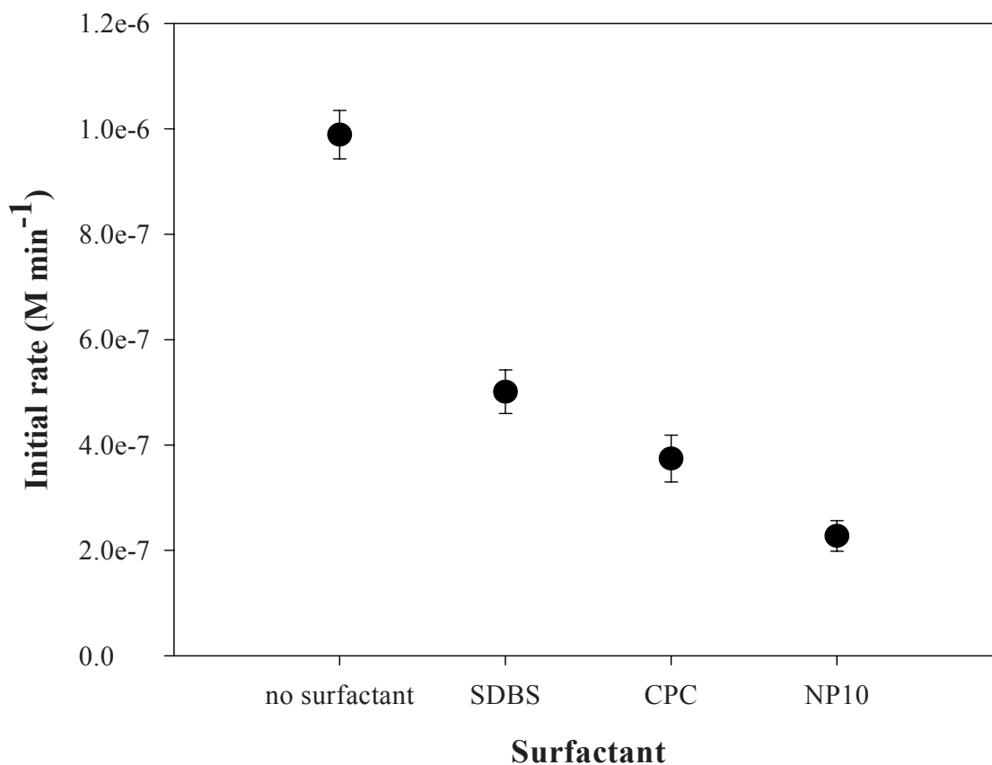
Figure 4.2. Initial rates of \text{NH}_4^+/\text{NH}_3 photocatalytic degradation in the presence of surfactants at pH \sim 10.1 . [Surfactant]: 2 \times 10^{-5} M; [NaCl]: 0.001 M; [\text{NH}_3]_{\text{T},0} ( [\text{NH}_4^+] + [\text{NH}_3] ): (1.06 \pm 0.14) \times 10^{-4} M. Error bars are 95% confidence intervals of initial rates of \text{NH}_4^+/\text{NH}_3 degradation.
