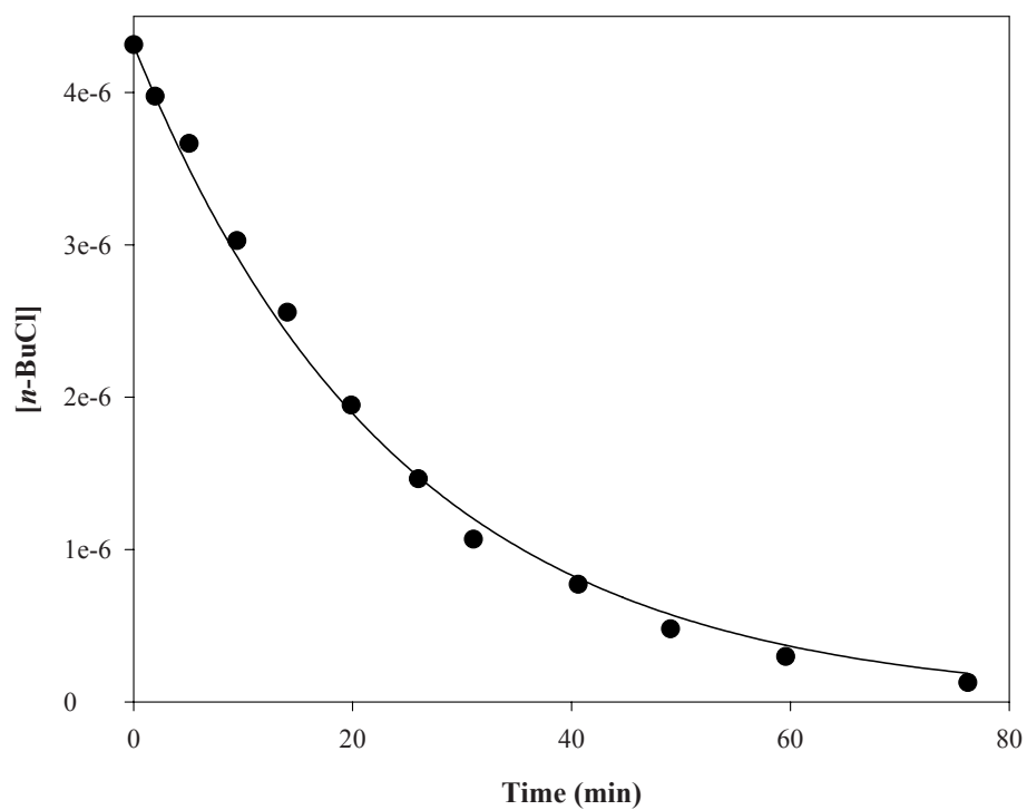
Figure D8. Photodegradation of n -BuCl with 1.2 \times 10^{-5} M Brij® 23 lauryl ether
