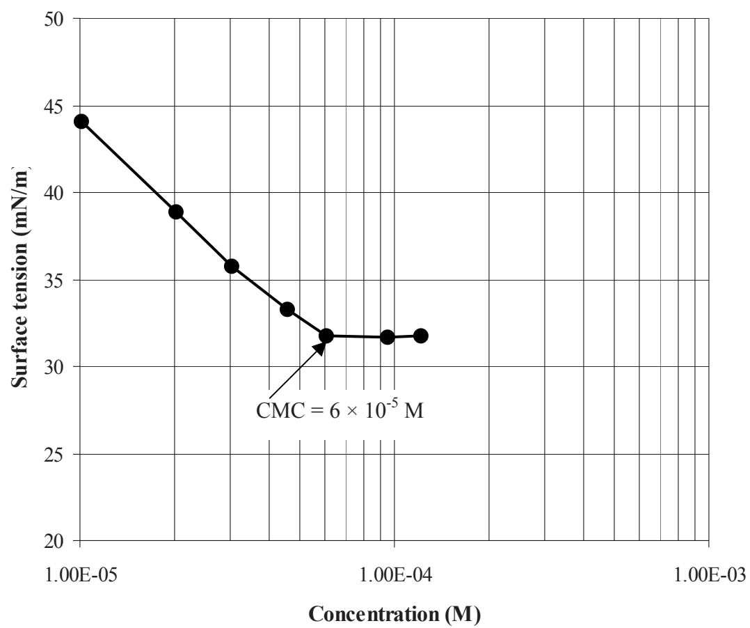
Figure F3. Surface tension versus concentration of NP10
