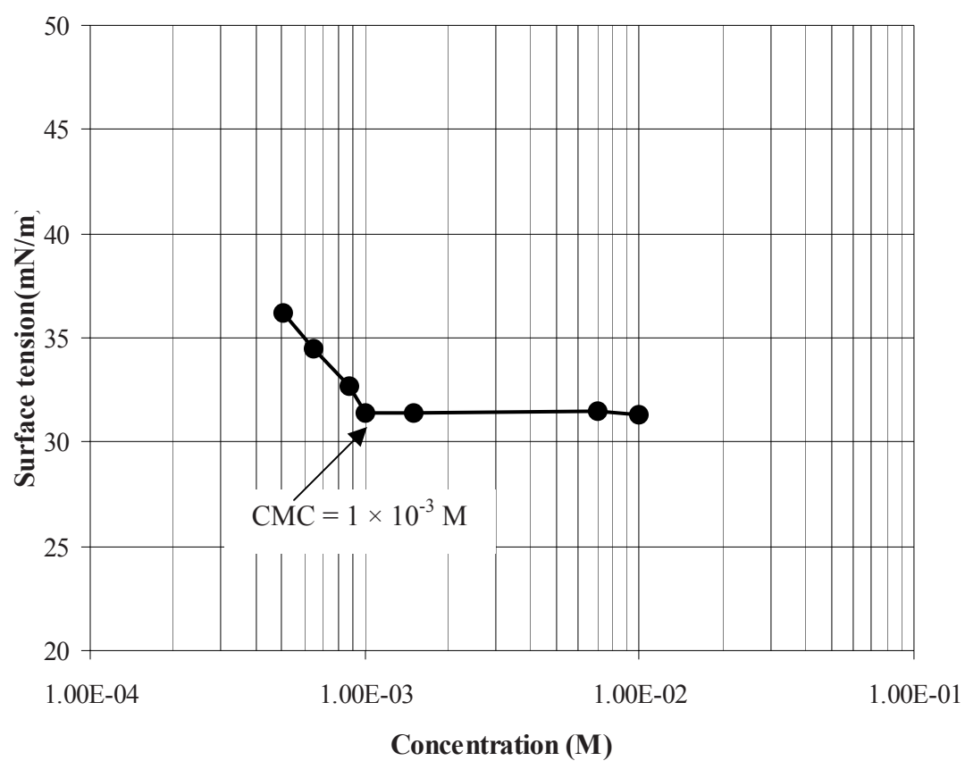
Figure F1. Surface tension versus concentration of SDBS
