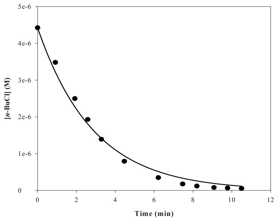
Figure D1. Photodegradation of n -BuCl without surfactants (control)
