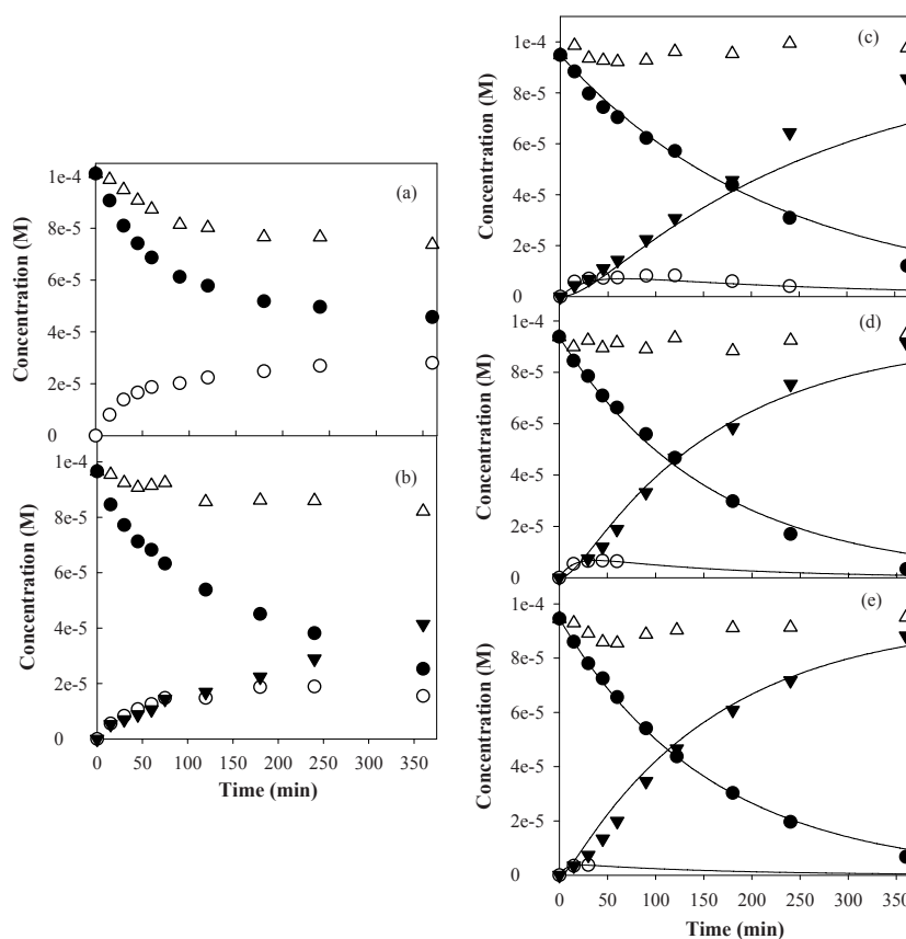
Figure 2.3. [\text{NH}_3]_{\text{T}} and products versus time at different \text{TiO}_2 concentrations. (a) 0 g/L, (b) 0.5 g/L, (c) 1 g/L, (d) 2 g/L, (e) 3 g/L; data points represent experimentally measured concentrations, [\text{NH}_3]_{\text{T},t} ( [\text{NH}_3] + [\text{NH}_4^+] at time t ) (●), [\text{NO}_2^-]_t (○), [\text{NO}_3^-]_t (▼), total nitrogen (Δ, sum of [\text{NH}_3]_{\text{T},t} , [\text{NO}_2^-]_t , and [\text{NO}_3^-]_t ); initial pH: 10.2; lines represent the consecutive first-order model fit for the concentrations of [\text{NH}_3]_{\text{T},t} , [\text{NO}_2^-]_t , and [\text{NO}_3^-]_t calculated from the rate constants k_1 and k_2 that were determined from the experimental data.
