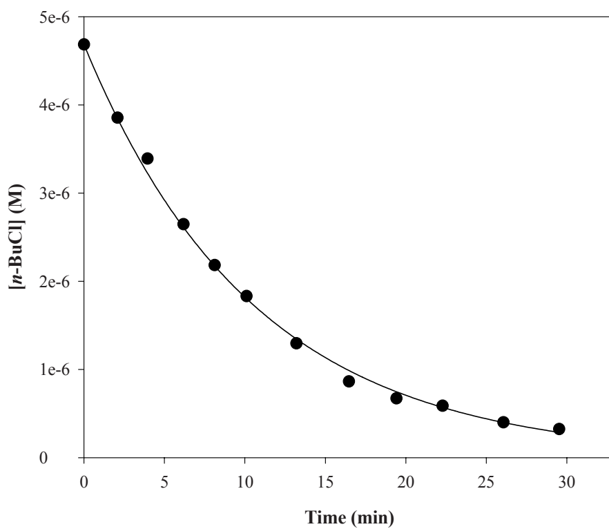
Figure D7. Photodegradation of n -BuCl with 2 \times 10^{-5} M cetyltrimethylammonium chloride
