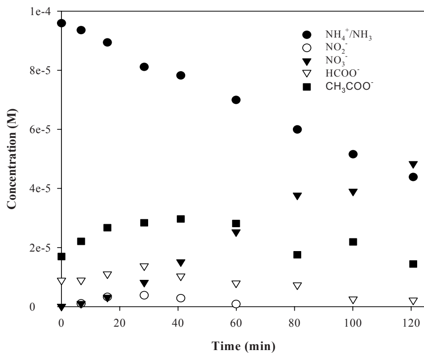
Figure E6. \text{NH}_4^+/\text{NH}_3 degradation with 2 \times 10^{-5} M sodium dodecylsulfate
