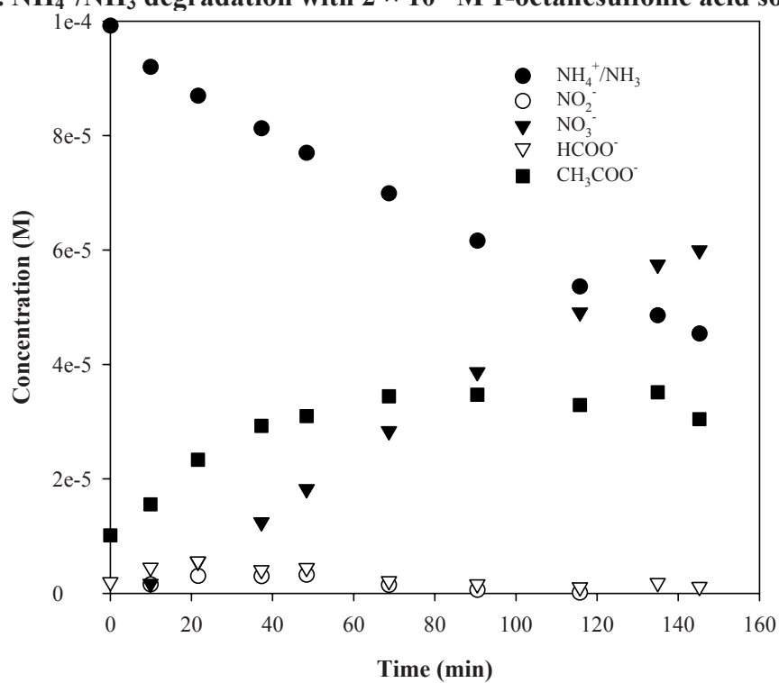
Figure E5. \text{NH}_4^+/\text{NH}_3 degradation with 2 \times 10^{-5} \text{ M} dihexyl sulfosuccinate sodium
