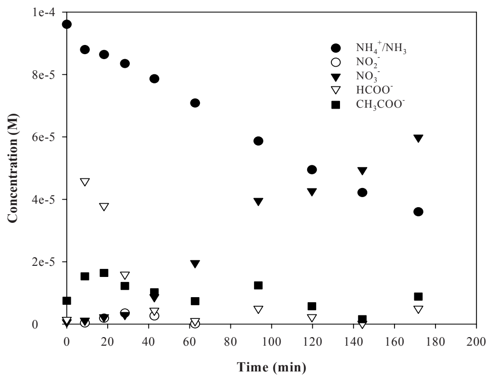
Figure E14. \text{NH}_4^+/\text{NH}_3 degradation with 2 \times 10^{-5} \text{ M} helicin
