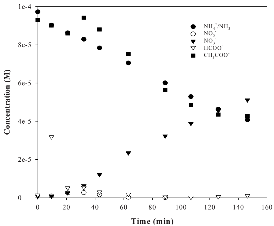
Figure E13. \text{NH}_4^+/\text{NH}_3 degradation with 2 \times 10^{-5} M ally-tetra-O-acetyl- \beta -D-glucopyranoside
