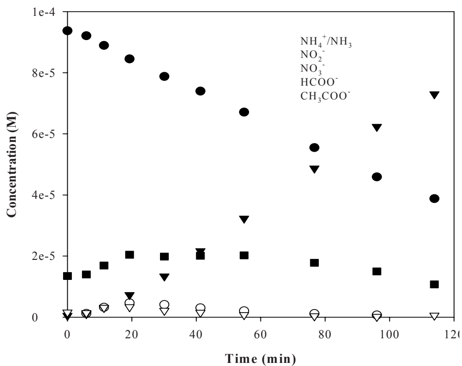
Figure E4. \text{NH}_4^+/\text{NH}_3 degradation with 2 \times 10^{-5} \text{ M} 1-octanesulfonic acid sodium
