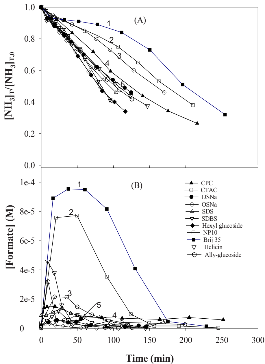
Figure 4.6. \text{NH}_4^+/\text{NH}_3 photocatalytic degradation (A) and formate formation (B) at pH ~ 10.1. [\text{NH}_3]_{\text{T},0} : (1.06 \pm 0.14) \times 10^{-4} M, [\text{surfactant}]/[\text{monosaccharides}] : 2 \times 10^{-5} M, except for Brij® 35 ( 1.2 \times 10^{-5} M); pH: ~10.1; [\text{NaCl}] : 0.001 M; the numbers on the figures represent \text{NH}_4^+/\text{NH}_3 and formate concentrations in the presence of Brij® 35 (1), NP10 (2), CTAC (3); CPC (4), and DSNa (5).
