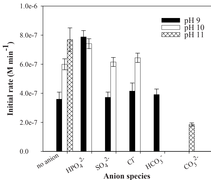
Figure 3.1. Effect of inorganic anions on \text{NH}_4^+/\text{NH}_3 photocatalytic oxidation at pH ~9 and ~10 (pH ~11 for \text{CO}_3^{2-} ). [\text{NH}_4^+/\text{NH}_3] : (9.6 \pm 0.6) \times 10^{-5} M; [\text{anion}] : 1 \times 10^{-3} M; [\text{TiO}_2] : 3 g/L; error bars are 95% confidence intervals.
