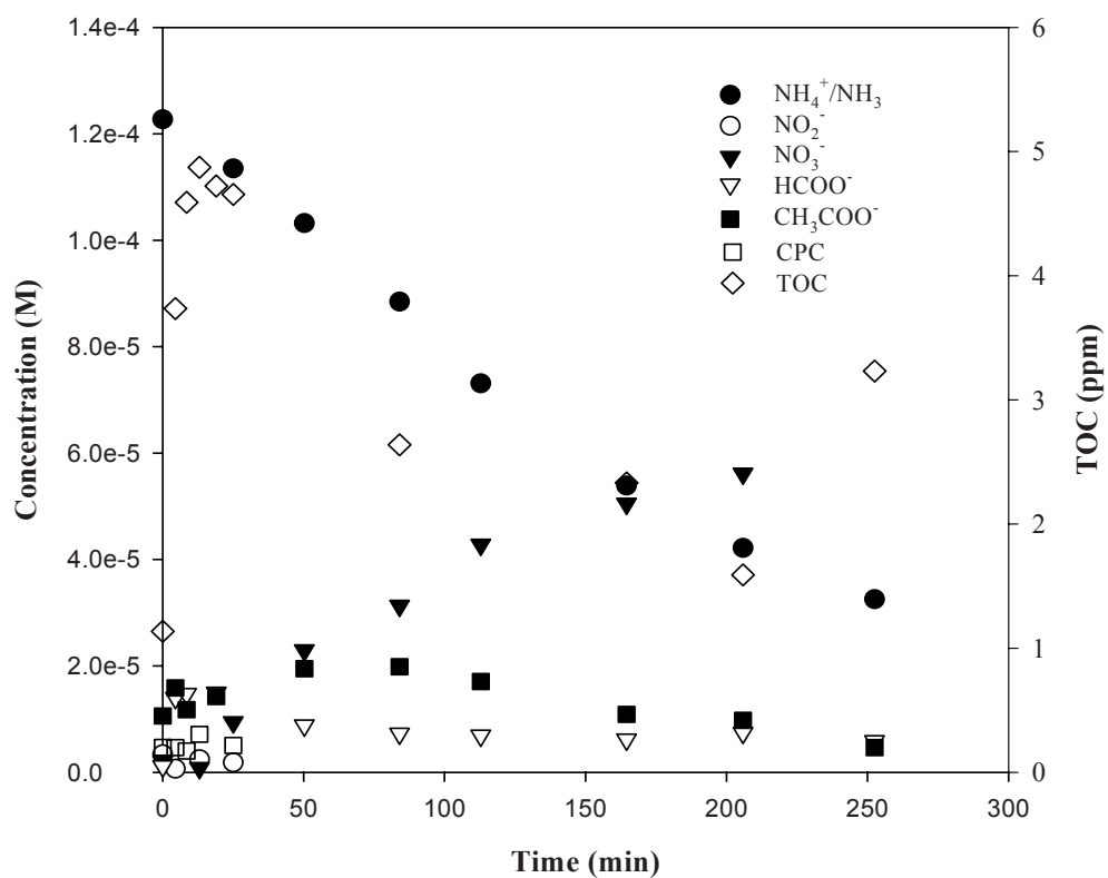
Figure E7. \text{NH}_4^+/\text{NH}_3 degradation with 2 \times 10^{-5} M cetylpyridinium chloride
