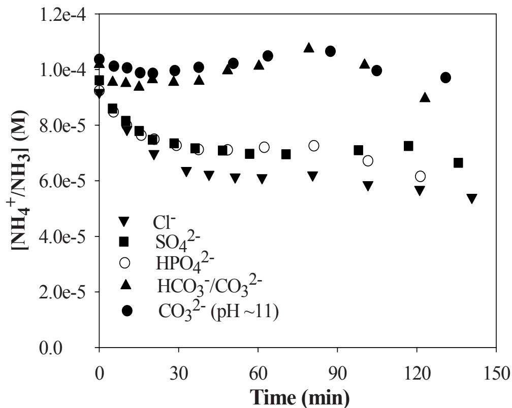
Figure 3.2. Effect of inorganic anions on the homogeneous photochemical oxidation of \text{NH}_4^+/\text{NH}_3 by UV/ \text{H}_2\text{O}_2 with a Vycor filter at pH ~10, except for the data series labeled \text{CO}_3^{2-} , which was done at pH ~11. [\text{NH}_4^+/\text{NH}_3] : (9.6 \pm 0.6) \times 10^{-5} M; [\text{H}_2\text{O}_2] : 0.001 M; [\text{anion}] : 0.005 M.
