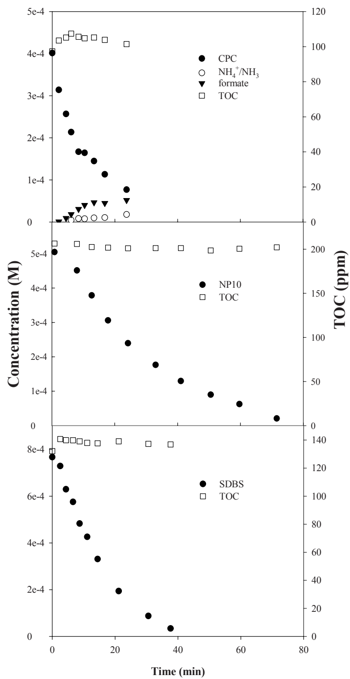
Figure E1. Homogeneous degradation of CPC, NP10, and SDBS at pH ~10.1. [NaCl]: 0.001 M.
