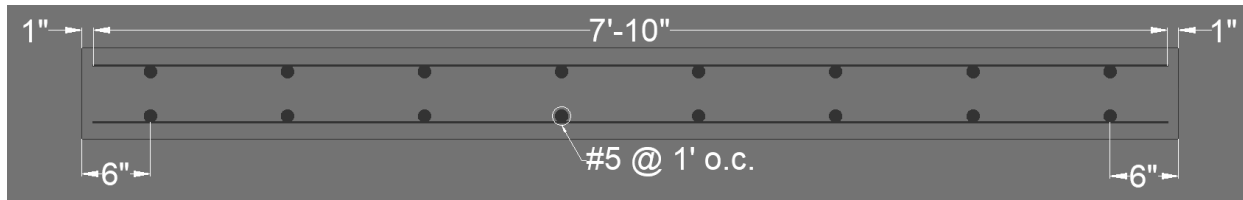
Figure 3-9: A-A' elevation of specimen design from Figure 3-3
