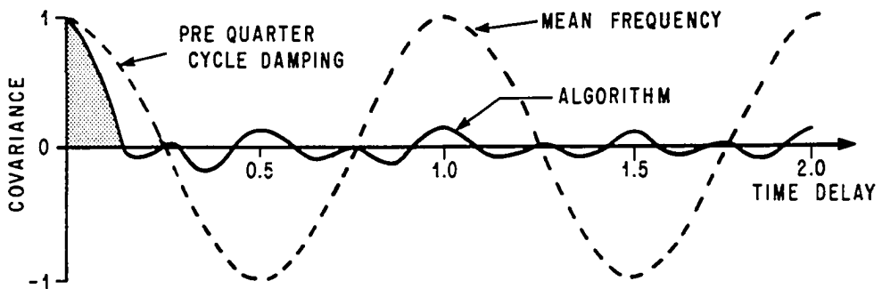
FIGURE 19. AUTOCOVARIANCE CURVES OF NARROWBAND AND BROADBAND PROCESSES.
