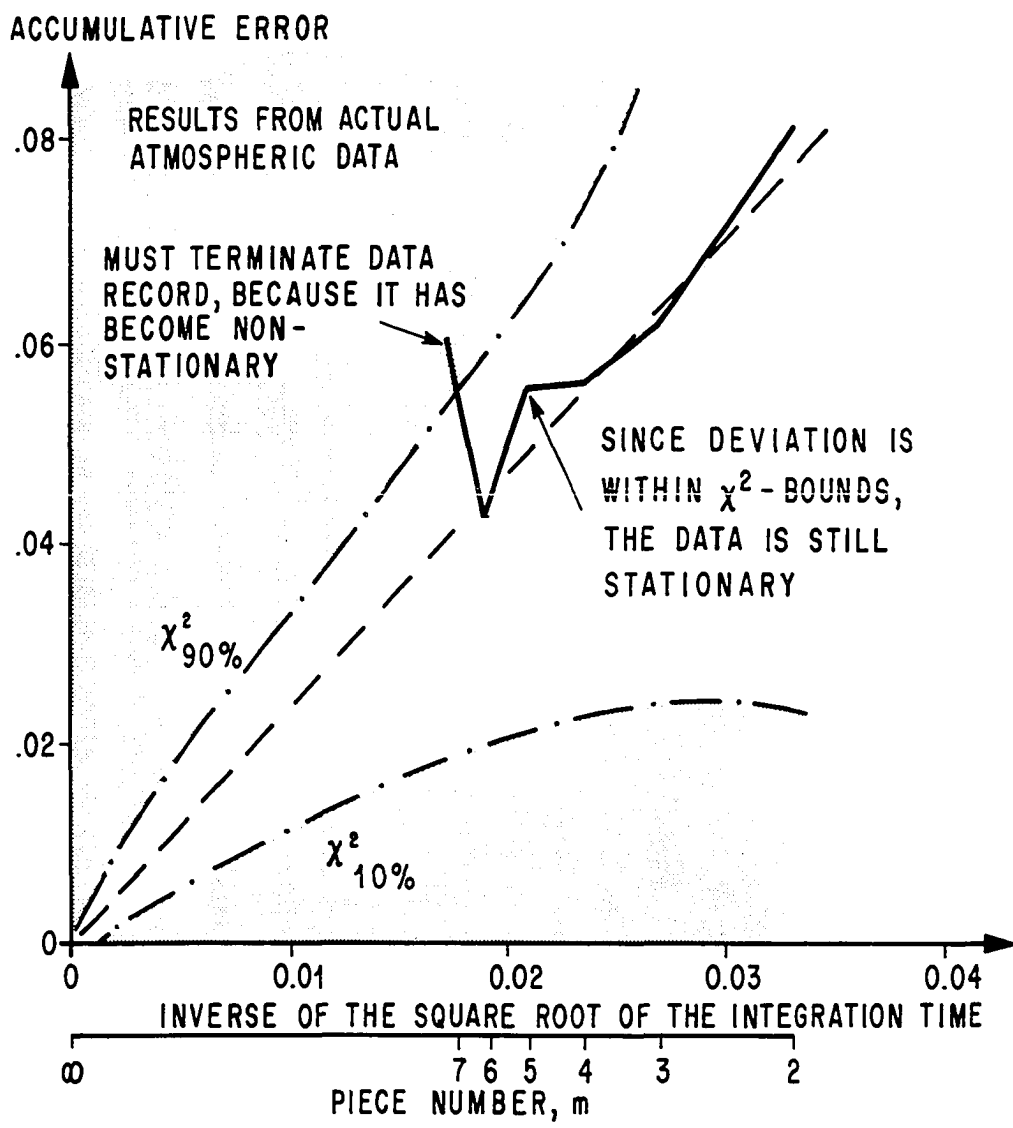
FIGURE 9. ACCUMULATIVE ERROR CURVE FOR A NONSTATIONARY PROCESS.
