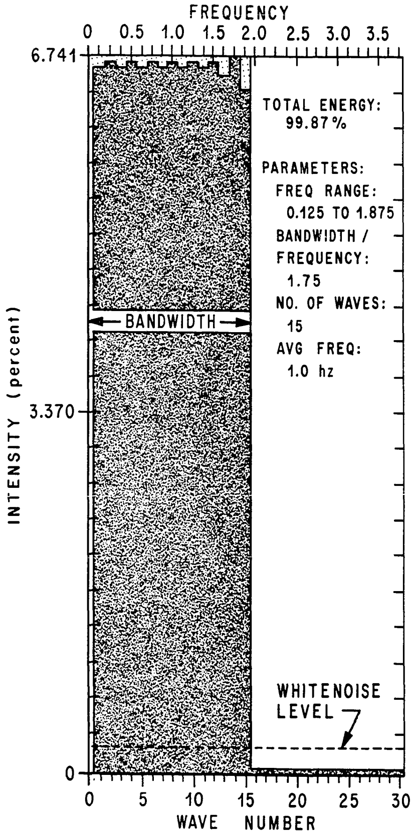
FIGURE 20. TRANSFORM OF SQUARE INPUT WITH INTEGRAL SPACING.
