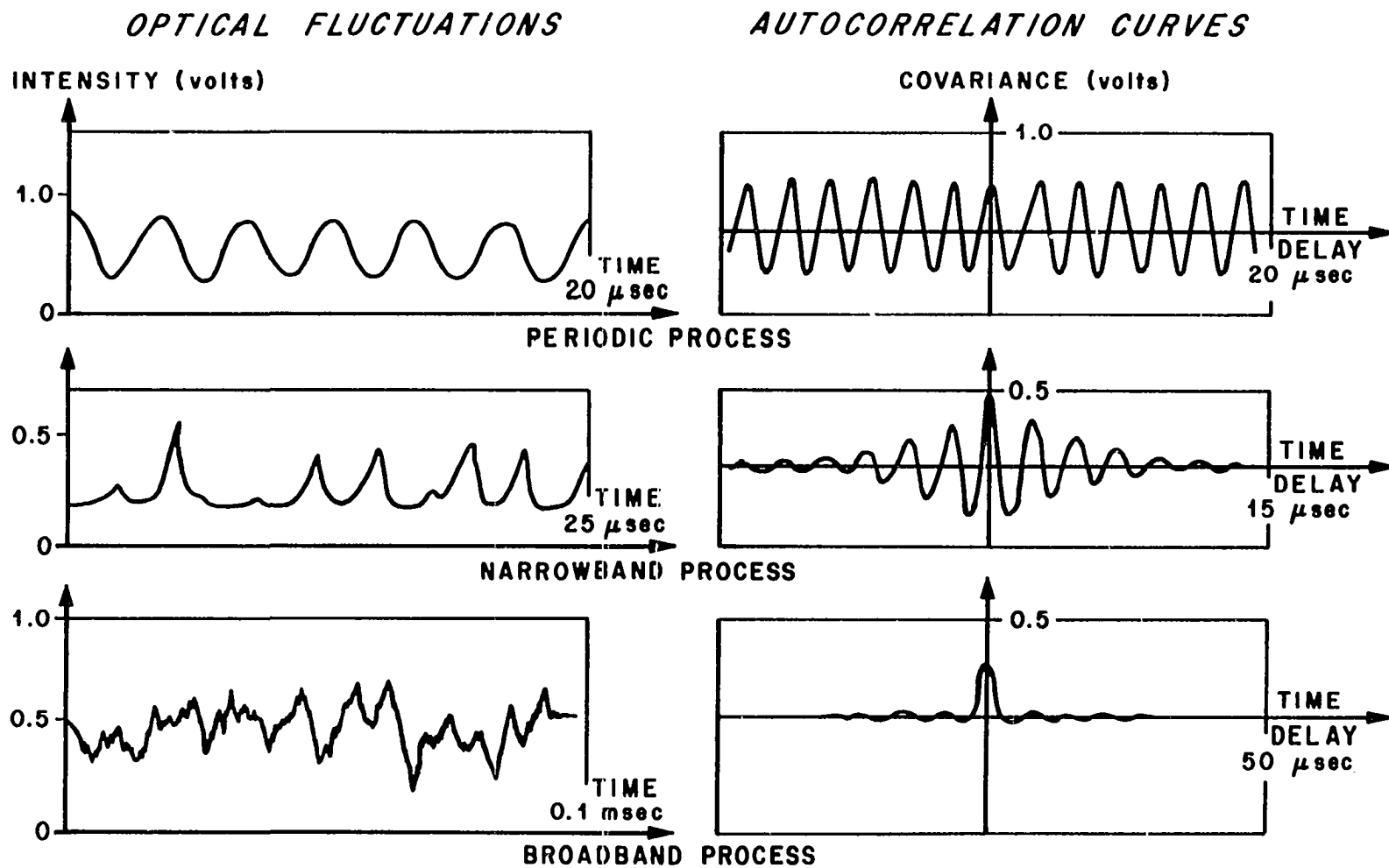
FIGURE 15. AUTOCORRELATION CURVES FOR MOVING STRIATIONS.
