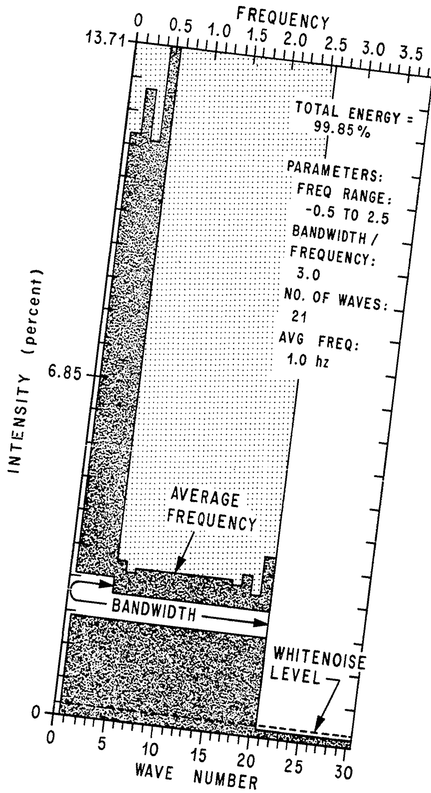
FIGURE 22. BROADBAND FOLDING.
