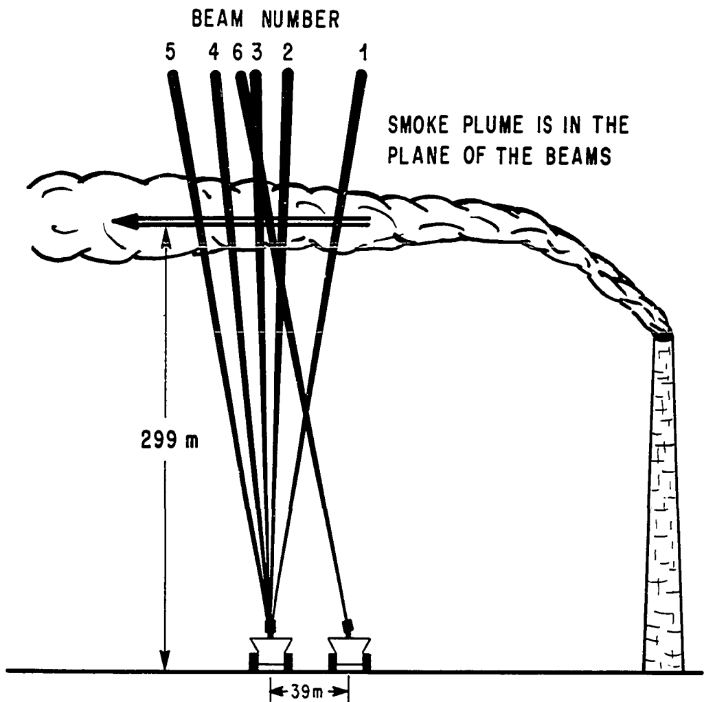
FIGURE 42. CROSSED-BEAM TEST ARRANGEMENT FOR FAN SYSTEM.
