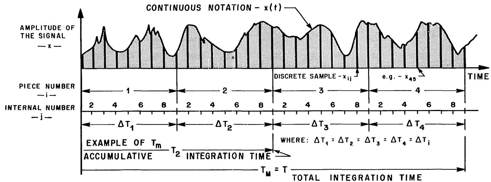
FIGURE 2. THE NOTATION OF THE TIME SERIES.
