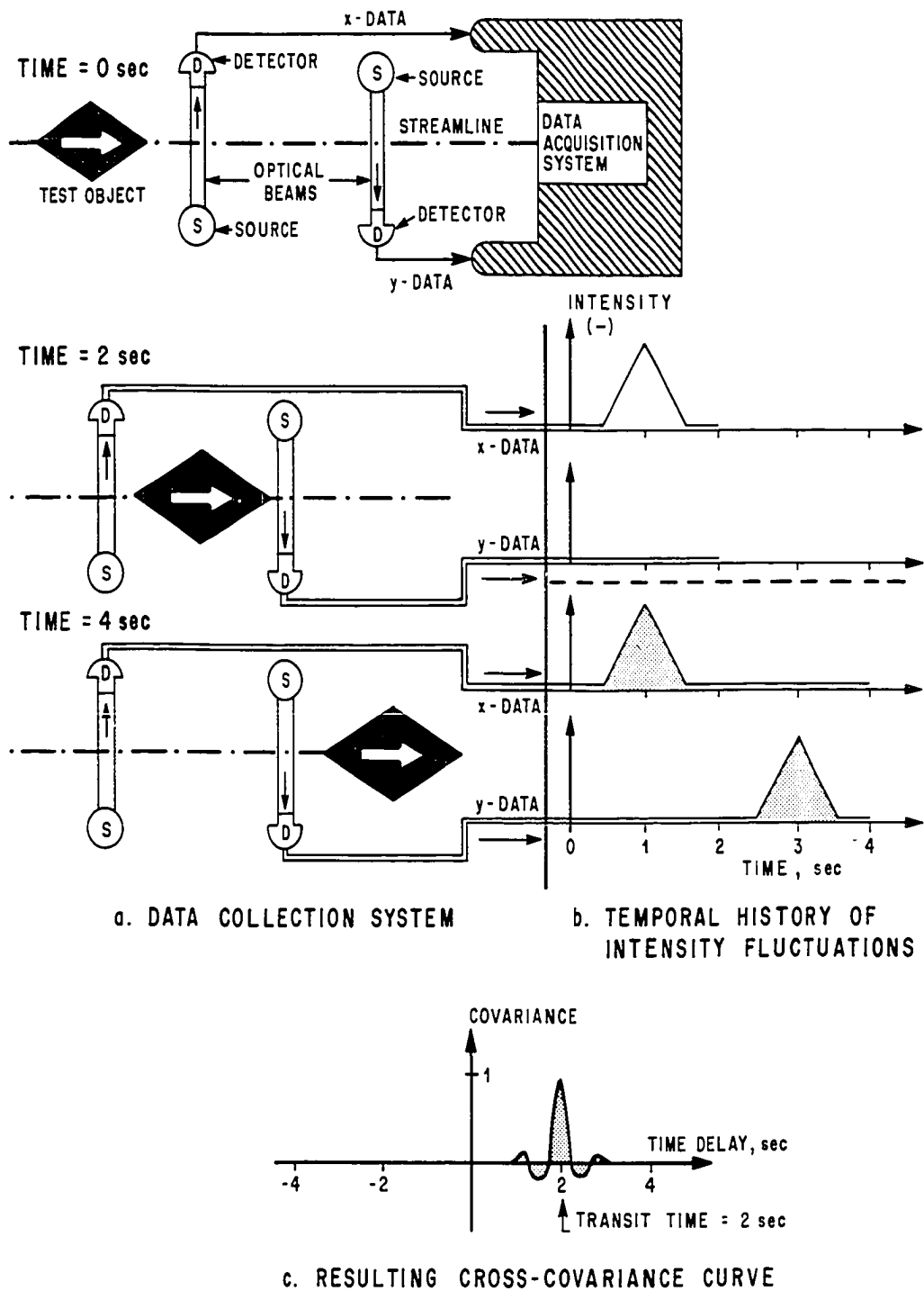
FIGURE 4. A ONE-EVENT, TWO-DIMENSIONAL PHYSICAL MODEL
