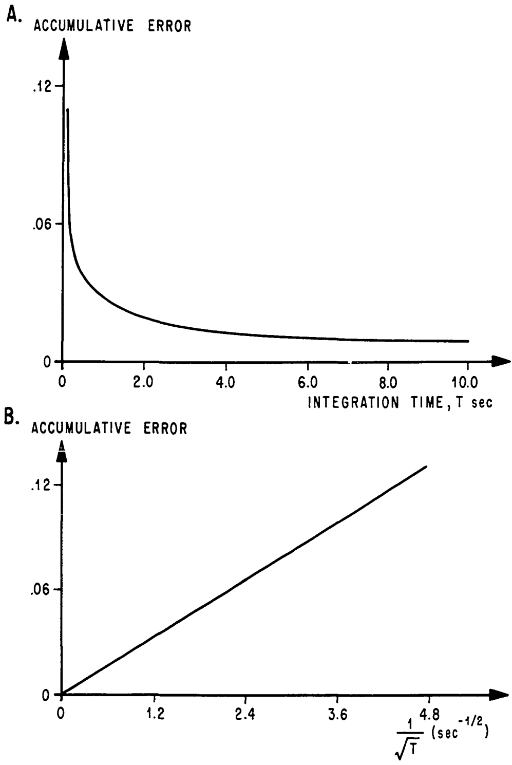
FIGURE 8. ACCUMULATIVE ERROR CURVE FROM COLD JET DATA [FISHER'S, JOHNSON'S]
