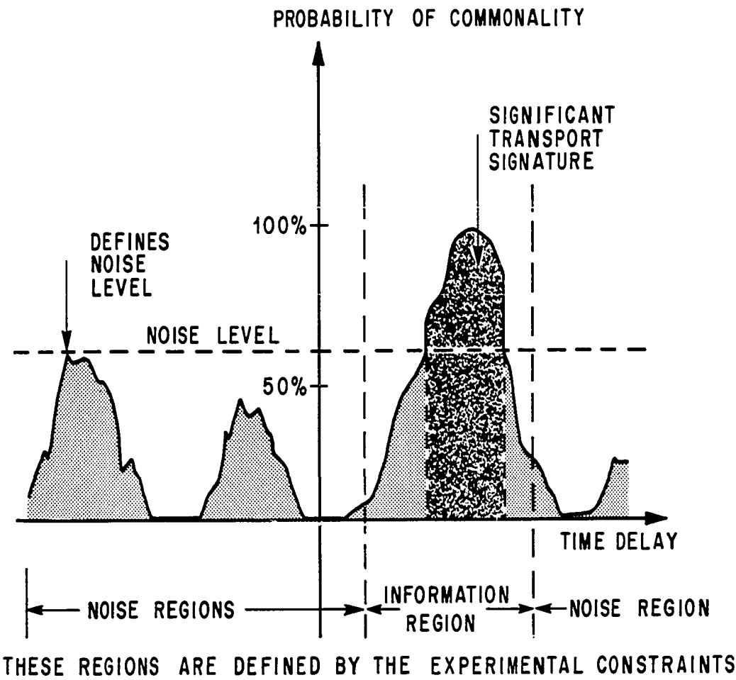
FIGURE 10. PROBABILITY OF COMMONALITY.
