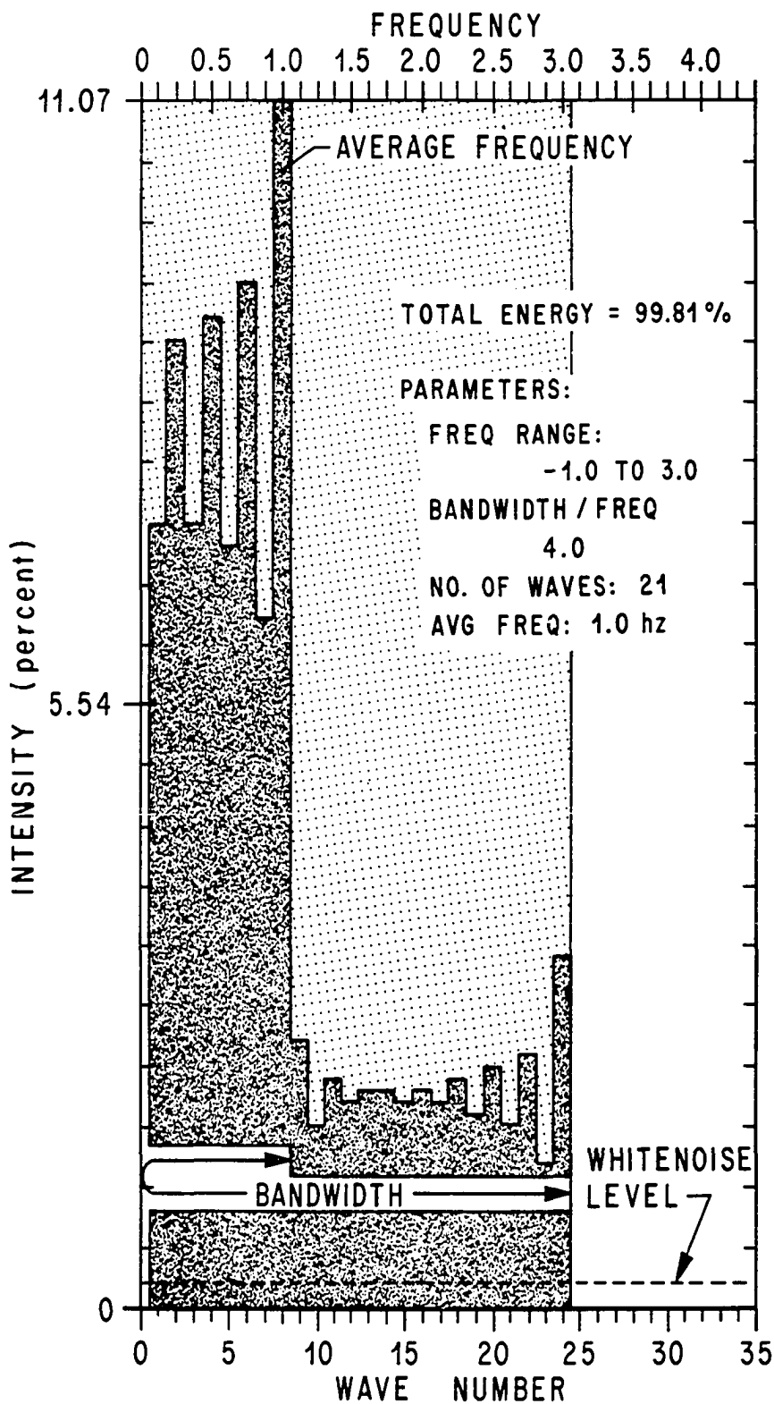
FIGURE 23. BROADBAND FOLDING AT AVERAGE FREQUENCY.
