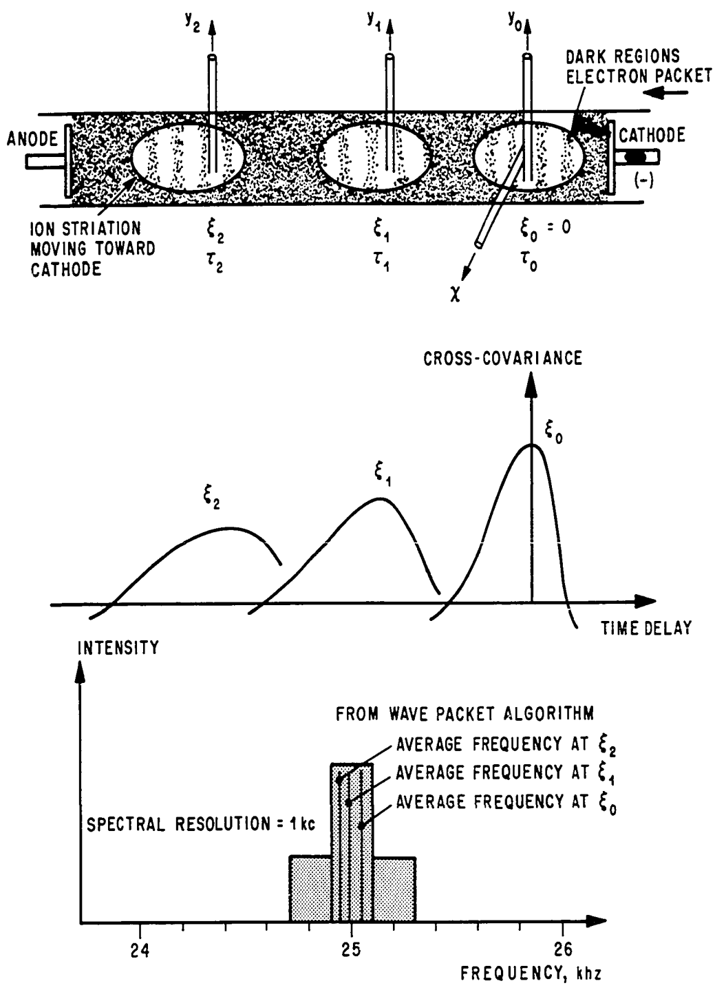
FIGURE 35. ELECTRON PACKET FLOW IN THE GLOW DISCHARGE.
