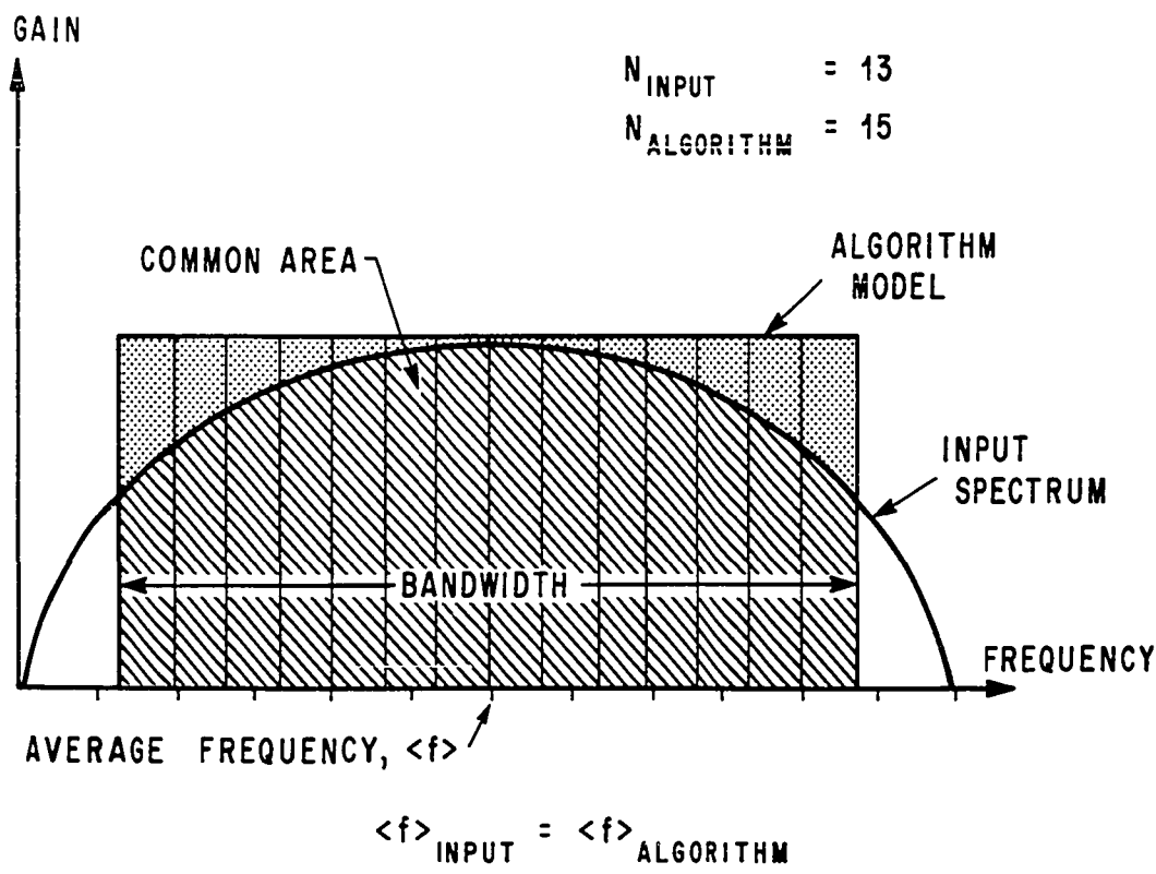
Figure 24. WAVE PACKET ALGORITHM FIT OF ELLIPTICAL ENVELOPE.
