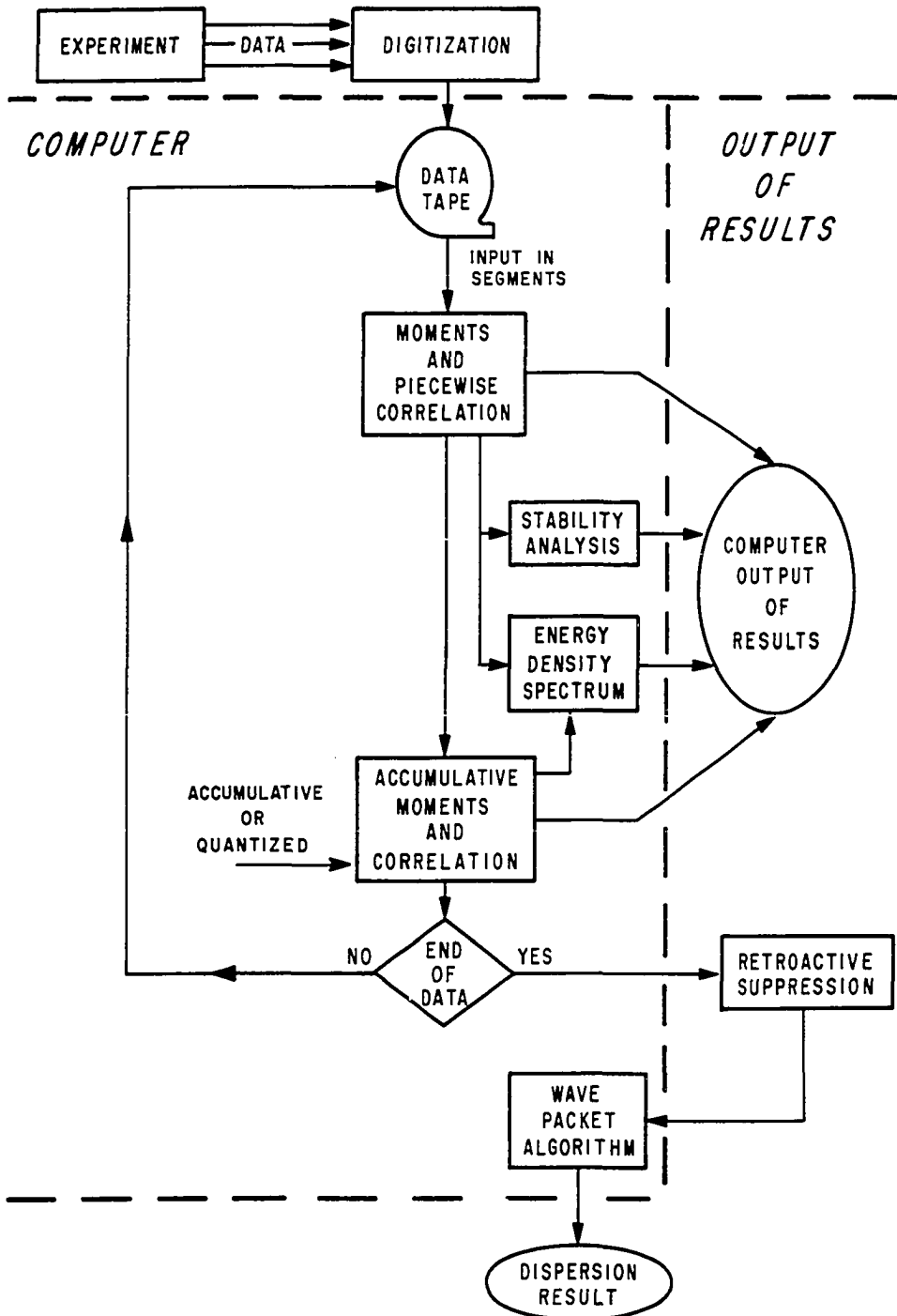
FIGURE 33. DATA REDUCTION BLOCK DIAGRAM FOR MLTCOR.
