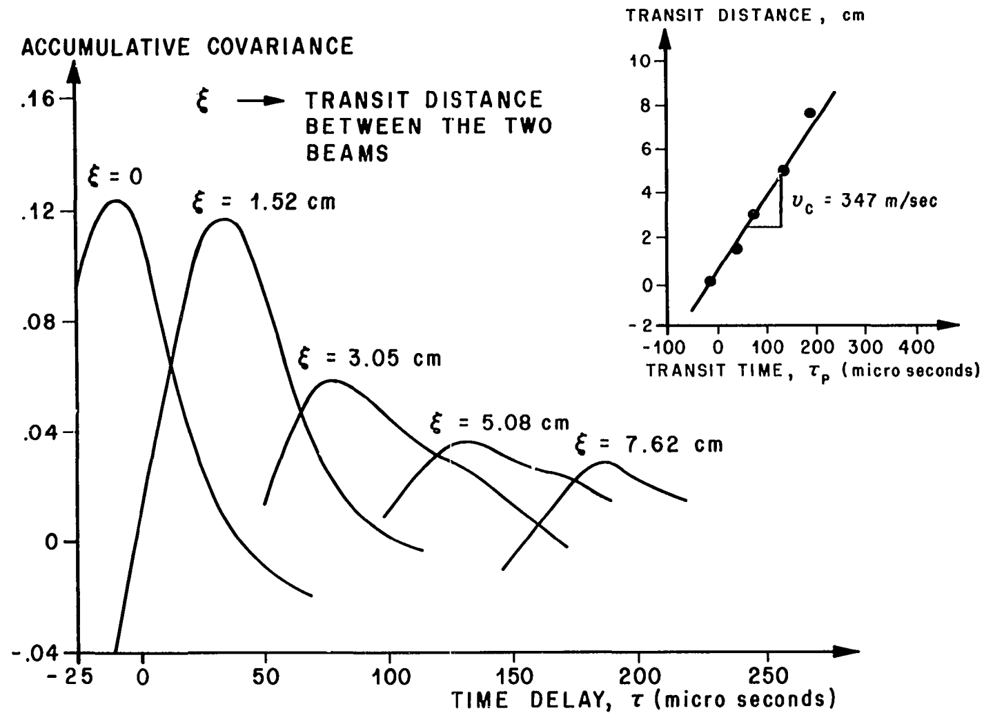
FIGURE 37. SPACE-TIME CORRELATION CURVES FOR COLD AIR JET.
