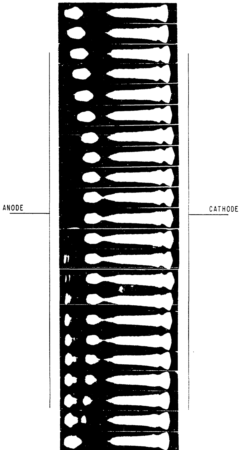
FIGURE 30. FORWARD-MOVING STRIATION.
