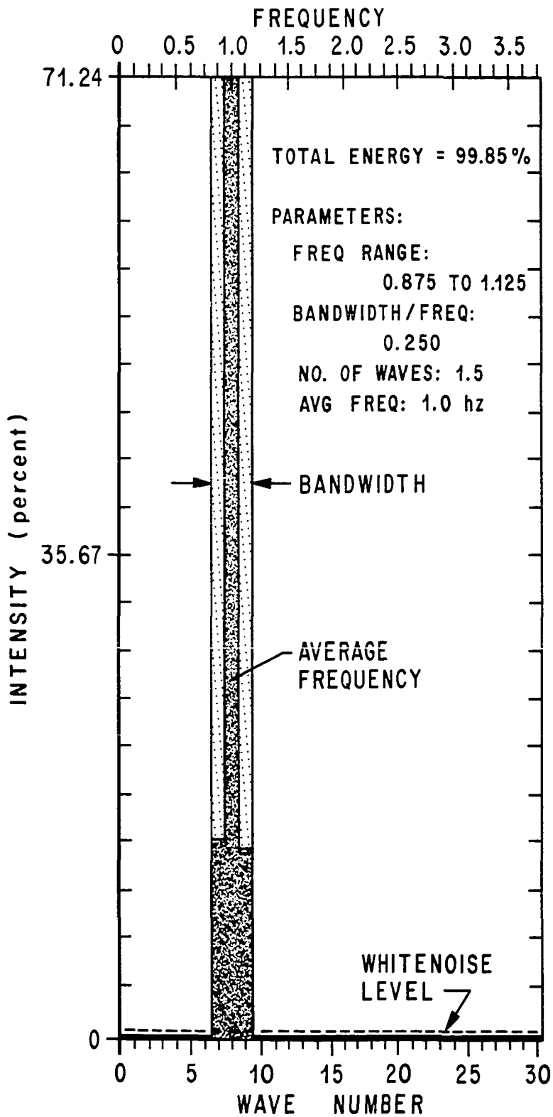
FIGURE 21. COMPRESSED BANDWIDTH.
