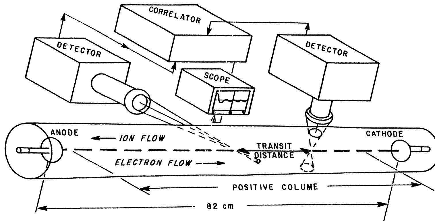
FIGURE 29. EXPERIMENTAL SETUP FOR GLOW DISCHARGE
