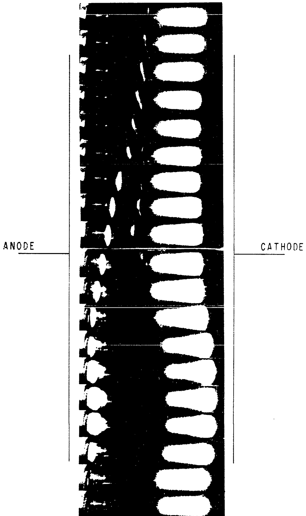
FIGURE 31. BACKWARD-MOVING STRAITION.
