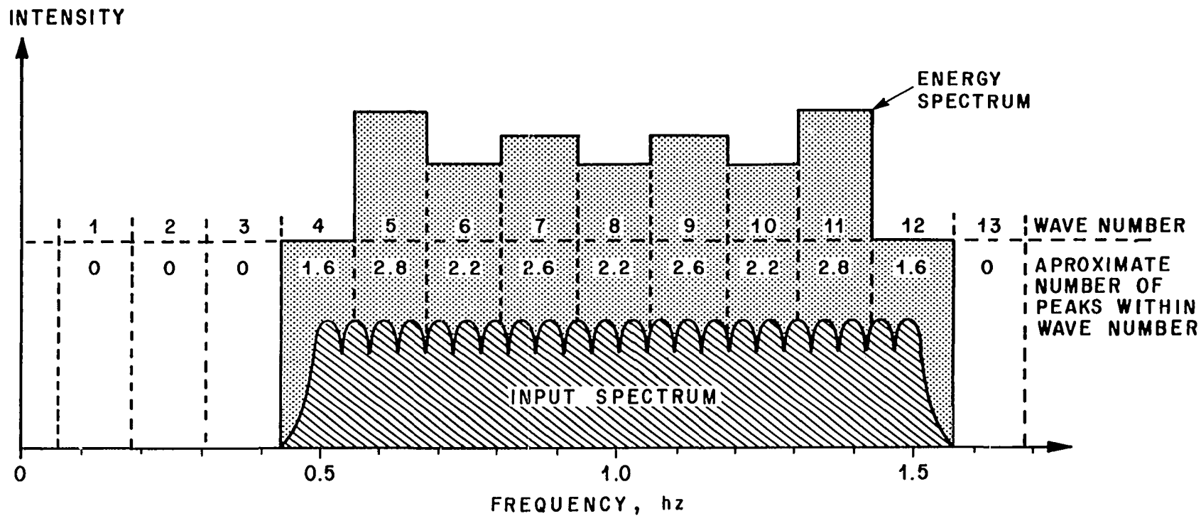
FIGURE 11. GRAPHICAL RELATION BETWEEN INPUT SPECTRUM AND ENERGY DENSITY SPECTRUM.
