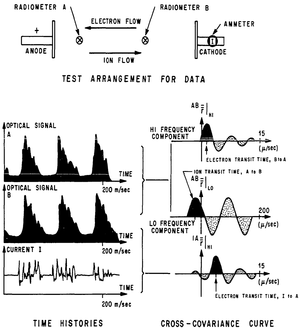
FIGURE 32. SEPARATION OF ELECTRON AND ION TRANSPORT.
