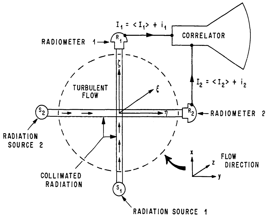
FIGURE 27. SCHEMATIC CROSS SECTION FOR THE CROSSED BEAM MONITORING SYSTEM IN A TURBULENT FLOW.
