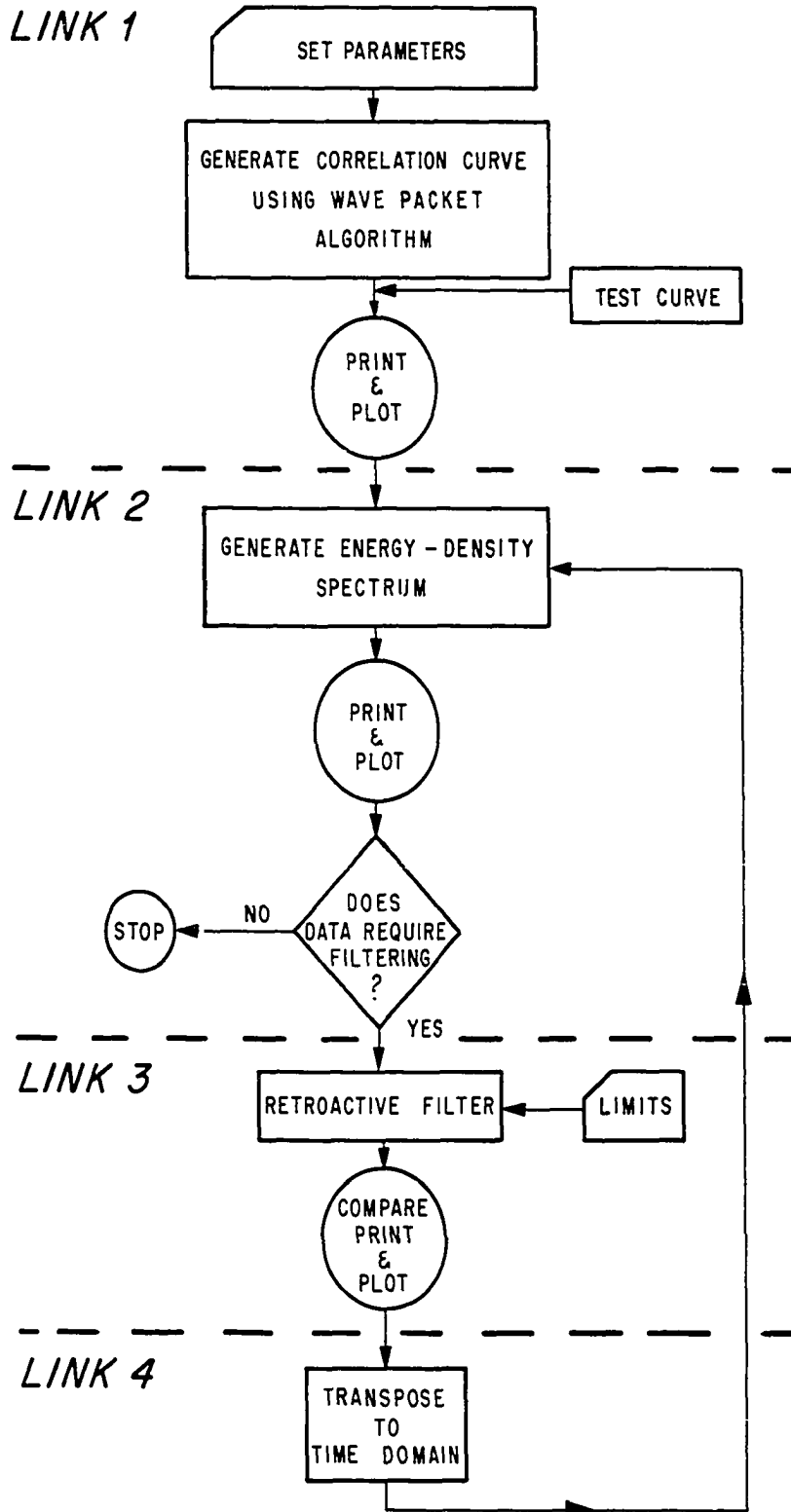
FIGURE 18. FLOW DIAGRAM OF SPECTRAL DECOMPOSITION PROGRAM.
