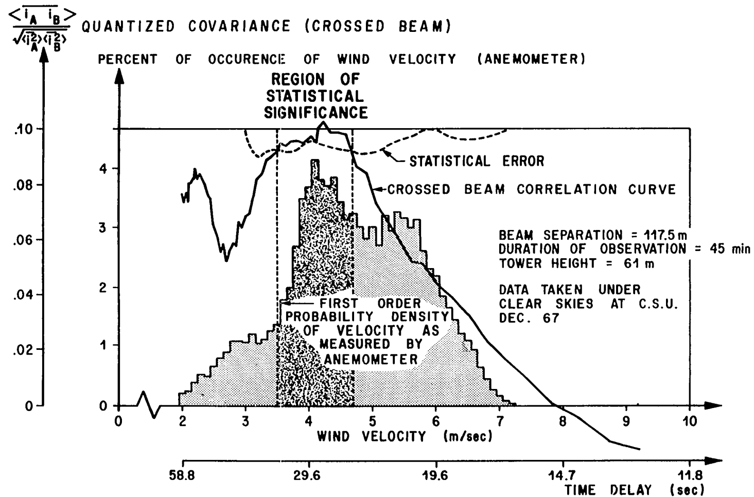
FIGURE 41. CROSSED BEAM AND ANEMOMETER COMPARISONS
