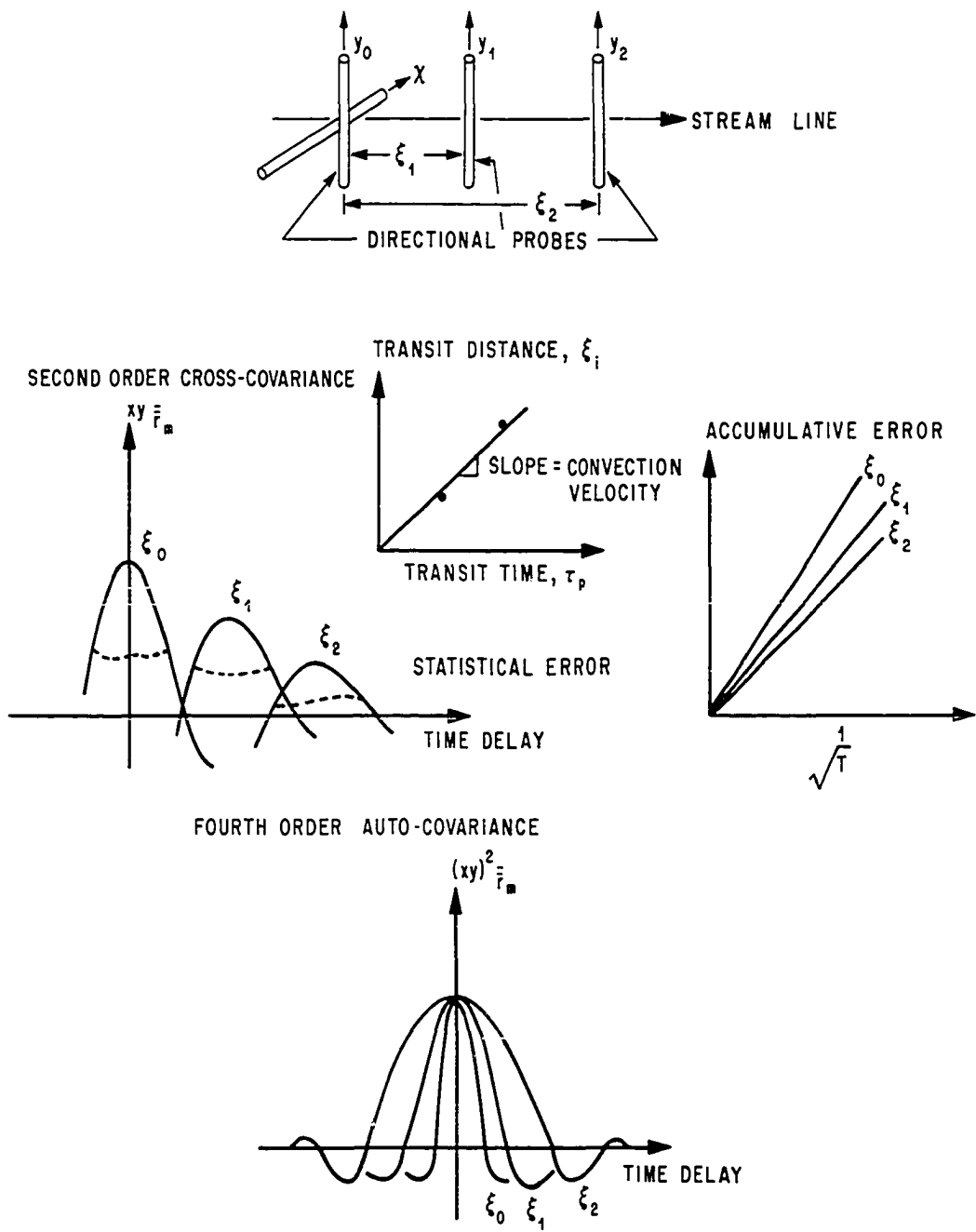
FIGURE 26. RETRIEVAL OF CONVECTIVE AND DISPERSIVE TRANSPORT.
