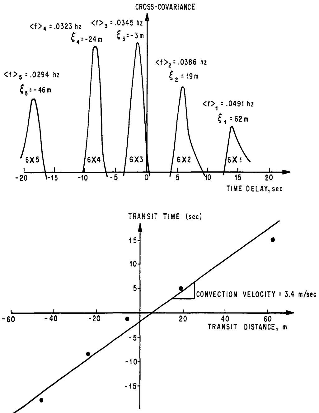
FIGURE 43. SMOKE-PLUME CONVECTION AND DISPERSION TRANSPORT.
