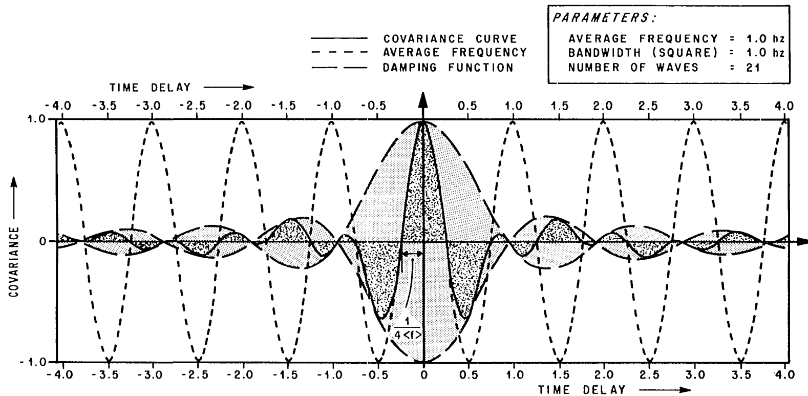
FIGURE 16. COVARIANCE CURVE FROM THE WAVE PACKET ALGORITHM
