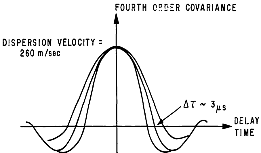
FIGURE 36. CONVECTION AND DISPERSION VELOCITIES FOR ELECTRON FLOW.
