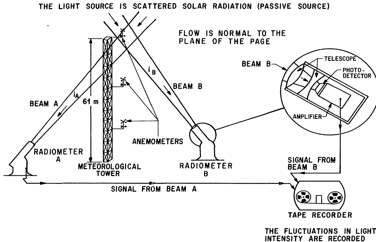
FIGURE 40. ATMOSPHERIC CROSSED BEAM DETECTION SYSTEM FOR CLEAR-AIR TURBULENCE.
