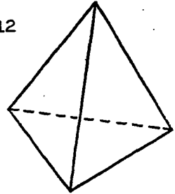
Tetrahedron
