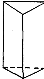
Triangular prism
