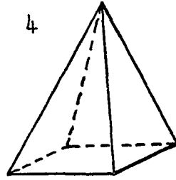
Square pyramid
