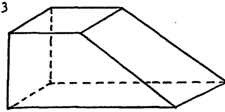
Trapezoidal solid
