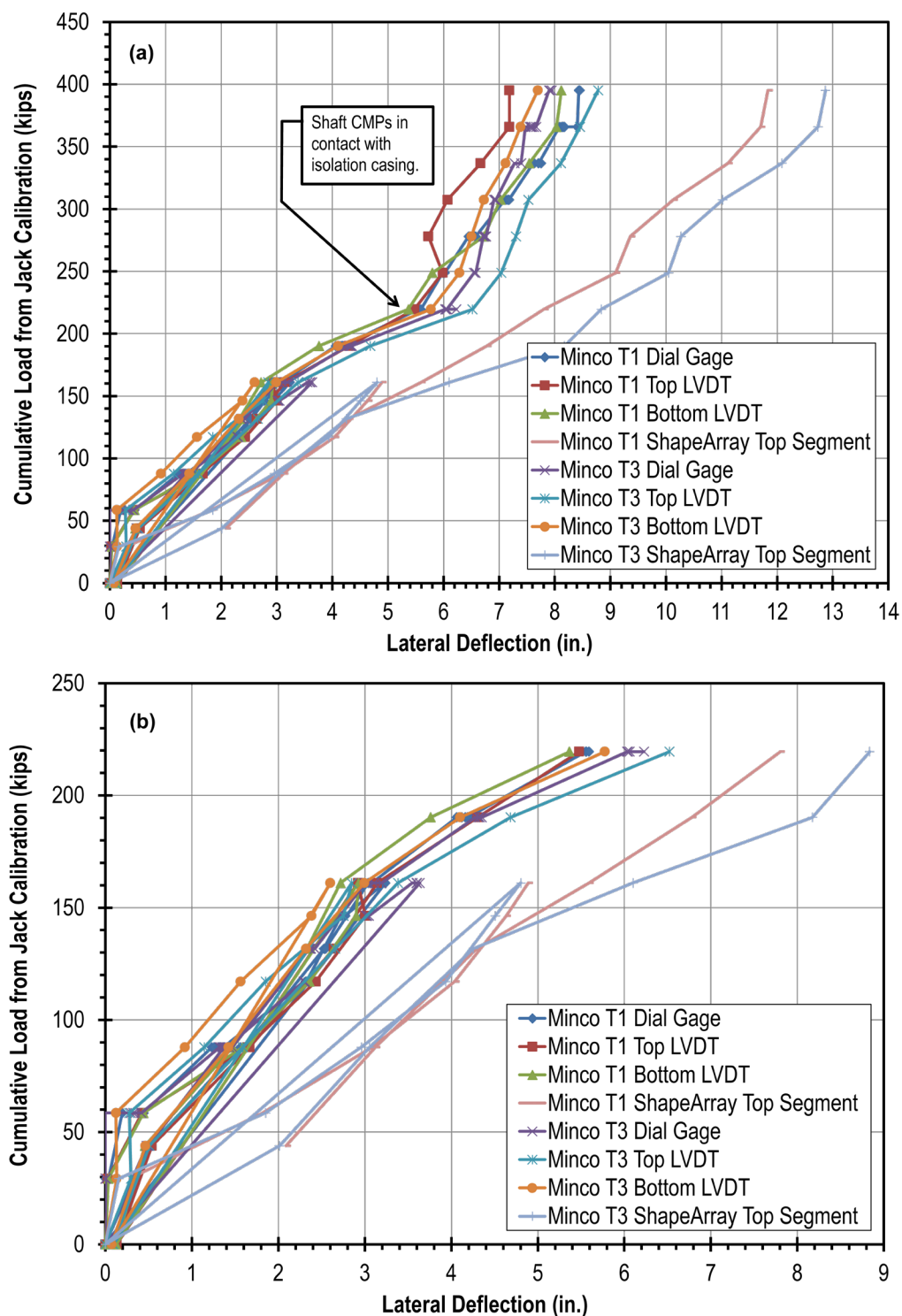
Figure 7.19 – Load-displacement curves for test of Minco shafts T1 and T3: (a) full test and (b) without load steps after shaft was clearly in contact with casing.
