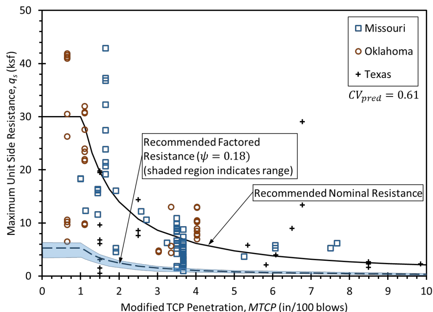
Figure 6.10 – Recommended nominal and factored unit side resistance for recommended TCPT-based design relation.
