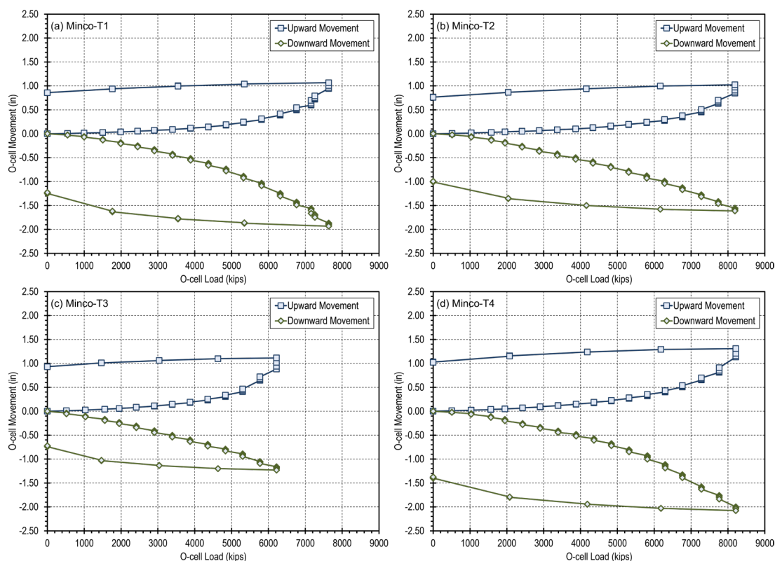
Figure 5.5 – Measured axial load-displacement response for Minco test shafts: (a) Minco-T1, (b) Minco-T2, (c) Minco-T3, and (d) Minco-T4.
