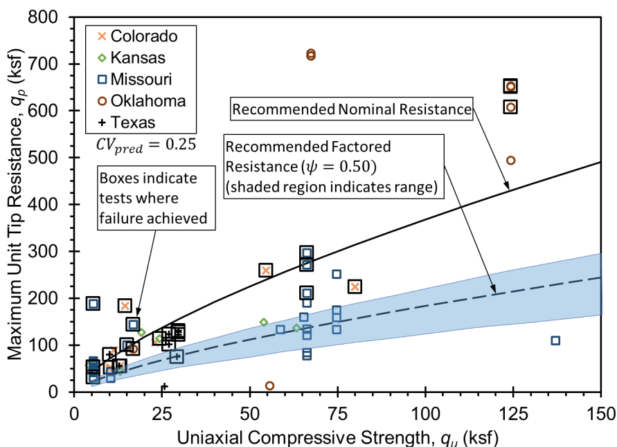
Figure 6.12 – Recommended nominal and factored unit tip resistance for recommended compressive strength-based design relation.
