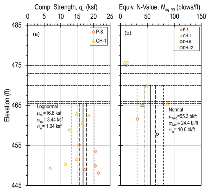
Figure 3.12 – Direct measurements of design parameters for the Hugo test site: (a) compressive strength and (b) SPT N -values.
