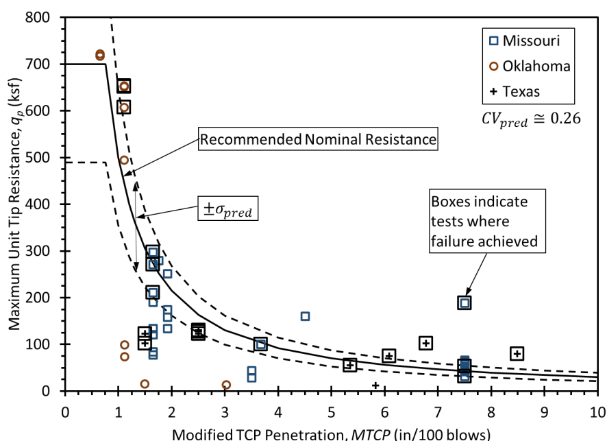
Figure 6.2 – Unit tip resistance from collected load tests in weak rock with recommended relation for design from TCPT measurements.
