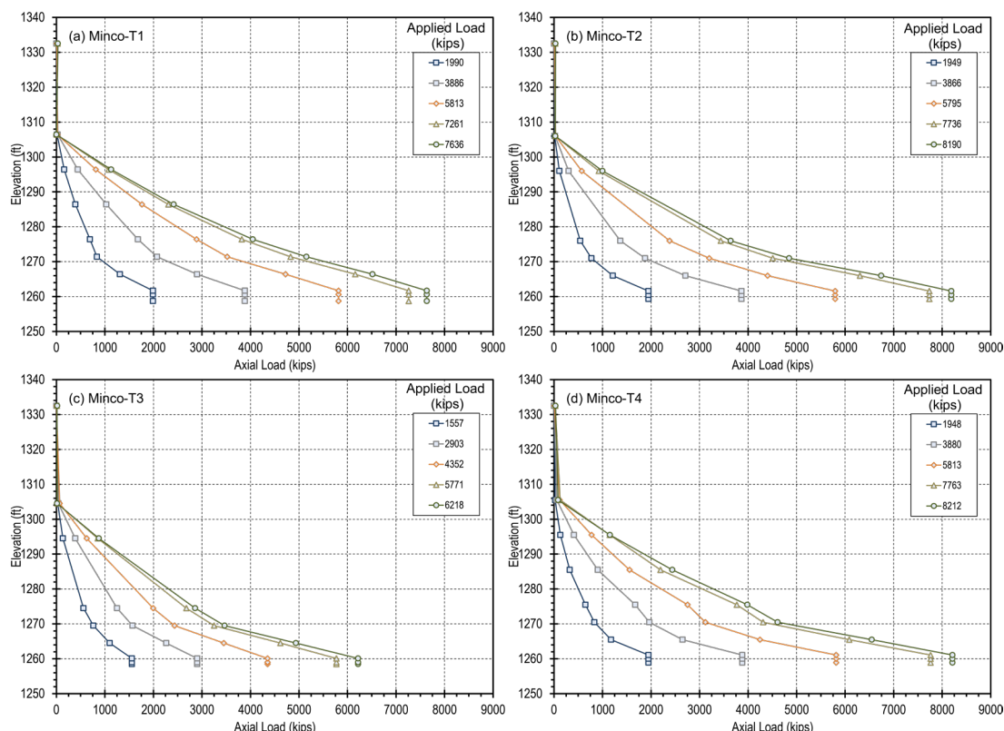
Figure 5.6 – Interpreted load transfer for Minco test shafts: (a) Minco-T1, (b) Minco-T2, (c) Minco-T3, and (d) Minco-T4.
