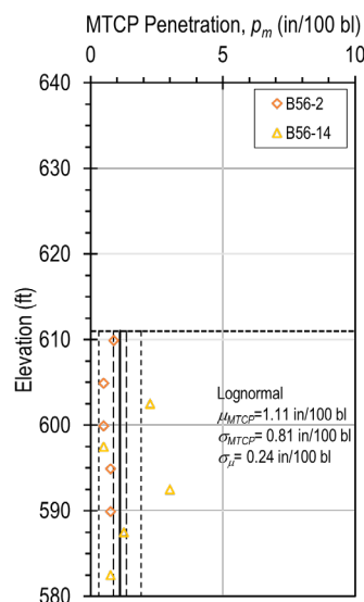
Figure 3.11 – TCPT penetration measurements for the Broken Arrow test site.
