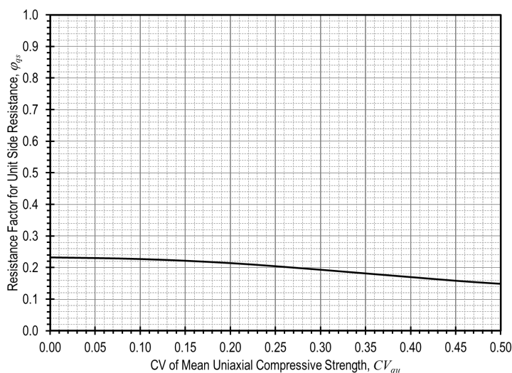
Figure 6.13 – Resistance factors for unit side resistance from compressive strength for weak rock.
