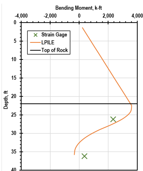
Figure 8.6 – Bending moments interpreted from strain gages and from calibrated L-PILE model for Minco T2 at an applied load of 161 kips.
