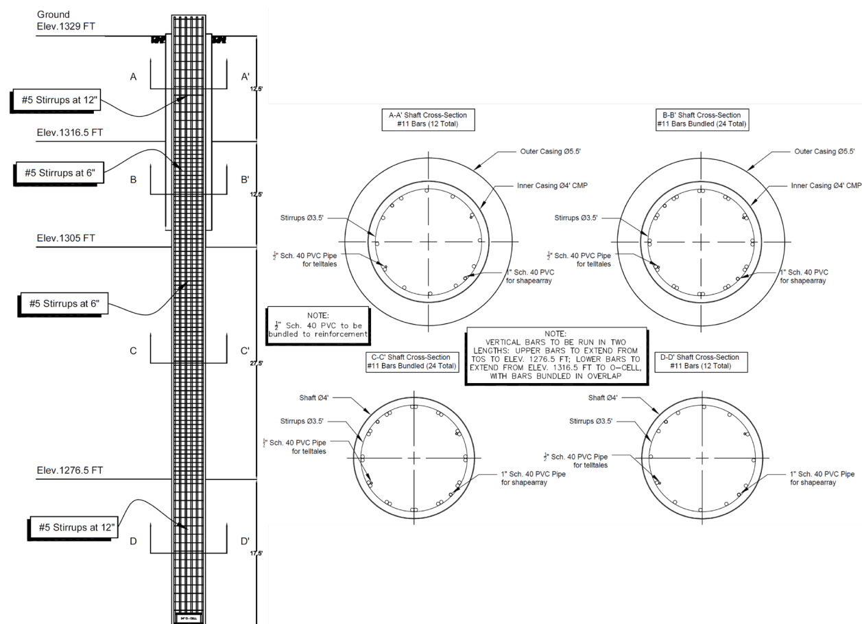
Figure 4.11 – Schematic drawings of test shafts at Minco site showing reinforcement details.
