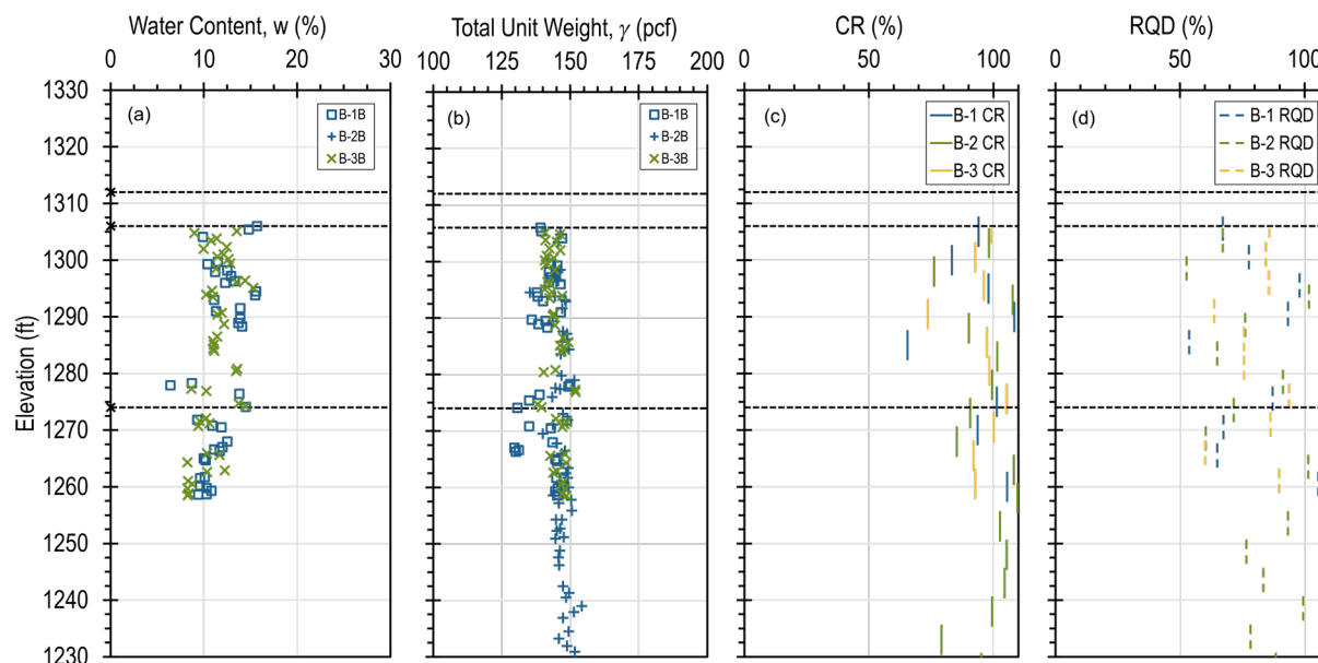
Figure 3.6 – Site characterization measurements for Minco test site: (a) water content, (b) total unit weight, (c) core recovery, and (d) RQD.
