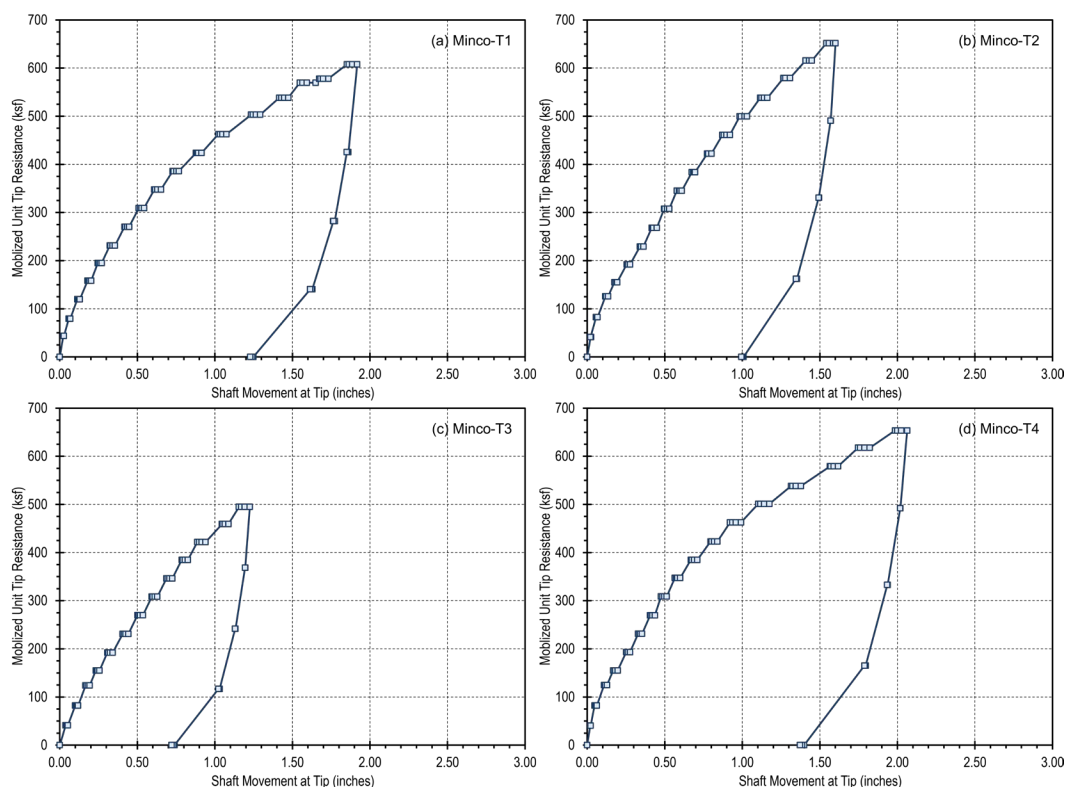
Figure 5.8 – Interpreted q - z response for Minco test shafts: (a) Minco-T1, (b) Minco-T2, (c) Minco-T3, and (d) Minco-T4.
