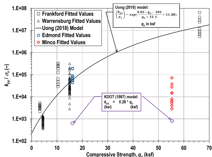
Figure 8.12 – Proposed relationship between k_{py} and compressive strength.
