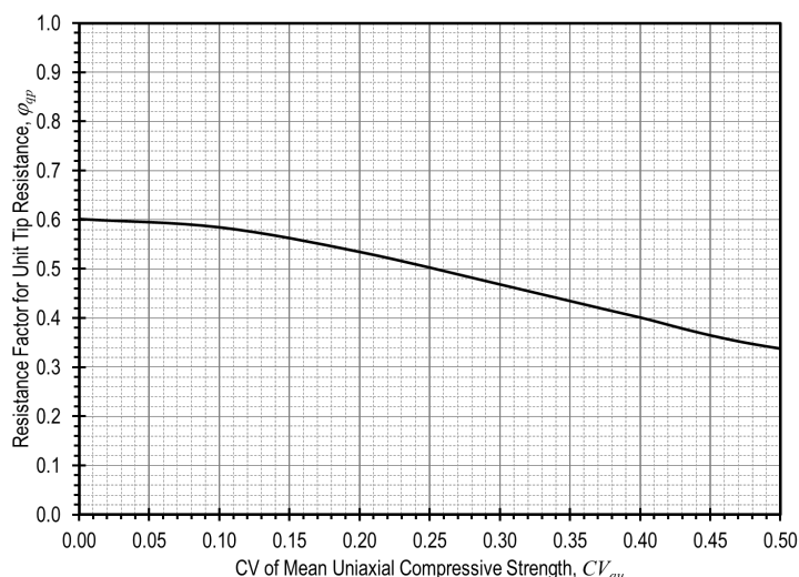
Figure 6.11 – Resistance factors for unit tip resistance from compressive strength for weak rock.
