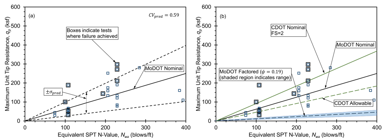
Figure 2.6 – MoDOT design relation for unit tip resistance in weak rock from SPT equivalent N -values: (a) nominal resistance showing prediction uncertainty and (b) nominal and factored unit resistance for MoDOT design method and allowable and nominal unit resistance from CDOT design method.
