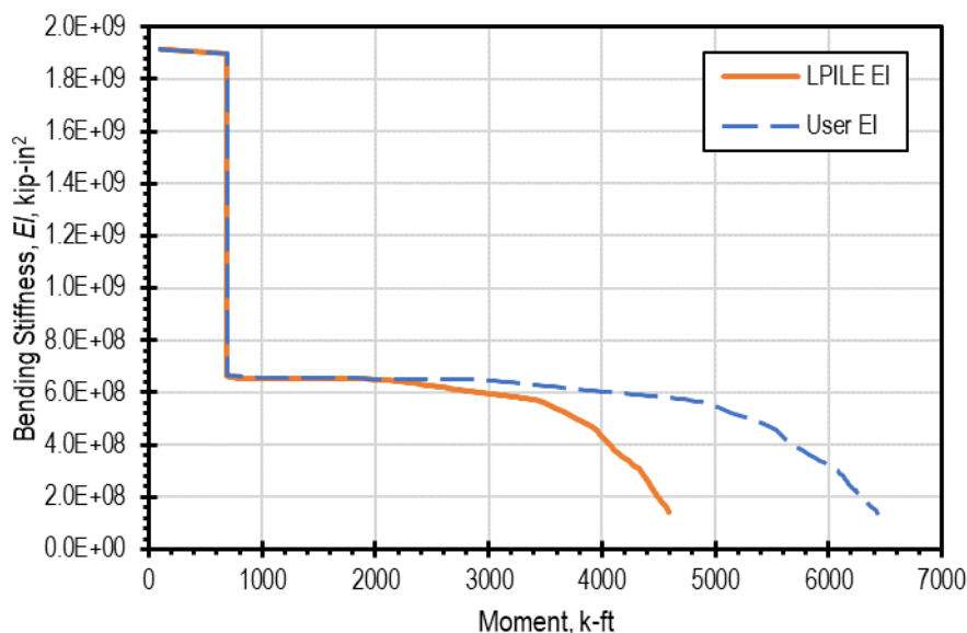
Figure 7.23 – Example user-input EI - M curve for Minco.
