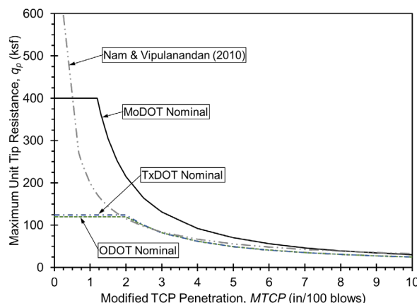
Figure 2.9 – Comparison of nominal unit tip resistance from different TCP-based design methods.
