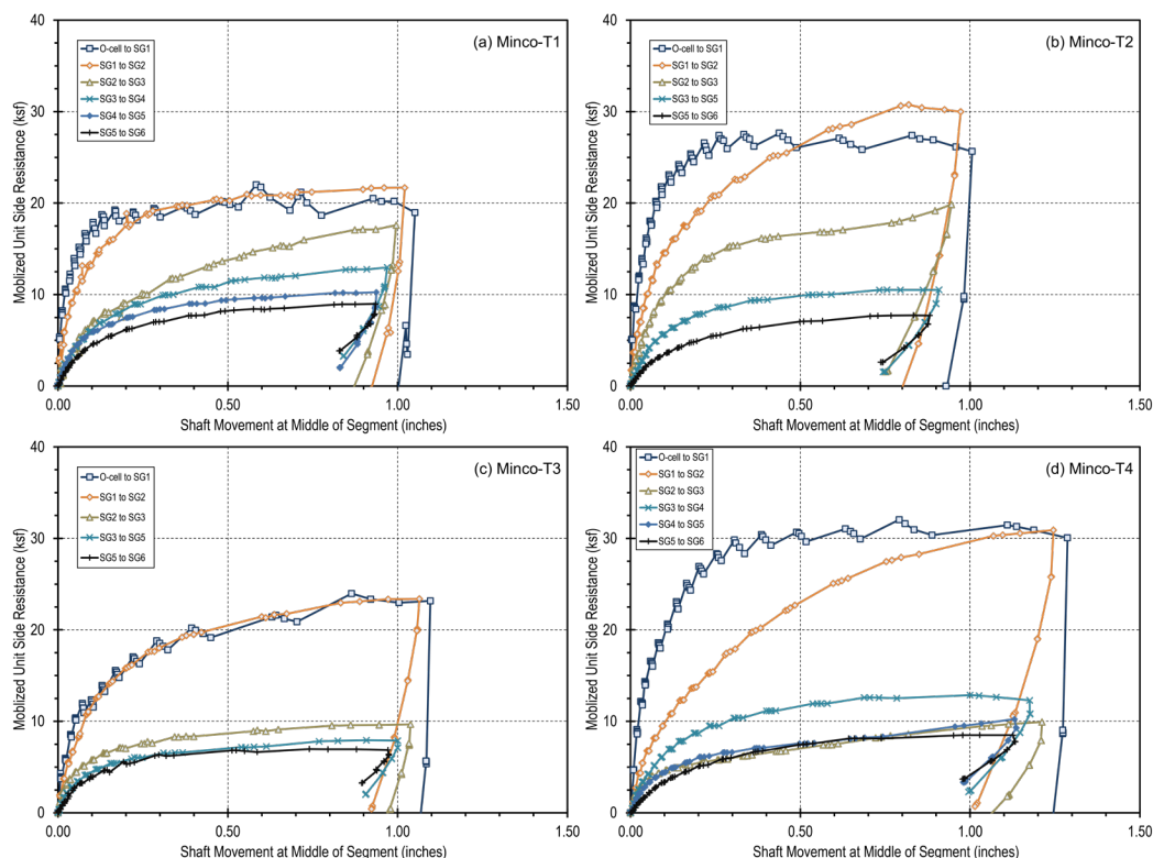
Figure 5.7 – Interpreted t - z response for Minco test shafts: (a) Minco-T1, (b) Minco-T2, (c) Minco-T3, and (d) Minco-T4.
