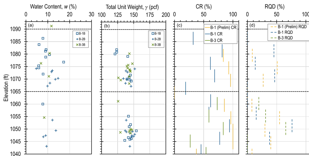
Figure 3.2 – Site characterization measurements for Edmond test site: (a) water content, (b) total unit weight, (c) core recovery, and (d) RQD.
