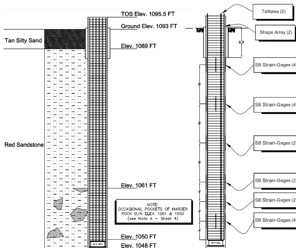
Figure 4.3 – Profile drawings of test shafts at Edmond site showing approximate depths of casing, bi-directional loading device, and instrumentation.
