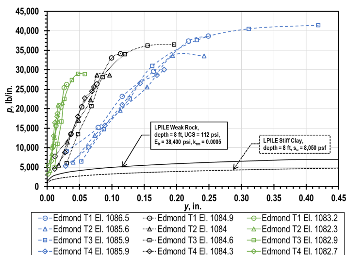
Figure 8.7 – Calibrated p - y curves for Edmond.
