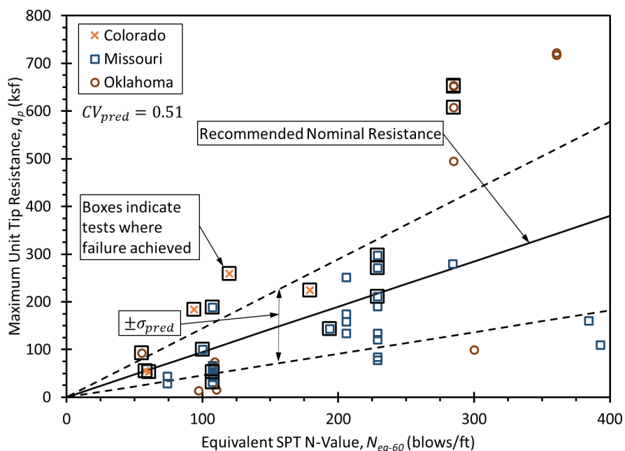
Figure 6.6 – Unit tip resistance from collected load tests in weak rock with recommended relation for design from N_{eq-60} .
