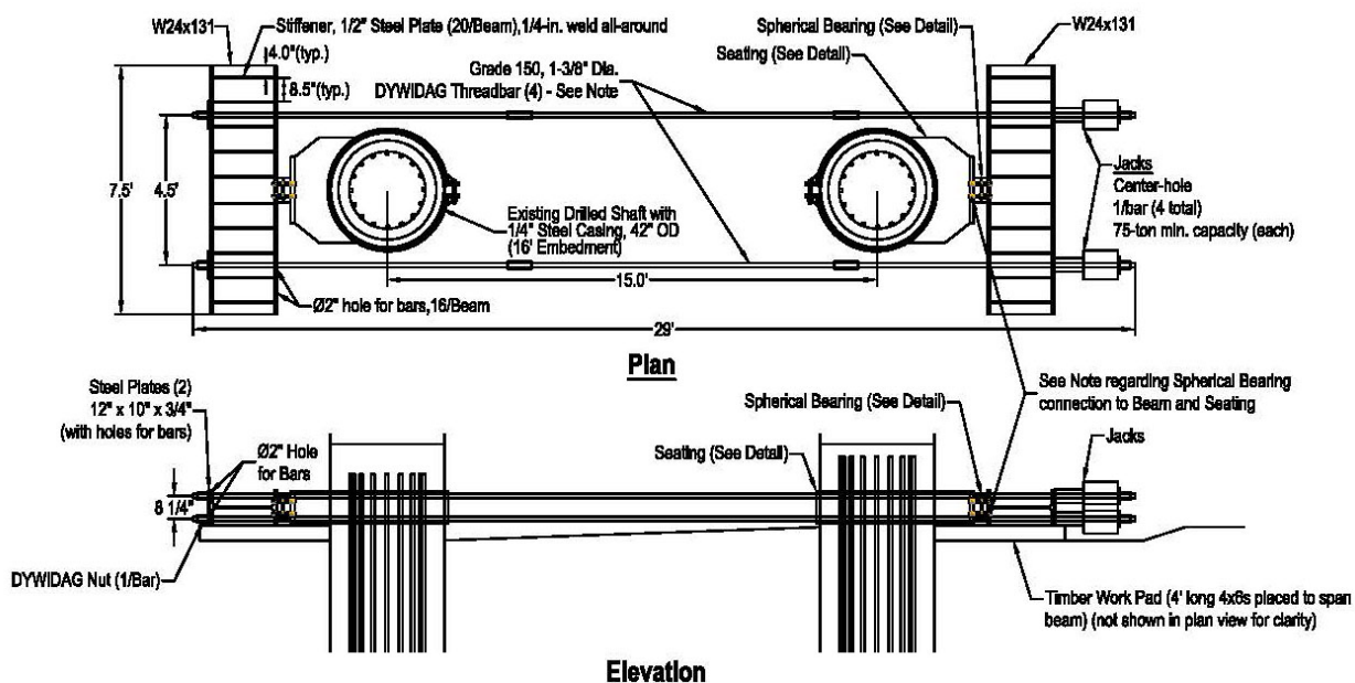
Figure 7.4 – Plan and elevation views of lateral load test frame.
