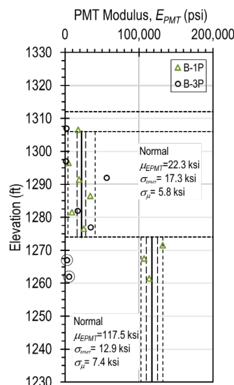
Figure 3.8 – Measurements of Pressuremeter Modulus for the Minco test site.
