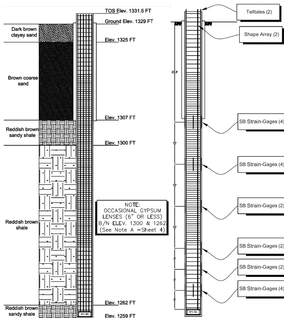
Figure 4.10 – Profile drawings of test shafts at Minco site showing approximate depths of casing, bi-directional loading device, and instrumentation.
