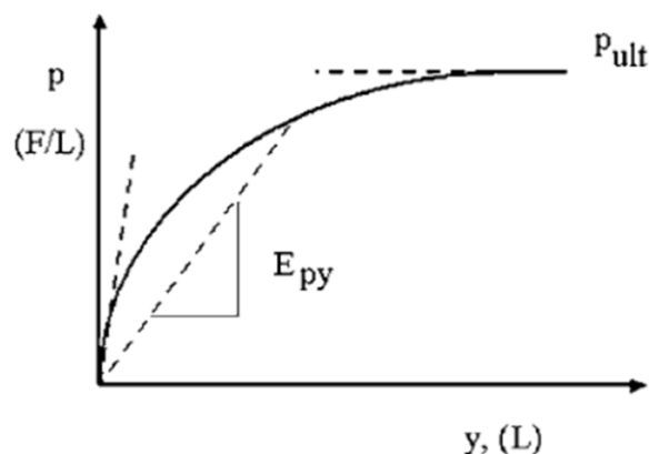
Figure 8.2 – Conceptual p - y curve (Reese et al., 2006).
