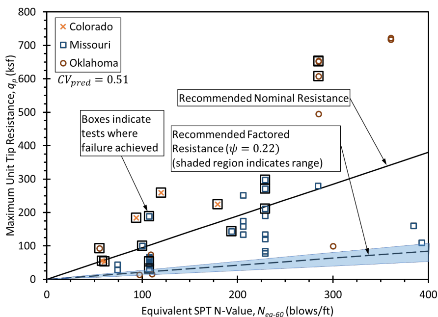
Figure 6.16 – Recommended nominal and factored unit tip resistance for recommended SPT-based design relation.
