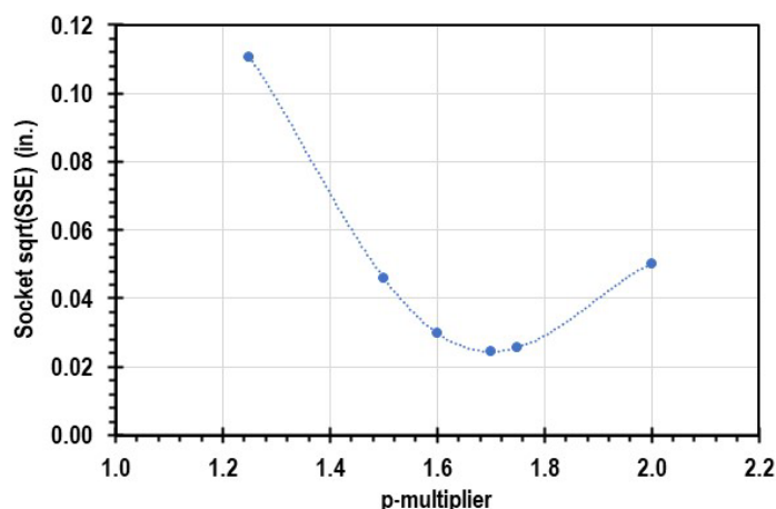
Figure 8.4 – Example plot of \sqrt{SSE} versus p -multiplier (for Minco T2 at 161 kips applied load).
