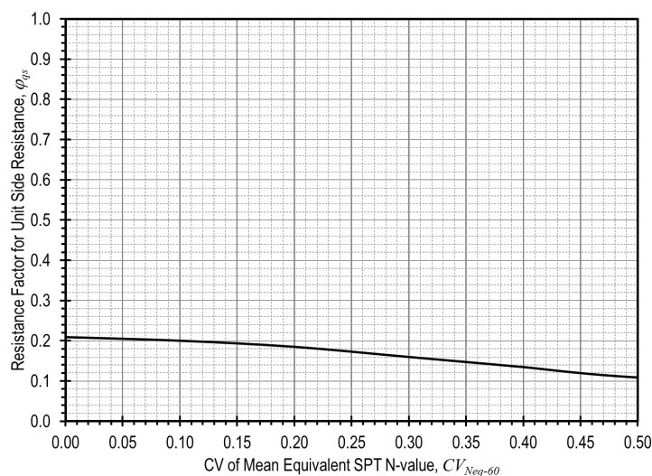
Figure 6.17 – Resistance factors for unit side resistance from SPT N_{eq-60} .
