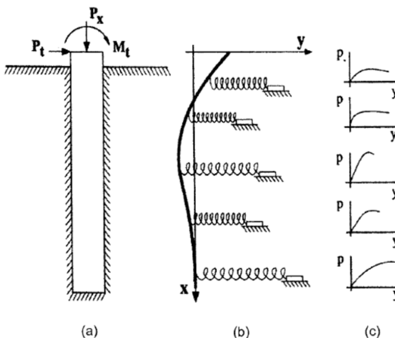
Figure 8.1 – Schematic representation of the p - y method: (a) deep foundation subjected to lateral loading, (b) soil modeled as a series of springs, and (c) p - y curves governing spring stiffness (Reese et al., 2006).
