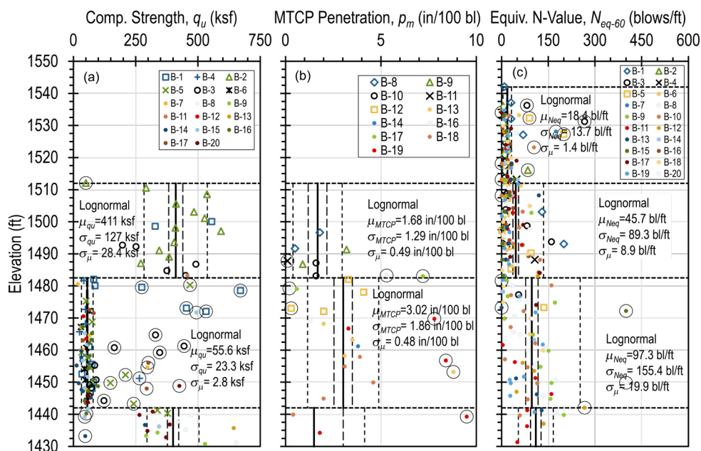
Figure 3.10 – Direct measurements of design parameters for the Harmon County test site: (a) compressive strength, (b) TCPT penetration, and (c) SPT N -values.
