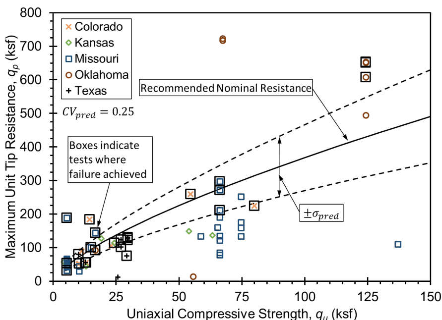
Figure 6.4 – Ultimate unit tip resistance from collected load tests in weak rock with recommended relation for design from compressive strength.
