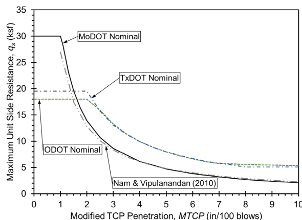
Figure 2.8 – Comparison of nominal unit side resistance from different TCP-based design methods.
