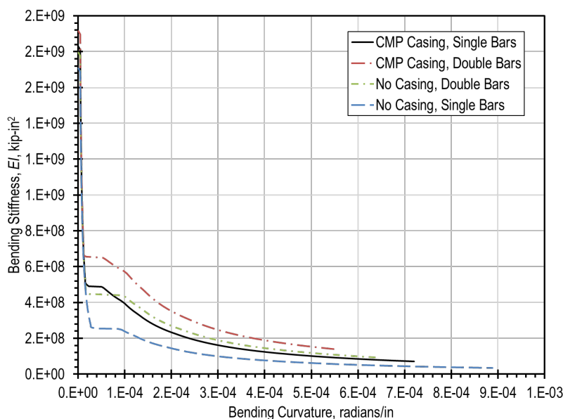
Figure 7.22 – Bending stiffness curve for Minco test shafts.
