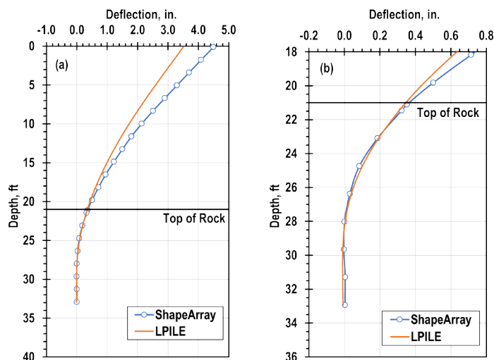
Figure 8.5 – Measured ShapeArray and calibrated L-PILE displacement values for Minco T2 at an applied load of 161 kips: (a) from top of shaft and (b) top of rock only.
