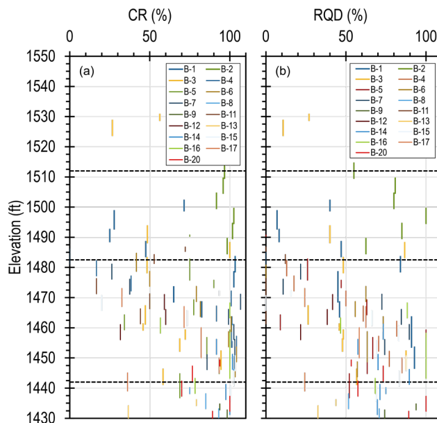
Figure 3.9 – Site characterization measurements for Harmon County test site: (a) core recovery, and (b) RQD.
