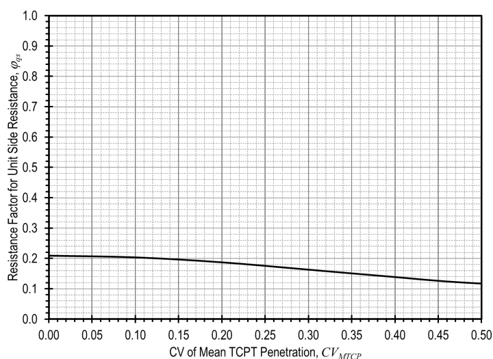
Figure 6.9 – Resistance factors for unit side resistance from TCPT penetration for weak rock.
