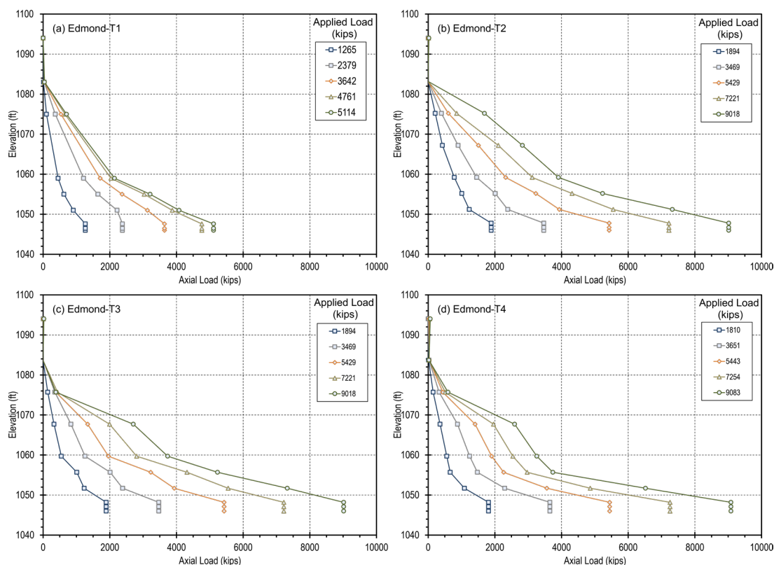
Figure 5.2 – Interpreted load transfer for Edmond test shafts: (a) Edmond-T1, (b) Edmond-T2, (c) Edmond-T3, and (d) Edmond-T4.
