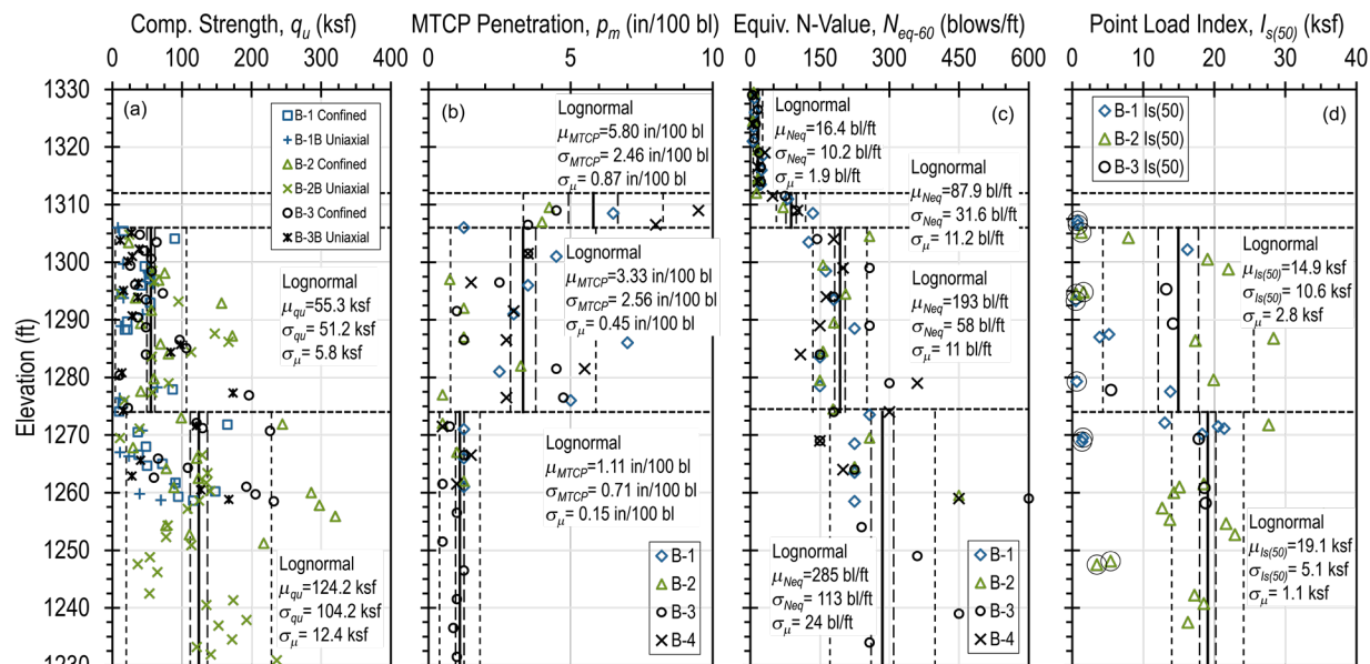
Figure 3.7 – Measurements of design parameters for the Minco test site: (a) compressive strength, (b) TCPT penetration, (c) SPT N -values, and (d) point load strength index.
