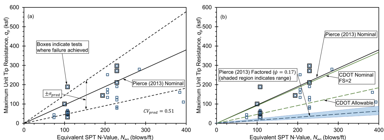
Figure 2.7 – Pierce (2013) design relation for unit tip resistance in weak rock from SPT equivalent N -values: (a) nominal resistance showing prediction uncertainty and (b) nominal and factored unit resistance for MoDOT design method and allowable and nominal unit resistance from CDOT design method.
