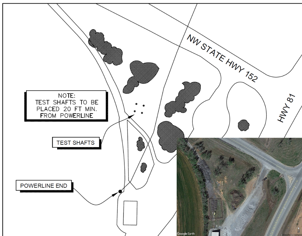
Figure 4.8 – Site plan for Minco site showing locations of the four test shafts.
