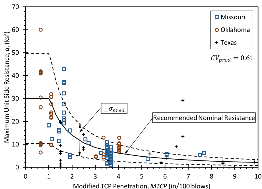
Figure 6.1 – Ultimate unit side resistance from collected load tests in weak rock with recommended relation for design from TCPT measurements.
