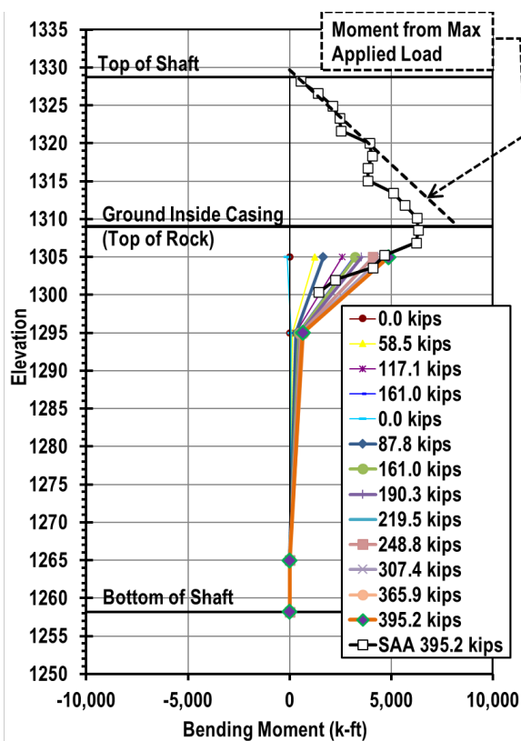
Figure 7.25 – Bending moment profile for Minco T1.
