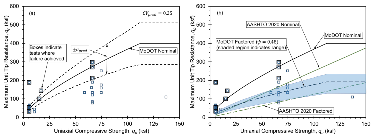
Figure 2.2 – MoDOT design relation for unit tip resistance in weak rock from compressive strength of rock core: (a) nominal resistance showing prediction uncertainty and (b) nominal and factored unit resistance for MoDOT and AASHTO (2020) design methods.
