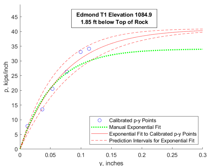
Figure 8.9 – Fitted p - y curve for Edmond T1, approximately 2 ft below the top of rock.
