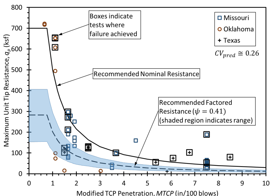
Figure 6.8 – Recommended nominal and factored unit tip resistance for recommended TCPT-based design relation.
