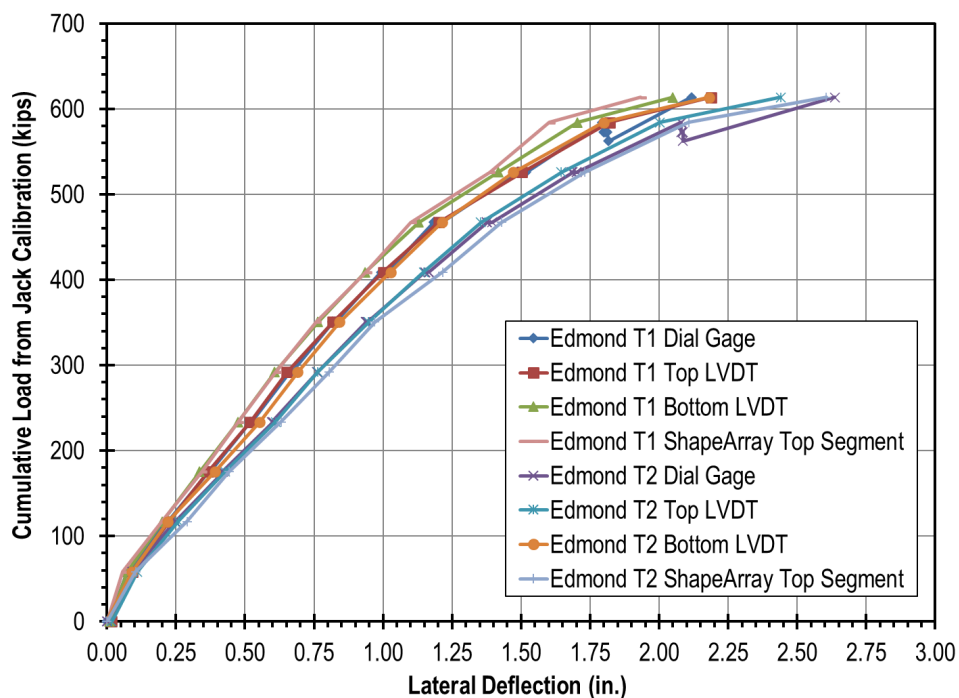
Figure 7.17 – Load-displacement curves for retest of Edmond shafts T1 and T2.
