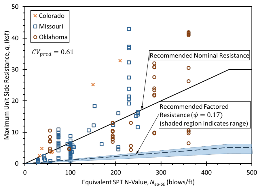
Figure 6.18 – Recommended nominal and factored unit side resistance for recommended SPT-based design relation.
