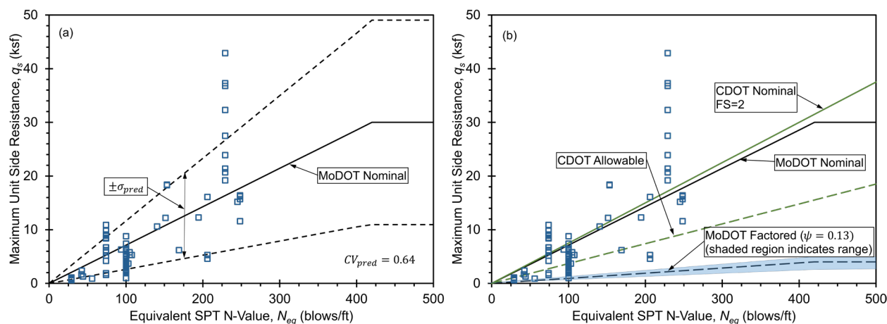
Figure 2.5 – MoDOT design relation for unit side resistance in weak rock from SPT equivalent N -values: (a) nominal resistance showing prediction uncertainty and (b) nominal and factored unit resistance for MoDOT design method and allowable and nominal unit resistance from CDOT design method.
