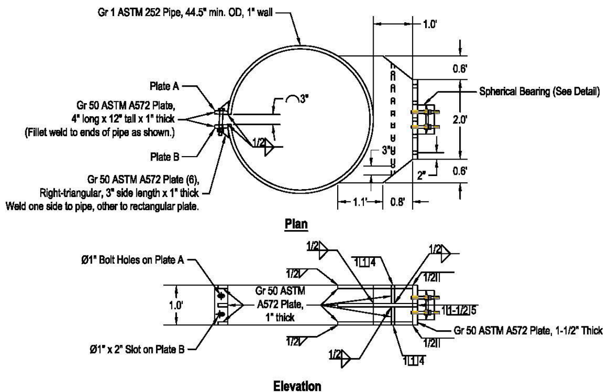
Figure 7.5 – Plan and elevation view of lateral load test frame seating detail.
