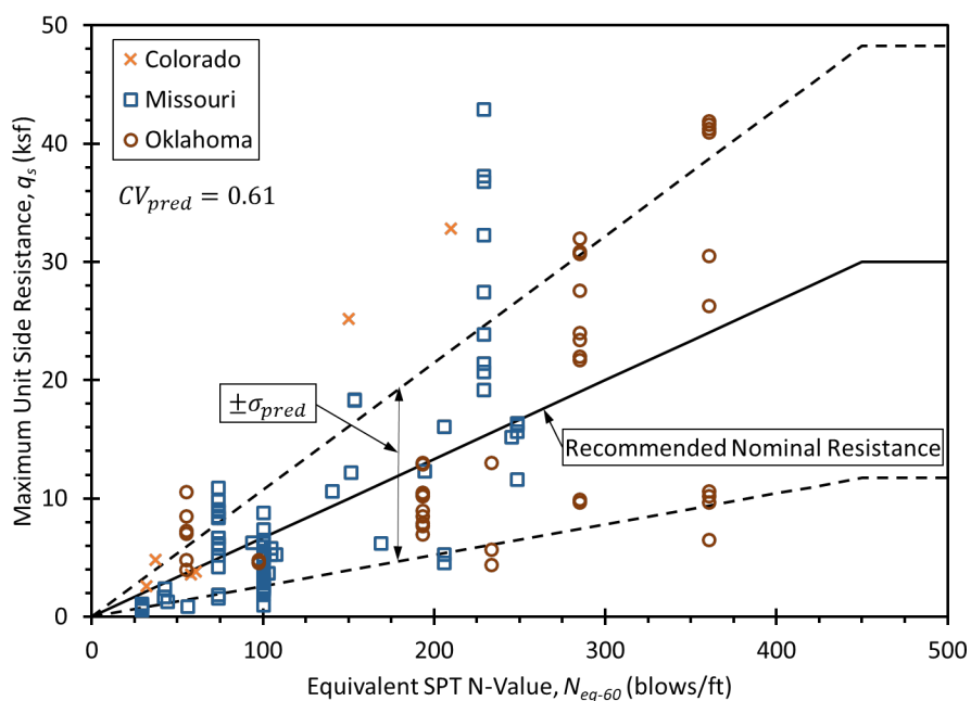
Figure 6.5 – Ultimate unit side resistance from collected load tests in weak rock with recommended relation for design from N_{eq-60} .
