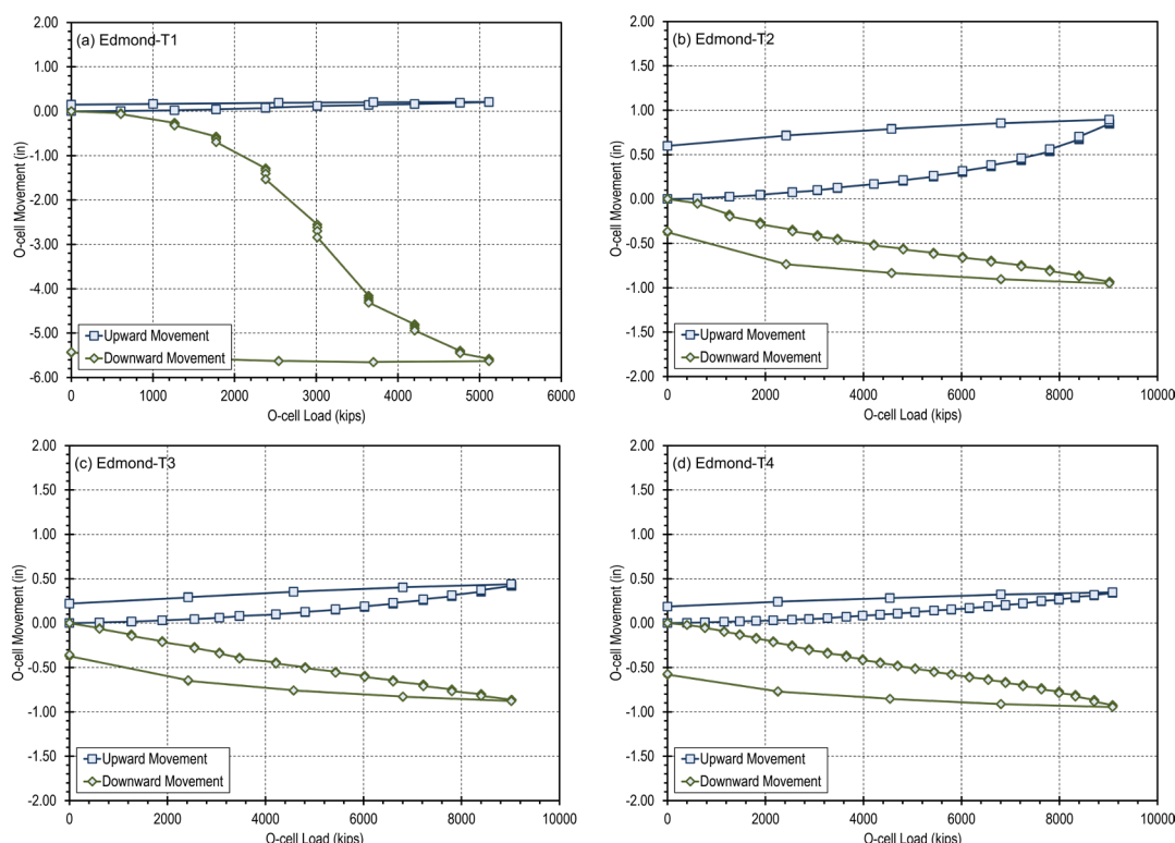
Figure 5.1 – Measured axial load-displacement response for Edmond test shafts: (a) Edmond-T1, (b) Edmond-T2, (c) Edmond-T3, and (d) Edmond-T4.
