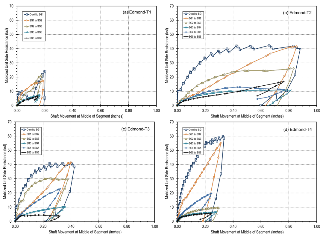
Figure 5.3 – Interpreted t - z response for Edmond test shafts: (a) Edmond-T1, (b) Edmond-T2, (c) Edmond-T3, and (d) Edmond-T4.
