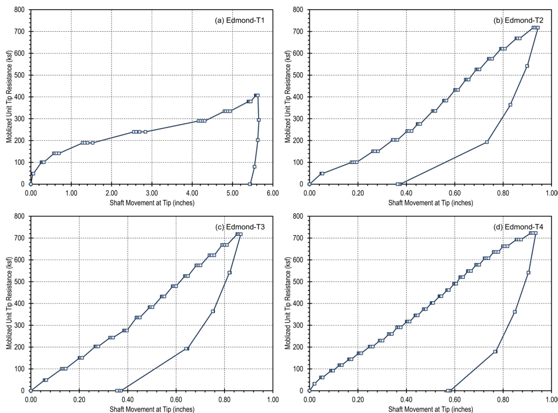
Figure 5.4 – Interpreted q - z for Edmond test shafts: (a) Edmond-T1, (b) Edmond-T2, (c) Edmond-T3, and (d) Edmond-T4.
