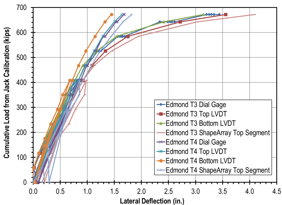
Figure 7.18 – Load-displacement curves for retest of Edmond shafts T3 and T4.
