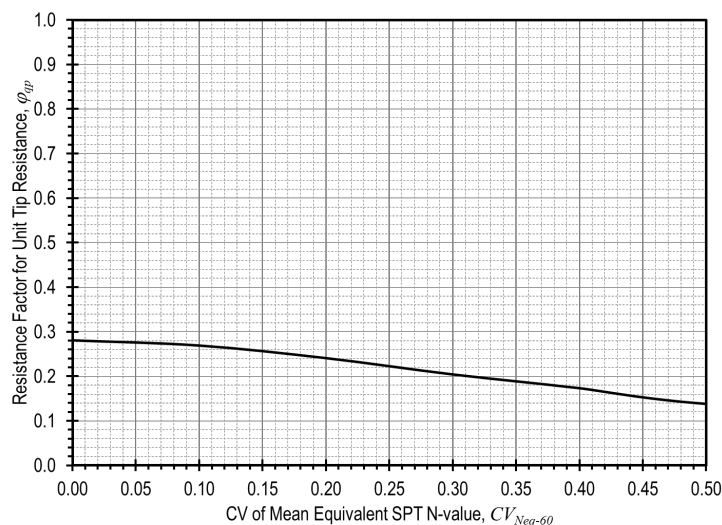
Figure 6.15 – Resistance factors for unit tip resistance from SPT N_{eq-60} .
