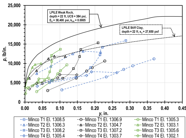
Figure 8.8 – Calibrated p - y curves for Minco.
