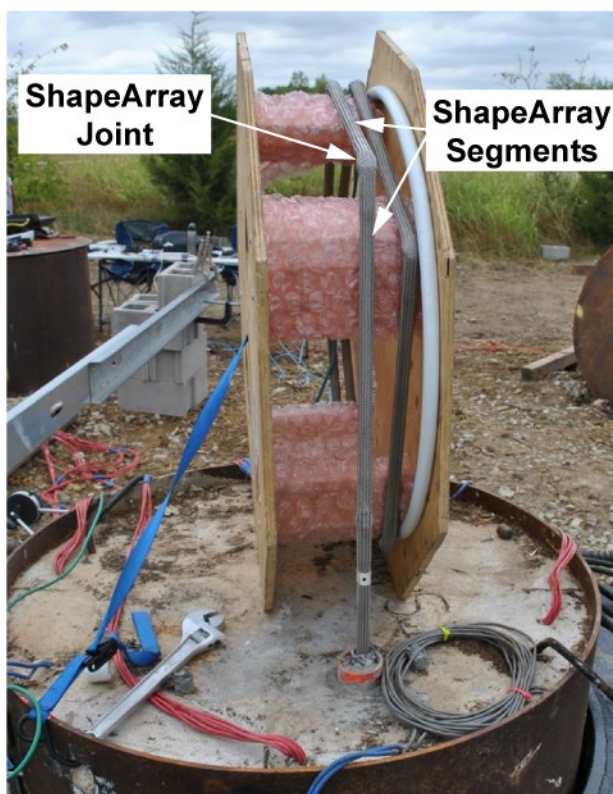
Figure 7.10 – ShapeArray segment and joint.
