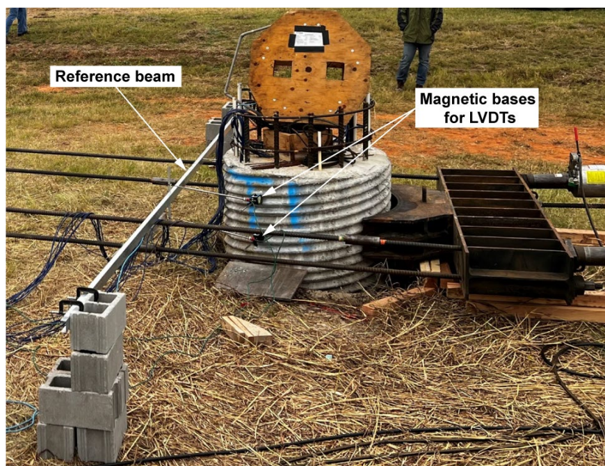
Figure 7.8 – LVDTs mounted to shaft and connected to reference beams.
