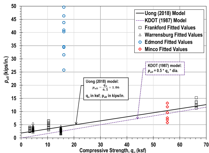
Figure 8.11 – Proposed relationship between p_{ult} and compressive strength.
