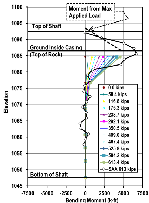
Figure 7.24 – Bending moment profile for Edmond T2.
