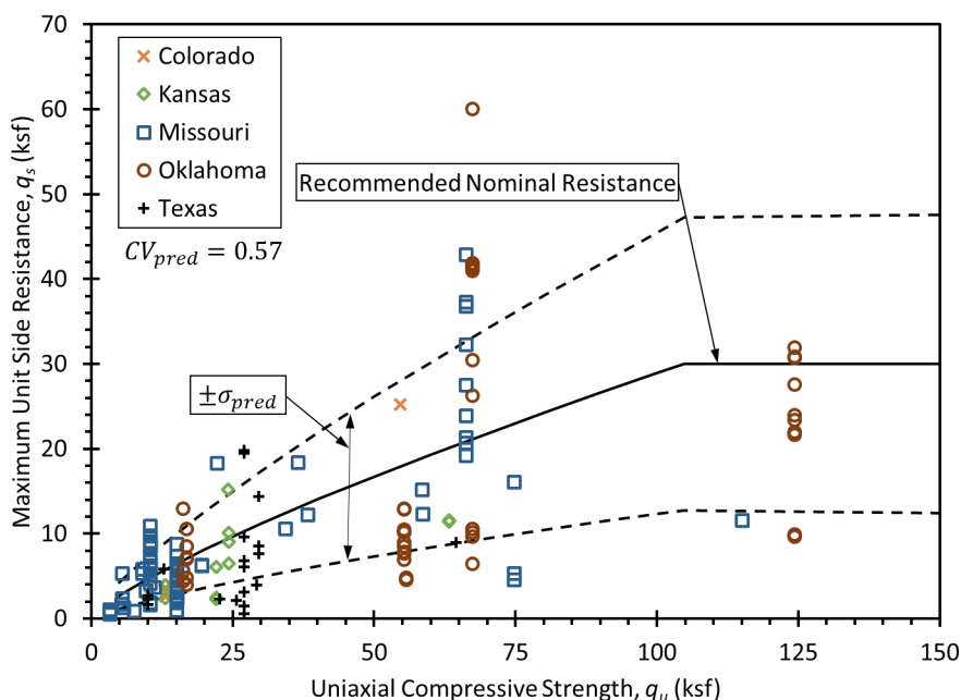
Figure 6.3 – Ultimate unit side resistance from collected load tests in weak rock with recommended relation for design from compressive strength measurements.
