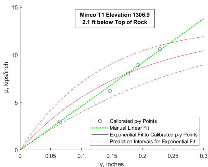
Figure 8.10 – Fitted p - y curve for Minco T1, approximately 2 ft below the top of rock.
