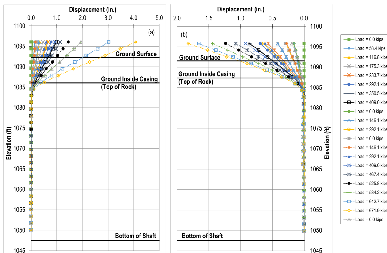
Figure 7.21 – ShapeArray displacement profiles for retest of Edmond shafts (a) T3 and (b) T4.
