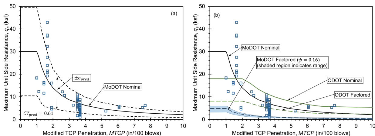
Figure 2.3 – MoDOT design relation for unit side resistance in weak rock from MTCP penetration values: (a) nominal resistance showing prediction uncertainty and (b) nominal and factored unit resistance for MoDOT and current ODOT design methods.
