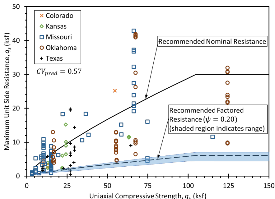
Figure 6.14 – Recommended nominal and factored unit side resistance for recommended compressive strength-based design relation.
