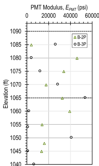
Figure 3.4 – Measurements of Pressuremeter Modulus for the Edmond test site.
