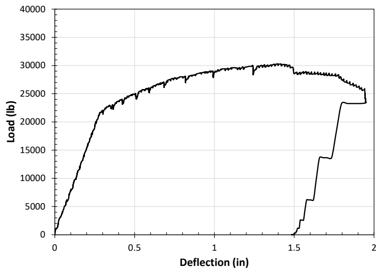
Figure 116. Load-deflection relationship for J3 slab joint 2
