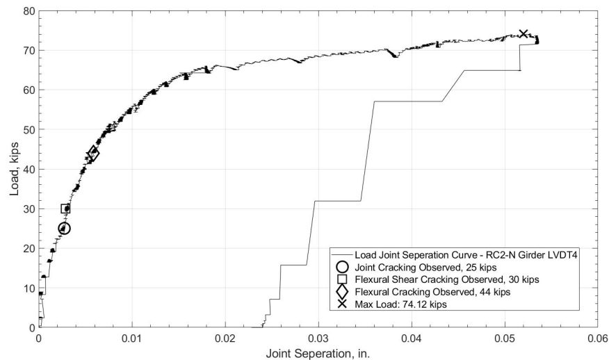
Figure 247. Load-joint separation curve at the RC2-N girder deck to joint interface west face
