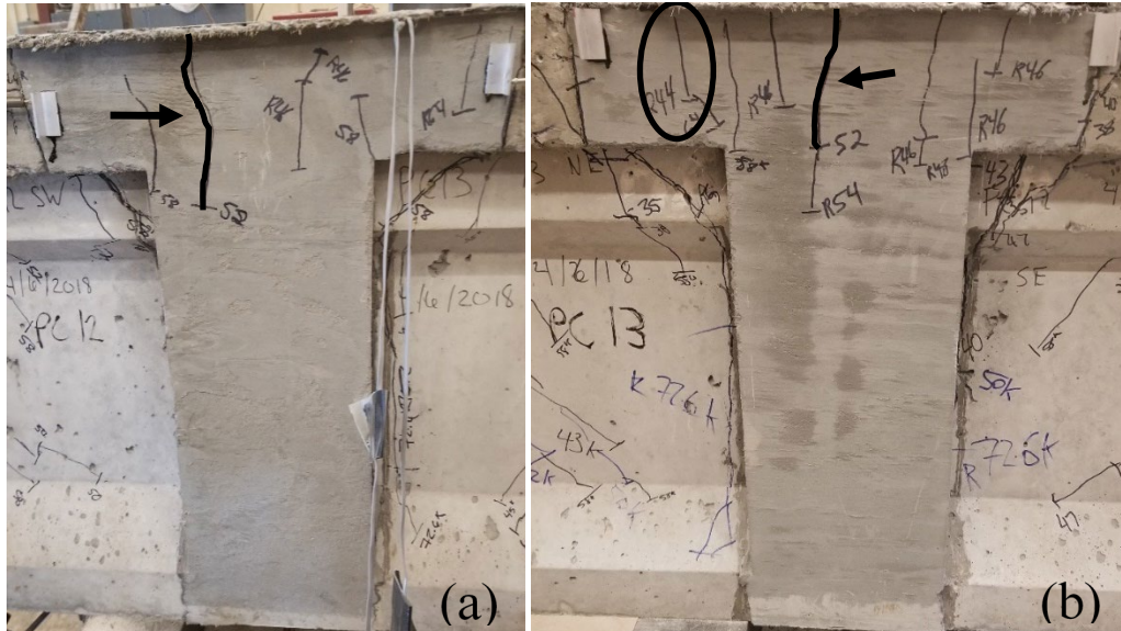
Figure 198. Initial continuity joint flexural cracking on the west face (a) and east face (b) at 52 kips of load. Arrows point to the dark lines that indicate the initial flexural cracks, and the dark oval shows the initial flexural cracks from the reload test. Other reloading cracks are indicated by an R before the load value.
