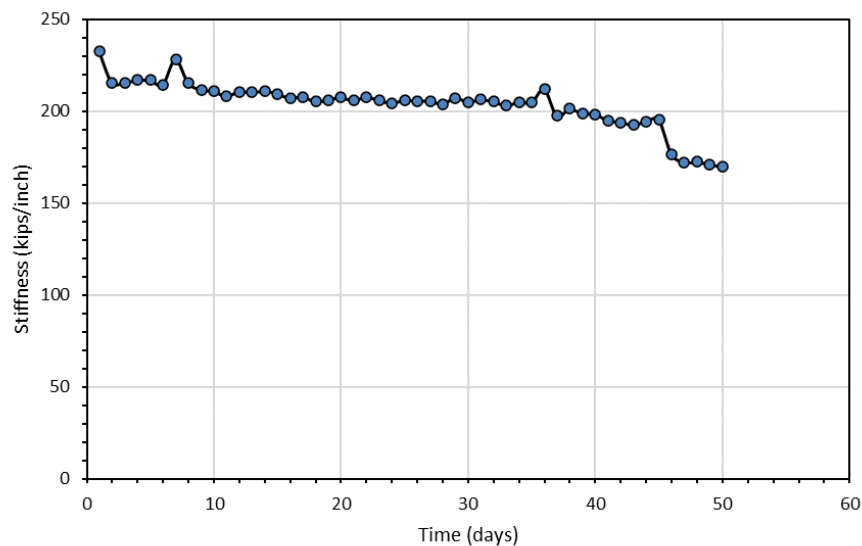
Figure 166. J3 slab 3 stiffness over 50-day loading period
