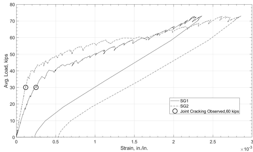
Figure 265. Load-strain curve for the RC3 joint
