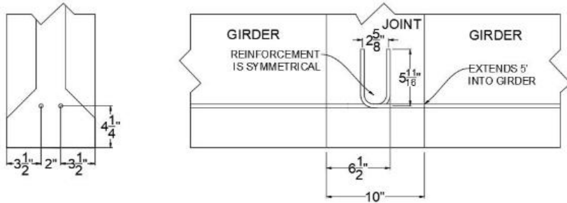
Figure 178. Newly constructed continuity joint mild steel detail for positive moment
