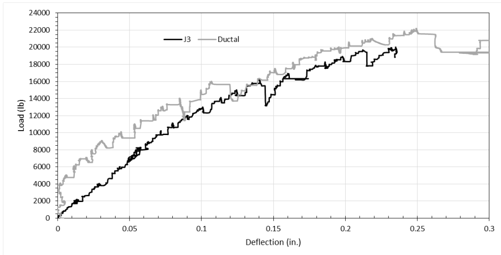
Figure 156. Load vs. deflection curves for J3 and Ductal® slab 2, part 1
