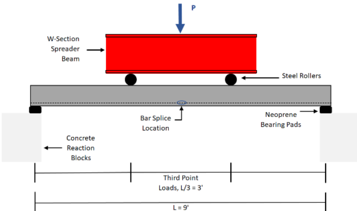
Figure 73. Third point bending test setup for UHPC splice beams
