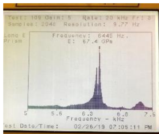
Figure 274. Typical Emodumeter transverse frequency output
