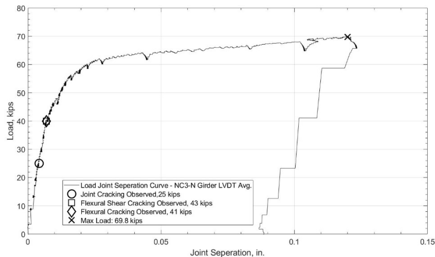
Figure 228. Load-joint separation curve at the NC3-N girder deck to UHPC joint interface.
