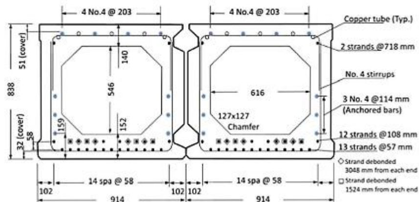
Figure 32. Cross-sectional view of box girders used for FHWA beam splice test (Maya and Graybeal 2017).
