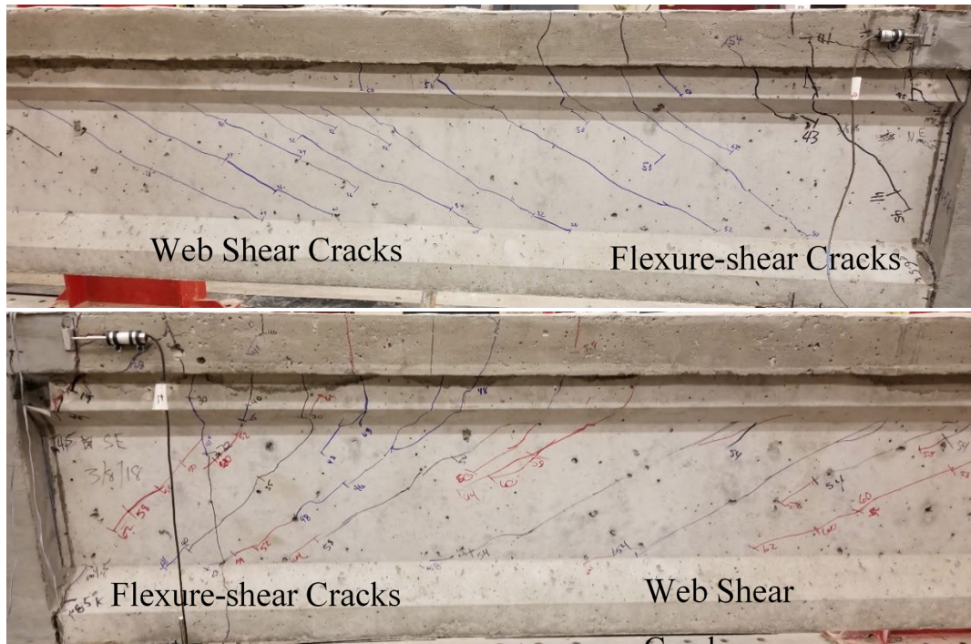
Figure 223. NC3-N girder with flexure-shear and shear cracks top and NC3-S girder with flexure-shear and shear cracks (bottom).
