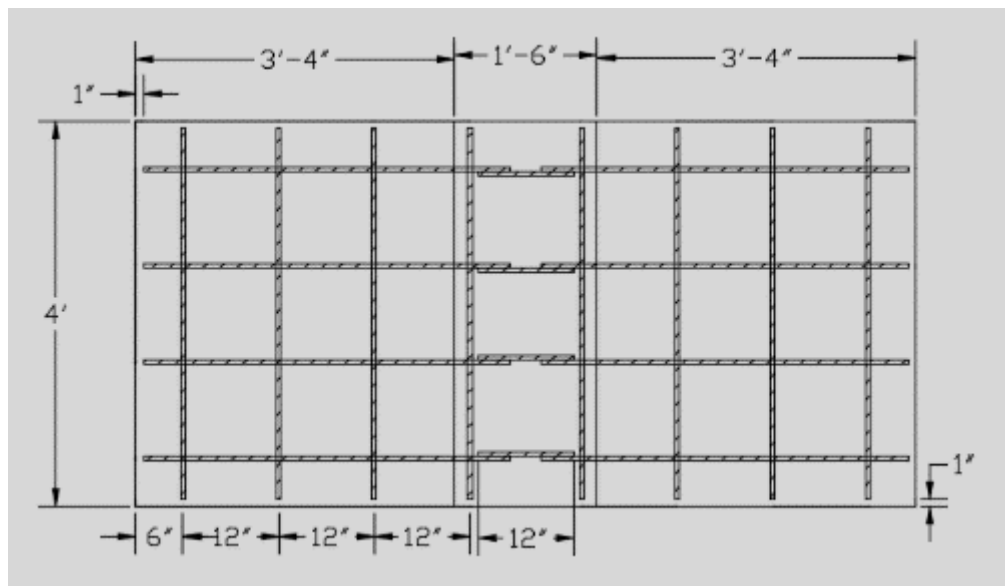
Figure 90. Plan view of reinforcement of slab specimens
