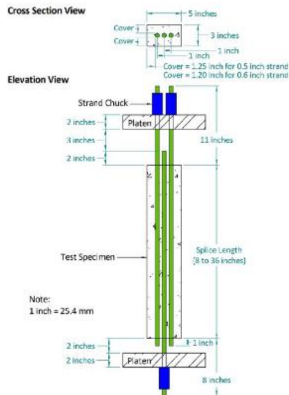
Figure 27. Geometry of FHWA prestressing strand-UHPC bond test specimen with 0.5 in. diameter strands (Graybeal 2014)
