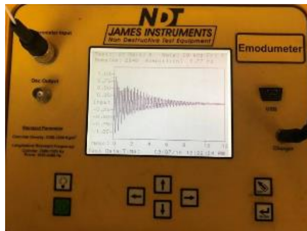
Figure 273. Typical Emodumeter transverse frequency measurement
