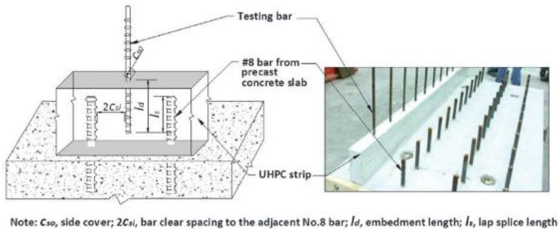
Figure 25. Overall configuration of FHWA reinforcing bar bond test specimens (Yuan and Graybeal 2014)
