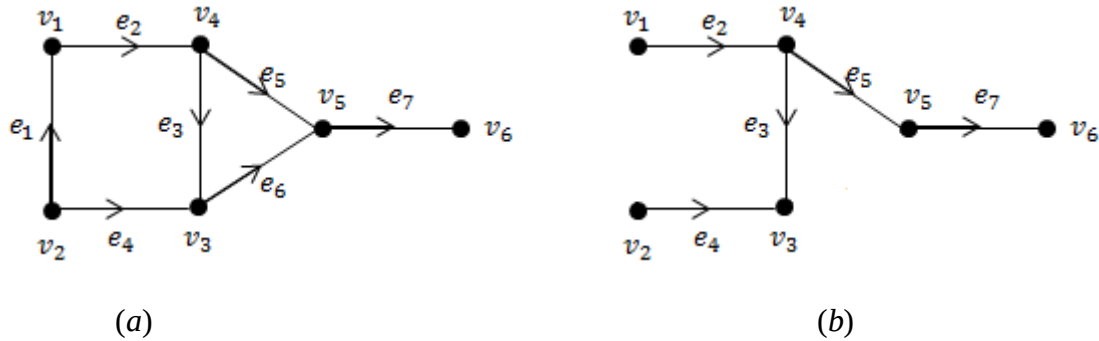
Figure 3.3: (a) A directed Graph N . (b) Spanning tree T of N .
