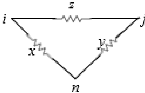
Figure 2.11: Three-node network.
