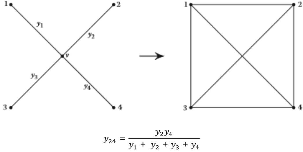
Figure 4.1: Star-delta transformation.
