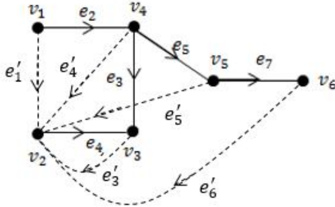
Figure 3.8: Graph containing spanning tree T and star tree (dotted) given in Figure 3.3.
