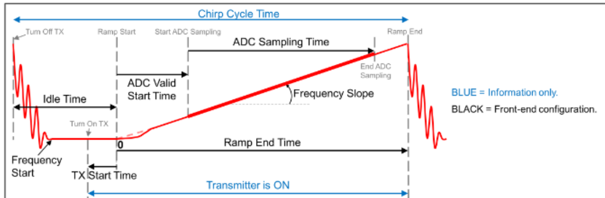
Figure C.1: Chirp illustration from Texas Instrument's user guide showing each chirp parameter. Source: TI mmwaveSDKUserGuide.
