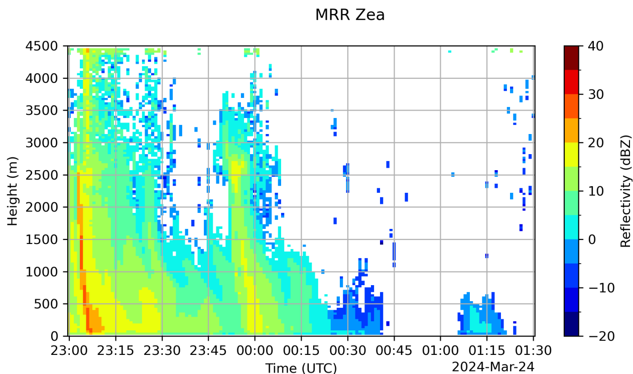
Figure 7.17: Height-time map for precipitation reflectivity from the colocated MRRs.
