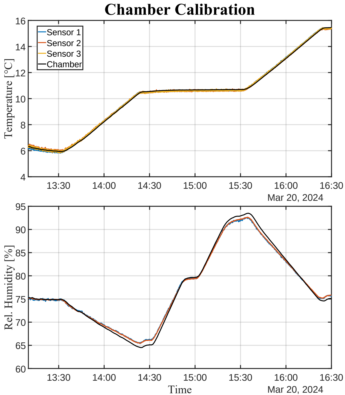
Figure A.1: Time series for the temperature and relative humidity experiment at the Oklahoma Mesonet's Calibration Laboratory. The black series represents the chamber reference values, and the colored series represents the calibrated individual sensors.
