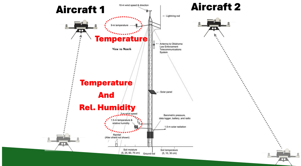
Figure 3.12: Experimental setup for the system’s performance evaluation under operational conditions. Two identical WxUAS were flown next to the reference Oklahoma Mesonet 10 m tower for colocated measurements.
