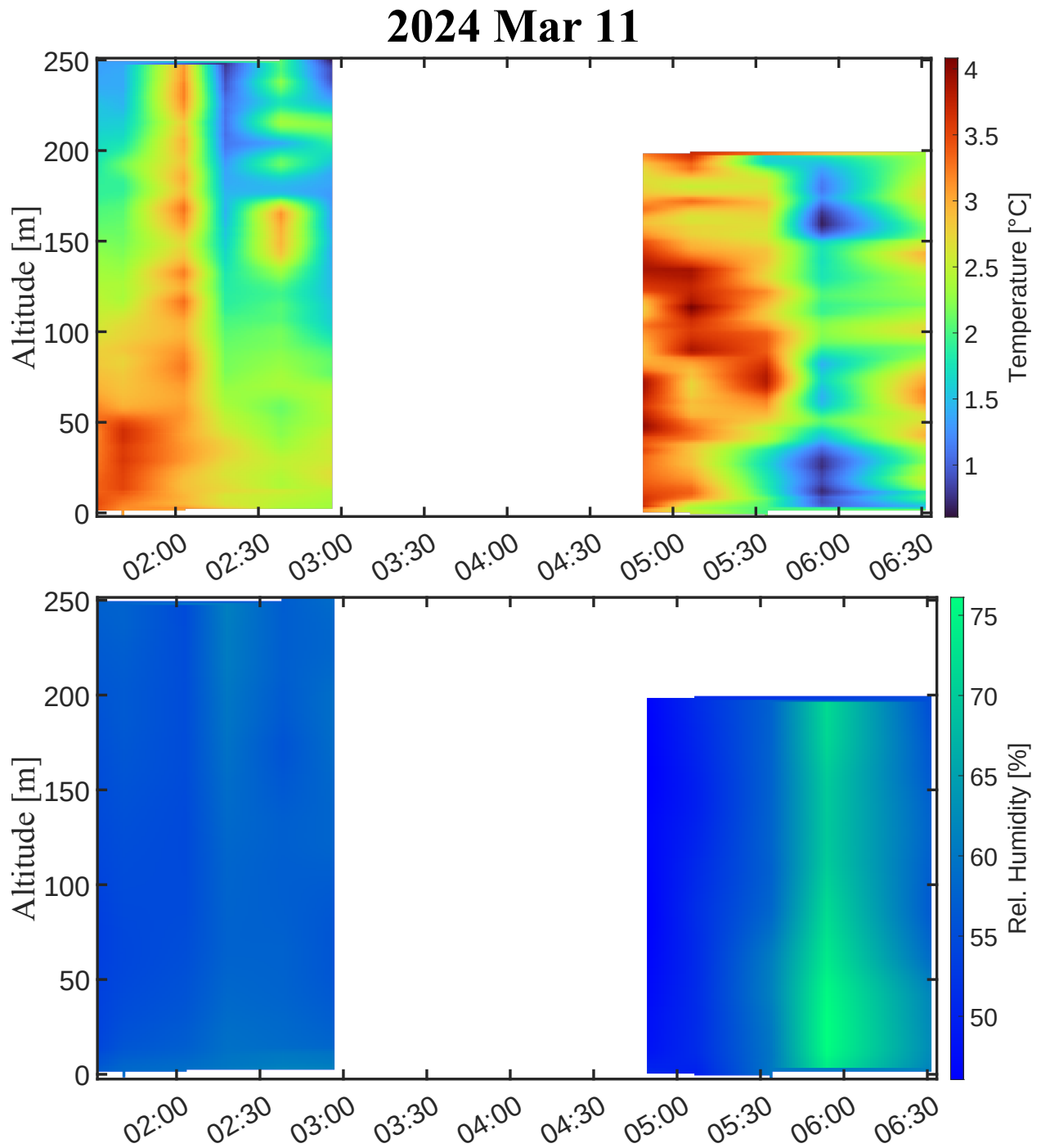
Figure 7.10: Temperature and relative humidity maps for the WxUAS profiles on March 11 th , 2024.
