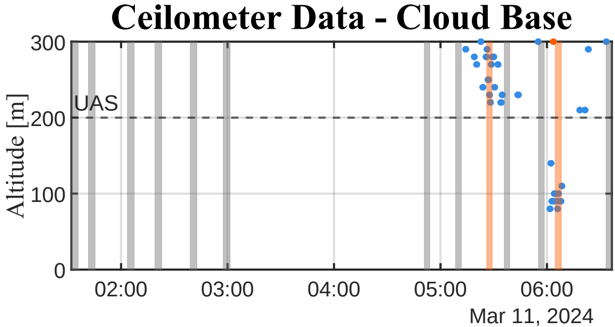
Figure 7.15: Height-time map for the Ceilometer’s cloud-based reports during the passage of the snow band on the backside of the low-pressure system.
