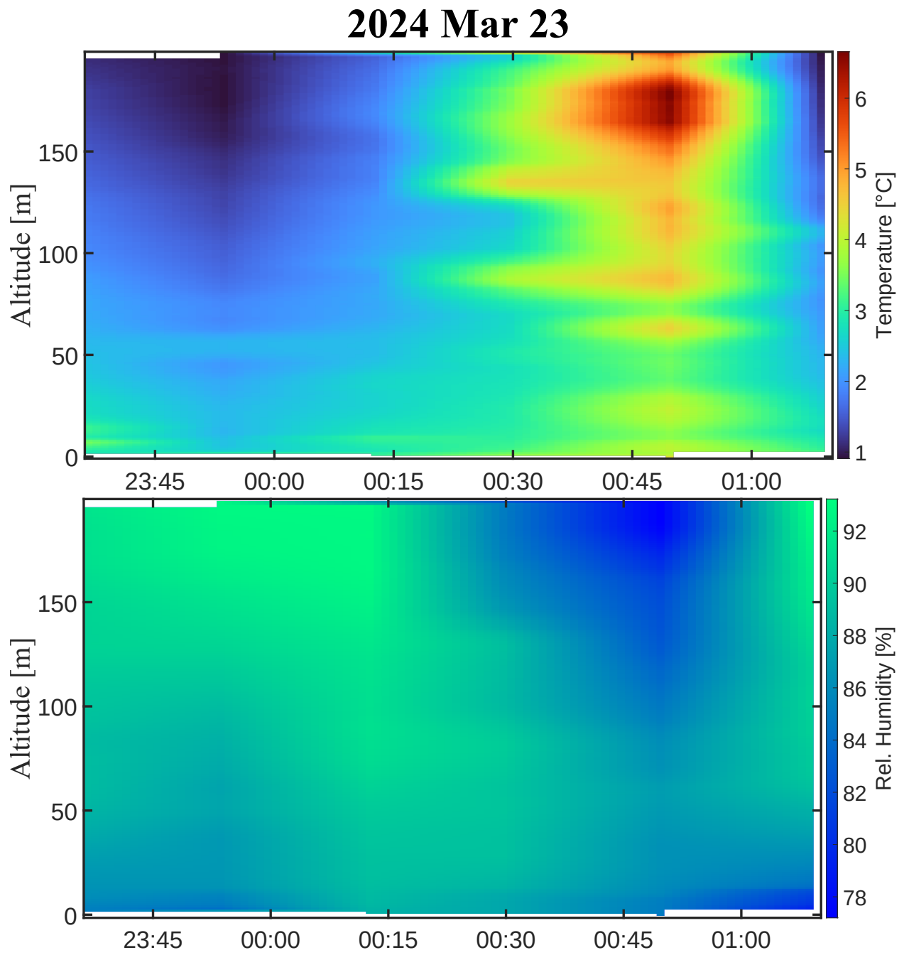
Figure 7.18: Temperature and relative humidity spatiotemporal maps for the WxUAS profiles on March 23 rd , 2024.
