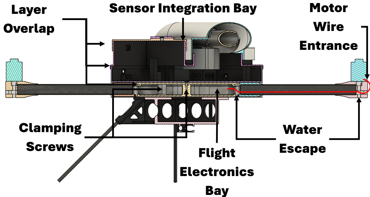
Figure 5.5: Diagonal cross-section view of the aircraft’s 3-dimensional computer-aided design illustrating the seal-less water resistance design techniques.
