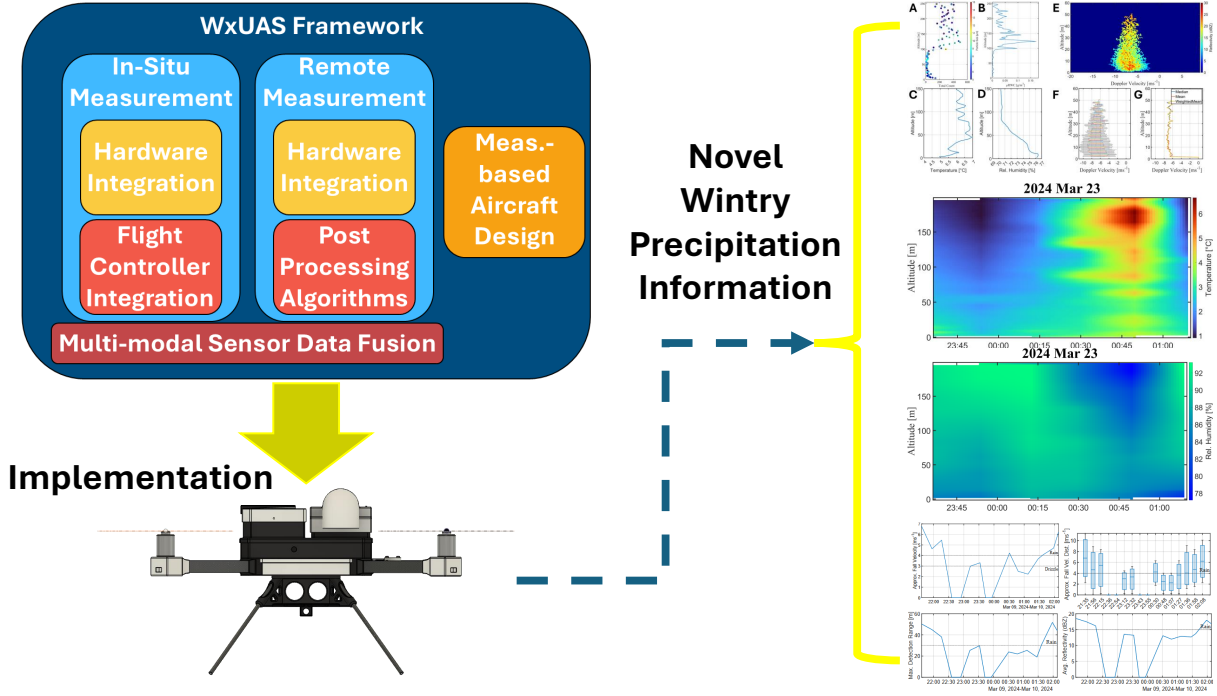
Figure 8.2: Diagram illustrating the framework, its modules, and how its implementation leads to novel atmospheric information.
