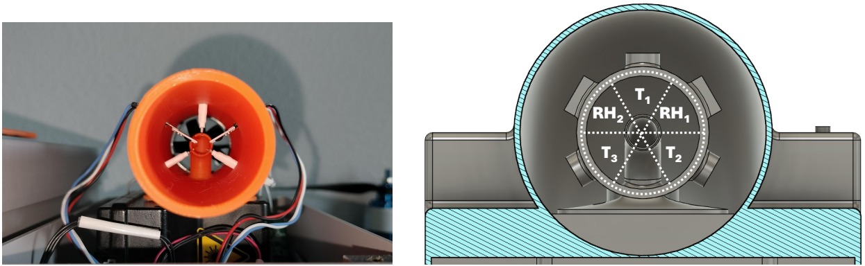
Figure 3.5: Concentric sensor ring with redundancy for increased accuracy. The right panel illustrates 60^{\circ} segmentation strategy, and the left panel illustrates its implementation.
