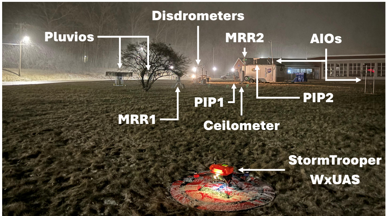
Figure 7.2: MAI 2 S instruments.
