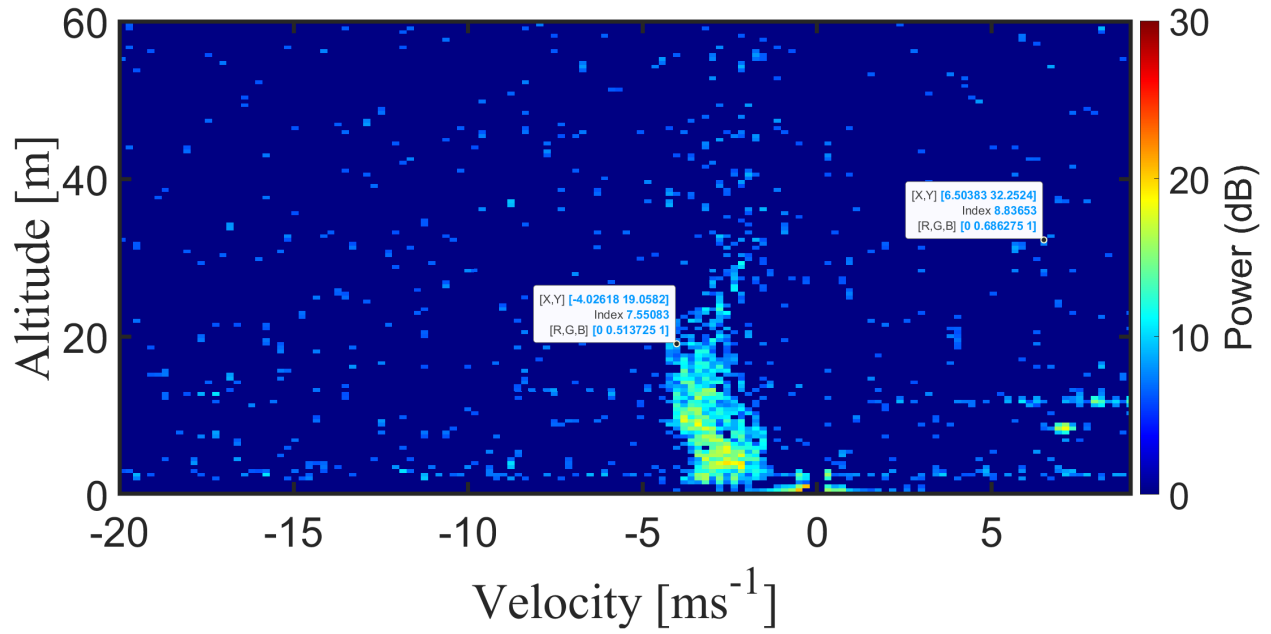
Figure 4.11: Range-Doppler map for the same drizzle event presented in Fig. 4.10 after the use of the motion correction, partial SLE, and a 5 dB threshold.
