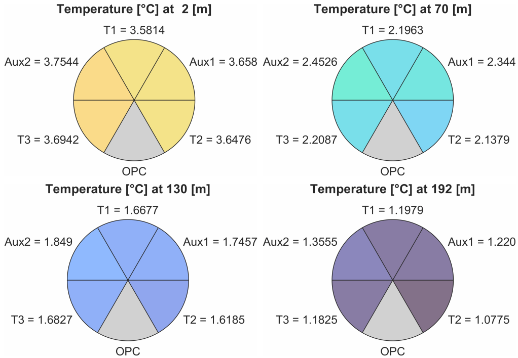
Figure 3.6: Example of enhanced neighboring sensor analysis showing temperature values for sensors across four stages of a profile to 200 m above ground level.
