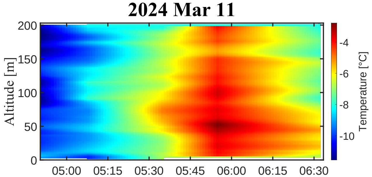
Figure 7.13: Wet bulb Temperature spatiotemporal map from the WxUAS profiles for March 11 th , 2024.
