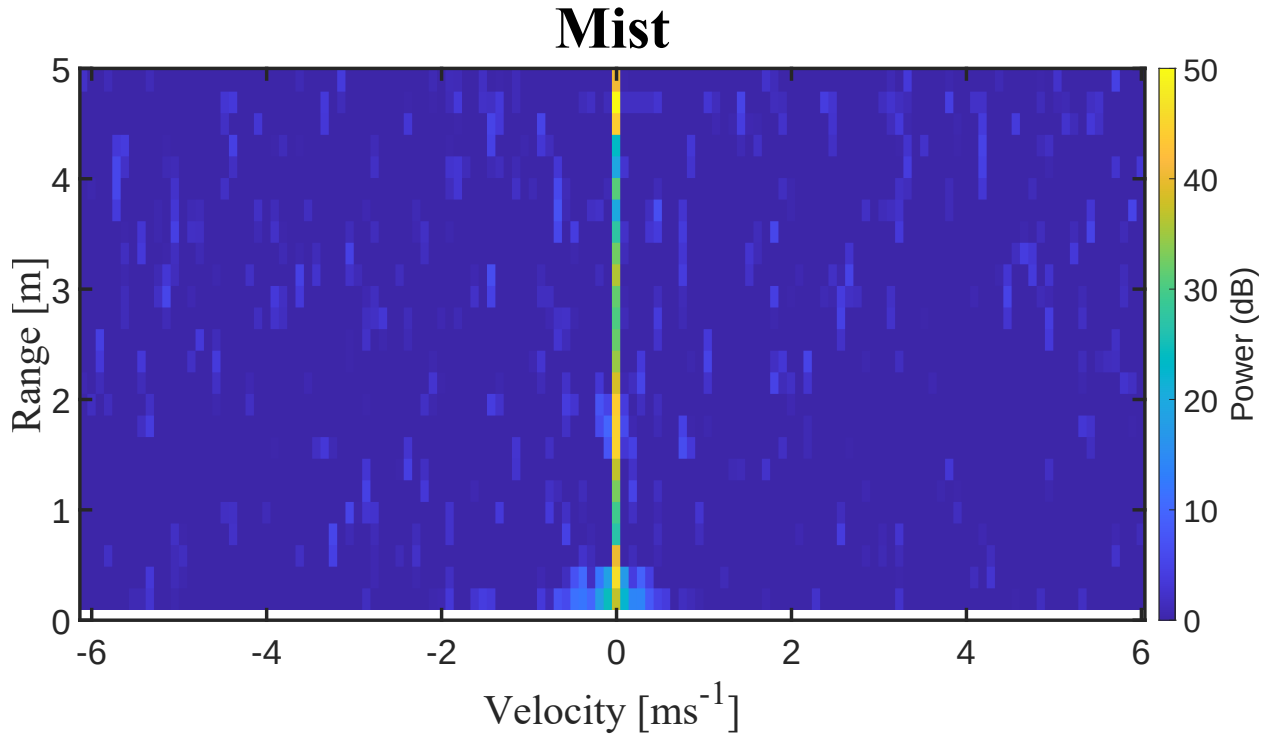
Figure 4.3: range-Doppler map for the mist generated by the handheld spray floating in front of the radar (i.e., perpendicular setup).
