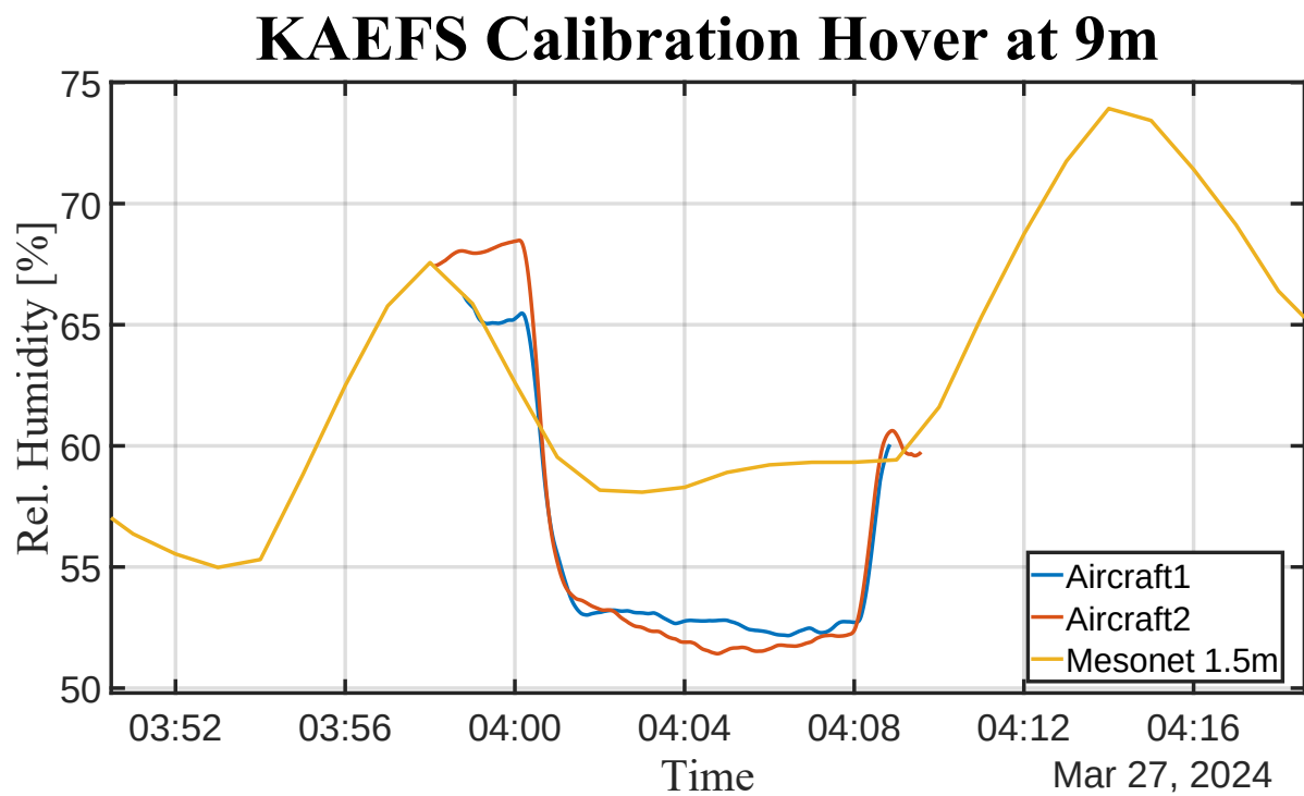
Figure B.3: Relative humidity time series for the tower data (1.5 m) with both aircraft data, including data before and after take-off.
