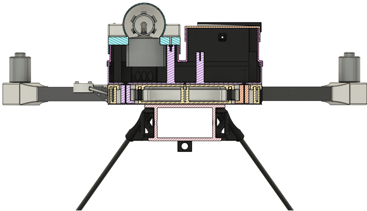
Figure E.2: 3-dimensional computer-aided design for this dissertation's WxUAS aircraft designs in a vertical cross-section cut of the orthographic back view illustrating the internal components and the overlapping layer technique for seal-less water-resistance.
