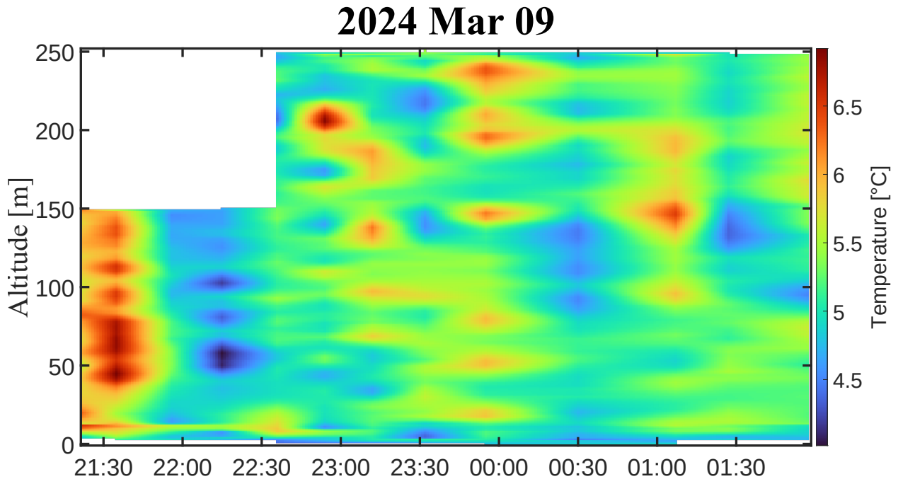
Figure 7.3: Spatiotemporal temperature map for the WxUAS profiles on March 9, 2024.
