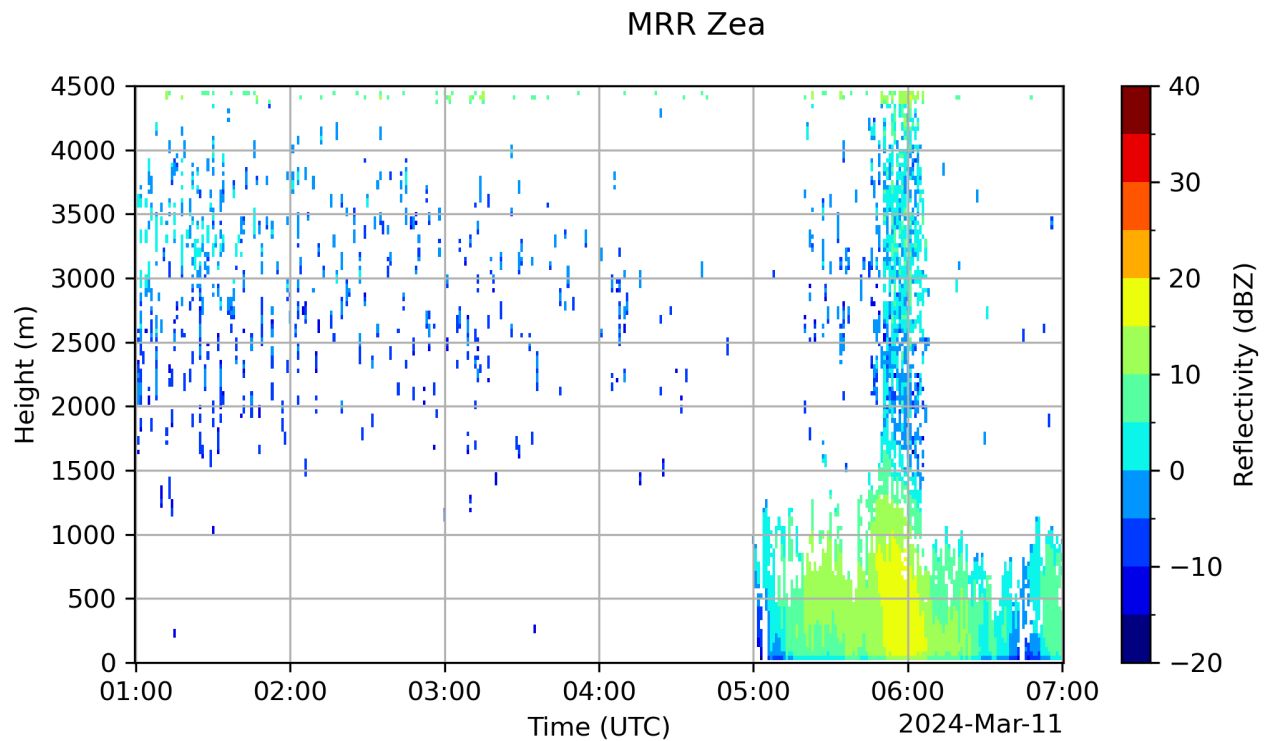
Figure 7.14: Height-time map for precipitation reflectivity from the colocated MRRs.
