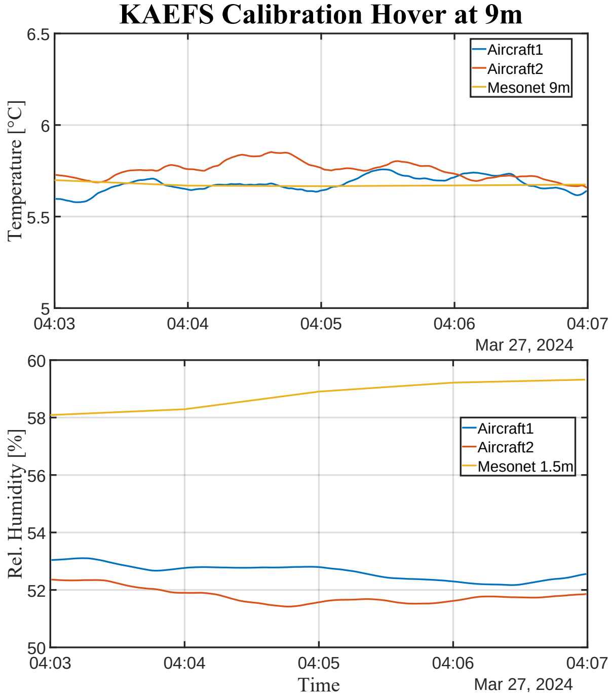
Figure B.1: Time series for the tower and two aircraft data highlighting the comparison interval. Mean and maximum absolute errors are found in Table 3.4.
