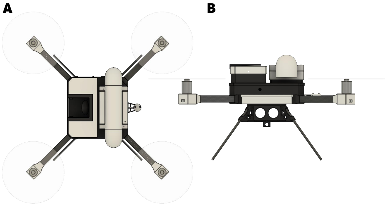
Figure E.1: 3-dimensional computer-aided design for this dissertation's WxUAS aircraft designs. (A) Orthographic top view and (B) orthographic front view.
