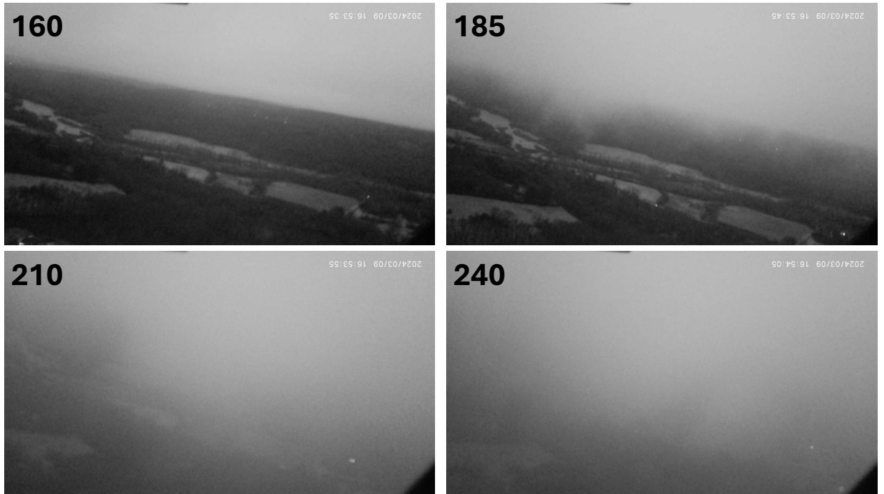
Figure 7.8: Frames from the WxUAS’s onboard camera at 160, 185, 210, and 240 m indicating the start of the cloud transition layer and base of the cloud layer during the profile at 22:55.
