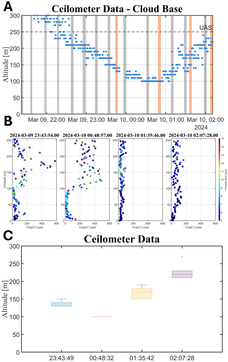
Figure 7.5: WxUAS cloud-sized particle distribution profiles compared to the colocated ceilometer. (A) ceilometer reports for the lowest cloud base. (B) WxUAS cloud-sized particle distribution profiles. (C) Box and whisker plot for the ceilometer lowest cloud base for the interval of the four WxUAS profiles.
