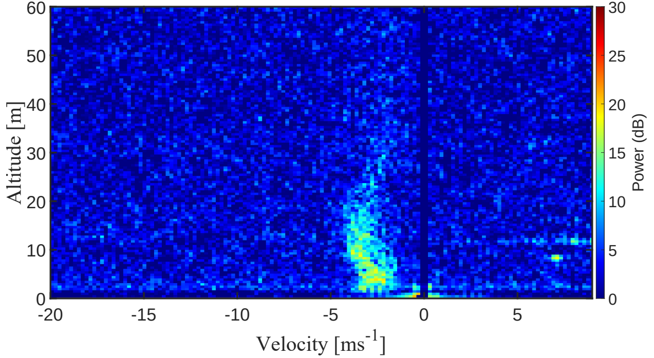
Figure 4.10: Range-Doppler map for an atmospheric profile during a drizzle event at the MAI 2 S field campaign. The data presented here includes the aircraft compensation and the SLE partial algorithms.
