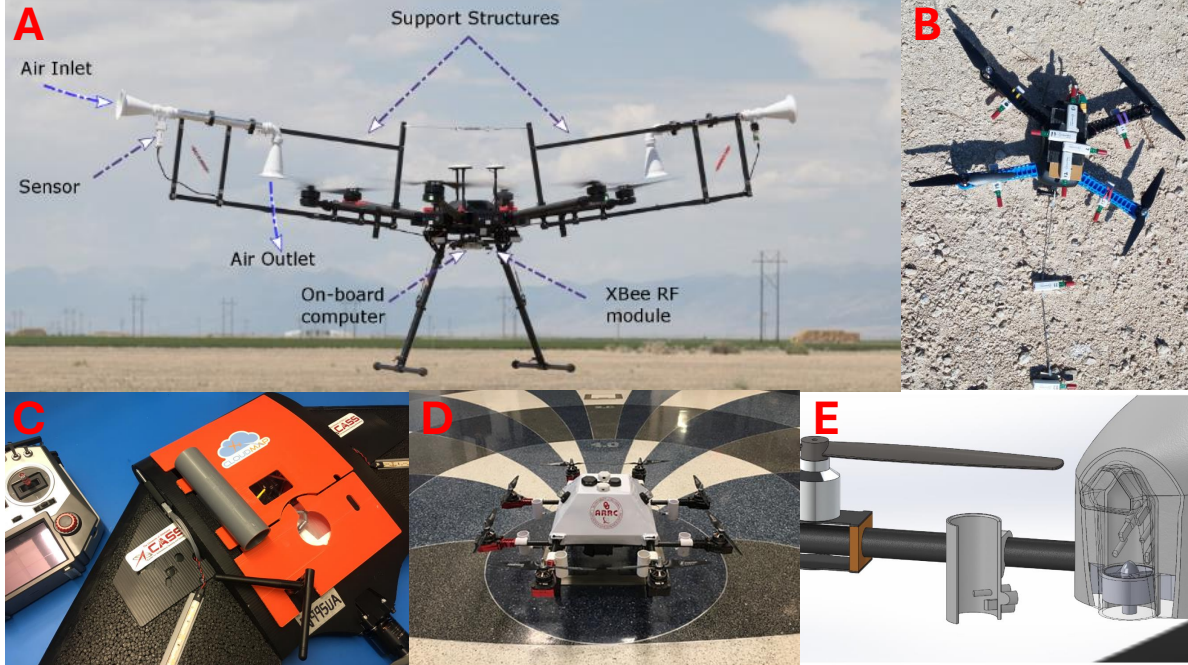
Figure 2.2: Examples of physical sensor integration into UAS: (A) Omnidirectional shielded integration with propeller-based passive aspiration [54]; (B) No shielding with partial propeller-based, passive ventilation [66]; (C) Fixed-wing two-layer shielding with passive ventilation through vehicle motion [8]; (D) Multi-direction with partial shielding and propeller-based ventilation [46]; (E) Comparison of directional shield with active aspiration with partial shielding and propeller-based ventilation [37].
