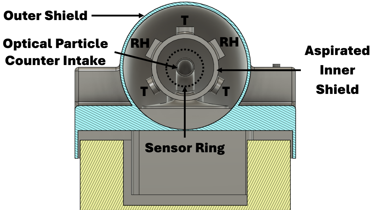
Figure 3.2: Frontal cross-section view of the two-layer custom sensor shield designed to prevent contact with freezing precipitation while allowing for direct atmospheric observation.
