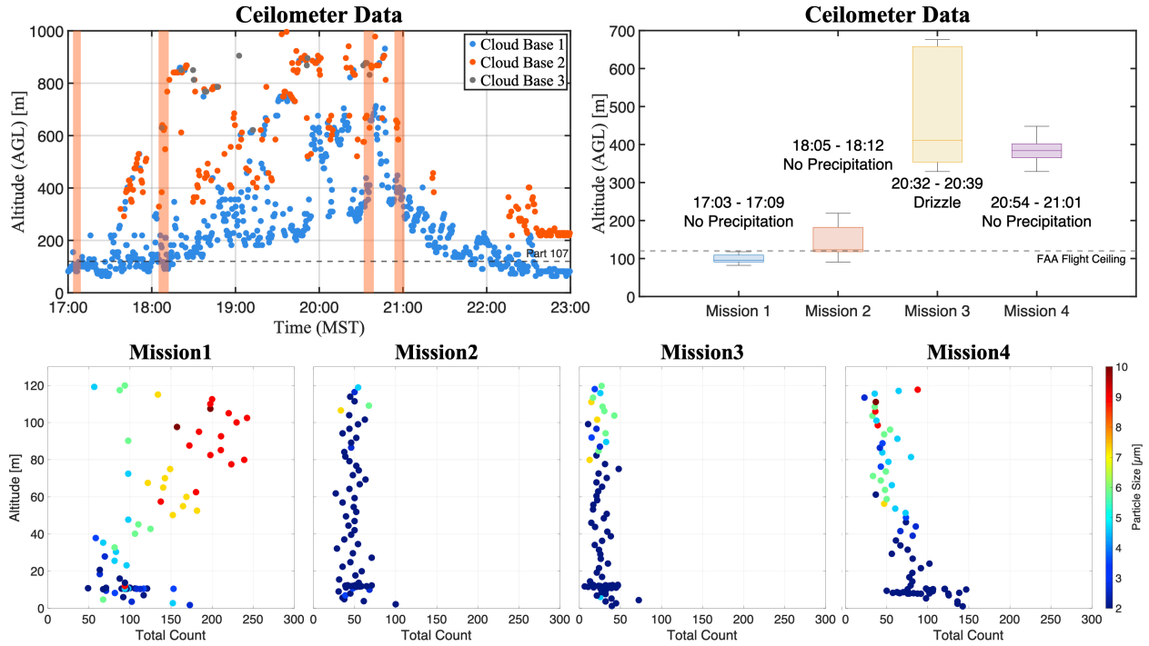
Figure 3.15: Ceilometer data (above) indicating the cloud base and the profiles of the particle size distribution (below) for each of the four flights to 120 m. The orange-shaded columns in the ceilometer’s scatter plot represent the time intervals for the four flights
