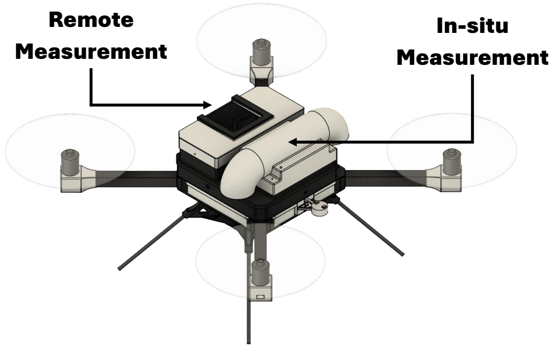
Figure 5.1: Isometric view of the 3-dimensional computer-aided design for this dissertation’s WxUAS technology demonstration platform with the remote (left) and in-situ (right) measurement solutions integrated as its topmost component.
