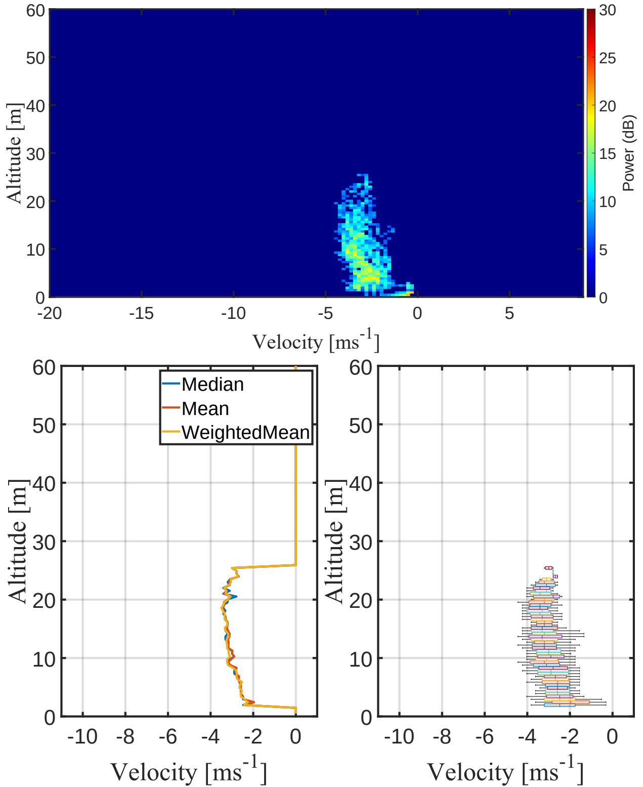
Figure 4.14: Illustration of the final range-Doppler map and velocity and distribution profiles using the motion compensation, SLE, and Context-Dependent Noise Reduction algorithms for the same drizzle event presented in Figs. 4.10 and 4.11.
