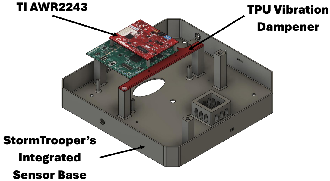
Figure 4.8: Illustration of the TPU-based suspended raft used to decouple the TI AWR2243 from motor-induced vibrations commonly found in multi-rotor UAVs.
