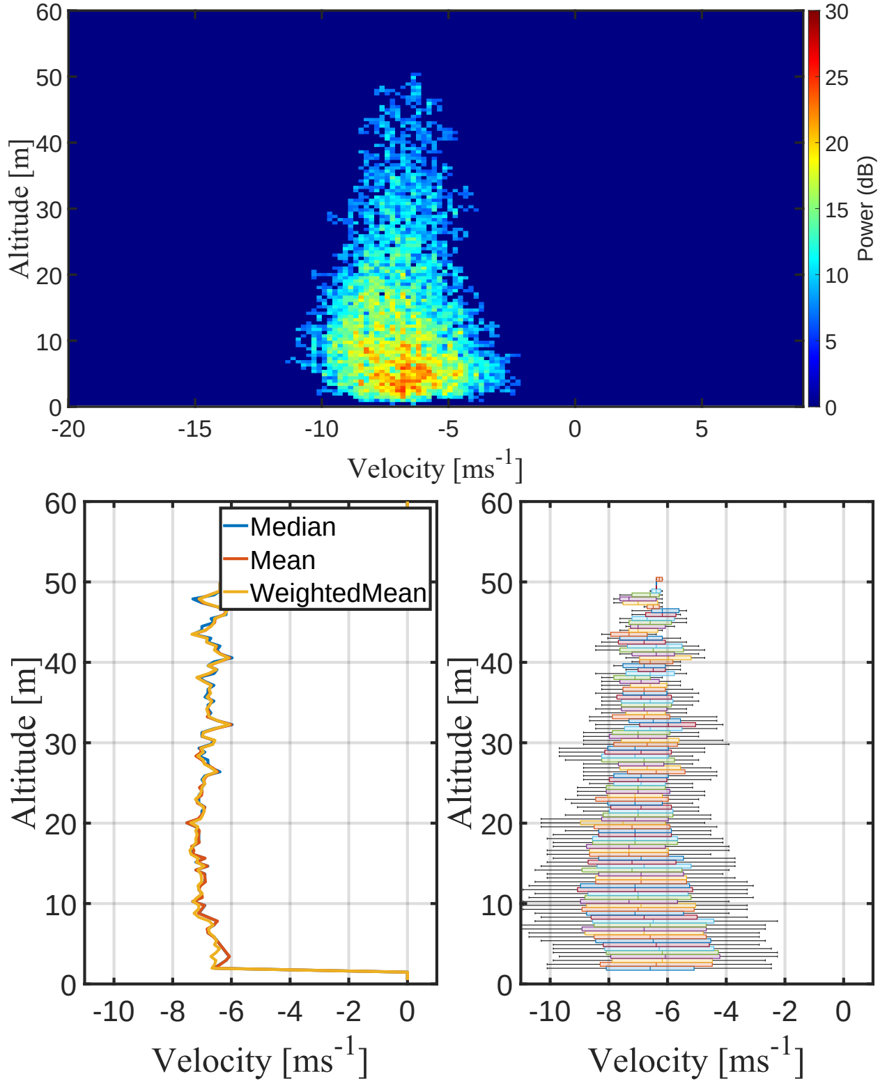
Figure 4.15: Illustration of the range-Doppler map and velocity and distribution profiles using the motion compensation, SLE, and Context-Dependent Noise Reduction algorithms for a new rain event.
