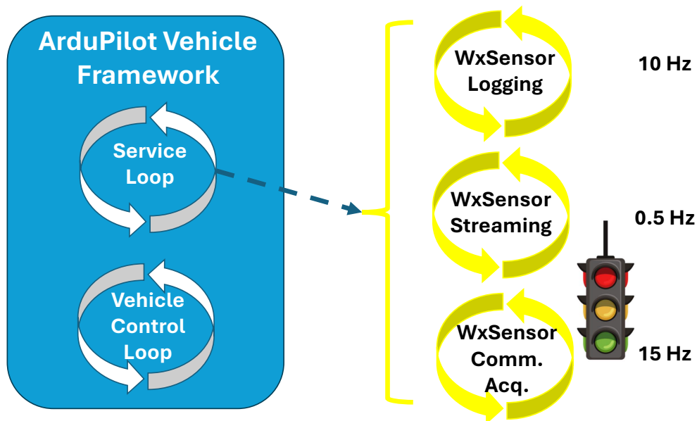
Figure 3.8: Diagram depicting the weather sensor library’s use of the framework’s service loop as a mitigation strategy for the risks associated with the direct integration method.
