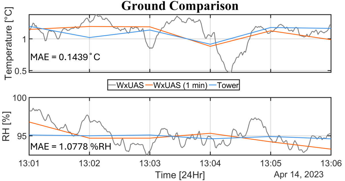
Figure 3.13: Results for the second temperature and relative humidity ground-based intercomparison experiment. The small mean absolute errors are below both manufacturers' reported accuracies.
