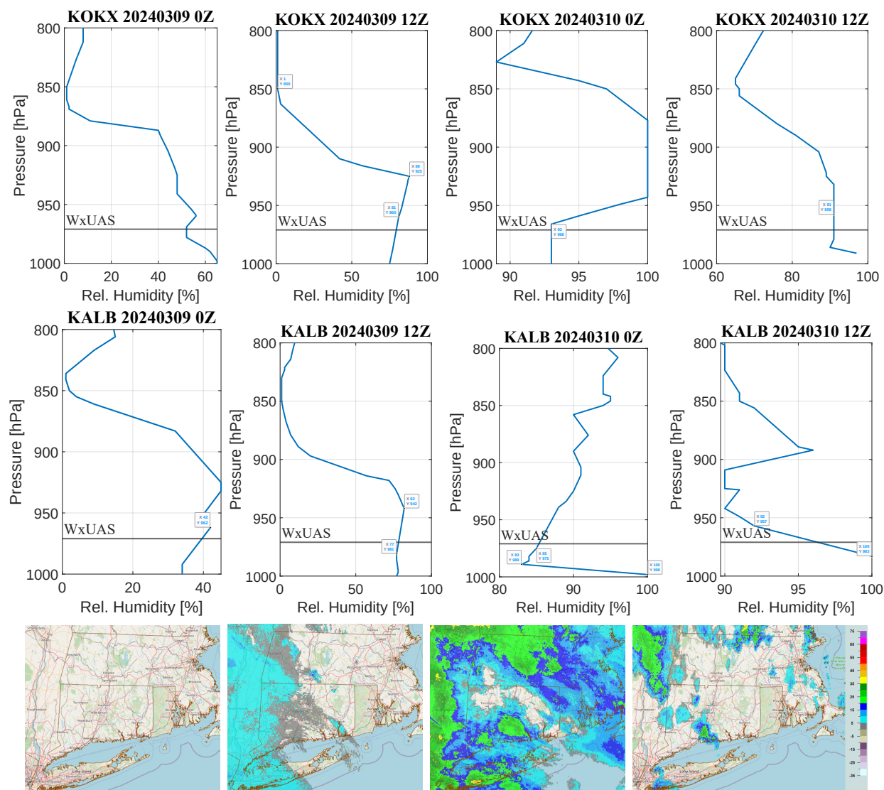
Figure 7.9: Complementary weather data from mesoscale networks. The top two rows present the relative humidity profiles from the KOKX and KALB sounding stations, and the bottom row presents the MRMS composite reflectivity at the same time steps.
