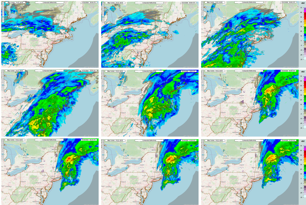
Figure F.3: MRMS composite reflectivity product for the northeastern United States from March 22 th , 18Z (top left) until the 24 th at 0130Z (bottom right). The initial two rows advance in a 6-hour step, while the final row advances in a 30-minute step to highlight the missed rain event at Storrs (CT).
