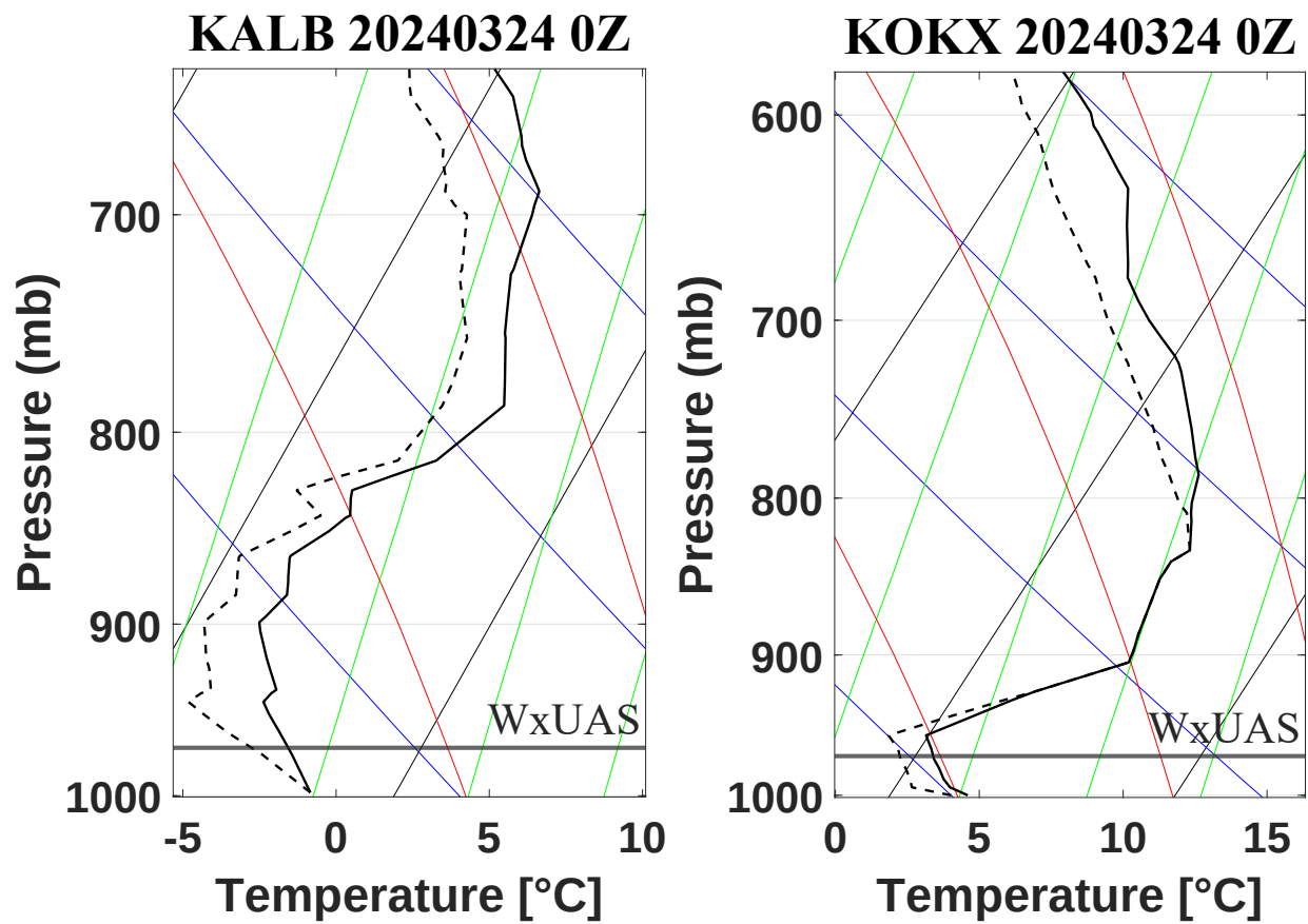
Figure F.4: Soundings from Albany (left), and Long Island (right) for March 24 th 0Z.
