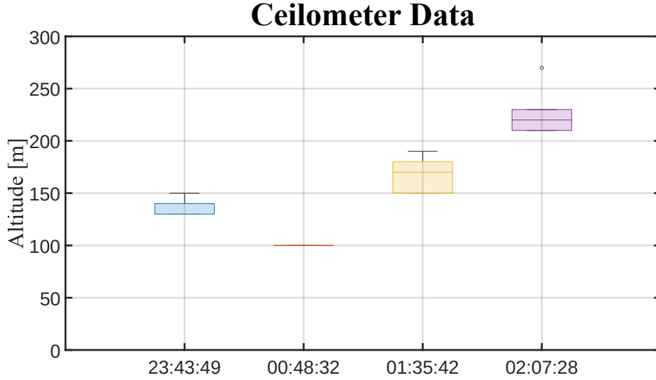
Figure 6.6: Distribution of the reported lowest cloud bases by a colocated ceilometer.
