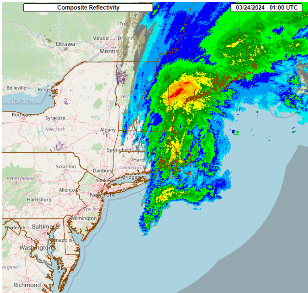
Figure 7.19: MRMS composite reflectivity for March 24 th , 2024 at 01:00.
