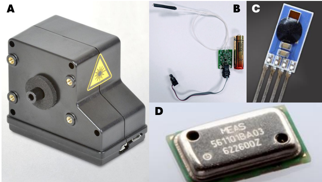
Figure 3.4: Sensors for in-situ measurements: (A) The OPC-N3 for particle size distribution, (B) the PT-100 bead thermistor and ADS1115 ADC for fast temperature; (C) the HYT 271 for slow temperature and relative humidity; and (D) the MS5611 for fast pressure measurements.
