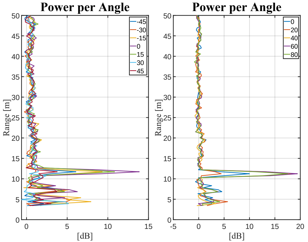
Figure D.2: Experiment results for the pitch angle compensation via beamforming in post-processing. Metal pole at broadside on the left and 60 degrees on the right.
