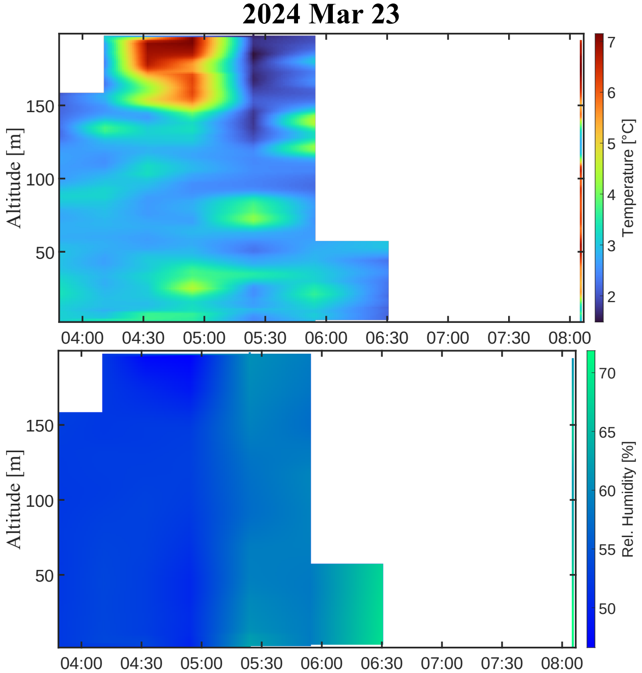
Figure 7.16: Temperature and relative humidity spatiotemporal maps for the WxUAS profiles on March 23 rd , 2024.
