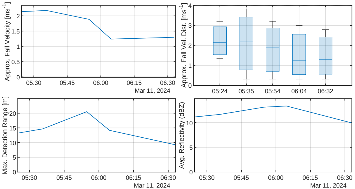
Figure 7.11: Radar-derived precipitation variables used for type and intensity classification for March 11 th , 2024.
