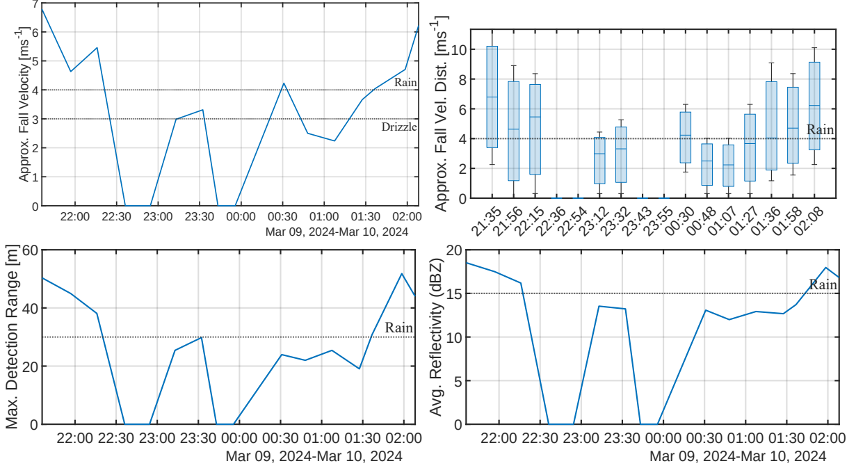
Figure 7.4: Radar-derived precipitation variables used for type and intensity classification. The dynamic classification thresholds for liquid precipitation are shown as a reference.
