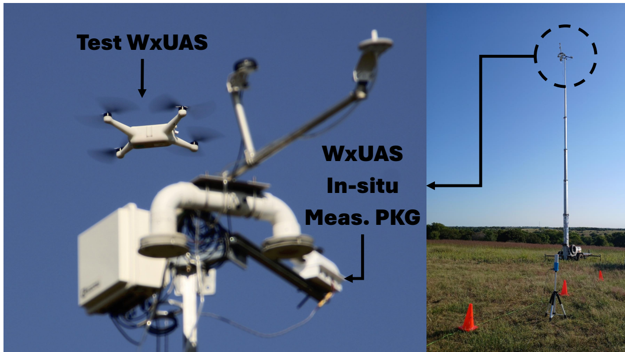
Figure 8.1: This dissertation’s in-situ measurements solution deployed as a calibration reference for 36 WxUAS from various manufacturers and research groups.
