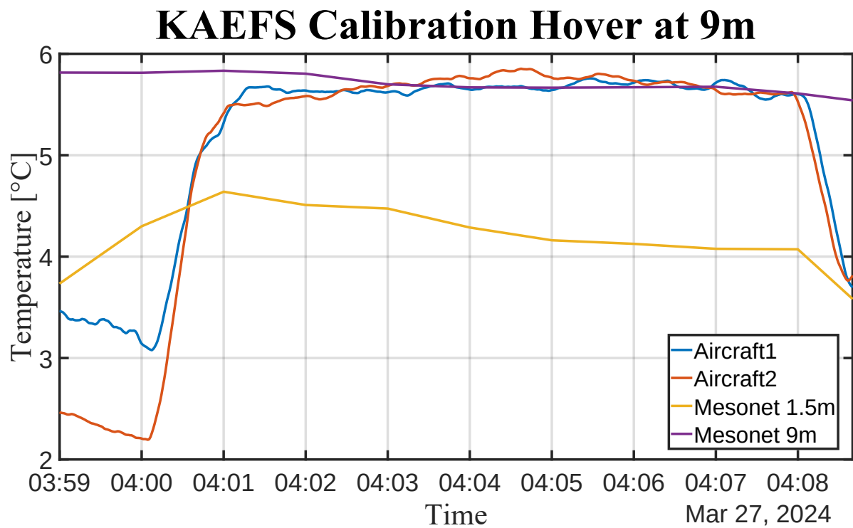
Figure B.2: Temperature time series for the tower data (1.5 and 9 m) with both aircraft data, including data before and after take-off.
