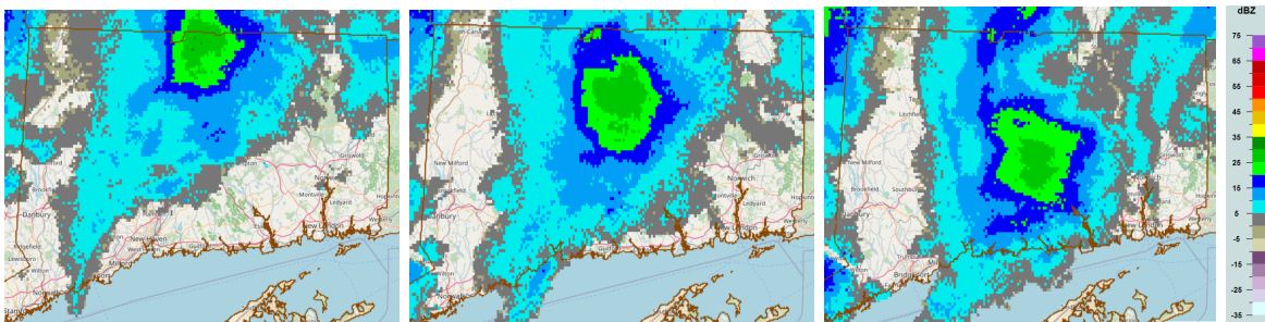
Figure 7.12: MRMS composite reflectivity for the snow band sampled on March 11 th , 2024: (left) 05:30, (center) 06:00, and (right) 06:30.
