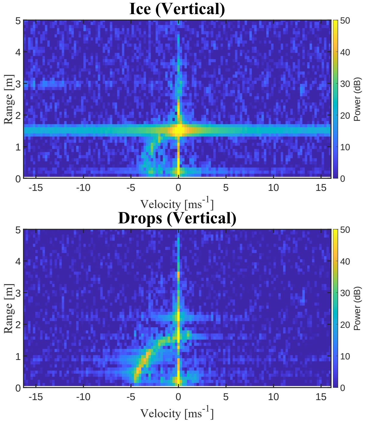
Figure 4.2: range-Doppler map for the large water drops and ice shavings falling vertically toward the radar (i.e., parallel setup).
