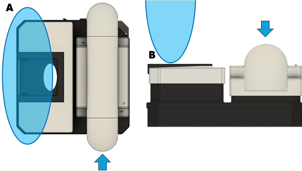
Figure 5.3: 3-Dimensional computer-aided design for this dissertation’s in-situ and remote measurement solutions with the critical obstruction zones for each measurement. (A) Orthographic top view, with elliptical shading over the radar’s field of view and arrow indicating the predominant direction for the incoming wind for in-situ samples. (B) Orthographic front view with the same obstruction regions.
