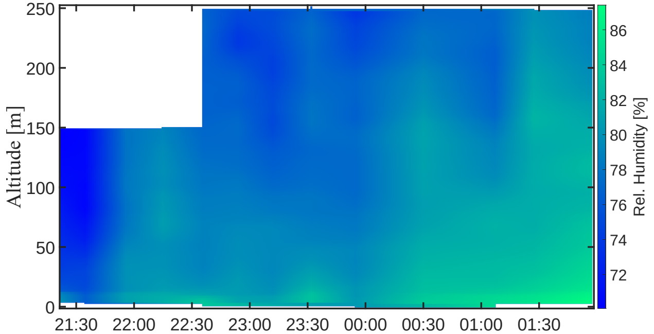
Figure 7.7: Relative humidity map for the WxUAS profiles on March 9, 2024.
