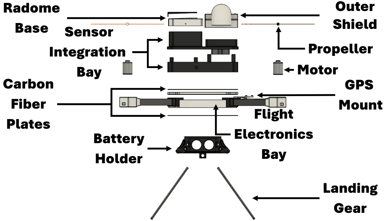
Figure 5.2: Exploded orthographic front view of the main components in the 3-dimensional computer-aided design for this dissertation’s WxUAS technology demonstration platform.
