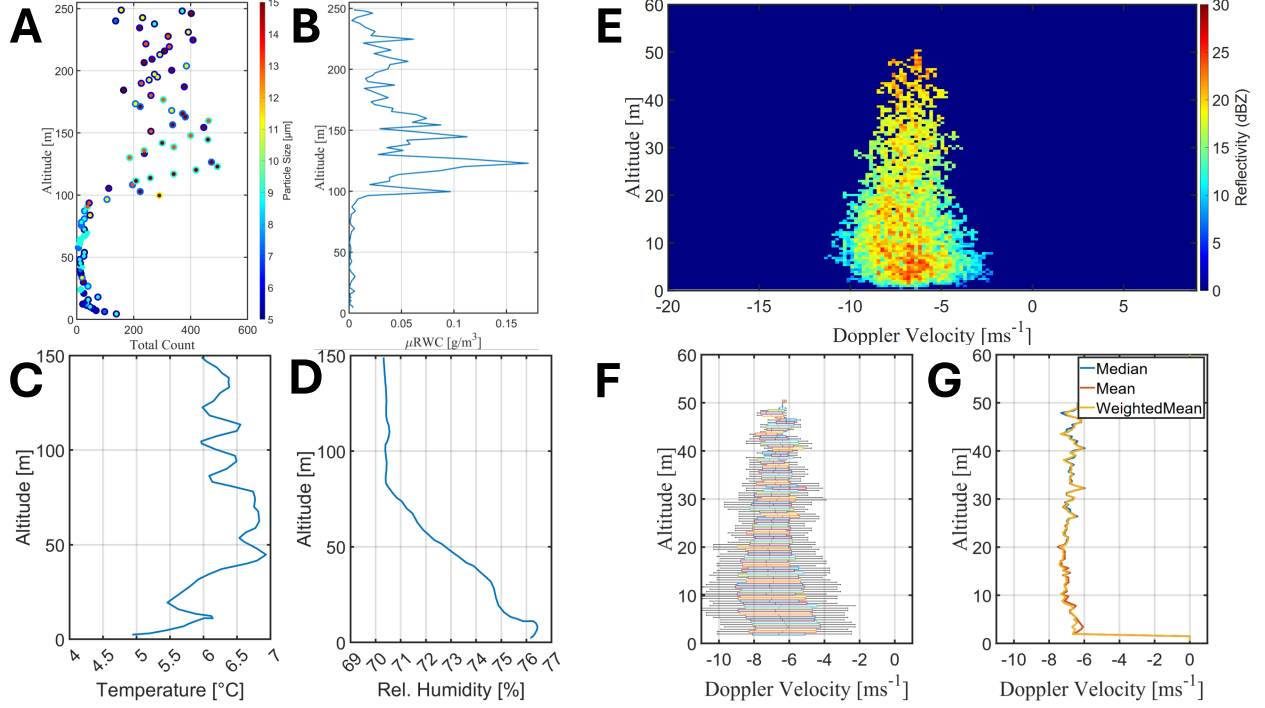
Figure 6.1: Illustration of the graphical summaries for a profile gathered by this dissertation’s WxUAS. Variations with height for: (A) particle size distribution, (B) micro-range Water content, (C) temperature, and (D) relative humidity. Along with one of the many similar snapshots produced by the radar during a profile with (E) Doppler-range map, (F) Doppler velocity distributions, and (G) mean velocity.
