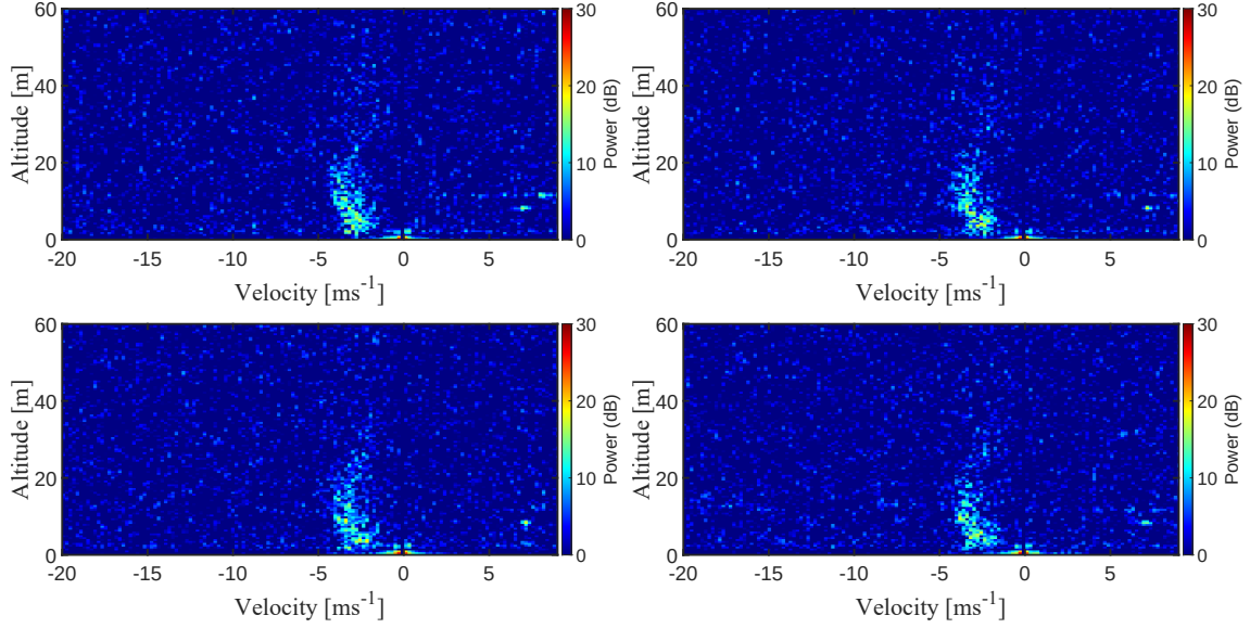
Figure 4.9: Range-Doppler map for the four frames of an atmospheric profile during a drizzle event at the MAI 2 S field campaign. The data presented here includes the aircraft compensation algorithm.
