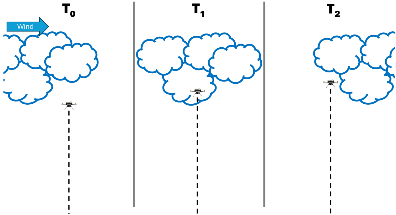
Figure 8.3: Illustration of weather passing through the WxUAS profile path and inducing unexpected measurement values (e.g., sharp increase and decrease in relative humidity).
