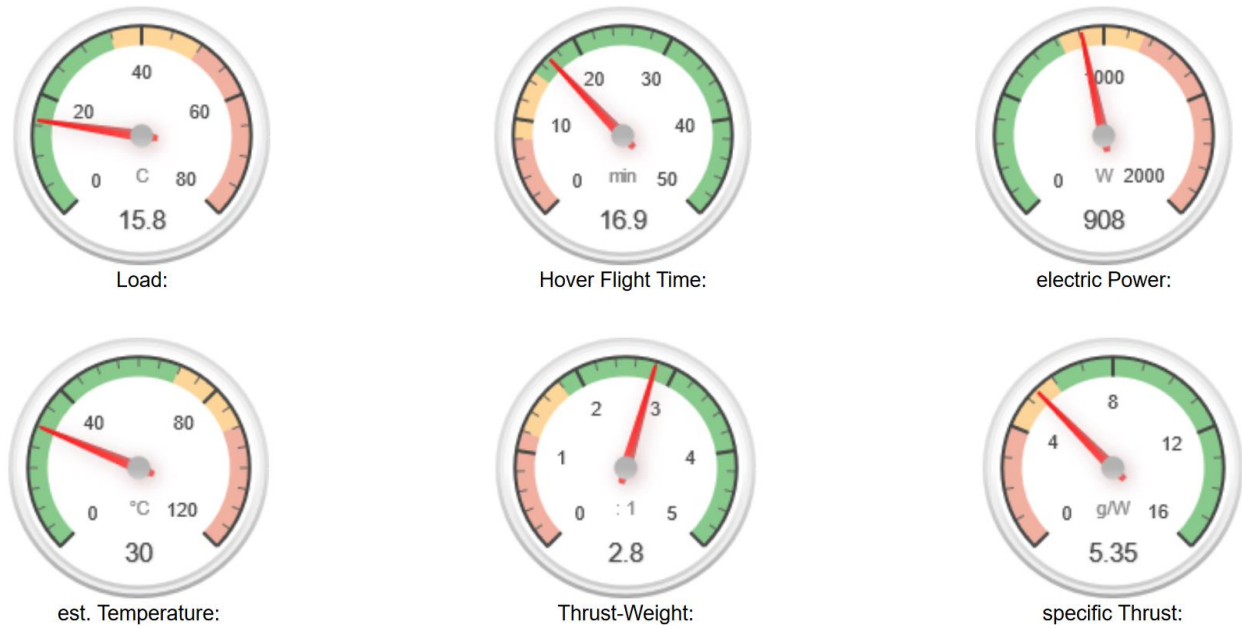
Figure 5.9: Performance metrics for the StormTrooper winter precipitation WxUAS in its baseline configuration.
