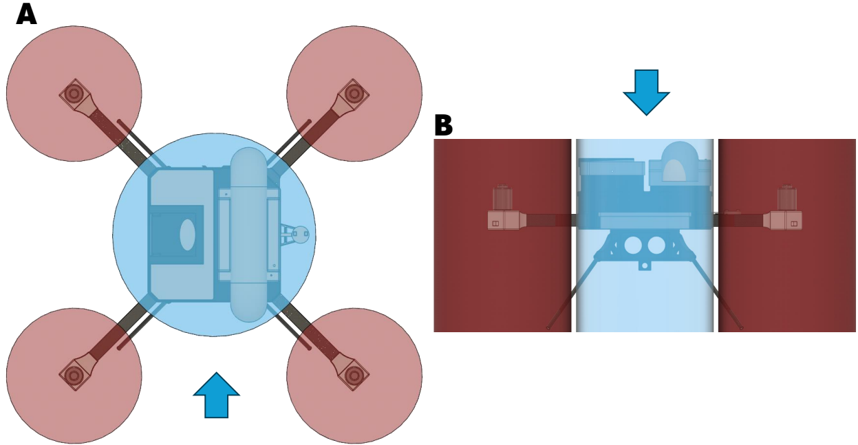
Figure 5.4: 3-Dimensional computer-aided design illustrating how the aircraft arm length can be defined based on propeller size to allow an unimpeded path to the sensors. (A) The aircraft’s orthographic top view with the red shaded areas representing the propeller discs and the blue shaded area representing the 1.5-propeller diameter clearance from above. (B) Orthographic front view with the same highlighted regions.
