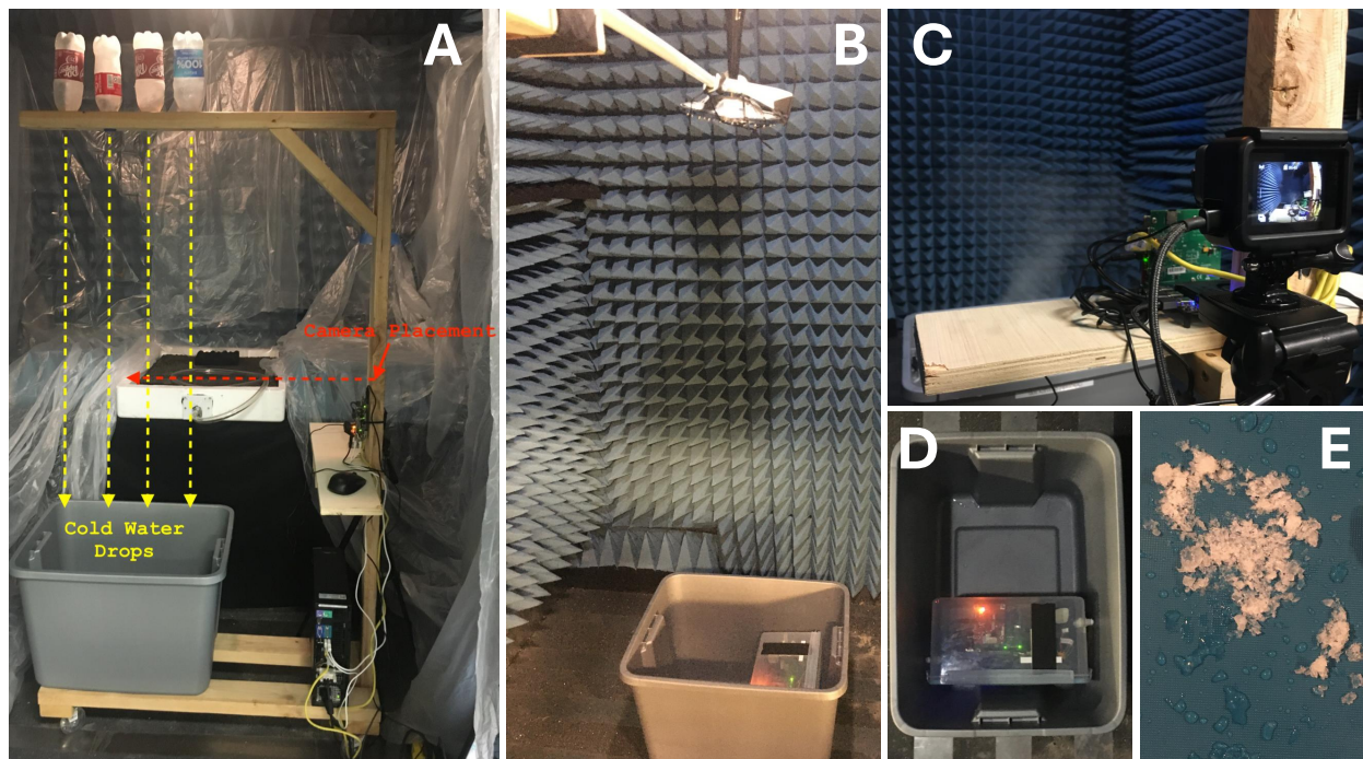
Figure 4.1: Experimental setup for initial evaluation of the TI AWR2243: (A) the setup for precipitation perpendicular to the radar beam, (B) the parallel setup. (C) The perpendicular “Mist” experiment. (D) The improvised radome to emulate a vertically pointing radar in parallel experiments. (E) The ice shavings used to mimic frozen precipitation.
