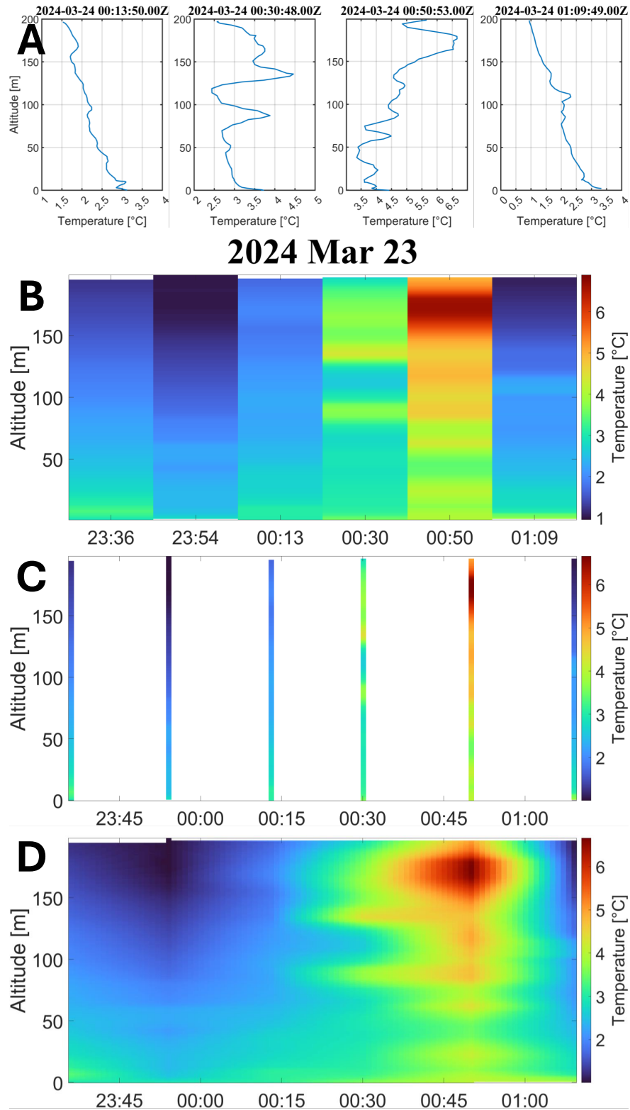
Figure 6.2: Illustration of the steps to produce the time-height maps that graphically summarize the WxUAS spatiotemporal datasets.
