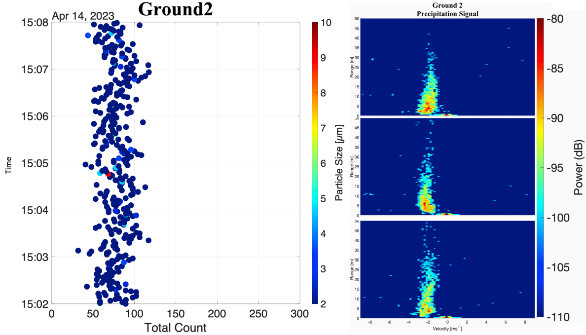
Figure 3.14: Results for particle size distribution (left) and power and Doppler velocity (right) during the second ground-based experiment. For the vertically pointing radar, negative Doppler velocities indicate particles falling towards the radar.
