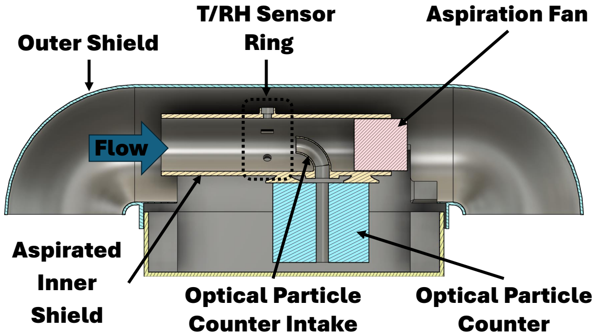
Figure 3.1: Lateral cross-section of the two-layer custom sensor shield designed to prevent contact with freezing precipitation while allowing for direct atmospheric observation.
