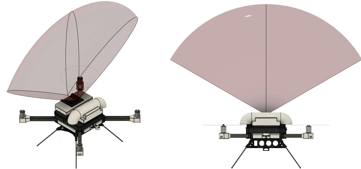
Figure 4.4: Illustration of the multiple angles scanned by the TI AWR2243 PAR, which can be leveraged to compensate aircraft motion in pitch.
