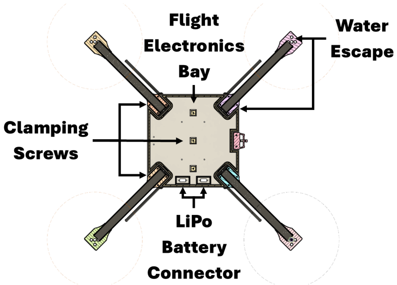
Figure 5.6: Horizontal cross-section of the aircraft's orthographic top view highlighting the two water escaping points within the motor arm.
