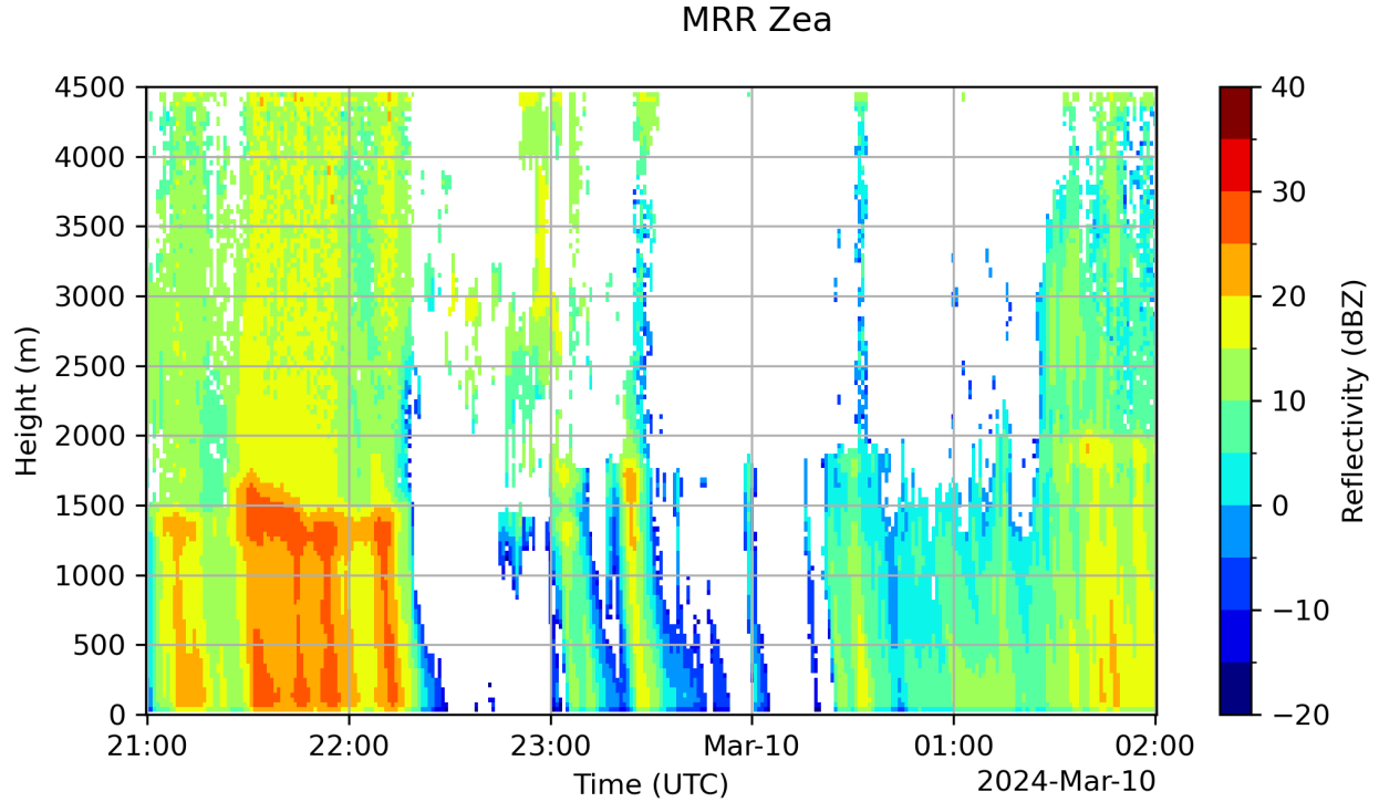
Figure 7.6: Height-time map for precipitation reflectivity from the colocated MRRs.
