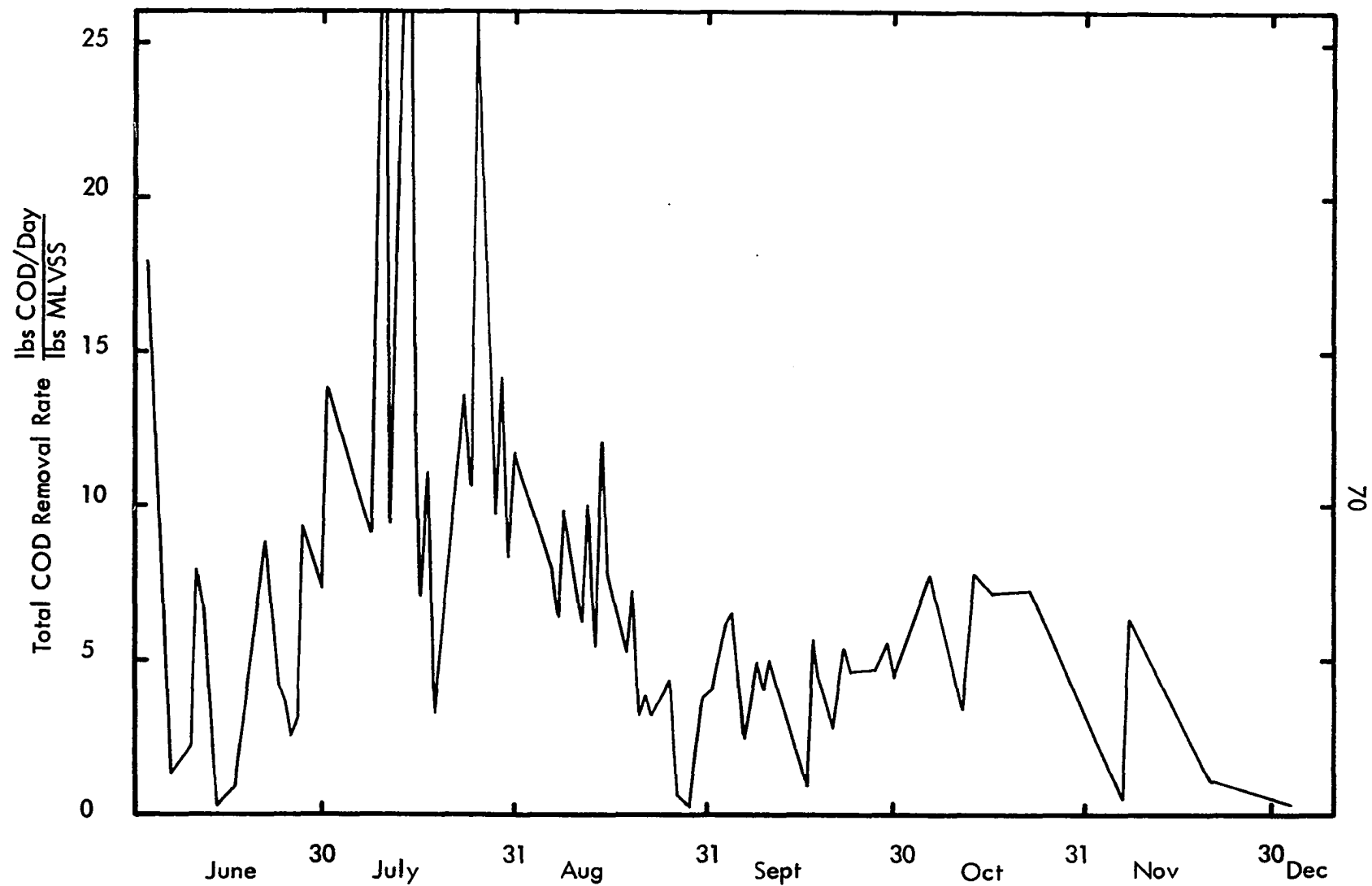
Figure 24 Soluble COD Removal Rate of Minimal Solids (High Loading) Unit
