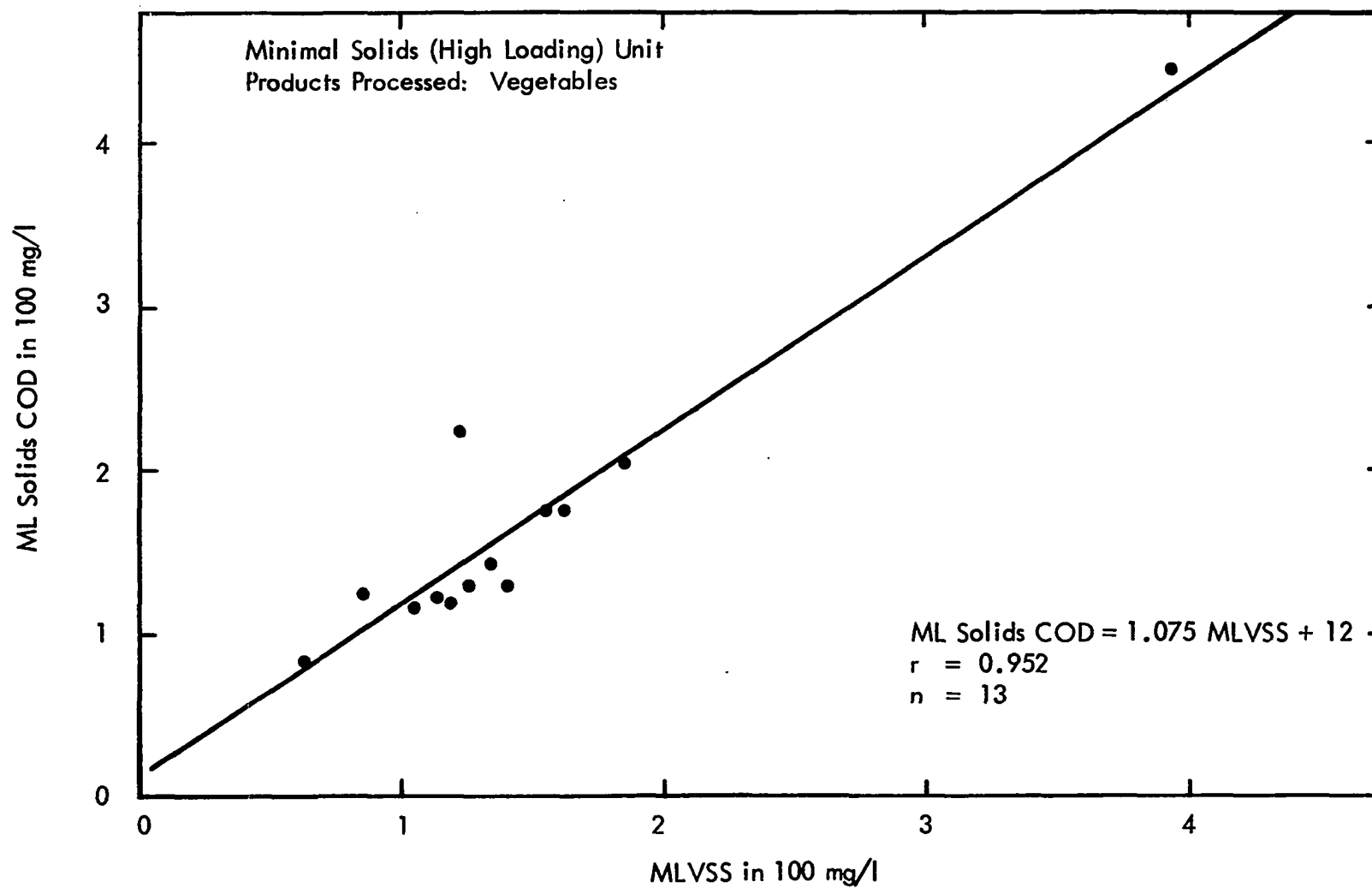
Figure 64 ML Solids COD vs MLVSS
