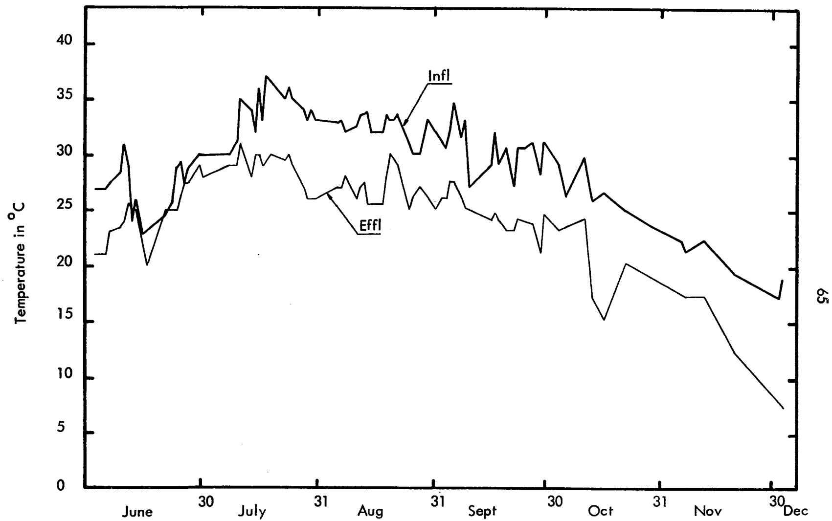
Figure 19 Temperature of Plant Influent and Effluent
