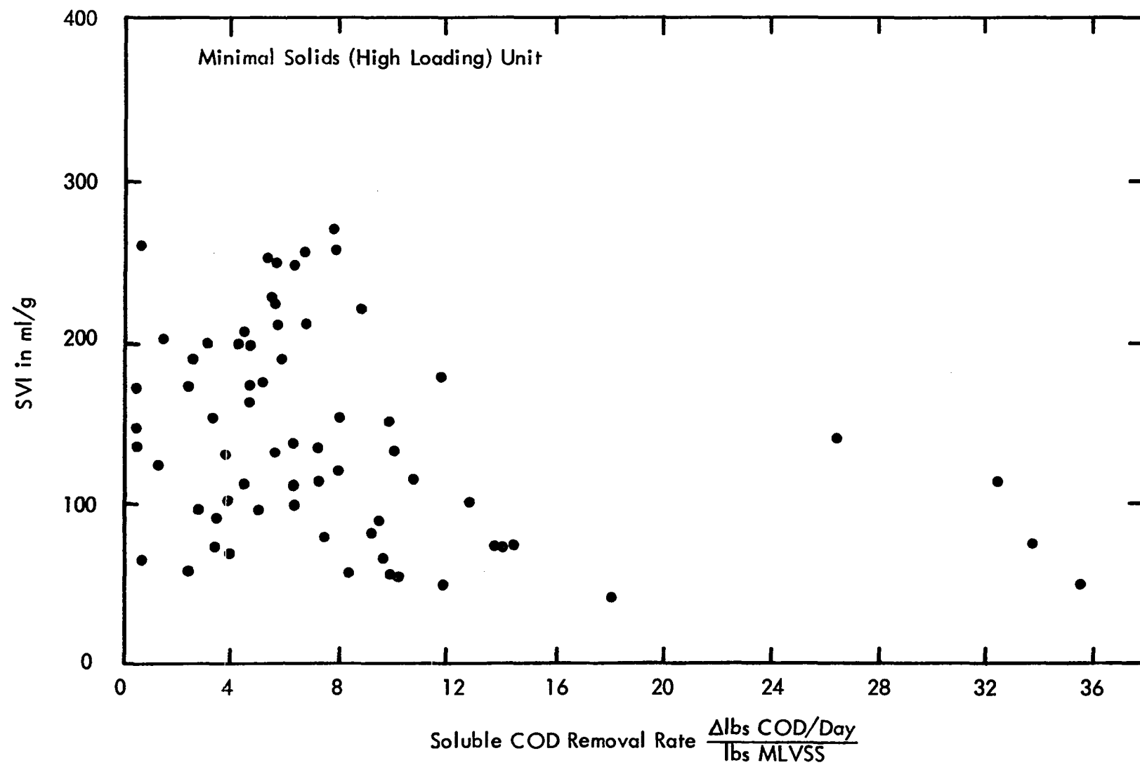
Figure 85 SVI vs Soluble COD Removal Rate
