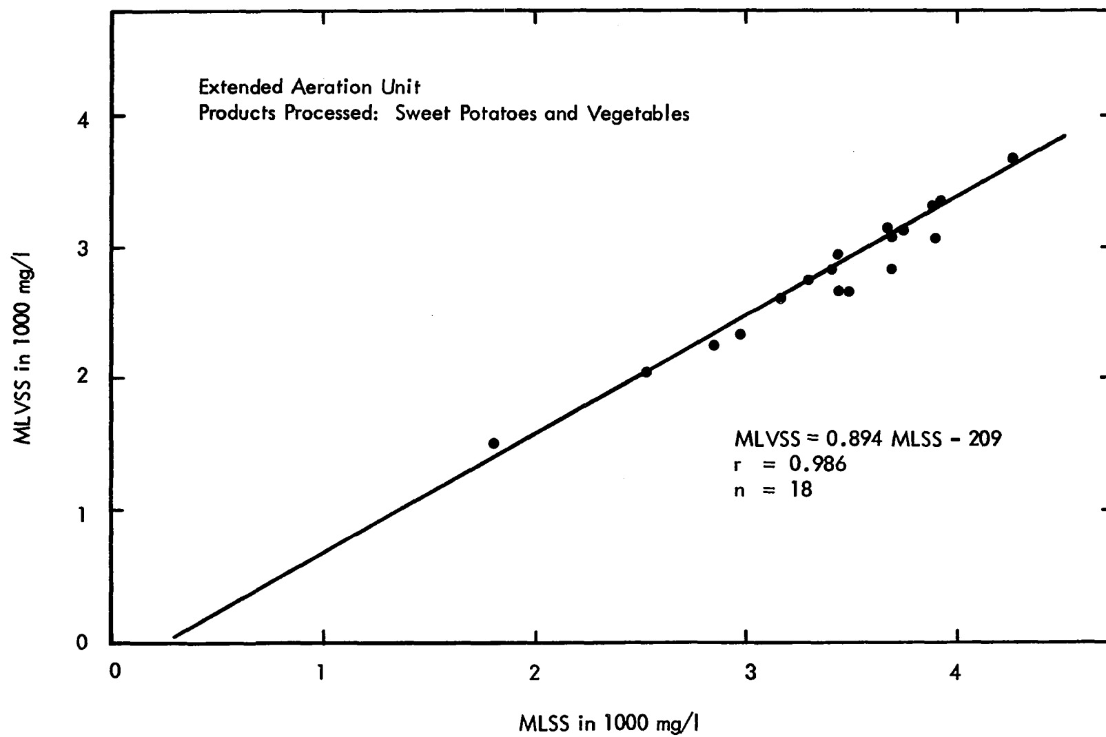
Figure 68 MLVSS vs MLSS
