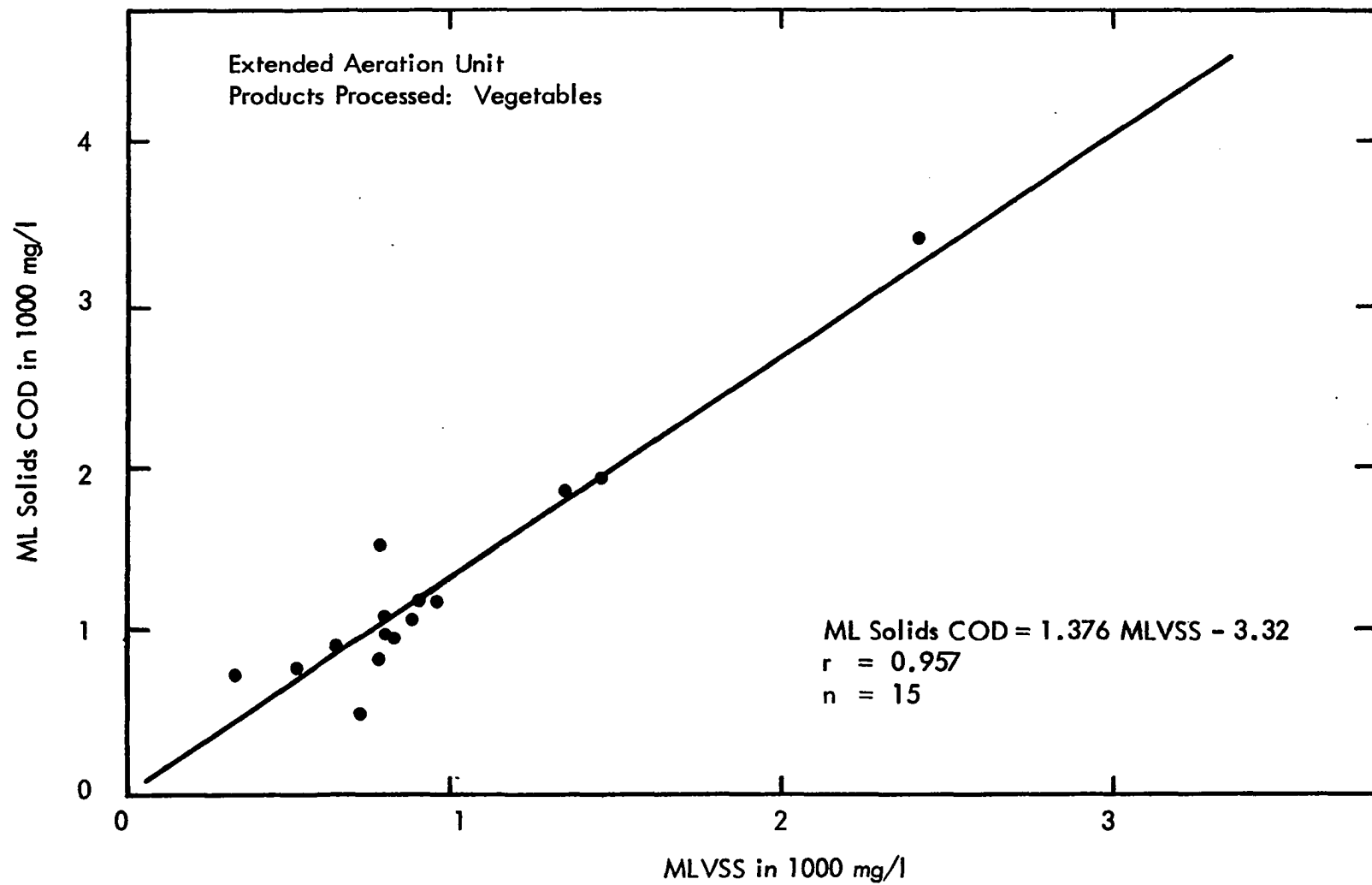
Figure73 ML Solids COD vs MLVSS
