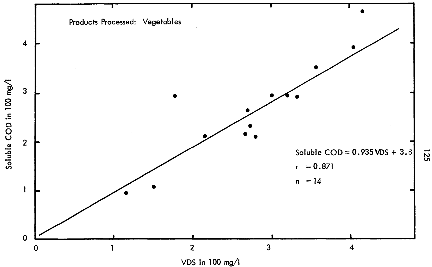
Figure 54 Plant Influent Soluble COD vs VDS
