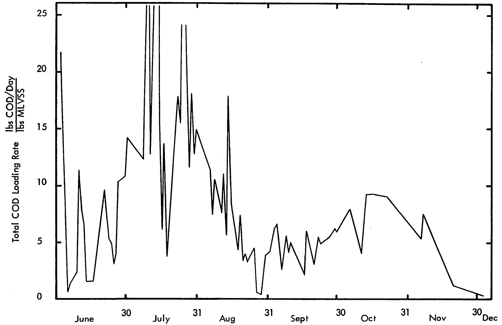
Figure 23 Total COD Loading Rate of Minimal Solids (High Loading) Unit
