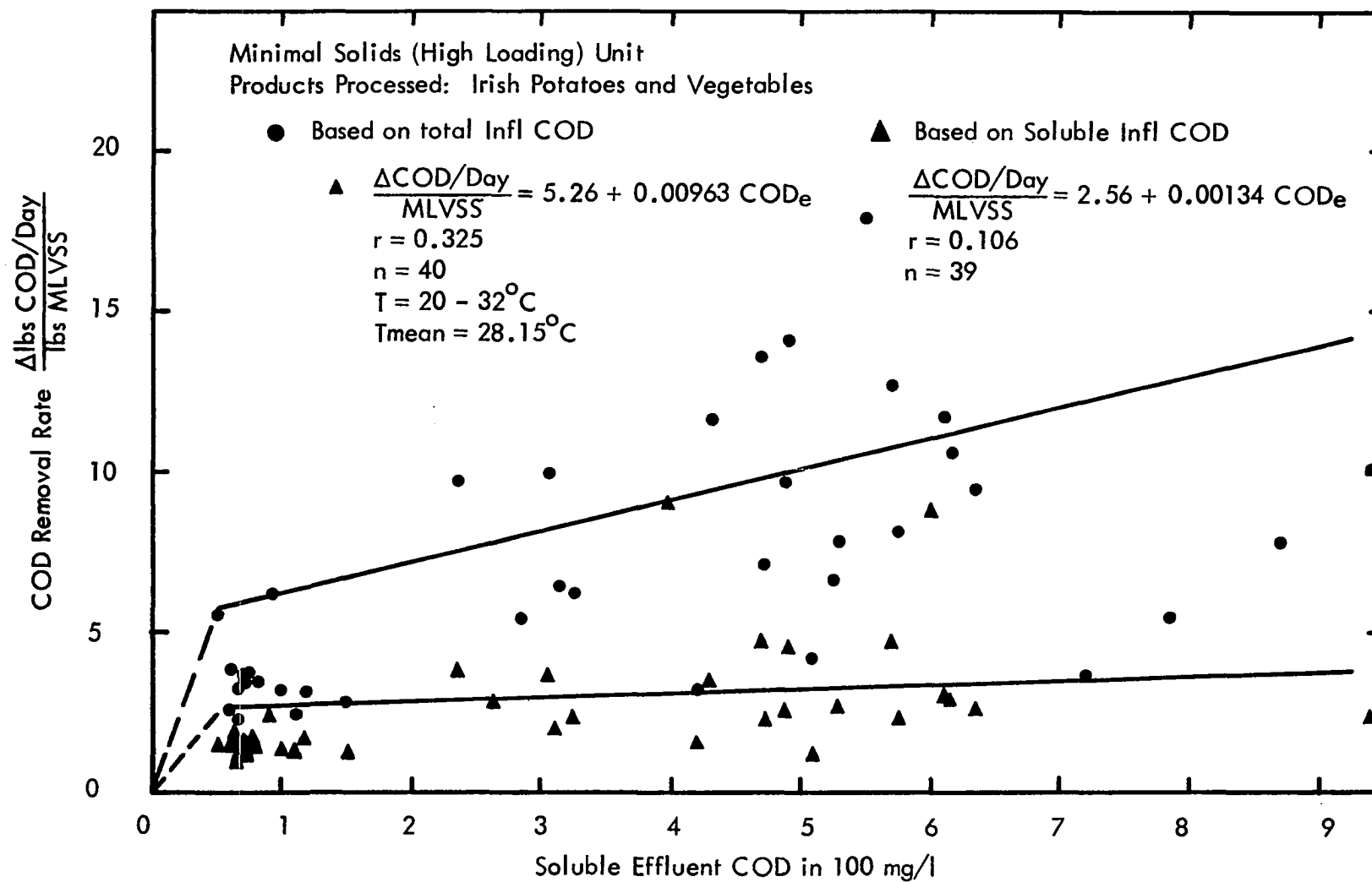
Figure 57 COD Removal Rate vs Soluble Effluent COD
