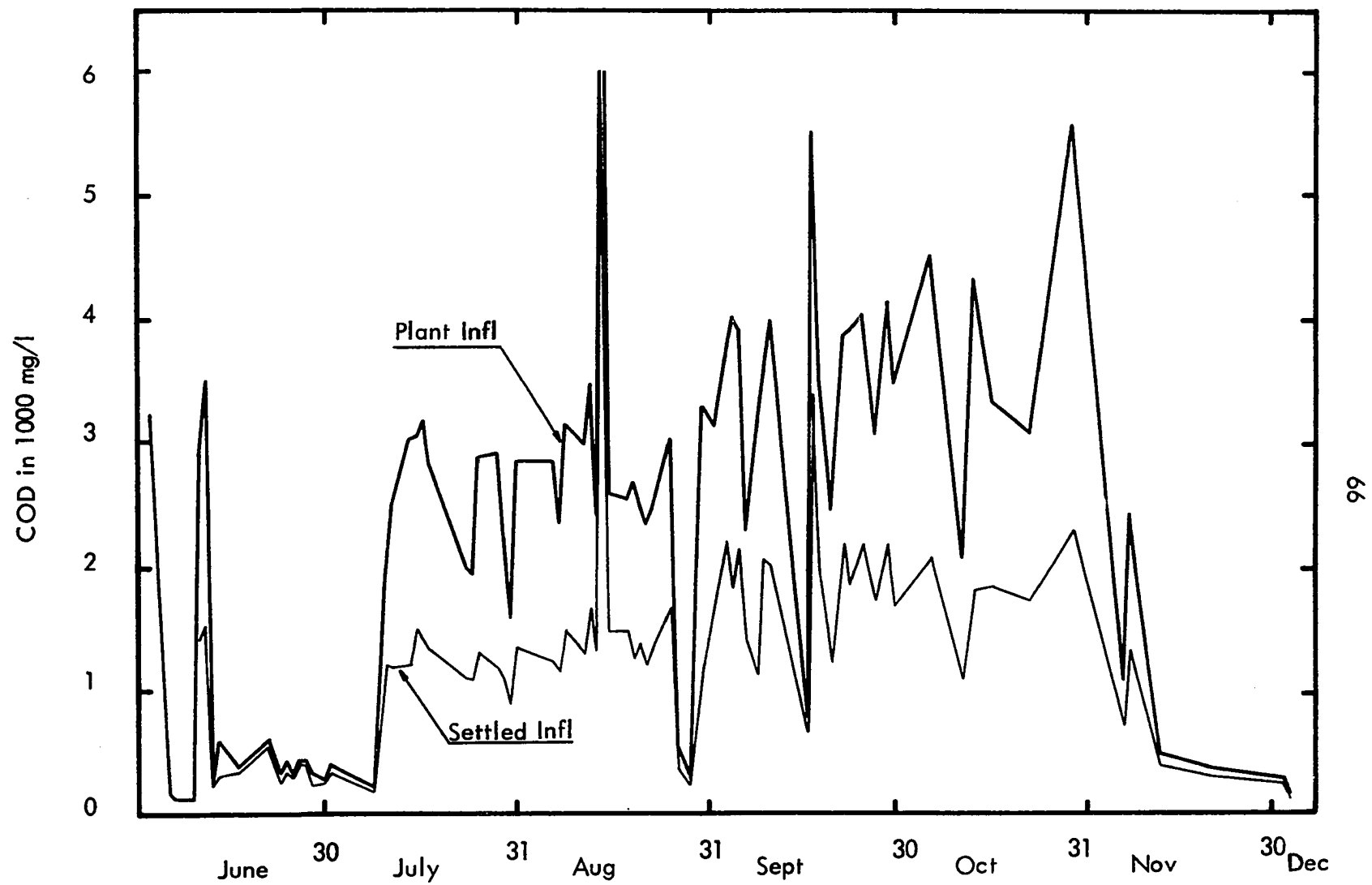
Figure 20 Plant Influent and Settled Influent COD
