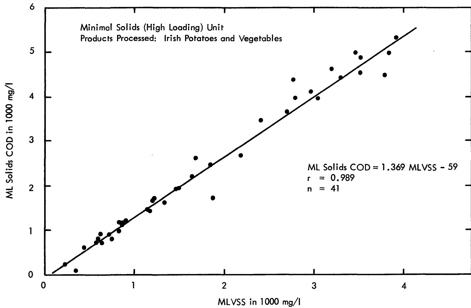
Figure 62 ML Solids COD vs MLVSS
