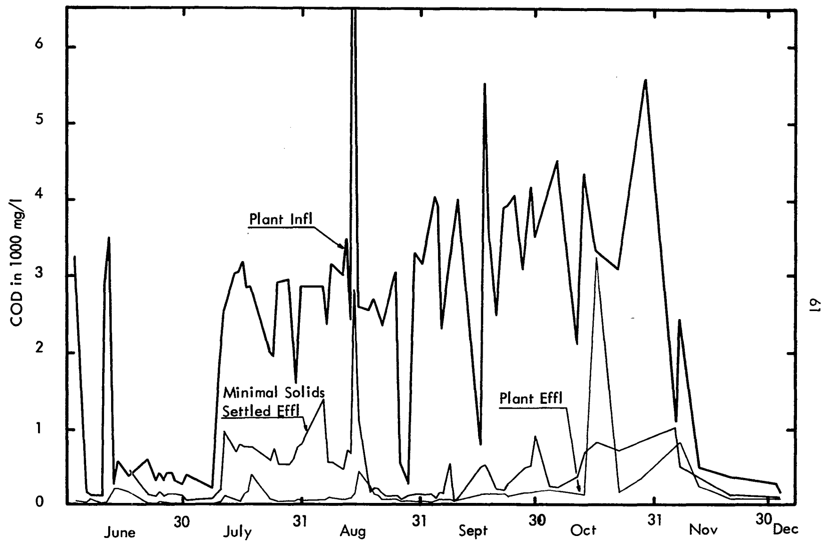
Figure 15 Treatment Plant Performance - COD
