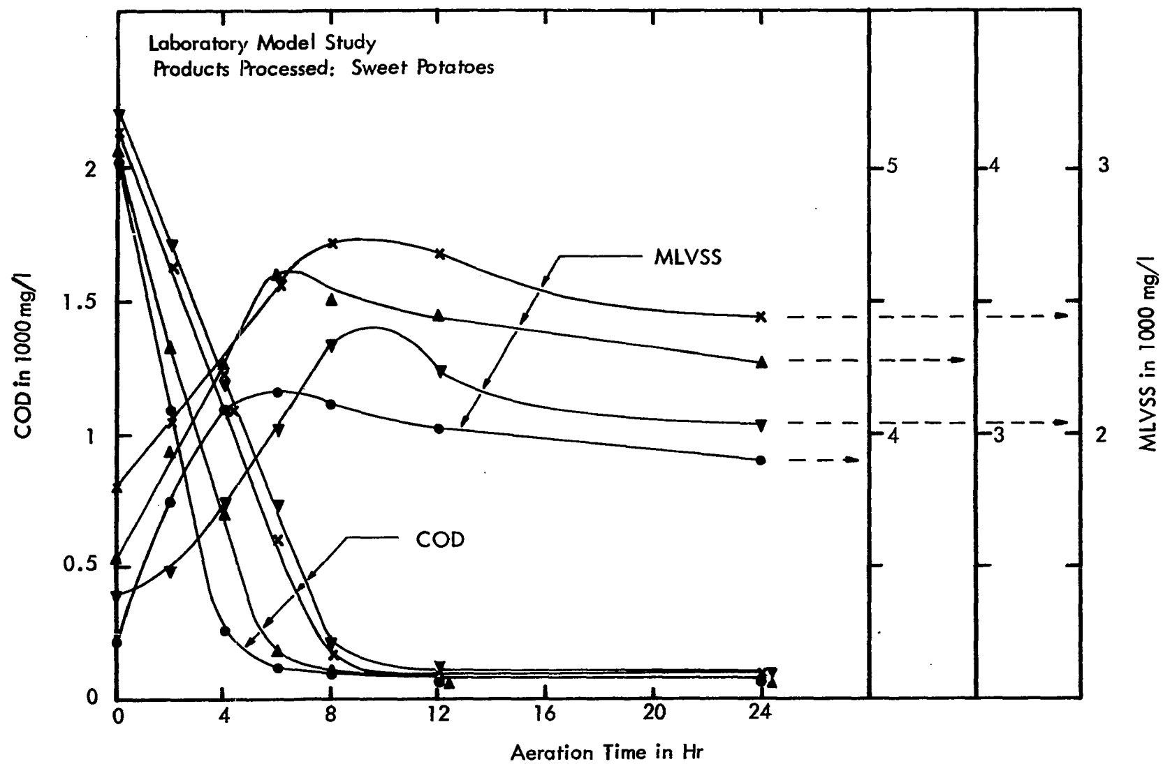
Figure 83 COD Removal and Bio-Solids Growth vs Aeration Time
