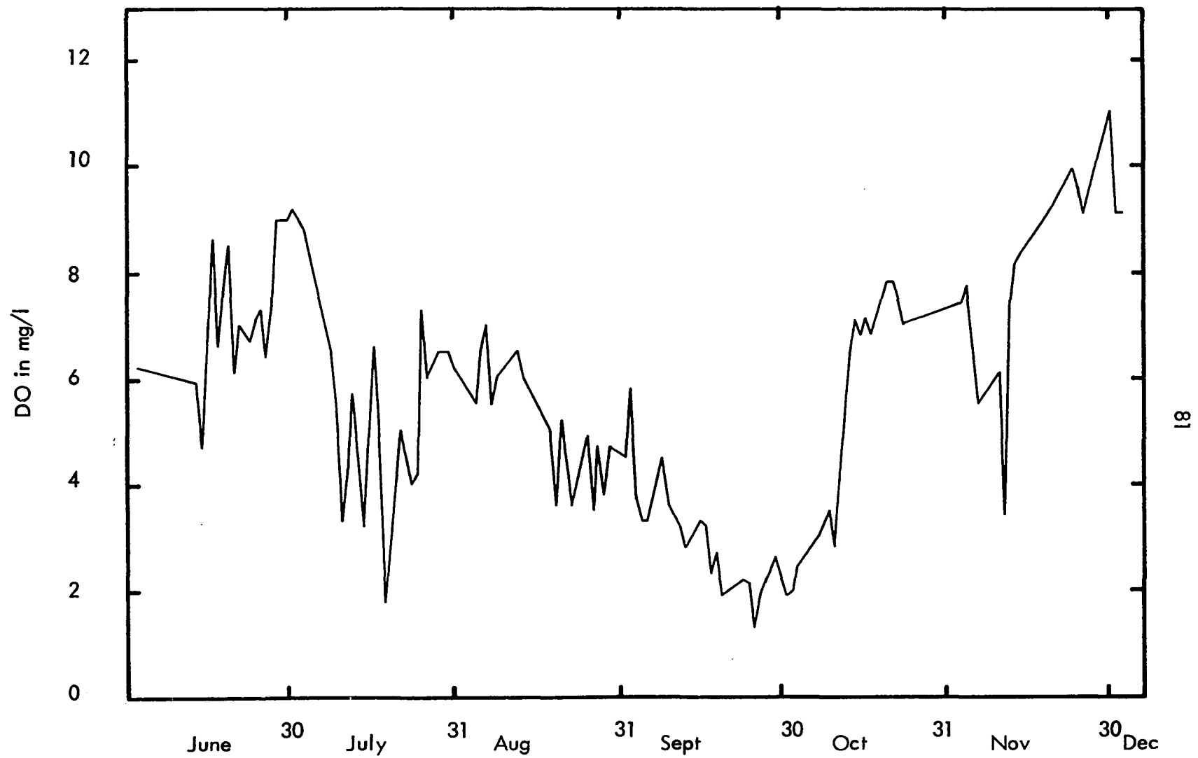
Figure 35 DO of Caney Creek at Outfall
