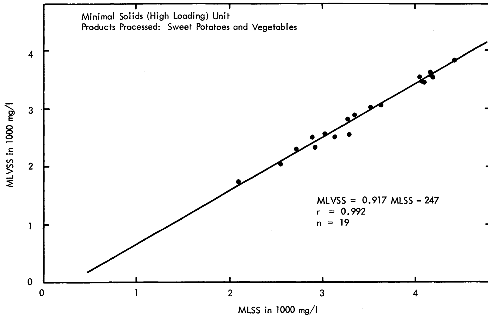
Figure 59 MLVSS vs MLSS
