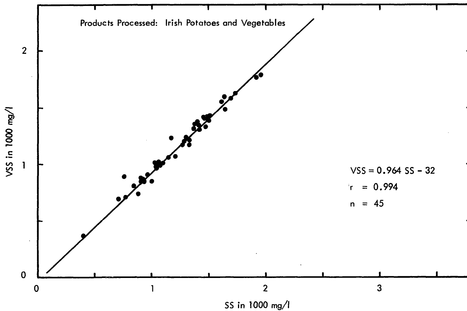
Figure 41 Plant Influent VSS vs SS
