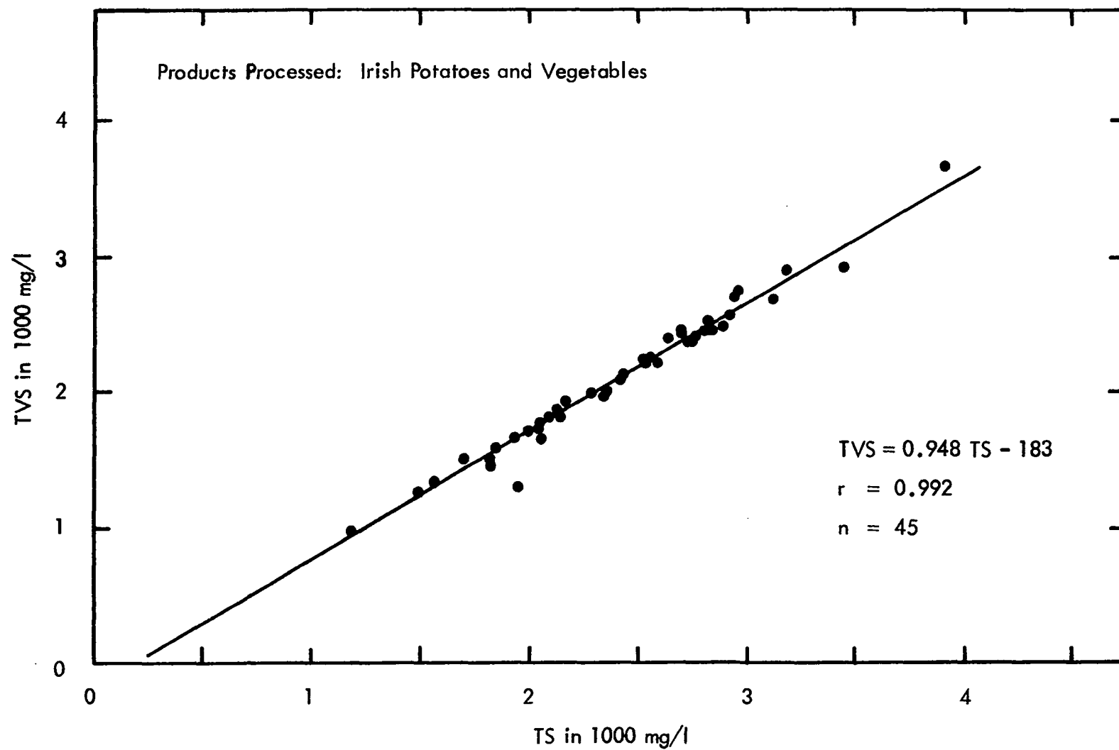
Figure 43 Plant Influent TVS vs TS
