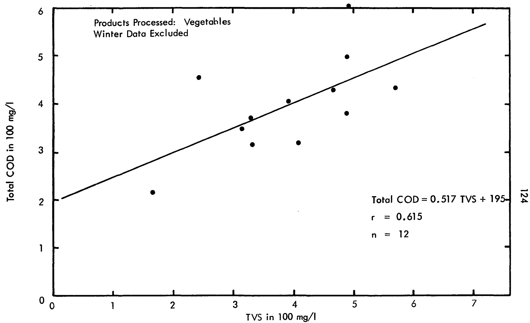
Figure 53 Plant Influent Total COD vs TVS
