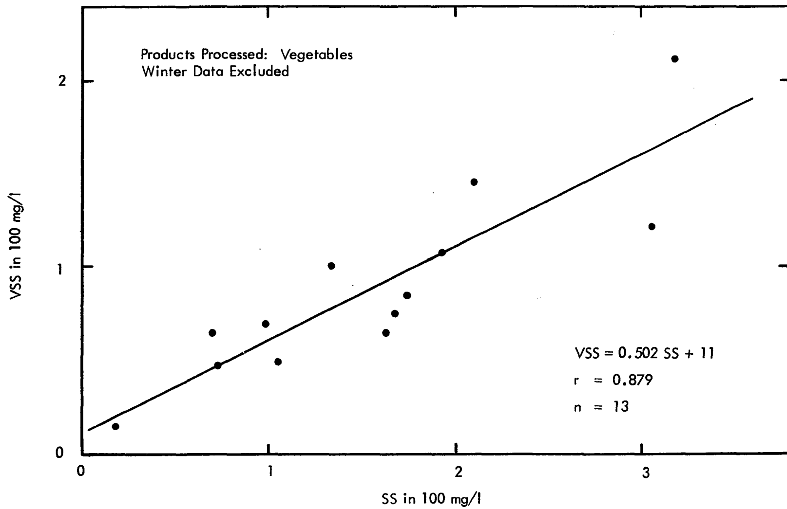
Figure 47 Plant Influent VSS vs SS
