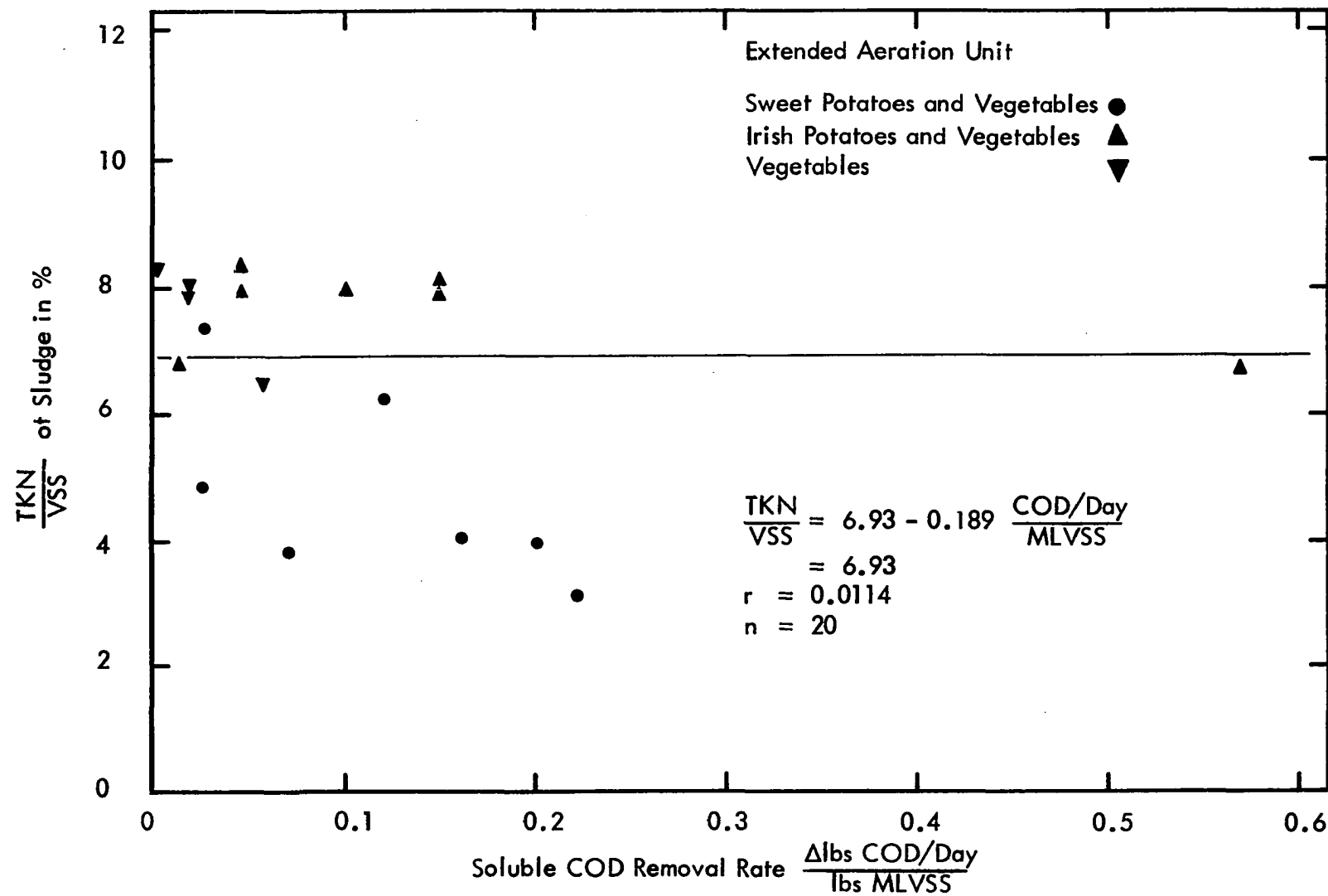
Figure 88 \frac{\text{TKN}}{\text{VSS}} of Sludge vs Soluble COD Removal Rate
