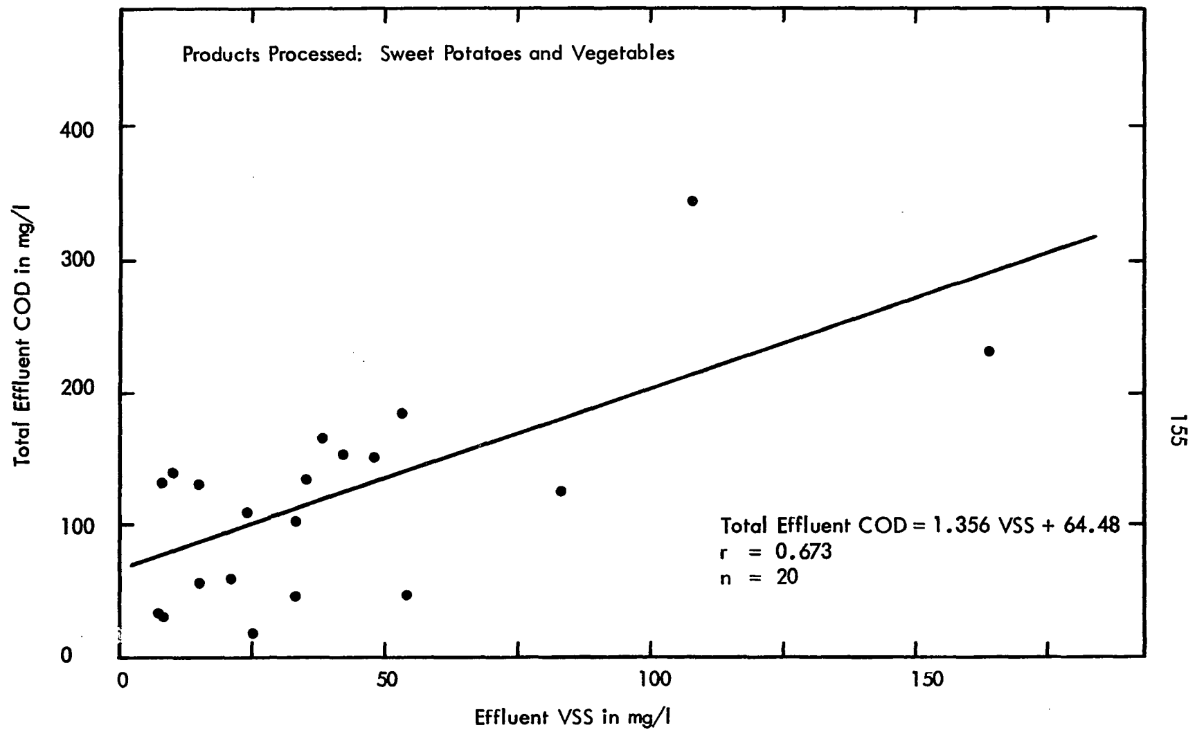
Figure 75 Plant Total Effluent COD vs VSS
