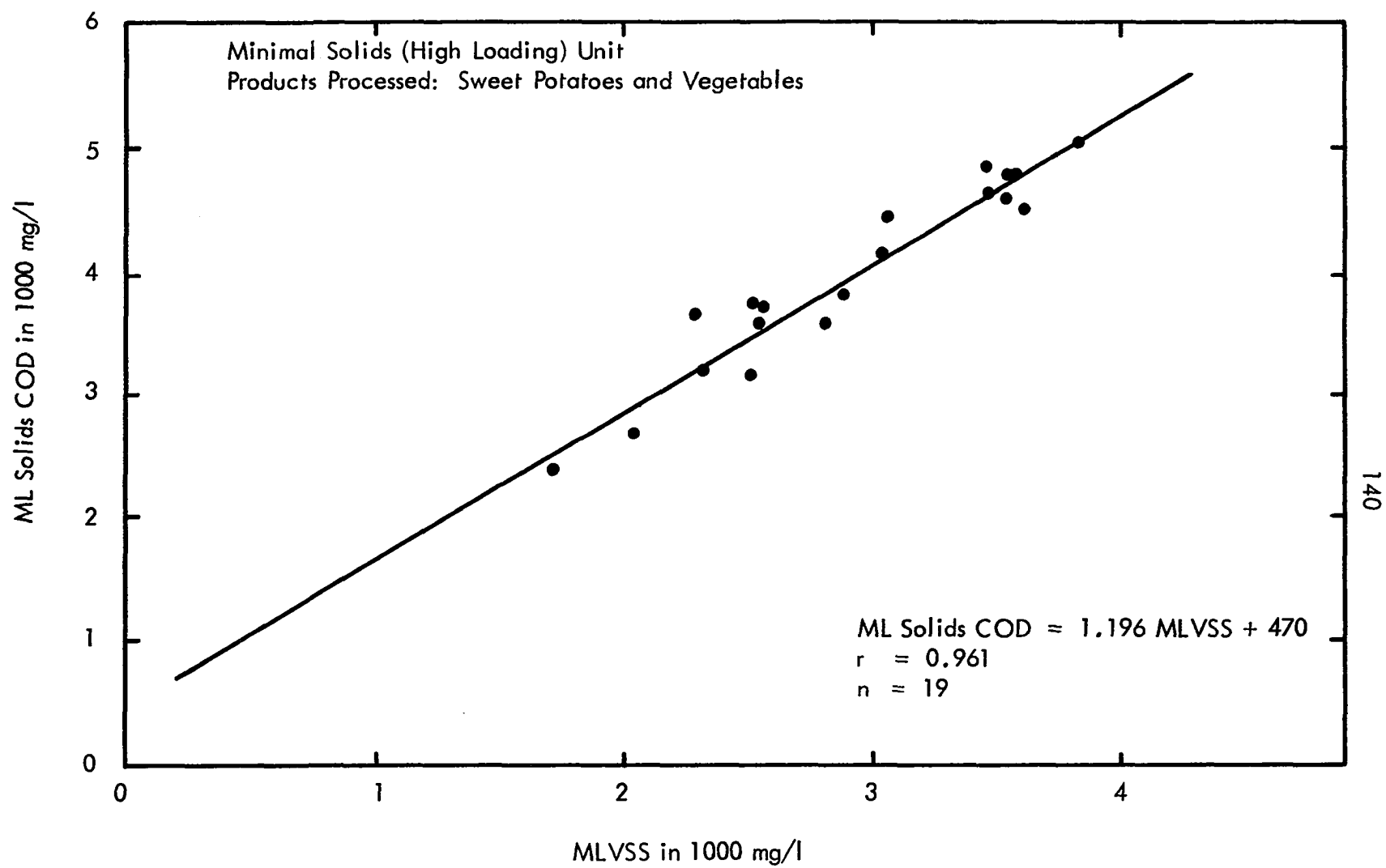
Figure 60 ML Solids COD vs MLVSS
