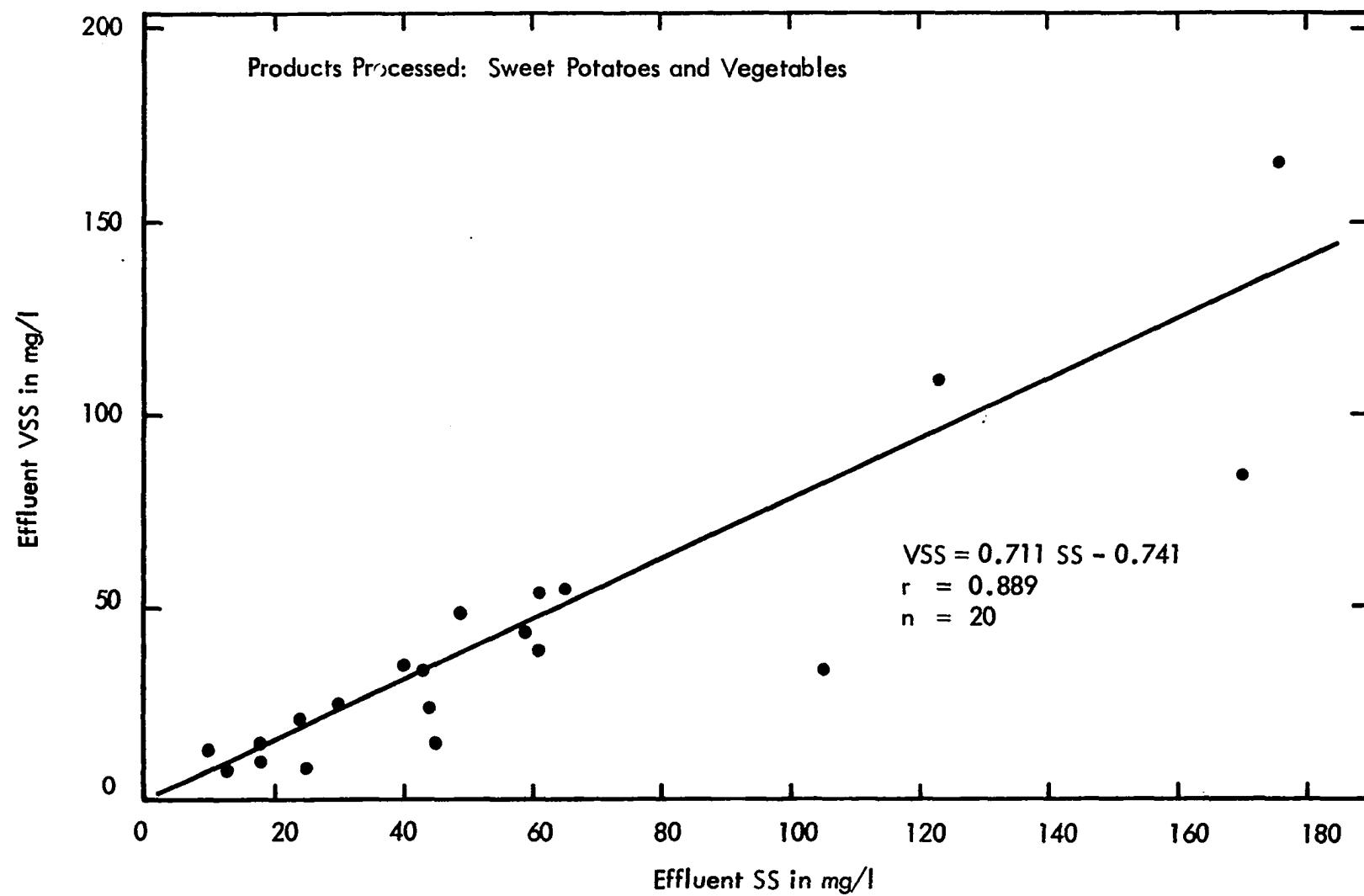
Figure 74 Plant Effluent VSS vs SS
