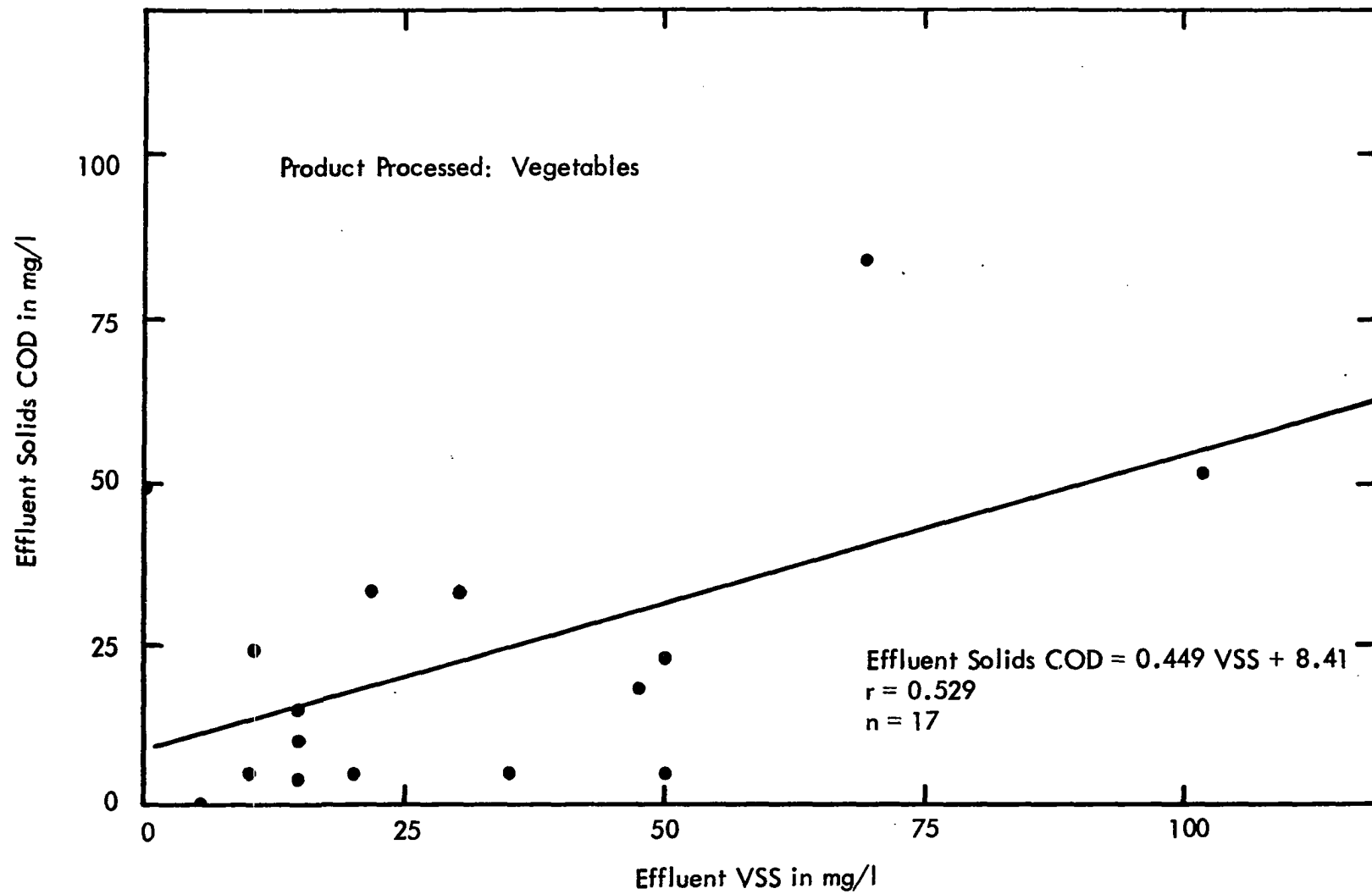
Figure 82 Effluent Solids COD vs VSS
