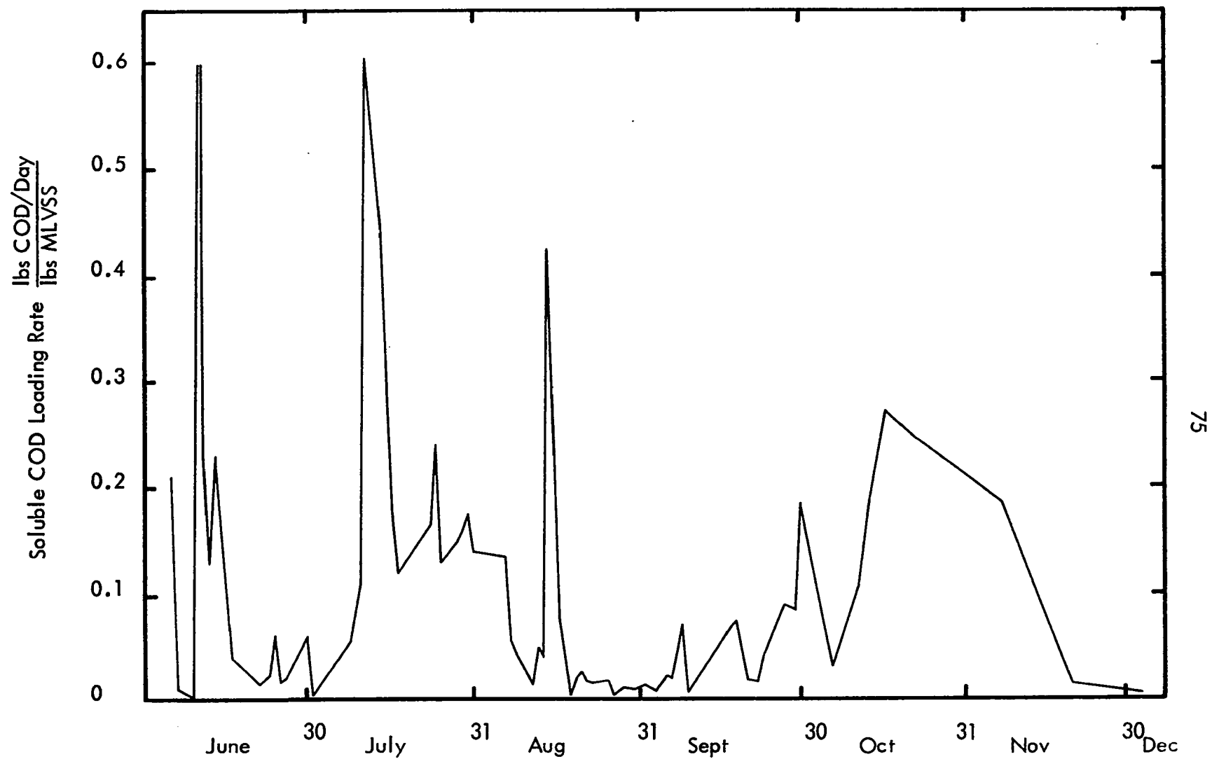
Figure 29 Soluble COD Loading Rate of Extended Aeration Unit
