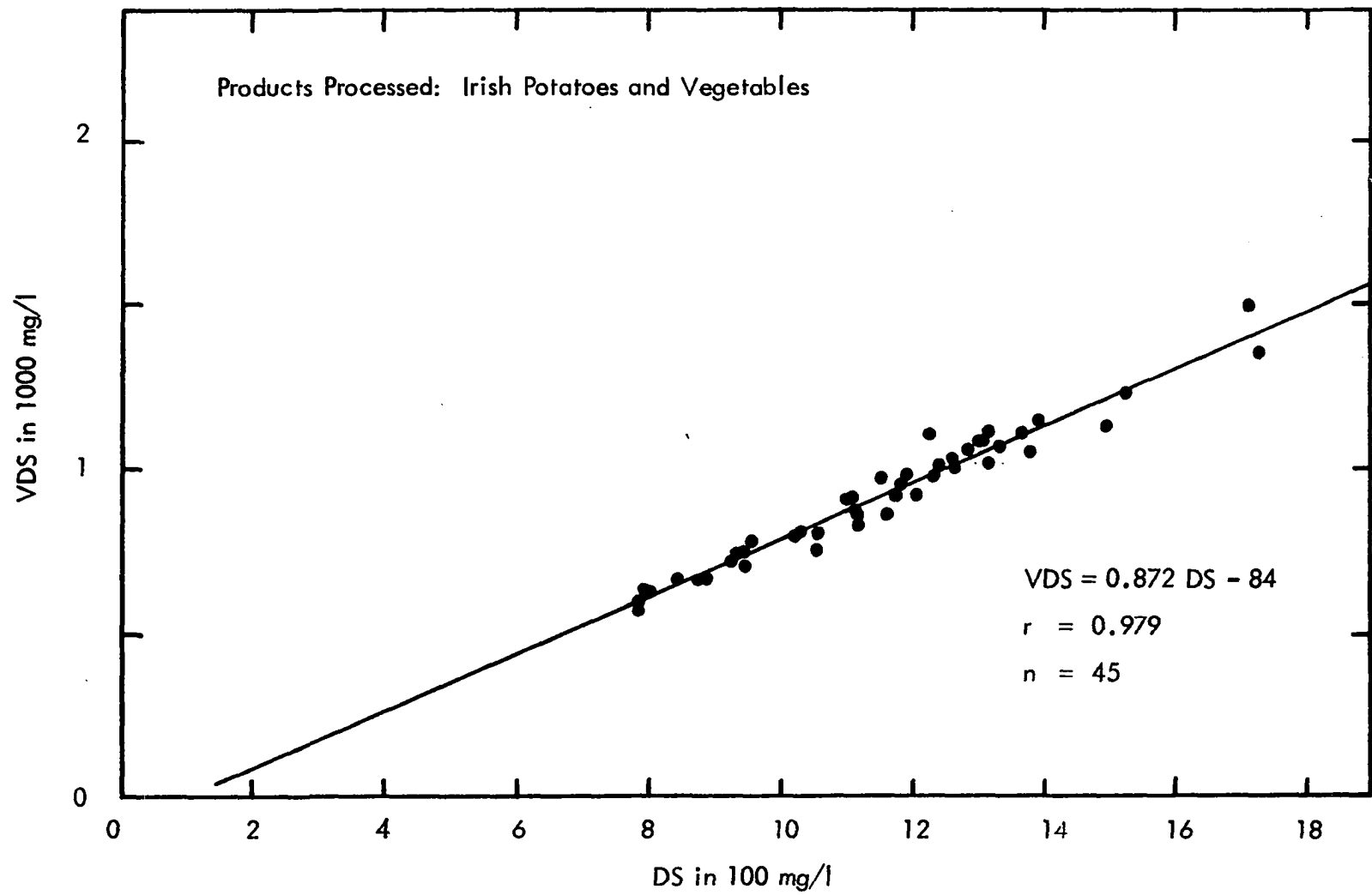
Figure 42 Plant Influent VDS vs DS
