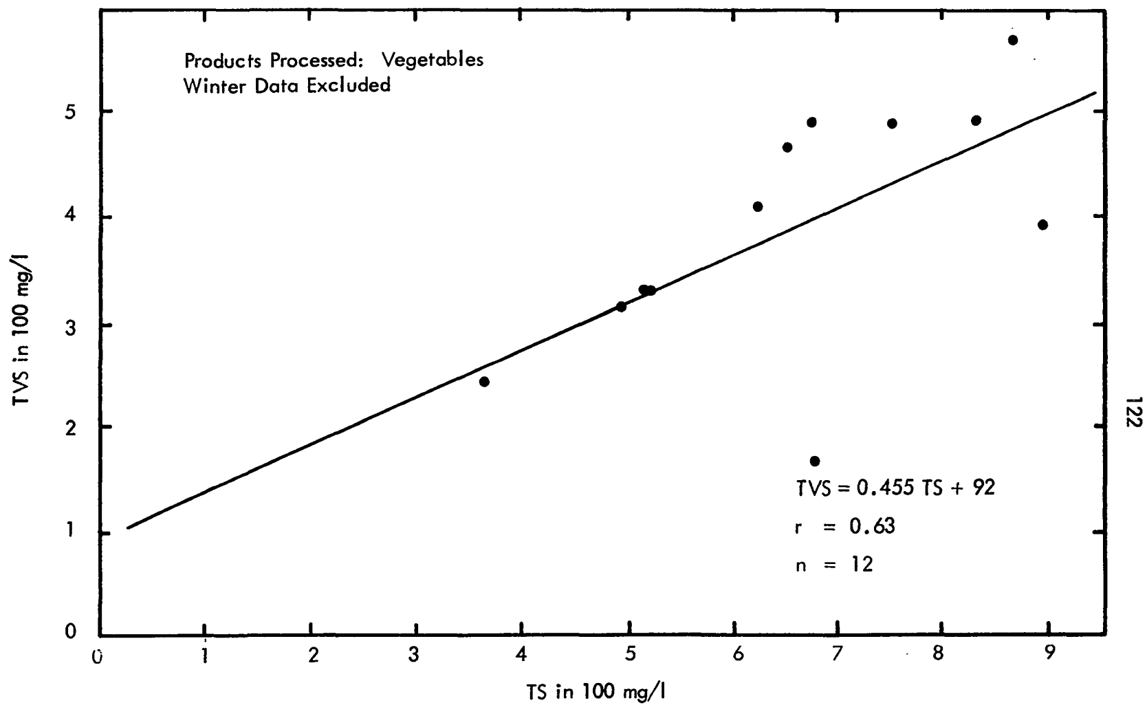
Figure 51 Plant Infuent TVS vs TS
