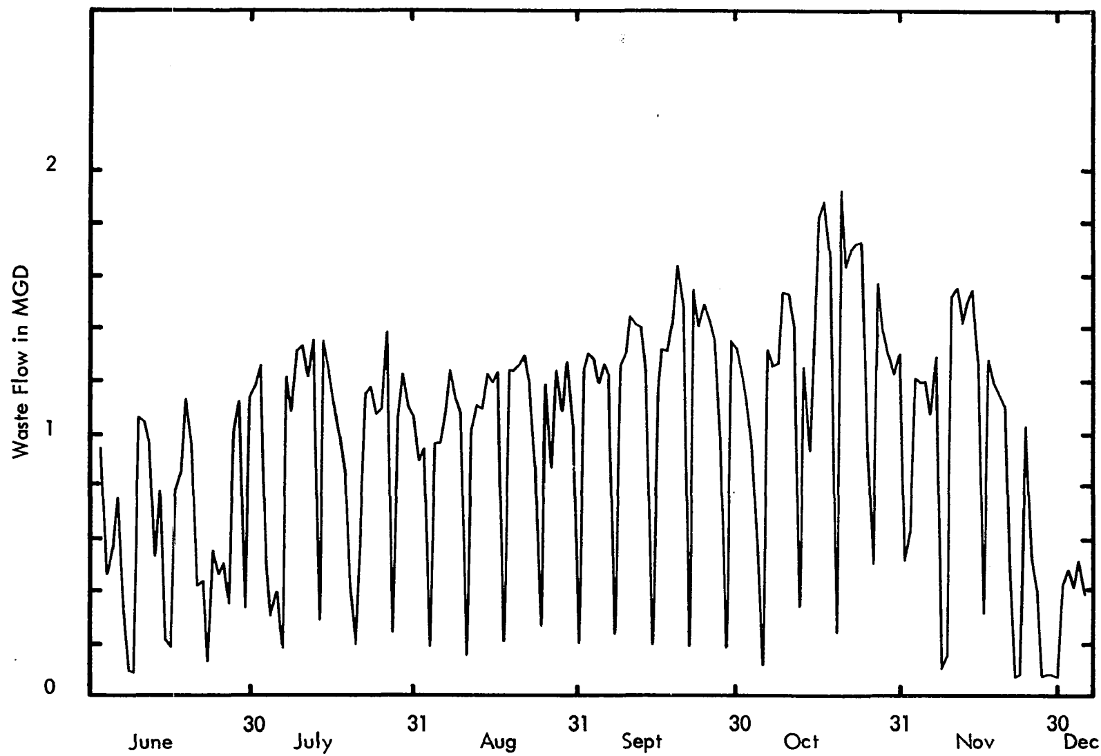
Figure 13 Waste Flow Variation
