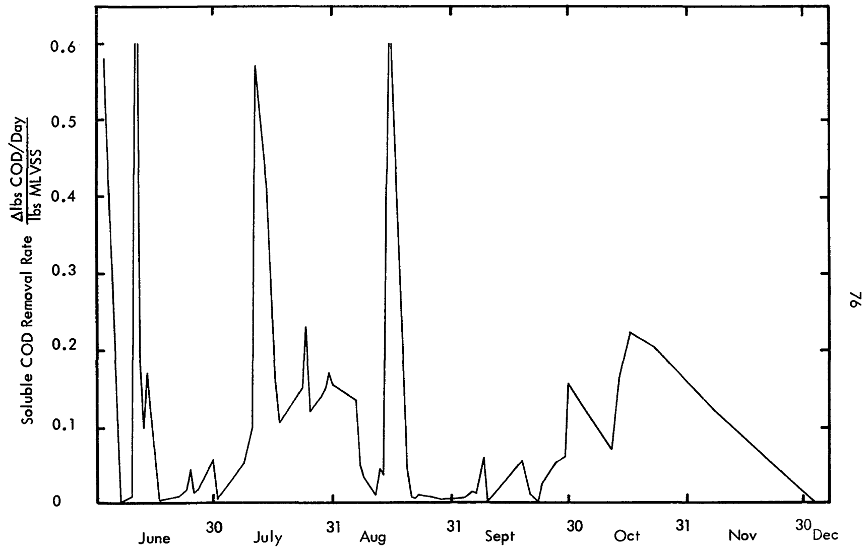
Figure 30 Soluble COD Removal Rate of Extended Aeration Unit
