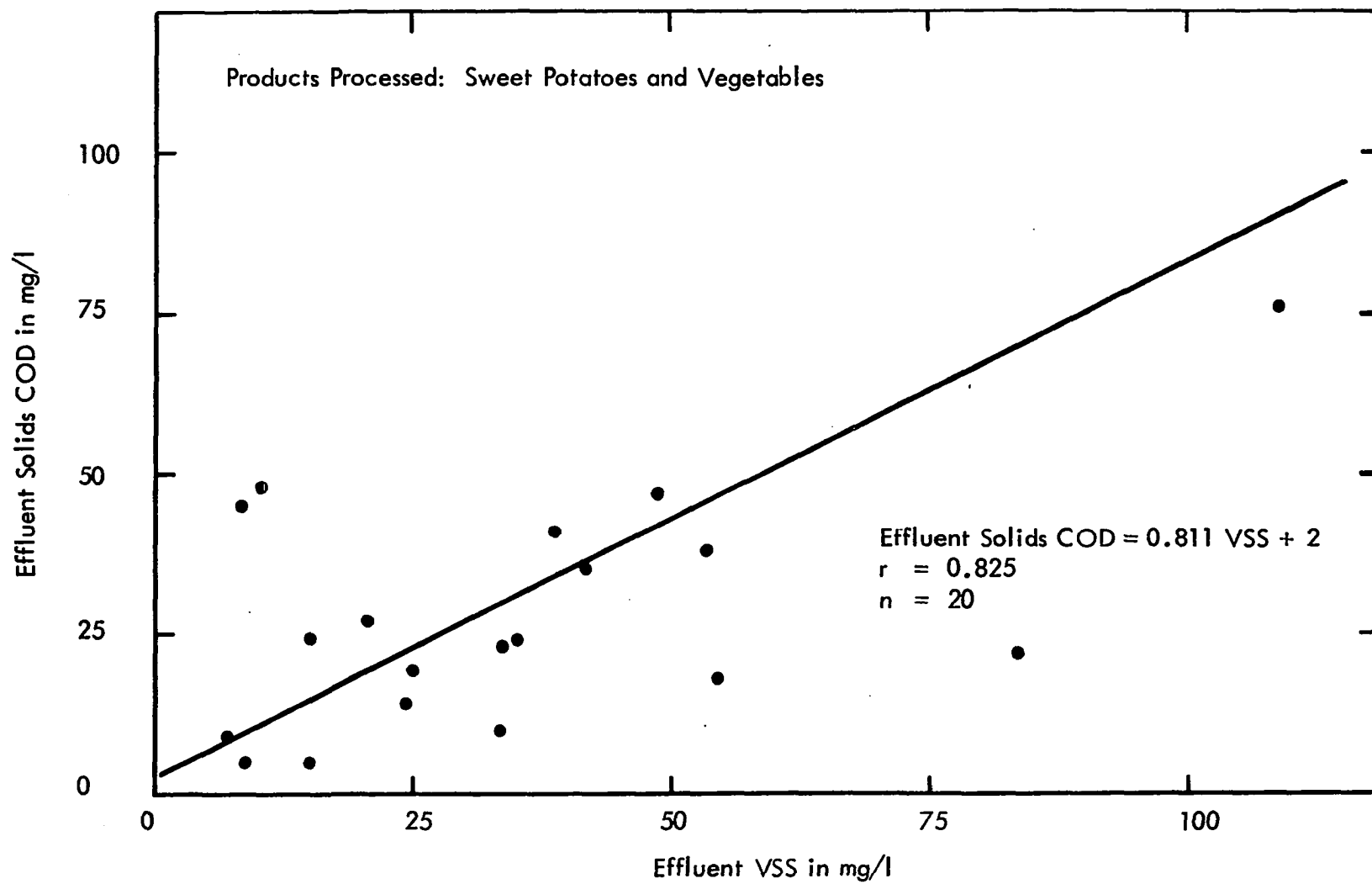
Figure 76 Effluent Solids COD vs VSS
