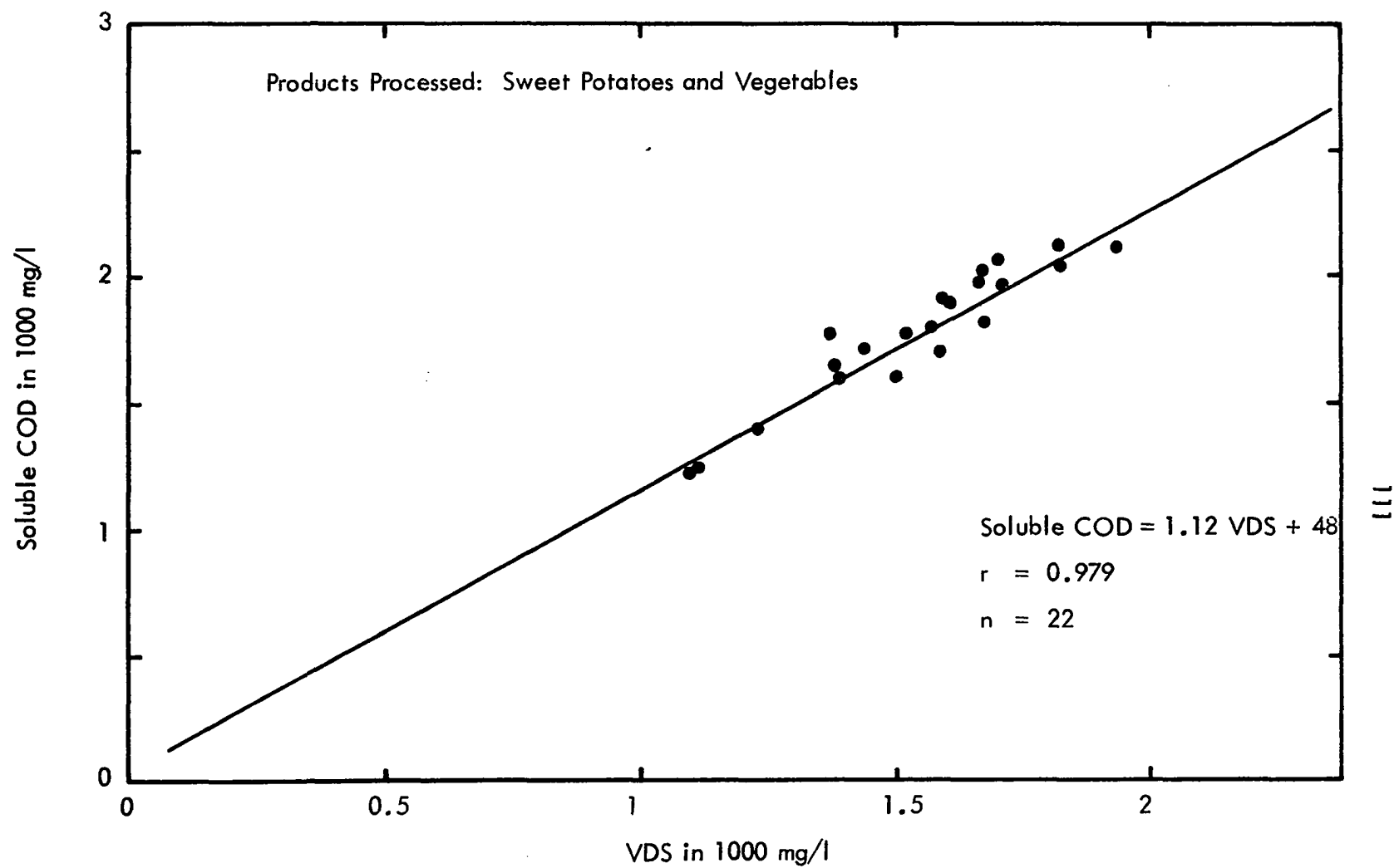
Figure 40 Plant Influent Soluble COD vs VDS
