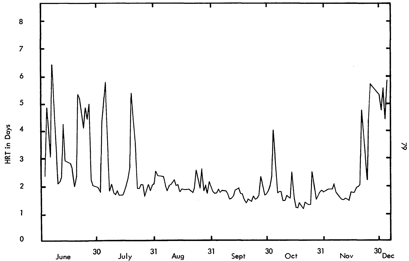
Figure 33 HRT of Extended Aeration Unit
