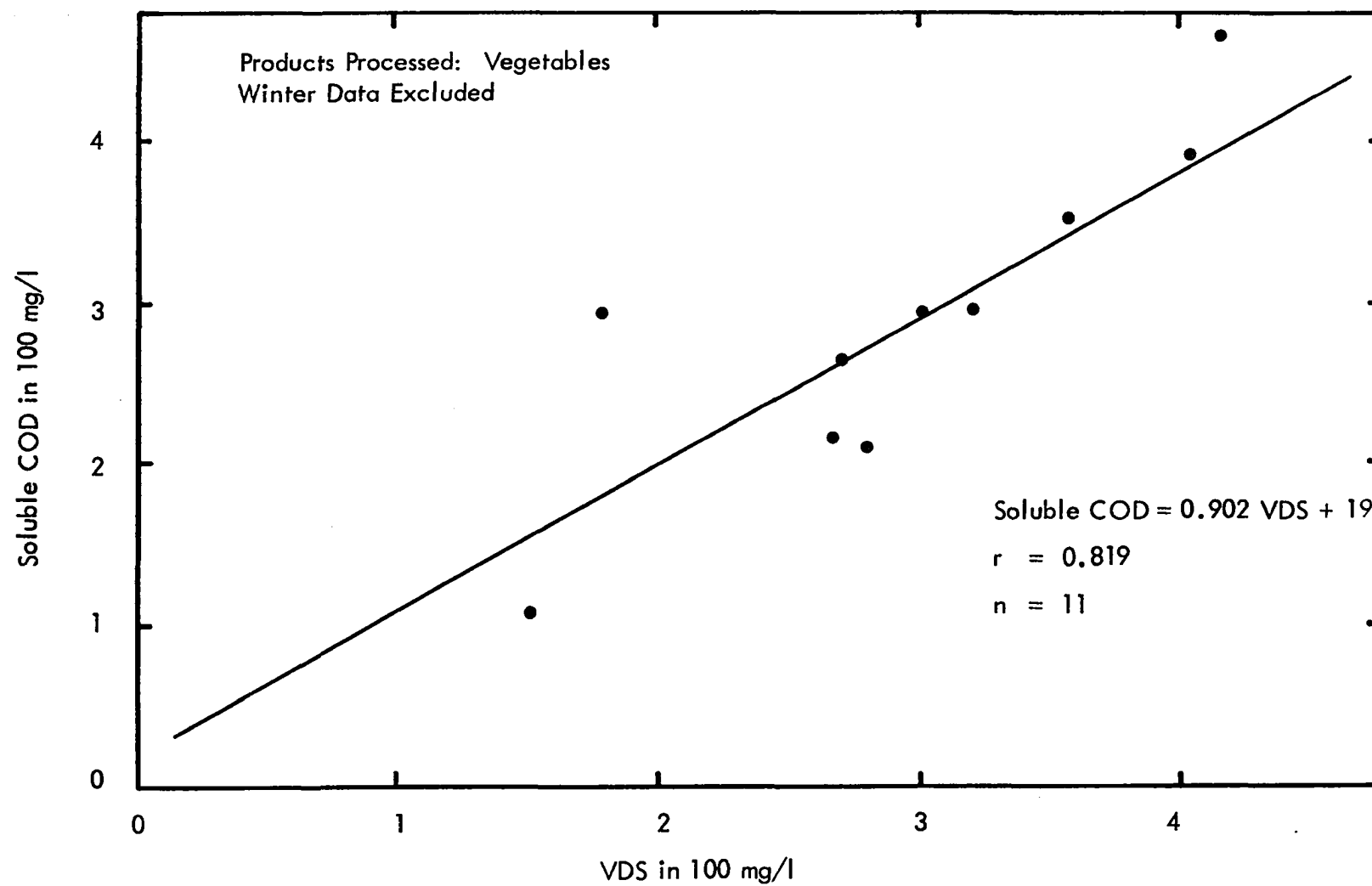
Figure 55 Plant Influent Soluble COD vs VDS
