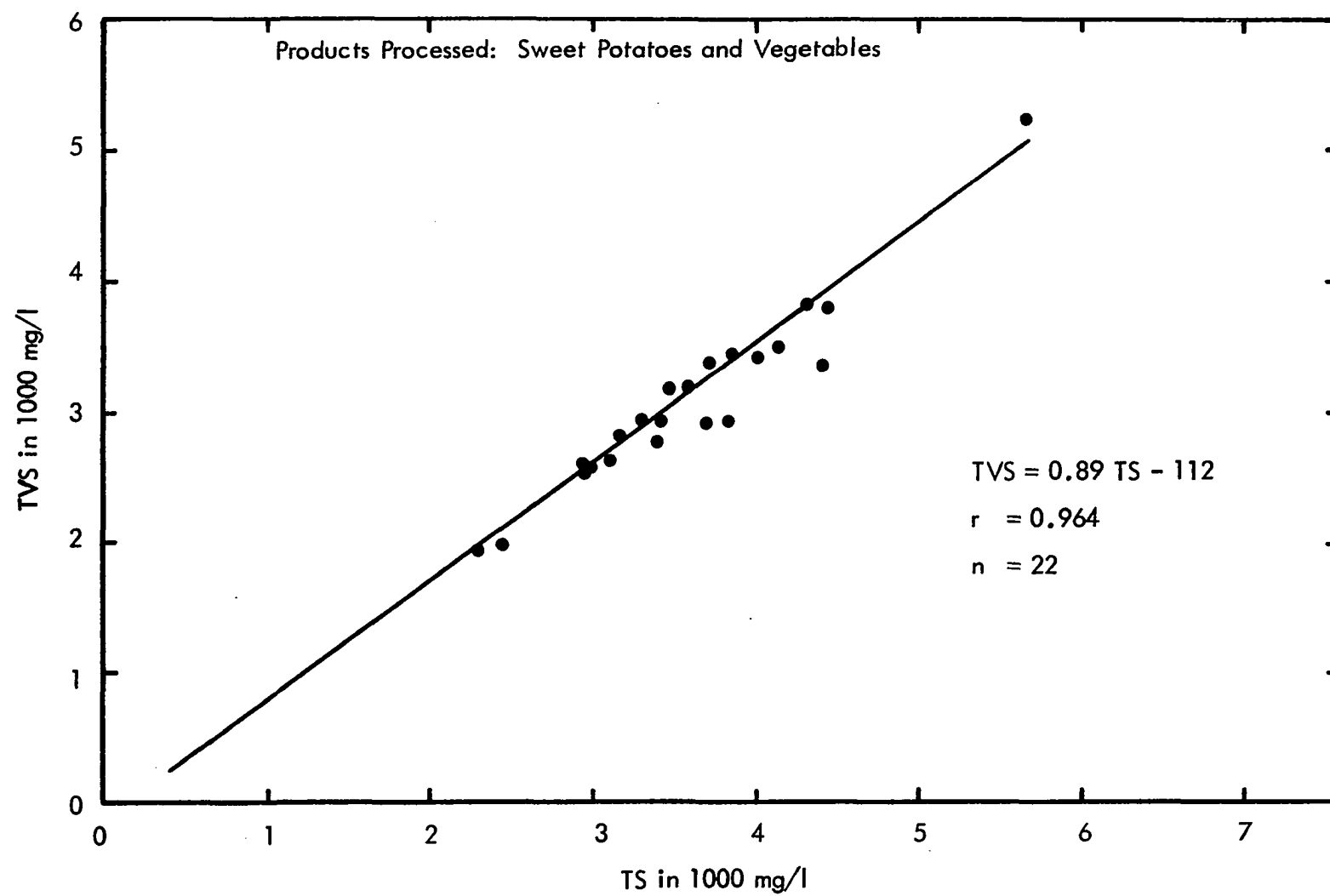
Figure 38 Plant Influent TVS vs TS
