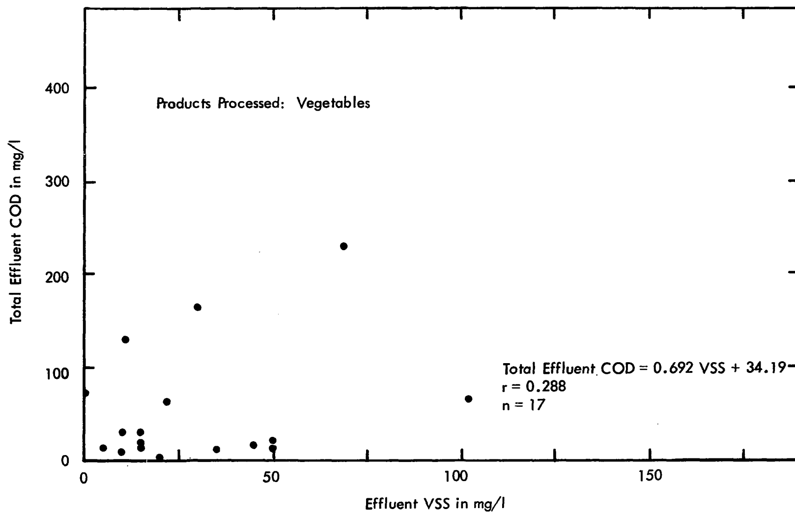
Figure 81 Plant Total Effluent COD vs VSS
