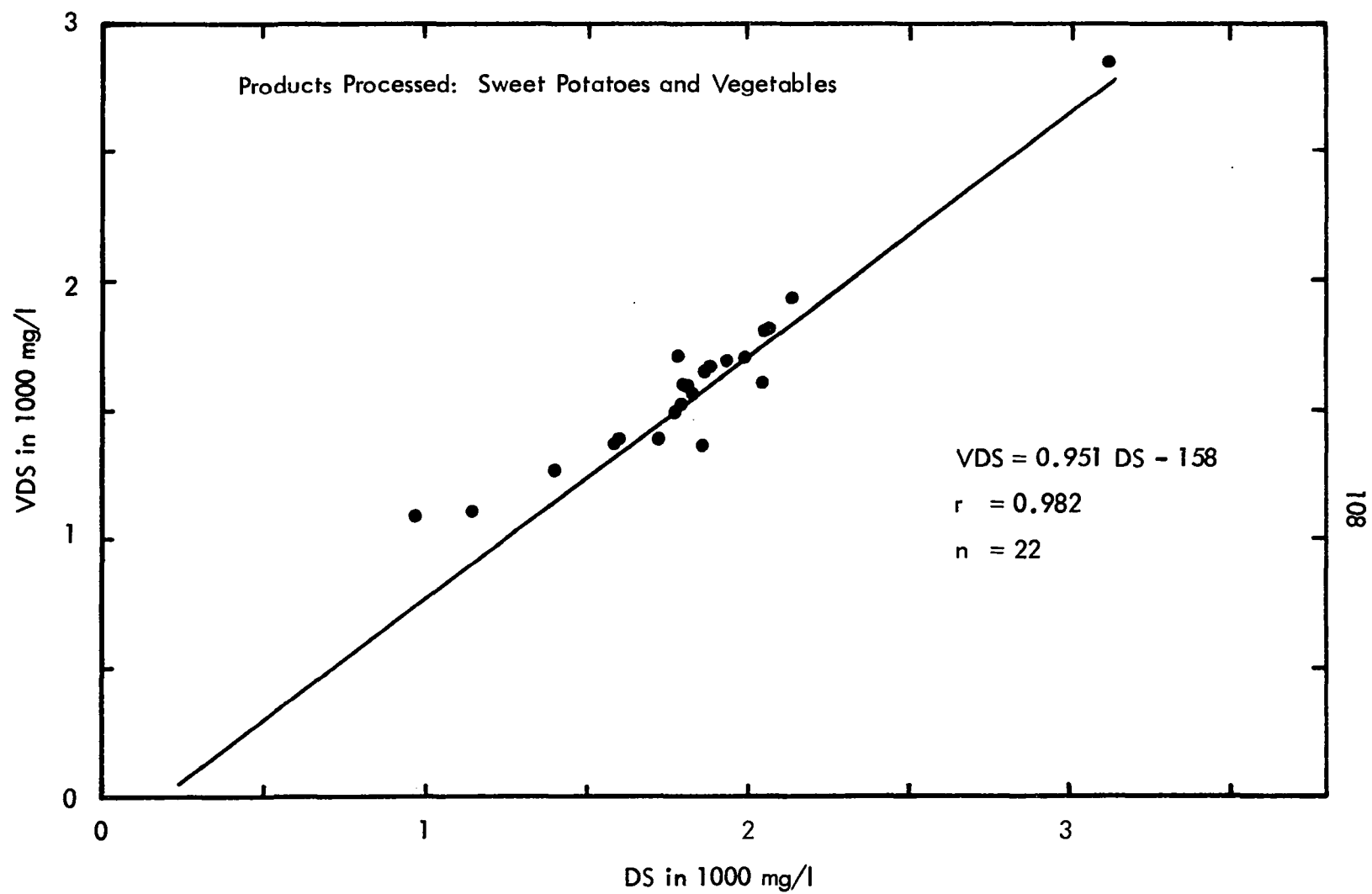
Figure 37 Plant Influent VDS vs DS
