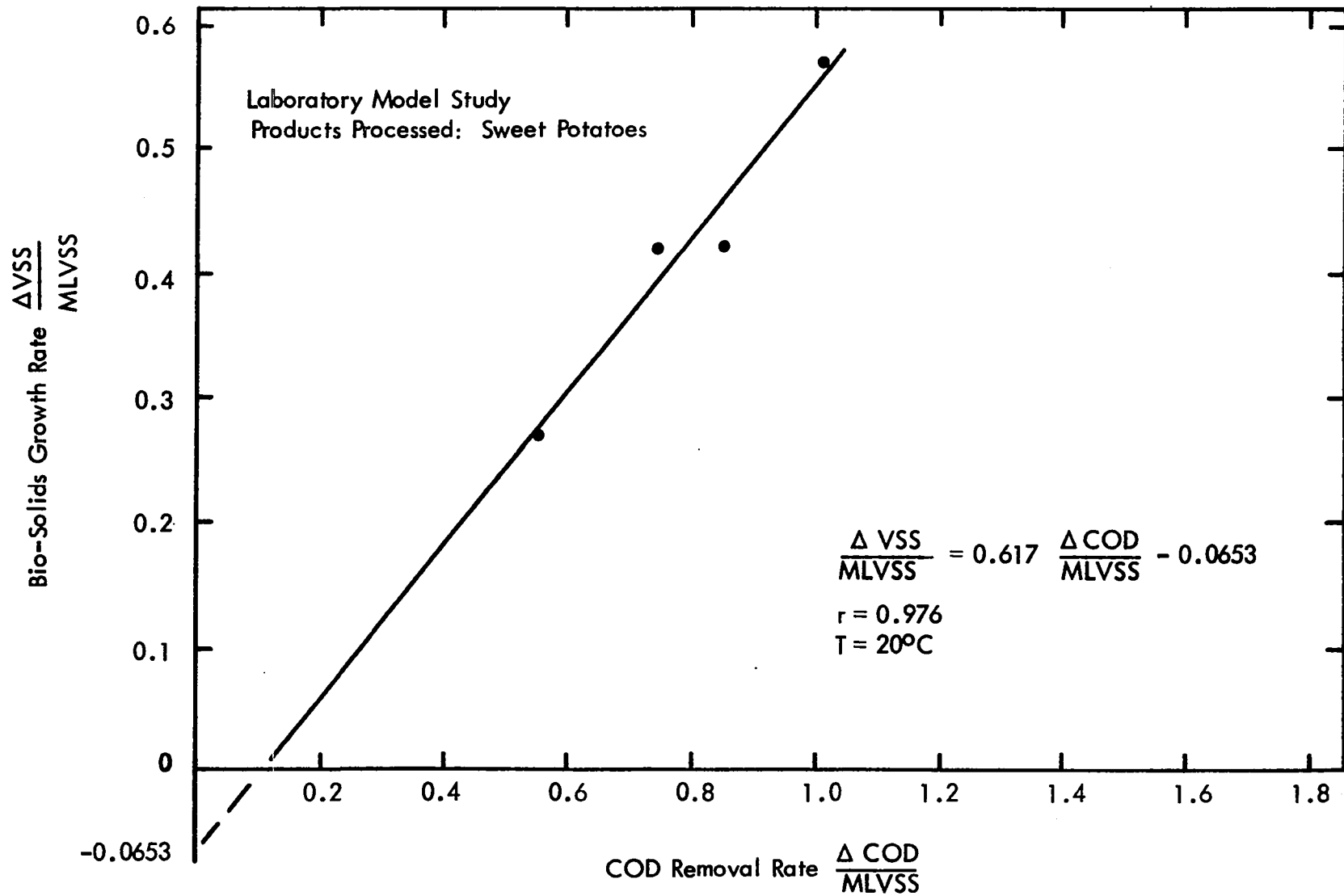
Figure 84 Bio-Solids Growth Rate vs COD Removal Rate
