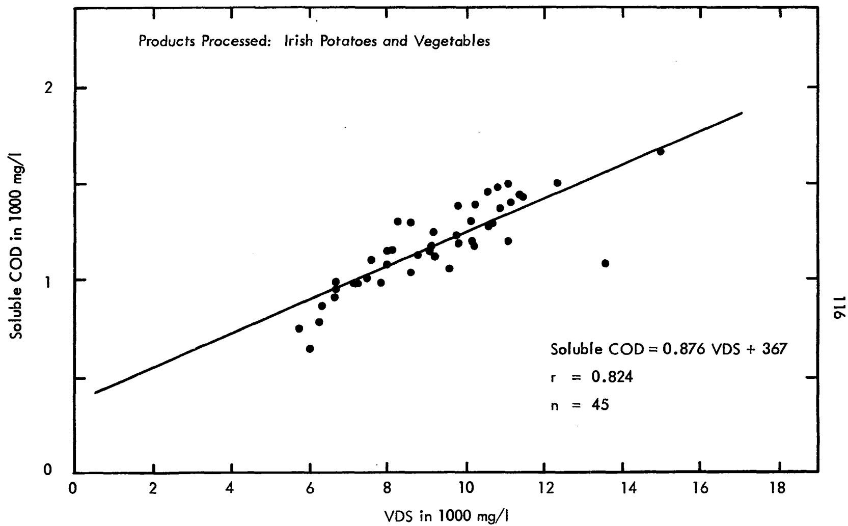
Figure 45 Plant Influent Total COD vs VDS
