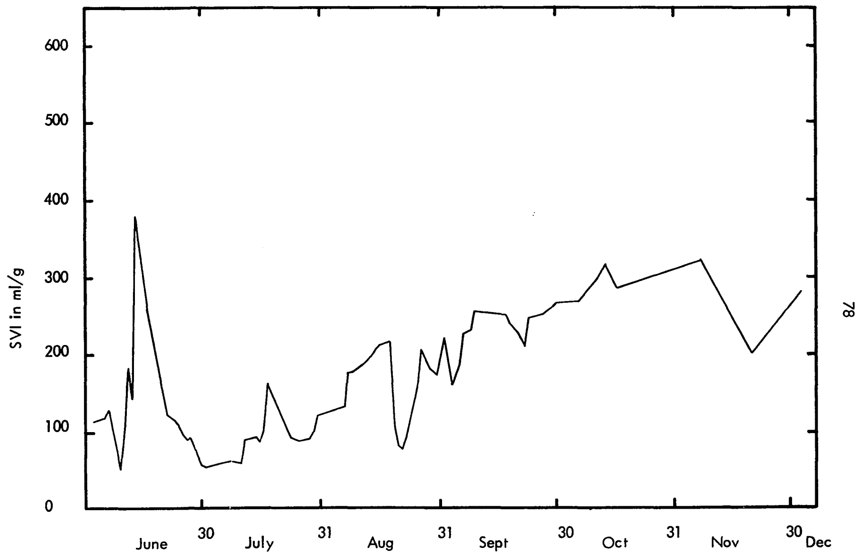
Figure 32 SVI of Extended Aeration Unit
