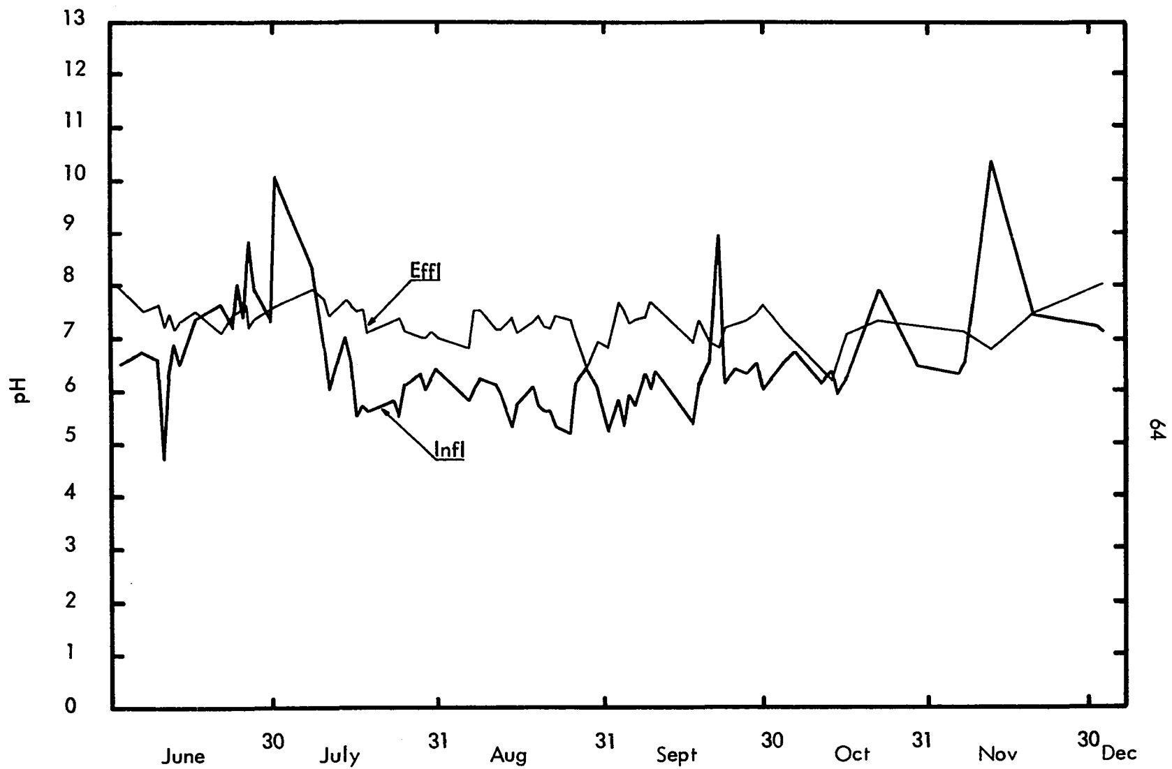
Figure 18 Treatment Plant Performance - pH
