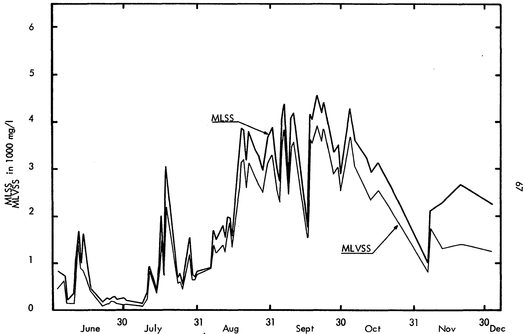
Figure 21 MLSS and MLVSS of Minimal Solids (High Loading) Unit
