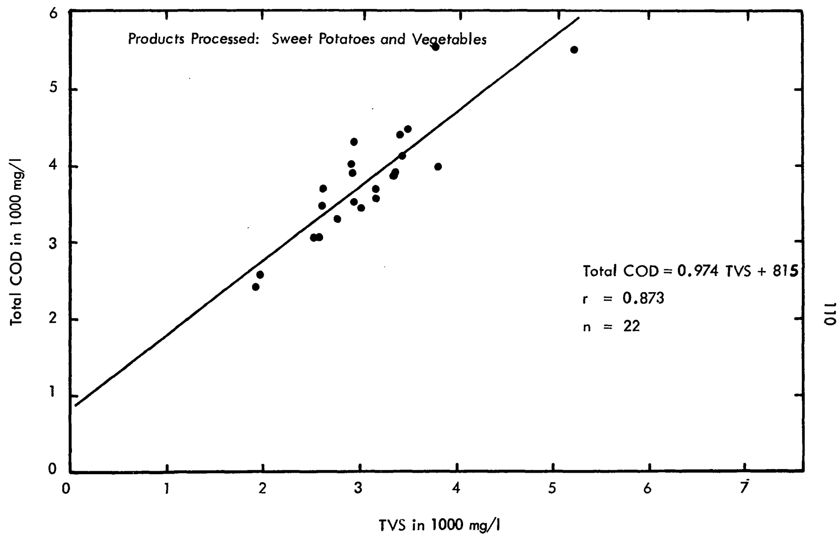
Figure 39 Plant Influent Total COD vs TVS
