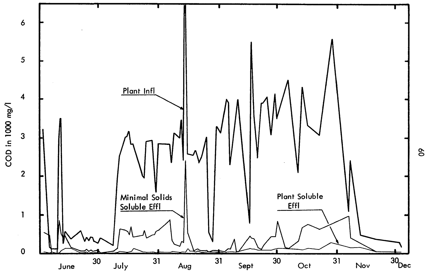
Figure 14 Treatment Plant Performance - COD
