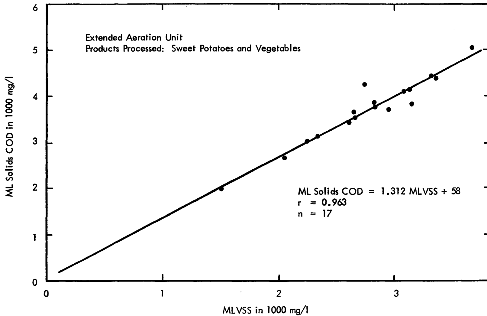
Figure 69 ML Solids COD vs MLVSS
