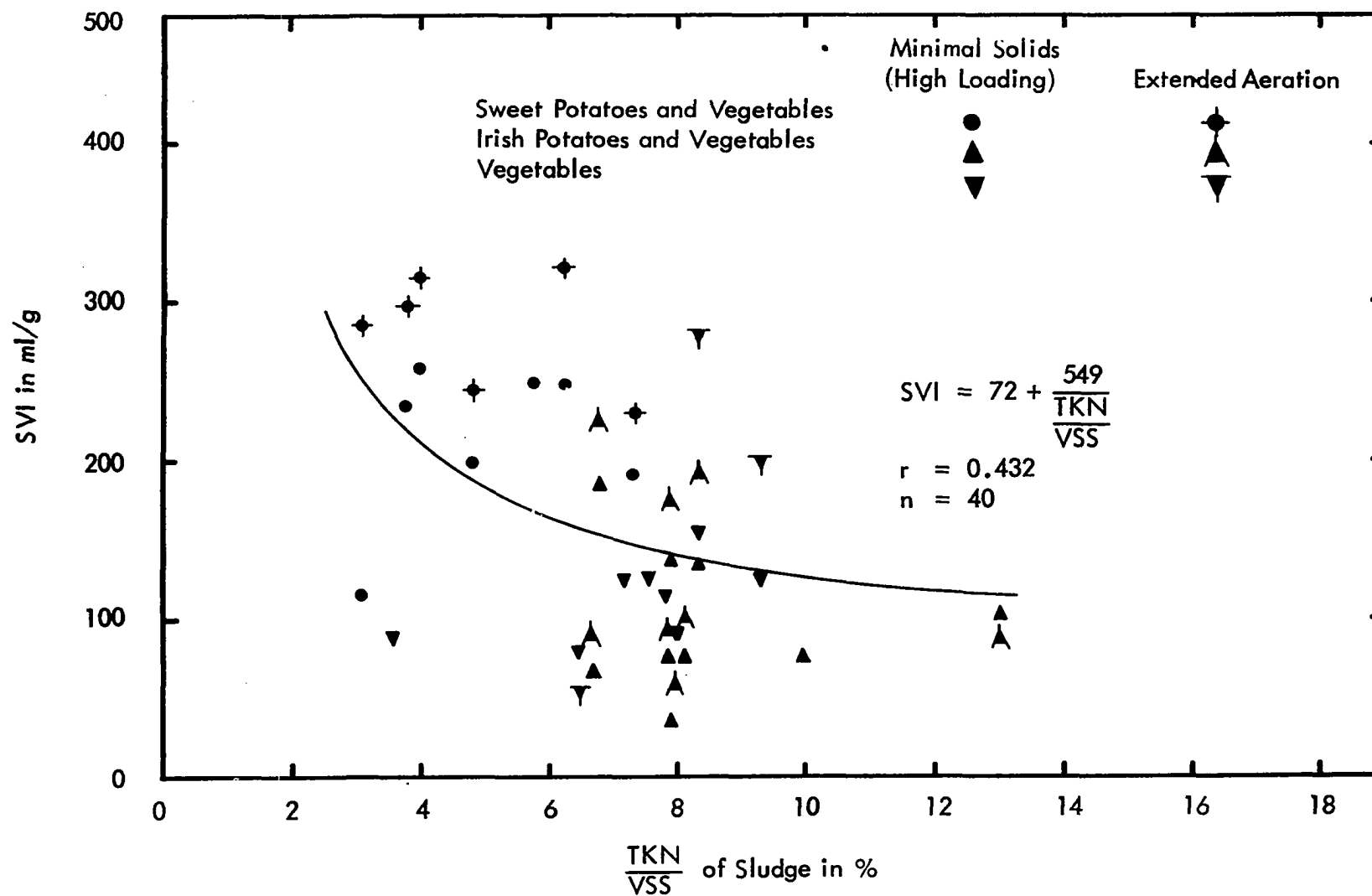
Figure 89 SVI vs \frac{TKN}{VSS} of Sludge
