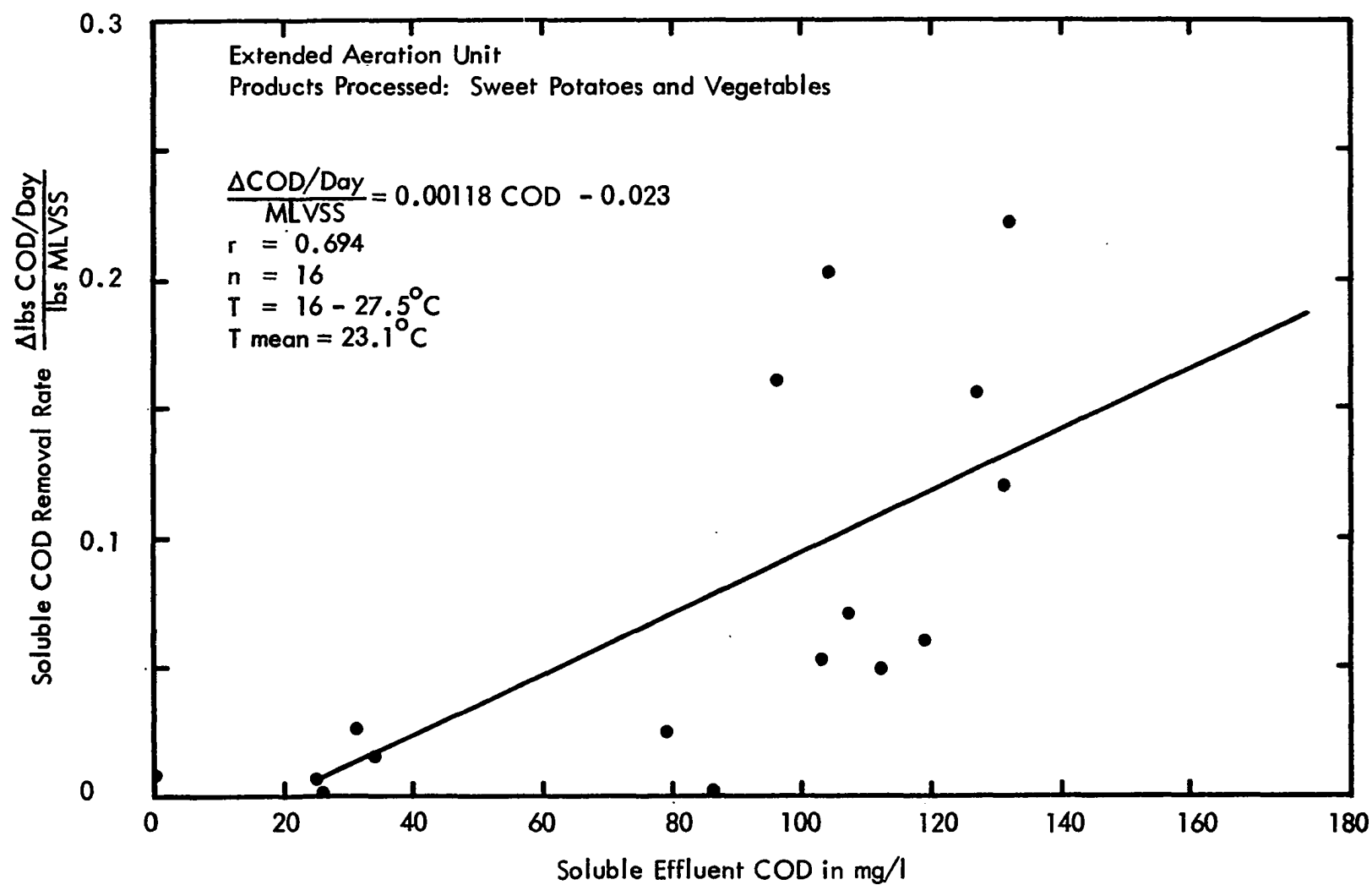
Figure 65 Soluble COD Removal Rate vs Soluble Effluent COD
