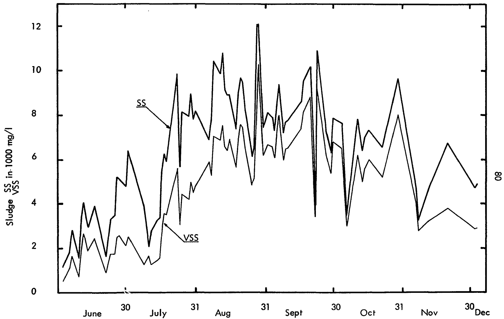
Figure 34 SS and VSS of Sludge
