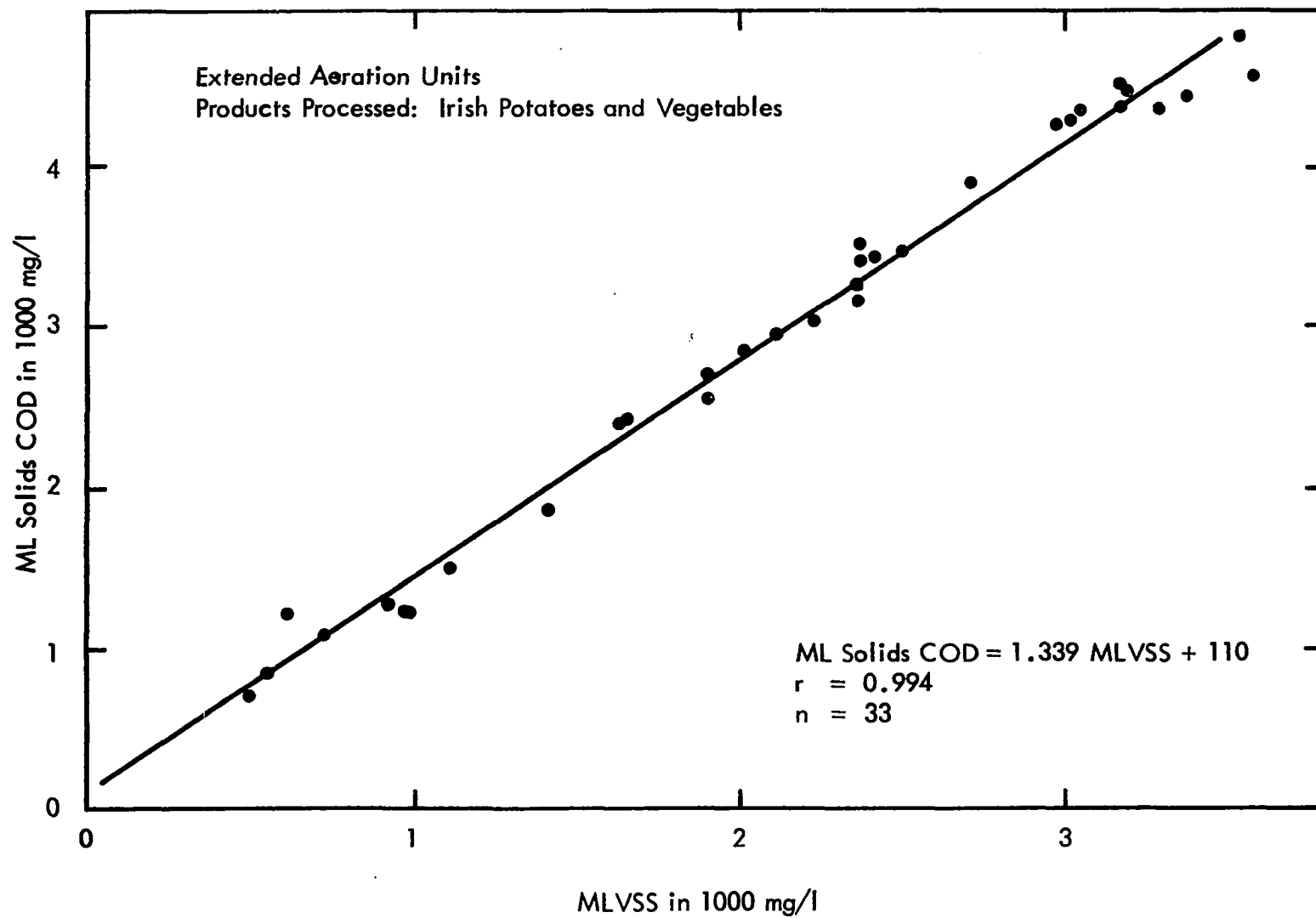
Figure 71 ML Solids COD vs MLSS
