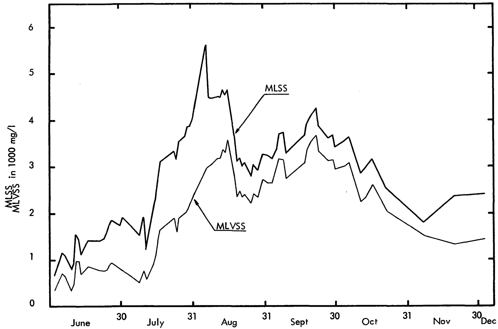
Figure 27 MLSS and MLVSS of Extended Aeration Unit
