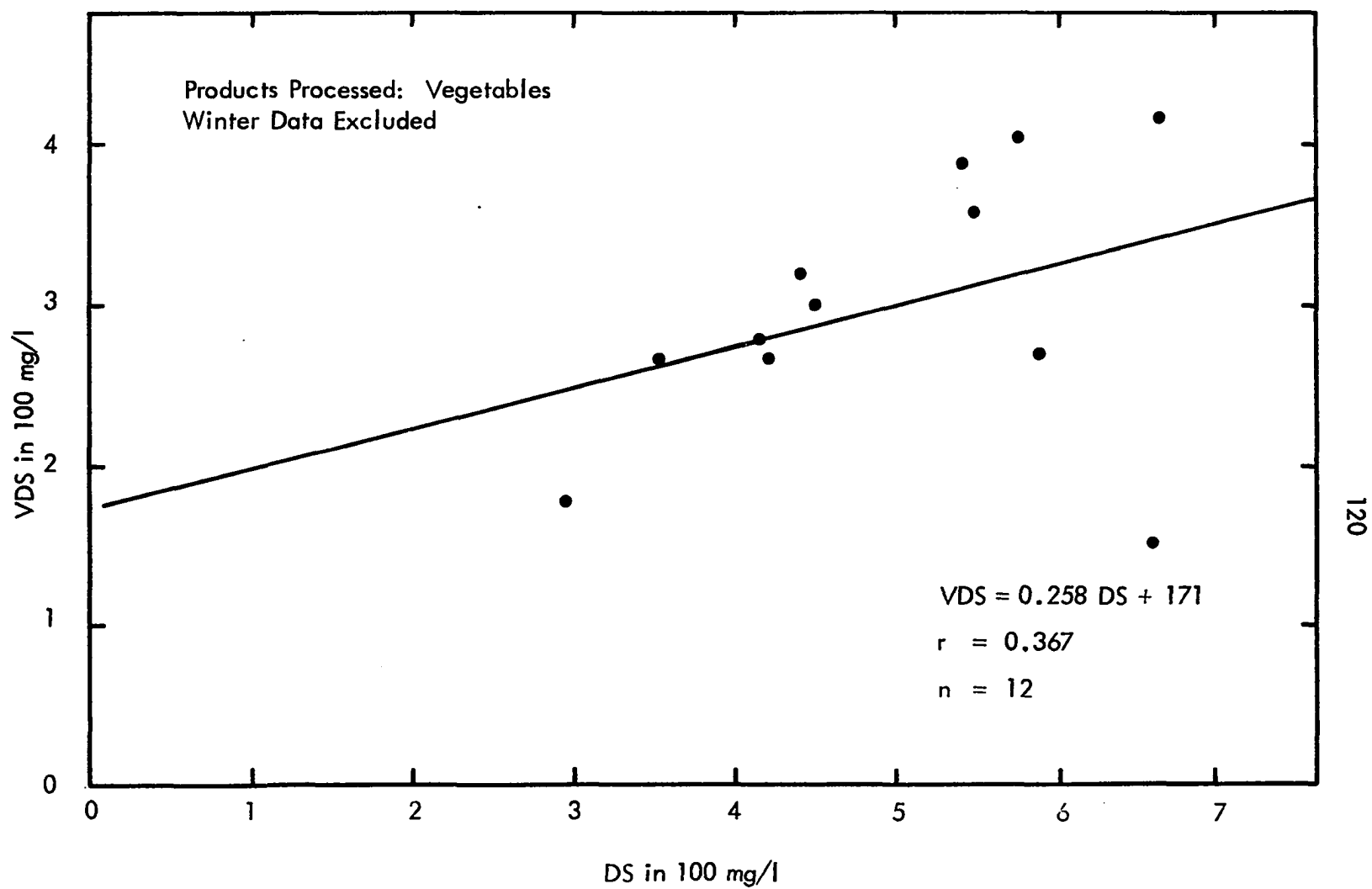
Figure 49 Plant Influent VDS vs DS
