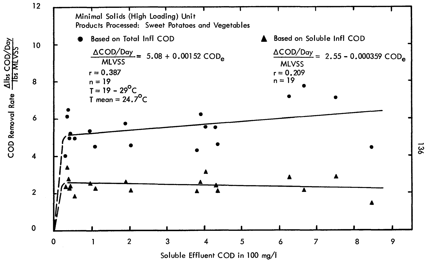
Figure 56 COD Removal Rate vs Soluble Effluent COD
