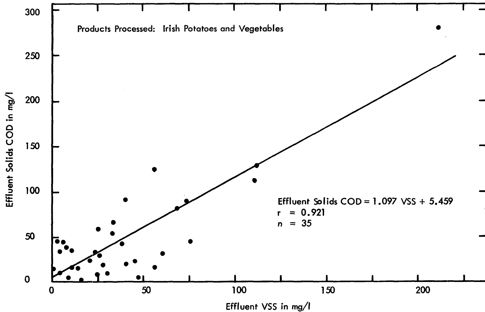
Figure 79 Effluent Solids COD vs VSS
