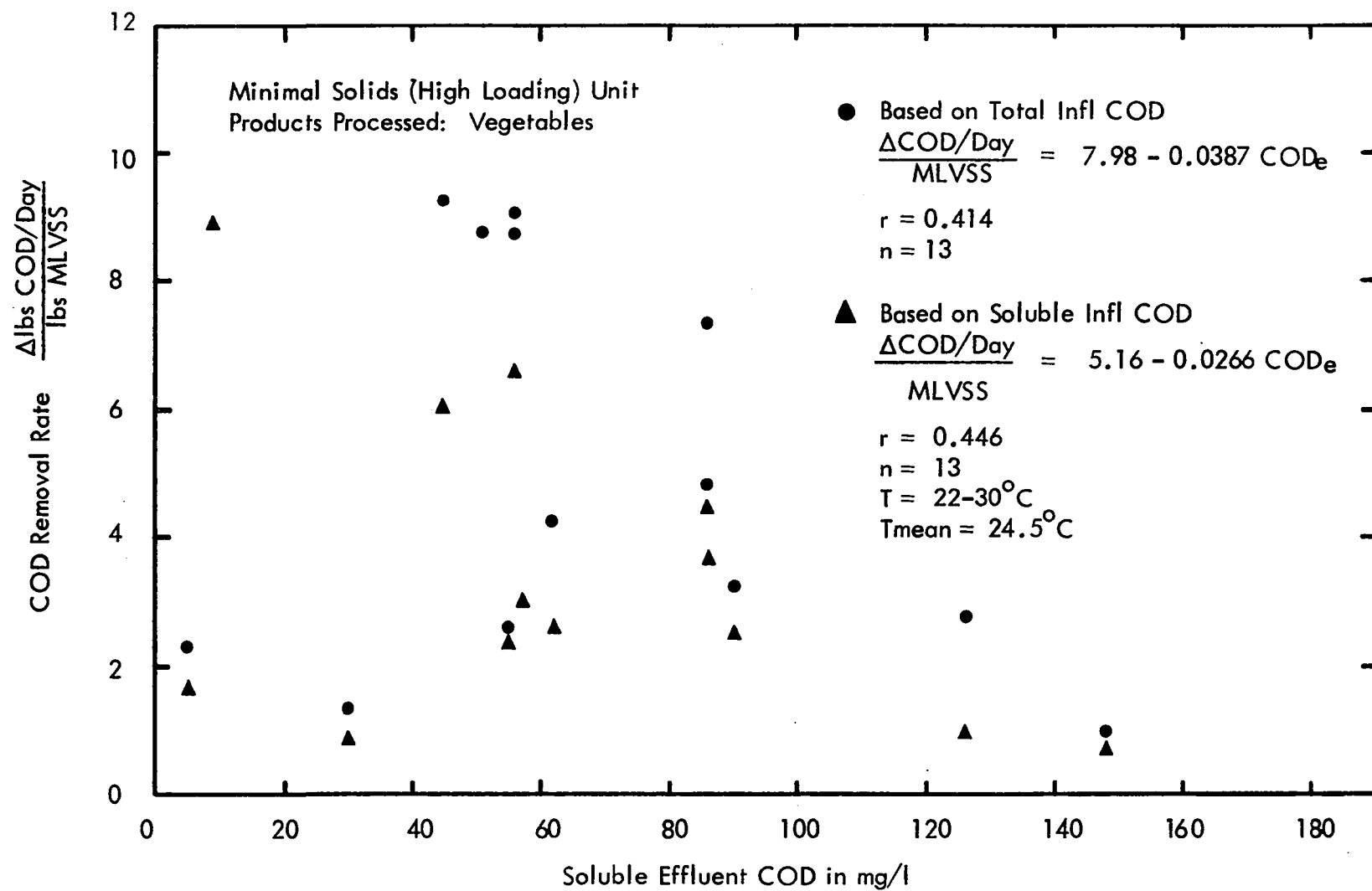
Figure 58 COD Removal Rate vs Soluble Effluent COD
