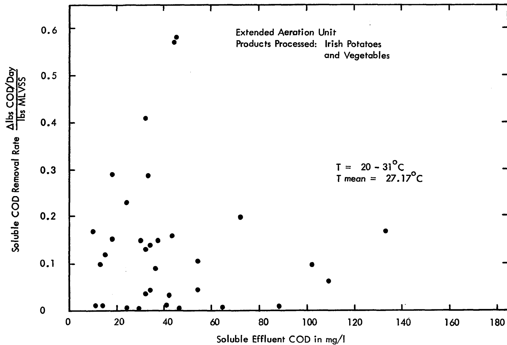
Figure 66 Soluble COD Removal Rate vs Soluble Effluent COD
