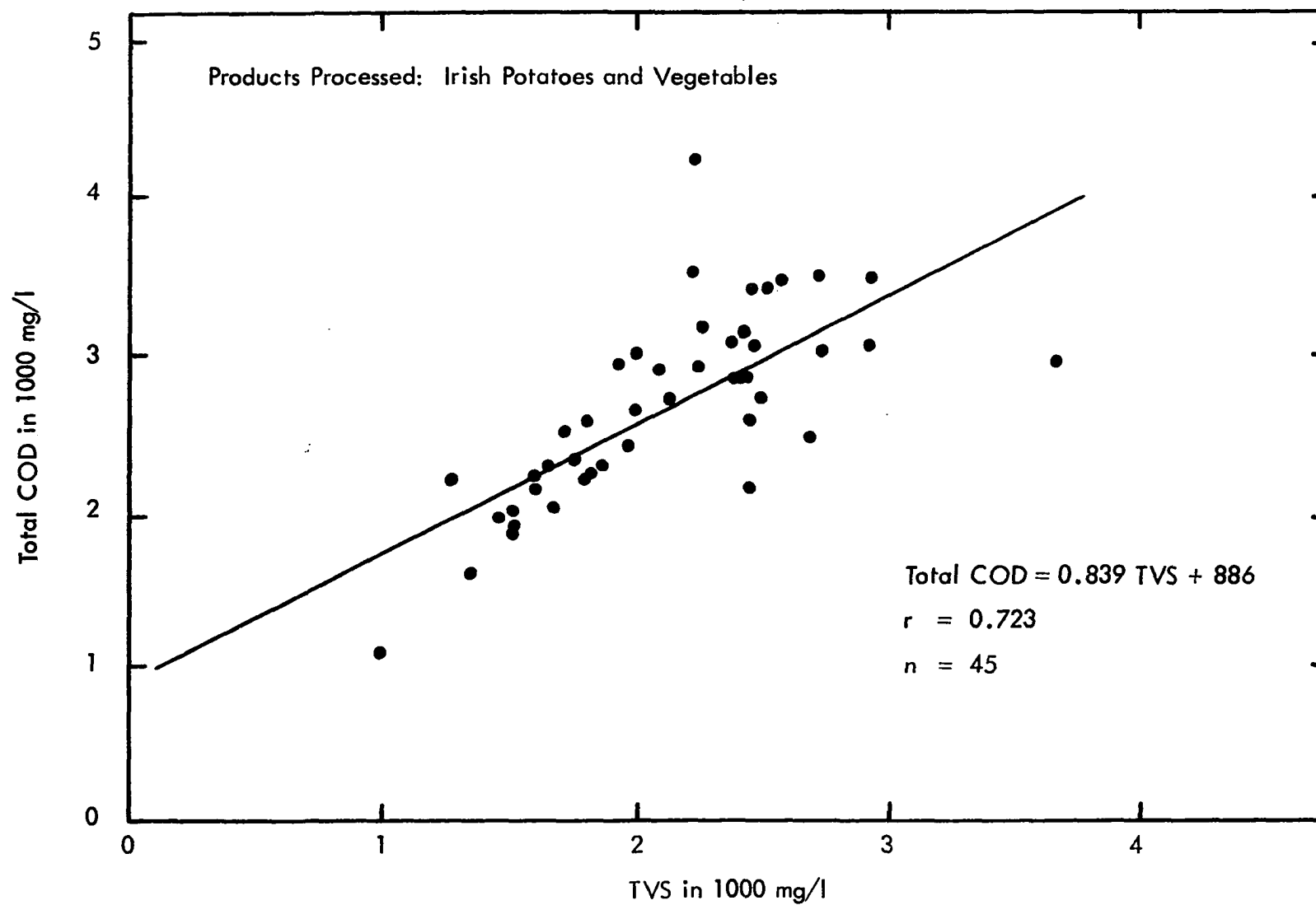
Figure 44 Plant Influent Total COD vs TVS
