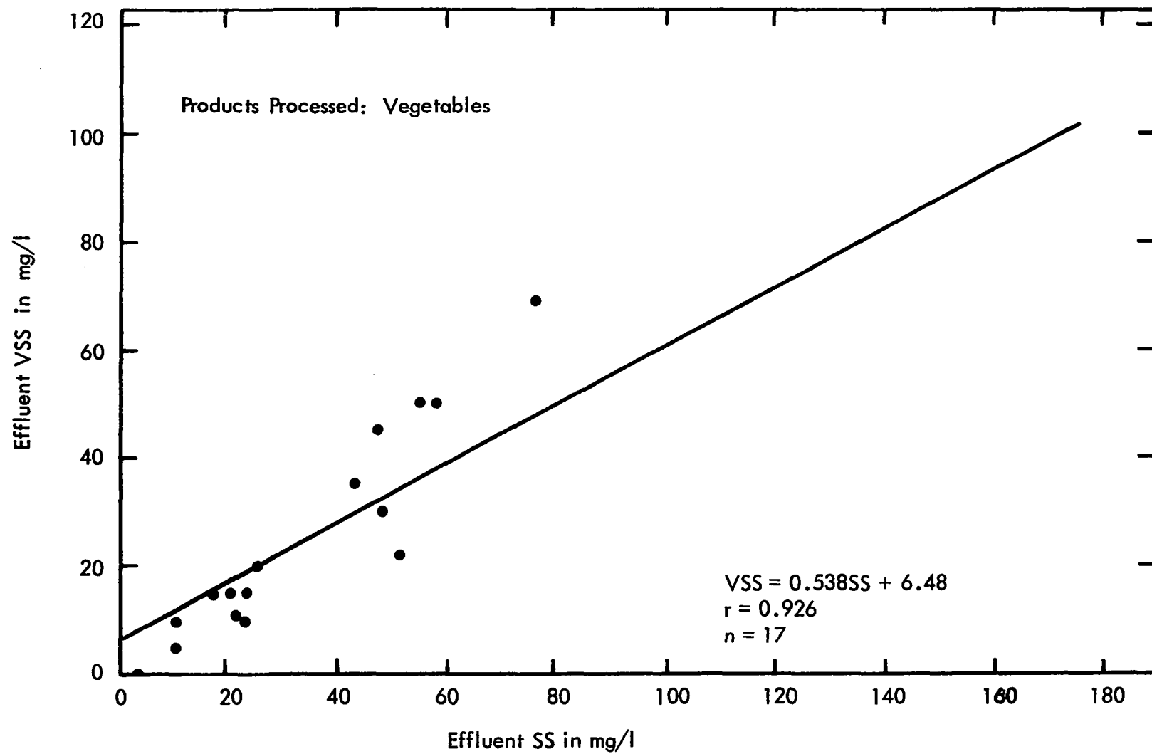
Figure 80 Plant Effluent VSS vs SS
