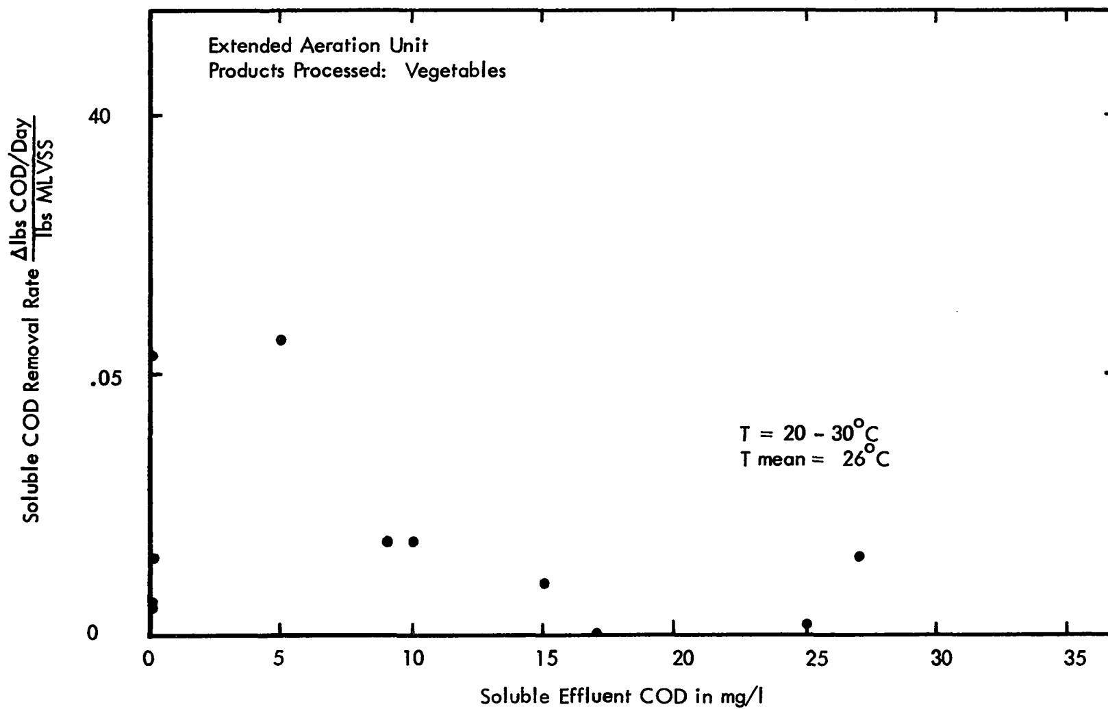
Figure 67 Soluble COD Removal Rate vs Soluble Effluent COD
