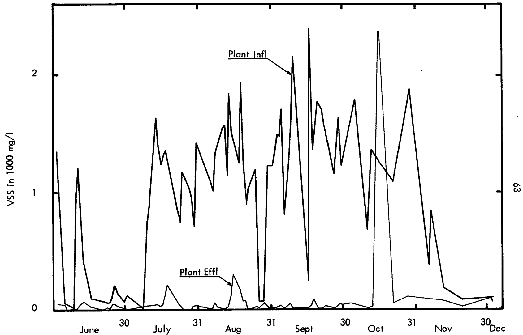
Figure 17 Treatment Plant Performance - VSS
