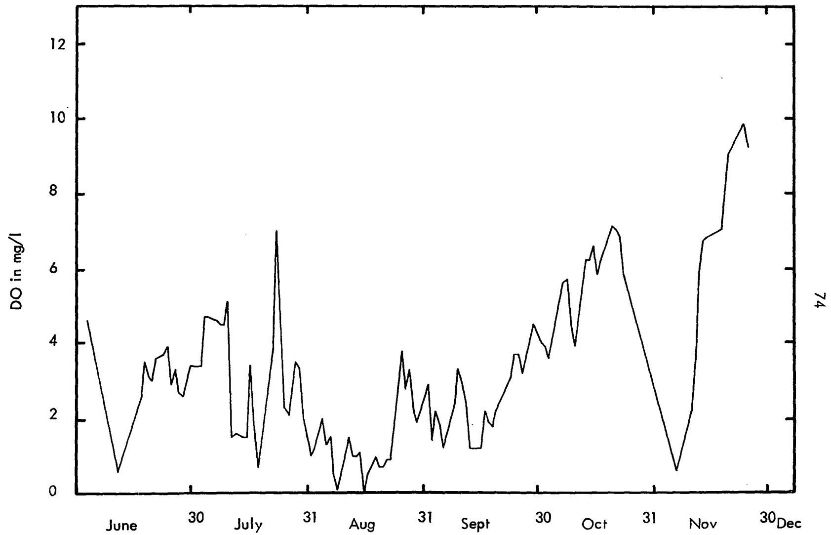
Figure 28 DO in Extended Aeration Unit
