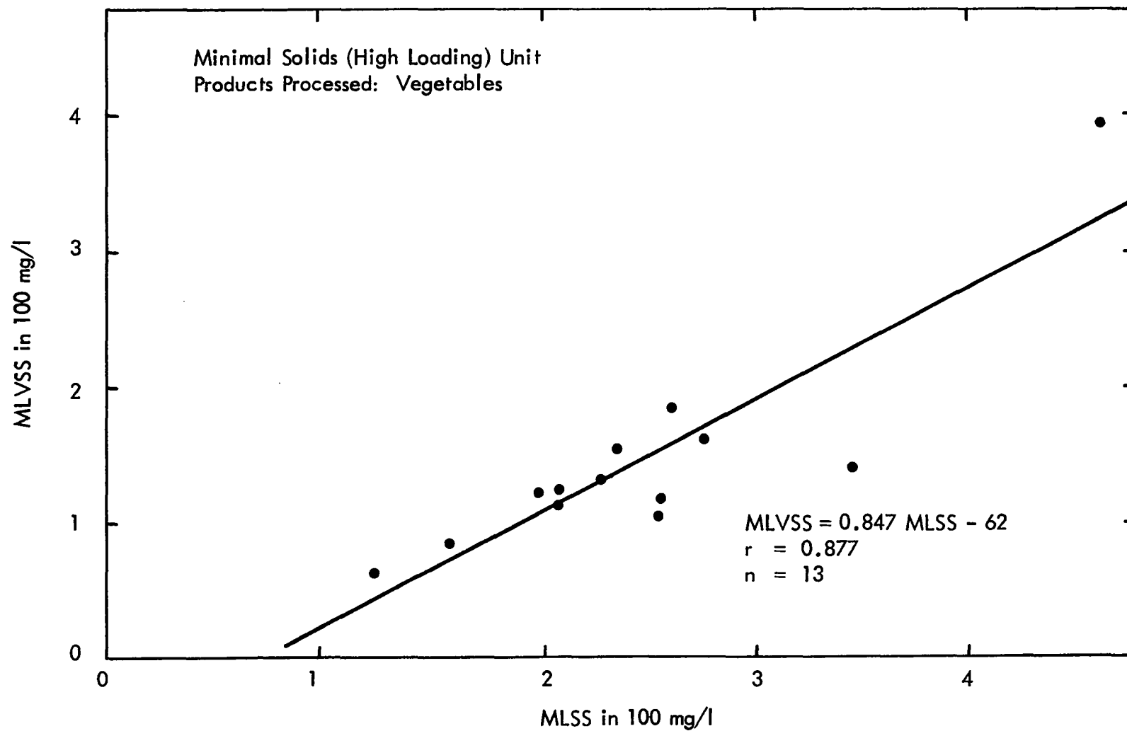
Figure 63 MLVSS vs MLSS
