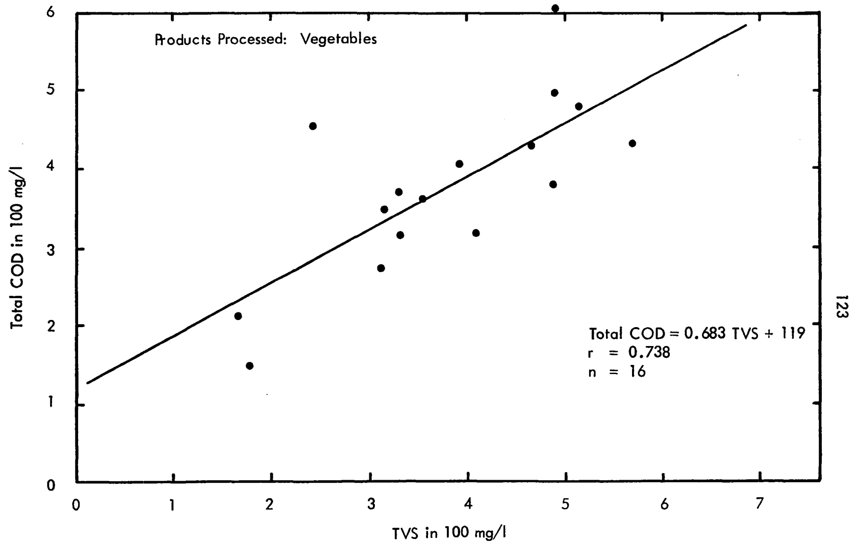
Figure 52 Plant Influent Total COD vs TVS
