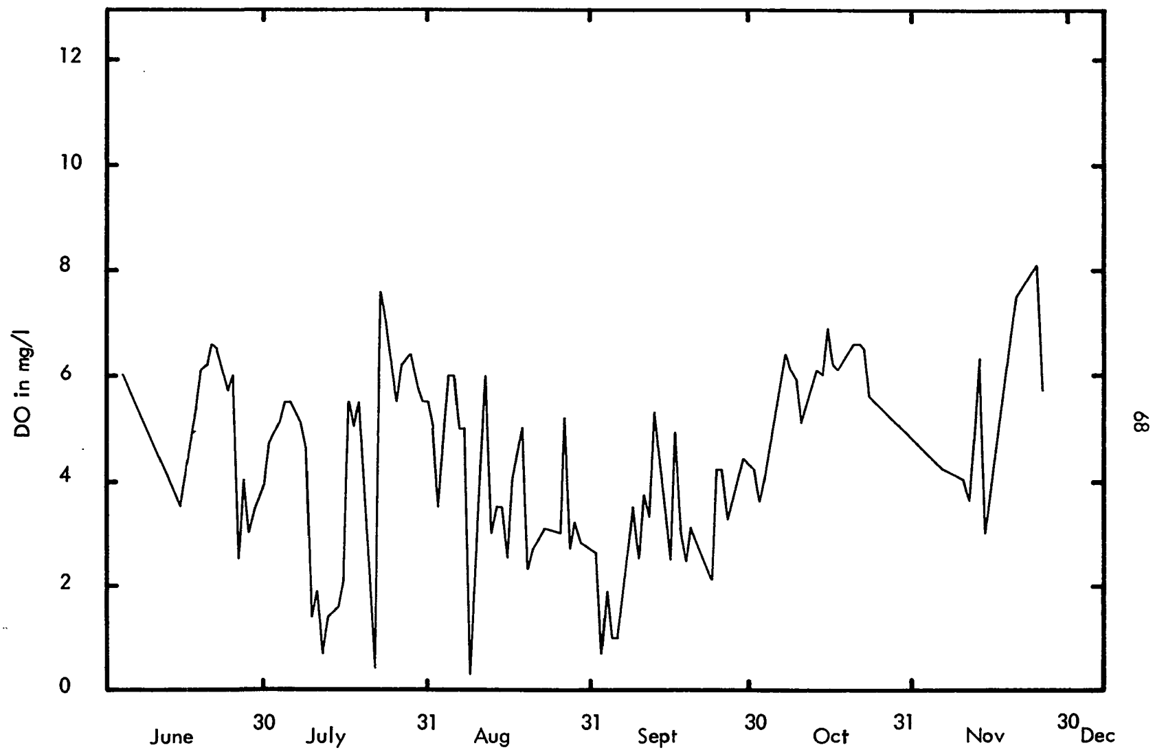
Figure 22 DO in Minimal Solids (High Loading) Unit
