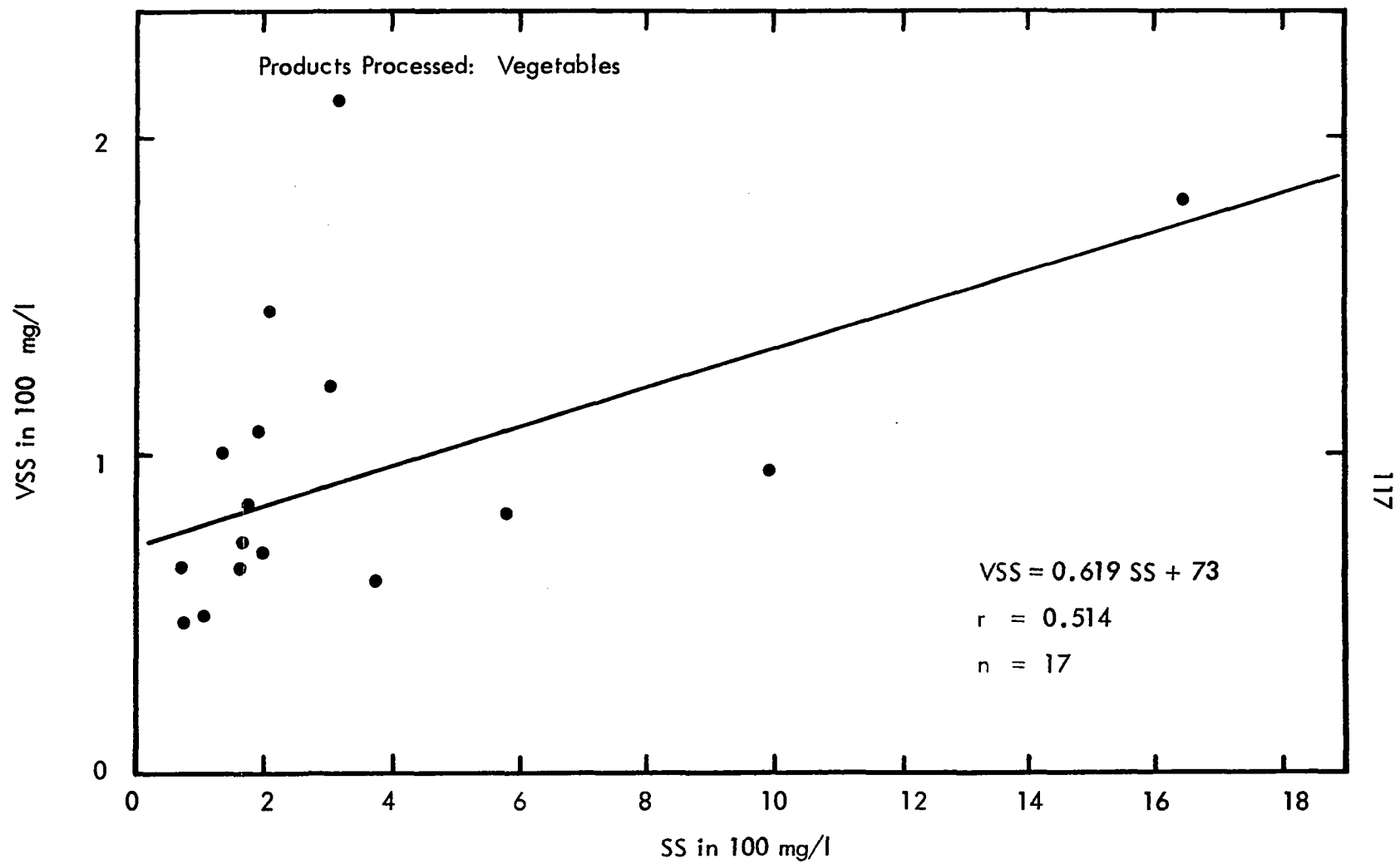
Figure 46 Plant Influent VSS vs SS
