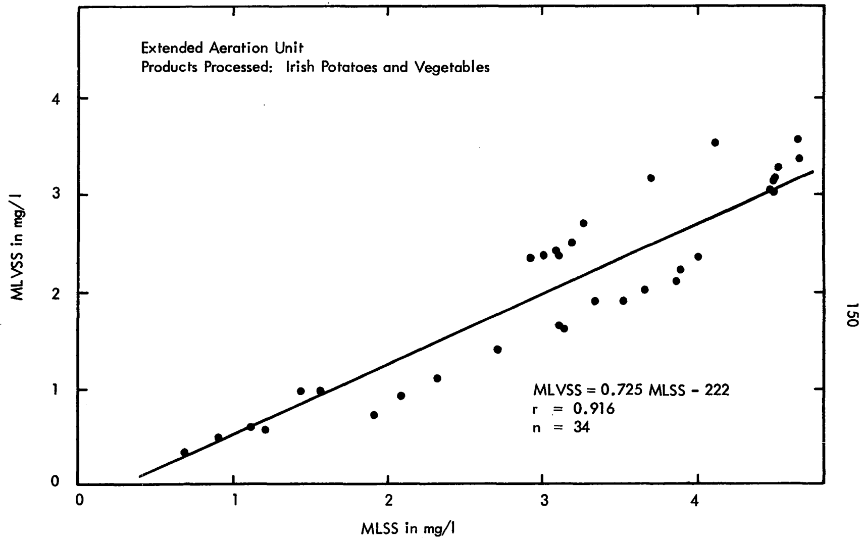
Figure 70 MLVSS vs MLSS
