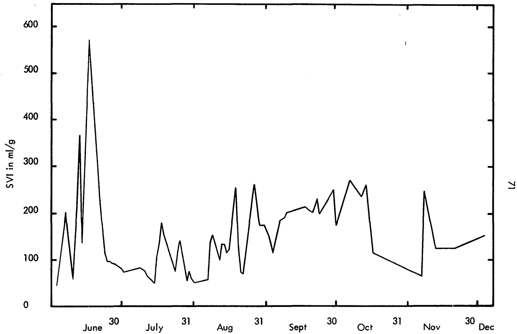
Figure 25 SVI of Minimal Solids (High Loading) Unit
