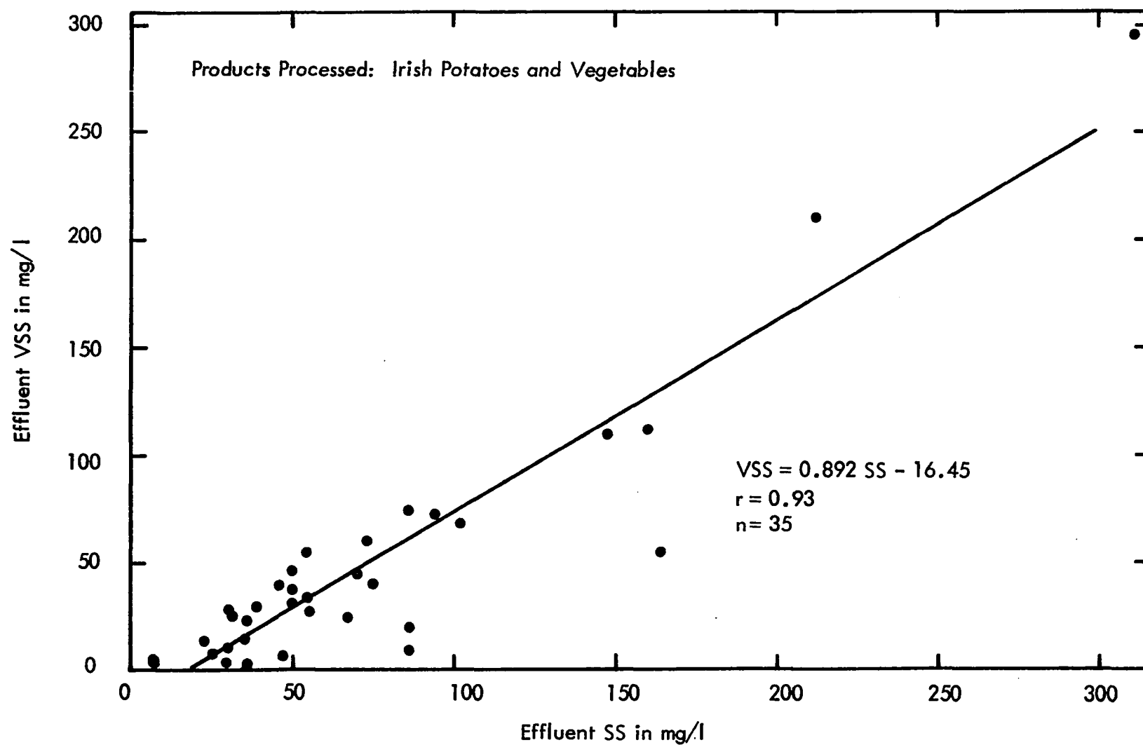
Figure 77 Plant Effluent VSS vs SS
