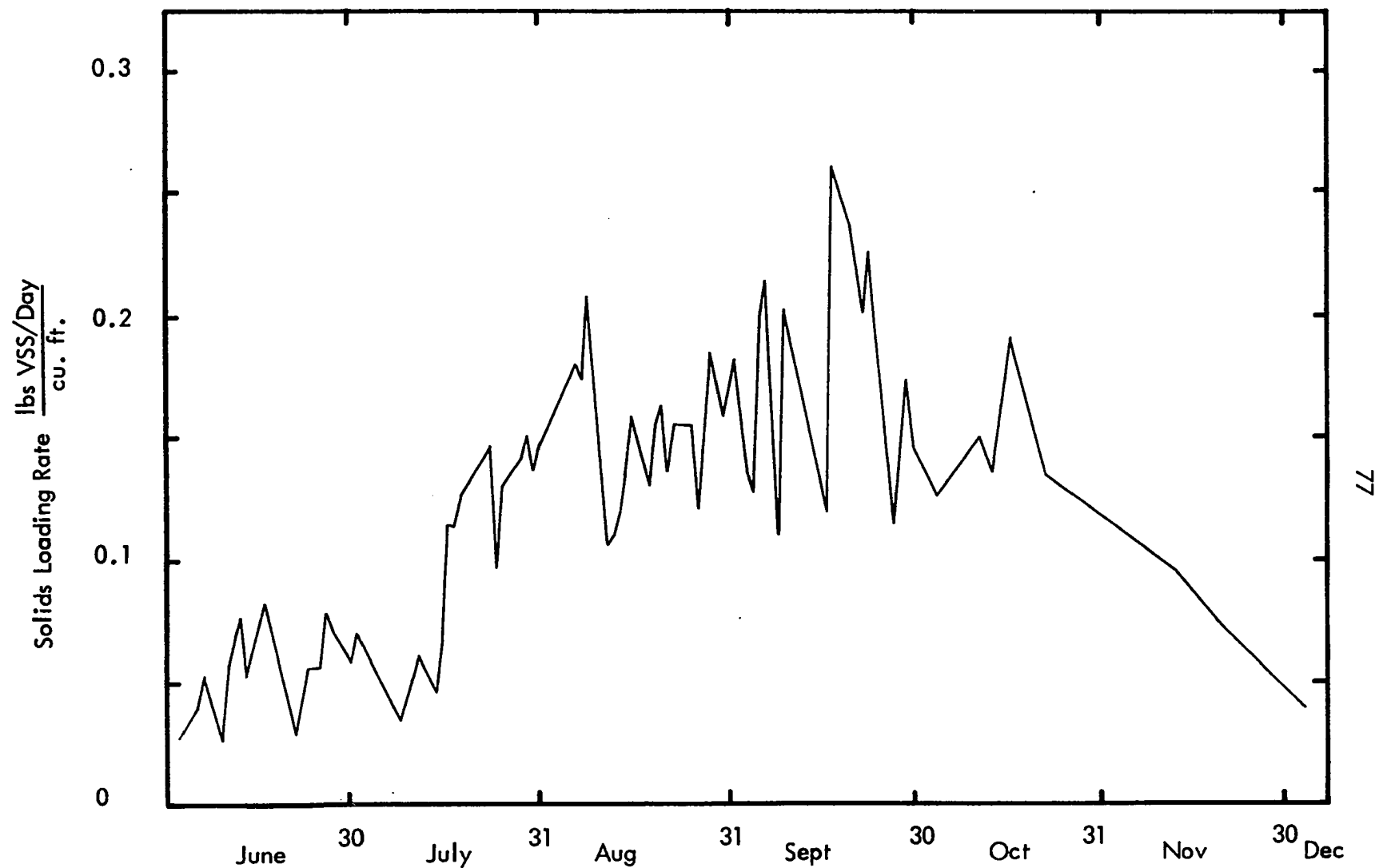
Figure 31 Solids Loading Rate of Extended Aeration Unit
