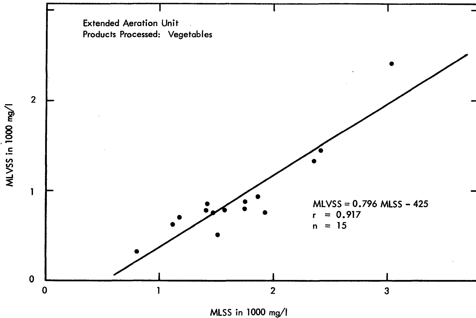
Figure 72 MLVSS vs MLSS
