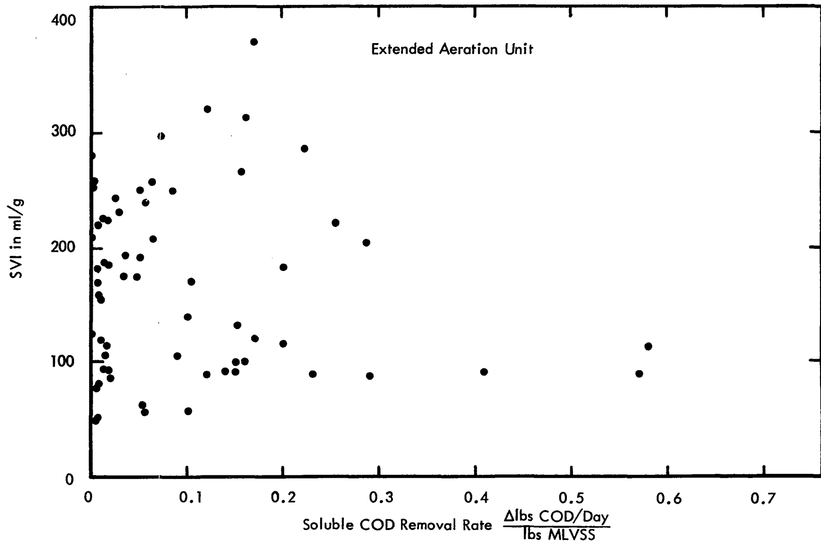
Figure 86 SVI vs Soluble COD Removal Rate
