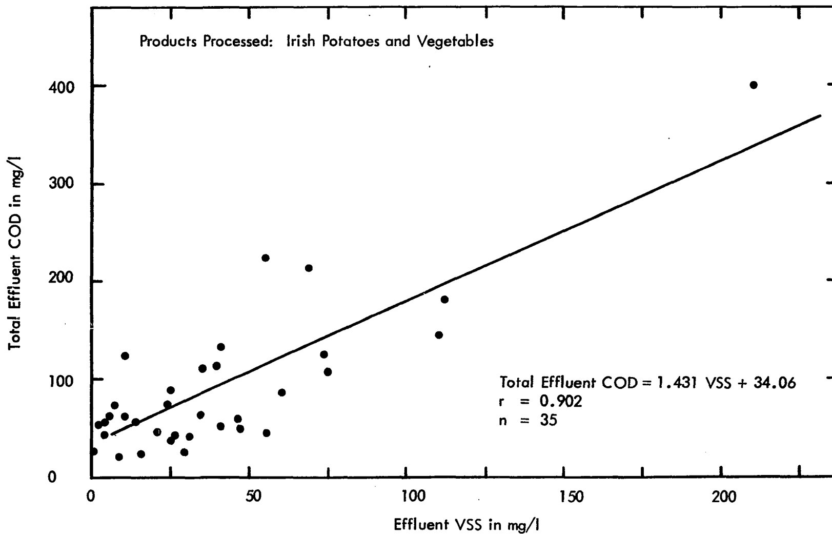
Figure 78 Total Effluent COD vs VSS
