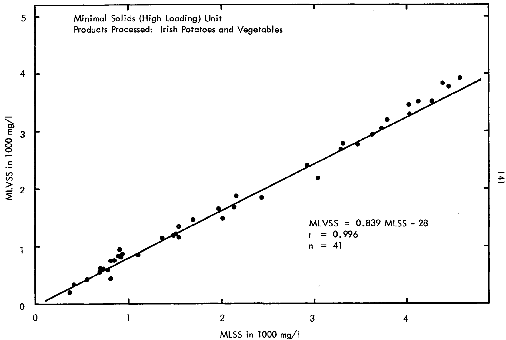
Figure 61 MLVSS vs MLSS
