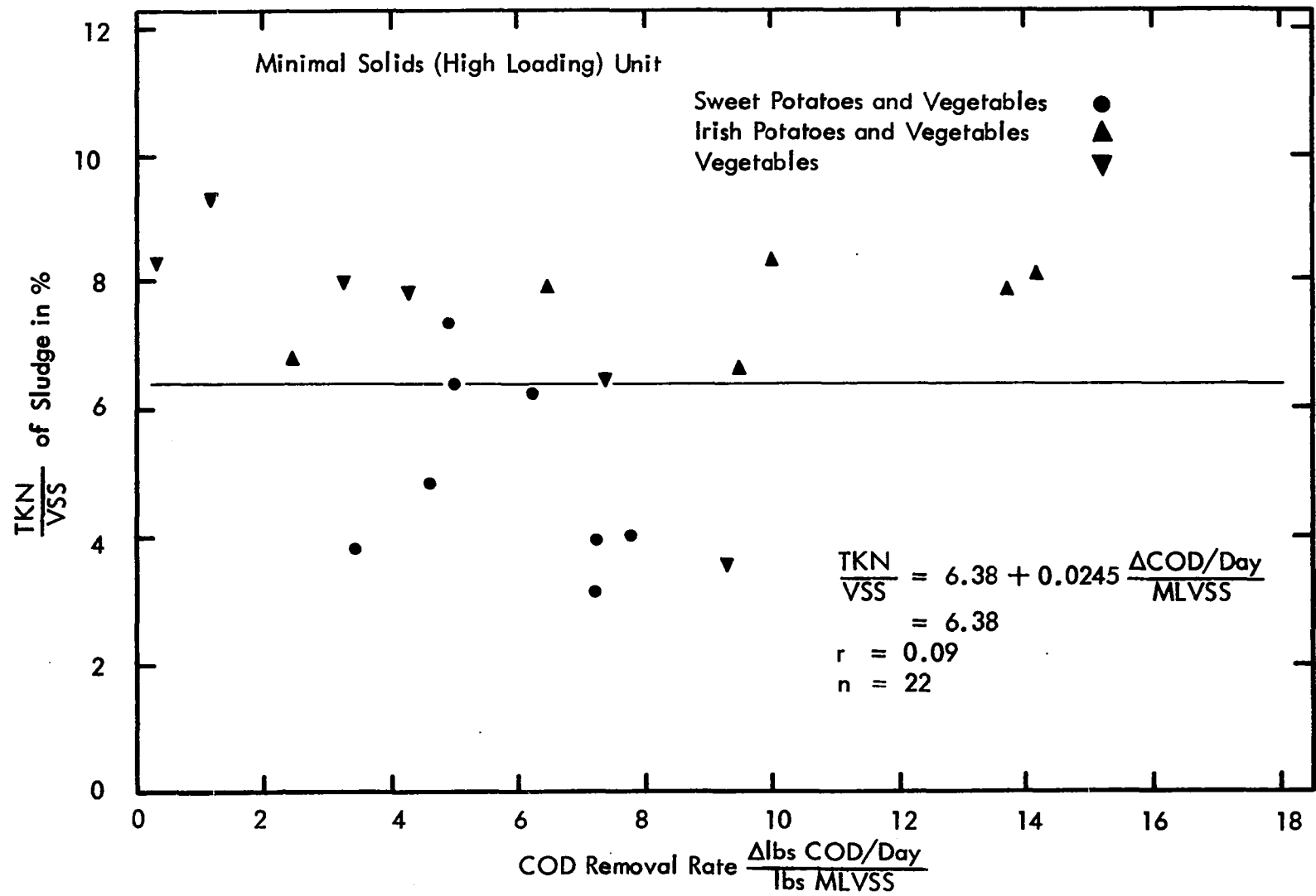
Figure 87 \frac{\text{TKN}}{\text{VSS}} of Sludge vs COD Removal Rate
