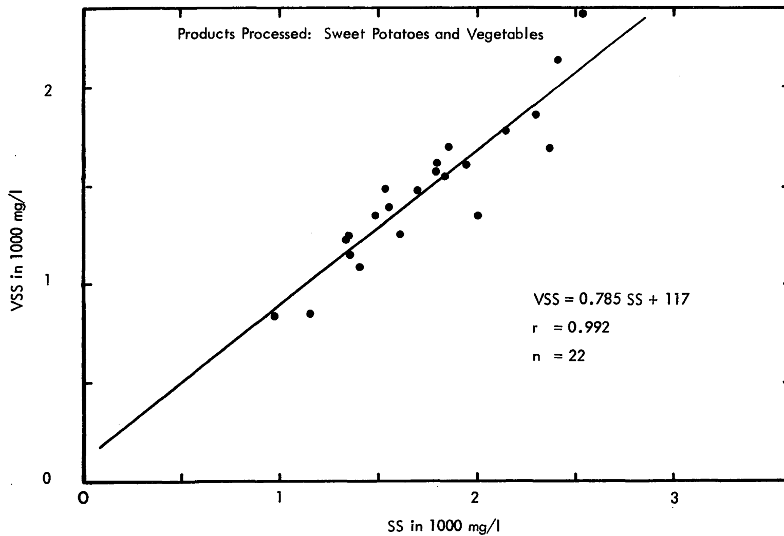
Figure 36 Plant Influent VSS vs SS
