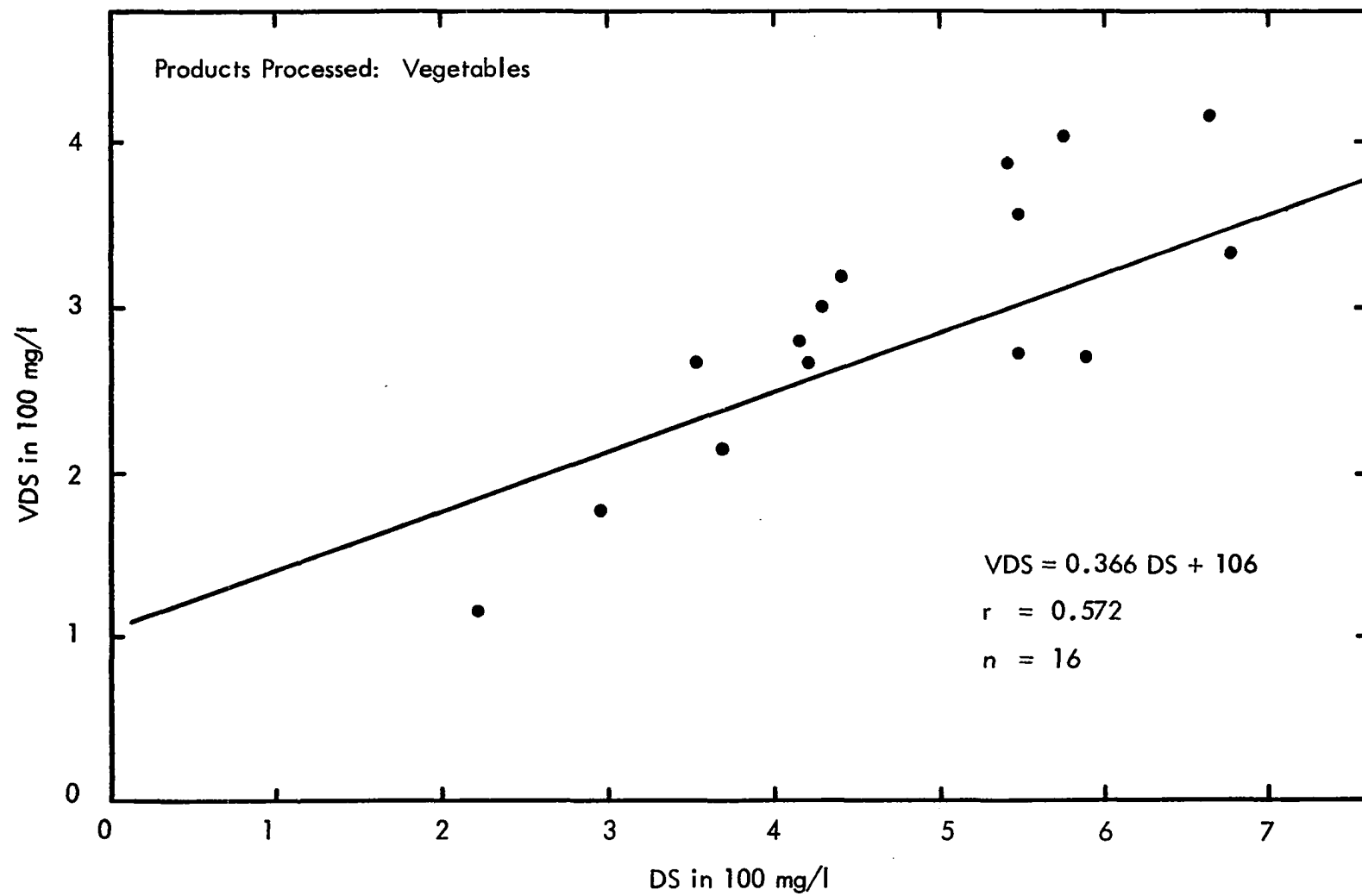
Figure 48 Plant Influent VDS vs DS
