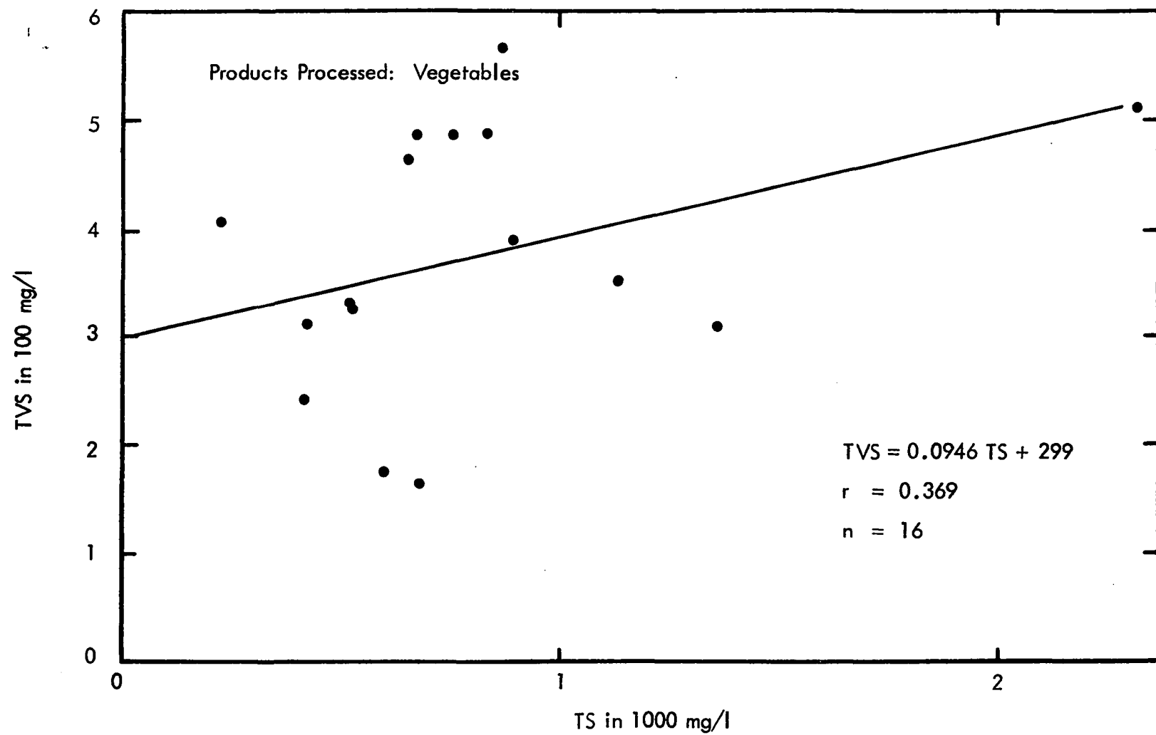
Figure 50 Plant Influent TVS vs TS
