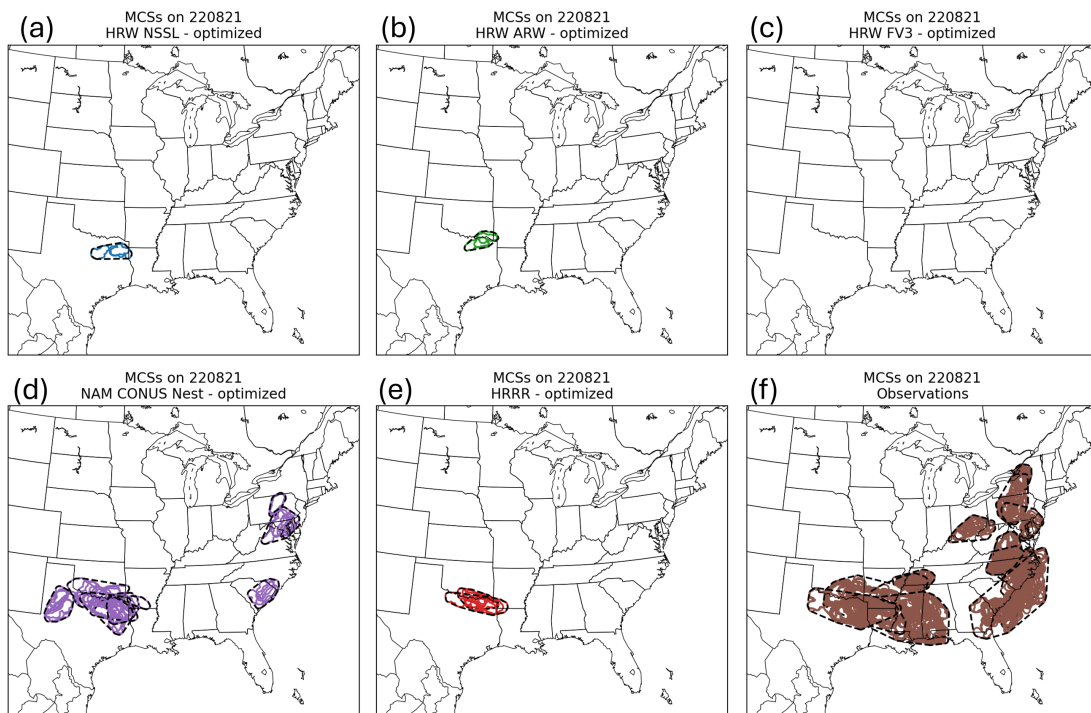
Figure 4.15: As in Figure 4.12 for 21 August 2022.
