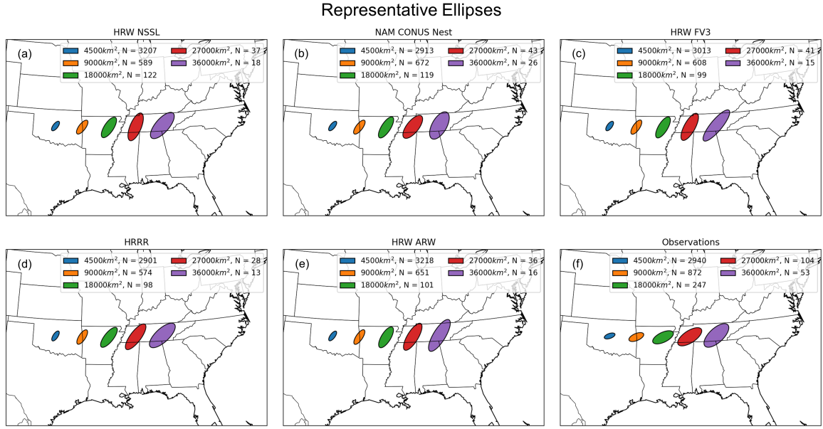
Figure 2.6: Ellipses of various sizes, with aspect ratio and orientation for each determined by the mean aspect ratio and orientation for ellipses of those sizes for the (a) HRW NSSL, (b) NAM CONUS Nest, (c) HRW FV3, (d) HRRR, and (e) HRW ARW models and (f) observations. The locations of the ellipses are not representative and are meant to help provide a sense of scale. The number of objects at a given size is shown in the legend.
