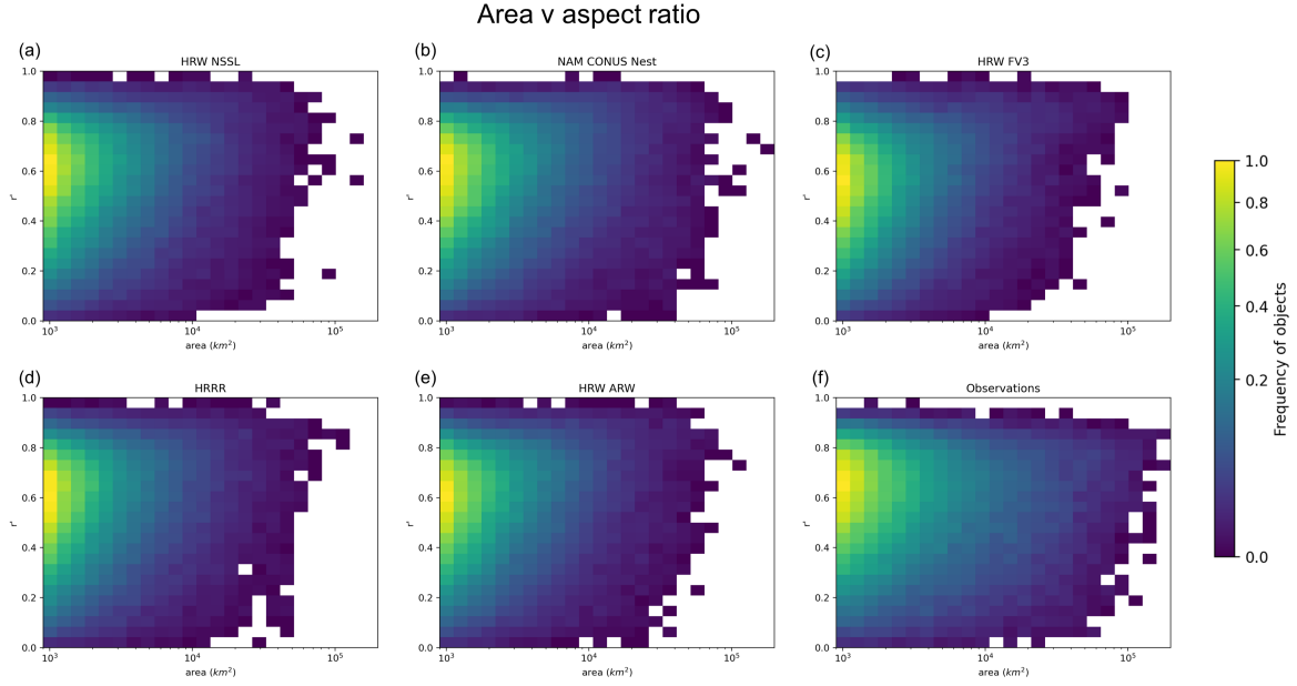
Figure 2.2: Density plot of object area against r' , with a minimum area of 900 \text{ km}^2 for the (a) HRW NSSL, (b) NAM CONUS Nest, (c) HRW FV3, (d) HRRR, and (e) HRW ARW models and (f) observations. Rounder objects have an r' closer 0, and less round objects have an r' closer to 1. The color scale uses a power law and is relative for each subfigure. The power law scale was chosen to emphasize differences at lower object counts.
