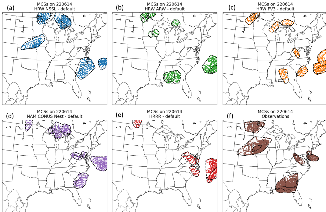
Figure 4.11: Modeled and observed MCSs for 14 June 2022. The solid colored lines are the individual MCSs and the black dashed lines are the convex hulls of each full MCS. The modeled MCSs were identified using the default parameters. (a) HRW NSSL, (b) HRW ARW, (c) HRW FV3, (d) NAM CONUS Nest, (e) HRRR, (f) Observations.
