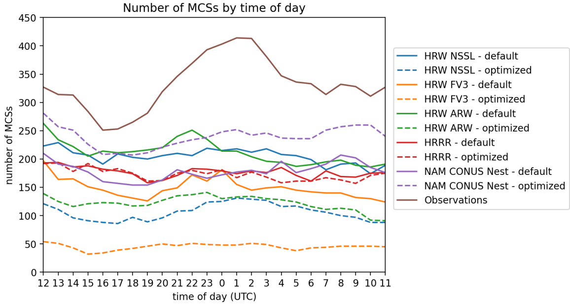
Figure 4.1: The total number of MCSs that occur during 2022 by time of day.
