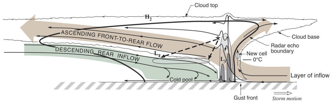
Figure 1.1: Conceptual model of a trailing stratiform MCS as viewed from a vertical cross section perpendicular to the convective line. The orange shading is the front to rear inflow, while the green shading is the rear inflow. The medium and dark gray shading is the radar reflectivity. Figure 17-12 from Houze (2018), which is a color version of Figure 1 from Houze et al. (1989).
