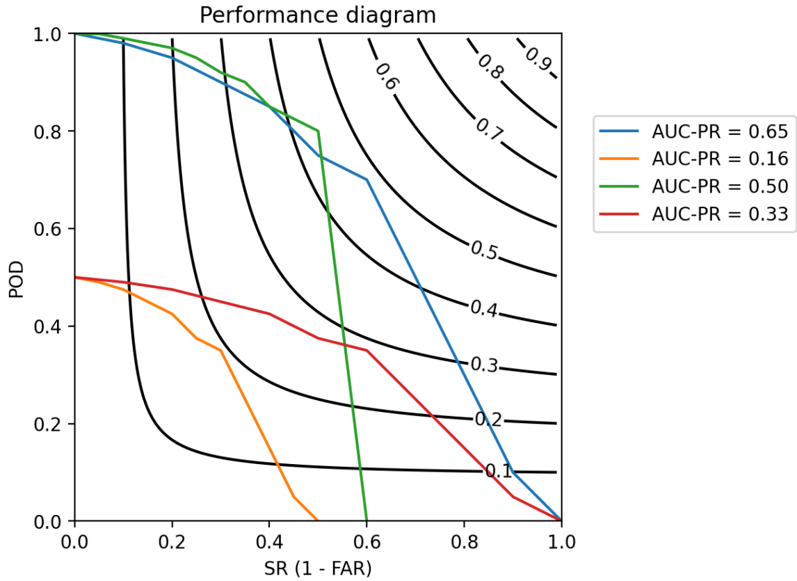
Figure 3.3: Performance diagram showing how AUC-PR varies with several different forecasts. The x-axis is success ratio (SR), which is equivalent to 1 minus the false alarm ratio (FAR). The y-axis is probability of detection (POD). The black contours are lines of constant critical success index (CSI).
