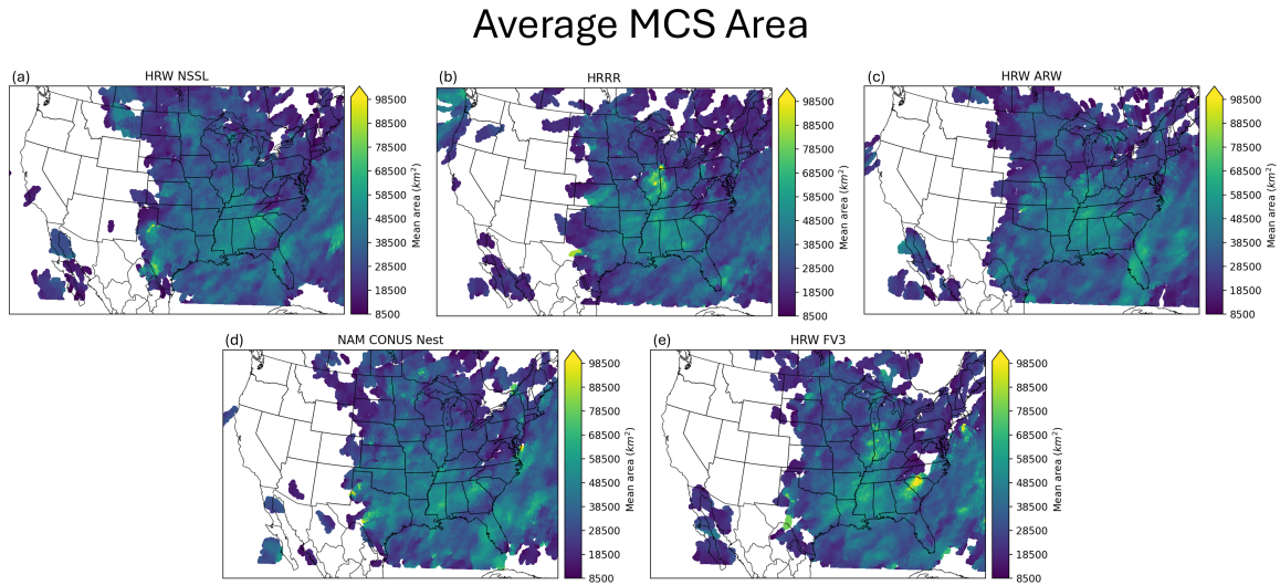
Figure 3.7: The average area of modeled MCSs in 2022 for the (a) HRW NSSL, (b) HRRR, (c) HRW ARW, (d) NAM CONUS Nest, and (e) HRW FV3.
