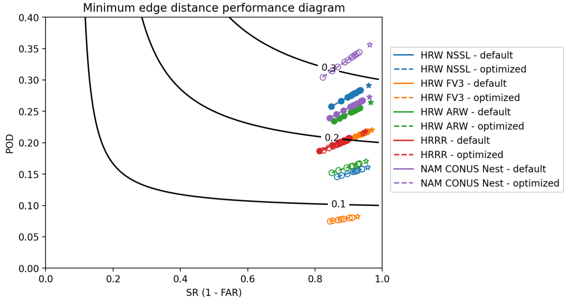
Figure 4.5: As in Figure 4.4 but for minimum edge distance between MCSs.
