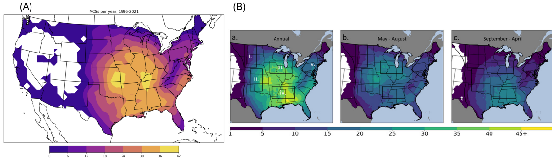
Figure 3.6: (A) Figure 2 from Wade et al. (2023) showing the average number of MCSs for 1996-2021. (B) Figure 1 from Haberlie and Ashley (2019) (a) shows the annual number of MCSs for 1996-2017, (b) and (c) show seasonal counts from May-August and September-April, respectively.
