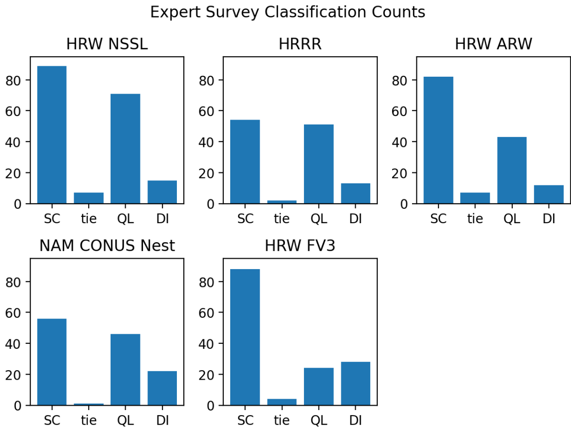
Figure 3.1: The counts of expert-labeled storm mode for each model in the HREF. SC are supercells, QL are linear, DI are disorganized.
