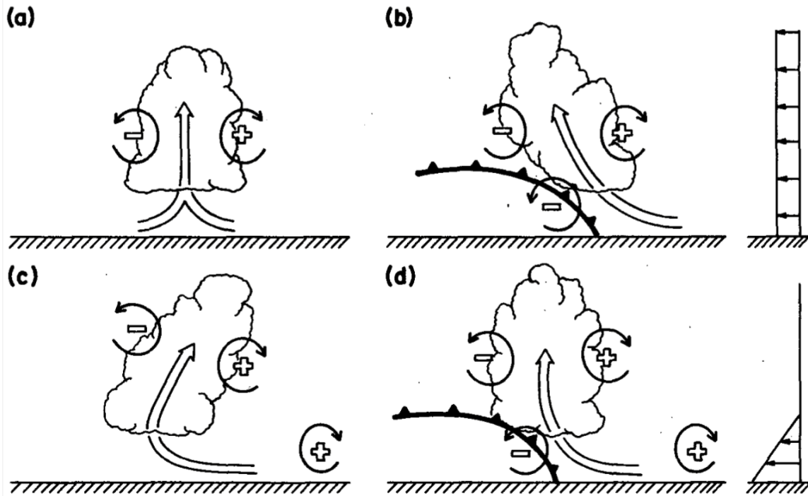
Figure 1.2: Schematic showing how an updraft can be influenced by shear and a cold pool. (a) with neither wind shear nor a cold pool, the storm is vertical (b) with a cold pool but no shear, the structure is biased by the negative vorticity from the cold pool and the storm leans upshear (c) with shear but no cold pool, the positive vorticity from the shear causes the storm to lean (d) with both a cold pool and wind shear, the vorticities may balance and cause the storm to remain vertical. Figure 18 from Rotunno et al. (1988).
