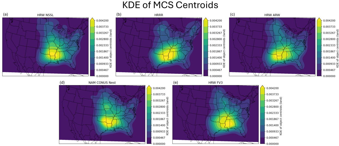
Figure 3.8: KDE of modeled MCS centroids in 2022 for the (a) HRW NSSL, (b) HRRR, (c) HRW ARW, (d) NAM CONUS Nest, and (e) HRW FV3. Only centroids over land were considered for the analysis.
