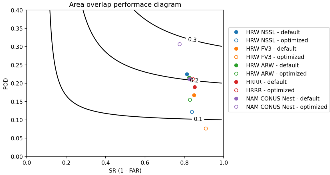
Figure 4.3: Performance diagram using area of overlap to count as hits. The y-axis is probability of detection and the x-axis is success ratio, which is equivalent to 1 minus the false alarm ratio. Note that the y-axis only goes from 0 to 0.4. The curved black lines are contours of critical success index (CSI).
