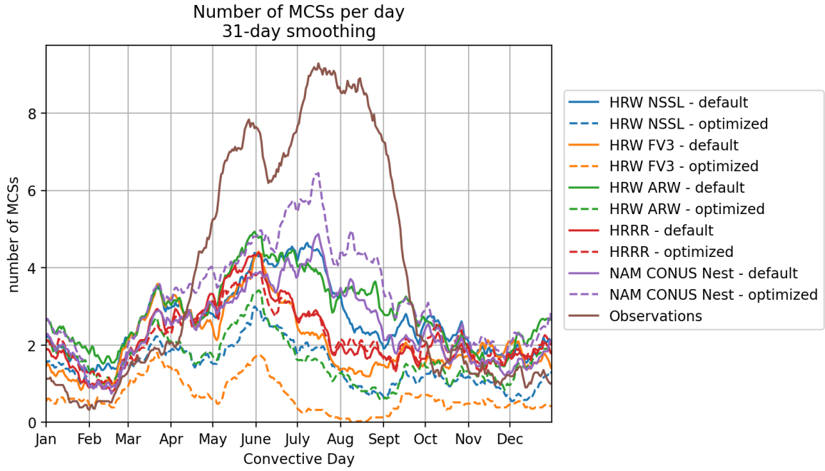
Figure 4.2: Average number of MCSs per day, using a 31-day smoothing window.
