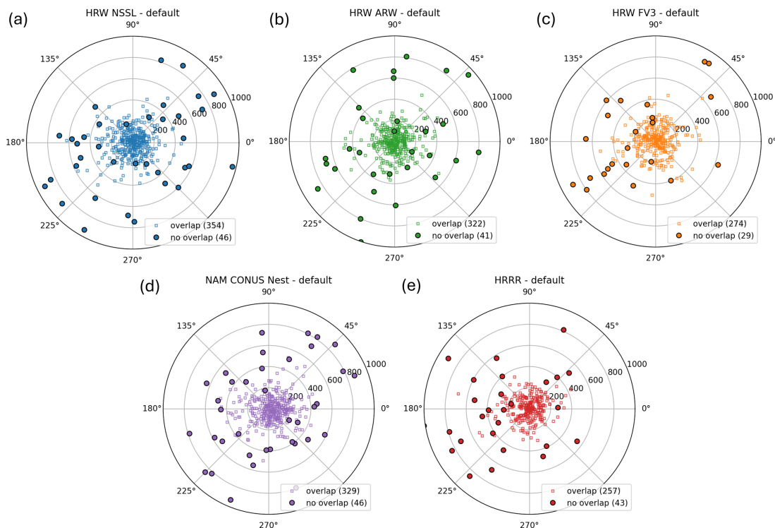
Figure 4.6: The storm-relative error vector from the centroid of each modeled MCS to the nearest observed MCS centroid using the default MCS identification parameters. The radius is in kilometers. The modeled storm direction is along the positive x-axis. The hollow square markers indicate when the modeled MCS overlapped with the observed MCS, and the filled dots indicate when there was no overlap. The models are (a) the HRW NSSL, (b) the HRW ARW, (c) the HRW FV3, (d) the NAM CONUS Nest, and (e) the HRRR. The numbers in the legend indicate the number of forecast MCSs in each category.
