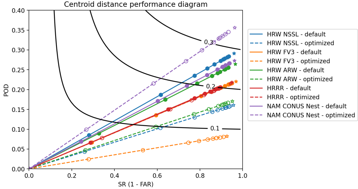
Figure 4.4: Performance diagram using centroid distance. The threshold distance to count as a hit varied from 0 km to 1000 km. Results are plotted every 1km to produce a curve. The dots are plotted every 100 km. The hollow dots are associated with the dashed lines and the optimized parameters while the solid dots are associated with the solid lines and the default parameters. The stars represent the limit where every forecast object on a day with observed objects is counted as a hit (in other words, if the distance threshold went towards infinity). Again note that the y-axis only goes from 0 to 0.4.
