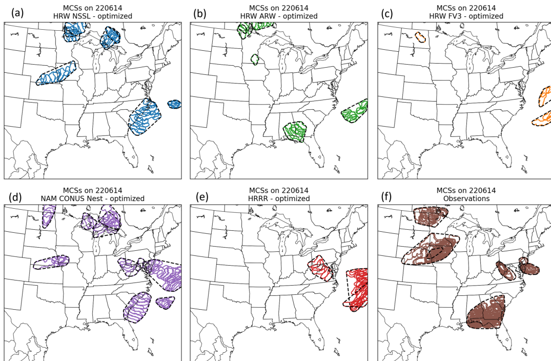
Figure 4.12: As in Figure 4.11, but modeled MCSs were identified using the MCS identification parameters optimized to match expert labeling.
