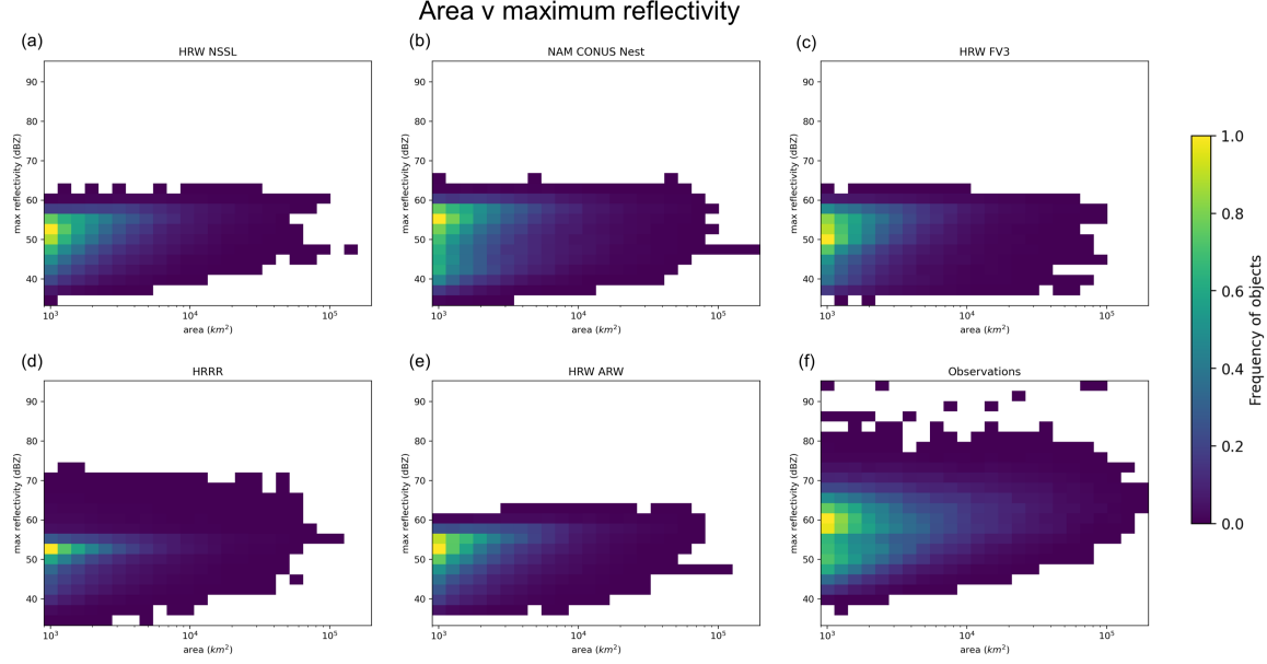
Figure 2.3: As in Figure 2.2 for area and maximum reflectivity in the object with a linear color scale.
