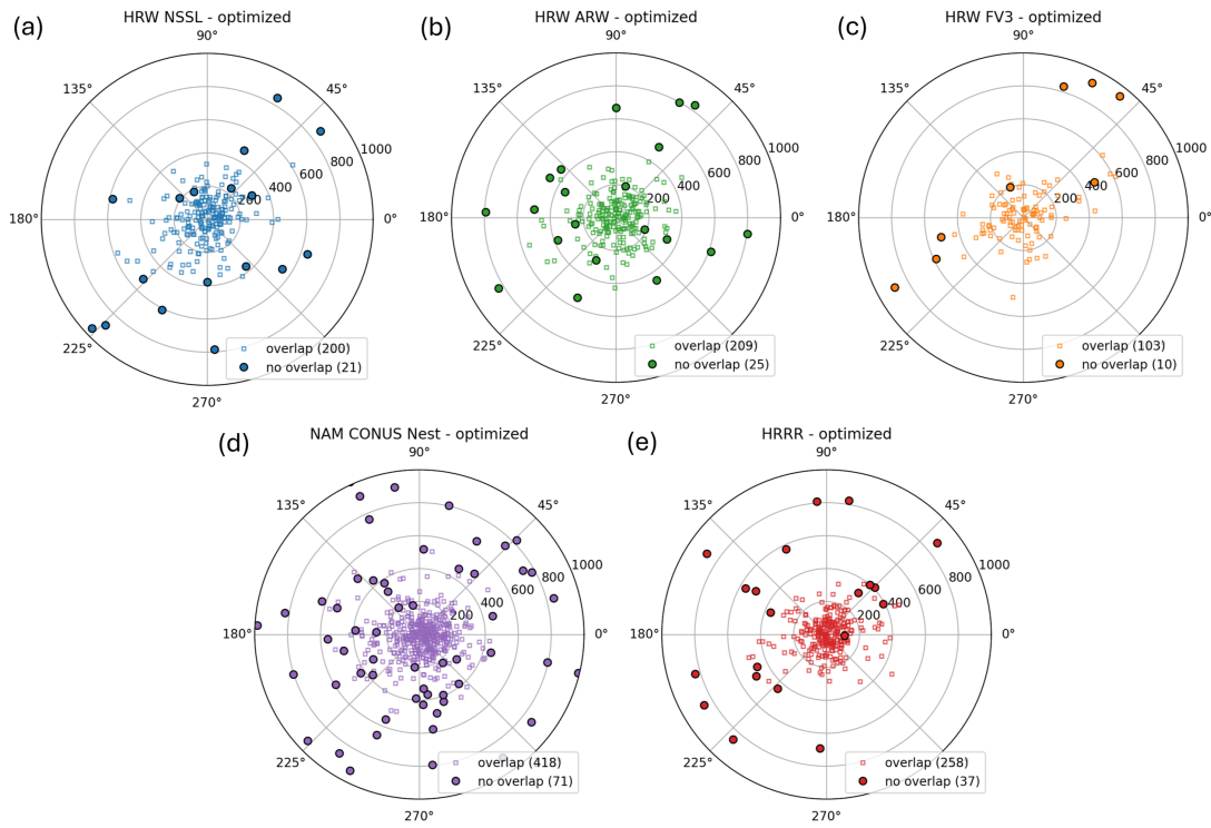
Figure 4.7: As in Figure 4.6 but for the optimized MCS identification parameters.
