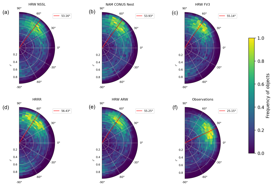
Figure 2.5: As in Figure 2.4 with a minimum area of 4500km^2 .
