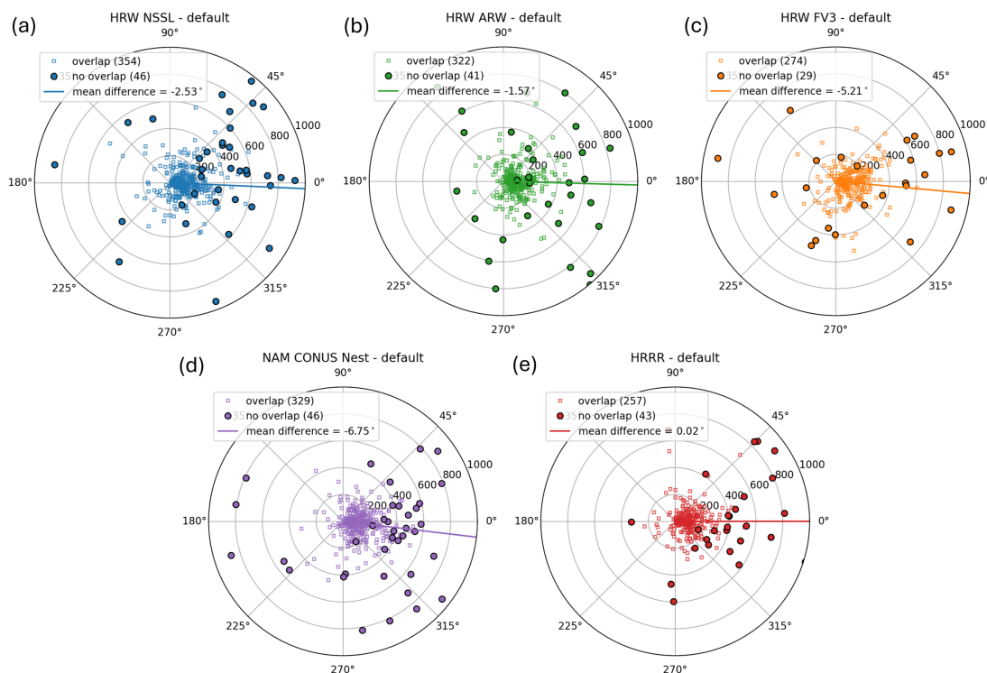
Figure 4.8: The difference in storm direction between the modeled MCS and the nearest observed MCS. The mean angle difference is plotted. The radius is the distance between the modeled MCS centroid and the nearest observed MCS centroid. The modeled storm direction is along the positive x-axis. The hollow square markers indicate when the modeled MCS overlapped with the observed MCS, and the filled dots indicate when there was no overlap. The models are (a) the HRW NSSL, (b) the HRW ARW, (c) the HRW FV3, (d) the NAM CONUS Nest, and (e) the HRRR. The numbers in the legend indicate the number of forecast MCSs in each category.
