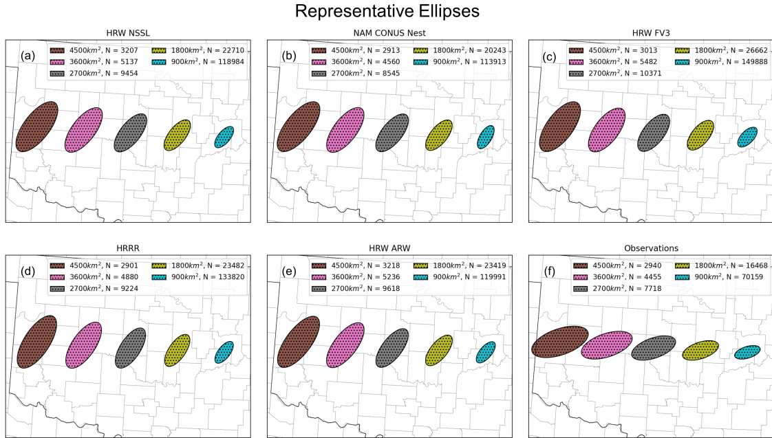
Figure 2.7: As in Figure 2.6, but for smaller ellipses.
