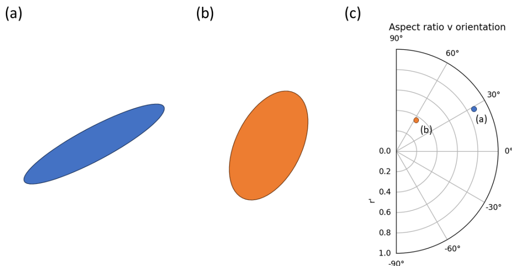
Figure 2.1: (a) A highly non-round ellipse with an orientation near 30^\circ and an r' near 0.8, (b) a rounder ellipse with an orientation near 60^\circ and an r' near 0.4, (c) the ellipses from (a) and (b) plotted on a polar plot.
