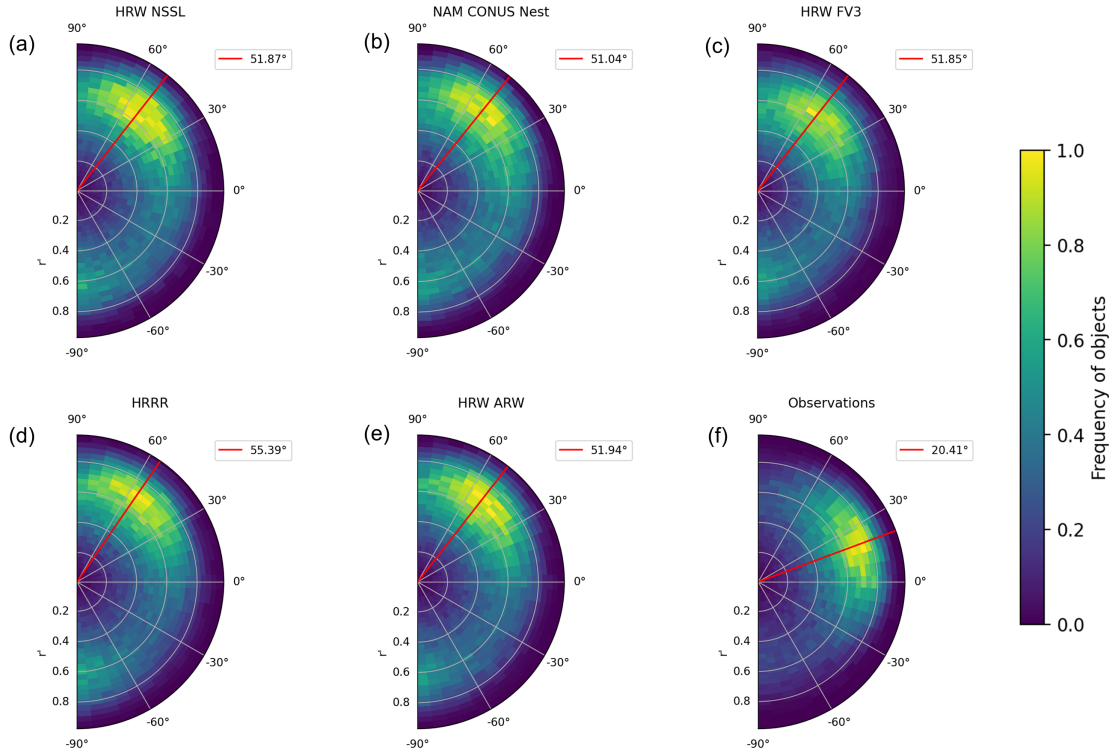
Figure 2.4: Aspect ratio and orientation plotted on polar axes, as described in Figure 2.1, subject to a 900 \text{ km}^2 minimum area for the (a) HRW NSSL, (b) NAM CONUS Nest, (c) HRW FV3, (d) HRRR, and (e) HRW ARW models and (f) observations. The labeled red line in each plot represents the mean orientation angle for the given plot. Rounder objects are closer to the origin, and less round objects are closer to the edge. The color scale is relative for each subfigure.
