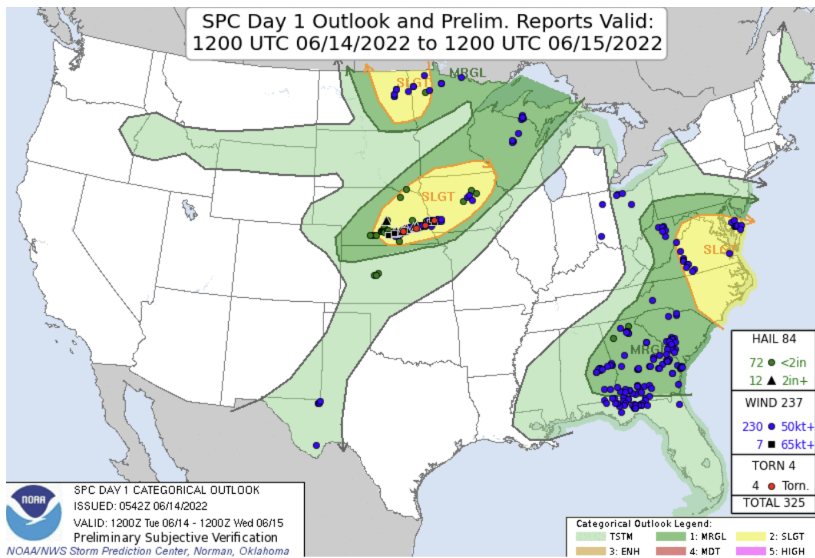
Figure 4.10: SPC Day 1 outlook and storm reports for 14 June 2022.
