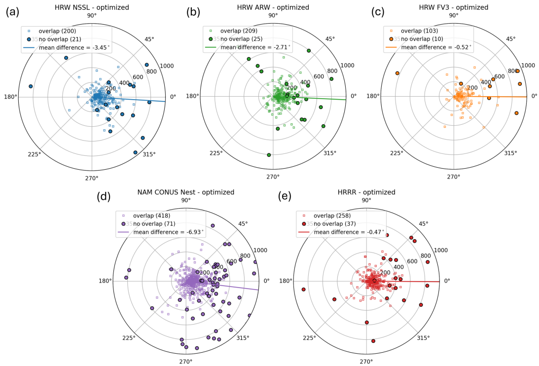
Figure 4.9: As in Figure 4.8 but for the optimized MCS identification parameters.
