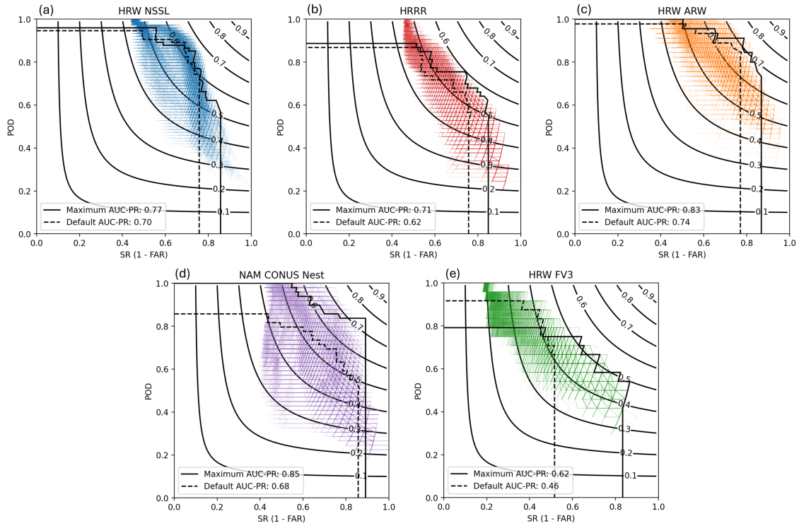
Figure 3.4: Performance diagrams showing the ability of the modified Wade algorithm to identify MCSs as labeled by the expert classification for each model. Each colored line is the performance of a single parameter set. The solid black line is the parameter set with the highest AUC-PR for each model and the dashed black line is the default parameters.
