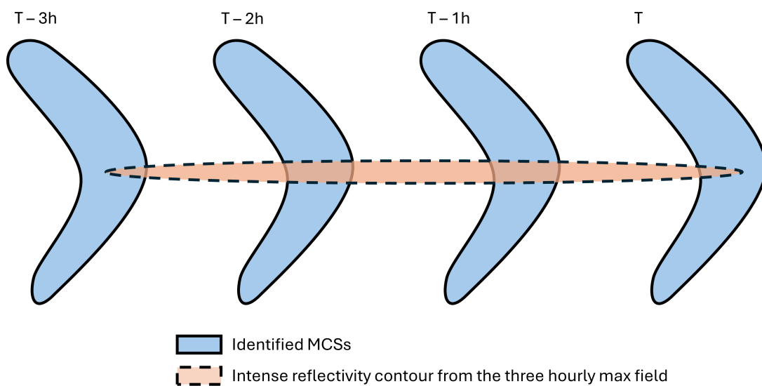
Figure 3.2: A schematic of the MCS tracking algorithm for time T . MCSs were identified at times T-3 , T-2 , T-1 , and T . The intense reflectivity contour (black dashed line) is 50 dBZ.
