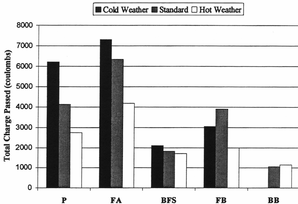
Fig. 4.40 RCIP at 28 Days, Temperature Study
