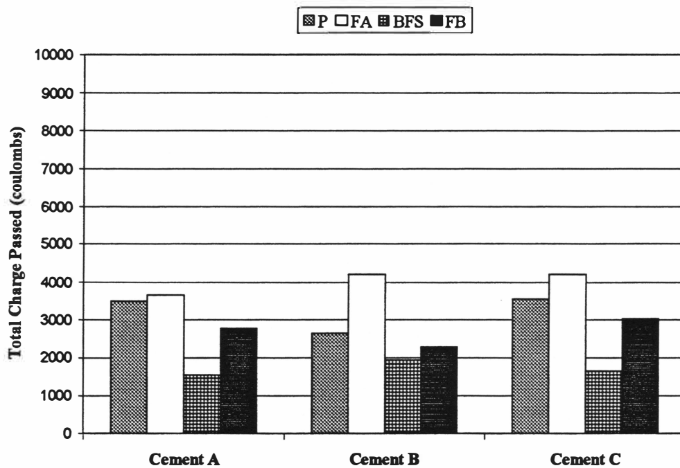
Fig. 4.15 90 Day Rapid Chloride Ion Penetrability, Cement Study
