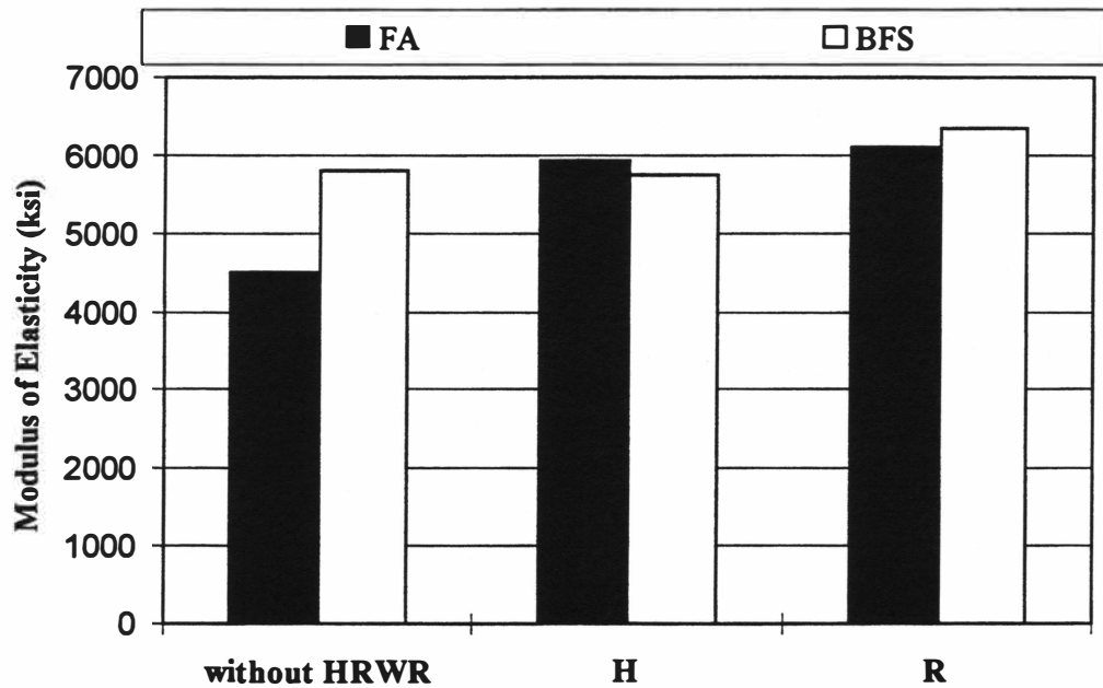
Fig. 4.60 Modulus of Elasticity of Class AA Concrete With and Without HRWR
