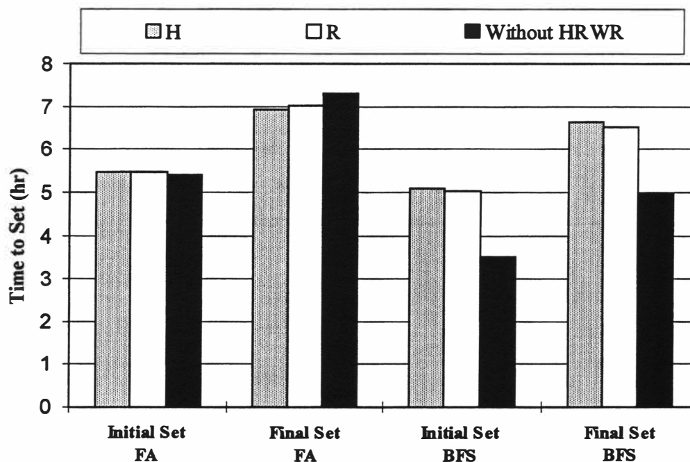
Fig. 4.54 Time to Set for Class AA Mixtures With and Without HRWR
