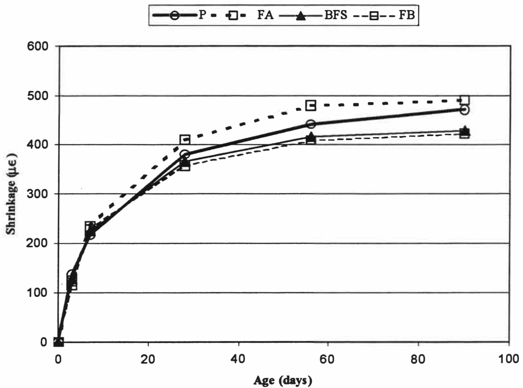
Fig. 4.12 Shrinkage Curves for Cement B Mixtures
