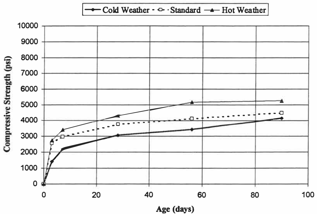
Fig. 4.25 Compressive Strength for FA Mixtures, Temperature Study
