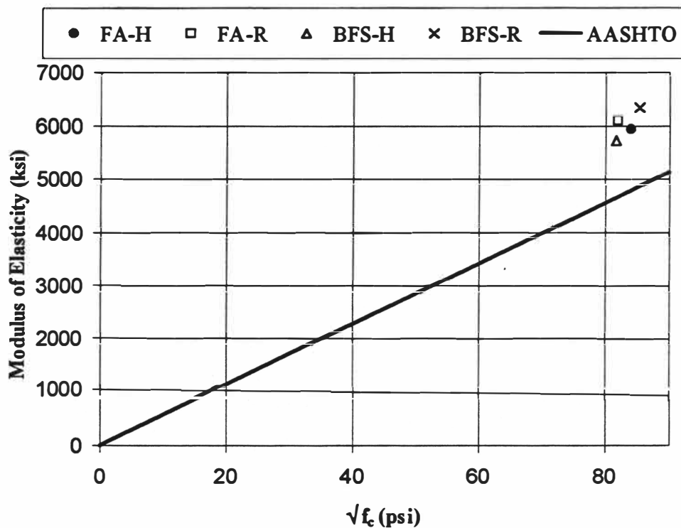
Fig. 4.61 28 Day Modulus of Elasticity of Class AA Concrete with HRWR
