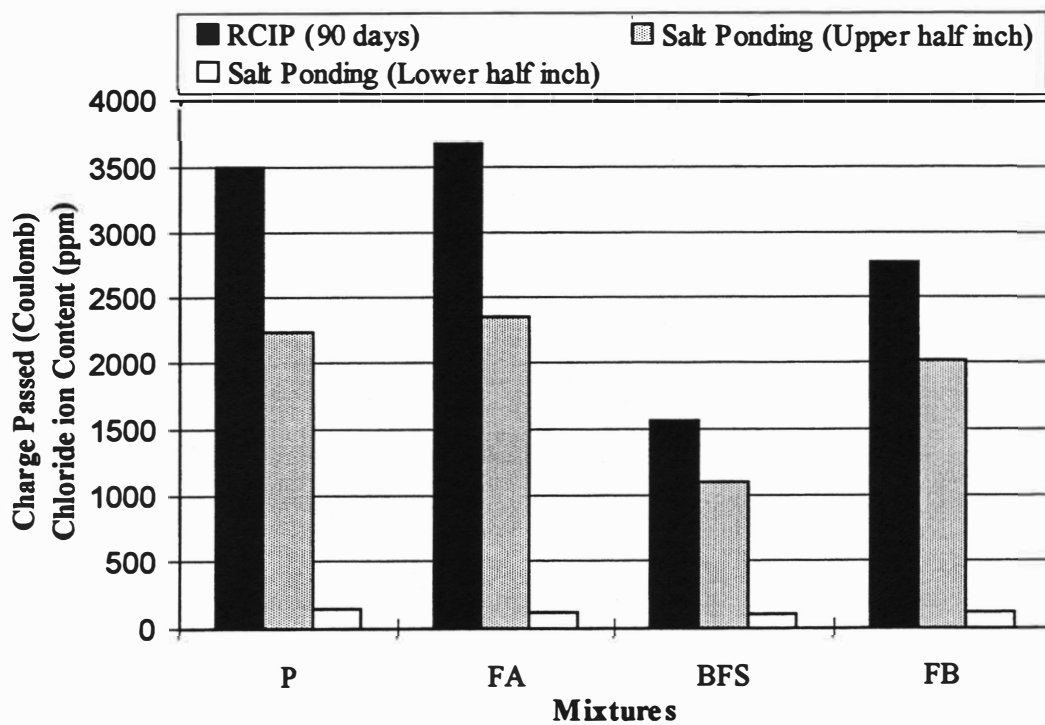
Fig. 4.20 Comparison of Salt Ponding and RCIP Test Results
