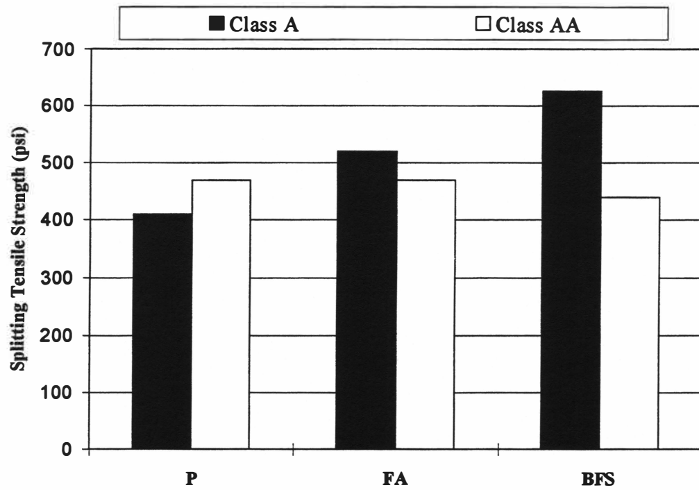
Fig. 4.47 Splitting Tensile Strength of Class A and AA Mixtures
