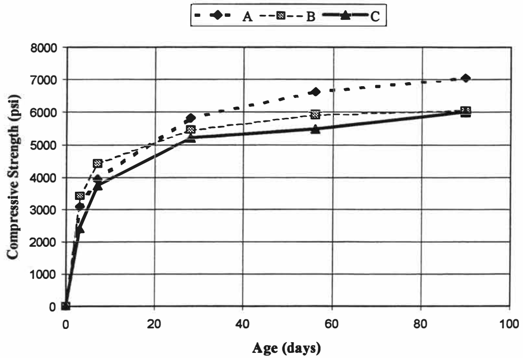
Fig. 4.6 Strength Gain for BFS Mixtures
