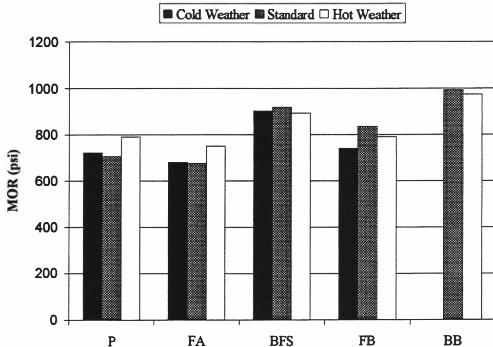
Fig. 4.29 Modulus of Rupture, Temperature Study
