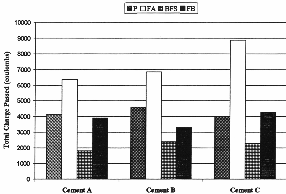
Fig. 4.14 28 Day Rapid Chloride Ion Penetrability, Cement Study
