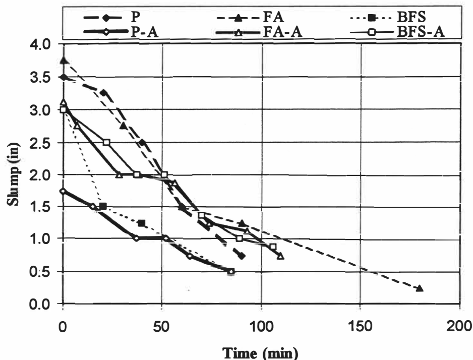
Fig. 4.42 Slump Loss of Class A and Class AA Concrete
