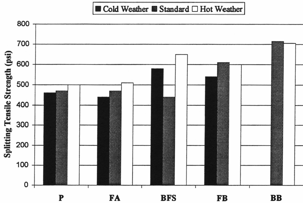
Fig. 4.31 Splitting Tensile Strength at 28 Days, Temperature Study
