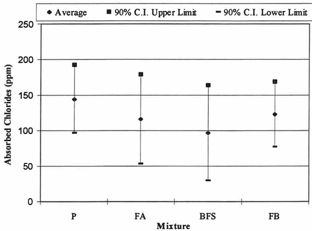
Fig. 4.19 Absorbed Chlorides in the Lower Half Inch
