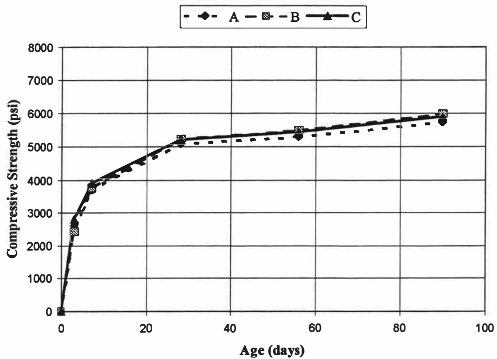
Fig. 4.7 Strength Gain for FB Mixtures
