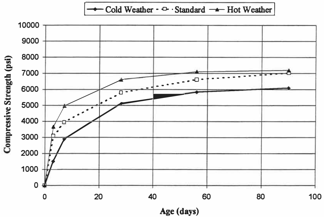
Fig. 4.26 Compressive Strength for BFS Mixtures, Temperature Study
