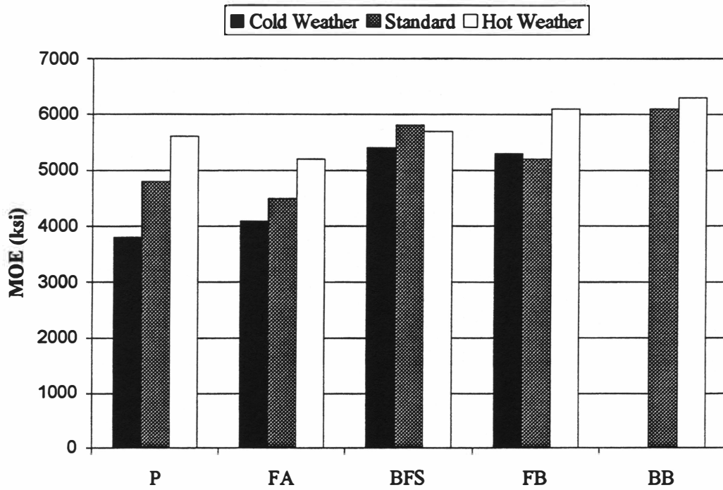
Fig. 4.34 Modulus of Elasticity at 28 Days, Temperature Study
