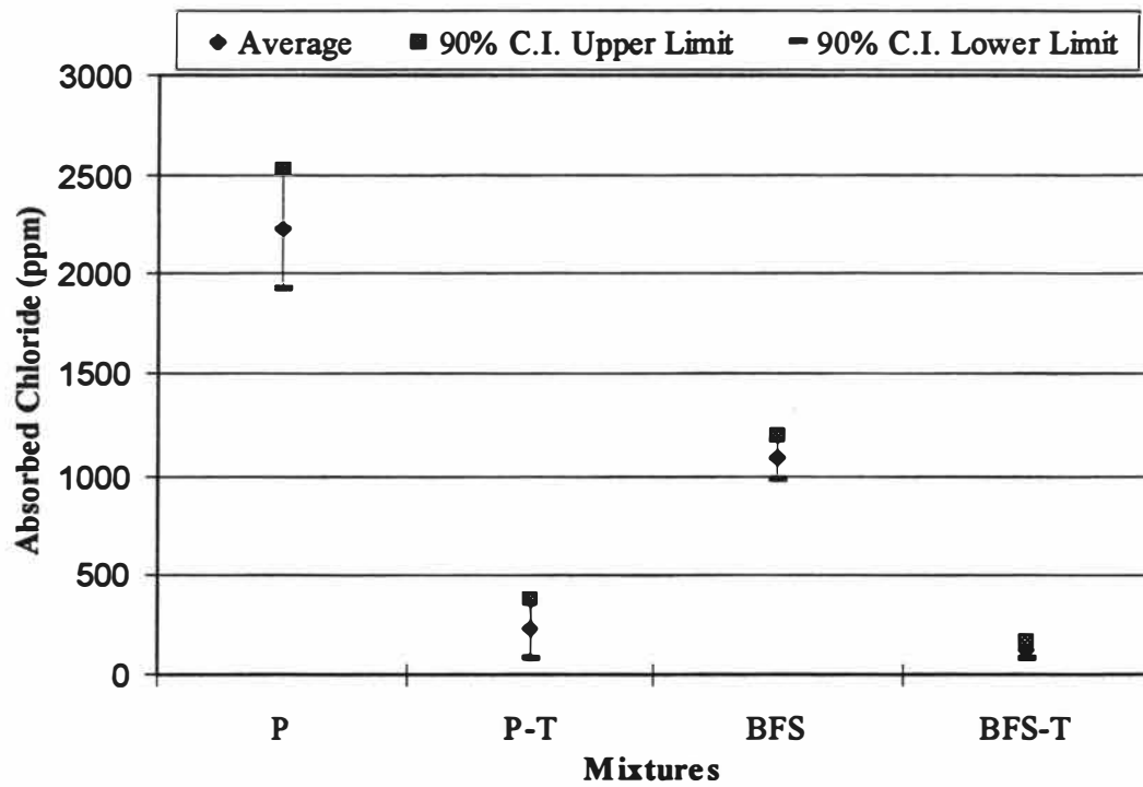
Fig. 4.64 Absorbed Chlorides in the Upper Half Inch, Silane Study
