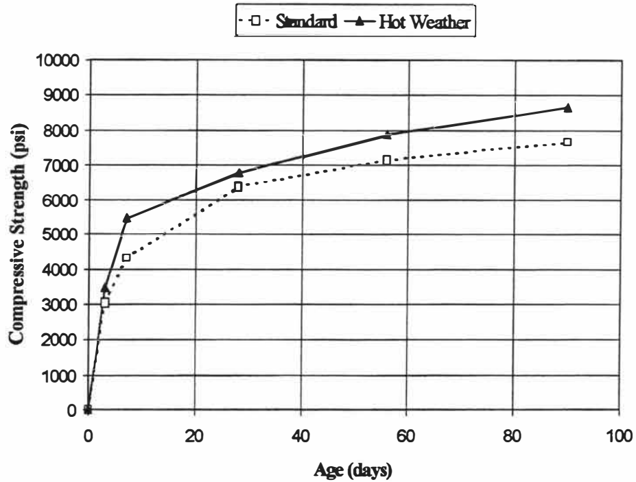
Fig. 4.28 Compressive Strength for BB Mixtures, Temperature Study
