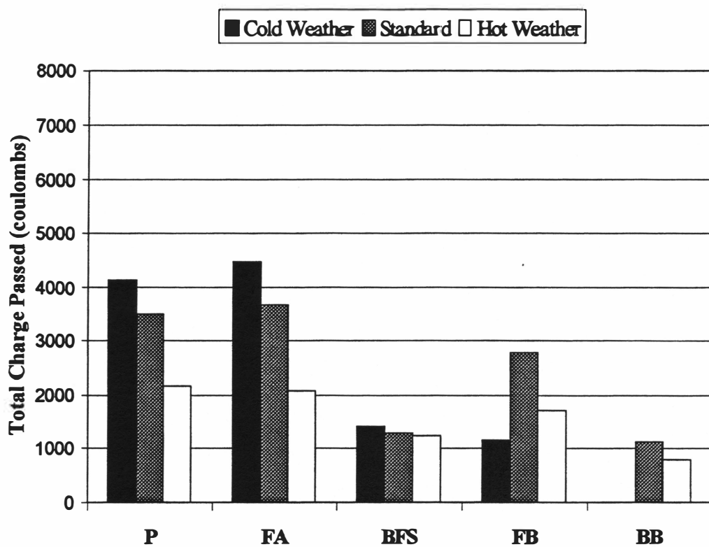
Fig. 4.41 RCIP at 90 Days, Temperature Study
