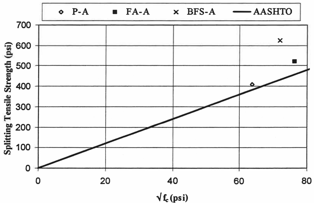
Fig. 4.48 Splitting Tensile Strength of Class A Concrete (28 days)
