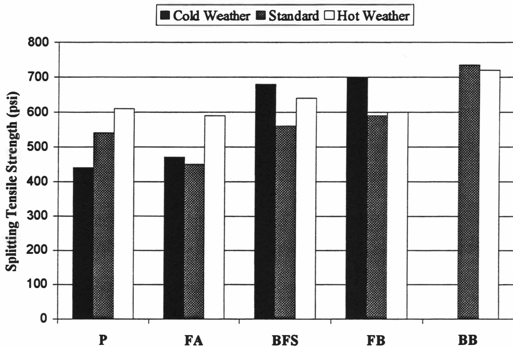
Fig.4.32 Splitting Tensile Strength at 90 Days, Temperature Study
