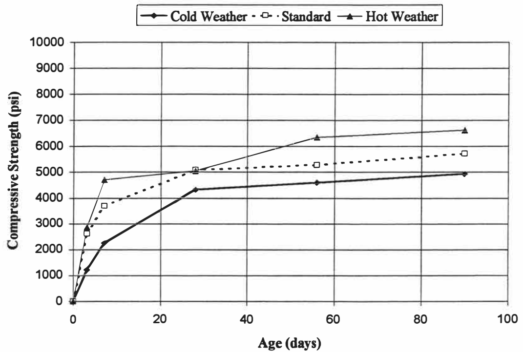
Fig. 4.27 Compressive Strength for FB Mixtures, Temperature Study
