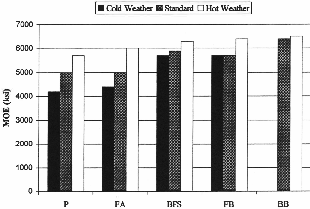
Fig. 4.35 Modulus of Elasticity at 90 Days, Temperature Study
