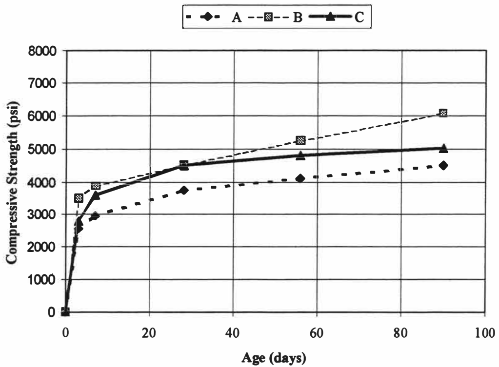
Fig. 4.5 Strength Gain for FA Mixtures
