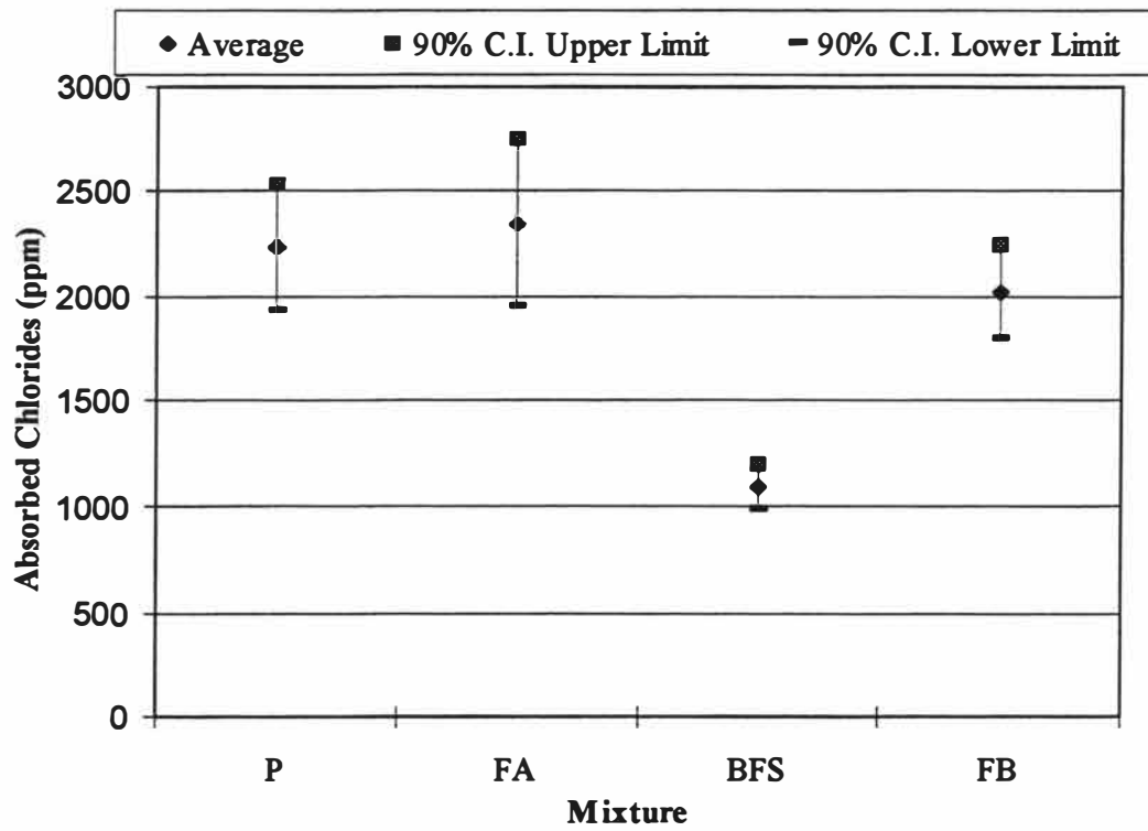
Fig. 4.18 Absorbed Chlorides in the Upper Half Inch
