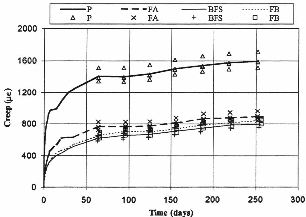
Fig. 4.16 Creep of Class AA Mixtures Over Time
