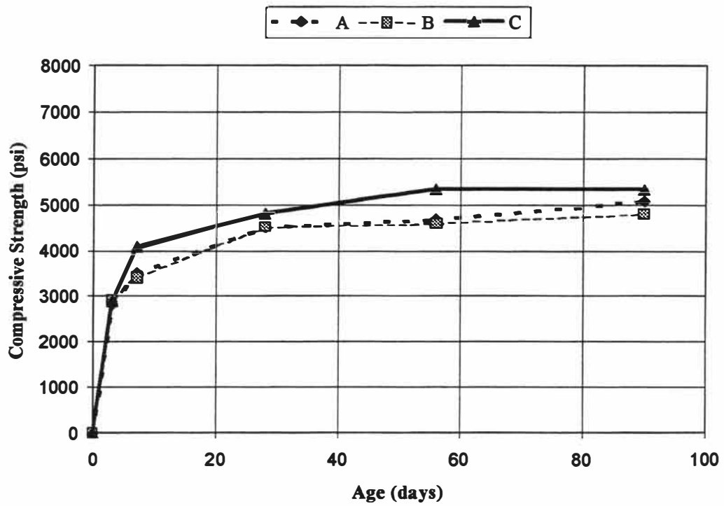
Fig. 4.4 Strength Gain for P Mixtures
