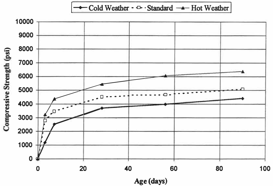
Fig. 4.24 Compressive Strength for P Mixtures, Temperature Study
