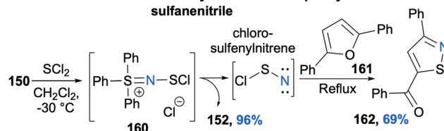
Scheme 21 Further in situ generation of sulfenylcarbenes.
