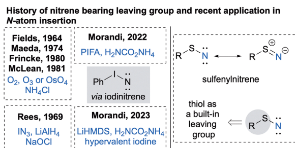
Scheme 32 History of nitrene-bearing leaving group vs. sulfenylnitrene.
