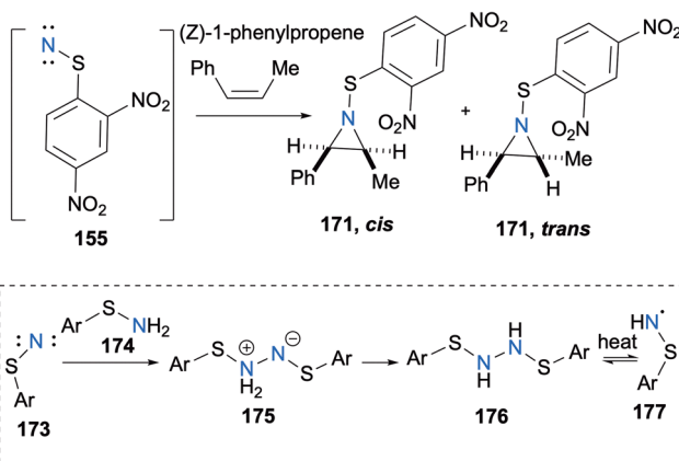
Scheme 23 Application of sulfenylnitrenes in aziridination.
