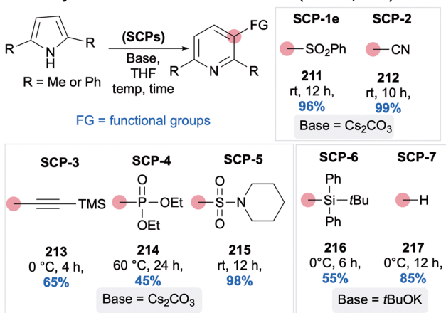
Scheme 28 Functionalized sulfenylcarbenes and their application.
