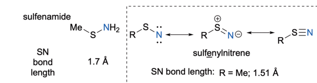
Scheme 15 N–S bond length in sulfenamide vs. sulfenylnitrene.
