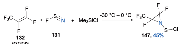
Scheme 20 In situ generation of halosulfenylaziridines.
