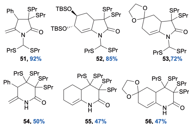
Scheme 5 Thermal generation/application of dithiocarbenes.
