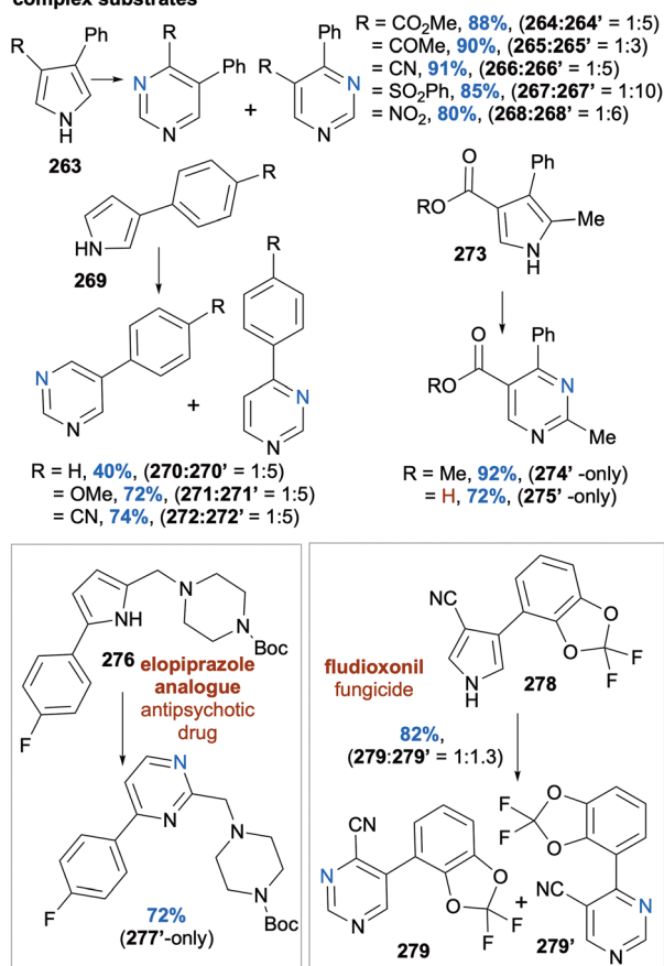
Scheme 36 Representative examples of pyrroles.
