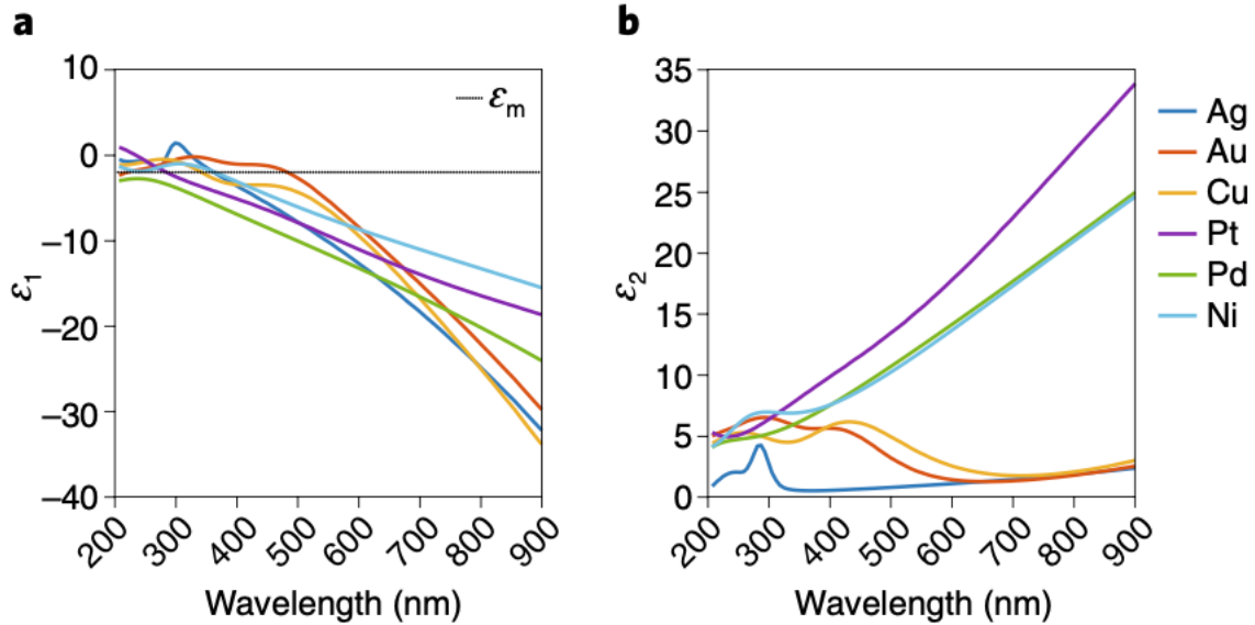
Figure 1.3 Dielectric function of noble and transition metals. (a) The real part (b) The imaginary part of the dielectric function (reproduced from reference 8 )
