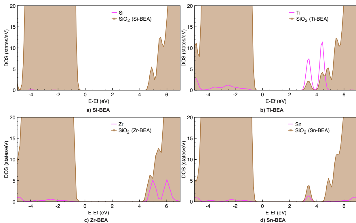
Figure 4.1.3 PDOS of M -BEA on metal (pink) and on \text{SiO}_2 framework (brown) for a) Si-BEA b) Ti-BEA c) Zr-BEA d) Sn-BEA.
