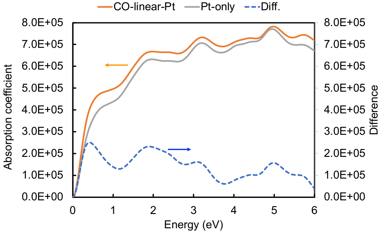
Figure 2.3 Example of absorption coefficient of CO adsorbed on Pt. Unit: \text{cm}^{-1}
