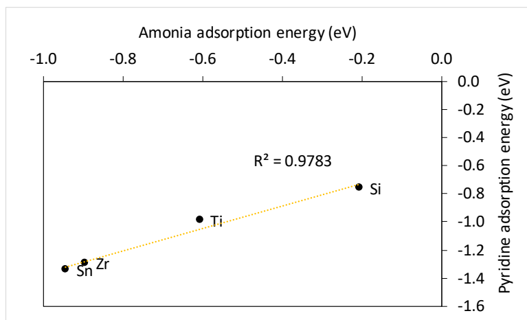
Figure A3.1 Relationship between \text{NH}_3 and pyridine adsorption energy on M-BEA.
