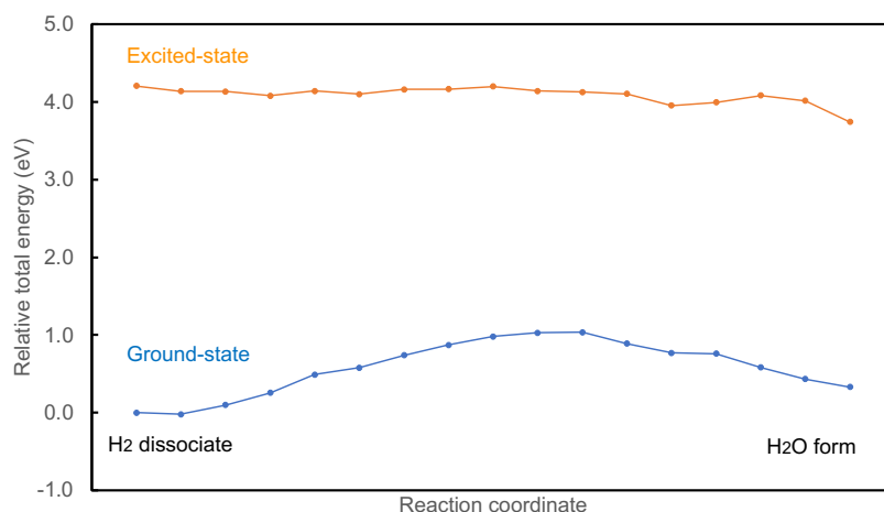
Figure A2.5 The ground- and excited-state energy profile of the oxygen vacancy formation step when one electron is added into the LUMO of \text{H}_2\text{O} by GPAW.
