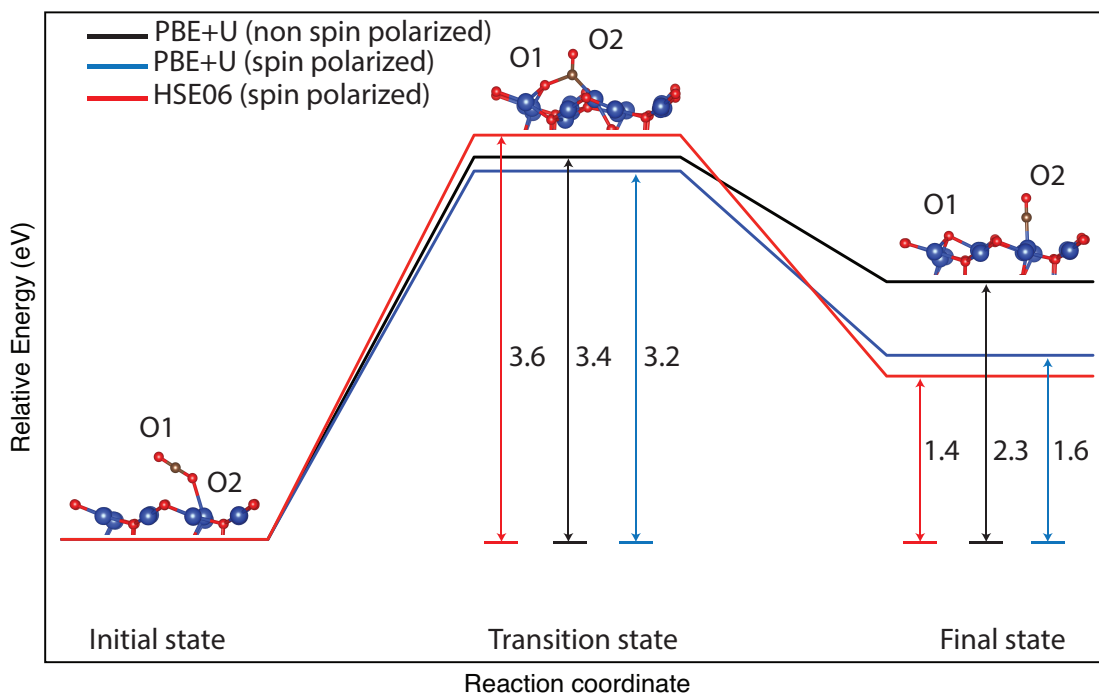
Figure 3.1.1 The energy diagram of CO 2 dissociation at the ground state calculated in PBE+U calculations with and without spin polarization and by spin-polarized HSE06 calculation. The blue, gray and red balls denote Cu, C and O atoms respectively.
