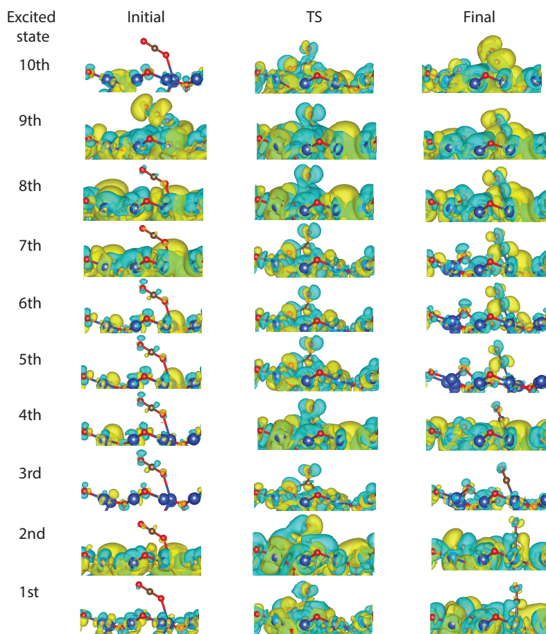
Figure A1.5 The charge density difference between the excited states (which has an added electron into unoccupied KS orbital and a hole at Fermi level) with the ground state. Cyan color represents for removed electron and yellow color represents for added electron. An isosurface value of 0.00067 \text{ e}/\text{\AA}^3 is used.
