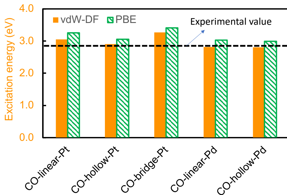
Figure 2.4 The excitation energy calculated based on vdW-DF or PBE as exchange-correlation functional using GPAW.
