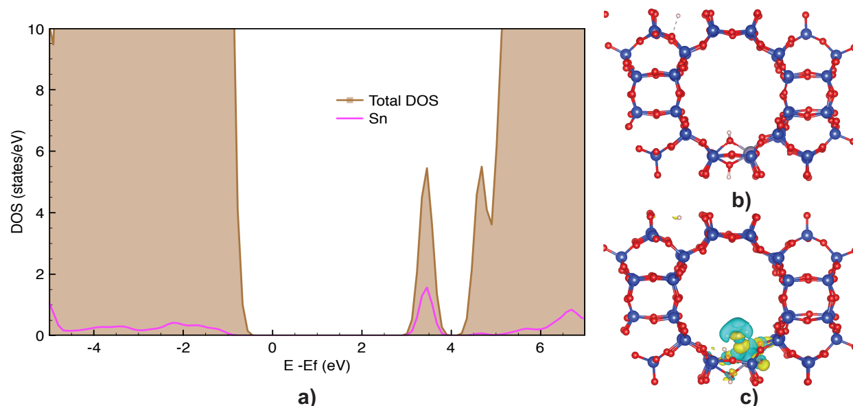
Figure 4.1.5 a) The total DOS and the PDOS of Sn of the open site configuration shown in (b), the charge redistribution when \text{NH}_3 adsorbed on the open site of Sn-BEA (c). The grey, blue, red and white balls denote Zn, Si, O and H atoms respectively.
