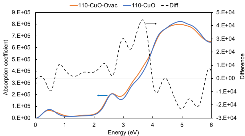
Figure A2.3 Absorption coefficient of the (110-CuO) surface with and without oxygen vacancy.
