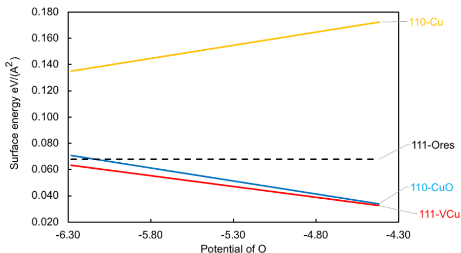
Figure A2.8 The surface energy of Cu 2 O. The O-terminated Cu 2 O (111) surface (111-Ores, black), the O-terminated Cu 2 O (111) surface with Cu vacancy (111-VCu, red), the mixed CuO-terminated (110) surface (110-CuO, blue) and the Cu-terminated (110) surface (110-Cu, orange).
