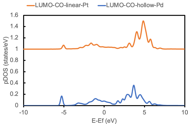
Figure 2.2 Example of pDOS on particular orbitals using GPAW: the pDOS on the LUMO of CO adsorbed on a Pt or Pd surface.
