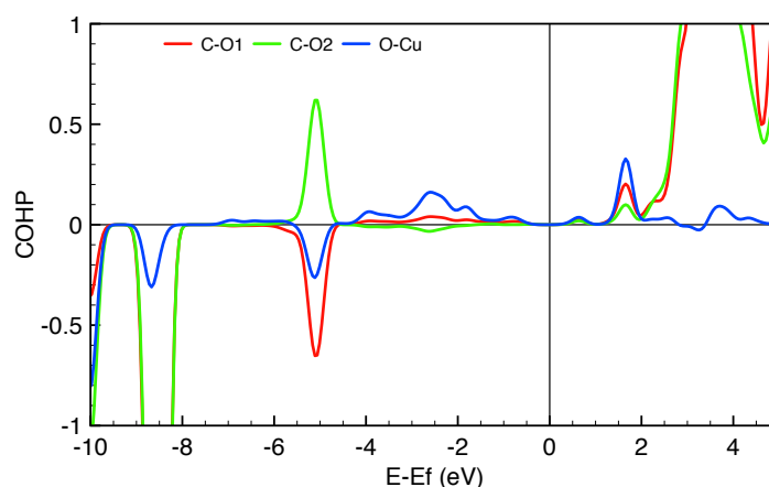
Figure A1.2 Crystal orbital Hamilton population (COHP) 138 of absorbed CO 2 on Cu 2 O (111) surface at the initial state
