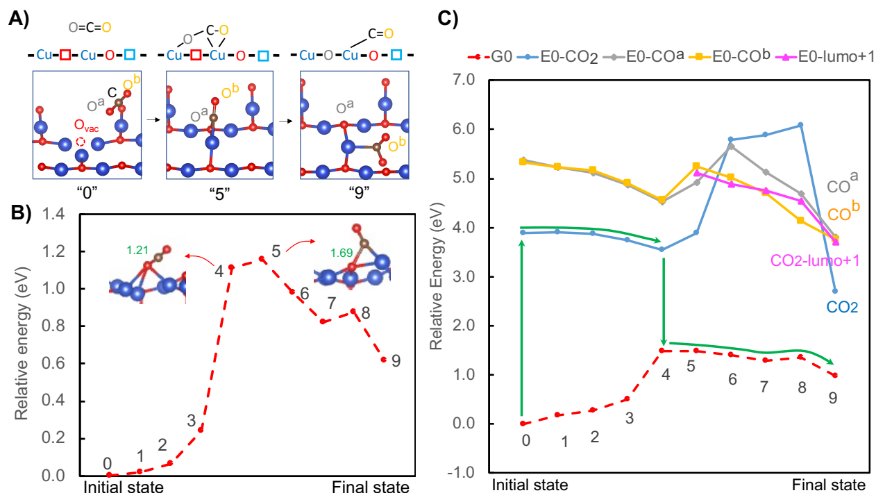
Figure 3.2.2 The CO 2 dissociation on 111-VCu-Ovac. (A) Configuration of the initial state (image 0), transition state (image 5), final state (image 9) and their corresponding schematic sketch. (B) Energy profile at the ground-state calculated in ten images (indexed 0 to 9) with VASP. The C-O a bond length is marked in green (Unit Å) (C) Energy profiles at excited states when an electron is added into the LUMO of CO 2 (blue, E0-CO 2 ), the first available antibonding state of C-O a bond (gray, E0-CO a ) or C-O b bond (orange, E0-CO b ), which are compared with the ground state (red dashed, G0); all calculated by GPAW. The magenta solid line (E0-lumo+1) is included to illustrate the case when the electron is added into the LUMO+1 of CO 2 from image 5 to 9.
