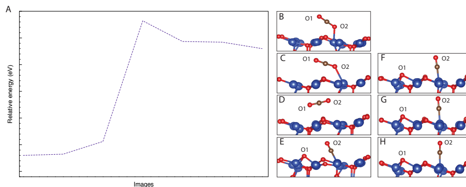
Figure A1.1 The NEB calculation results (A) and the represented configurations along reaction pathway after running about 1,000 steps (B-H). Based on NEB, the transition state and activation energy were calculated further by applying the dimmer method. We also tried to calculate the NEB calculation for breaking the C-O2 bond with O2 remains at unsaturated Cu and the C-O1 travelling to the nearby unsaturated Cu. However, the calculation cannot be converged.
