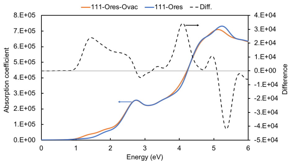
Figure A2.1 Optical absorption coefficient of the (111-Ores) surface with and without oxygen vacancy. Unit: cm -1 .
