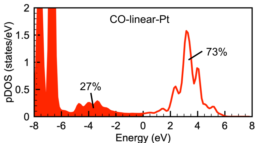
Figure 2.1 Example of pDOS on adsorbed molecule using VASP: the pDOS on CO adsorbed on a Pt surface.
