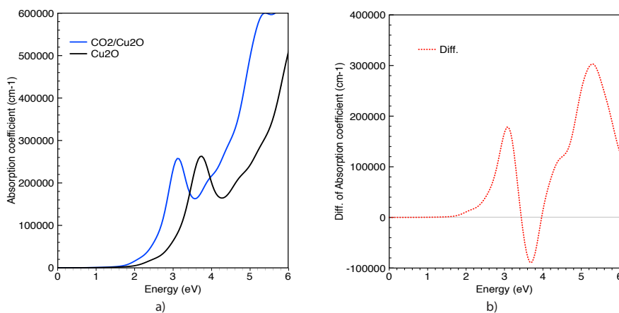
Figure A1.4 a) The absorption coefficient of Cu 2 O (black) and Cu 2 O with adsorbed CO 2 (blue); b) The difference of absorption coefficient between the two structures with and without adsorbed CO 2 on Cu 2 O. Both calculations were performed using the HSE06 functional. For the Cu 2 O result plotted in the figure, we removed the CO 2 while keeping the other atoms fixed at their positions.
