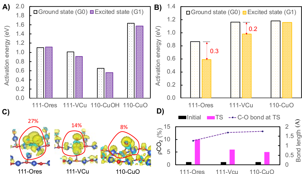
Figure A2.7 DFT results when one additional electron is added into the lowest unoccupied states of the charged system by VASP. (A) The intrinsic activation energy at the ground- and excited state of the oxygen vacancy formation step. (B) The intrinsic activation energy at the ground- and excited-state of the CO 2 dissociation step. (C) The charge density difference projected on CO 2 and under-coordinate Cu atoms at the transition state between the ground- and excited-PES. (D) The relationship between charge density localized on CO 2 at the initial state and the transition state, and the C-O bond length at the transition state.
