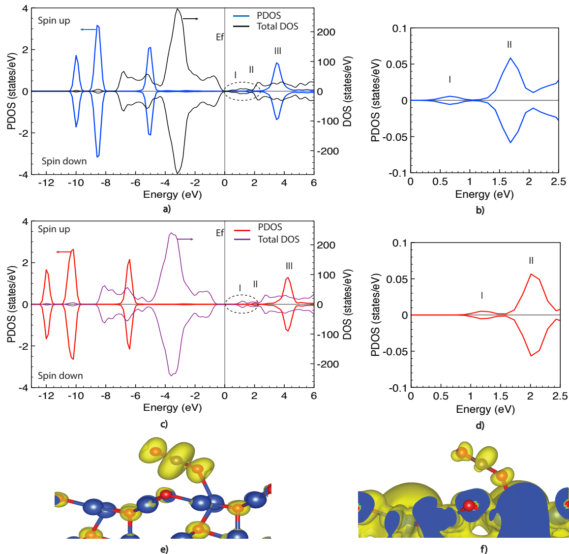
Figure 3.1.2 The projected density of state (PDOS) of CO 2 adsorbed on Cu 2 O and the total DOS calculated by PBE+U (a) and HSE06 (c). The zoom in areas from Fermi level to 2.5eV of PDOS are shown in b) for PBE+U calculations and in d) for HSE06 calculations. The partial charge of CO 2 adsorbed on Cu 2 O (111) surface at initial state: (e) partial charge from 3.0 to 4.0 eV above
