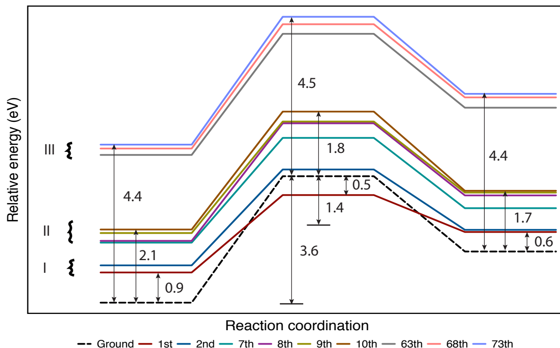
Figure 3.1.4 Ground state and excited state energies (eV) along reaction pathway predicted by the HSE06 functional combined with the \Delta SCF approach. Each colored line represents a reaction profile mapping from the initial state to the final state by manipulating electronic occupation at different electronic states above the Fermi level. Groups of I, II, III correspond to the groups of states shown in the density of states calculations.
