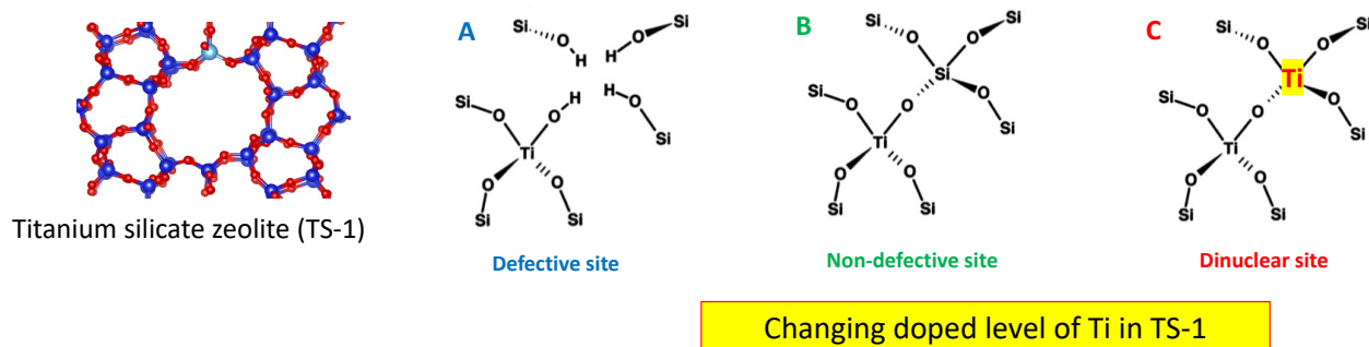
Figure 4.2.1 Illustration of different doped level of Ti in TS-1
