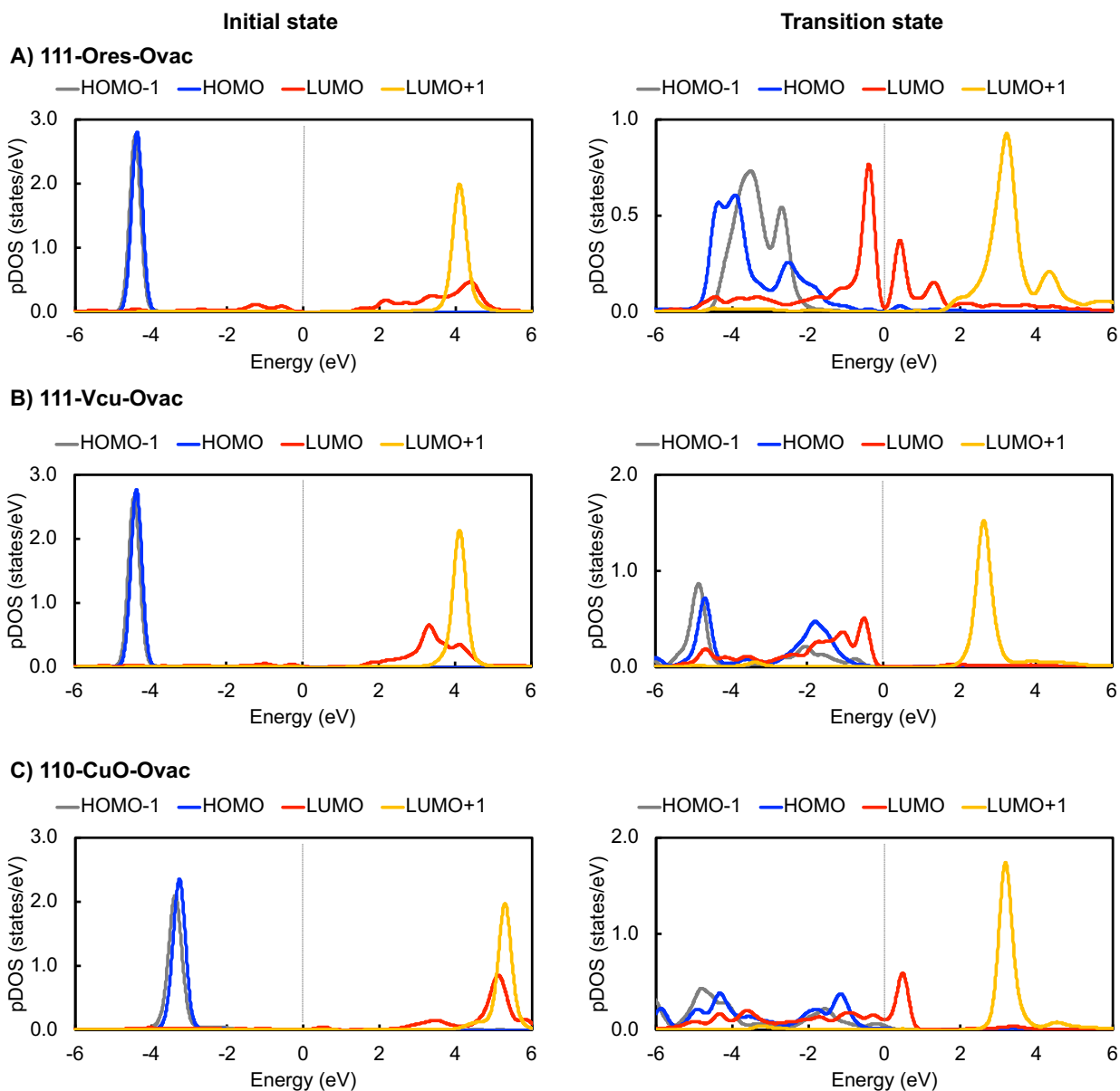
Figure 3.2.4 Projected density of states onto the \text{CO}_2 molecular orbitals at the ground level. The pDOS of \text{CO}_2 at the initial states (left) and the transition states (right) on (A) (111-Ores-Ovac), (B) (111-VCu-Ovac), and (C) (110-CuO-Ovac) surface.
