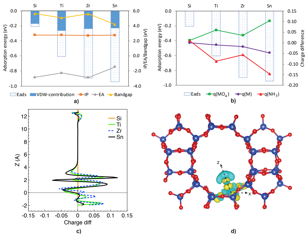
Figure 4.1.1 Calculations to explore main factors for molecular adsorption. (a) Plot of the adsorption energy of \text{NH}_3 on M-BEA together with IP, EA, Bandgap. (b) Plot of the adsorption
