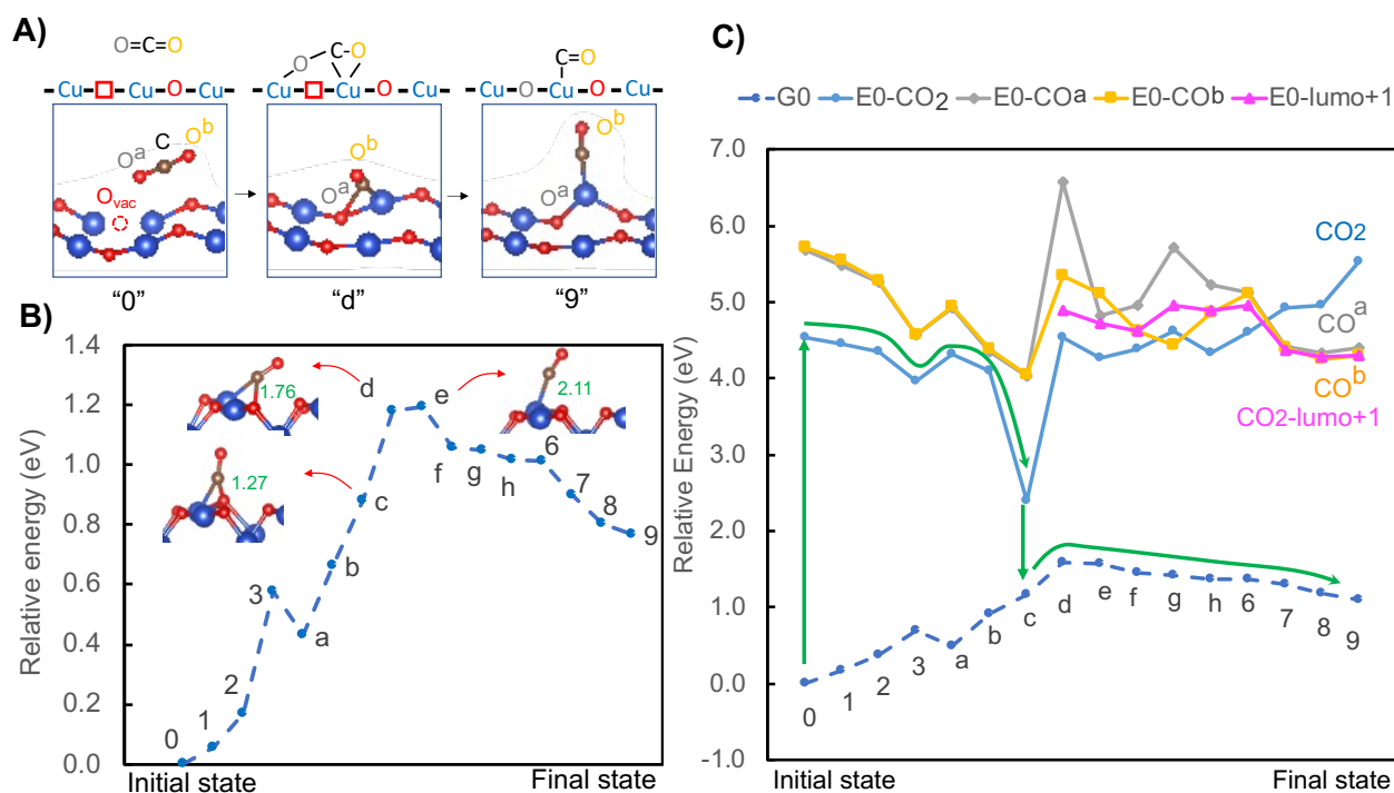
Figure 3.2.3 The CO 2 dissociation on 110-CuO-Ovac. (A) Configuration of the initial state (image 0), the transition state (image d) and the final state (image 9) with their corresponding schematic sketch (B) Ground-state energy profile calculated by VASP. The initially selected images (0-9) were further expanded between image 4 and 5 to form additional eight images (a-h). The C-O a bond length is marked in green (Unit Å) (C) Energy profile at excited states when an
