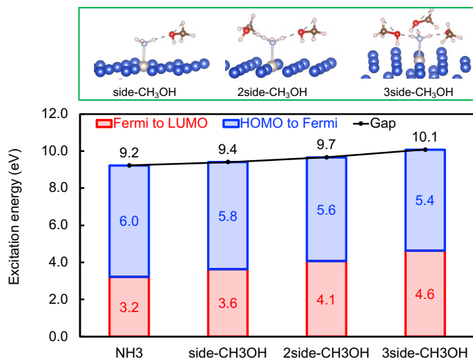
Figure 5.3 The effect of \text{CH}_3\text{OH} . The excitation energy to excite electron from HOMO of \text{NH}_3 to Fermi level (blue), excite electron from Fermi level to LUMO of \text{NH}_3 (red), and the HOMO-LUMO gap (black). Optimized configuration of \text{NH}_3 only (Base case, black), \text{NH}_3 with \text{CH}_3\text{OH} (Green) on \text{RuCu}_{83} are shown in the top channel.
