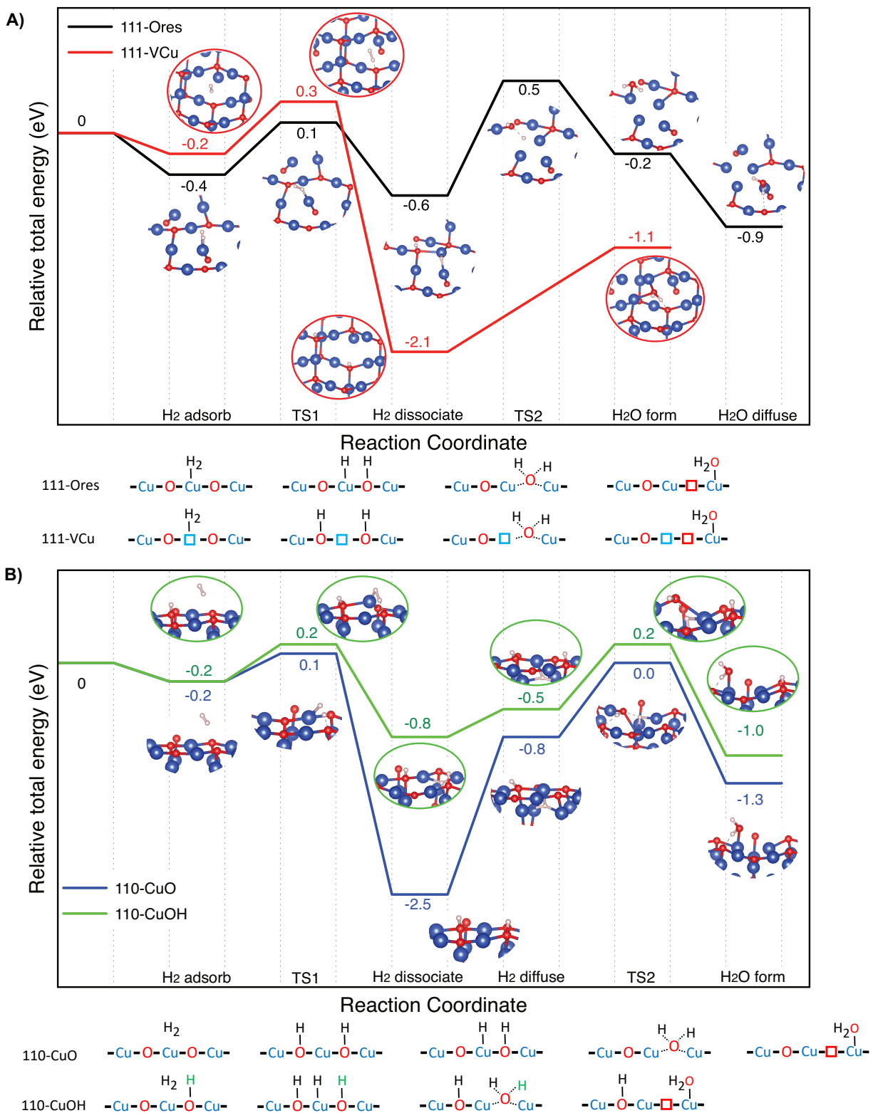
Figure 3.2.5 Energy diagram of oxygen vacancy formation by hydrogenation on Cu 2 O. (A) (111-Ores) and (111-VCu); (B) (110-CuO) and (110-CuOH).
