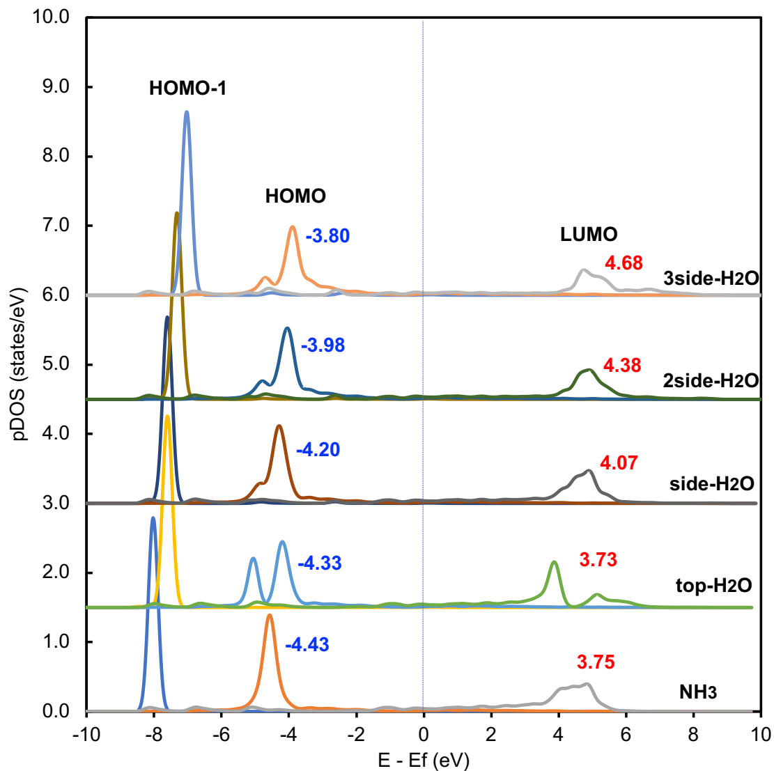
Figure 5.2 Density of states projected on adsorbed \text{NH}_3 when only \text{NH}_3 adsorbed on \text{RuCu}_{83} (and \text{NH}_3 with \text{H}_2\text{O} ). The center of the HOMO and LUMO of \text{NH}_3 are shown above the main peak.
