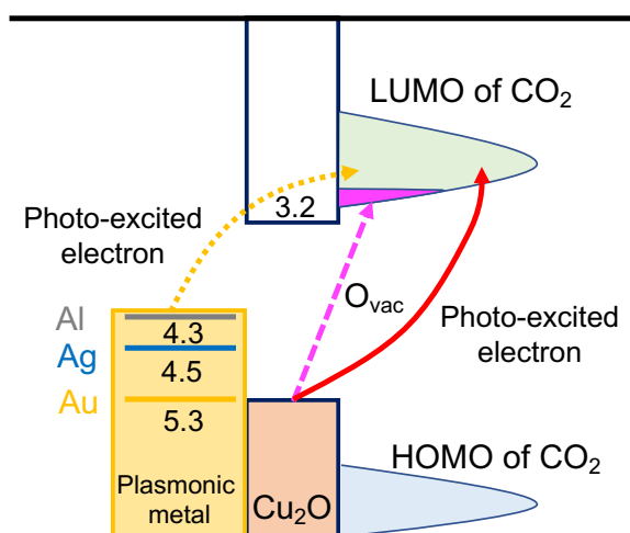
Scheme 1: Illustration of how combination of the excess electrons localized at the oxygen vacancy and photo-excited energetic electrons can populate the unoccupied molecular states and promote the CO 2 dissociation. The mean energy of LUMO with respect to the Cu 2 O valence band maximum is 3.6, 3.4 and 4.8 eV for (111-Ores-Ovac), (111-VCu-Ovac) and (110-CuO-Ovac), respectively.
