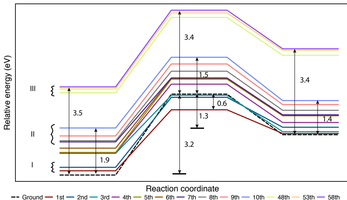
Figure 3.1.3 Ground state and excited state energies (eV) along reaction pathway obtained using the PBE+U calculations combined with the \Delta SCF approach. Each colored line represents a reaction profile mapping from the initial state to the final state by manipulating electronic occupation at different electronic states above the Fermi level. Groups of I, II, III correspond to the groups of states shown in the DOS calculations in Figure 3.2. The excitation at the initial, transition and final states are labelled for some of the vertical transitions.
