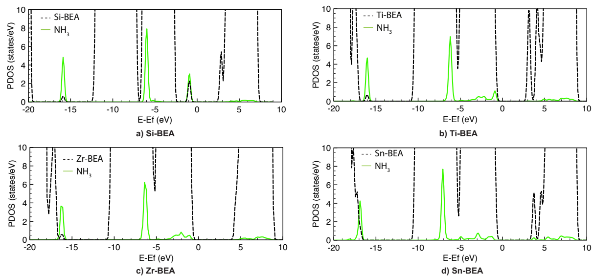
Figure A3.3 PDOS of adsorbed \text{NH}_3 (green) on M -BEA (black): a) Si-BEA b) Ti-BEA c) Zr-BEA d) Sn-BEA
