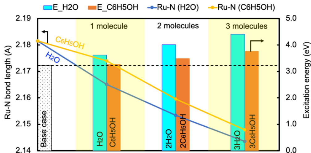
Figure 5.5 The changing of the excitation energy to excite electron from Fermi level to LUMO of \text{NH}_3 and the Ru-N bond length as the number of \text{H}_2\text{O}/\text{C}_6\text{H}_5\text{OH} molecules increased
