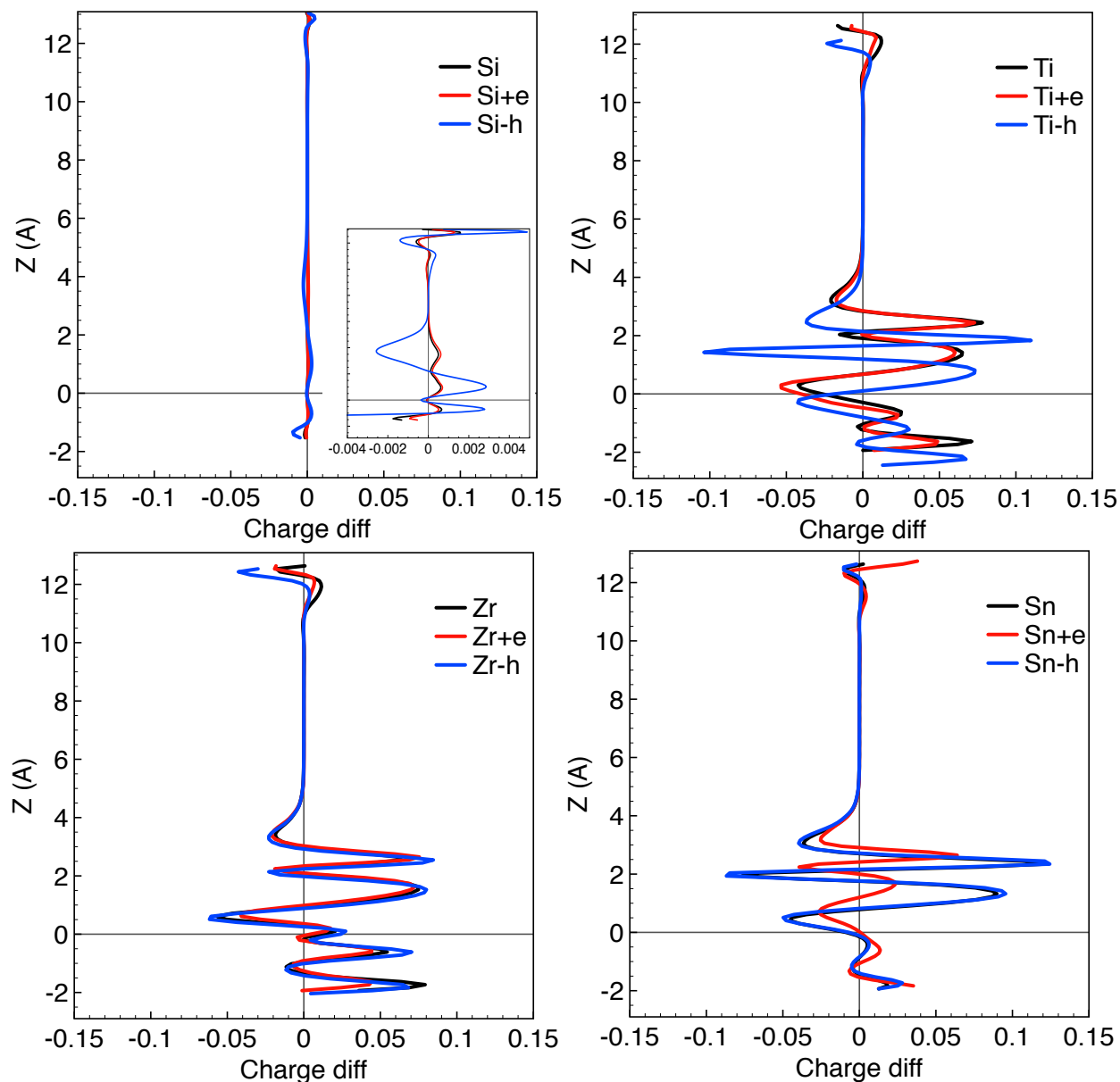
Figure A3.4 (duplicated from Figure 4 of the main text): Charge redistribution at the interface between the Lewis acid (M-BEA) and \text{NH}_3 in the z direction at the ground state (back color), at excited states with an energized electron (red color) and at excited states with an energized hole (blue color).
