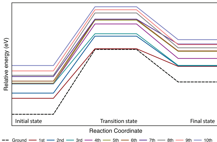
Figure A1.3 Ground state and excited state energies (eV) along reaction pathway predicted by the PBE+U functional combined with the \Delta SCF approach. Each colored line represents a reaction profile mapping from the initial state to the final state by manipulating electronic occupation at different electronic states above the Fermi level and a hole at Fermi level
