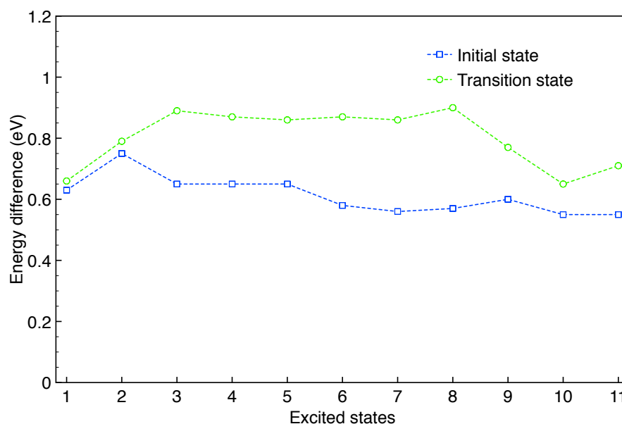
Figure 3.1.5 The energy difference of the total energies between the system with an added electron and a hole at Fermi level of \text{Cu}_2\text{O} and the system with an added electron only (PBE+U).
