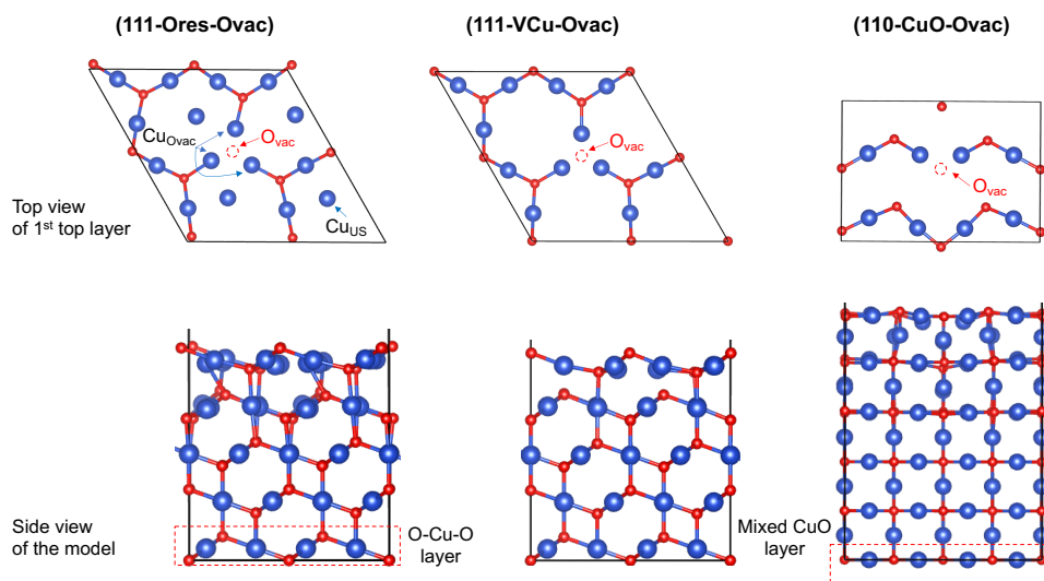
Figure A2.4 The model of the oxygen-deficient surfaces of \text{Cu}_2\text{O} . The blue and red balls denote for Cu and O atoms respectively.
