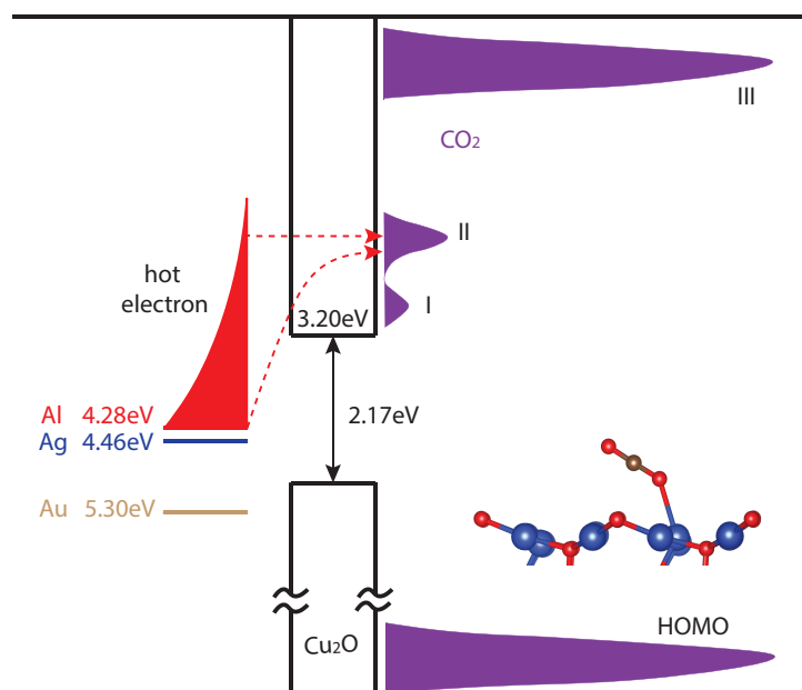
Figure 3.1.6 Possible charge transfer mechanism. The work function of Al, Ag, and Au taken from literatures 56, 58, 59
