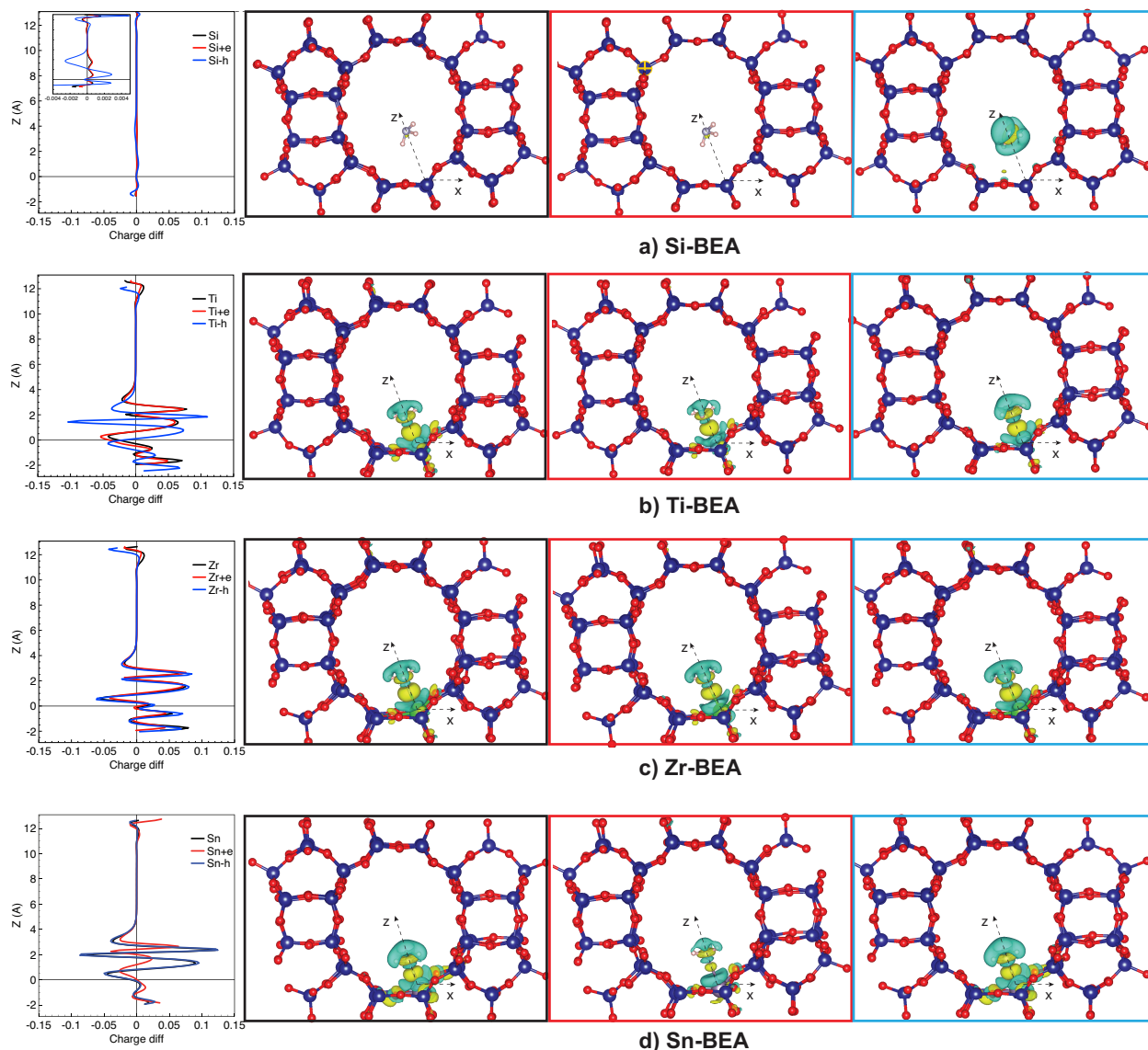
Figure 4.1.4 Charge redistribution at the interface between \text{NH}_3 and M-BEA neutral (black), M-BEA with 1 added electron (red), M-BEA with 1 removed electron (blue) for a) Si-BEA b) Ti-BEA c) Zr-BEA d) Sn-BEA. The blue, red and white balls denote Si, O and H atoms respectively.
