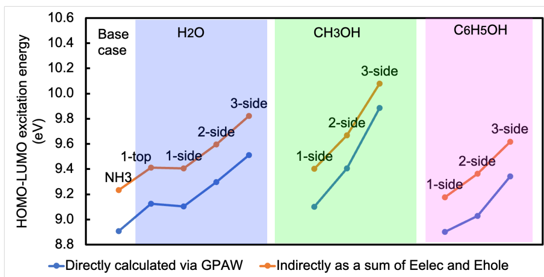
Figure A4.3 Comparison of the HOMO-LUMO gap when it is directly calculated via GPAW versus when it is indirectly calculated as a sum of E_{elec} and E_{hole} .
