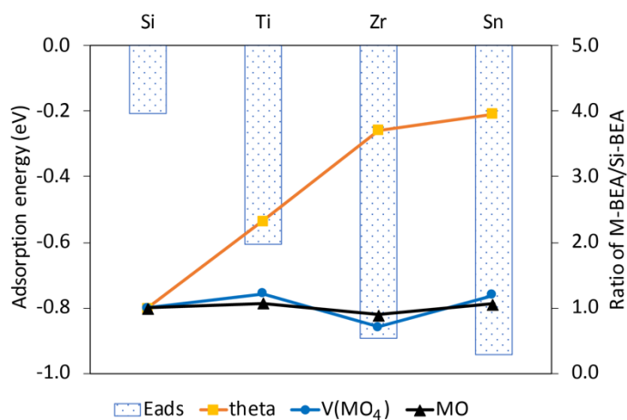
Figure A3.2 Relationship between \text{NH}_3 adsorption energy on M-BEA with the mean square deviation from regular tetrahedron angle (O-M-O angle) (theta, \theta ), the volume of tetrahedral ( \text{V}_{\text{MO}_4} ) and the average bond M-O bond length with the four oxygen nearby metal center.
