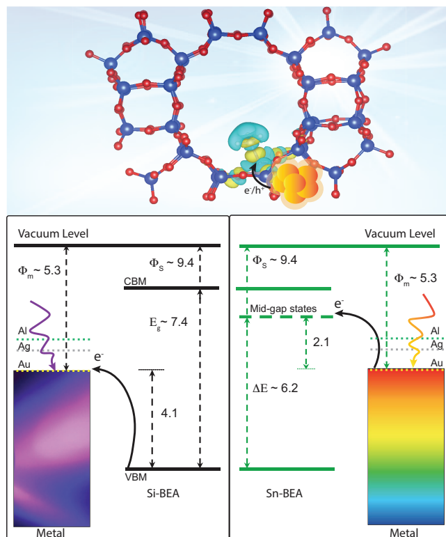
Figure 4.1.6 Electron excitation to the conduction band edge and mid-gap states in Si-BEA and Sn-BEA. The work function of pure silica form of BEA is obtained from the work function of \text{SiO}_2 polymorph of ZSM-5 124 , and the work function of Au is taken from literature 58 . Units are eV.
