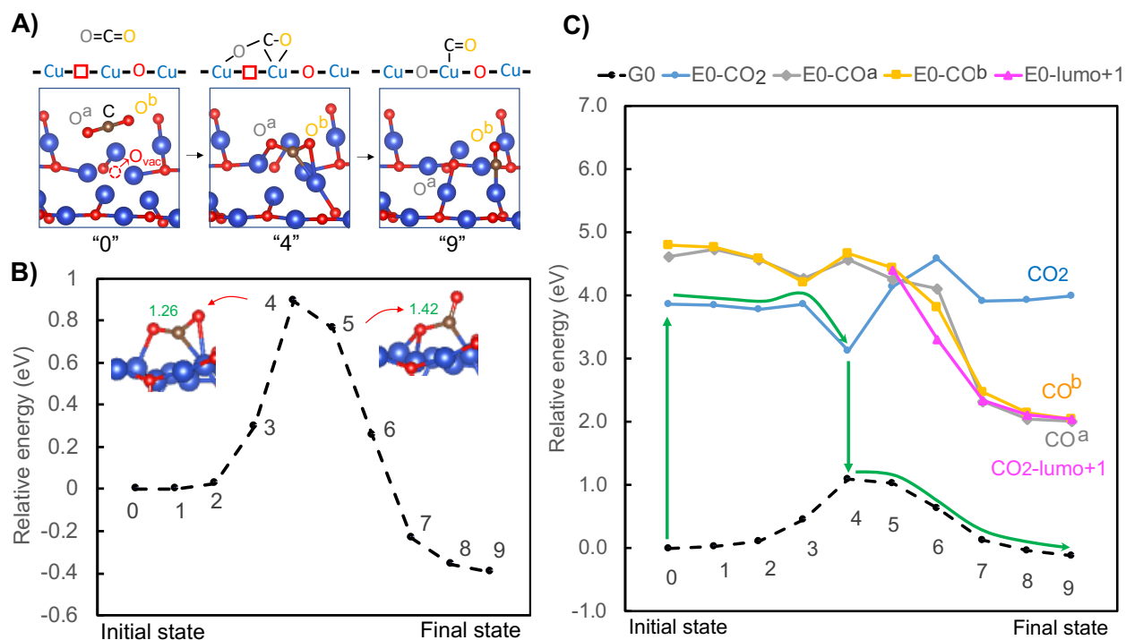
Figure 3.2.1 The CO 2 dissociation on 111-Ores-Ovac. (A) Configurations of the initial state (image 0), the transition state (image 4), the final state (image 9), and their corresponding schematic sketches. The two oxygen in CO 2 is labeled as a and b for distinguishment. (B) Ground-state energy profile calculated over ten images (indexed 0 to 9) with VASP. The C-O a bond length is marked in green (Unit Å). (C) Energy profile at excited states, when an electron is added into the LUMO of CO 2 (blue, E0-CO 2 ), the first available antibonding state of C-O a bond (gray, E0-CO a ) or C-O b bond (orange, E0-CO b ), which are compared with the ground state (black dashed, G0); all calculated by GPAW. The magenta solid line (E0-lumo+1) is included to illustrate the case when the electron is added into the LUMO+1 of CO 2 from image 5 to 9.
