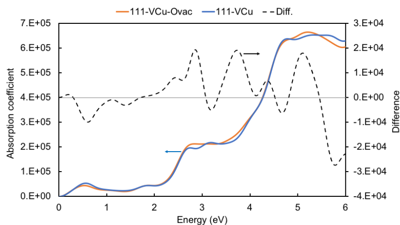
Figure A2.2 Absorption coefficient of the (111-VCu) surface with and without oxygen vacancy. Unit: cm -1 .
