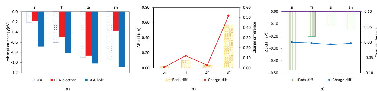
Figure 4.1.2 Adsorption of \text{NH}_3 in M-BEA with an additional electron or a hole. (a) The heat of adsorption of \text{NH}_3 on neutral M-BEA (white) compared with values with an added electron (red) and with one removed electron (blue). The relationship between the change of heat of adsorption and the electron localization on metal when (b) one electron is added into M-BEA, and (c) one electron is removed from M-BEA.
