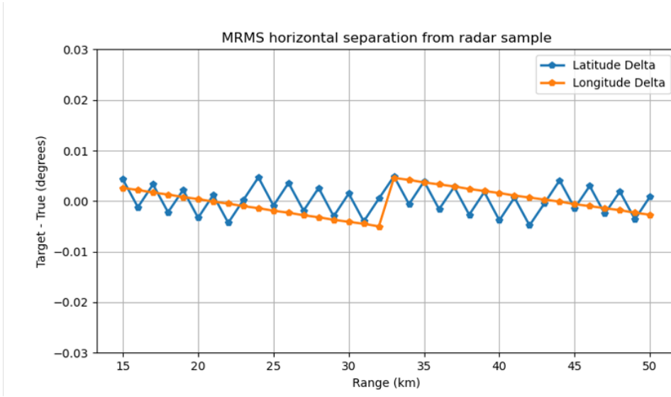
Figure 4.9: Target PAR horizontal latitude/longitude samples relative to MRMS latitude/longitude locations.
