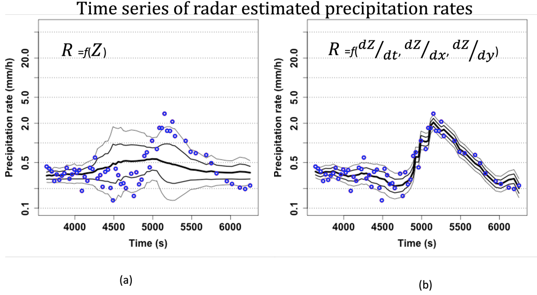
Figure 4.21: Time series of rain rate estimation results showing observed and modeled values over the study period.
