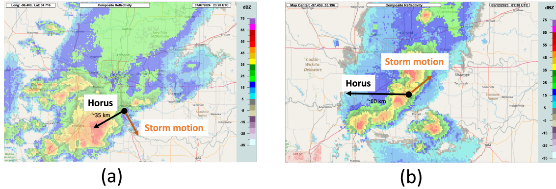
Figure 3.2: (a) Event 1 on July 7, 2024 at 23:20 UTC (b) Event 2 on May 12, 2023 at 1:38 UTC
