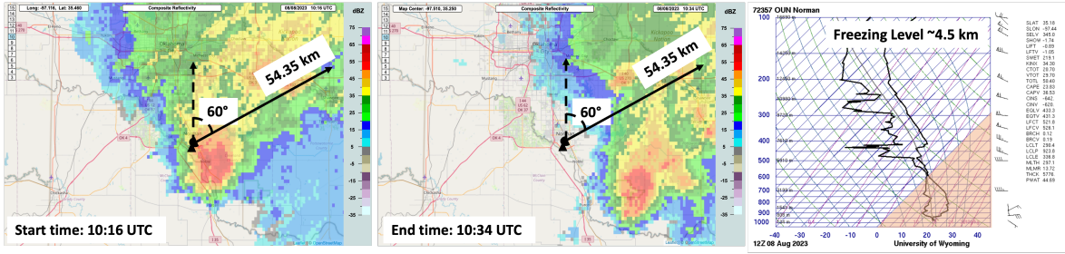
Figure 4.8: A composite Z extracted from the MRMS operational product viewer shows the spatial coverage of the frontal system near Norman, Oklahoma (USA), on August 8, 2023, that contained localized hail at (a) the measurement start time of 10:16 UTC, (b) the measurement end time of 10:34 UTC (National Severe Storms Laboratory, NOAA (2024)), and (c) a sounding taken at 12 UTC in Norman revealing a freezing level near 4.5 km (University of Wyoming Department of Atmospheric Science (2023)).
