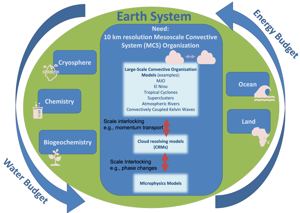
Figure 1.2: Inspired by the work of Moncrieff (2010), this figure shows the interconnected Earth-system components that collectively influence atmospheric processes. While past work has improved understanding of the ocean, land, cryosphere, atmospheric chemistry, and biogeochemistry, a critical unresolved element is convective organization, whose feedbacks extend throughout the full range of atmospheric scales.
