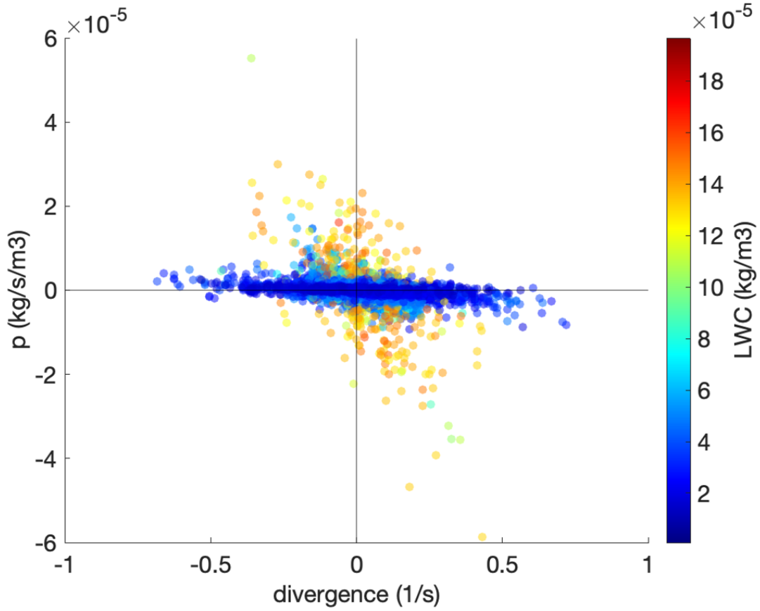
Figure 4.31: Relationship between p and the divergence of the 3D wind field. Positive divergence generally corresponds to reductions in LWC (negative p ), while negative divergence (convergence) is associated with LWC generation within the storm.
