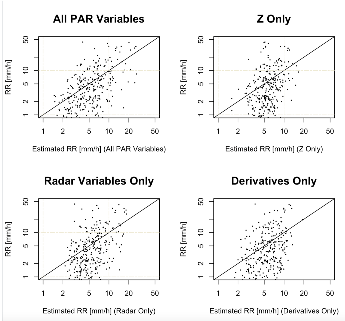
Figure 4.14: Scatter plot of MRMS R vs. estimated R for various GAMLSS-based estimators.
