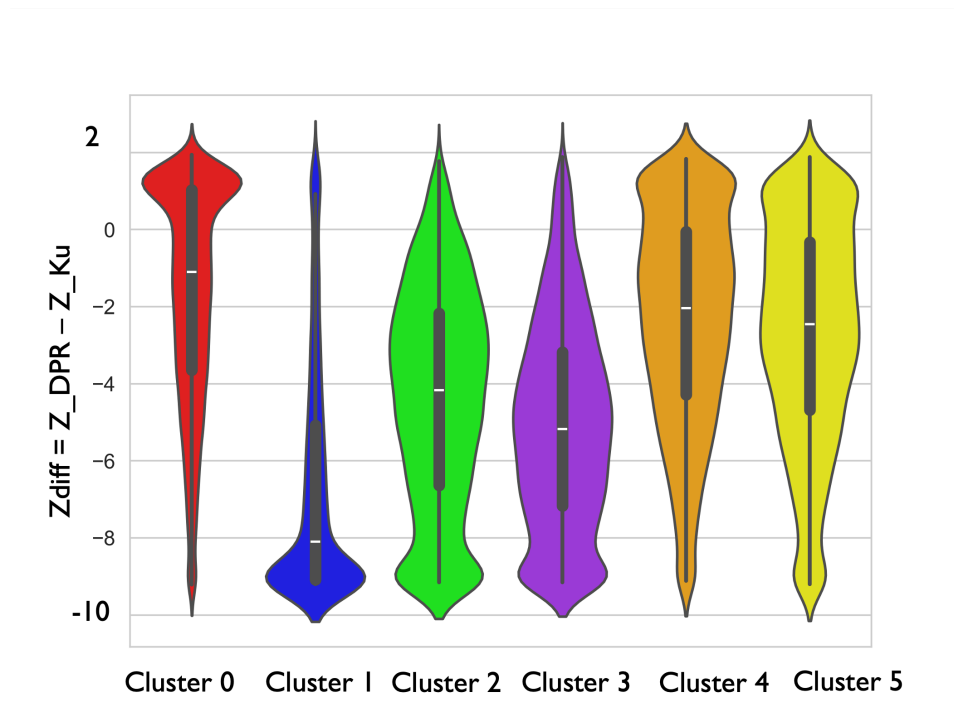
Figure 9.12: Violin plot of the difference in reflectivity between the matched scan (dependent on the dual-frequency algorithm) and the normal scan (Ku-only) reflectivities for each convective cluster.
