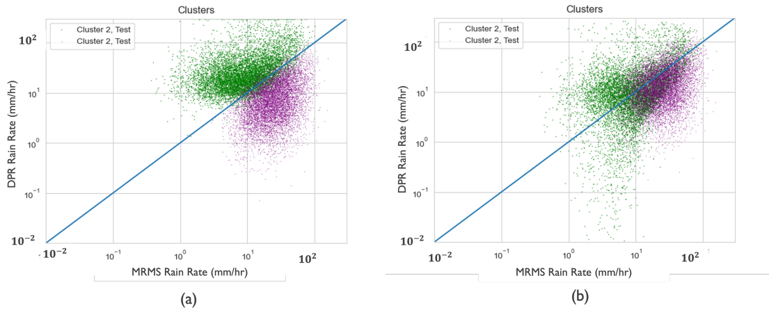
Figure 9.10: (a) Rain rate bias plots of Cluster 2 (green) and Cluster 3 (purple) and (b) after NUBF correction was applied allowing Cluster 2 to take the value of each individual data points lower 75th confidence bound for rain rate and allowing Cluster 2 to take the upper bound of each points confidence interval. A reduced RR bias due to NUBF correction motivates the conclusion that these clusters have biases driven by NUBF.
