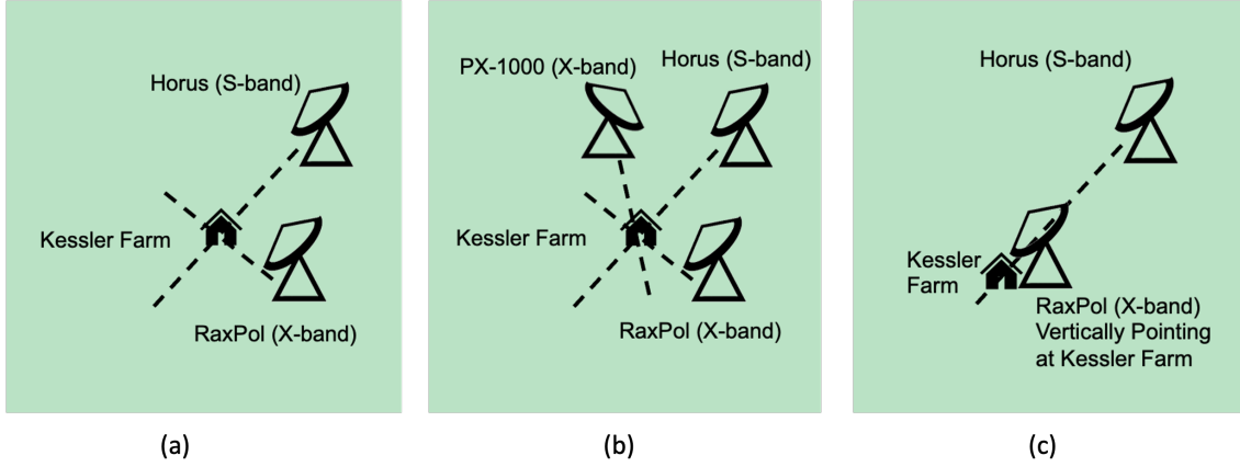
Figure 2.6: Proposed operating scenarios for the PROWEX campaign are shown including (a) a crossed scan with Horus operating with an S-band RHI crossed with RaXPol operating orthogonally with an RHI, (b) RaXPol crossing paths in an RHI with both Horus and PX-1000, and (c) Horus RHIs crossed with a vertically pointing RaXPol at the location of the reference precipitation observation at KAEFS.
