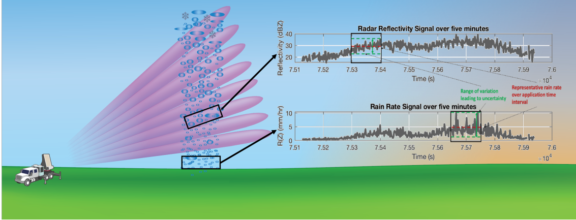
Figure 3.1: RHI observation depiction showing five minutes of radar reflectivity data collected every 0.76 s by the Horus phased array radar on July 7, 2024. Applications like QPE or validation with in-situ instruments require averaging the true underlying continuous signal over an application time domain, depicted by a box surrounding 30 s of data. Within this application interval, a representative value is shown with a red dashed line along with an uncertainty range delineated with dashed green lines. Any instantaneous observation taken to represent the interval may lack representativeness due to the underlying signal’s range of variation within this time domain.
