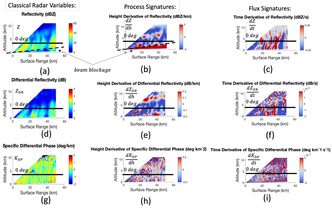
Figure 4.5: Radar variables (a) Z , (d) Z_{DR} , and (g) K_{DP} (left column) as well as their altitude derivatives (center column; (b) dZ/dh , (e) dZ_{DR}/dh , and (h) dK_{DP}/dh ) and their time derivatives (right column; (c) dZ/dt , (f), and (i) dK_{DP}/dt ) from time 10:19:61 UTC on August 8, 2023 near Norman, Oklahoma. The 0° C isotherm is marked by a horizontal black line at 4.5 km in altitude. An angled dashed black line marks a zone of near-surface beam blockage in sub-figures a and b. All variables are considered to be quasi-continuous in space and time; each RHI scan is completed within 16 s.
