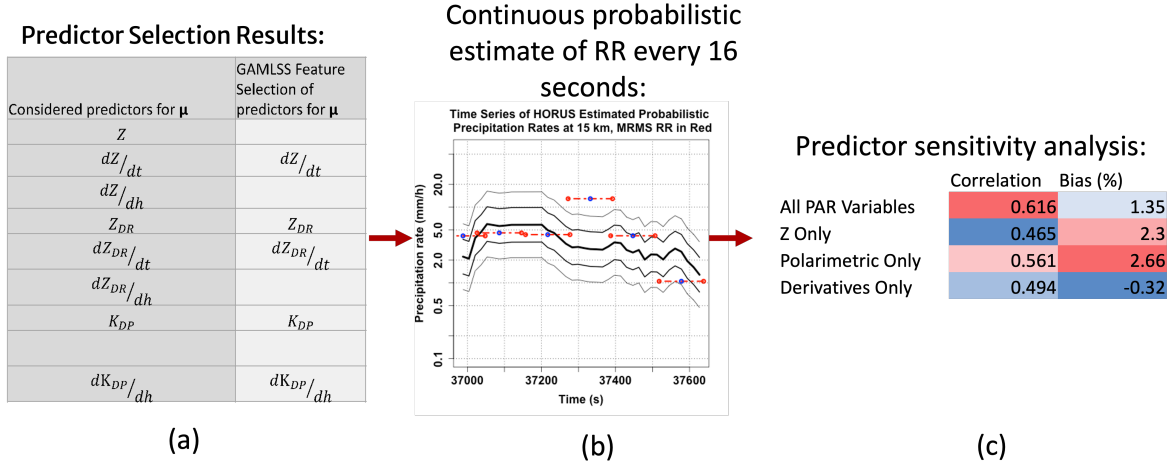
Figure 4.12: Considered and selected predictors for the estimation of mean R resulting in a trained probabilistic estimator with terms \mu(dZ/dt, Z_{DR}, dZ_{DR}/dt, K_{DP}, dK_{DP}/dh) . (a) GAMLSS is used to select these predictors and (b) generate continuous probabilistic R estimates every 16 s. (c) A predictor sensitivity analysis shows the highest correlation to be with the inclusion of all selected PAR variables. It is compared to correlations and bias metrics for estimators using predictors of Z only polarimetric variables, and derivatives only from the set of considered predictors.
