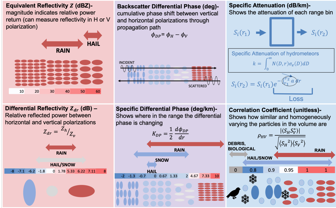
Figure 2.7: The radar variables of Z , \phi_{dp} , A , Z_{dr} , K_{dp} , and \rho_{hv} are conceptually summarized. Z is sensitive to the size of the drops, as this impacts the magnitude of the power scattered to the radar. \phi_{dp} is impacted by the cumulative size and concentration through the whole path of travel of the radar wave. A practically provides the attenuation of the radar signal by each radar bin. Z_{dr} is impacted by the size and shape of hydrometeors, as these variables depend on power reflected back for two antenna polarizations. K_{dp} is the range derivative of \phi_{dp} showing how \phi_{dp} changes for each radar bin. \rho_{hv} is close to a value of 1 for volumes with particle homogeneity in returns for both polarizations. (Content from this figure has been adapted from material in Basara (2022))
