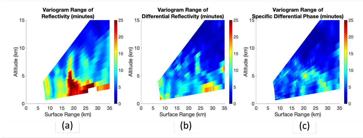
Figure 5.3: Horus decorrelation time of (a) Z , (b) Z_{DR} , and (c) K_{DP} over a variogram fit in time from 23:19:21 UTC to 23:59:59 UTC
