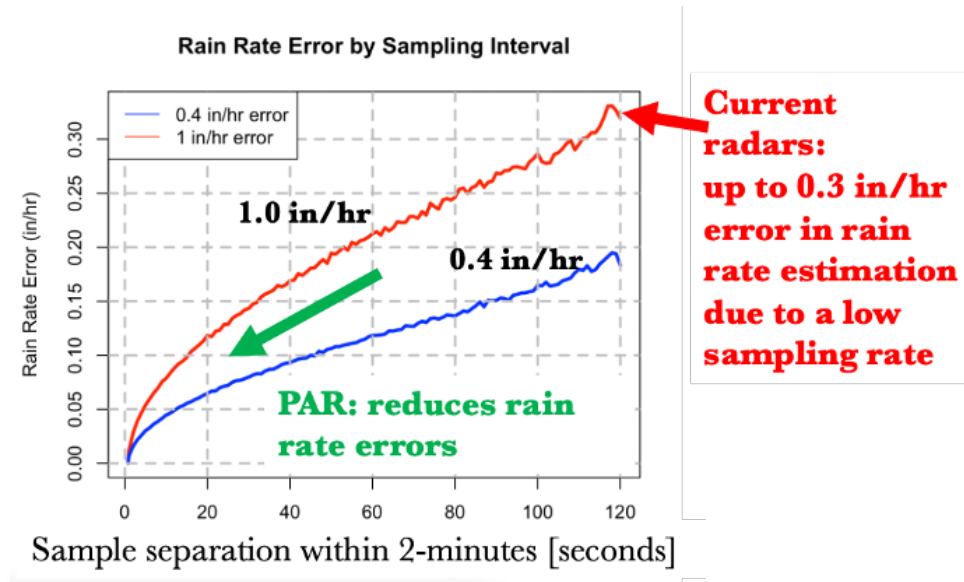
Figure 1.5: Rain-rate error versus sampling interval. Faster PAR sampling reduces error from about 0.3 to 0.15 when the true rain rate is 1 in/hr .
