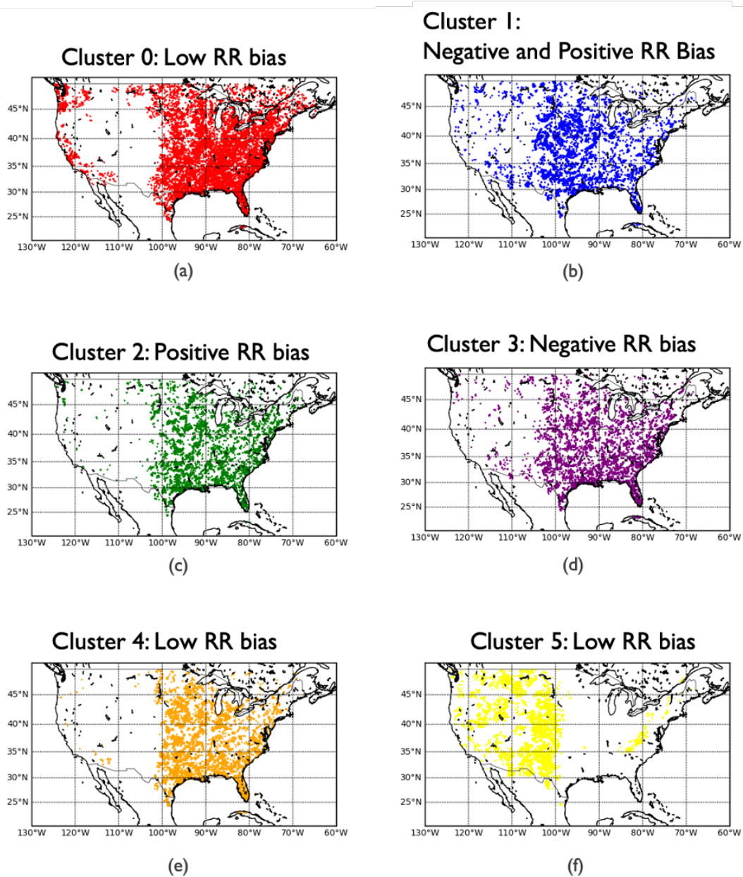
Figure 9.7: Spatial distribution of convective k-means clusters over CONUS.
