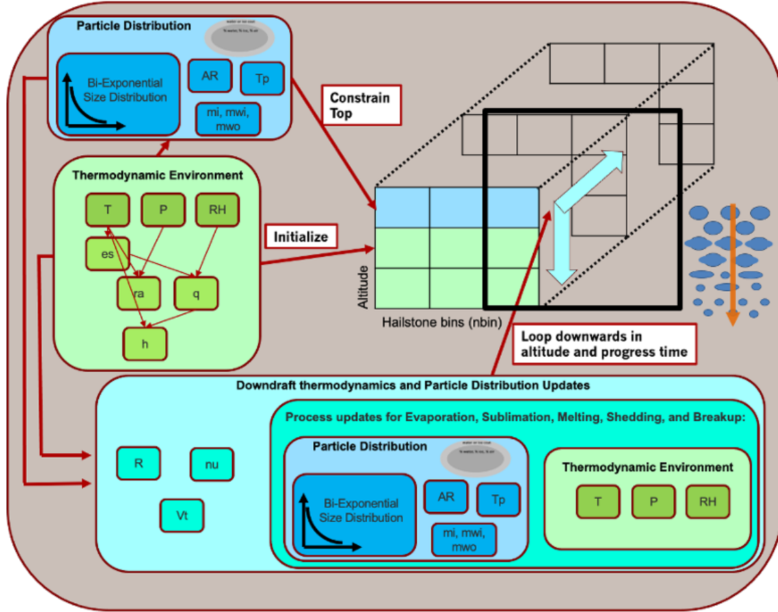
Figure 2.8: Microphysical processes evolve as a function of time and height. For the 1D SBM model, a distribution of hydrometeors is set at some altitude in an initial thermodynamic environment defined by temperature ( T ), pressure ( P ), and relative humidity ( RH ). Then the model steps forward in time and progresses downwards in altitude as the particles fall. At each altitude and time step the distribution and thermodynamic environment are updated as the particles undergo processes like evaporation, sublimation, melting, shedding, and drop breakup. These processes evolve as a function of time and height. Symbol Key: Axial Ratio ( AR ), Particle Temperature ( T_p ), Mass of ice ( mi ), Mass of water inside the particle ( mwi ), Mass of water on the outside of the particle ( mwo ), density of moist air ( ra ), heat ( h ), saturation vapor pressure ( es ), mixing ratio ( q ), Reynolds number ( R ), Kinematic viscosity of air ( nu ), Particle terminal velocity ( V_t )
