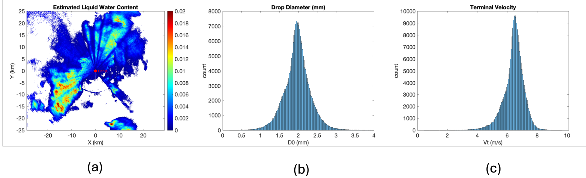
Figure 4.28: Microphysical measurement estimates derived from Horus Z and Z_{dr} at 3.78^\circ elevation on June 3, 2025. (a) PPI map of estimated liquid water content (LWC, \text{g}/\text{m}^3 ). (b) Histogram of drop diameters calculated using Equation (4.7). (c) Histogram of estimated drop terminal velocities from Equation (4.6).
