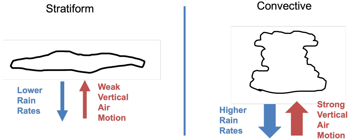
Figure 2.2: Stratiform precipitation tends to be characterized by low rain rates, less than about 10 mm/hr, and weak vertical air motion, less than about 2 m/s. Convective precipitation is characterized by higher rain rates and stronger vertical air motion (Houze Jr (1997a)).
