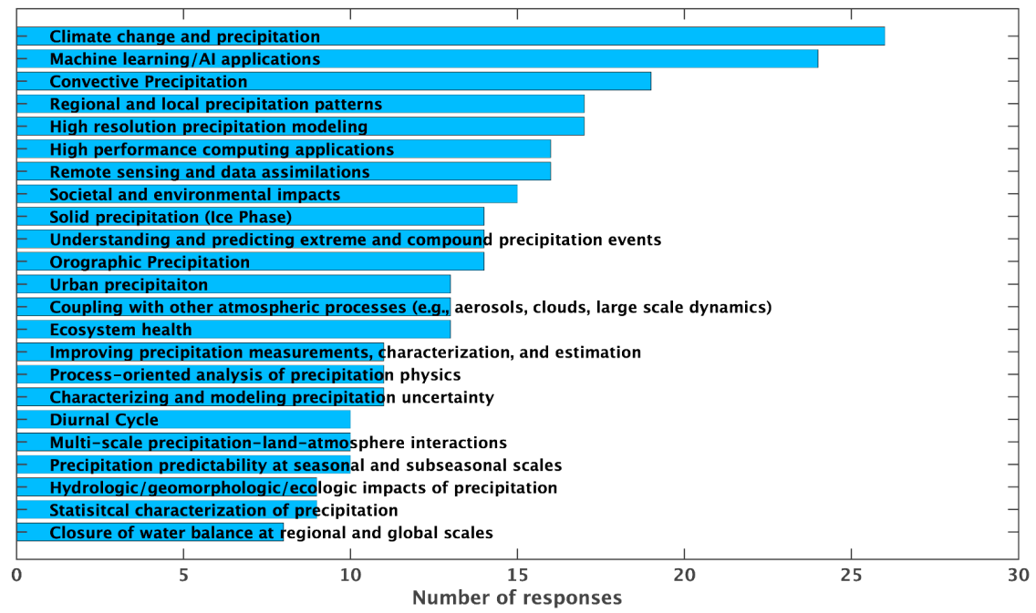
Figure 1.1: IPC-14 Student and Early Career Workshop focus areas were identified with the use of a pre-conference survey distributed to the community through advertisements to working groups and universities in the area of precipitation science.
