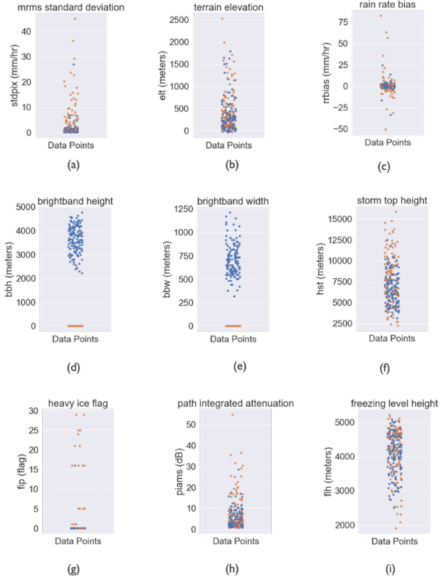
Figure 9.2: Strip-plot analysis illustrating the separation of variables between Cluster 0 (blue) and Cluster 1 (orange) through K-means clustering utilizing the full dataset, including precipitation classified as convective, stratiform with no bright band, and stratiform with a bright band. Each strip-plot depicts the distribution of a specific variable within each cluster, highlighting distinctive patterns and cluster separations, including (a) stdpix, (b) elt, (c) rain rate bias defined to be the DPR rain rate minus the MRMS rain rate at the surface, (d) bbh, (e) bbw, (f) hst, (g) fip, (h) piams, and (i) flh. For visualization purposes the plot contains a random subset of the full data set of 255,586 data points for visualization.
