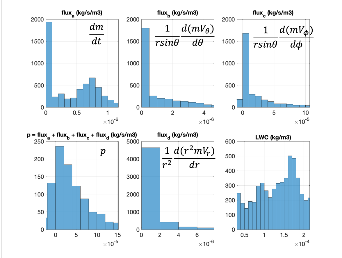
Figure 4.30: Distributions of the four flux terms used in the analysis.
