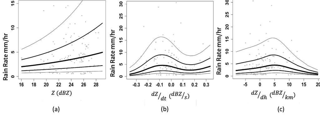
Figure 4.19: Reflectivity ( Z ), the time derivative of reflectivity ( dZ/dt ), and the height derivative of reflectivity ( dZ/dh ) are derived from PX-1000 radar profiles.
