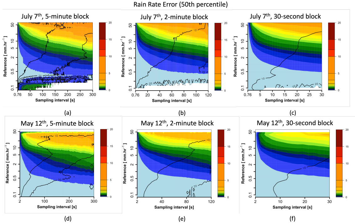
Figure 3.8: 50th percentile of the population of additive rain rate error |R_{reftrue} - R| with contours indicating the percent error \frac{|R_{ref} - R|}{R_{ref}} plotted verses R_{ref} (y-axis) and sampling interval \Delta t (x-axis).
