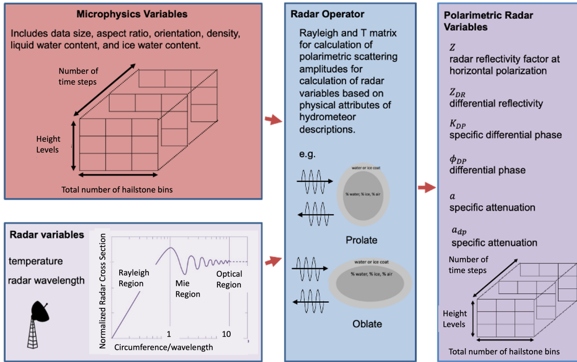
Figure 2.9: The 1D SBM model generates microphysics particle properties like particle aspect ratio, orientation, density, liquid water content, and ice water content. These, as well as radar-influencing variables like temperature and radar wavelength, are fed into the radar operator, which performs T-matrix calculations to produce simulated polarimetric radar variables.
