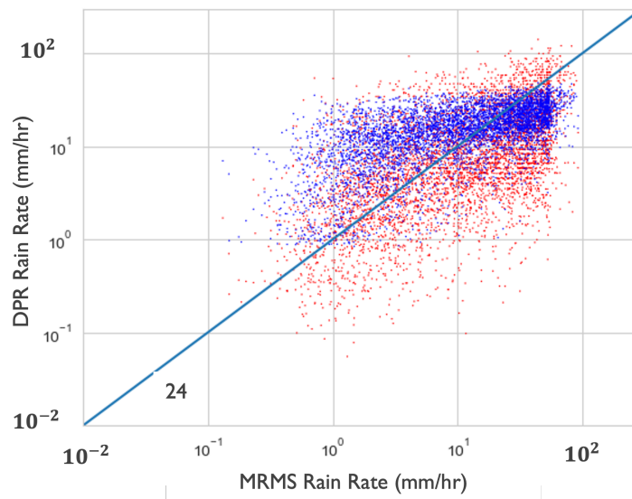
Figure 9.11: Depiction of multiple-scattering correction: red points indicate a subset of Cluster 1 from the convective dataset with a heavy ice flag greater than 20 and a difference between the DPR normal-scan reflectivity and the DPR matched-scan reflectivity greater than 6 dB. The blue points in indicate the same subset of points transformed using the Ku-band TRMM Rain Relationship as in Iguchi et al. (2000). A reduced RR bias due to multiple scattering correction motivates the conclusion that these clusters have a population of datapoints with biases driven by multiple scattering.
