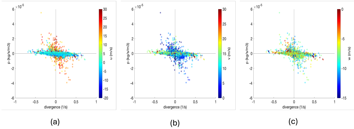
Figure 4.33: Dependence of p on wind magnitude. Strong positive horizontal winds combined with small or near-zero vertical winds are associated with large process rate magnitudes. This is consistent with the flux analysis in Figure 4.30a,b, which shows horizontal advection as the dominant contributor, while vertical motions (especially strong downdrafts) also influence the process rates, as seen in Figure 4.30c.
