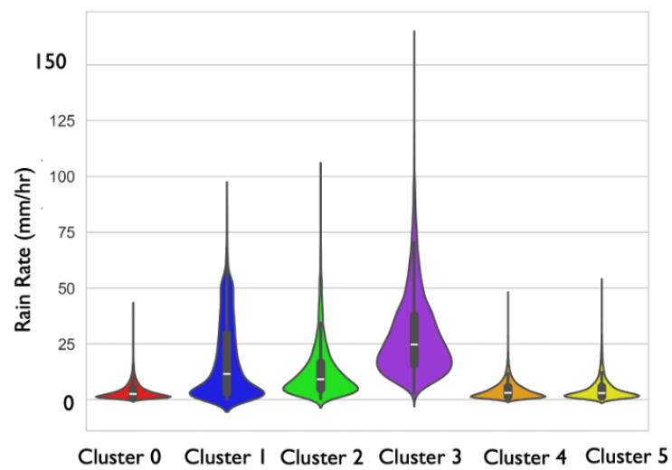
Figure 9.6: Violin plots showing MRMS rain rate (mm/hr) associated with each convective cluster.
