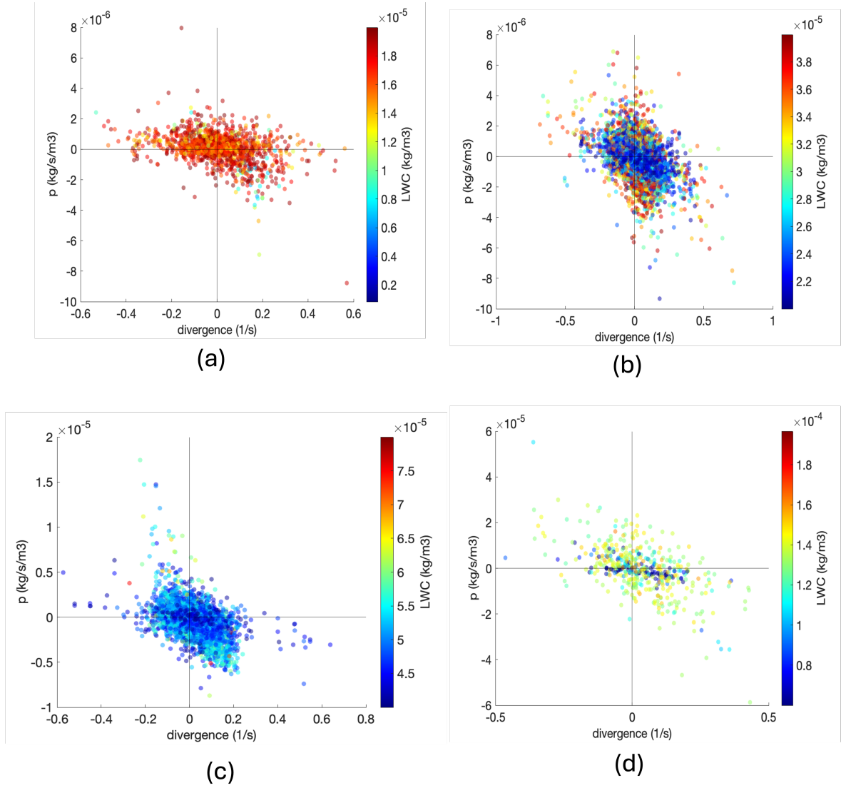
Figure 4.32: Dependence of the p -divergence relationship on liquid water content (LWC). Panels show the relationship for different LWC ranges (kg/m): (a) 0.1 \times 10^{-5} < \text{LWC} < 2 \times 10^{-5} , (b) 2 \times 10^{-5} < \text{LWC} < 4 \times 10^{-5} , (c) 4 \times 10^{-5} < \text{LWC} < 8 \times 10^{-5} , and (d) 8 \times 10^{-5} < \text{LWC} < 20 \times 10^{-5} . These subsets illustrate that the mass generation trend varies with LWC magnitude.
