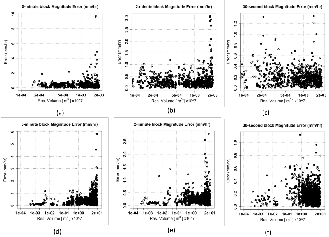
Figure 3.9: 50th percentile of rain rate magnitude error (mm/hr, y-axis) versus resolution volume ( m^3 * 10^7 , x-axis in log-scale). July 7 th with T = (a) 5 min, (b) 2 min, and (c) 30 s. The rain rate error for the observed event on May 12 th is also shown for T = (d) 5 min, (e) 2 min, and (f) 30 s.
