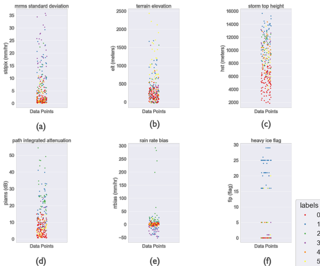
Figure 9.5: Strip-plot analysis illustrating the separation of variables between Cluster 0 (red), 1 (blue), 2 (green), 3 (purple), 4 (orange), and 5 (yellow) through K-means clustering utilizing only datapoints from the full dataset classified as convective. Each strip-plot depicts the distribution of a specific variable within each cluster, highlighting distinctive patterns and cluster separations, including (a) stdpix, (b) elt, (c) hst, (d) piams, (e) rain rate bias defined to be the DPR rain rate minus the MRMS rain rate at the surface, and (f) fip. For visualization purposes the plot contains a random subset of the full data set of 61,302 convective data points for visualization. This visual analysis provides insights into the role of individual variables in defining cluster boundaries and identifying key features that distinguish clusters within the dataset.
