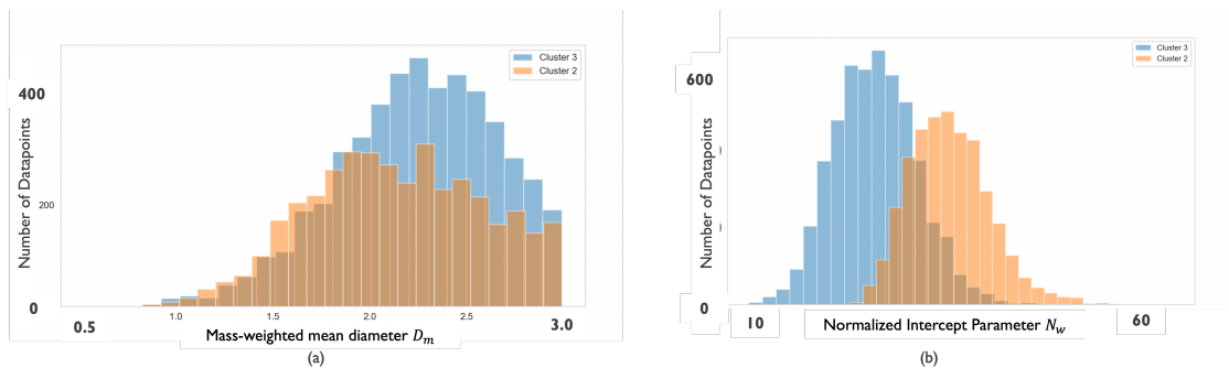
Figure 9.8: Separation between Cluster 2 and Cluster 3 in (a) D_m and (b) N_w
