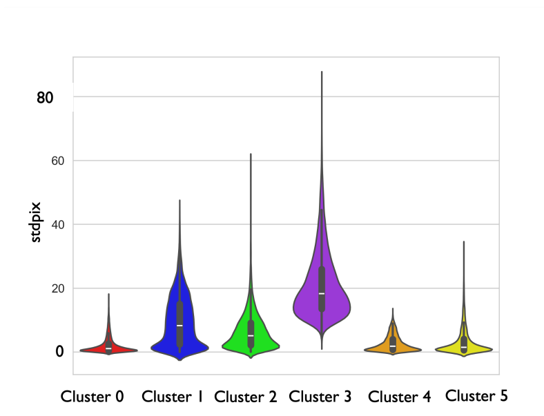
Figure 9.9: Violin plots showing MRMS standard deviation (mm/hr) associated with each convective cluster from Section 3b.
