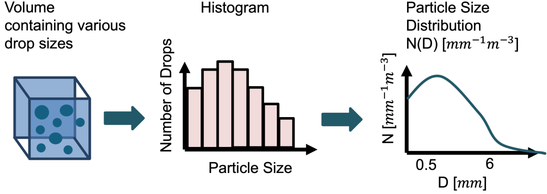
Figure 2.3: Within an observed volume of space (e.g., radars illuminate volumes of space), particles come in many shapes and sizes (e.g., with different equivalent diameters, D ). The PSD represents the number of drops of each diameter. In microphysics models, this can be represented either as discrete diameter bins or as a continuous distribution (e.g., a gamma or exponential distribution).
