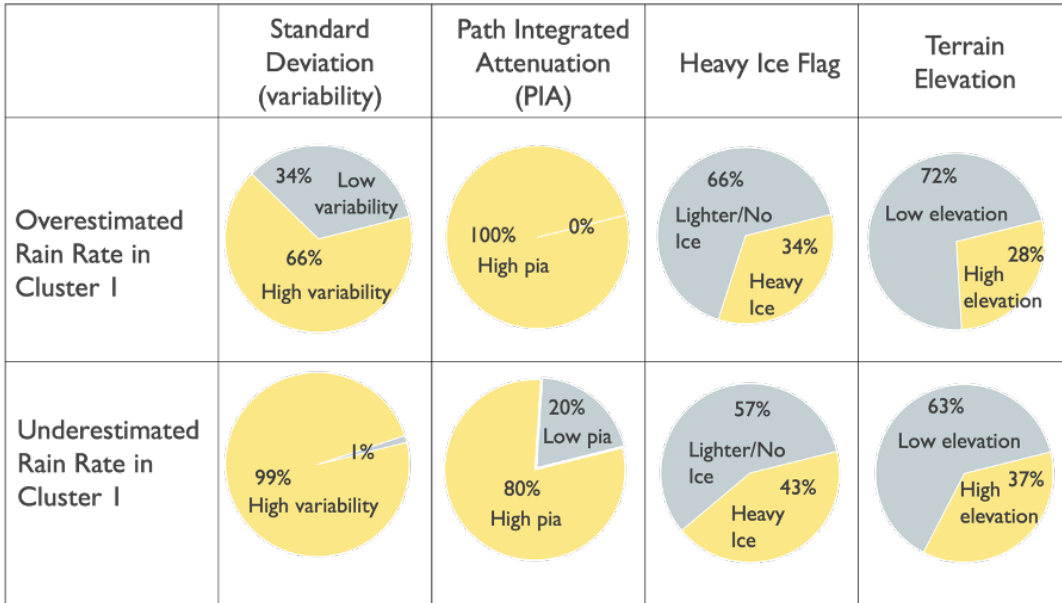
Figure 9.3: Percentage of outlier DPR observations (with a rain rate bias > 10 mm/hr) in Cluster 1 from the DPR two-year dataset associated with stdpix > 2.2 dB, indicating high R_{MRMS} variability within the DPR footprint; piams > 6.06 dB, indicating high matched scan path integrated attenuation; fip > 4 indicating heavy ice; and elt > 368 meters, indicating high elevation. Importantly, the portion of the data that is classified to be convective is shaded in yellow, motivating a further focus on convective-type precipitation in Section 3b.
