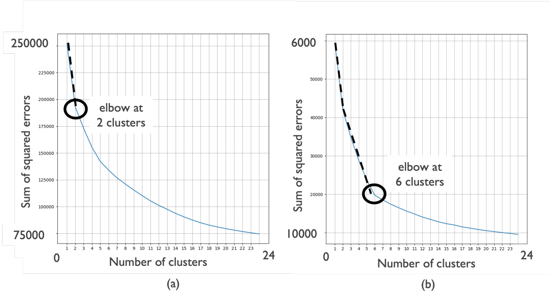
Figure 9.4: The elbow method (Kumar et al. (2011)) was used to choose the number of clusters for the K-means clustering analysis in (a) section 3a utilizing the complete dataset and (b) section 3b, a subset of the full dataset classified as convective precipitation
