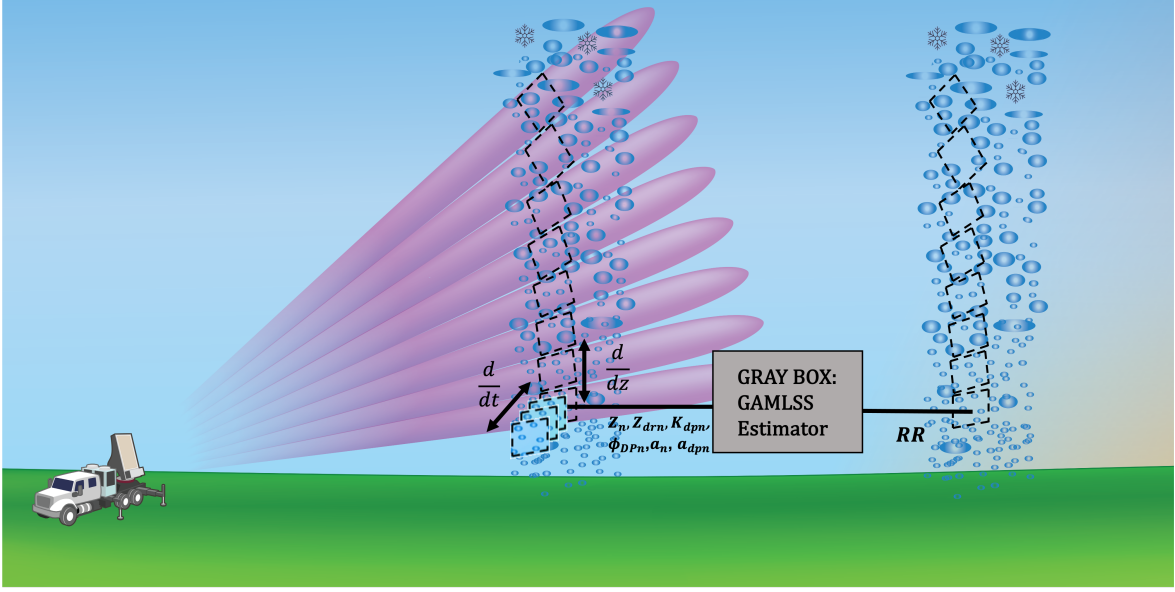
Figure 4.7: R can be derived at every range bin from PAR returns using an algorithm of choice. This work considers a probabilistic R estimate using an additive regression model to predict R from unique polarimetric PAR variables.
