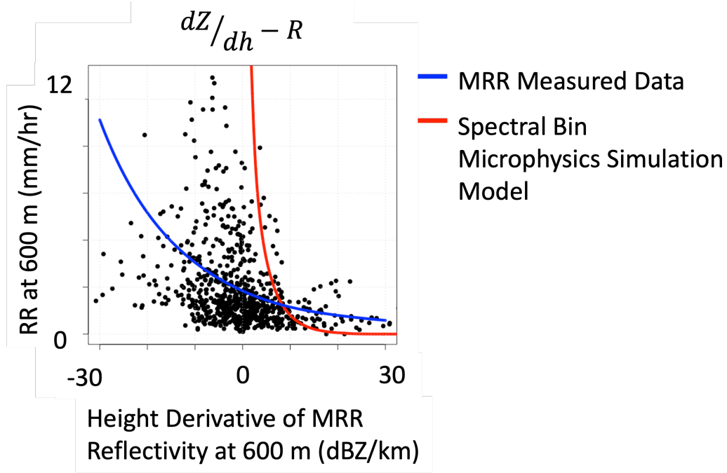
Figure 4.3: Comparison of the relationship between reflectivity height derivatives and R for observed (blue) and simulated (red) datasets. Both exhibit a power-law dependence, illustrating the consistent physical relationship between reflectivity gradients and rainfall intensity across distinct regimes. The observed curve corresponds to the warm-rain event at KAEFS, while the simulated curve corresponds to the hail-melting downdraft case from the SBM model.
