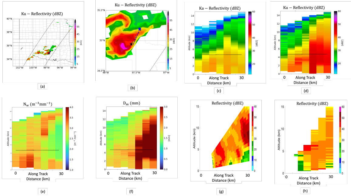
Figure 5.1: DPR attenuation-corrected Ku-band estimated surface reflectivity at 23:38:18 UTC on July 7, 2024, over (a) the DPR swath and (b) zoomed in on the location of Horus (blue dot) along with the Horus RHI extent (blue dashed line); DPR cross sections of attenuation-corrected reflectivity along the black dotted line in (b) for (c) Ka-band and (d) Ku-band; Cross sections of DPR estimated hydrometeor distribution parameters: (e) the log of the normalized intercept parameter N_w and (f) the mass-weighted mean diameter; Collocated Horus RHI S-band reflectivity (g) at native resolution and (h) resampled to the resolution of the GPM-DPR; In panels (c) to (f), the horizontal dotted lines figure the isotherm 0^\circ \text{C} altitude.
