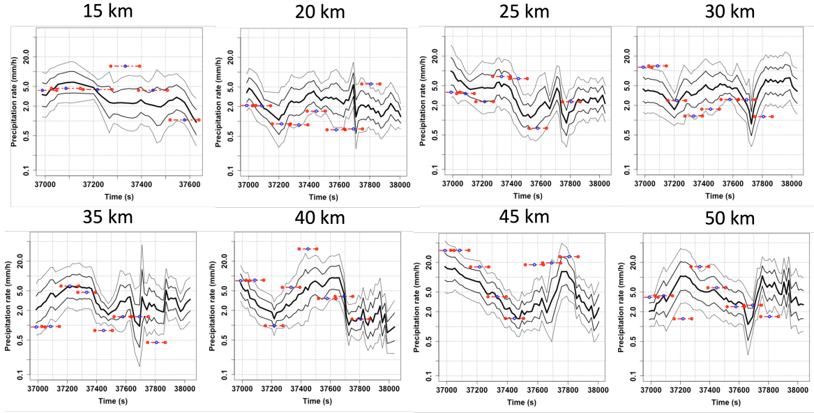
Figure 4.13: Time series of Horus estimated probabilistic QPE at various distances from the radar, including the estimated median (center black curve), 25th and 75th percentiles (inner curves), and 90th and 10th percentiles (outer curves). The included training data (MRMS gauge corrected R_s ) at each distance from the radar is marked in red and constitutes 14 percent of the total continuous MRMS data set. Error bars are overlaid on the MRMS R_s to indicate the potential for time errors by the MRMS data capture.
