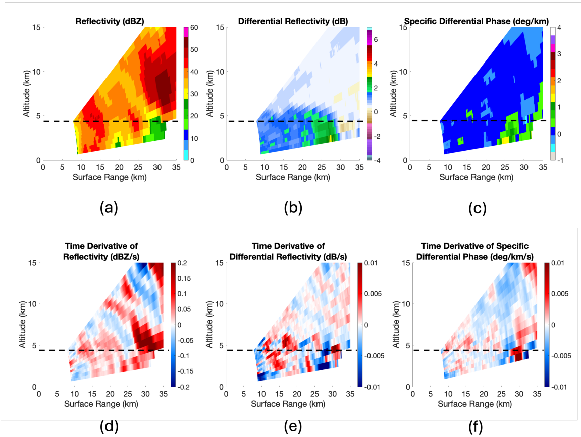
Figure 5.2: Horus snapshot of (a) Z , (b) Z_{DR} , and (c) K_{DP} as well as (d) dZ/dt , (e) dZ_{DR}/dt , and (f) dK_{DP}/dt at 23:38:18 UTC on July 7, 2024. The horizontal dotted line indicates the isotherm 0^{\circ}\text{C} altitude.
