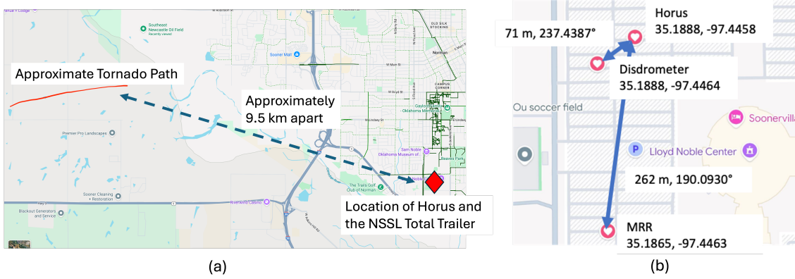
Figure 4.23: (a) Approximate path of the June 3, 2025, Norman, OK, tornado relative to the Horus radar and NSSL’s TOTAL trailer at the Lloyd Noble Center. (b) Zoomed view of the instrument deployment showing the locations of Horus and the TOTAL disdrometer. (Compilations (2025)).
