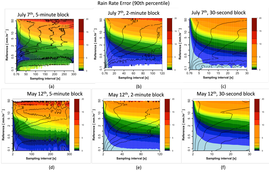
Figure 3.7: 90th percentile of the population of additive rain rate error |R_{ref} - R| with contours indicating the percent error \frac{|R_{ref} - R|}{R_{ref}} plotted verses R_{ref} (y-axis) and sampling interval \Delta t (x-axis).
