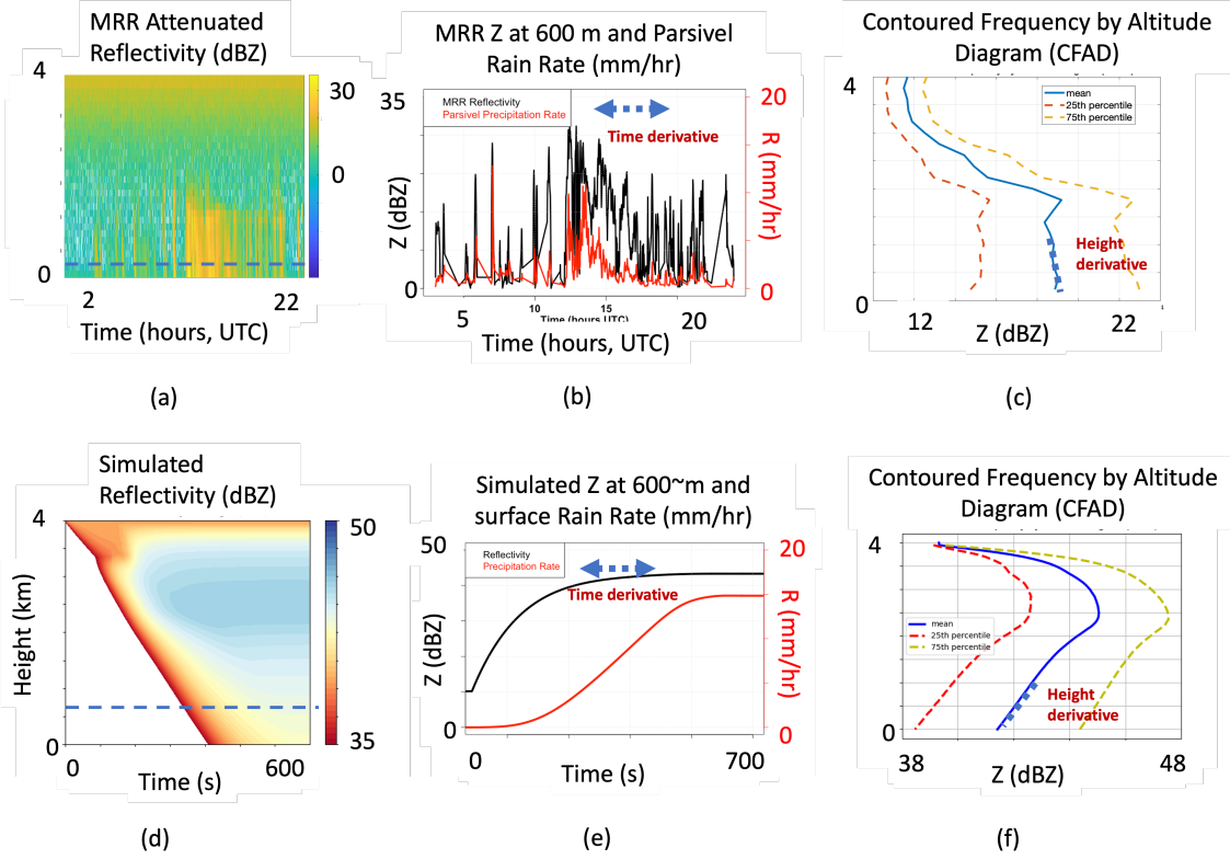
Figure 4.2: (a) The 600 m altitude at which MRR reflectivity values are extracted. (b) Overlay of MRR reflectivity and disdrometer-observed R over 24 hours. (c) CFAD showing mean, 25th, and 75th percentiles of reflectivity for the day, illustrating precipitation behavior in the time and altitude derivatives of Z . (d) Horizontally incident T-matrix-derived Z outputs at S-band from the 1D SBM for hail melting in a downdraft from 4 km to the surface over 700 s. (e) Comparison of Z extracted at 600 m with ideal surface rain rate values, and CFAD of simulated Z over 700 s.
