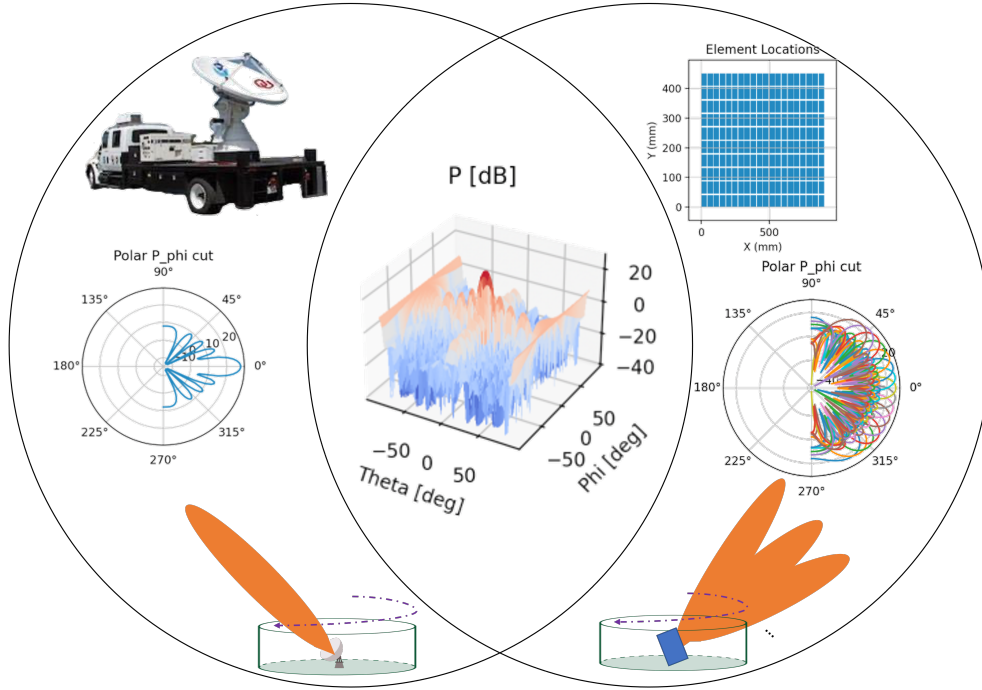
Figure 2.4: Both PAR and dish-style radars (center) are capable of focusing transmitted and received energy to achieve narrow beamwidths, can be designed as dual-polarimetric systems, and often include a radome. Traditional dish-style radars (left) feature a single transmit and receive beam that, due to mechanical steering, can take 5-6 min to complete a VCP (e.g., NEXRAD), which inherently features gaps in vertical coverage. PAR (right) can simultaneously receive any number of programmed beams to help close gaps in vertical coverage. (Dish radar image from NOAA National Severe Storms Laboratory (2025b))
