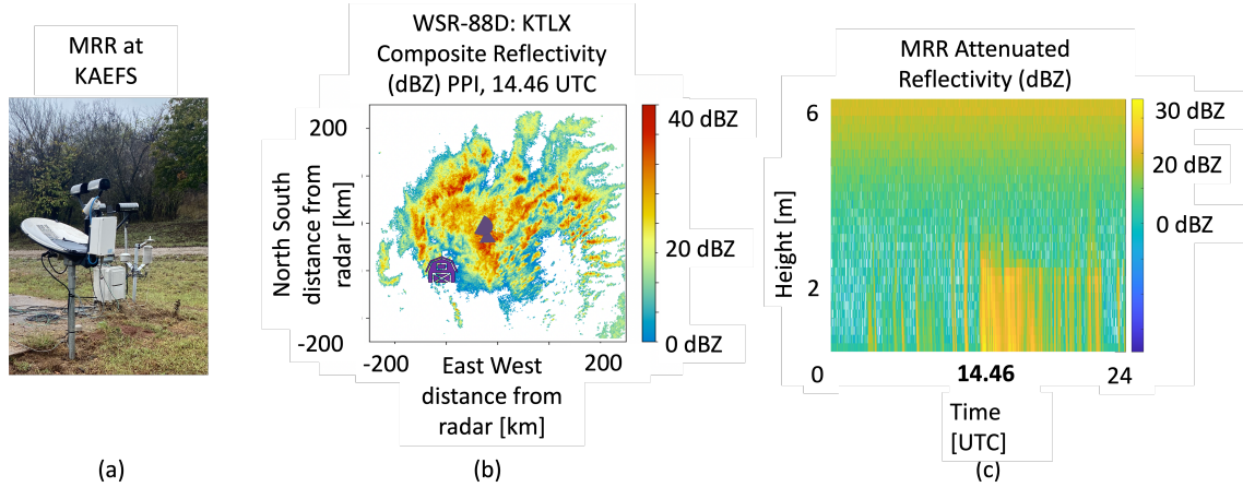
Figure 4.1: A pseudo-PAR case study conducted on October 25, 2019, using a 24 GHz FMCW Micro Rain Radar co-located with a 2DVD disdrometer and two Parsivel2 disdrometers at KAEFS. The time-resolution of both measurements was 1-minute. (a) Photograph of the measurement site, (b) KAEFS location (farm icon) on WSR-88D composite reflectivity plot with radar site shown by a radar icon, and (c) 24-hour MRR attenuated reflectivity time–height plot.
