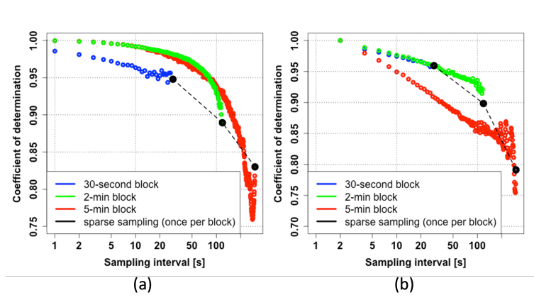
Figure 3.10: Correlation between the reference rain rate sampled at the minimum sampling interval (e.g. 0.76 s or 2 s) over T = 30 s (blue), 2 min (green), and 5 min (red) for (a) the July 7, 2024 case with a minimum sampling interval of 0.76 s and (b) the May 12, 2023 case with a minimum sampling interval of 2 s
