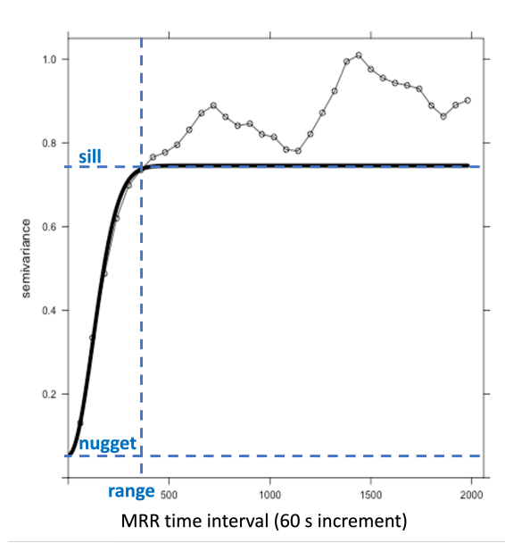
Figure 3.3: An example of a gaussian variogram model fit (bold line) to an empirical variogram compiled from a single radar range gate from MRR observations separated by interdistances from 60 s to 2000 s. The variogram metrics discussed in this chapter are marked: sill, range, and nugget.
