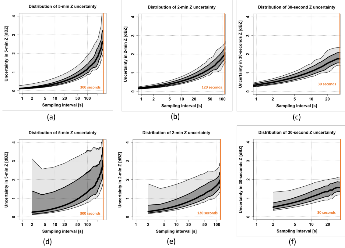
Figure 3.6: Estimates of Z uncertainty, or expected temporal observation error E_{o,t} , are shown for July 7 th over various temporal domains, T = (a) 5 min, (b) 2 min, and (c) 30 s. Estimates of Z are shown for May 12 th for T = (d) 5 min, (e) 2 min, and (f) 30 s. Shaded areas represent the 25/75th percentiles and 10/90th percentiles of the uncertainty values for all the blocks in the considered dataset.
