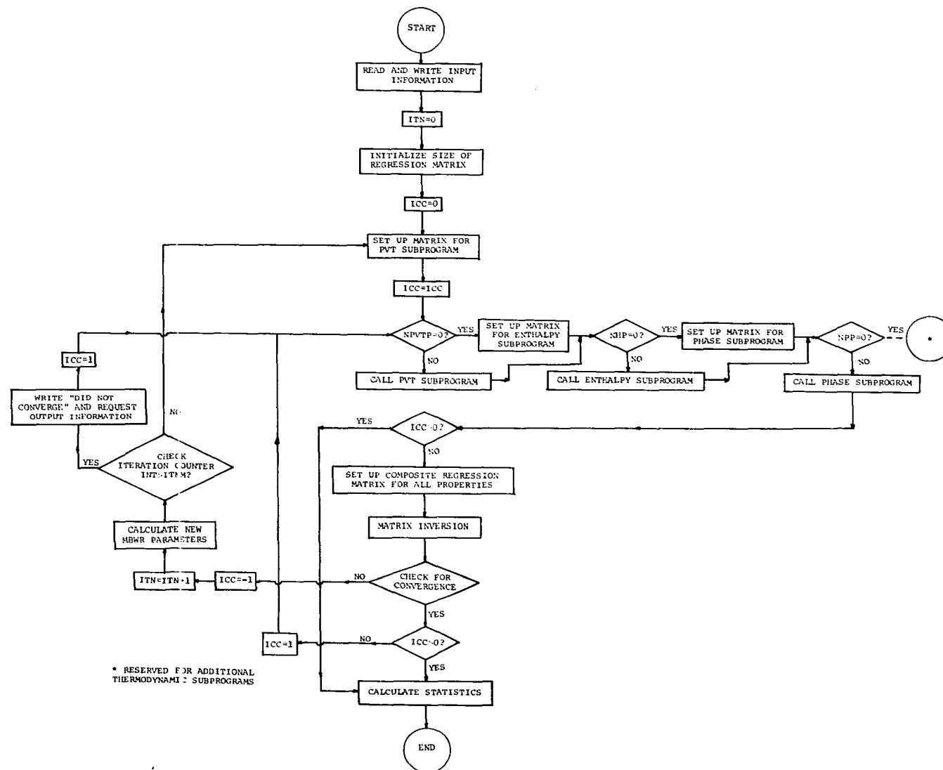
Figure 9. Flow Sheet for Main Program.
