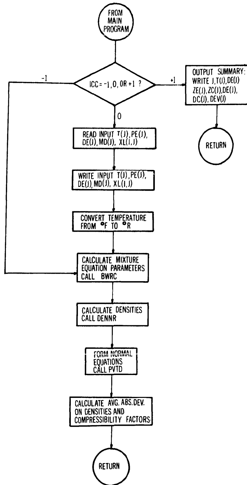
Figure 10. Flow Sheet for PVT Subprogram.
