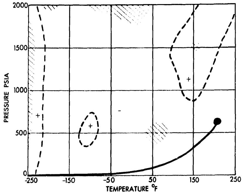
Figure 20. Comparison of Enthalpy Departures Calculated by the Modified BWR Equation with Experimental Values for Propane.
