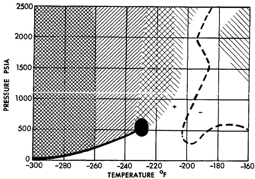
Figure 25. Comparison of Enthalpy Departures Calculated by the Original BWR Equation Using Crain and Sonntag's Parameters with Experimental Values for Nitrogen.
