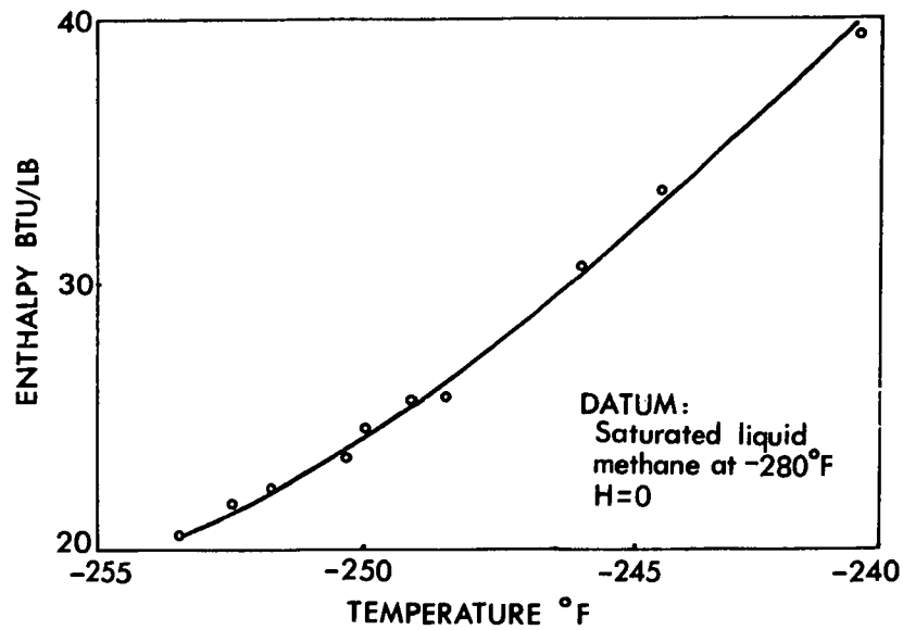
Figure 2. Enthalpies of Methane at Constant Density (0.934 lb mole/ft 3 )
