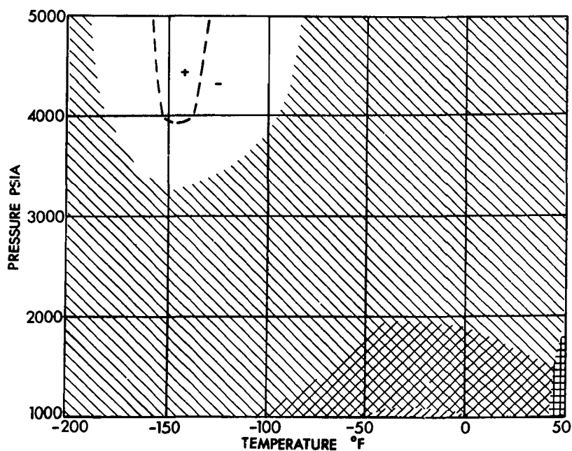
Figure 29. Comparison of Densities Calculated by the Modified BWR Equation Using Set III Parameters with Experimental Values for the 50 Mole % Propane Mixture
