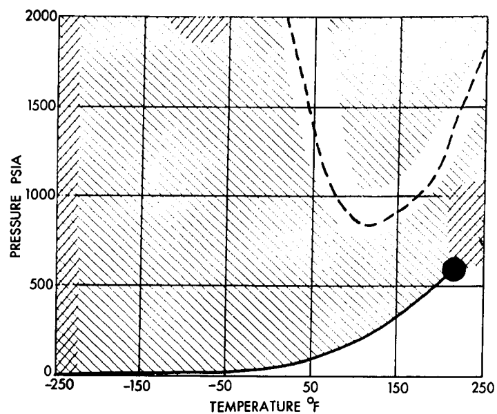
Figure 18. Comparison of Densities Calculated by the Modified BWR Equation with Experimental Values for Propane
