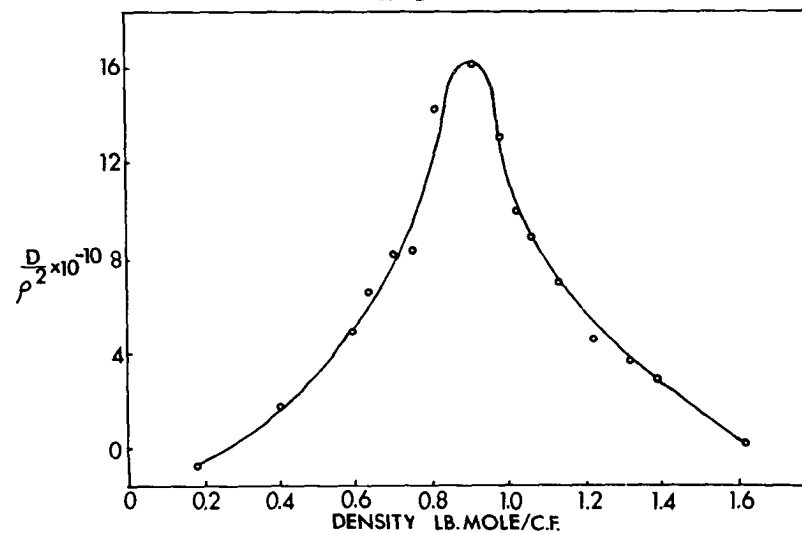
Figure 7. Density Dependence of D in Equation (19)
