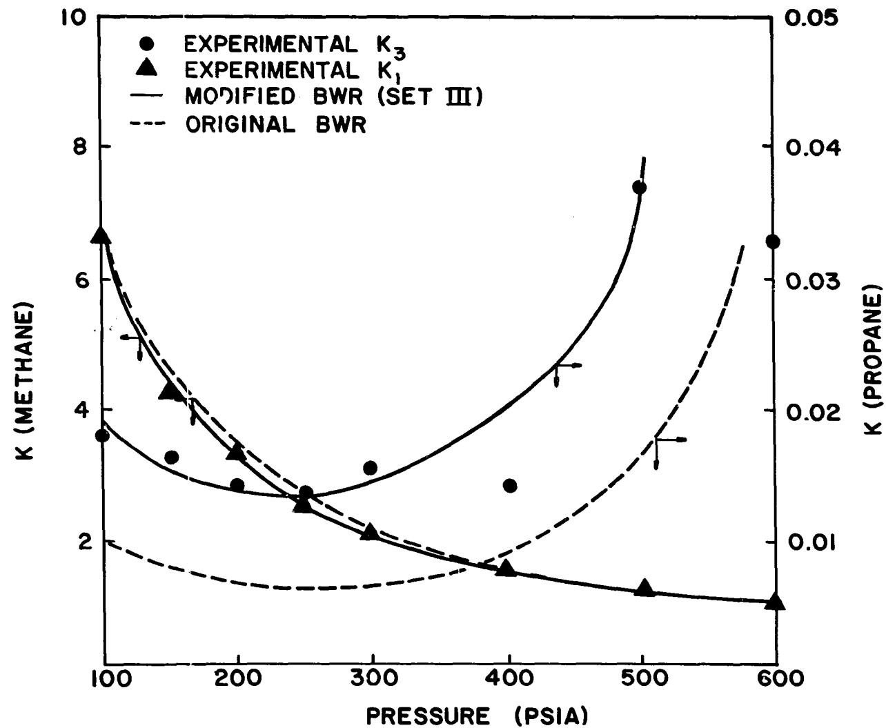
Figure 33. Comparison of Predicted K-values for Methane and Propane Using the Modified and Original BWR Equation with Experimental Values.
