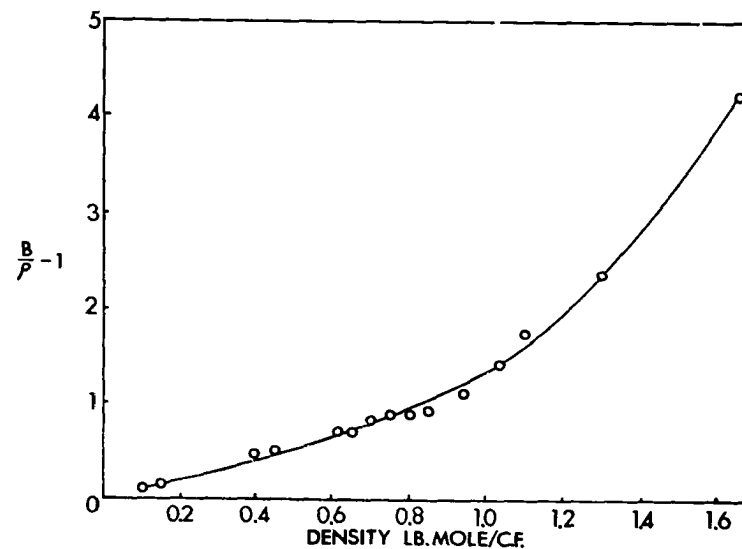
Figure 5. Density Dependence of B in Equation (19)
