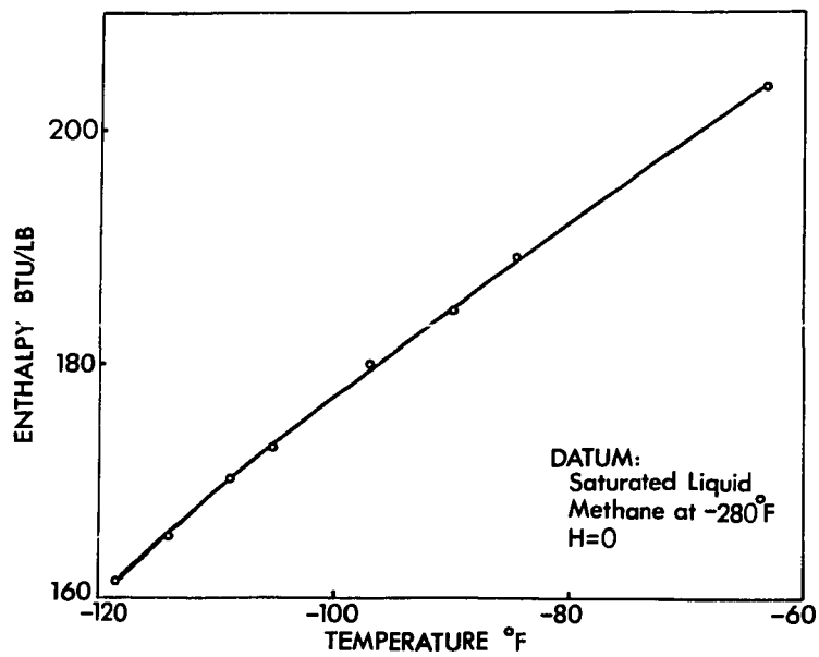
Figure 3. Enthalpies of Methane at Constant Density (1.64 lb mole/ft 3 )
