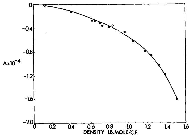
Figure 4. Density Dependence of A in Equation (19)
