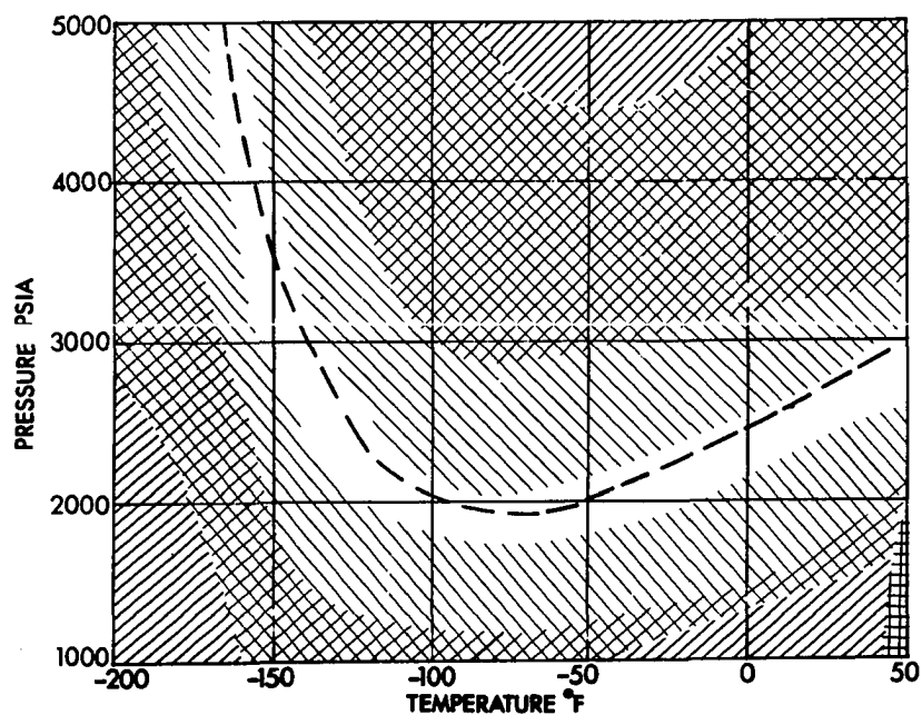
Figure 30. Comparison of Densities Calculated by the Original BWR Equation with Experimental Values for the 50 Mole % Propane Mixture
