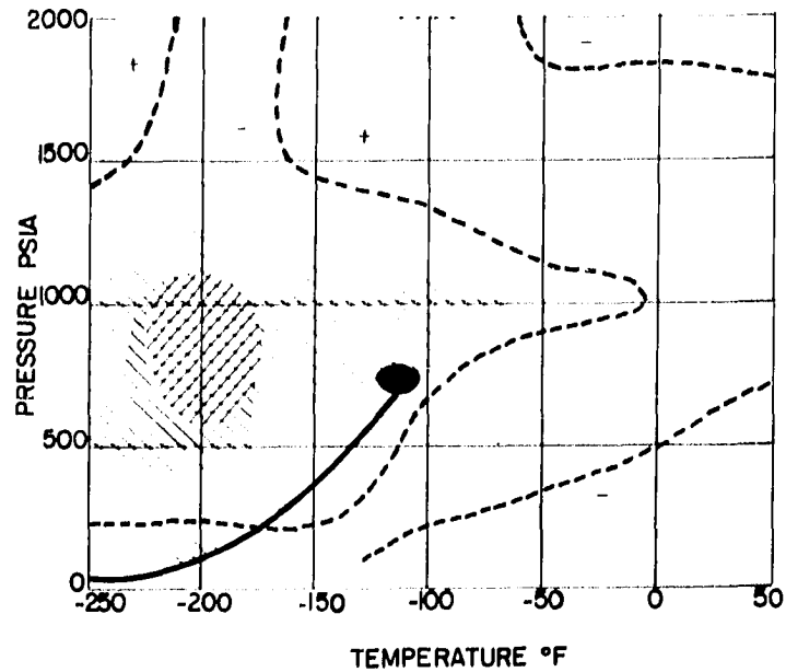
Figure 16. Comparison of Enthalpy Departures Calculated by the Modified BWR Equation with Experimental Values for Methane.
