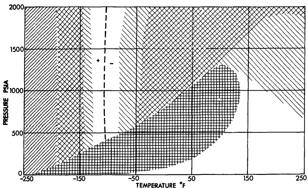
Figure 31. Comparison of Enthalpy Departures Calculated by the Modified BWR Equation Using Set III Parameters with Experimental Values for the 50.6 Mole % Propane Mixture.
