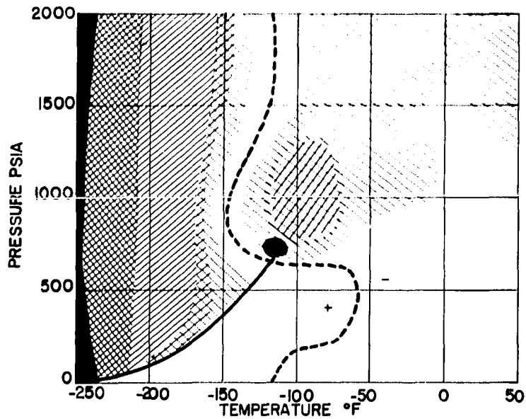
Figure 17. Comparison of Enthalpy Departures Calculated by the Original BWR Equation with Experimental Values for Methane.
