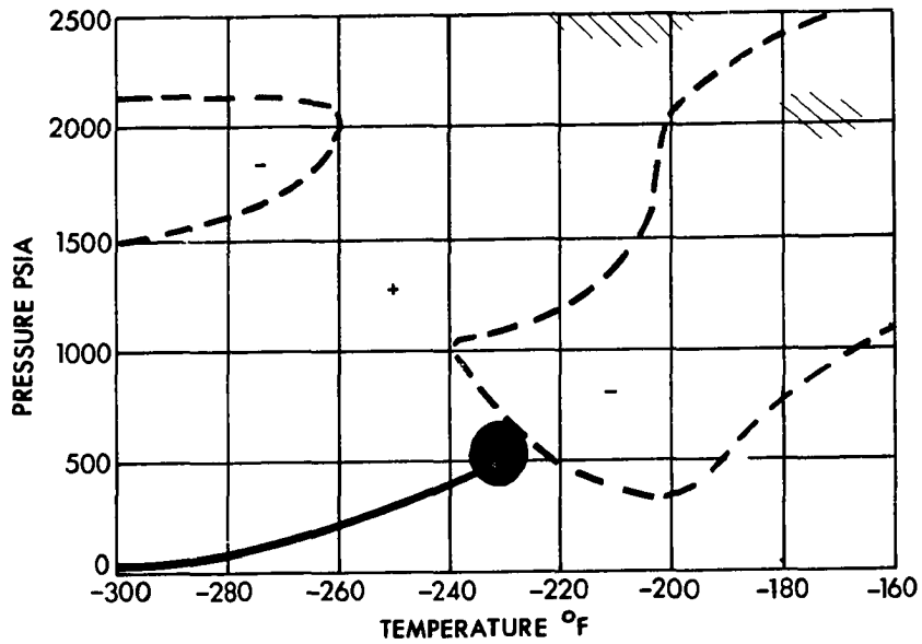
Figure 24. Comparison of Enthalpy Departures Calculated by the Modified BWR Equation with Experimental Values for Nitrogen
