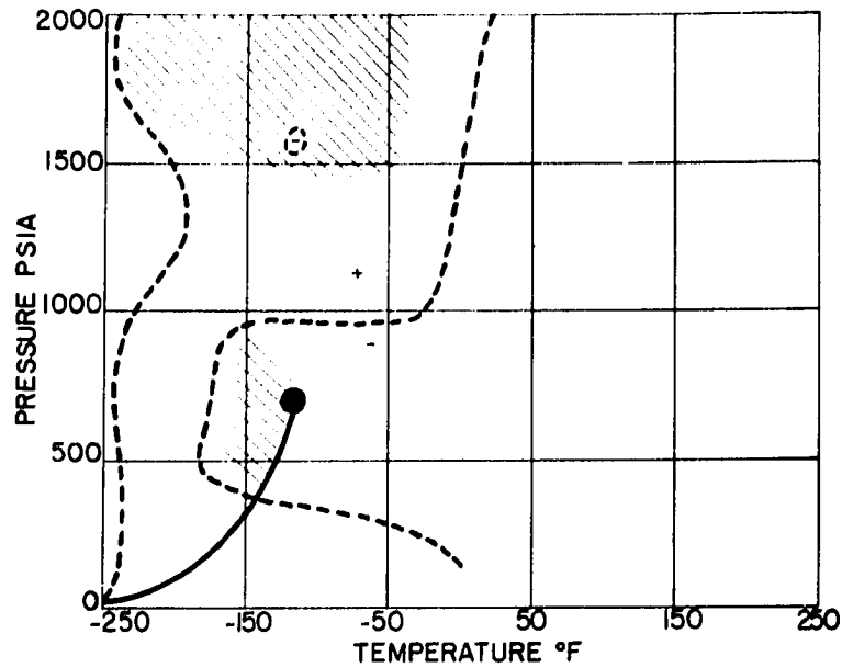
Figure 14. Comparison of Densities Calculated by the Modified BWR Equation with Experimental Values for Methane
