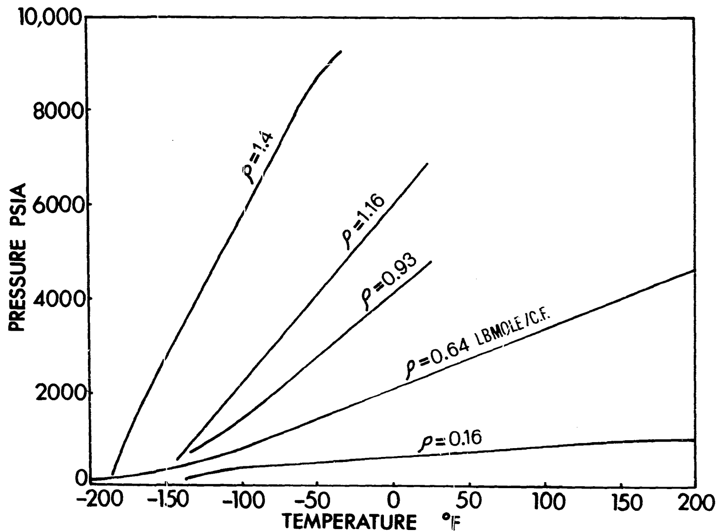
Figure 1. Variation of Pressure with Temperature of Methane Isochores
