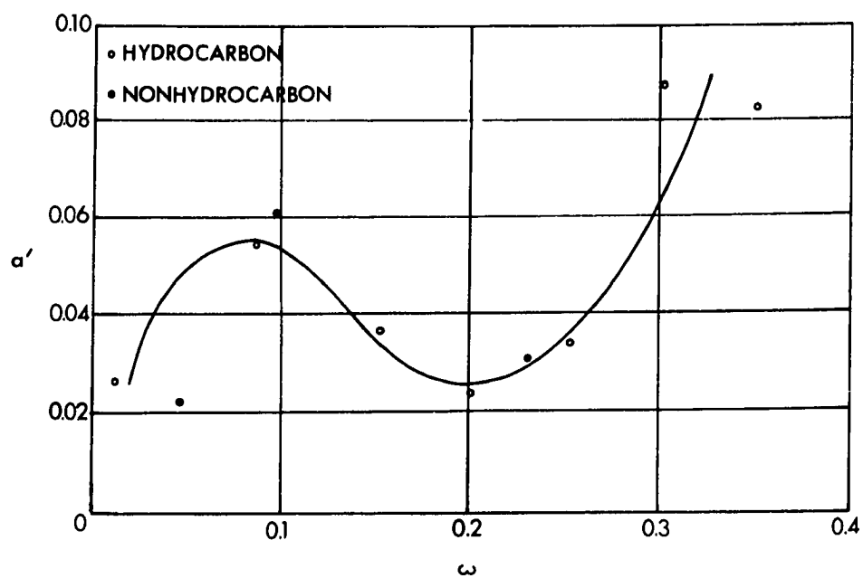
Figure 26. Variation of the Reduced Parameter a' with Acentric Factor
