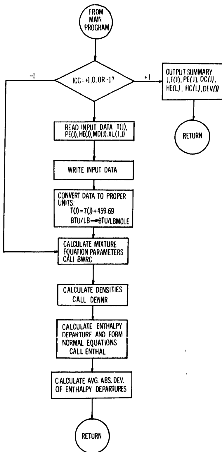
Figure 11. Flow Sheet for Enthalpy Subprogram.
