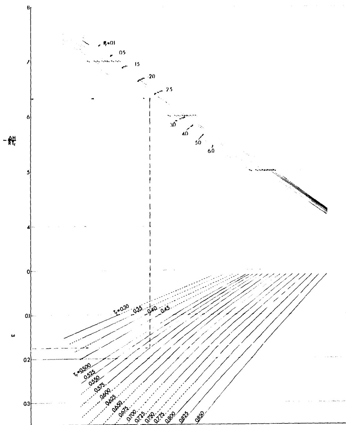
Figure 35. Corresponding States Correlation of Liquid Enthalpy Departures for Normal Fluids.
