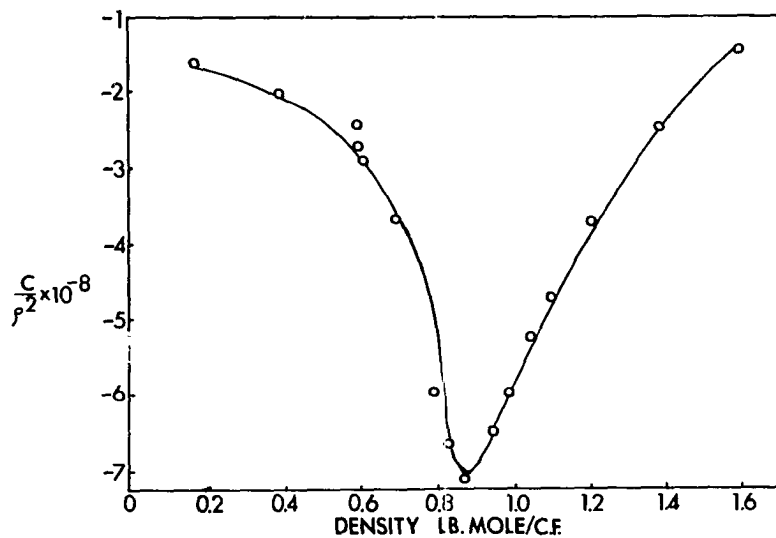
Figure 6. Density Dependence of C in Equation (19)
