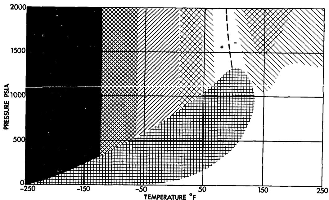
Figure 32. Comparison of Enthalpy Departures Calculated by the Original BWR Equation with Experimental Values for the 50.6 Mole % Propane Mixture
