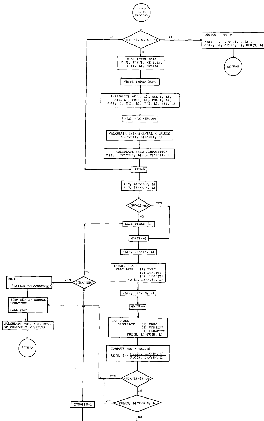
Figure 12. Flow Sheet for Phase Equilibrium Subprogram.
