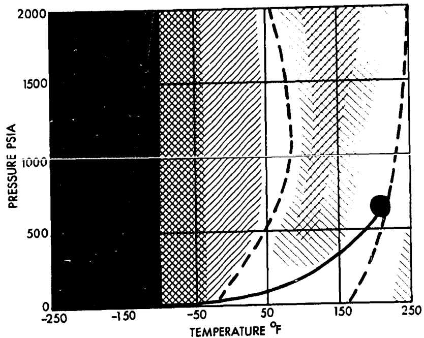
Figure 21. Comparison of Enthalpy Departures Calculated by the Original BWR Equation with Experimental Values for Propane.
