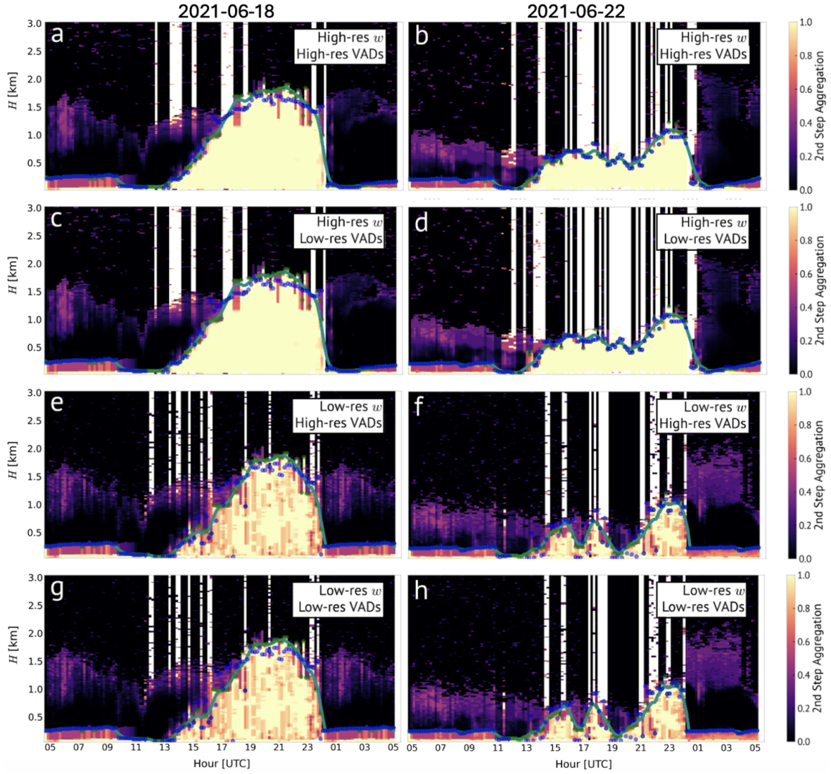
Figure 2.12: A comparison of second-generation aggregate values for the two clear-sky cases: 18 June 2021 is shown in the left column, and 22 June 2021 in the right column. Whether the input data has high- or low-resolution w or VAD data is detailed in the panel inserts as ‘high-res’ or ‘low-res’.
