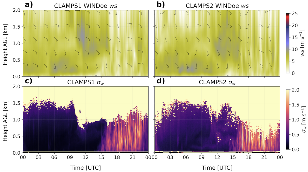
Figure 2.20: Time-height cross-section of CLAMPS1 and CLAMPS2 10-minute WINDoe-derived winds (Figs. 2.20a and 2.20b) and 10-minute \sigma_w with no SNR-filtering applied (Figs. 2.20c and 2.20d) during the PBLTops campaign on 25 August 2020.
