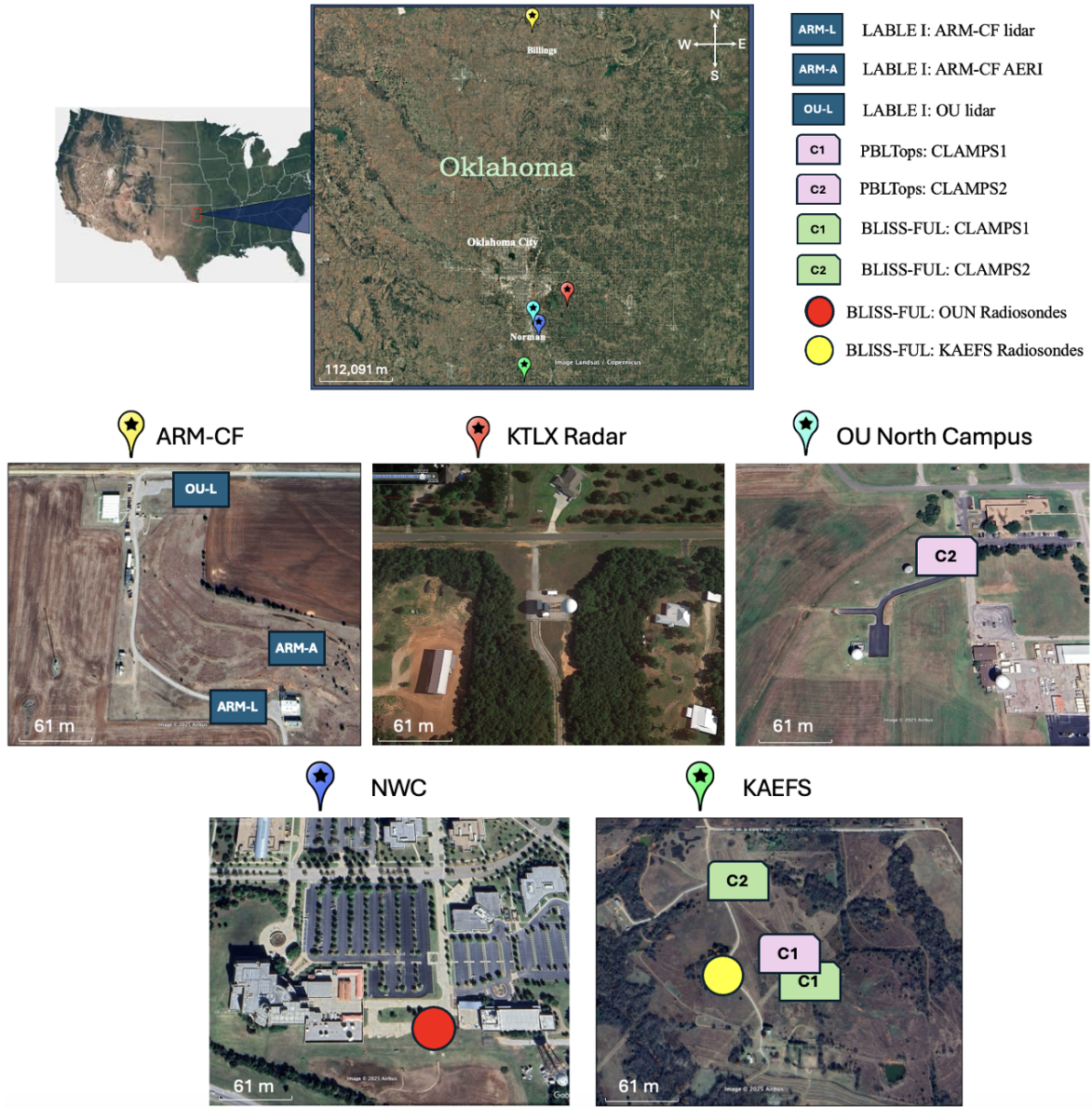
Figure 2.3: Map of field campaigns and observational instruments of interest beginning with the continental U.S (top left) and zooming into the north-central Oklahoma region (top middle). The sites at the bottom illustrate all stationary instrumentation sites or locations where campaigns took place, labeled based on the corresponding keys on the top right. Satellite imagery was obtained from Google Earth.
