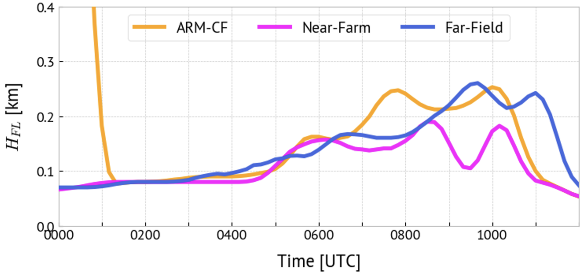
Figure 4.6: Outputs from the second-generation fuzzy-logic algorithm for ARM-CF (yellow line), near-farm (pink line), and far-field (blue line) on 2023-08-16 when turbines are not expected to be operating because rotor-layer winds were less than 3 \text{ m s}^{-1} throughout the period.
