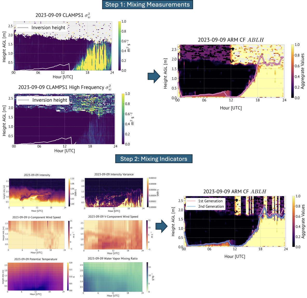
Figure 2.6: Time-height cross-sections of the variables considered in each step of the fuzzy-logic processing and their resulting H_{FL} outputs. Step 1 depicts profiles of mixing measurements ( \sigma_w^2 , high frequency \sigma_w^2 , and inversion height) that help make up the first generation estimate, and step 2 shows profiles of mixing indicators (intensity, intensity variance, the u - and v -component ws , \theta , and q ) that help make up the second generation estimate. A more detailed diagram on each step can be found in Smith and Carlin (2024), specifically their Figure 4.
