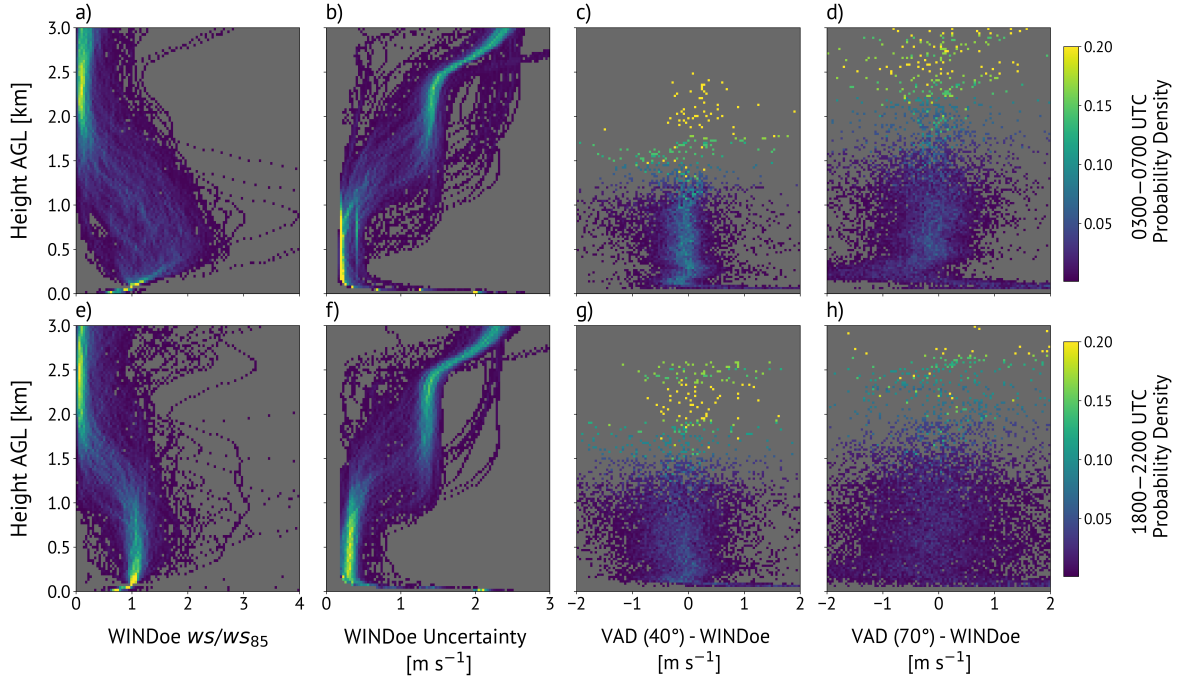
Figure 2.10: As in Figure 2.9, but for the OU lidar. Here, the difference was measured at both the 40° and 70° elevation angles.
