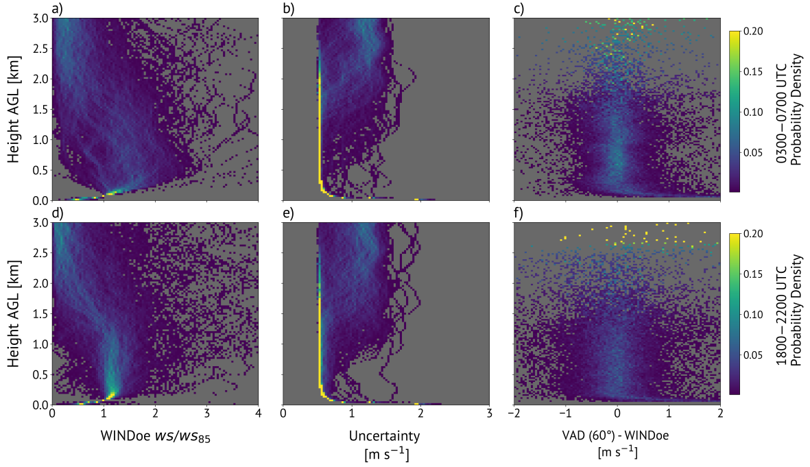
Figure 2.9: Probability density functions of the ARM-CF lidar for WINDoe ws , its uncertainty, and the difference between VADs and WINDoe for a period of time in the SBL (Figs. 2.9a-2.9c) and the CBL (Figs. 2.9d-2.9f).
