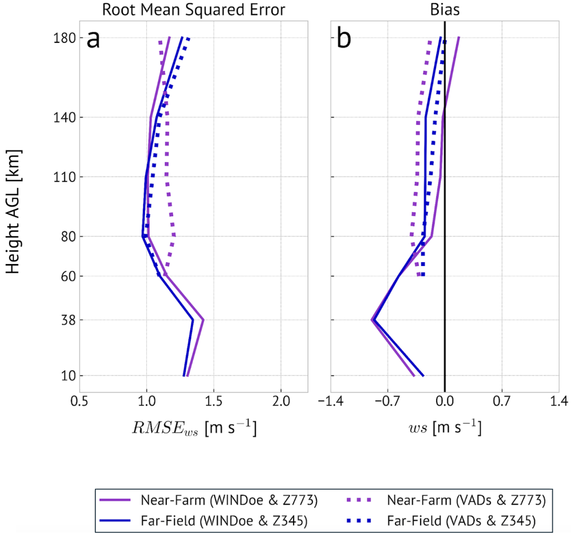
Figure 3.4: Root mean squared error of the ws between WINDoe and ZephIR data (Fig. 3.4a, solid lines) and the ZephIR and CLAMPS scanning lidar VAD retrievals (Fig. 3.4a, dotted lines) during the 2022 fall-winter campaign. Fig. 3.4b shows the same dataset comparisons but with mean bias calculations. WINDoe data were matched to the nearest ZephIR and VAD data heights. The ZephIR-VAD comparisons start at roughly 60 m where observations from the CLAMPS lidars begin.
