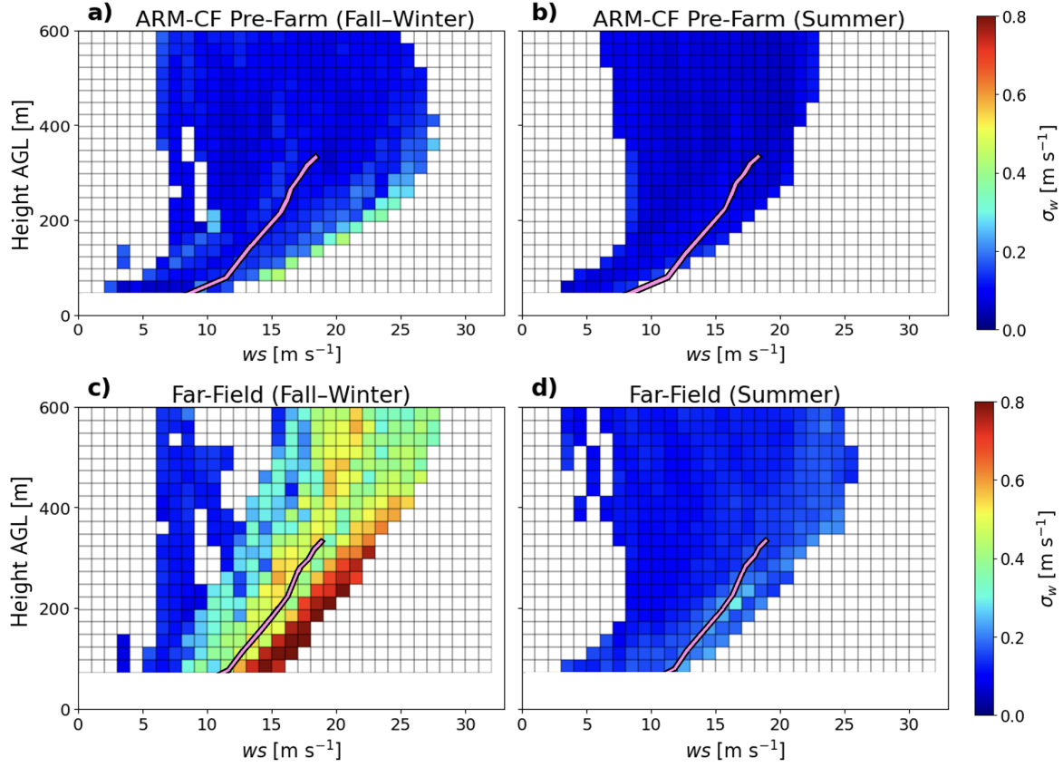
Figure 3.13: Profiles of median \sigma_w from environments without nearby wind farms during the ARM-CF and AWAKEN fall-winter (Figs. 3.13a and 3.13c) and summer (Figs. 3.13b and 3.13d). The pink line denoting V_T as computed from B15.
