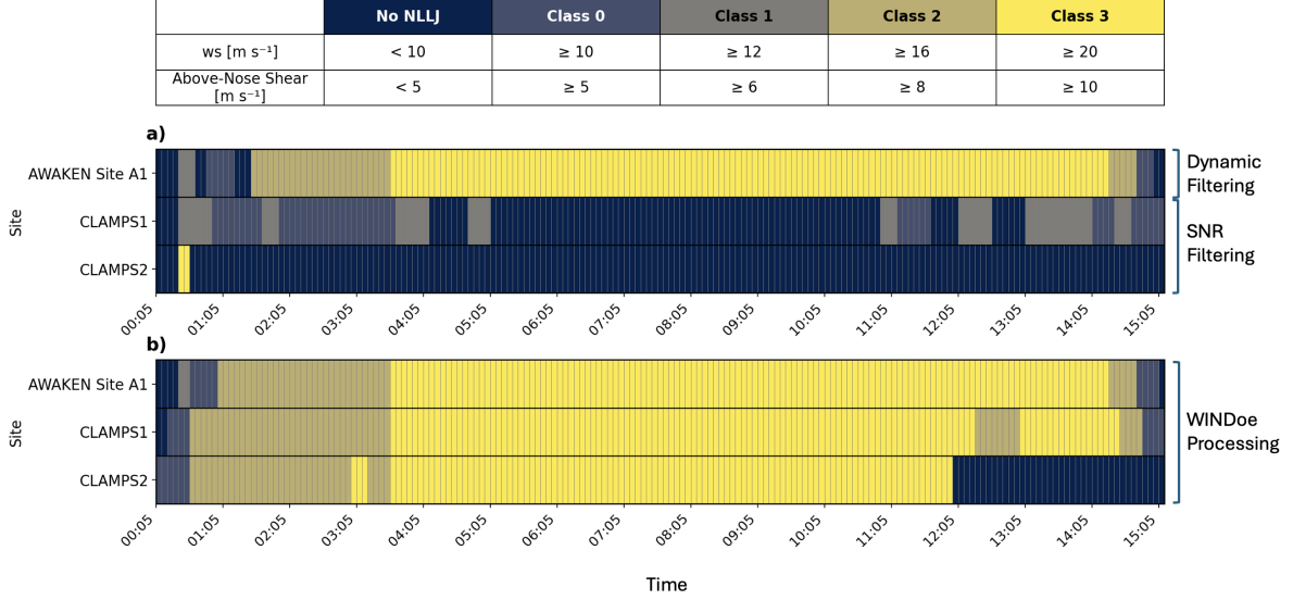
Figure 2.5: The classification metric for NLLJ magnitude (table) and the results of that classification applied to AWAKEN A1, CLAMPS1, and CLAMPS2 on 23 September 2023 (0005-15:15). In Figure 2.5a, each site showcases the results using different types of lidar data filtering: site A1 implemented a six-beam method with a dynamic filtering method, and both CLAMPS show VADs with the traditional SNR filtering at 0.008. These are compared with NLLJ classification results using the same data but retrieved via WINDoe (Figure 2.5b).
