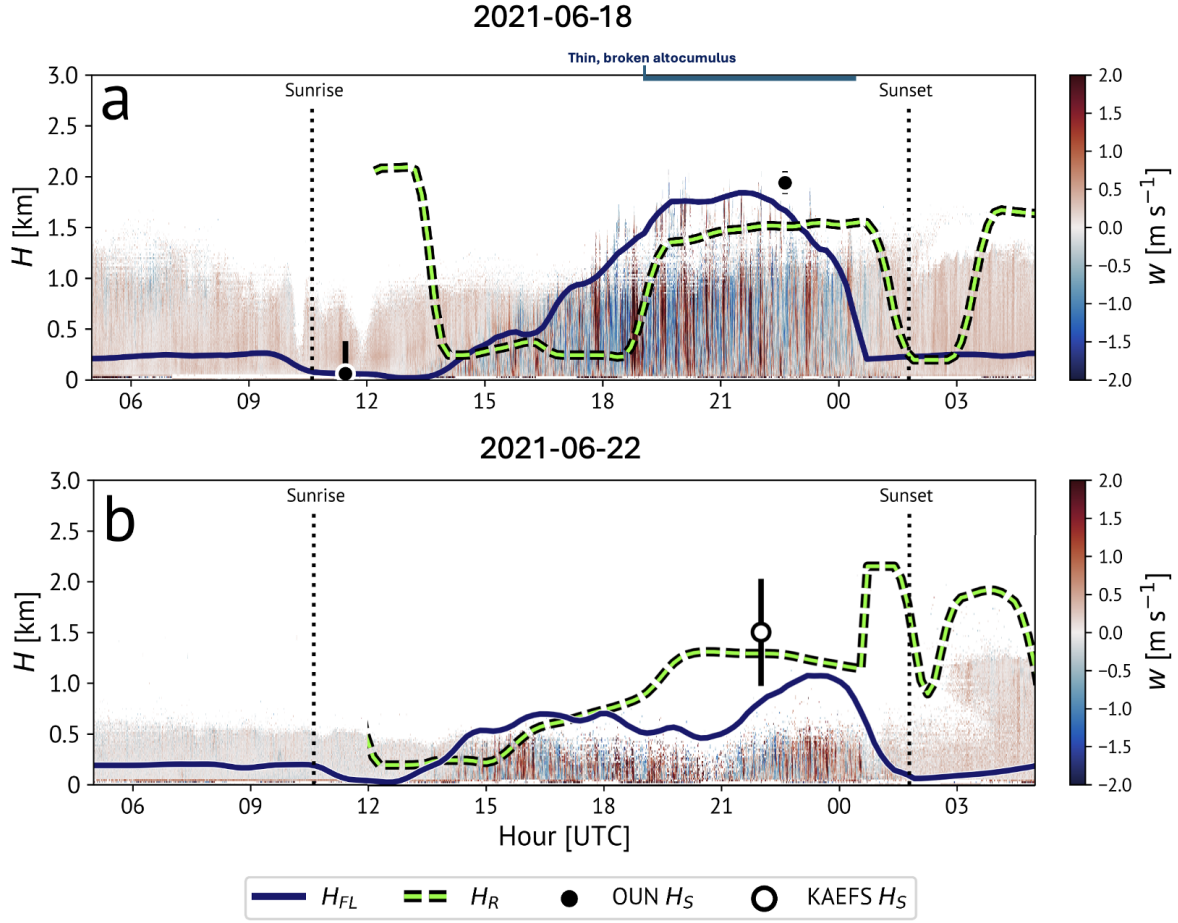
Figure 2.13: The three main H estimation methods ( H_S for the sounding method, H_R for the radar method, and H_{FL} for the fuzzy-logic method) under mainly clear sky conditions (18 June 2021 0500 UTC - 19 June 2021 0500 UTC for Fig. 2.13a and 22 June 2021 0500 UTC - 23 June 2021 0500 UTC for Fig. 2.13b). The H_R (green dashed line), and H_{FL} (dark blue line) methods are overlaid on CLAMPS1 w observations, a crucial contributor in the first generation aggregation of H_{FL} . All H_S results are shown with circle markers (filled for OUN and open for KAEFS), and the black vertical lines associated with them represent the standard deviation of the techniques applied. Local sunrise and sunset times are shown with vertical dashed lines. The start of any period clouds first appear over all sites were denoted at the top of the plot by the types of clouds they were.
