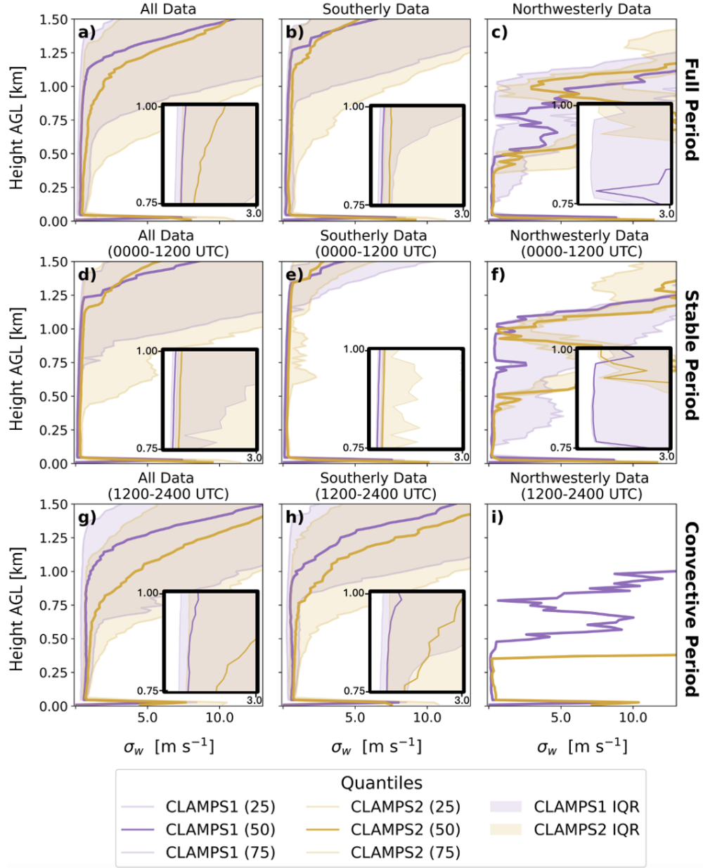
Figure 2.21: PBLTops percentiles of \sigma_w throughout the full diurnal cycle for all available data (Fig. 2.21a), only southerly data (Fig. 2.21b), and only northwesterly data (Fig. 2.21c). The same approach is employed but only for the SBL (Figs. 2.21d-2.21f) and only for the CBL (Figs. 2.21g - 2.21i). The 50th percentile served as the mean measure, while the 25th and 75th percentile served as left and right outer bounds, respectively. To compare usable measurements not contaminated by noise, zoomed-in versions of each panel from a 0-3 m s -1 x-axis and 0.075-1.0 km y-axis are shown at the right of their original version, except for Fig. 2.21i where the data was not within the inset map bounds.
