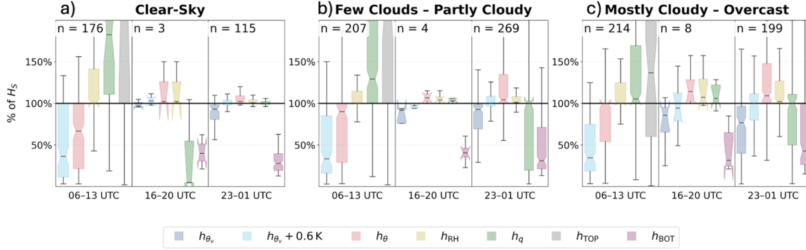
Figure 2.7: The seven radiosonde techniques as percentages of the H_S median (represented as the black horizontal line), separated by sky coverage conditions (Fig. 2.7a, 2.7b, and 2.7c represents clear-sky, few clouds-partly cloudy, and mostly cloudy-overcast, respectively). Within each sky condition category, a time window is applied for three different periods throughout the diurnal cycle to account for radiosondes not being released exactly on the hour. The number of samples (n) in each of these ranges is listed at the top left.
