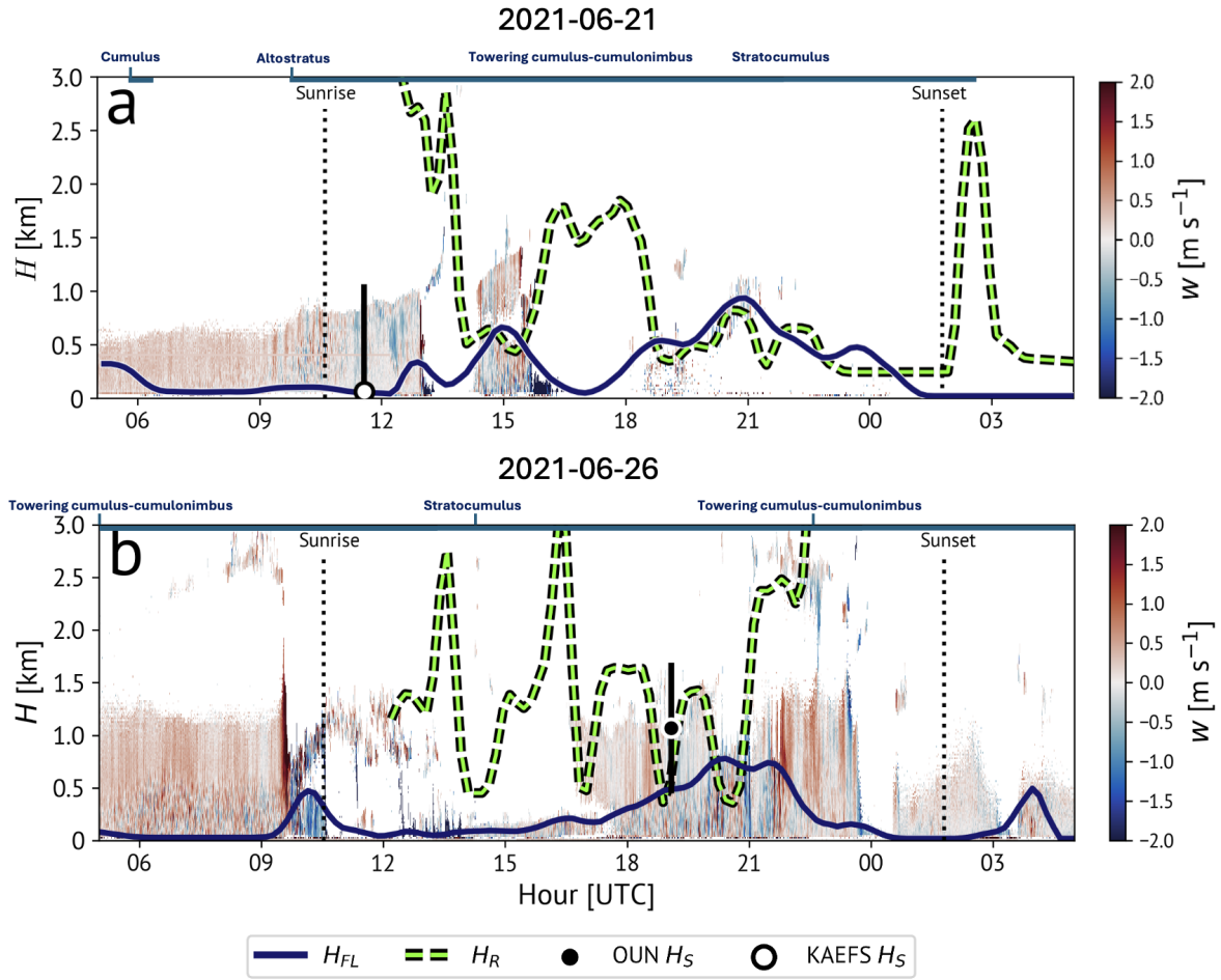
Figure 2.17: As in Fig. 2.13, but for cases with mostly cloudy-overcast conditions.
