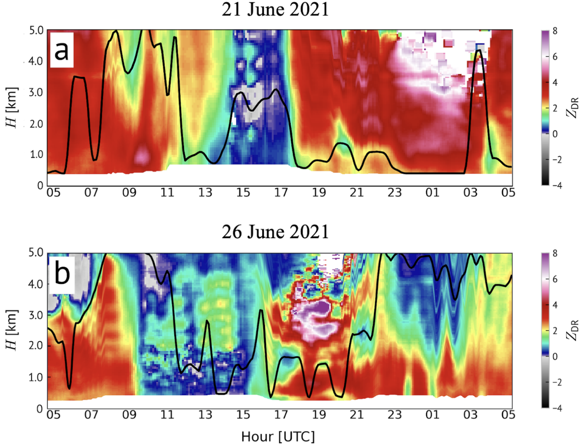
Figure 2.18: Radar QVPs of Z_{DR} values using the same cases from Figure 2.17 (21 June 2021 for Fig. 2.17a and 26 June 2021 for Fig. 2.17b). Note the difference in the y-axis range compared to previous figures to view the extent of the detected H_R , though it does still exceed this larger range at times.
