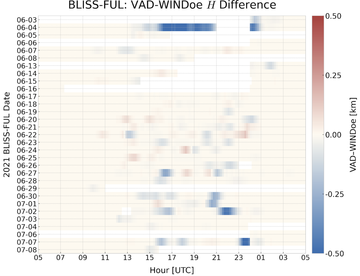
Figure 2.11: Differences between H_{FL} using VAD- and WINDoe-derived wind profiles throughout the 0500-0500 UTC diurnal cycle for all BLISS-FUL cases. White areas indicate periods of missing data.
