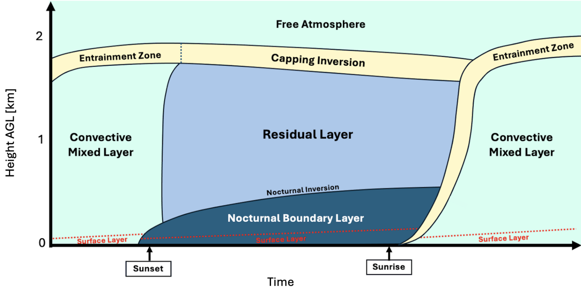
Figure 1.1: Schematic of the idealized diurnal ABL (adapted from Stull (1988)).
