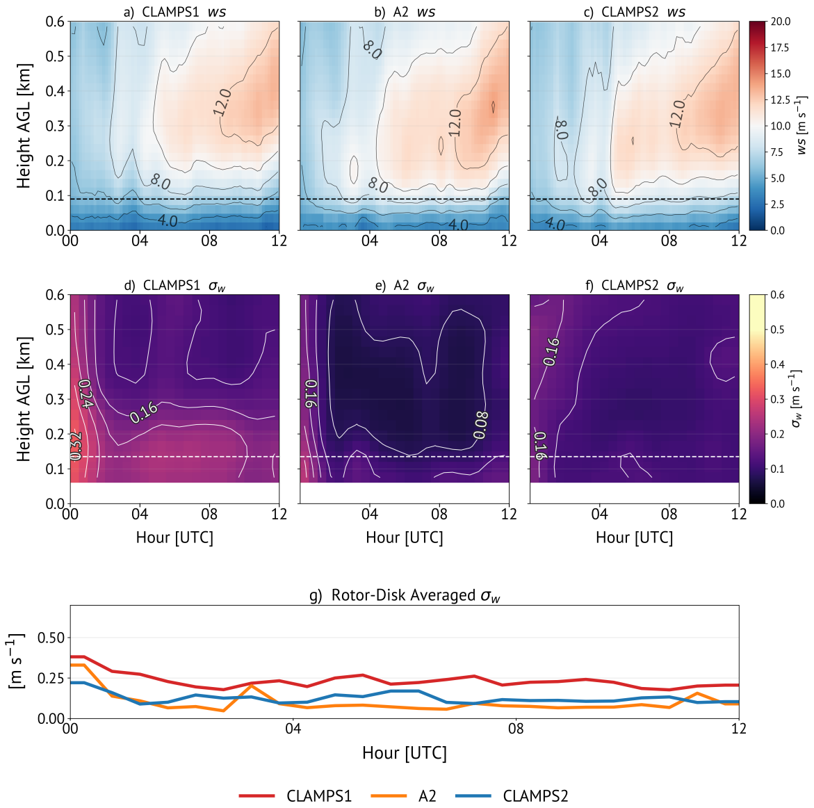
Figure 3.11: As in Fig. 3.10, but as composites for moderate NLLJ cases.
