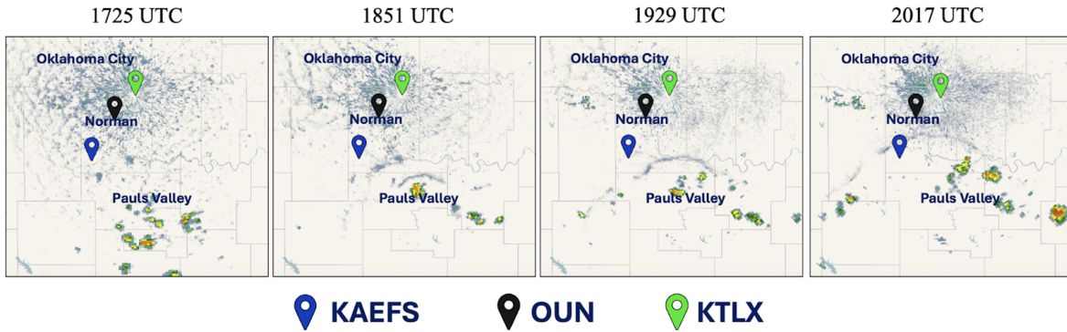
Figure 2.16: Radar imagery detailing the outflow from clustered thunderstorm cells near Pauls Valley, Oklahoma on 6 July 2021.
