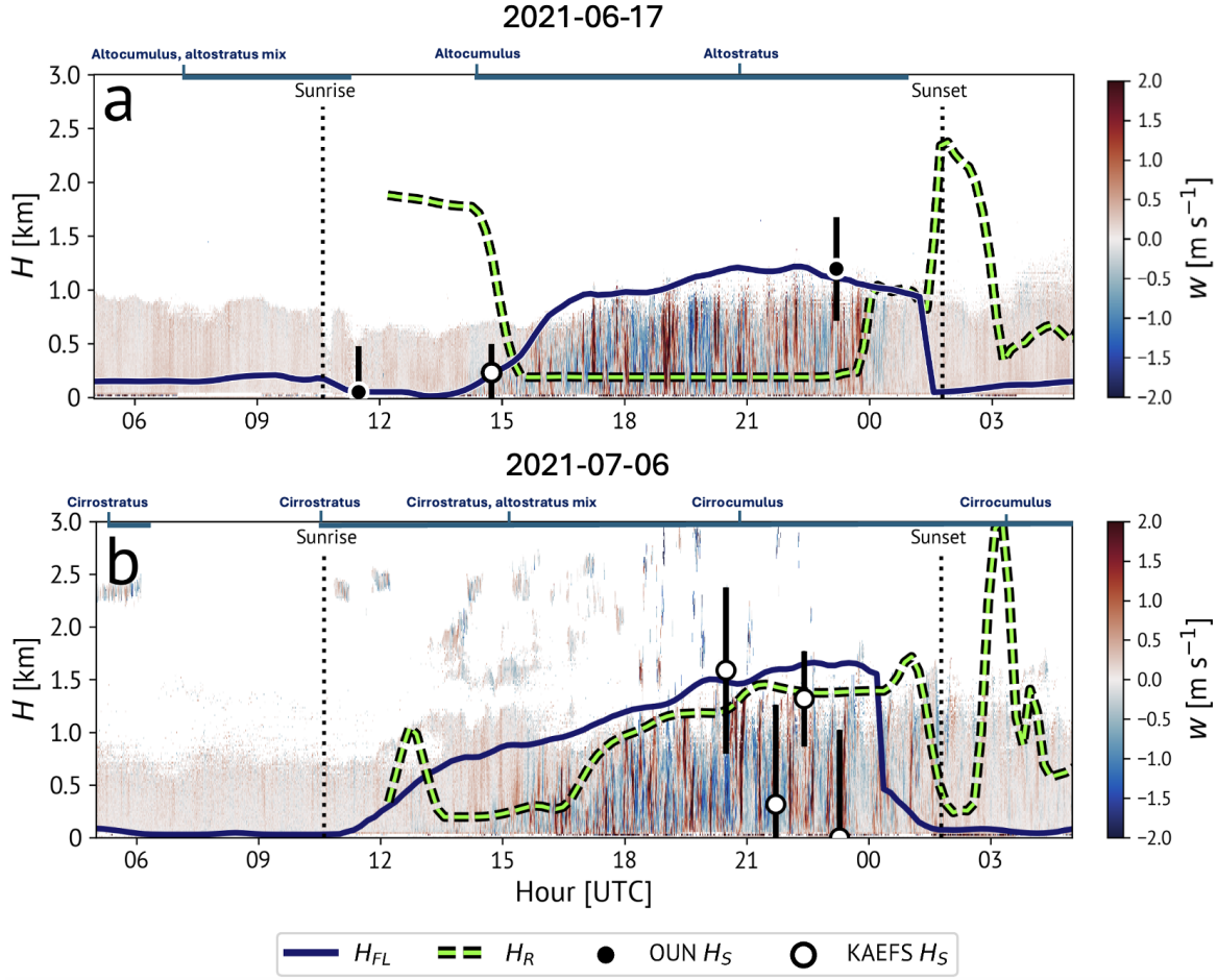
Figure 2.15: As in Figure 13, but for cases with few-partly cloudy conditions.
