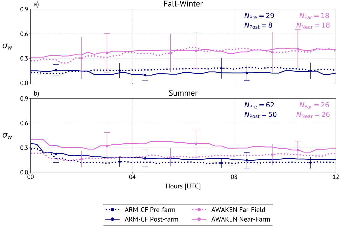
Figure 3.7: Comparison of averaged \sigma_w levels between environments with and without nearby wind farms from the southerly sector between 0000-1200 UTC. Fig. 3.7a corresponds to the fall-winter periods from ARM-CF pre-farm (blue dashed line), ARM-CF post-farm (blue solid line), AWAKEN far-field (pink dashed line), and AWAKEN near-farm (pink solid line). Fig. 3.7b shows the same but during the summer periods.
