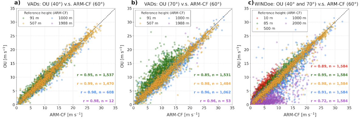
Figure 2.8: Scatterplots of ARM-CF and OU lidar VADs during LABLE I when the OU lidar was scanning two different elevation angles (40°; Fig. 2.8a, and 70°; Fig. 2.8b). The VADs were SNR-filtered at 0.008. The same is shown in Fig. 2.8c but for WINDoe, where the OU output was comprised of both the 40° and 70° elevation angles together. Results from four different range gates throughout the ABL are shown for all panels except Fig. 2.8c., which included a fifth measure at 10 m to demonstrate the abilities of its coverage.
