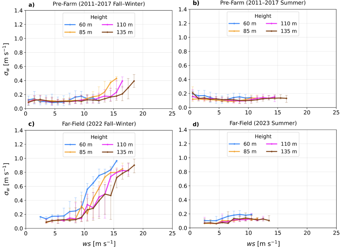
Figure 3.14: The V_T from non-waked environments as calculated from ARM-CF and AWAKEN fall-winter (Figs. 3.14a and 3.14c) and ARM-CF and AWAKEN summer (Figs. 3.14b and 3.14d) at rotor layer heights (60, 85, 110, and 135 m).
