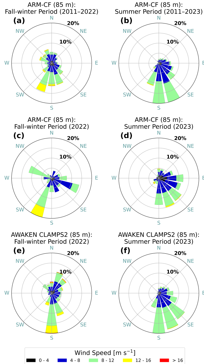
Figure 3.5: Wind roses of using WINDoe data of the analysis periods of interest during the fall-winter and summer seasons from the ARM-CF lidar (Figs. 3.5a-3.5b) and the CLAMPS2 lidar. Only CLAMPS2 data from the far-field site is shown since, unlike CLAMPS1, had correct wd during the summer.
