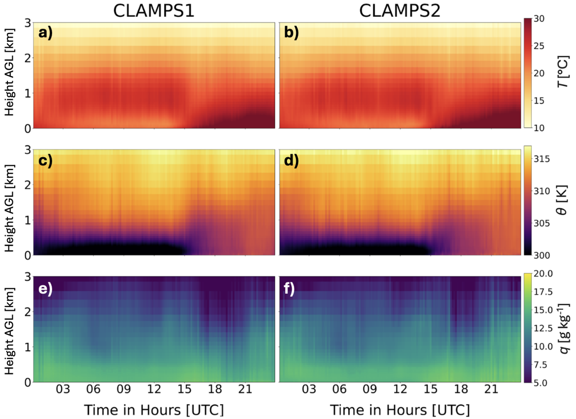
Figure 2.2: Sample TROPoe profiles of T , \theta , and q from CLAMPS1 (left column) and CLAMPS2 (right column) from 23 September 2023.
