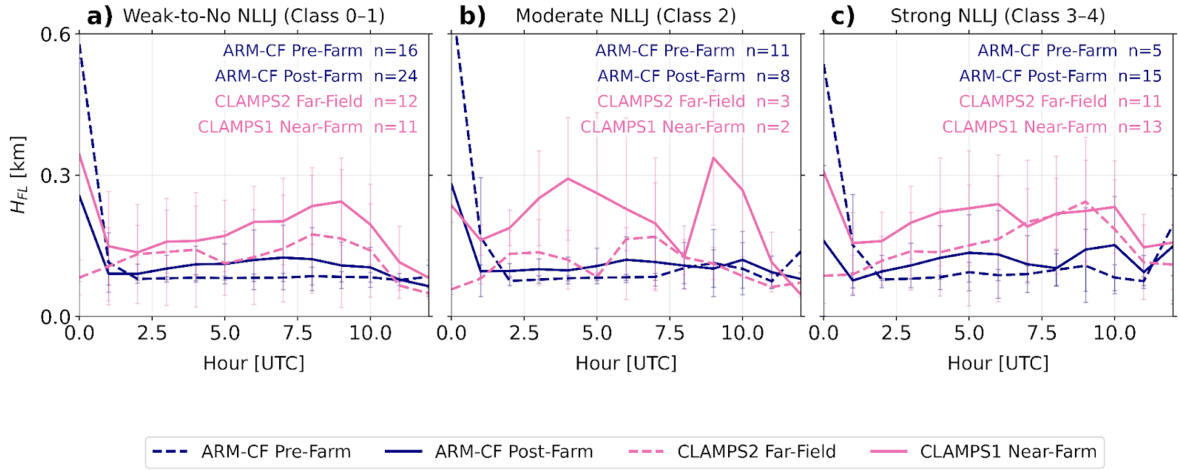
Figure 4.2: As in Fig. 4.1, but categorized by different NLLJ regimes: weak-to no (Fig. 4.2a), moderate (Fig. 4.2b), and strong (Fig. 4.2c).
