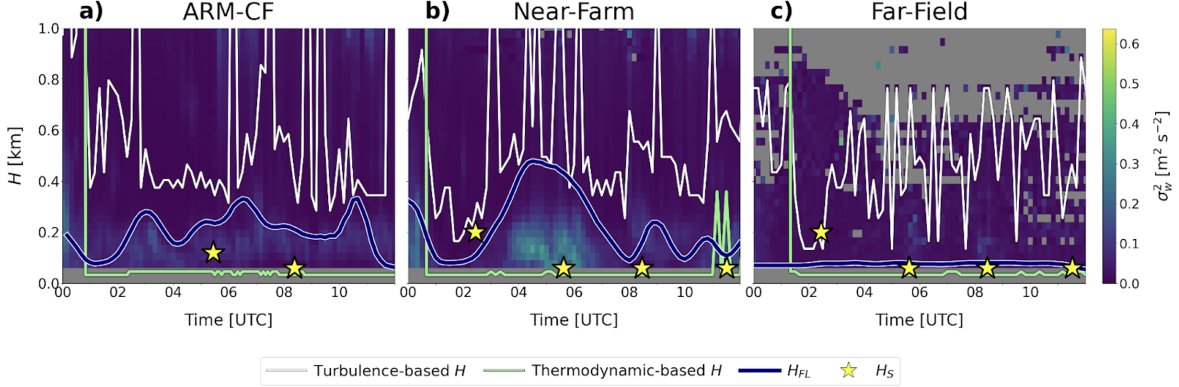
Figure 4.3: Comparisons on 2023-08-17 between ARM-CF, near-farm, and far-field of four H methods: H_S (yellow star), H_{FL} (blue line), the turbulence-based method (white line), and the thermodynamic-based method (green line). Radiosondes originating from the ARM-CF site were displayed alongside with the three H methods from ARM-CF, and radiosondes originating from AWAKEN’s site H were displayed with the near-farm and far-field H methods.
