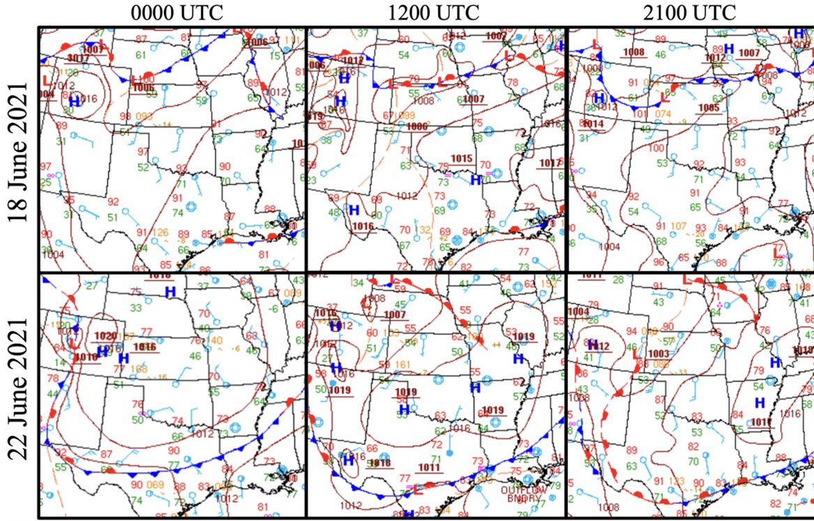
Figure 2.14: Surface synoptic maps from NOAA’s Weather Prediction Center for 18 June 2021 (top row) and 22 June 2021 (bottom row) at 0000, 1200, and 2100 UTC.
