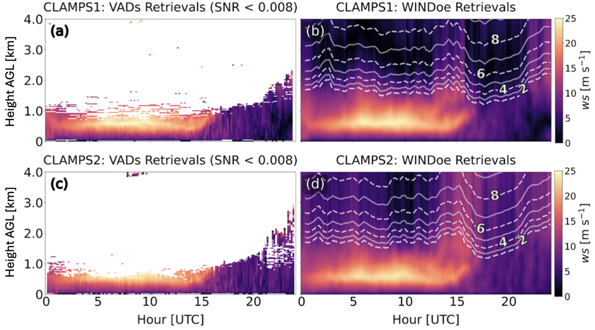
Figure 2.4: A comparison of VADs filtering at an SNR threshold of 0.008 from CLAMPS1 (Fig. 2.4a) and CLAMPS2 (Fig. 2.4c) with WINDoe retrievals from CLAMPS1 (Fig. 2.4b) and CLAMPS2 (Fig. 2.4d) for the case of 23 September 2023. White contours show WINDoe wind speed uncertainty in \text{m s}^{-1} .
