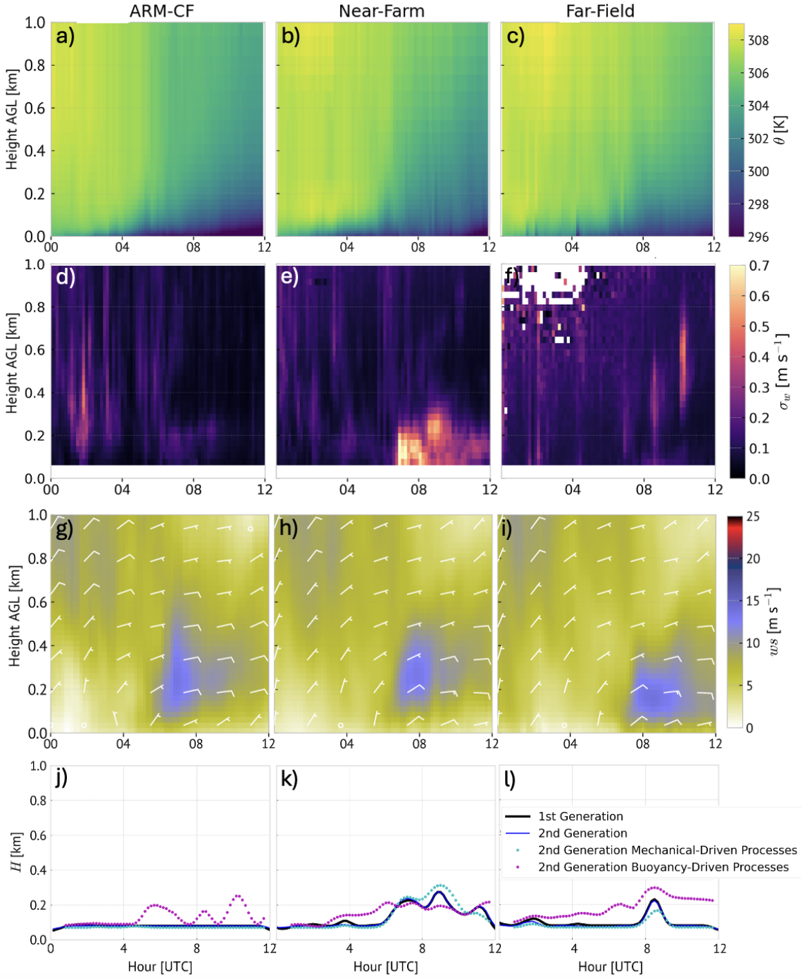
Figure 4.5: As in Fig. 4.4, but for the northerly case of 2023-08-30.
