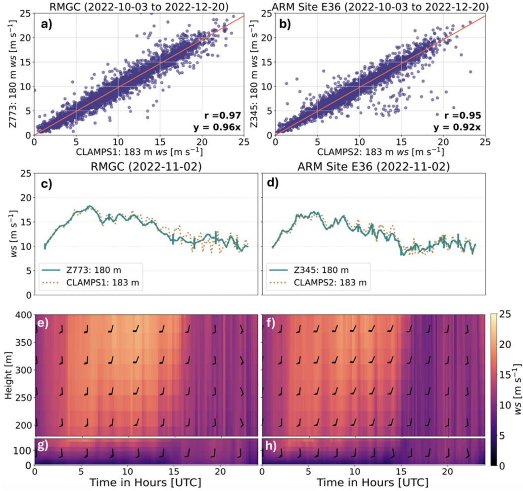
Figure B.1: Evaluation and combination of ws data from the ZephIR and CLAMPS lidars. The left column shows data from the near-field site, Rolling Meadows Golf Club (RMGC), collected by CLAMPS1 and Z773. The right column shows data from the far-field site of E36, collected by CLAMPS2 and Z345. Panels B.1a and B.1b show for each site, respectively, a scatterplot of winds at the measurement height closest to 180 m (exact for ZephIR, 183 m for CLAMPS) from the entire winter campaign. Panels B.1c and B.1d show a time series of winds at the same measurement heights on 2 November 2022 with error bars corresponding to the standard deviation of averaged ZephIR data. Finally, panels B.1e and B.1f are time-height cross sections of CLAMPS wind speed observations with wind barbs overlaid, also for 2 November 2022. Panels B.1g and B.1h, showing the ZephIR lidar wind speed observations in a similar way, are meant to combine with panels B.1e and B.1f above to demonstrate the two lidars as a complementary profile.
