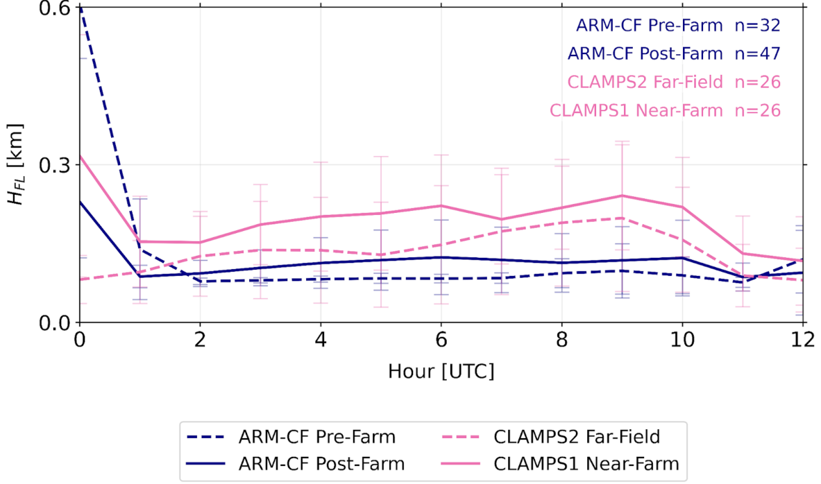
Figure 4.1: Averages from second-generation output of H_{FL} runs for ARM-CF (pre-farm, dashed blue line; post-farm, solid blue line) and CLAMPS (far-field, dashed pink line; near-farm solid pink line) data from the summer periods. At the top right of the panel, the number of samples from each of the plotted averages is listed.
