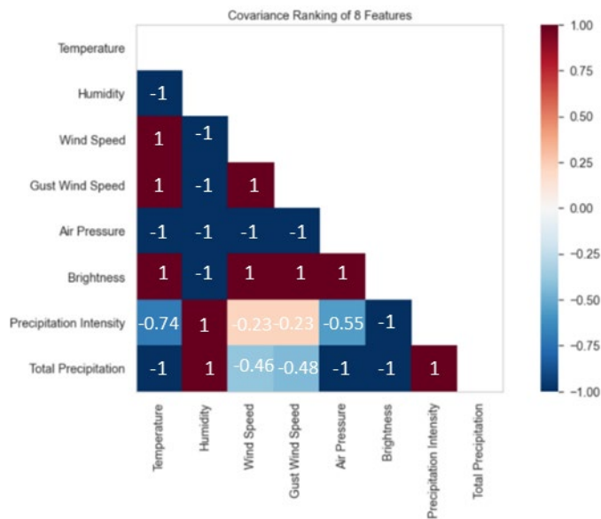
Figure 43. Pairwise covariance correlation between all data attributes.
