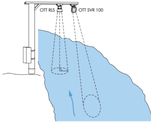
Figure 26. SVR and RLS mounting setup.
