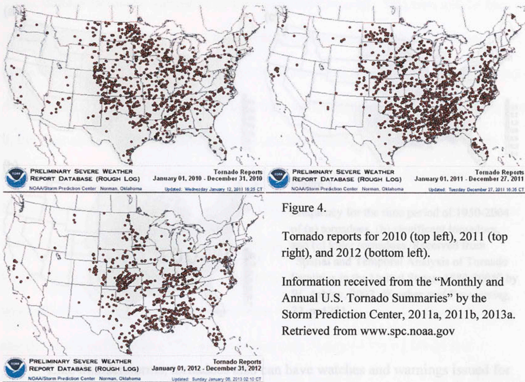
Figure 4. Annual Tornado Reports
