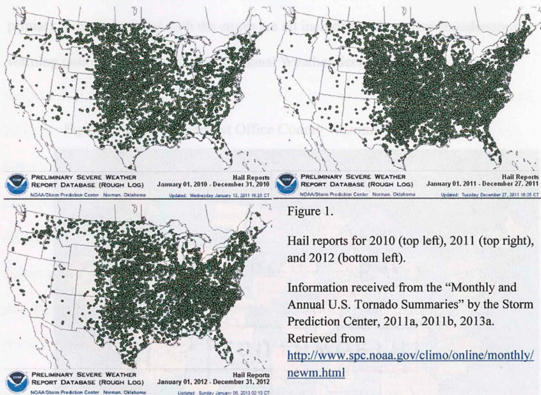
Figure 1. Annual Hail Reports
