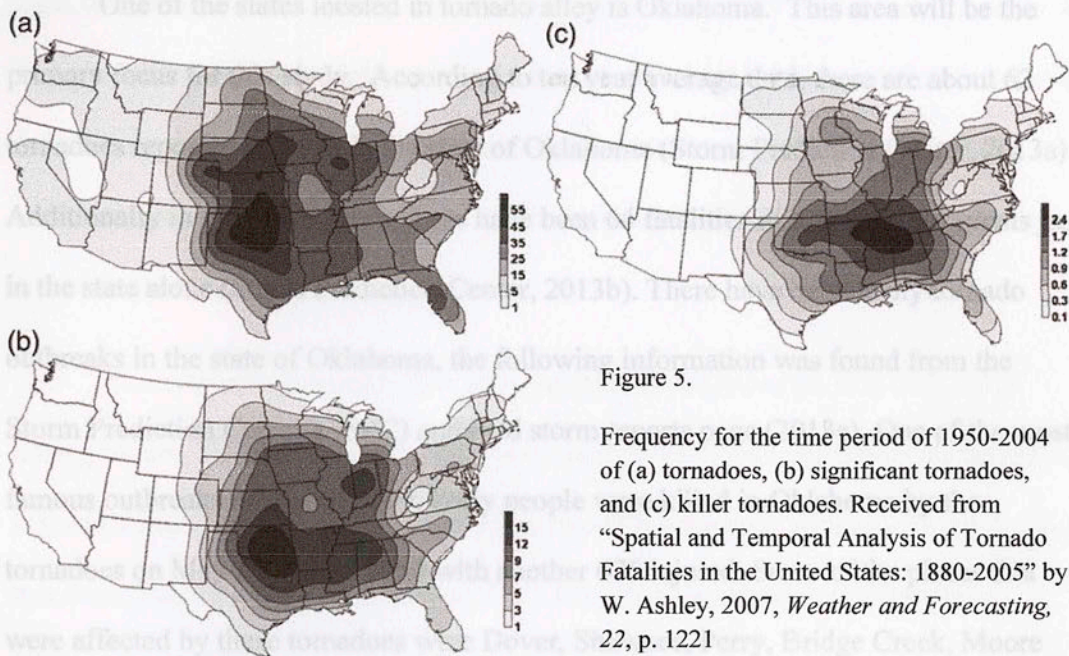
Figure 5. Frequencies of Tornadoes
