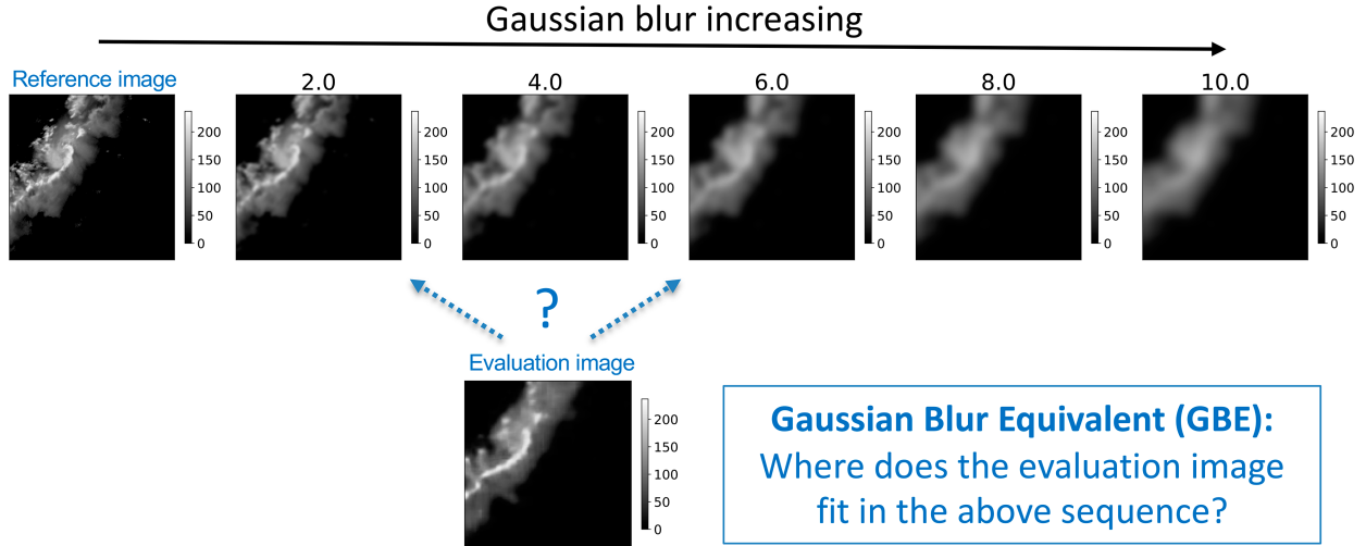
FIG. 6. Core idea of GBE to calibrate a sharpness metric: How much do we have to blur the reference image to get the same (minimum, mean, or maximum) sharpness value as for the evaluation image?
