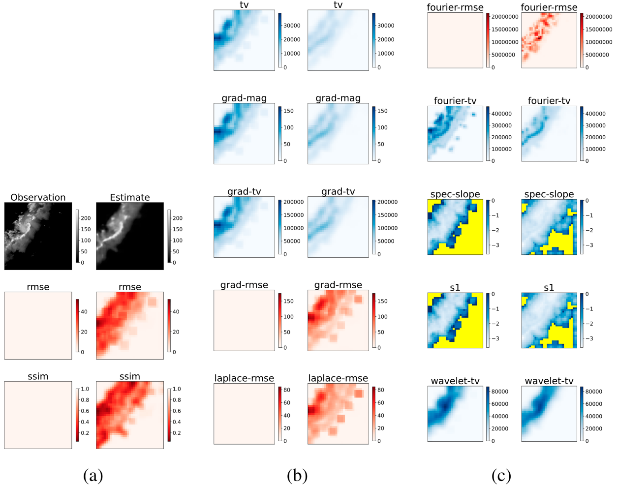
FIG. 5. Heat maps comparing observed radar (reference) with the corresponding GREMLIN estimate (evaluation image) for (a) metric group 1, (b) metric group 2, and (c) metric group 3. The color map for SSIM is inverted because SSIM indicates stronger similarity by a higher value—in contrast to standard similarity measures, such as RMSE. Yellow indicates pixels with invalid values.
