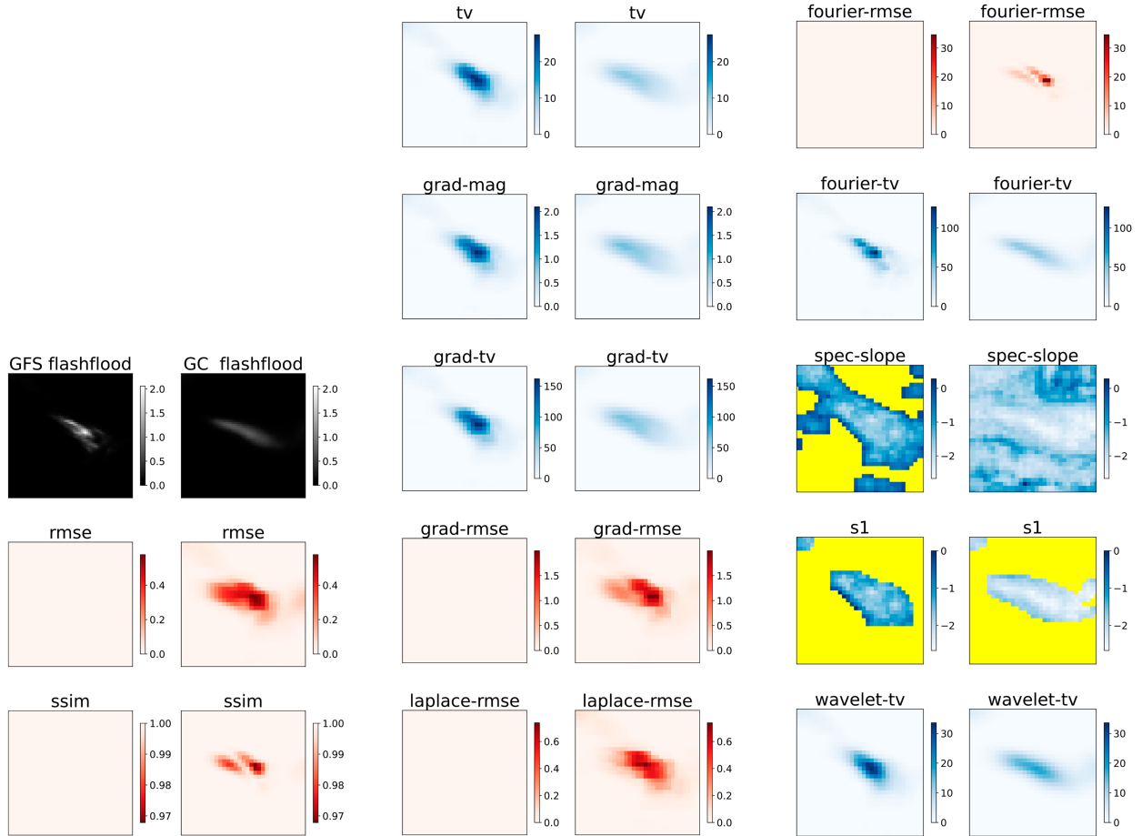
FIG. 10. Heat maps for the flash flood event for GFS vs. GraphCast forecasts of 6-h accumulated precipitation at a lead time of 48 h. The contrast threshold for metric S_1 used here is 0.1.
