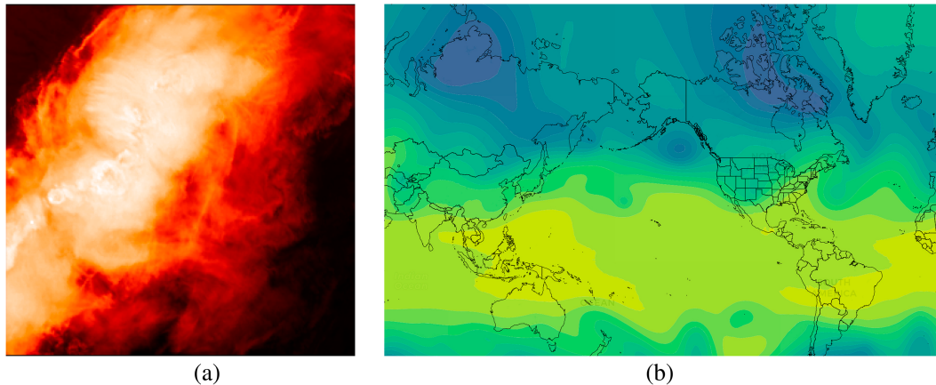
FIG. 4. Two examples of meteorological imagery: (a) satellite image from GOES-16 showing clouds; (b) forecast of 500-mb geopotential height at 5-day lead time from GraphCast (Lam et al. 2023) initialized on 23 Apr 2024 (0000 UTC). Image credit for (b) GraphCast visualization from our real-time visualization website for purely AIWP models (Radford et al. 2025). The richness of texture in the cloud image and the lack of clear boundaries in the geopotential height forecast illustrate why using only sharpness measures that focus on edges, i.e., boundaries between “objects,” would disregard many important details in meteorological imagery.
