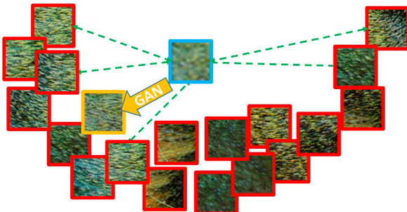
FIG. 2. Schematic illustrating the typical results obtained by a standard CNN and a GAN for the ill-defined task of generating high-resolution imagery from low-resolution imagery. The patches in red represent a subset of the infinitely many solutions to the problem (ensemble members), the patch in blue represents the solution obtained by a CNN with MSE loss function (roughly ensemble average), and the patch in yellow represents a GAN solution (approximation of single ensemble member). Image credit: Figure adapted from Fig. 3 in Ledig et al. (2017)—reprinted with permission from IEEE.
