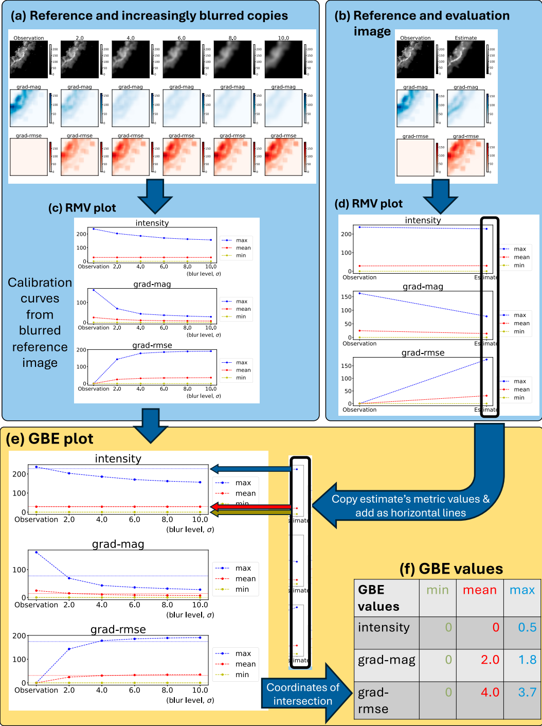
FIG. 7. Calculation of GBE plot and GBE values, illustrated using GREMLIN example and three sample metrics, intensity, Grad-Mag, and Grad-RMSE.
