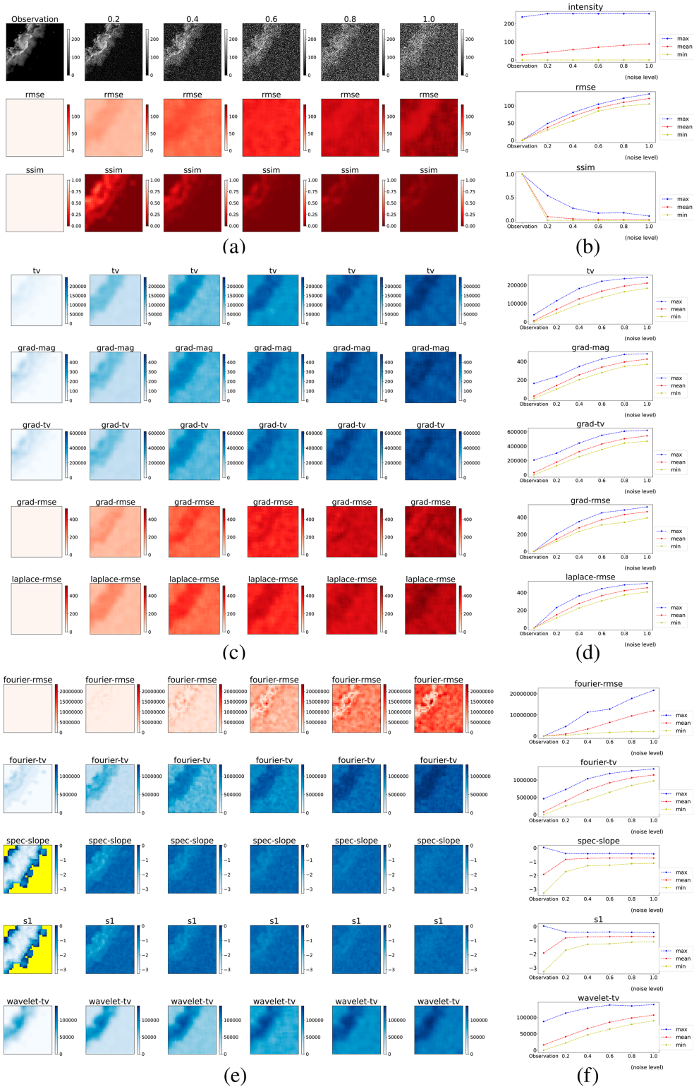
FIG. 14. Response of metrics to adding white noise to a satellite image. (a),(c),(e) Heat maps and (b),(d),(f) RMV plots for metric groups 1, 2, and 3.
