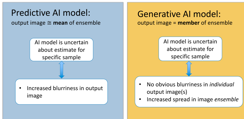
FIG. 3. How uncertainty is expressed in imagery from predictive vs. generative AI models.
