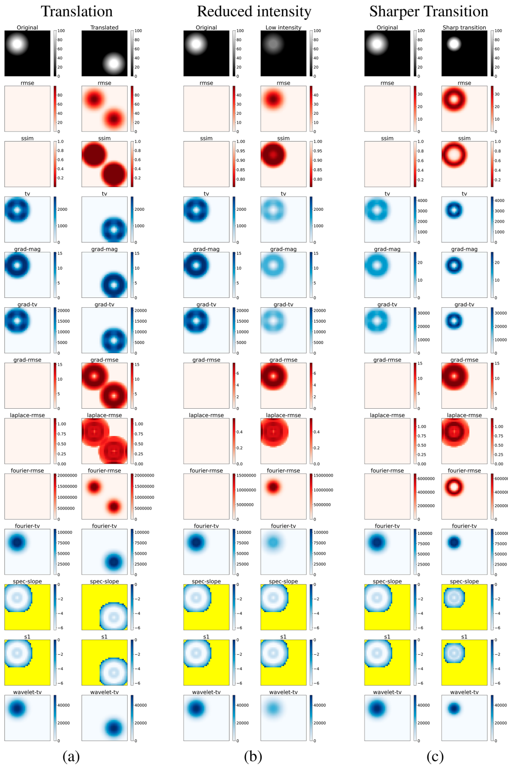
FIG. 16. Heat maps for all metrics demonstrating the effect of changing (a) the location of a feature, (b) intensity of an image (including all features), and (c) the rate of transition from feature to background.
