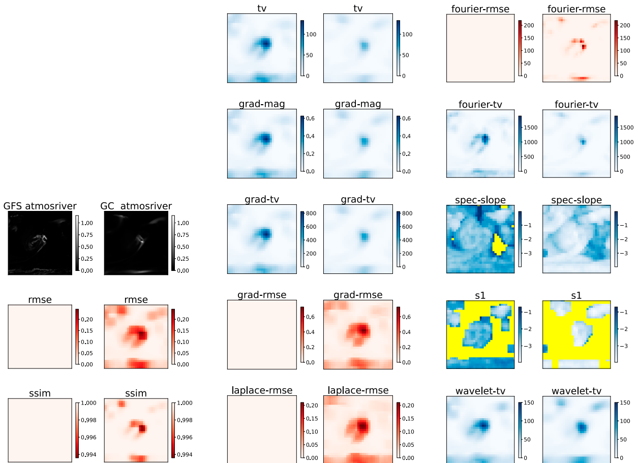
FIG. 12. Heat maps for the atmospheric river event for GFS vs. GraphCast forecasts of 6-h accumulated precipitation at a lead time of 168 h. The contrast threshold for metric S_1 used here is 0.1.
