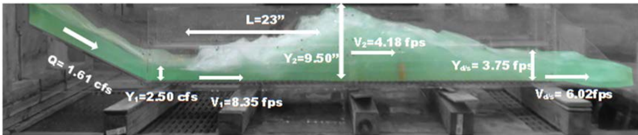
Figure 21. Hydraulic jump characteristics for Experiment 10C. 0.6% slope, 1.2d.
