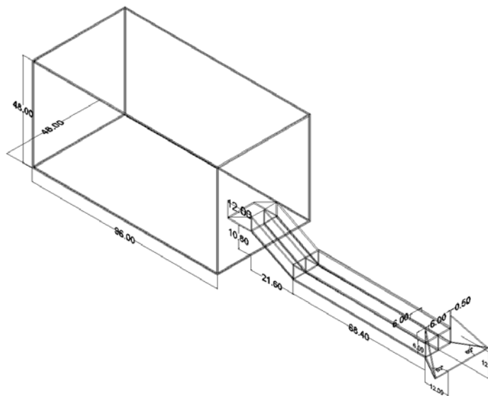
Figure 1-2. Model B: Pressure Flow
