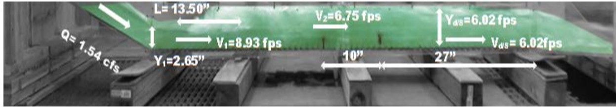
Figure 23. Hydraulic jump characteristics for Experiment 24C for 1% slope. 1.2d.
