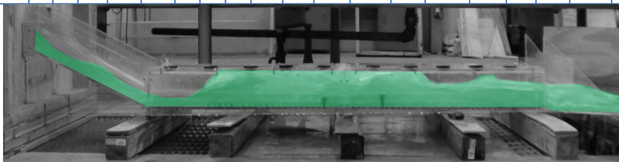
Figure A107. Experiment 36A for 0.3% slope.
