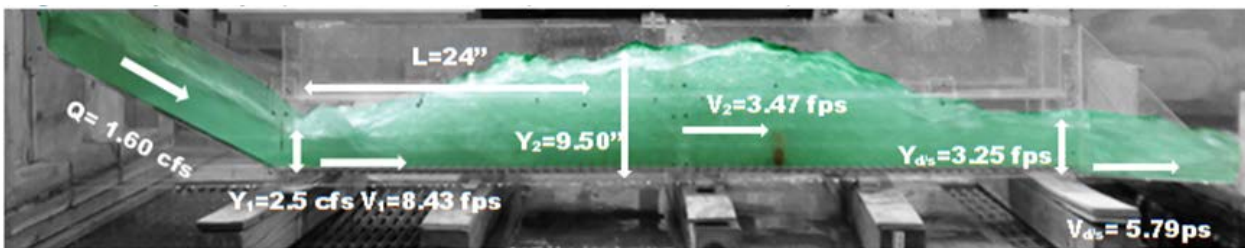
Figure 22. Hydraulic jump characteristics for Experiment 15C. 0.3% slope, 1.2d.
