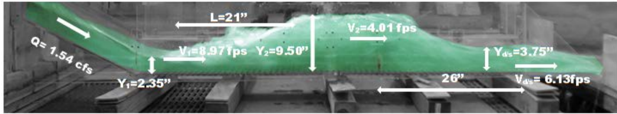
Figure 20. Hydraulic jump characteristics for Experiment 5C. 1% slope, 1.2d.
