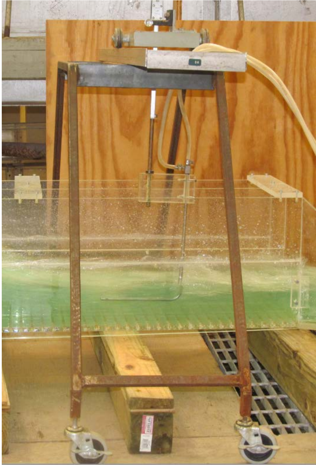
Figure 18. Pitot Tube with mount over the culvert model
