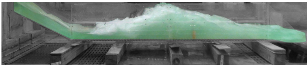
Figure A45. Experiment 15C for 0.3% slope.
