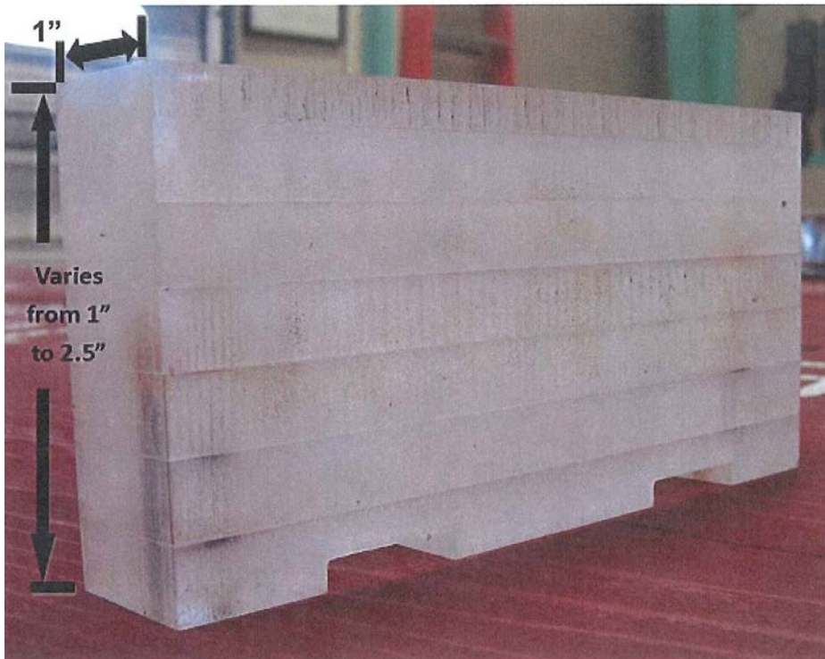
Figure 10. Typical sill dimensions
