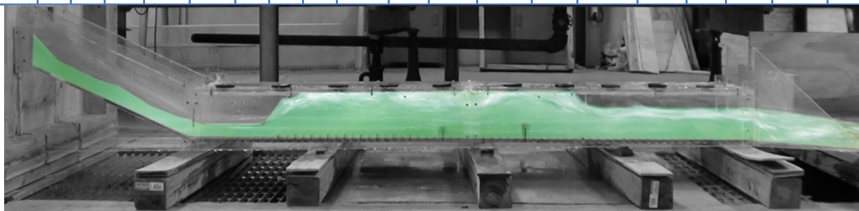
Figure A80. Experiment 27A for 1% slope.
