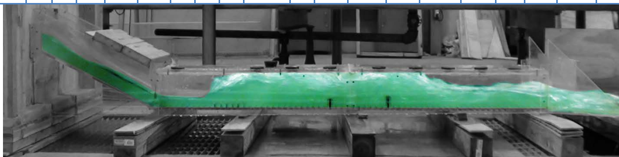
Figure A89. Experiment 30A for 0.6% slope.
