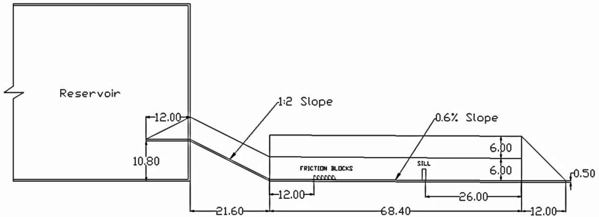
Figure 4. Profile View of 0.6% slope model
