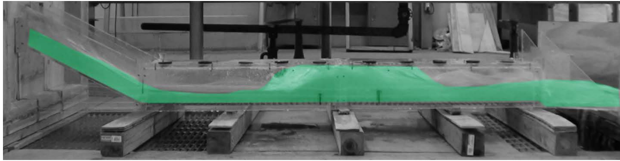
Figure A102. Experiment 34B for 0.3% slope.
