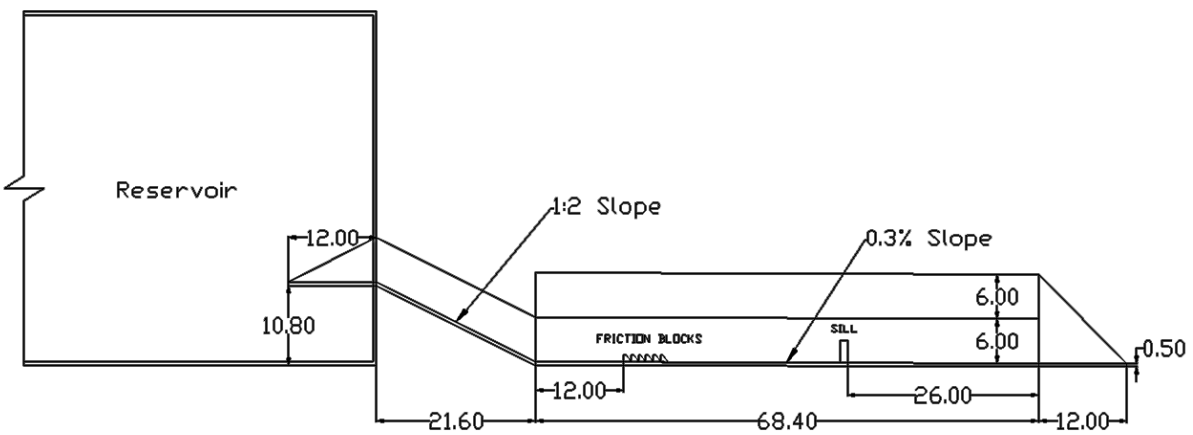
Figure 5. Profile View of 0.3% slope model
