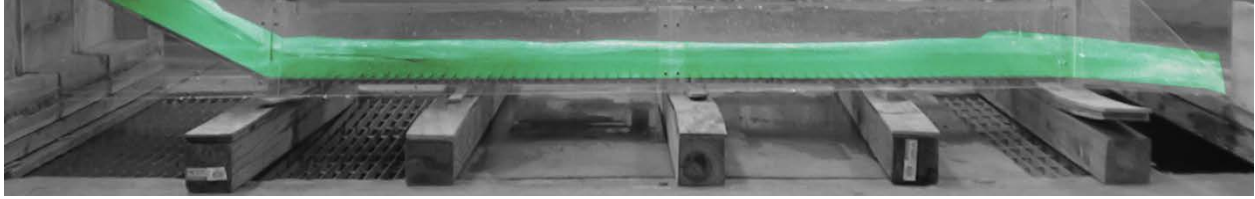
Figure A56. Experiment 19B for 1% slope.
