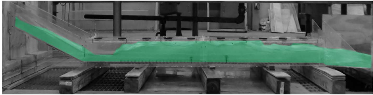
Figure A96. Experiment 32B for 0.6% slope.
