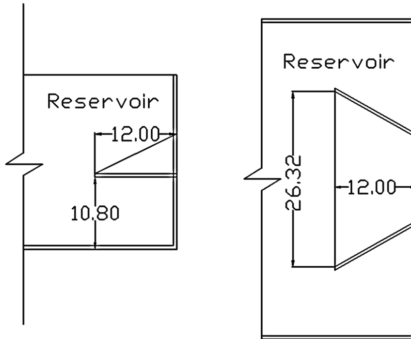
Figure 6. Profile and Plan View of Reservoir Inlet (Upstream)
