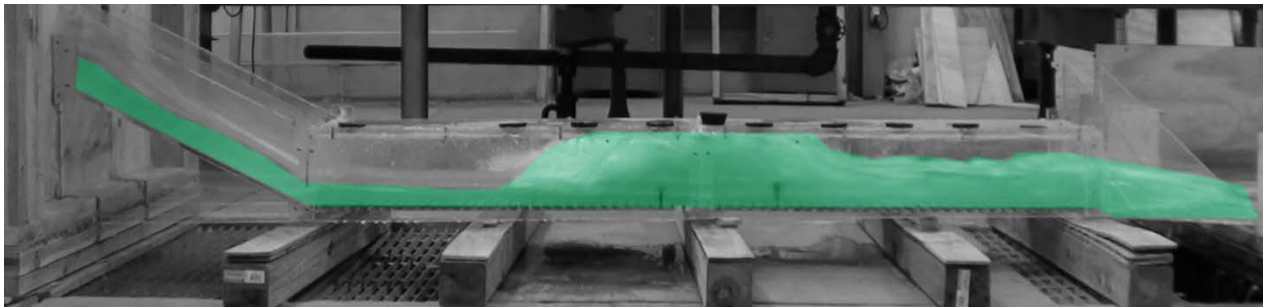
Figure A86. Experiment 29A for 0.6% slope.
