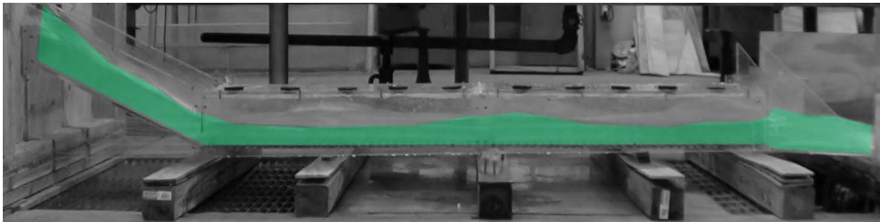
Figure A100. Experiment 33C for 0.3% slope.
