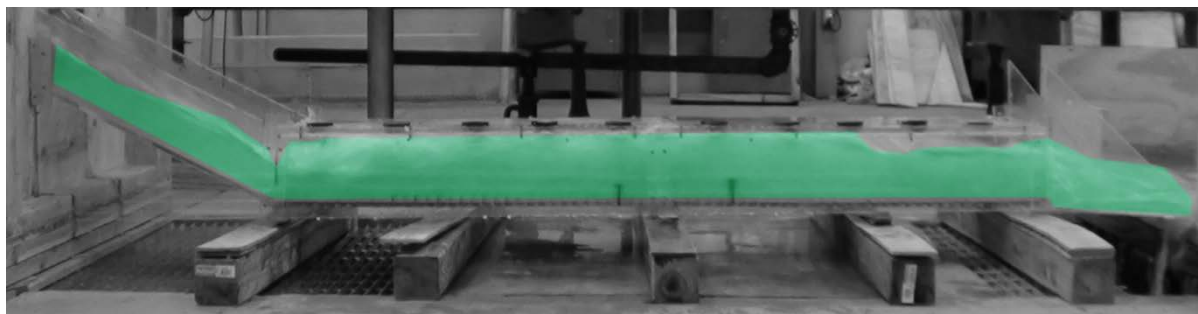
Figure A109. Experiment 36C for 0.3% slope.
