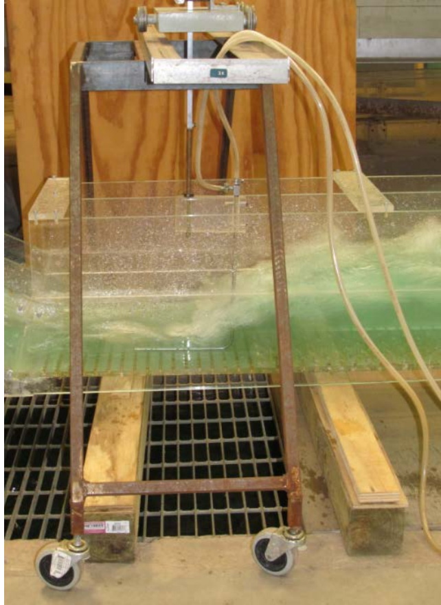
Figure A117. Pitot Tube plugged in culverts upstream to V_{u/s}
