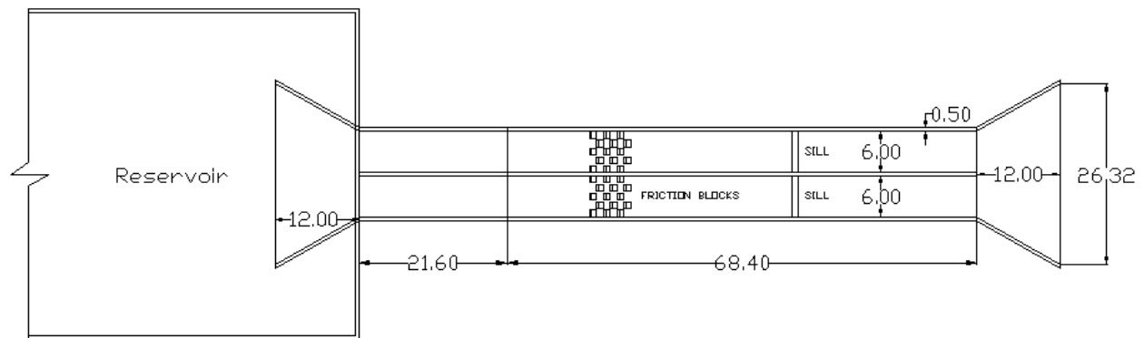
Figure 2. Plan View of model
