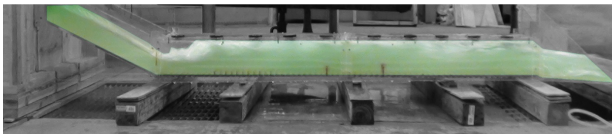
Figure A79. Experiment 26C for 1% slope.
