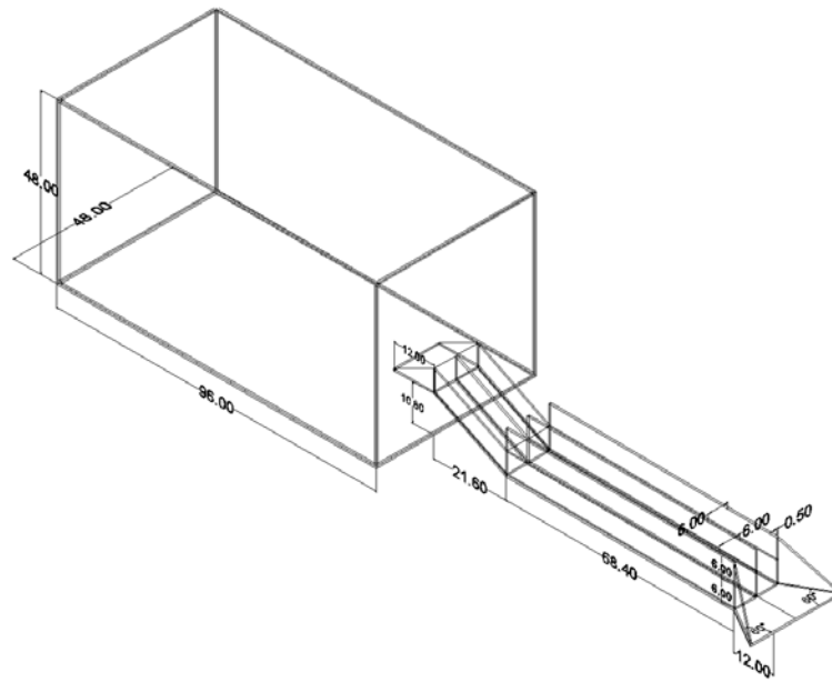
Figure 1-1. Model A: Open Channel Flow
