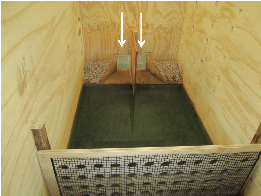
Figure 15. Reservoir and channel inlet for culvert model.
