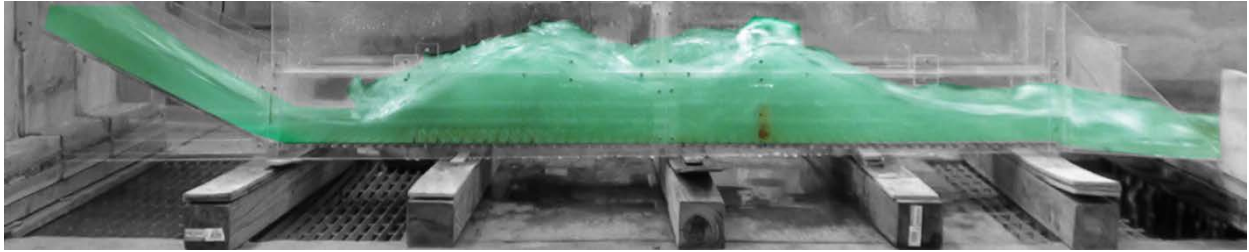
Figure A50. Experiment 17B for 0.3% slope.
