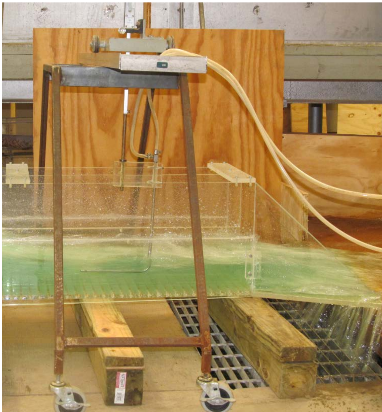
Figure A116. Pitot Tube plugged in culverts downstream to V_{d/s}
