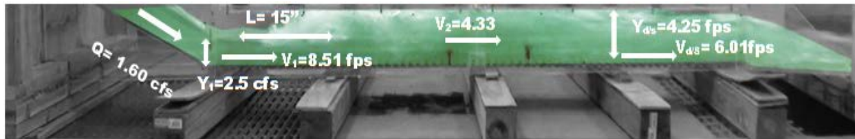
Figure 25. Hydraulic jump characteristics for Experiment 34C for 3% slope, 1.2d
