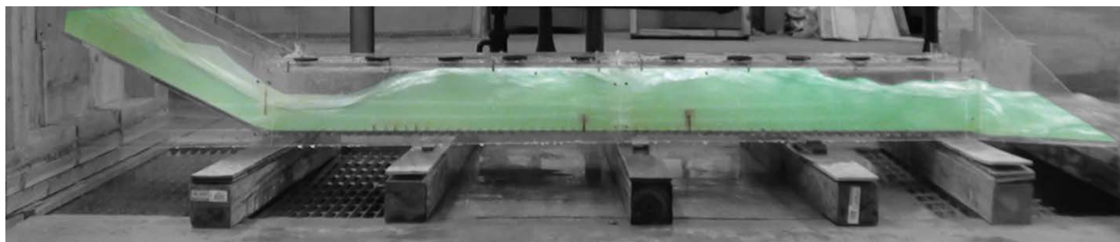
Figure A75. Experiment 25B for 1% slope.
