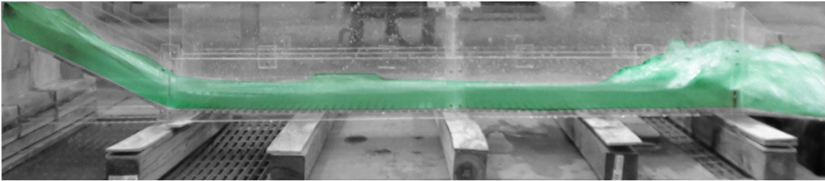
Figure A5. Experiment 2B for 1% slope
