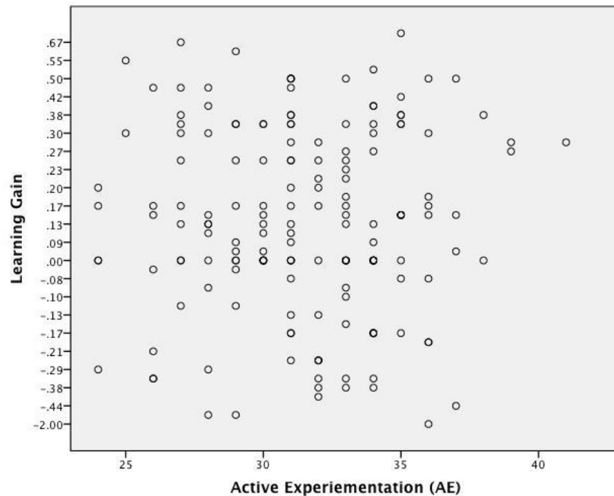
Figure 4.10. Relationship between preference for Active Experimentation on the LSI and learning gain
