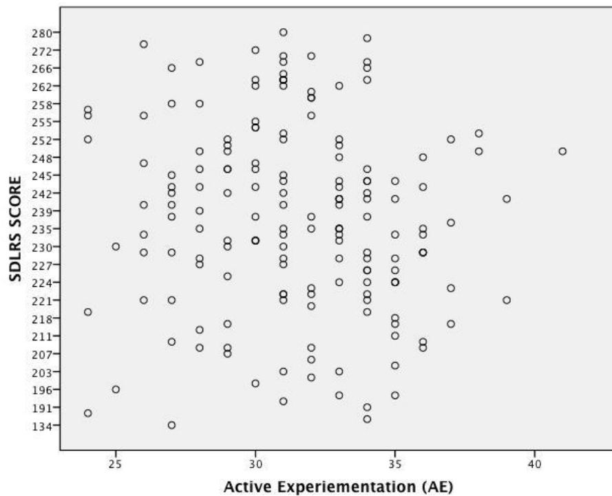
Figure 4.11. Relationship between SDLRS score and AE preference
