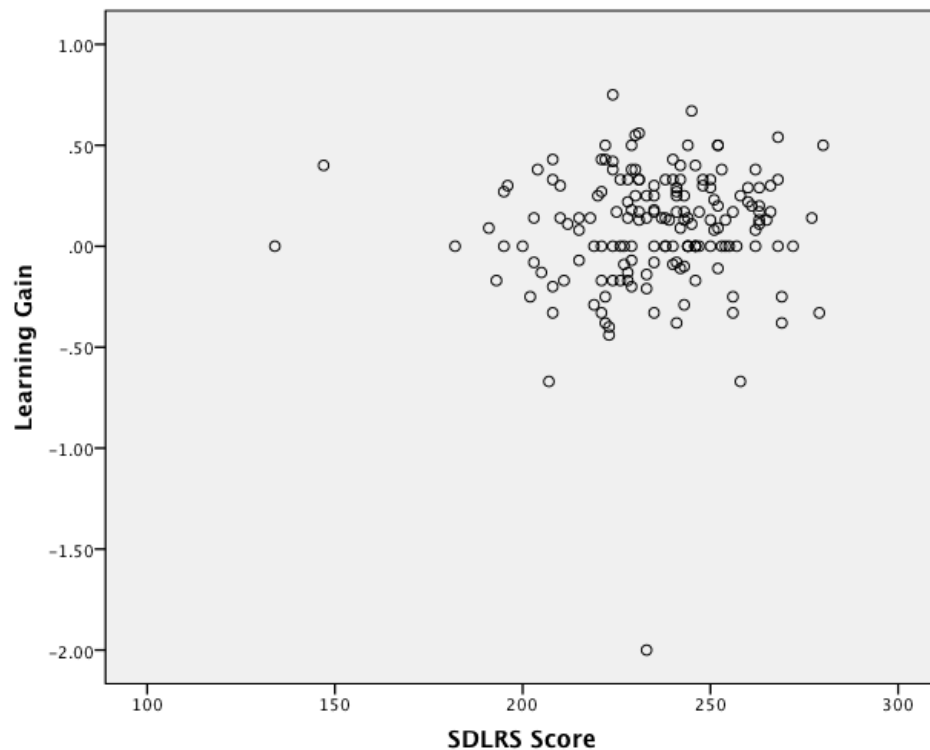
Figure 4.9. Relationship between SDLRS score and employees' learning gain
