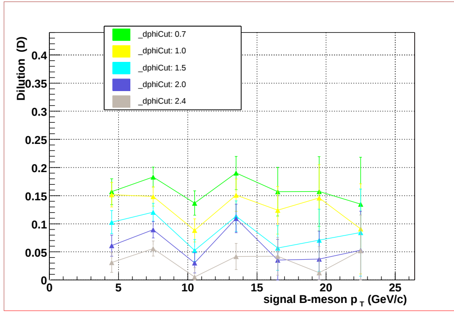
Figure 7.5: The tagging dilution for the MC Gluon Splitting B- sample. .
