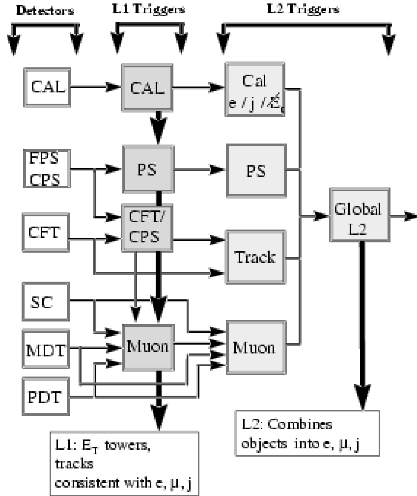
Figure 3.16: L1 and L2 trigger elements. The horizontal arrows denote information flow.
