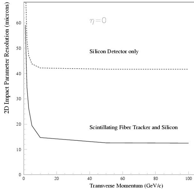
Figure 4.3: Resolution of 2-dimensional DCA for the global tracks at \eta=0 as a function of transverse momentum.
