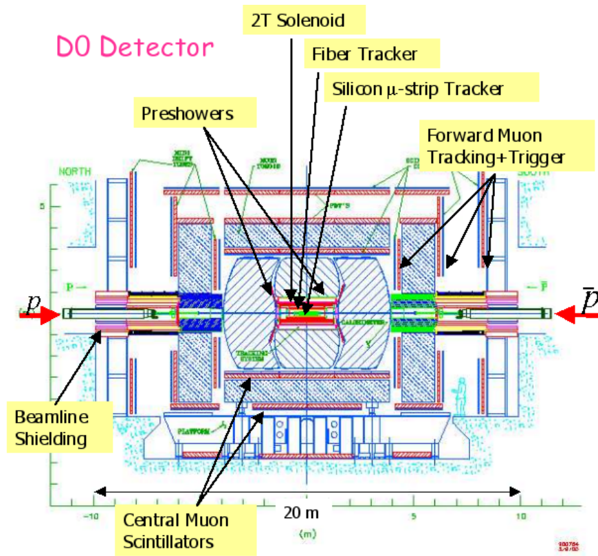
Figure 3.3: The r-z view of the DØ Run II detector
