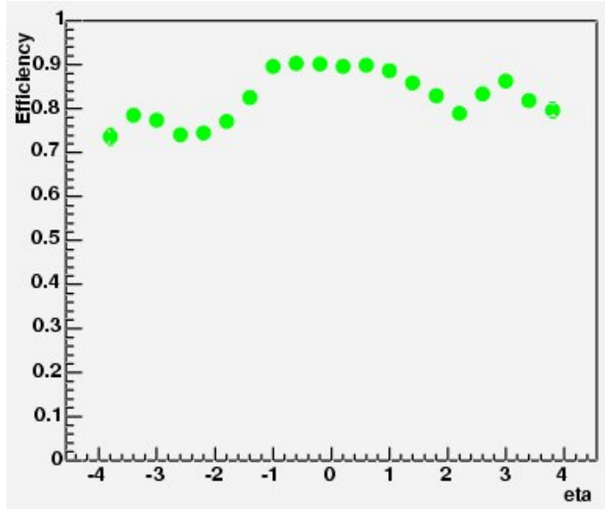
Figure 4.4: The reconstruction efficiency of the tracks on Z \rightarrow \mu\mu events.
