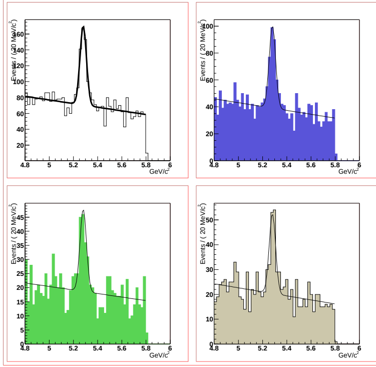
Figure 10.1: Invariant mass for candidate B \rightarrow J/\psi K_s events. The data sample was obtained by DØ Run II detector, corresponding to 225 \text{ pb}^{-1} luminosity. The first plot is for all candidate B , the second plot is for tagged events, the third is for the events tagged as B^0 , the last is for the events tagged as \bar{B}^0 .
