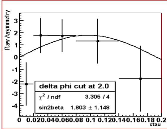
Figure 10.2: The time dependent measurement of CP asymmetry parameter \sin(2\beta) with different \Delta\phi cuts.
