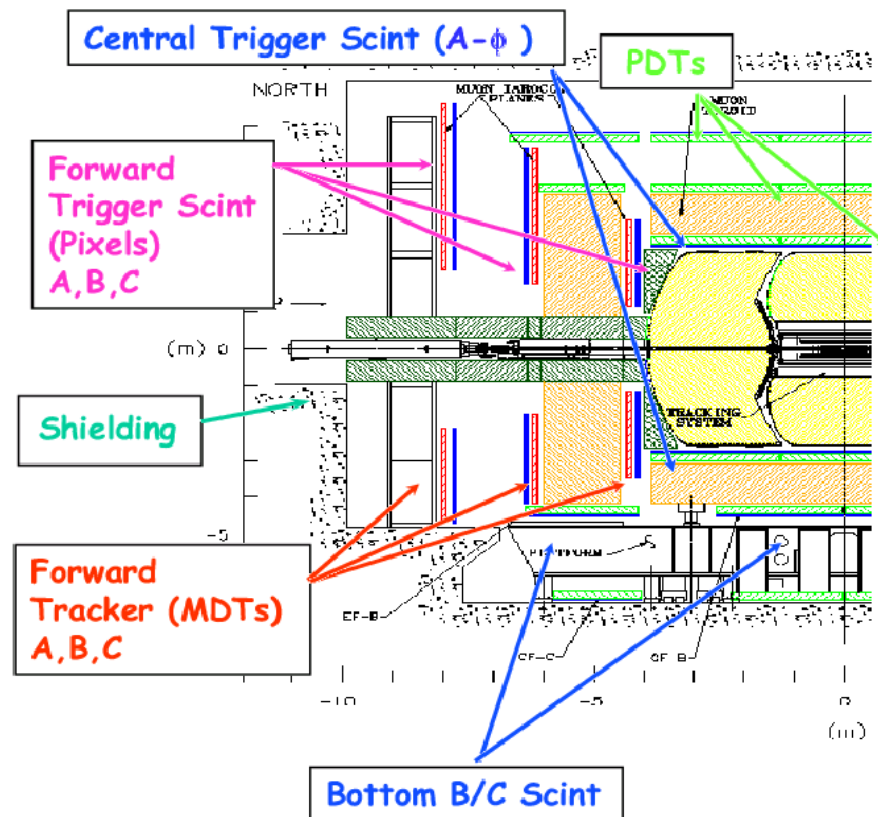
Figure 3.14: The r-z view of the half muon system.
