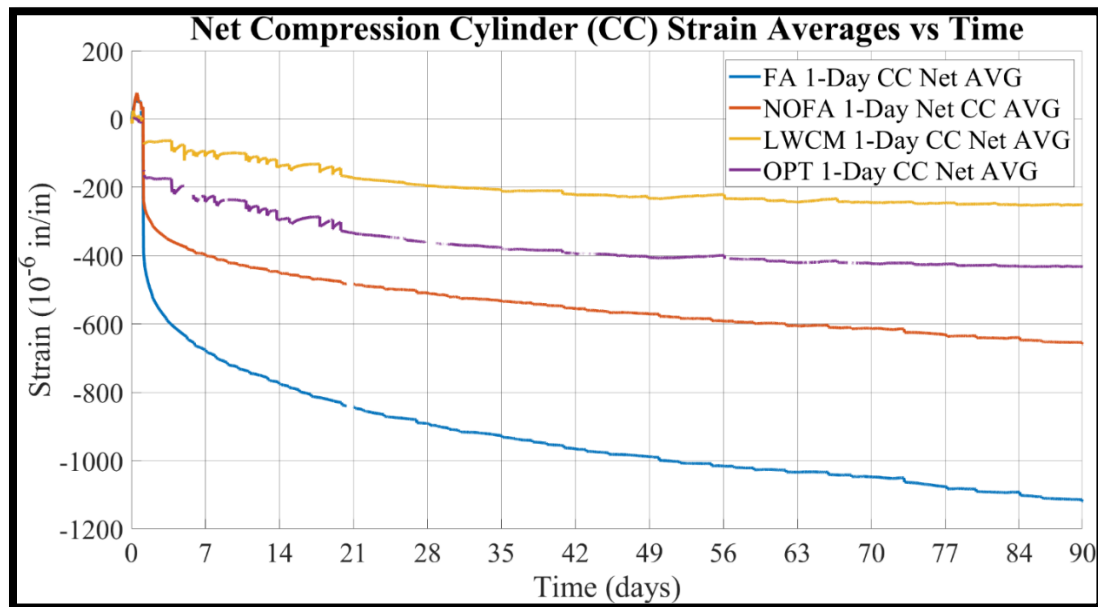
Figure 5.11 Net Compression Strain vs. Time.
