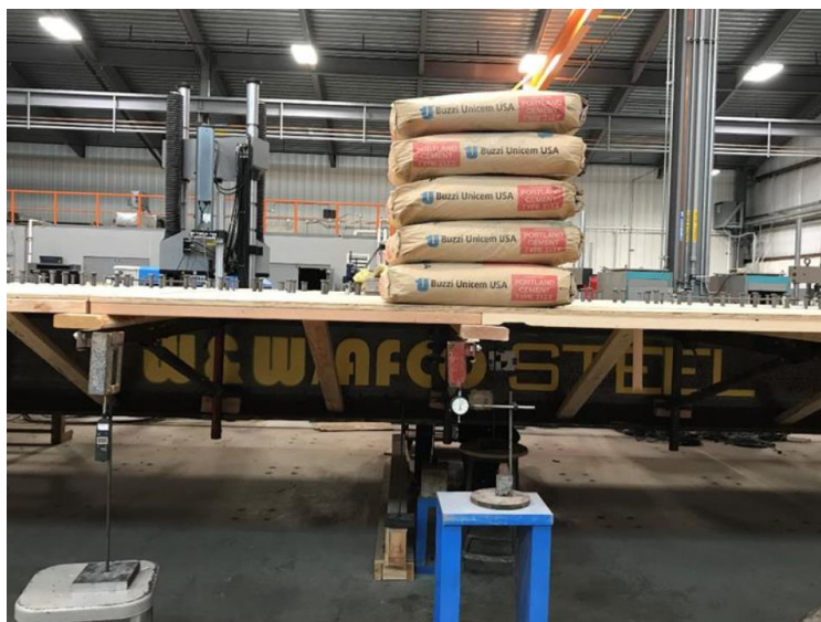
Figure 4.4: Cement sacks are being used to provide eccentric loading to the formwork and bracing systems in order to measure the load effects on temporary structures.
