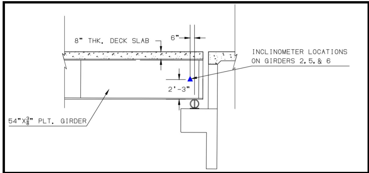
Figure 6.2: Inclinator sensor location drawing
