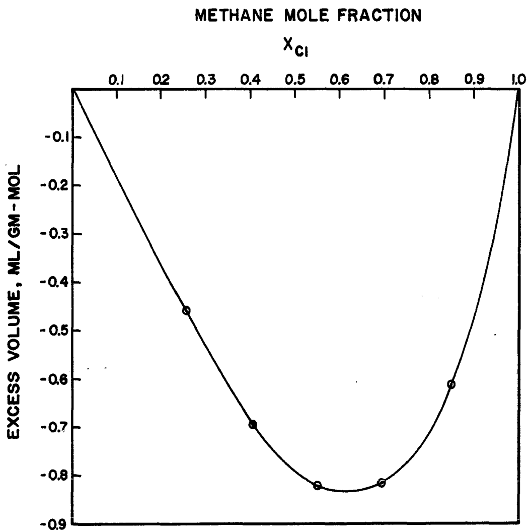
Figure 11. EXCESS VOLUME OF METHANE+PROPANE MIXTURE AT -165.0°C.
