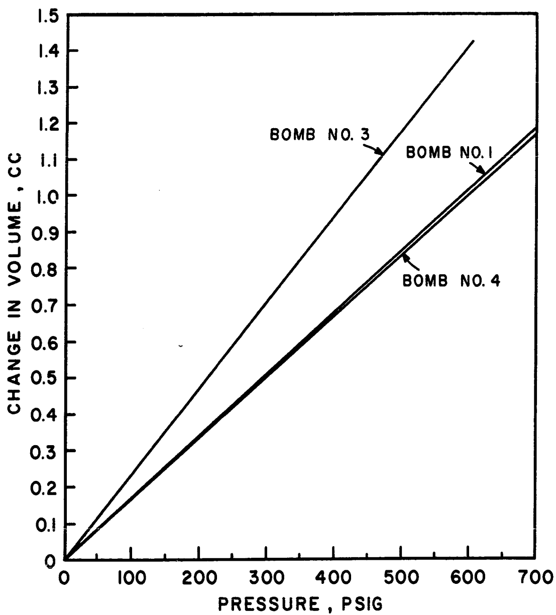
FIGURE B-1. CHANGE IN THE VOLUME OF THE WEIGHING BOMB AS A FUNCTION OF PRESSURE.
