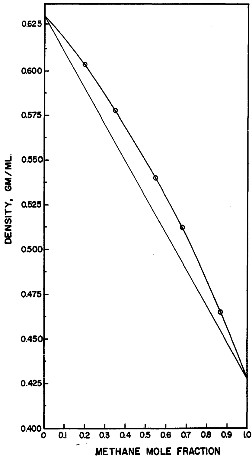
Figure 7. SATURATED LIQUID DENSITY OF METHANE+ETHANE MIXTURE AT -165.0°C
