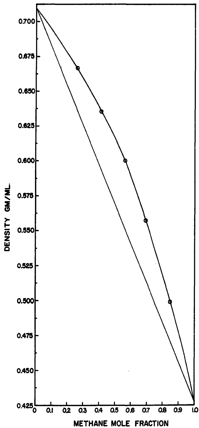
Figure 8. SATURATED LIQUID DENSITY OF METHANE+ PROPANE MIXTURE AT -165.0°C.
