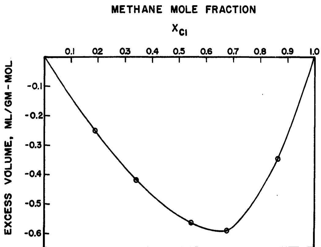
Figure 10. EXCESS VOLUME OF METHANE+ETHANE MIXTURE AT -165.0°C.
