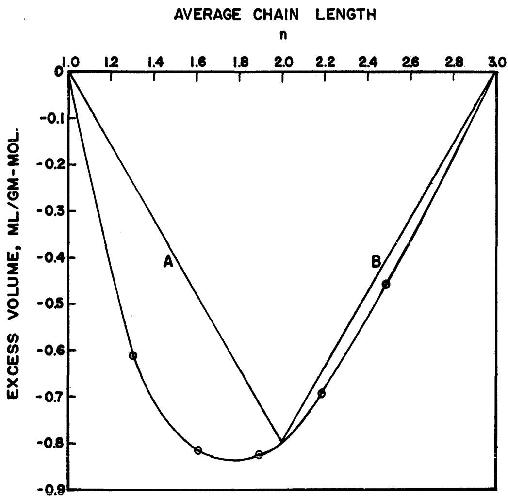
Figure 13. EXCESS VOLUME OF METHANE + PROPANE MIXTURE AT -165.0^{\circ}\text{C} VS. AVERAGE CHAIN LENGTH
