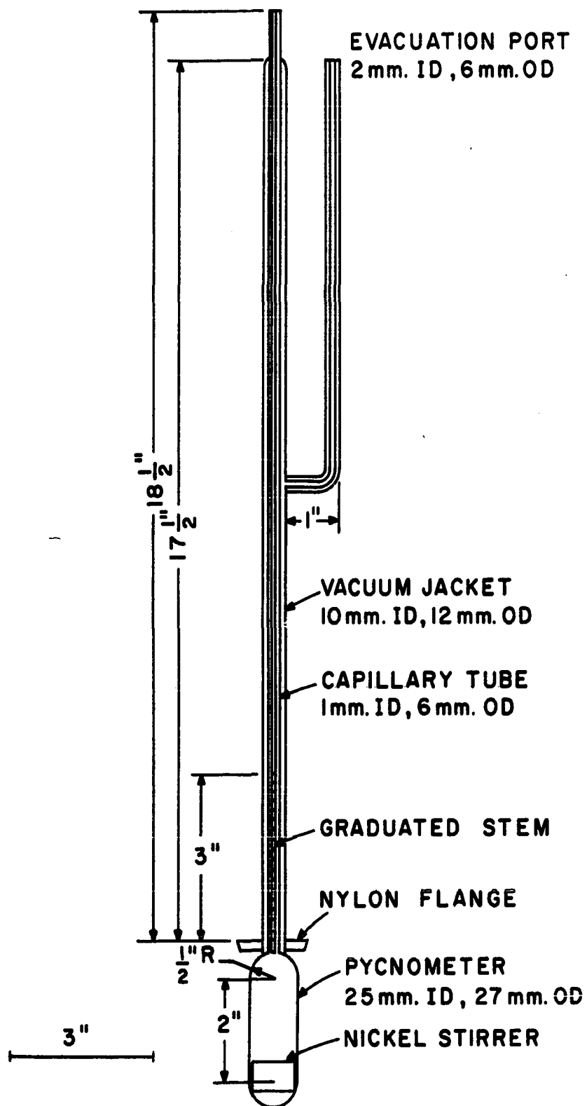
FIGURE 4. SCHEMATIC DIAGRAM OF FUSED QUARTZ PYCNOMETER.
