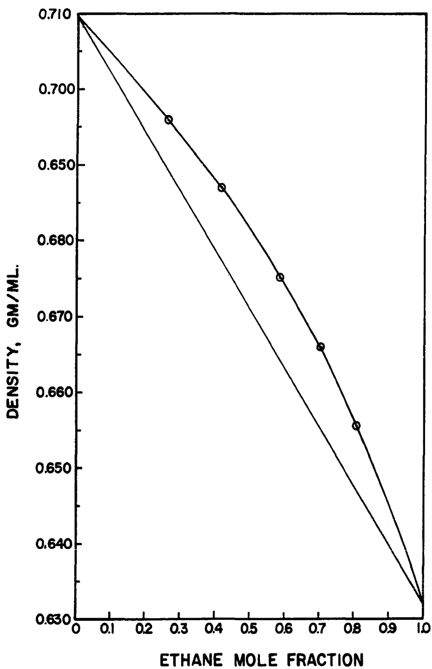
Figure 9. SATURATED LIQUID DENSITY OF ETHANE+ PROPANE MIXTURE AT -165.0°C.
