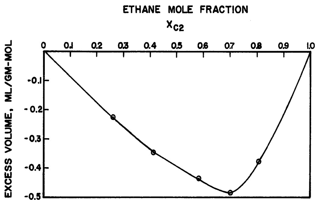
Figure 12. EXCESS VOLUME OF ETHANE+PROPANE MIXTURE AT -165.0°C.
