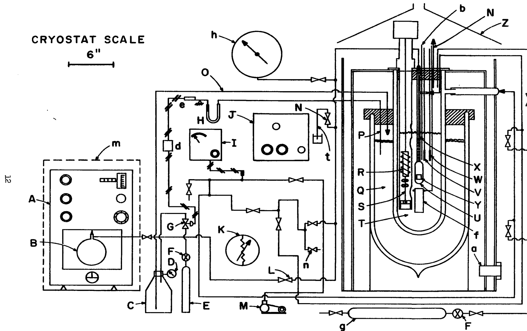
FIGURE I. SCHEMATIC DIAGRAM OF THE EXPERIMENTAL APPARATUS
