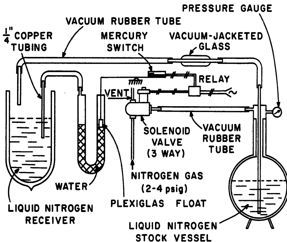
Figure 5. AUTOMATIC CONTROL OF THE LIQUID NITROGEN LEVEL.
