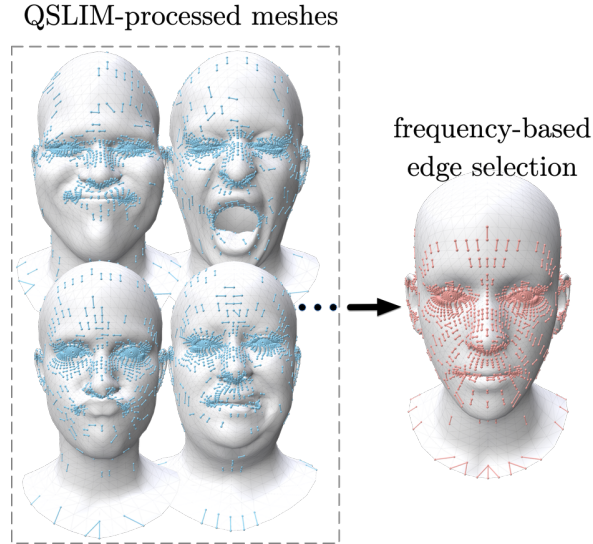
Figure 3.2: QSLIM is applied to the meshes, and edges are selected based on their frequency. Red edges show those contracted during down-sampling.
