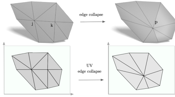
Figure 3.3: Utilizing conformal parameterization to map the 1-ring of a collapsed edge to the UV space. Notably, the vertices post and pre-collapse maintain identical boundary vertices.
