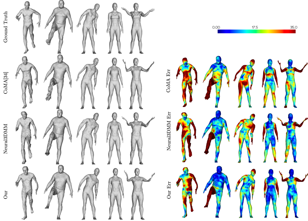
Figure 2.6: Colour coding of the per vertex euclidean error of the reconstructions. Top row is ground truth. The error values are saturated at 35 (millimeters)
