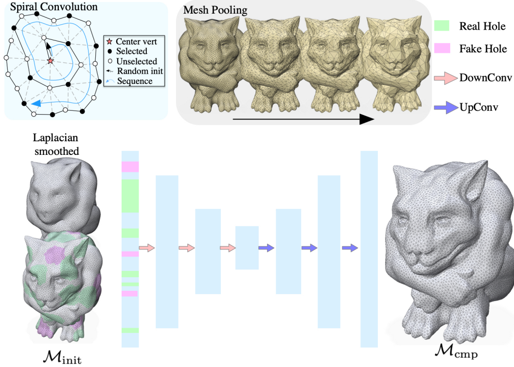
Figure 5.5: Self-supervised training of our refinement model. Pooling and unpooling are implemented via QSLIM-based precomputed transformation matrices, consistent with prior mesh autoencoder designs [20]. The model predicts vertex displacements to reconstruct the inpainted surface from an oversmoothed mesh using both real (green) and fake (pink) holes.
