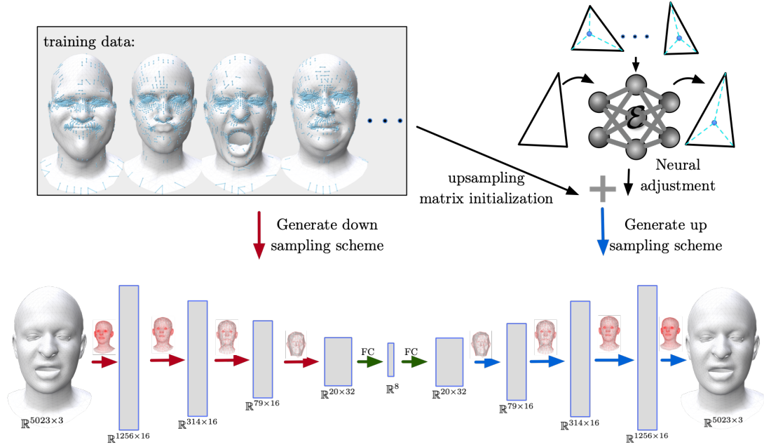
Figure 3.1: Unlike standard mesh autoencoders that build down/up matrices from a single mesh, our method employs a novel coarsening scheme and neural unpooling layer on a fixed topology mesh dataset. The resulting transformation matrices or hierarchies can be seamlessly integrated into mesh generative models without altering the user’s network architecture.
