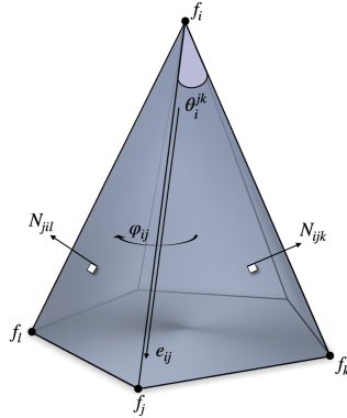
Figure 2.9: Discrete schematic diagram, N_{ijk} is unit normal of triangle ijk , \theta_i^{jk} is interior angle at vertex i of triangle ijk , \varphi_{ij} is dihedral angle at oriented edge ij .
