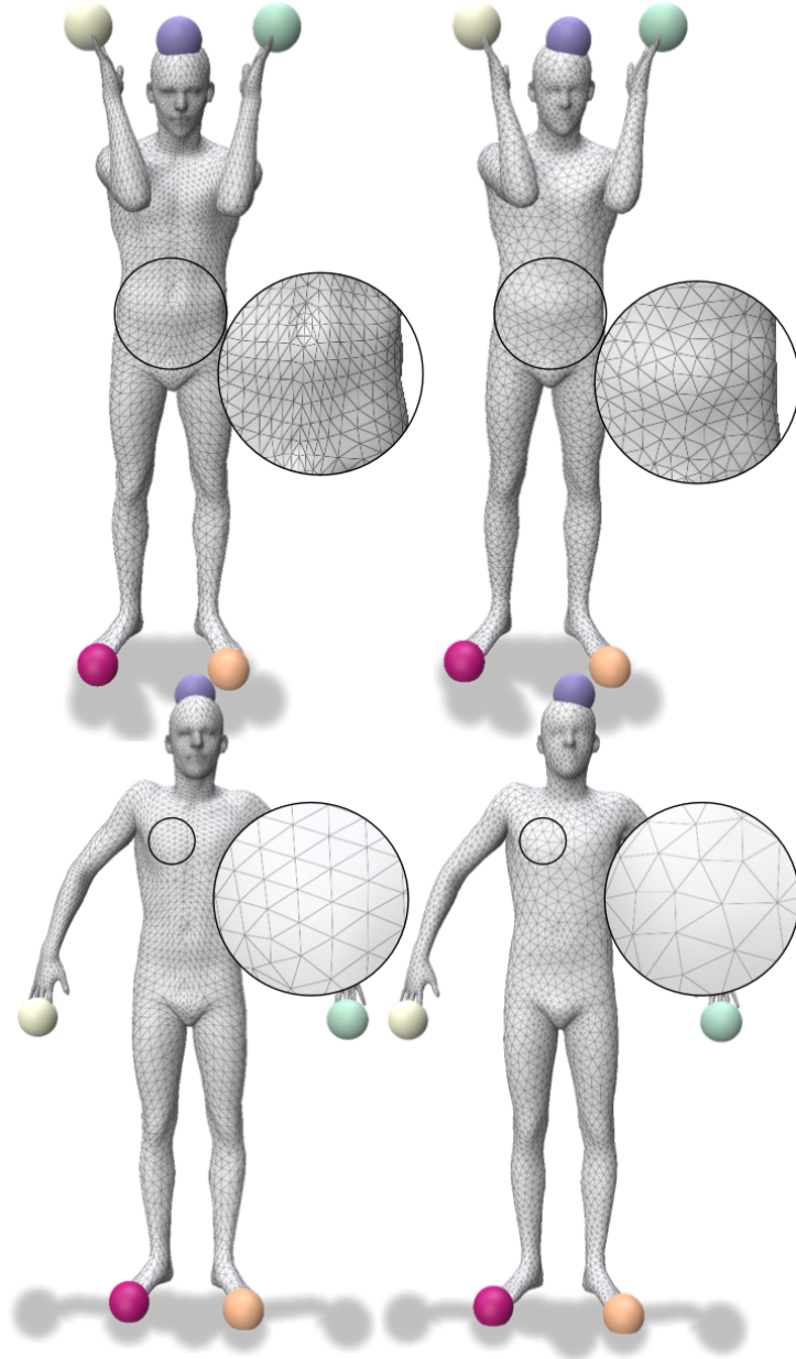
Figure 4.11: Our approach produces stable and consistent landmark placement across remeshed surfaces (right), demonstrating sampling and resolution agnosticism. This robustness enables reliable shape matching across a wide range of mesh representations, including those with significantly different vertex counts.
