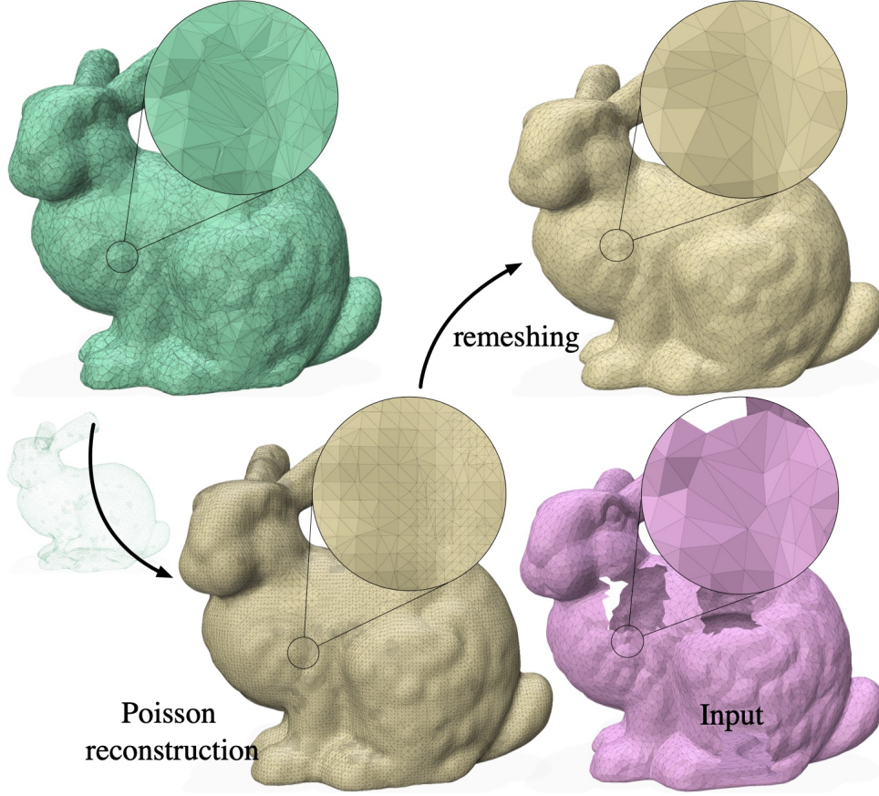
Figure 5.3: Poisson surface reconstruction is applied to the initial isosurface to improve mesh quality, followed by remeshing to ensure a uniform vertex density comparable to the input mesh.
