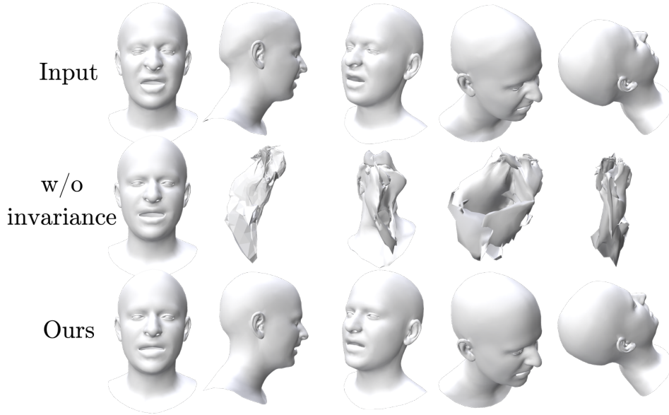
Figure 3.7: Employing local coordinates embedded within each mesh as both inputs and outputs, our methodology achieves invariance to rigid motions. This adaptation yields a marked enhancement in quality relative to preceding methods that lack such invariance.
