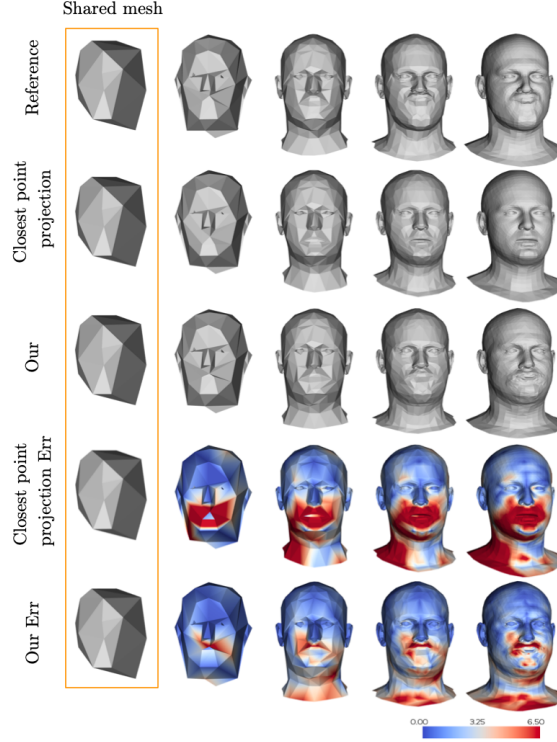
Figure 2.8: Visualization of unpooling meshes with error: The first row lists the pooling meshes in reverse order. The two unpooling methods share the same initial coarse mesh. The second and third rows present the results of the closest point projection [20, 22] and our proposed unpooling method, respectively. The error values are saturated at 6.5 (millimeters)
