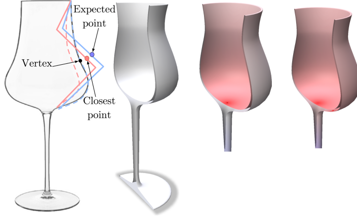
Figure 3.4: Heat diffusion illustrated on a wine glass. Through local mapping, inside-out projection is avoided, resulting in an outward heat spread on the surface (center right), as opposed to the incorrect heat flow caused by closest point projection (right).
