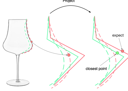
Figure 2.3: Closest point projection
