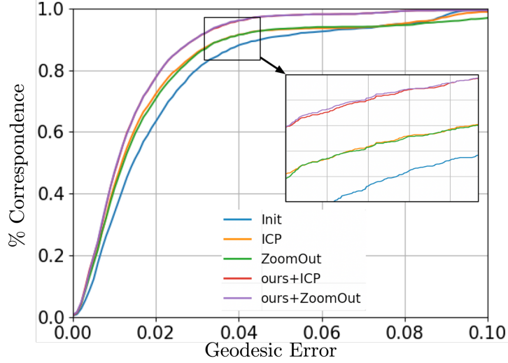
Figure 4.10: Evaluation on Dynamic FAUST using geodesic error measures. We present ICP and ZoomOut predictions both before and after applying our augmentation. The initialization parameters are set to w_{d-comm} = 0.1 and w_{orient} = 0.1 .
