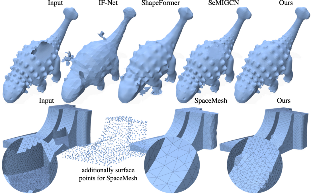
Figure 5.7: Comparison with representative data-driven methods. While IF-Net and ShapeFormer produce coarse reconstructions and SeMIGCN failed to inpaint the shape geometries, SpaceMesh additionally requires surface point inputs. Our method achieves clean, detailed, and watertight repairs directly from the incomplete mesh.
