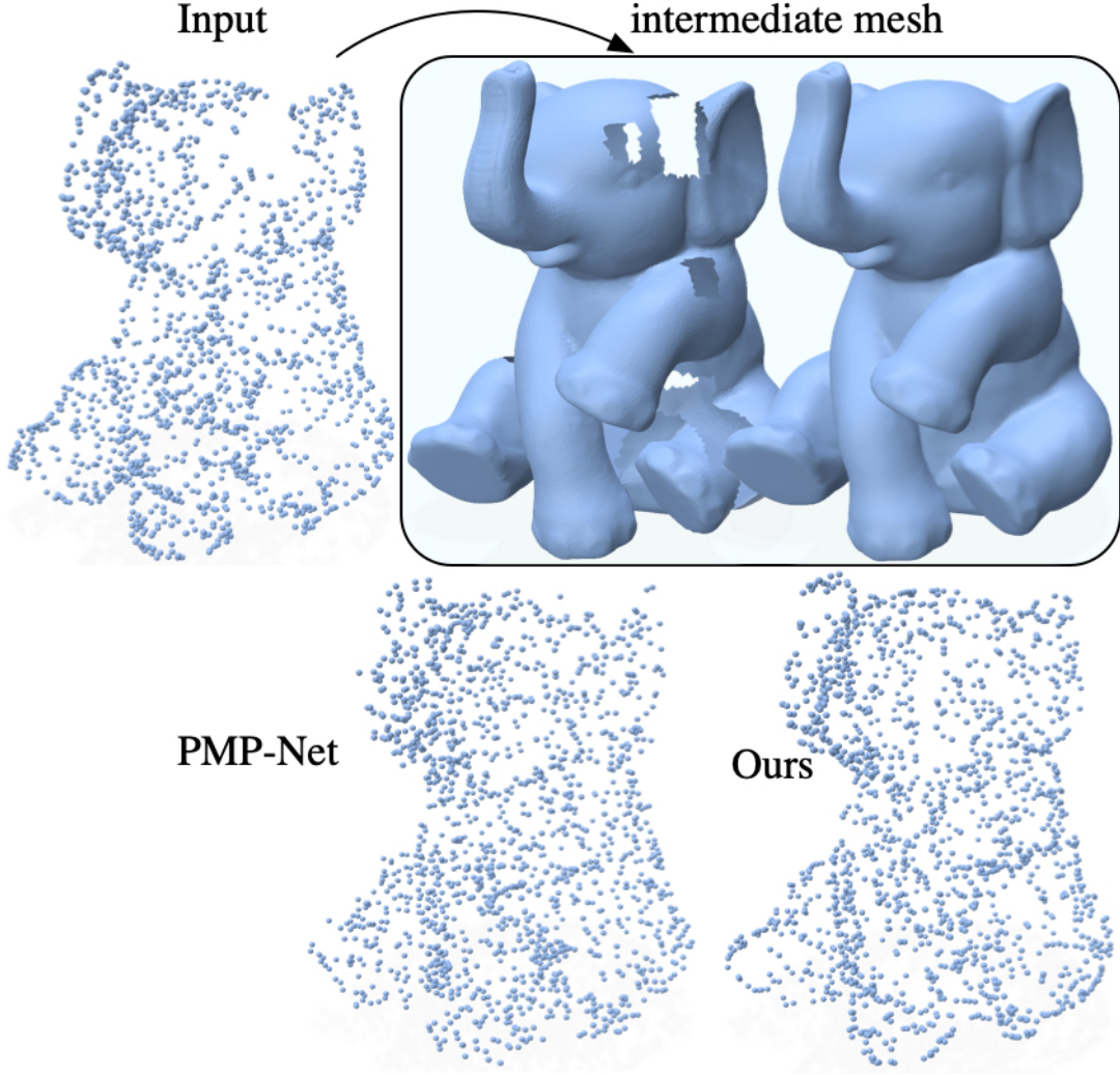
Figure 5.8: Point cloud completion results. Our method reconstructs an intermediate mesh from the incomplete input, repairs it, and resamples a consistent point cloud.
