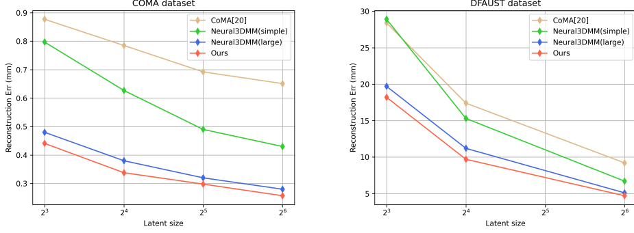
Figure 2.7: Reconstruction errors of different methods
