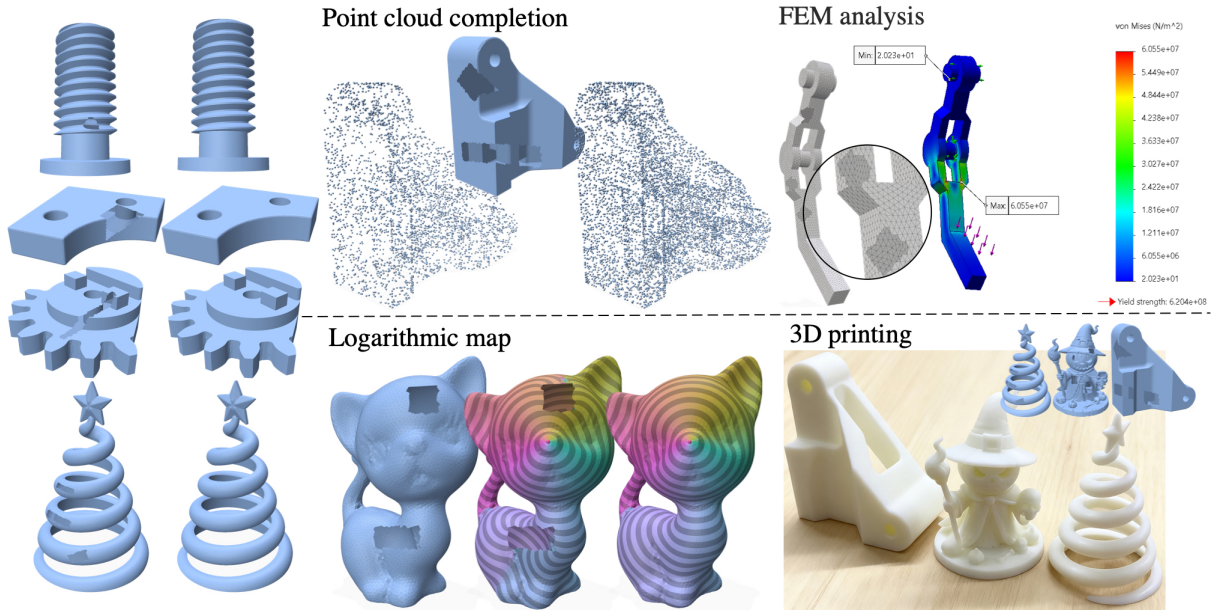
Figure 5.1: Our data-free neural mesh inpainting method restores missing regions directly on the input mesh while preserving geometric and topological consistency. The repaired meshes can be seamlessly applied to downstream tasks such as point cloud completion, FEM simulation, logarithmic map computation, and 3D printing.
