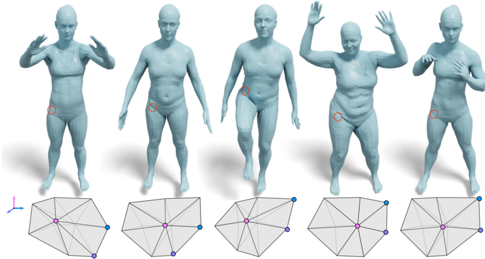
Figure 3.6: Registered data allows us to order the three vertices of the triangle canonically. We feed vertex features into multi-layer perceptrons (MLP).
