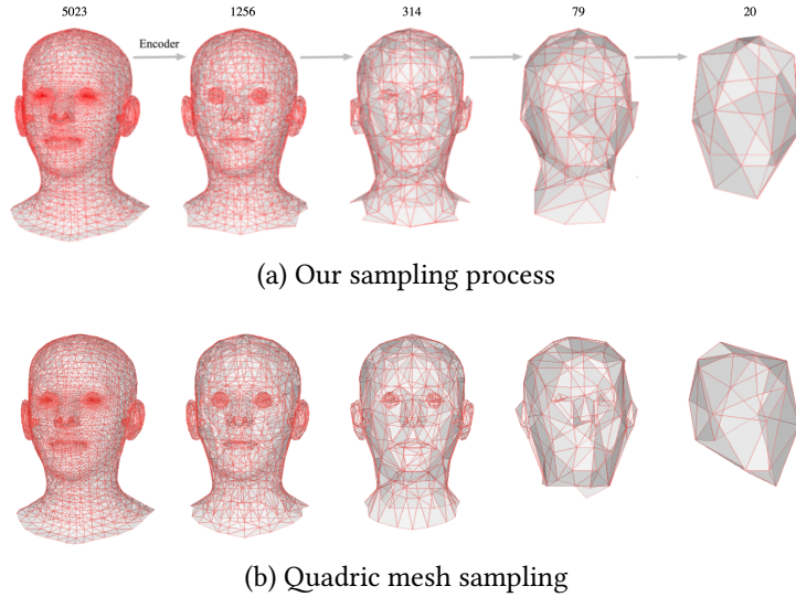
Figure 2.2: Network architecture and comparison for mesh sampling
