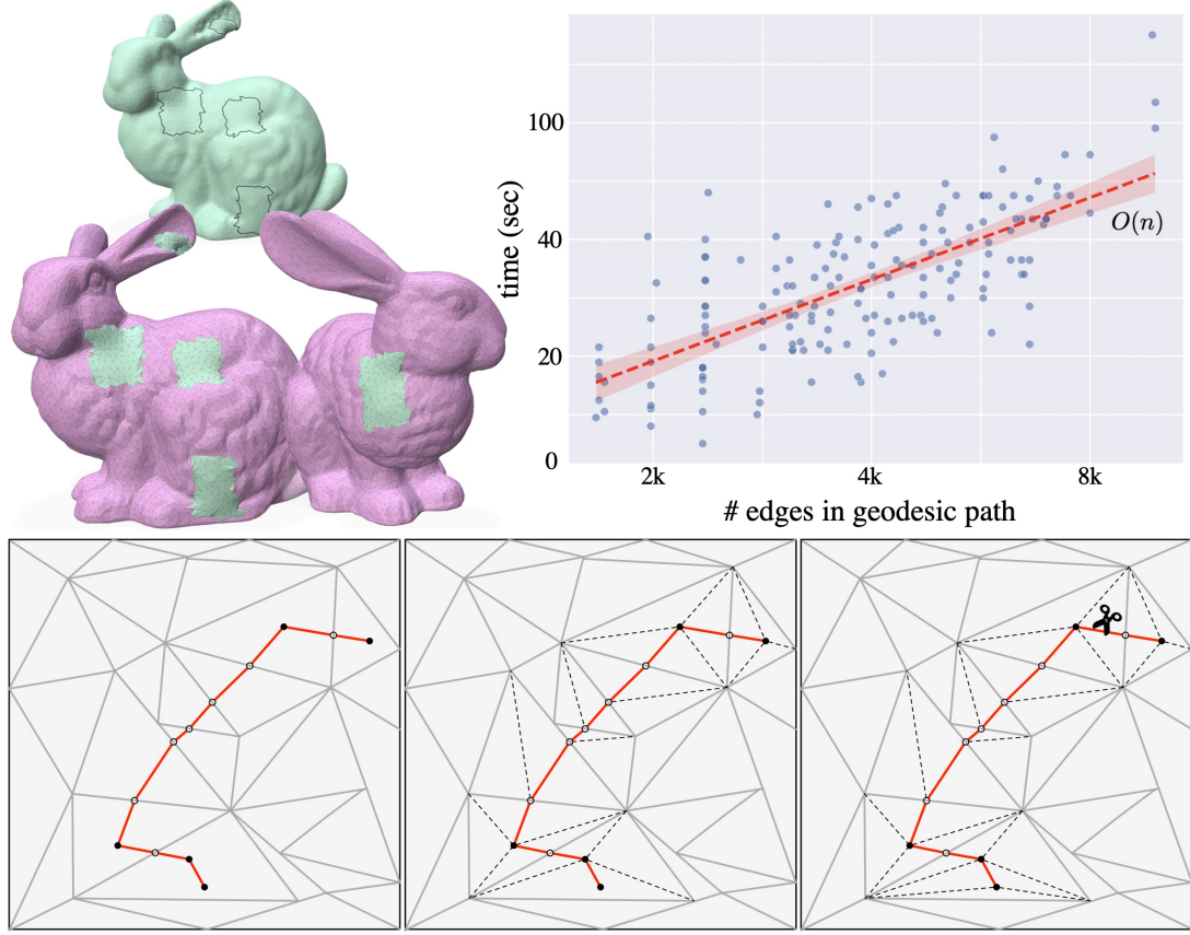
Figure 5.4: Top: path stitching between the projection and input meshes. Bottom: retriangulating the faces intersected by the geodesic yields a valid cutting path (red) represented by mesh edges. The measured runtime (top-right) confirms a linear O(n) relationship between path length and computation time. In this example, the bunny model contains 14K faces, with 400 edges along the geodesic path, and the entire cutting process takes 2.1 seconds.
