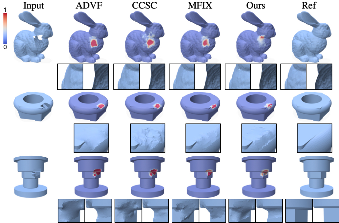
Figure 5.6: Inpainting results on meshes with holes. The reconstructed meshes are colorized according to the distance to the ground-truth surfaces. Traditional geometry-based methods tend to produce noticeable bulges or inward dents near the repaired regions, while our method yields smoother and more accurate reconstructions.
