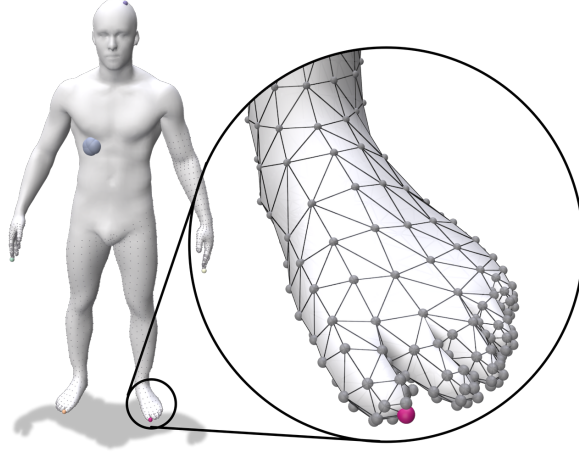
Figure 4.5: Selecting the vertices with the greatest geodesic distance from the set of Karcher means, shown in light blue
