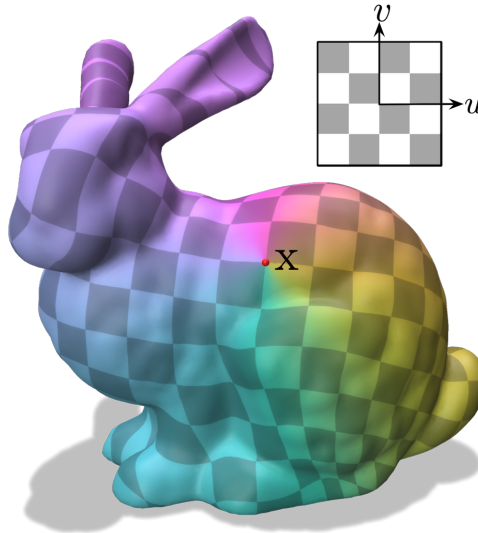
Figure 4.1: The logarithmic map refers to a specific 2D parameterization of a surface, relative to a chosen point x . A global logarithmic map facilitates the translation of algorithms from the Euclidean space to curved domains.
