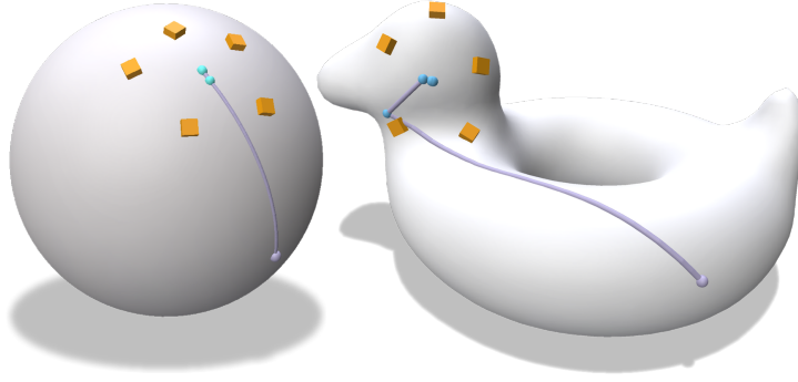
Figure 4.2: In the case of the Karcher mean, given a collection of points, we can get the expected solution in just 2–3 steps; here we show selected points (orange), and the initial guess (purple).
