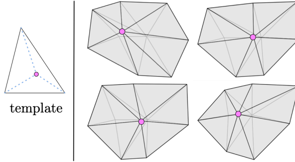
Figure 3.5: Barycentric coordinates resulting from mapping discarded vertices to the closest triangle are depicted. Despite contracting the same edge to the same end, the projection point differs depending on the given geometry. Relying solely on the template representation leads to an inaccurate up-sampling matrix.
