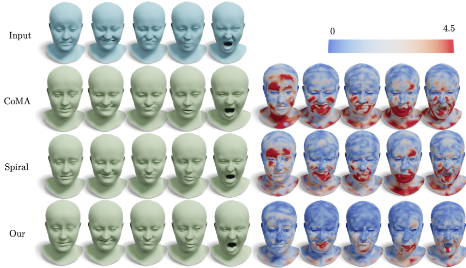
Figure 3.9: Qualitative assessment of reconstruction outcomes. Each vertex’s Euclidean error is color-coded, with the error values capped at 4.5 millimeters. Warmer hues denote larger errors.
