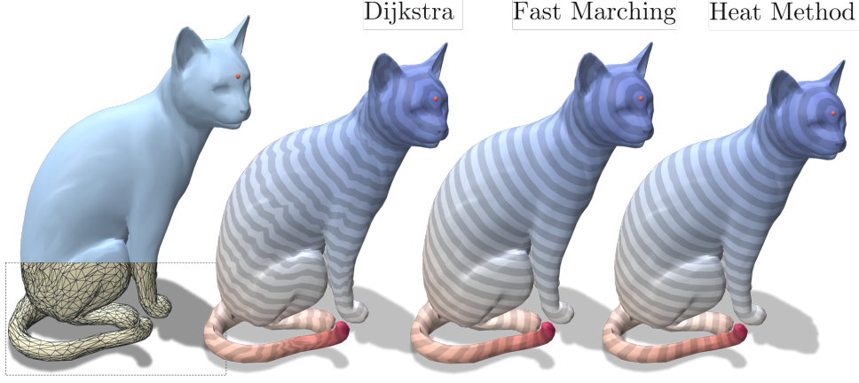
Figure 4.3: Comparison of geodesic distance fields computed using Dijkstra, Fast Marching, and the Heat Method. The heat method, based on solving linear elliptic PDEs, produces smoother distance isolines with fewer numerical artifacts, especially on irregular meshes. According to benchmarks by Crane et al. [116], the heat method achieves up to 68 \times speedup over Fast Marching on large meshes (e.g., 1.45s vs. 98.1s on a 1.6M-triangle model) with comparable or better mean error.
