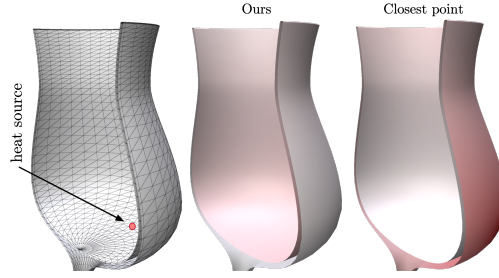
Figure 2.4: The heat source is placed inside the wine glass. The closest projection caused the error, where the heat does not diffuse along the surface
