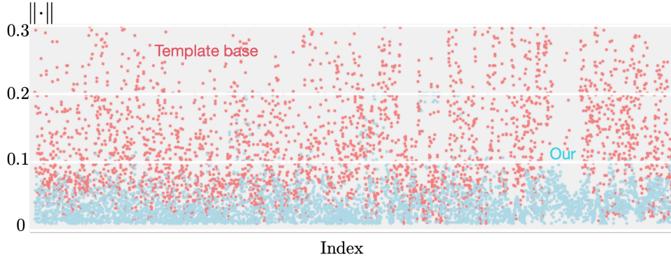
Figure 3.8: By looking at the error in the function of the Euclidean domain of upsampling mesh. We can see that the shared weight cannot handle the diverse mesh. We randomly picked mesh from the CoMA dataset, the reduction from 5024 to 315 vertices (6%) then upsampling by a different strategy. Each point illustrates the error between estimated and original coordinates.
