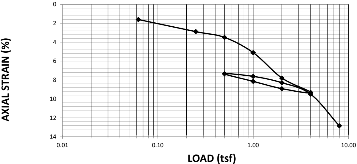
Figure B 1. Site 3- Muskogee 3.6 ft sat Consolidation test results
