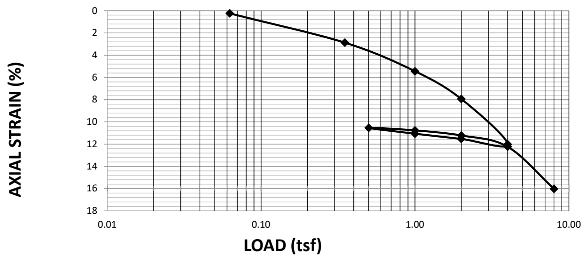
Figure B 3. Site 8- Fairview 6 ft sat Consolidation test results
