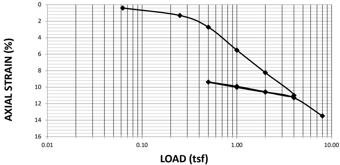
Figure B 2. Site 3- Muskogee 3.5 ft unsat Consolidation test results
