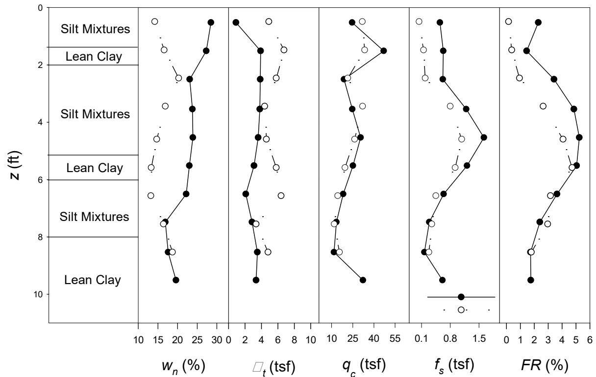
Figure 16. Data representing depth against soil stratigraphy, w_n , \psi , q_c , f_s , and FR during wet and dry periods in Site 9 (Fears Lab). Soil profiles are based on samples obtained from companion test borings
