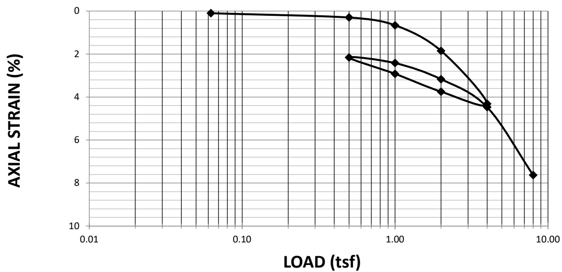
Figure B 4. Site 4- Wagoner 7.7 ft sat Consolidation test results
