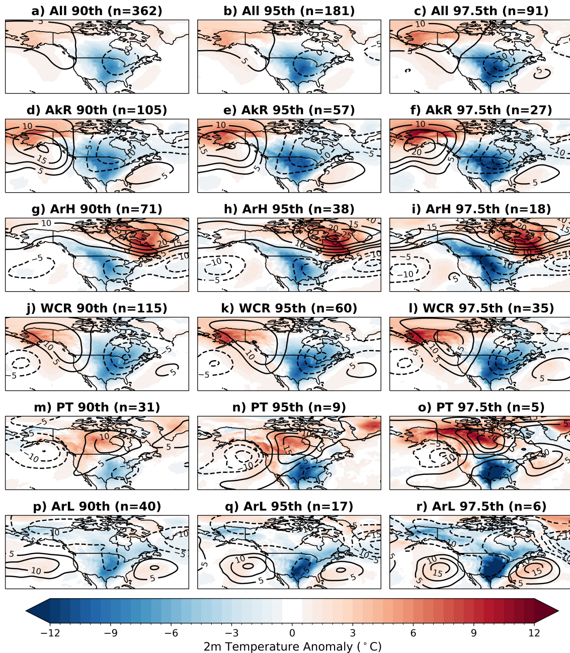
Figure 6.4: Composite maps of ERA5 T2M anomalies (shading, °C) and 500 hPa GPH anomalies (dam, contours), respective to the 1991-2020 climatology, for days exceeding the 90th, 95th, and 97.5th percentile thresholds of all peak load anomalies for a)–c) all days, d)–f) AkR days, g)–i) ArH days, j)–l) WCR days, m)–o) PT days, and p)–r) ArL days. The sample size is given for each composite.
