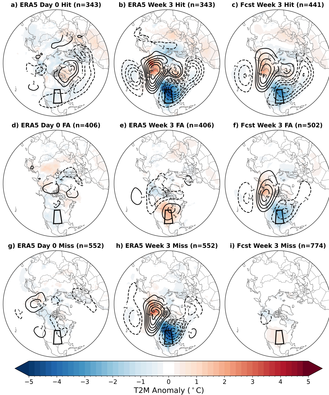
Figure 4.3: Composite maps of T2M anomalies (shading, °C) and 500 hPa GPH anomalies (contours, dam) for confident hit, false alarm and miss forecasts for (a,d,g) ERA5 initialization day, (b,e,h) ERA5 Week 3, and (c,f,i) multi-model mean Week 3, respectively. The black box shows the region used to define central US cold spells and solid contours show positive GPH anomalies while dashed contours show negative GPH anomalies.
