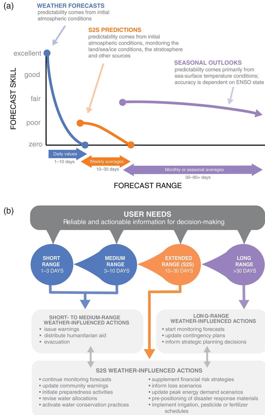
Figure 1.1: (a) A schematic depicting the qualitative estimate of forecast skill based on forecast range from short-range weather forecasts to long-range seasonal predictions, including potential sources of predictability. (b) A schematic diagram highlighting the relationship between the S2S ‘extended-range’ forecast range and other prediction timescales, with examples of actionable information that can enable decision-making across sectors. Adapted from White et al. (2017).
