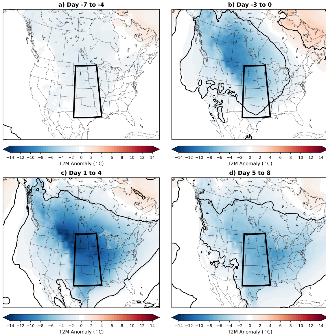
Figure 2.1: Lagged composites of T2M anomalies (°C, shaded) across North America for the 37 identified Great Plains CAOs since 1950, with respect to CAO onset (Day 0) for (a) Days -7 to -4, (b) Days -3 to -0, (c) Days +1 to +4 and (d) Days +5 to +8. Black contours represent significance at the 95th percentile level via a bootstrapping approach of 5000 iterations. The black box represents the region used to define the CAOs. Negative lags indicate days prior to CAO onset day (Day 0), and positive lags indicate days after CAO onset.
