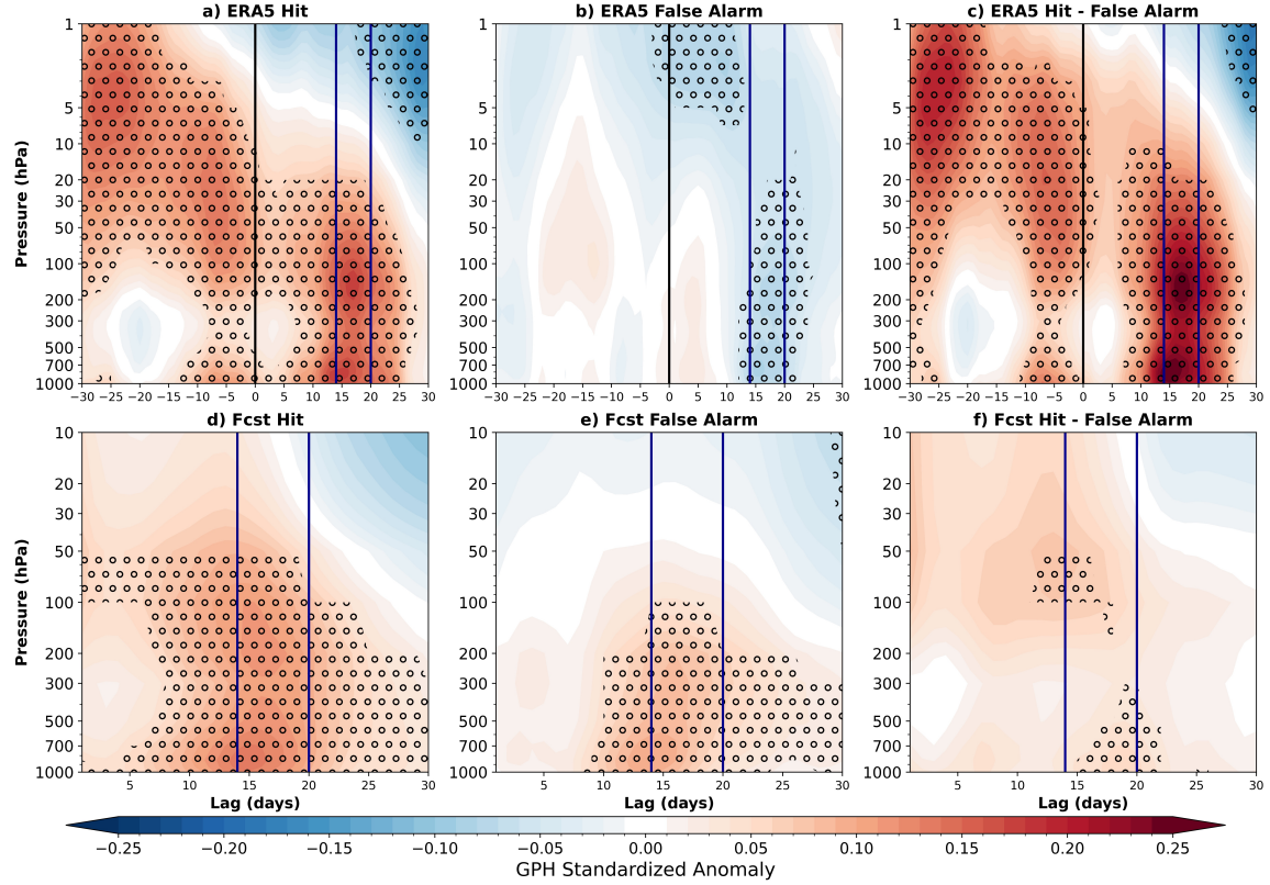
Figure 4.5: Composites of polar cap (60-90°N) averaged GPH anomalies (shading) as a function of lag from initialization and pressure level for Week 3 cold spell confident hit forecasts, confident false alarm forecasts, and the difference between the confident hit and false alarm forecasts in a)–c) ERA5 and d)–f) the S2S models, respectively. Circles represent statistical significance at the 95th percentile via 5000-iteration bootstrapping, the blue lines represent the Week 3 cold, and the black solid line represents initialization date.
