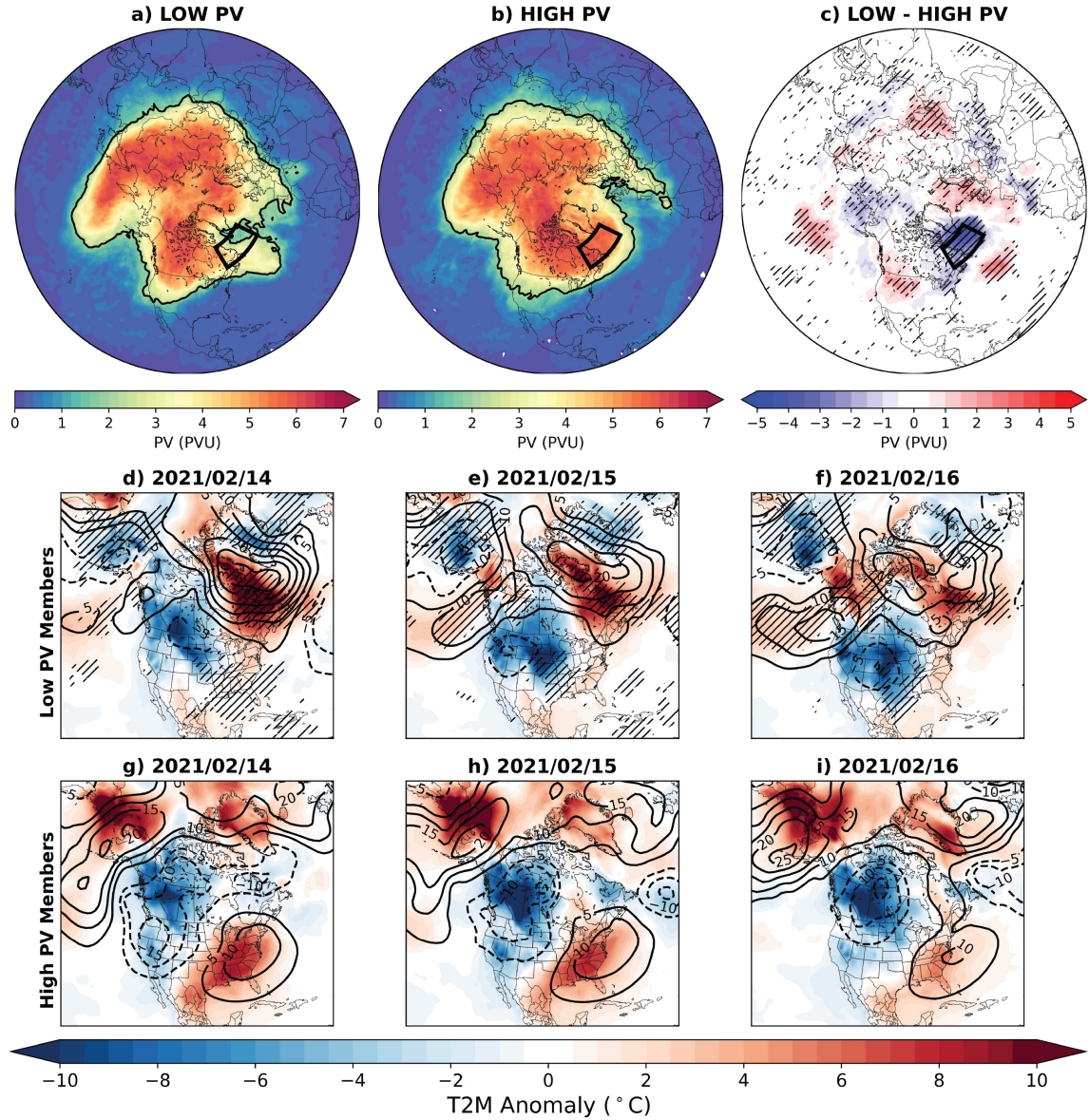
Figure 5.5: As in Fig. 5.4 but for the Labrador Sea wave break between 9-11 February 2021.
