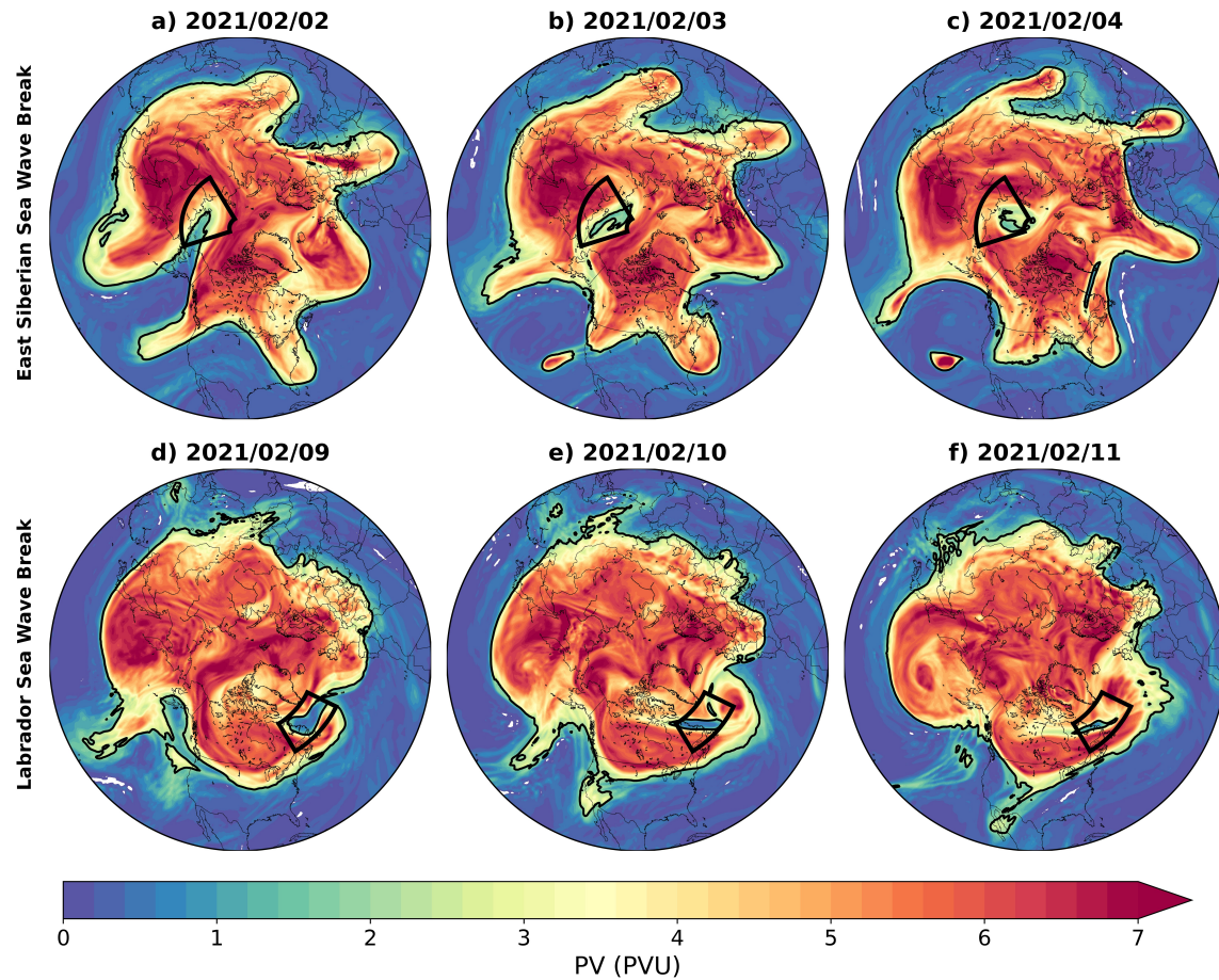
Figure 5.2: ERA5 320 K PV (PVU, shaded) for two wave breaks during the evolution of the February 2021 CAO: a) – c) an East Siberian Sea anticyclonic wave break between 2-4 February 2021 and d) – f) a Labrador Sea cyclonic wave break between 9-11 February 2021. The black contour represents the 2 PVU boundary. Black boxes in a) – c) and d) – f) represent the two wave break regions, respectively.
