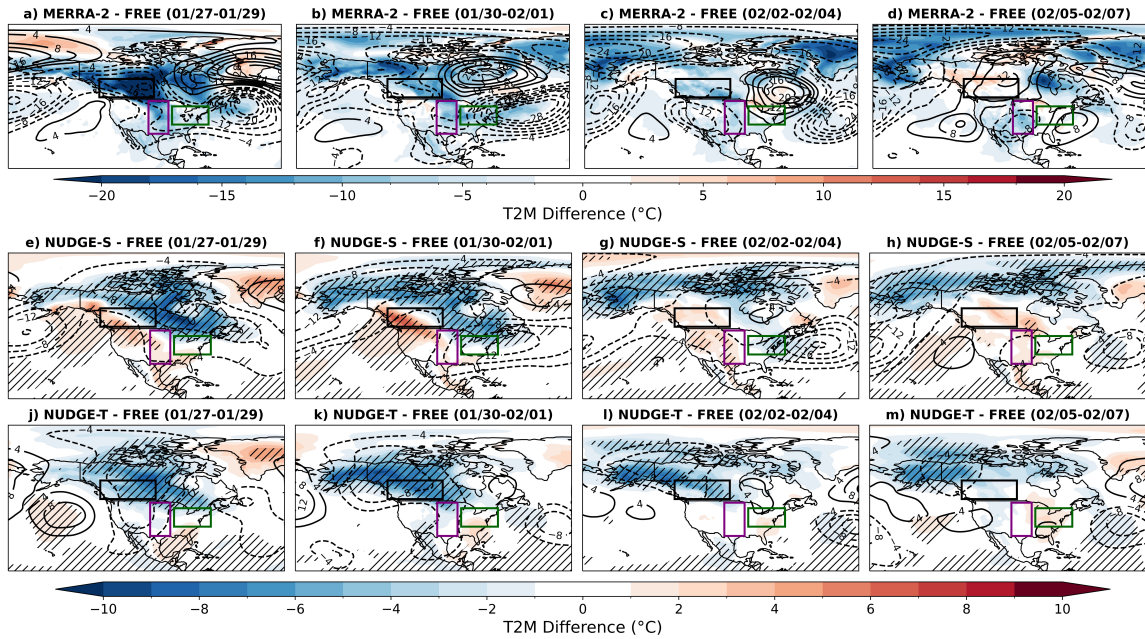
Figure 3.9: The difference in T2M (°C, shading) and 500 hPa GPH (dam, contours) from the ensemble mean FREE run for a)–d) MERRA-2, e)–h) the NUDGE-S ensemble mean, and j)–m) the NUDGE-T ensemble mean, for the 29 December 2003 initialization at 3-day averaged periods from 27 January–29 January 2004 through 5 February–7 February 2004, respectively. Hatching shows statistical significance at the 95th percentile on the difference in the T2M via 5000-iteration bootstrapping with replacement.
