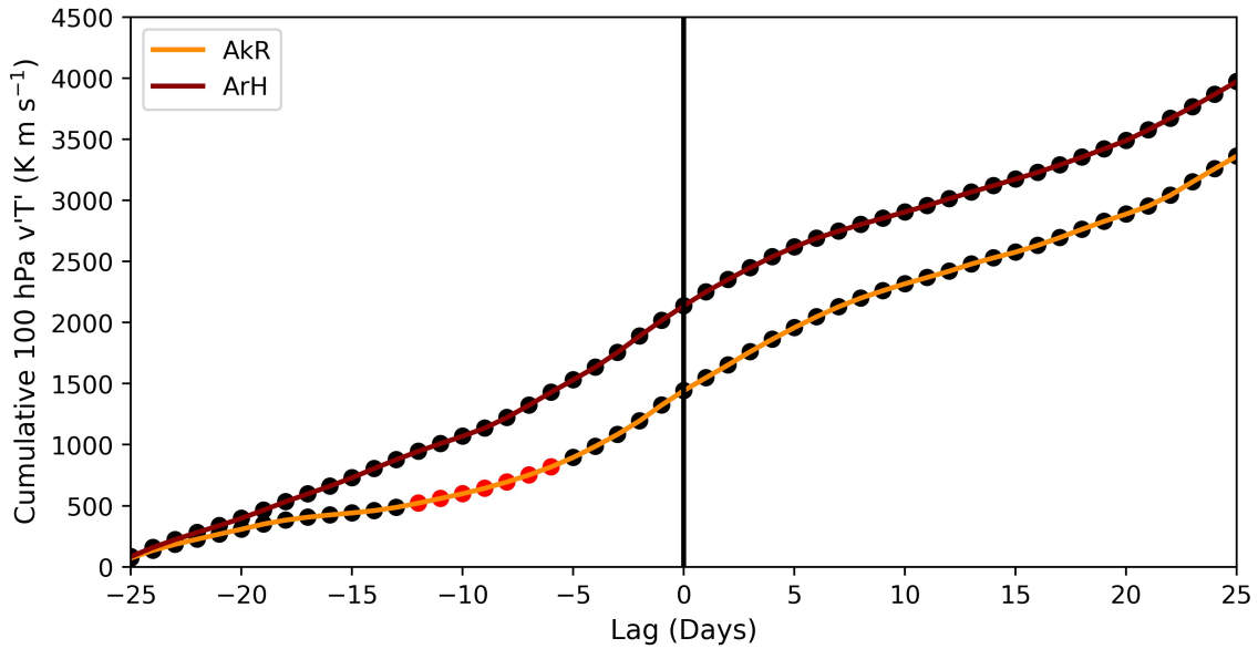
Figure A.5: Lagged composite of the cumulative total 100 hPa v'T' ( \text{K m s}^{-1} ) averaged over the Siberian region ( 55-75^\circ\text{N} and 145-185^\circ\text{E} ) for AkR-CAOs (orange) and ArH-CAOs (dark red) with respect to CAO onset (Day 0). Statistical significance at the 95th percentile is shown via red dots via a 5000-iteration bootstrapping approach.
