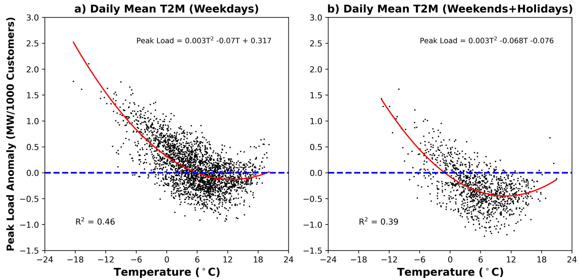
Figure A.14: Scatter plots of peak load anomaly (MW/1000 customers) versus daily mean ERA5 T2M ( ^{\circ}\text{C} ) for (a) non-holiday weekdays and (b) weekend days and non-weekend holidays. We have selected Christmas Day, Thanksgiving Day, and New Year's Day as the holidays to select. The daily average T2M has been averaged over the boxed region in Fig. 2. The red lines represent the second degree polynomial model for the relationship between the two parameters in each plot, with the equation of this polynomial shown on the plot, where T represents the temperature, as well as the coefficient of determination ( R^2 ) value for peak load anomaly respective to the polynomial model. The blue dashed lines represent an average daily peak load between 1999-2022.
