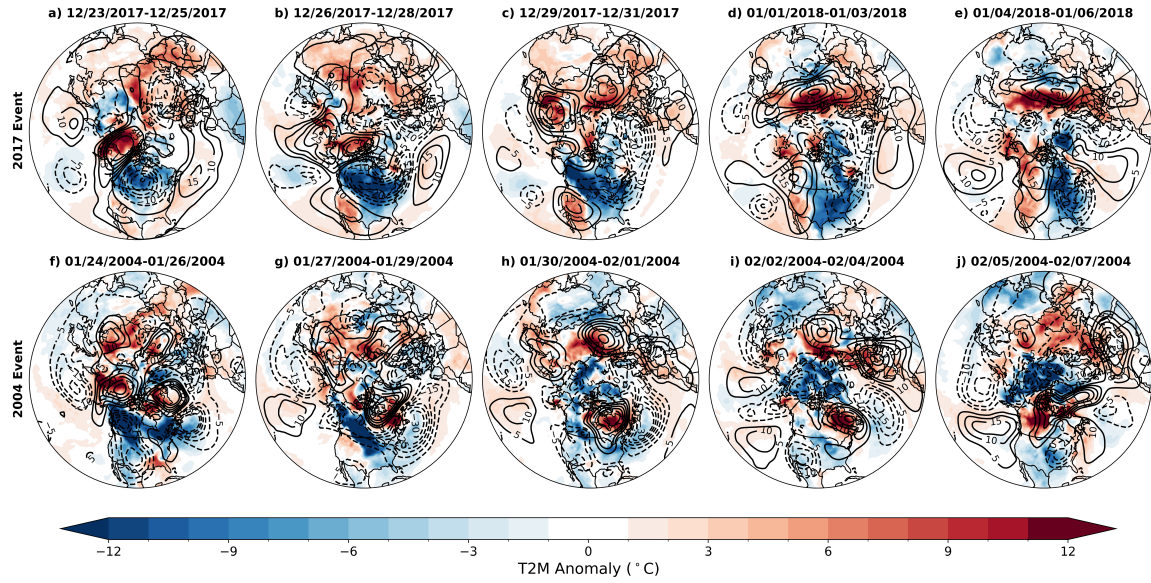
Figure 3.1: Maps of MERRA-2 T2M anomalies ( ^{\circ}\text{C} , shading) and 500 hPa GPH anomalies (dam, contours) averaged for 3-day periods from a) 23 December 2017 – 25 December 2017 through e) 4 January 2018 – 6 January 2018 for the December 2017 central US CAO event, and f) 24 January 2004 – 26 January 2004 through j) 5 February 2004 – 7 February 2004 for the January 2004 central US CAO event. Anomalies are calculated with respect to the 1999-2020 climatology, where the seasonal cycle is removed from each day.
