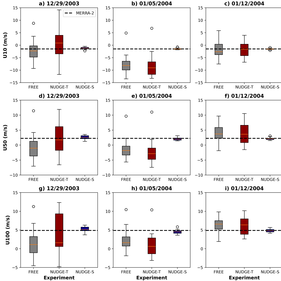
Figure 3.8: Boxplots of the polar cap averaged (60-90°N) zonal wind at a)–c) 10 hPa, d)–f) 50 hPa, and g)–i) 100 hPa all averaged between 12–26 January 2004, for subseasonal initializations of 29 December 2003, 5 January 2004, and 12 January 2004, respectively. Gray boxes denote the FREE experiments, red boxes denote the NUDGE-T experiments, and blue boxes denote the NUDGE-S experiments. The orange lines represent the ensemble median, the lower and upper bounds of the box indicate the 25th and 75th percentiles, the whiskers extend from the box to the farthest data point lying within 1.5 times the interquartile range from the box, and the circles are those points that lie outside of the whiskers.
