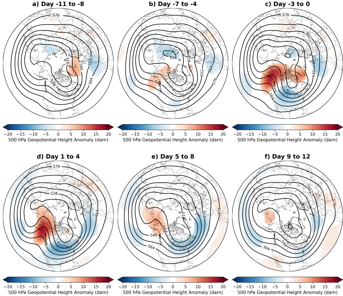
Figure 2.2: Lagged composites of the full-field GPH (dam, black contours) and only the significant ( p < 0.05 ) linearly-detrended 500 hPa GPH anomalies (dam, shaded) across the Northern Hemisphere for the 37 Great Plains CAOs, with respect to CAO onset (Day 0) at 4-day intervals from (a) Days -11 to -8 through (f) Days +9 to +12. Statistical significance is calculated via a bootstrapping approach of 5000 iterations. Negative lags indicate days prior to CAO onset day (Day 0), and positive lags indicate days after CAO onset.
