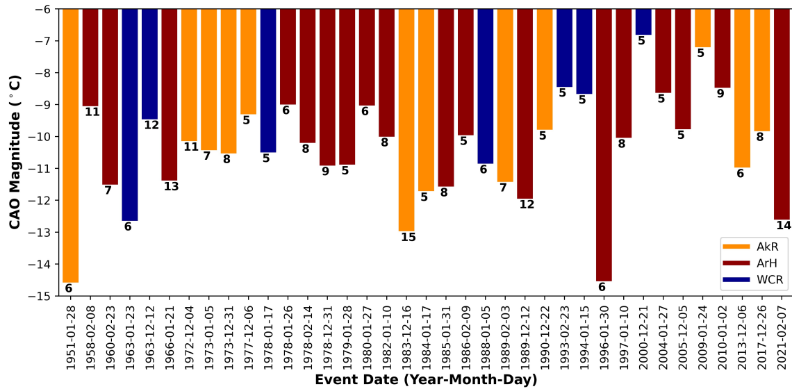
Figure 2.6: Magnitude (°C) of each of the 37 defined CAOs using the non-detrended T2M anomalies, categorized by weather regime: AkR (orange), ArH (red) and WCR (blue). Bold numbers below the bars represent the length (days) of each of the CAOs.
