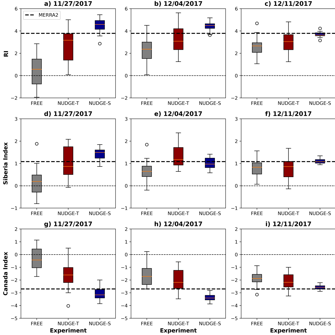
Figure 3.3: Boxplots of a)–c) the RI, d)–f) the Siberian component of the RI, and g)–i) the Canadian component of the RI all averaged between 14–25 December 2017, for sub-seasonal initializations of 27 November 2017, 4 December 2017, and 11 December 2017, respectively. Gray boxes denote the FREE experiments, red boxes denote the NUDGE-T experiments, and blue boxes denote the NUDGE-S experiments. The orange lines represent the ensemble median, the lower and upper bounds of the box indicate the 25th and 75th percentiles, the whiskers extend from the box to the farthest data point lying within 1.5 times the interquartile range from the box, and the circles are those points that lie outside of the whiskers.
