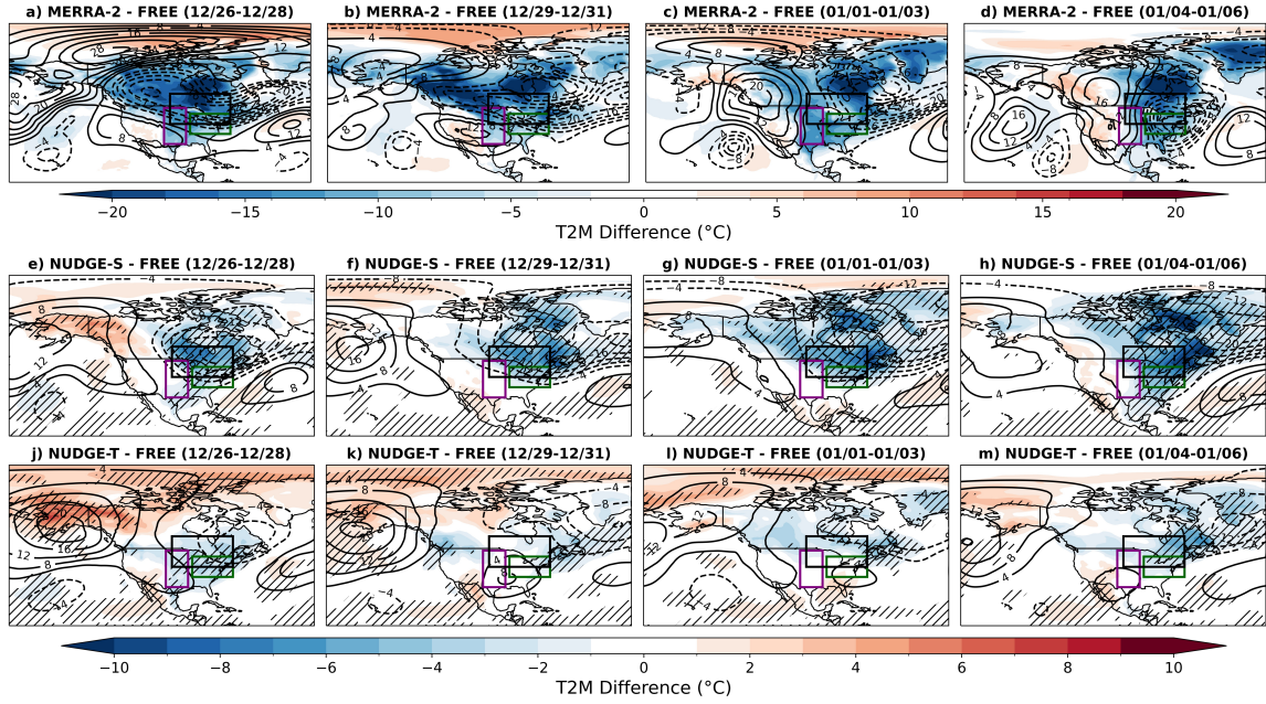
Figure 3.4: The difference in T2M ( ^{\circ}\text{C} , shading) and 500 hPa GPH (dam, contours) from the ensemble mean FREE run for a)–d) MERRA-2, e)–h) the NUDGE-S ensemble mean, and j)–m) the NUDGE-T ensemble mean, for the 27 November 2017 initialization at 3-day averaged periods from 26–28 December 2017 through 4–6 January 2018, respectively. Hatching shows statistical significance on the T2M difference field at the 95th percentile via 5000-iteration bootstrapping with replacement. The black boxes represent the area that usually has the coldest T2M response to reflection events in Messori et al. (2022) ( 40\text{--}55^{\circ}\text{N} , 260\text{--}290^{\circ}\text{E} ), the purple box represents the Great Plains ( 30\text{--}48^{\circ}\text{N} , 257\text{--}268^{\circ}\text{E} ), and the green box represents the northeast US ( 35\text{--}45^{\circ}\text{N} , 270\text{--}290^{\circ}\text{E} ).
