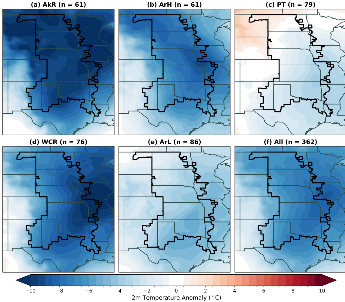
Figure A.15: Composite maps of ERA5 T2M anomalies (shading, °C), respective to the 1991-2020 climatology, for days exceeding the regime-specific 90th percentile of peak load anomalies in each weather regime of a) AkR, b) ArH, c), PT, d) WCR, e) ArL, and f) all days. The black contour represents the SPP region and the sample size is given for each composite.
