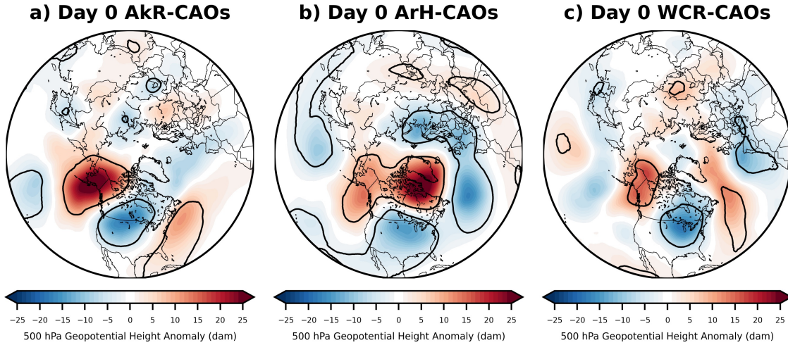
Figure 2.5: Onset day composites of linearly-detrended 500 hPa GPH anomalies (dam, shaded), with respect to the 1981-2010 climatology, are shown for (a) AkR-, (b) ArH- and (c) WCR-CAOs. Black contours represent statistical significance ( p < 0.05 ) via 5000-iteration bootstrapping without replacement.
