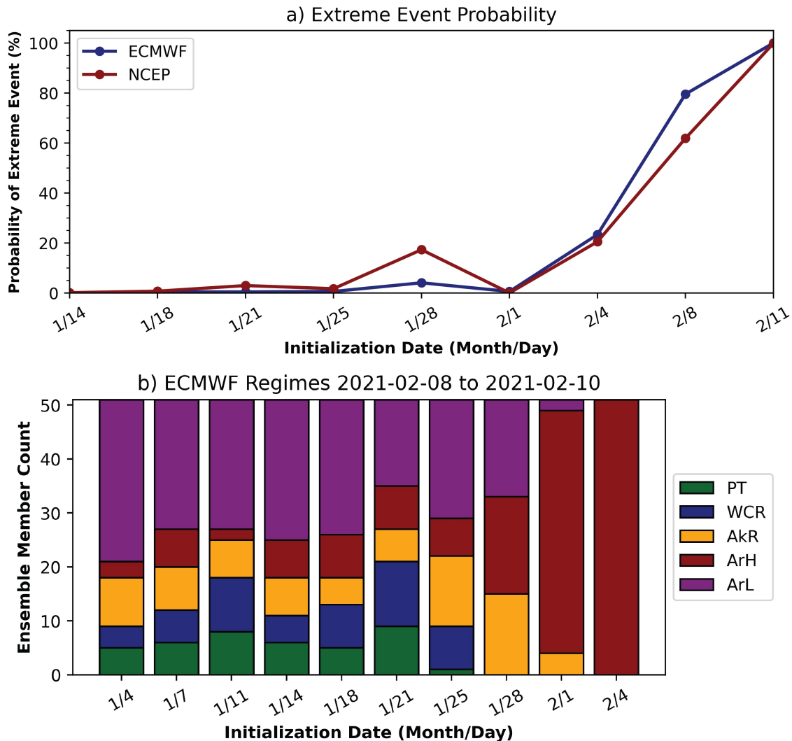
Figure 5.3: a) Probability of an extreme Great Plains T2M anomaly event between 12-18 February 2021 at the 10th percentile as a function of initialization date for ECMWF (blue line) and NCEP (red line). b) A bar plot of the ensemble distribution of 5 North American weather regimes for the 8-10 February 2021 as a function of initialization date within the ECMWF model the Pacific Trough (PT), West Coast Ridge (WCR), Alaskan Ridge (AkR), Arctic High (ArH), and the Arctic Low (ArL).
