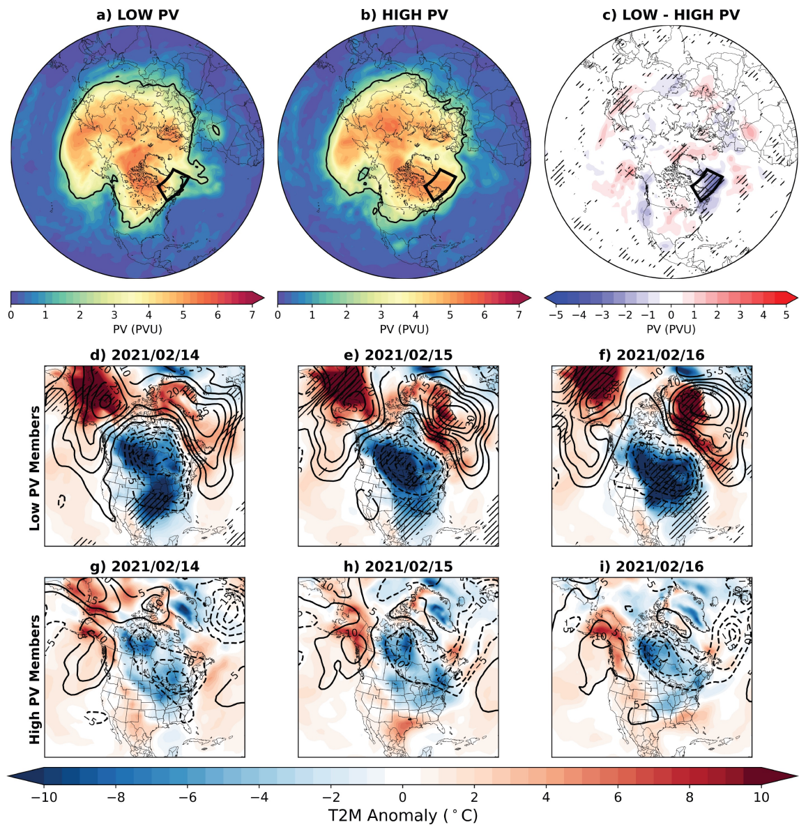
Figure A.12: As in Fig. 5.5 but for the 3 highest and lowest Labrador Sea 320 K PV ensemble members in the NCEP model.
