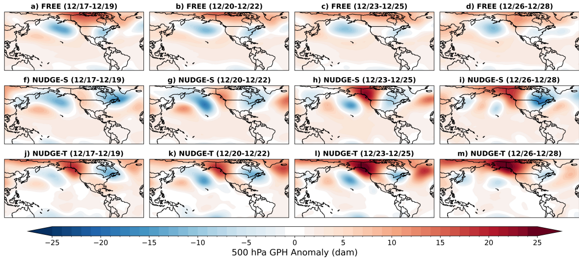
Figure A.8: The evolution of the ensemble mean 500 hPa GPH anomalies (shading, dam) in the 27 November 2017 initialization for 3-day averaging periods of 17–19 December 2017, 20–22 December 2017, 23–25 December 2017, and 26–28 December 2017 for a)–d) the FREE experiment, f)–i) the NUDGE-S experiments, and j)–m) the NUDGE-T experiments, respectively.
