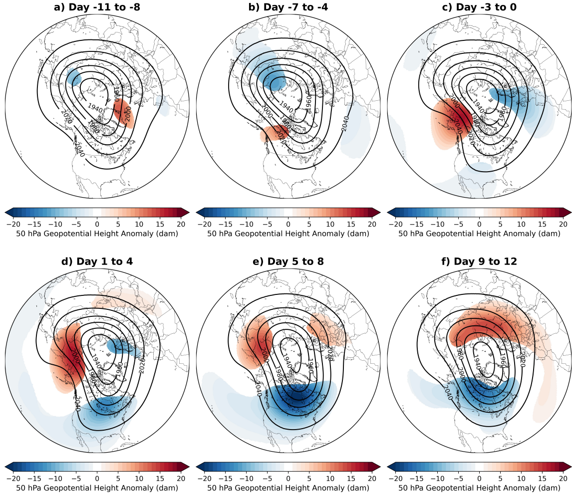
Figure 2.3: As in Fig. 2.2 but for 50 hPa full-field GPH (dam; contours) and only significant ( p < 0.05 ) linearly-detrended GPH anomalies (dam; shading) .
