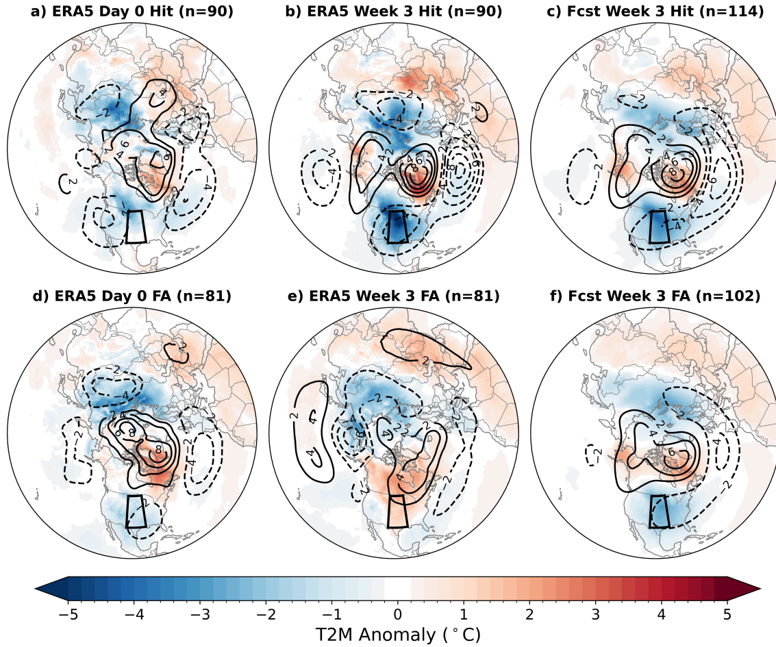
Figure 4.8: As in Fig. 4.3 but for forecasts initialized in weak polar vortex states.
