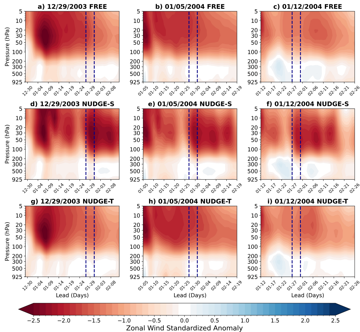
Figure A.9: The evolution of the zonal wind standardized anomaly (shading) averaged over the polar cap (60–90°N for the three subseasonal forecast initializations of 29 December 2003, 5 January 2004, and 12 January 2004 for a)–c) the FREE experiments, d)–f) the NUDGE-S experiments, and g)–i) the NUDGE-T experiments. The dashed lines show the start and end dates of the central US CAO.
