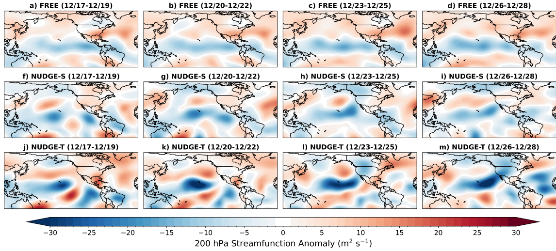
Figure A.7: The evolution of the ensemble mean 200 hPa streamfunction anomalies (shading, \text{m}^2 \text{s}^{-1} ) in the 27 November 2017 initialization for 3-day averaging periods of 17–19 December 2017, 20–22 December 2017, 23–25 December 2017, and 26–28 December 2017 for a)–d) the FREE experiment, f)–i) the NUDGE-S experiments, and j)–m) the NUDGE-T experiments, respectively.
