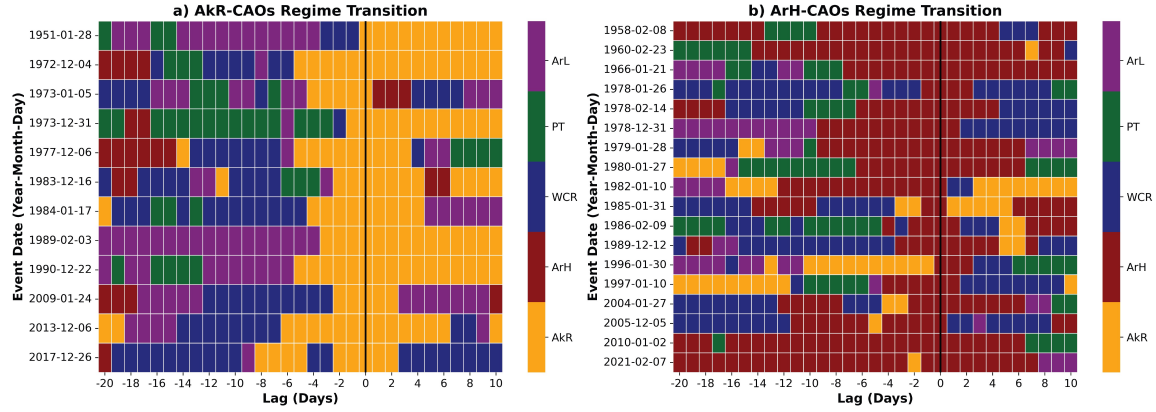
Figure 2.12: North American weather regime transitions for a) AkR-CAOs and b) ArH-CAOs in the US Great Plains, between Days -20 and +10.
