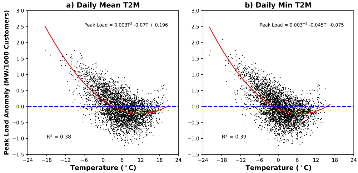
Figure 6.2: Scatter plots of peak load anomaly (MW/1000 customers) versus ERA5 (a) daily average T2M (°C) and (b) daily minimum T2M (°C), where both temperature variables have been averaged over the boxed region in Fig. 6.1. The red lines represent the second degree polynomial model for the relationship between the two parameters in each plot, with the equation of this polynomial shown on the plot, where T represents the temperature, as well as the the coefficient of determination ( R^2 ) value for variance explained in peak load anomaly respective to the polynomial model. The blue dashed lines represent an average daily peak load between 1999-2022.
