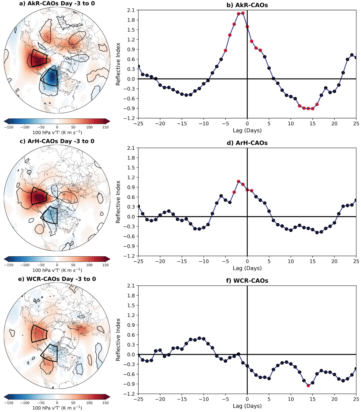
Figure 2.7: Composites of 100 hPa v'T' (K m s -1 , shaded) for Days -3 to 0 in (a), (c), and (e), and RI in (b), (d), and (f) for AkR-, ArH-, and WCR-CAOs, respectively. The RI is defined as in Matthias and Kretschmer (2020) but between 55-75°N, and 145-185°E and 220-260°E for Siberia and Canada, respectively (thick black lines on (a), (c), and (e)). Black contours on (a), (c), and (e) and red dots on (b), (d), and (f) show statistical significance ( p < 0.05 ) via 5000-iteration bootstrapping. The two southerly dashed lines are latitudes 60°N and 70°N, as used in Fig. 2.8. Negative and positive lags indicate days before and after CAO onset day (Day 0), respectively.
