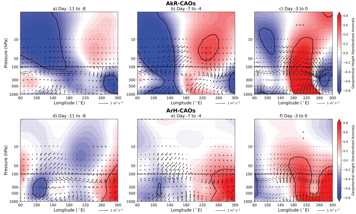
Figure 2.8: Lag composites of the linearly-detrended standardized anomalies of GPH (shaded) and full-field WAF (vectors) at 4-day intervals from Days -11 to -8 through Days -3 to 0 for: (a) to (c) AkR-CAOs and (d) to (f) ArH-CAOs, averaged between 60-70°N. Yellow dots represent statistical significance ( p < 0.05 ) of the the vertical component of the WAF via a 5000-iteration bootstrapping without replacement. Black contours represent statistical significance ( p < 0.05 ) of the GPH anomalies using the same method. Negative lags indicate days prior to CAO onset day (Day 0), and positive lags indicate days after CAO onset. Scaling of the WAF vectors was achieved by dividing the vertical WAF component by a scale factor of 0.1 above 200 hPa and by a scale factor of 0.3 below and including 200 hPa, and dividing the zonal WAF component by 10 above 200 hPa and by 50 below and including 200 hPa.
