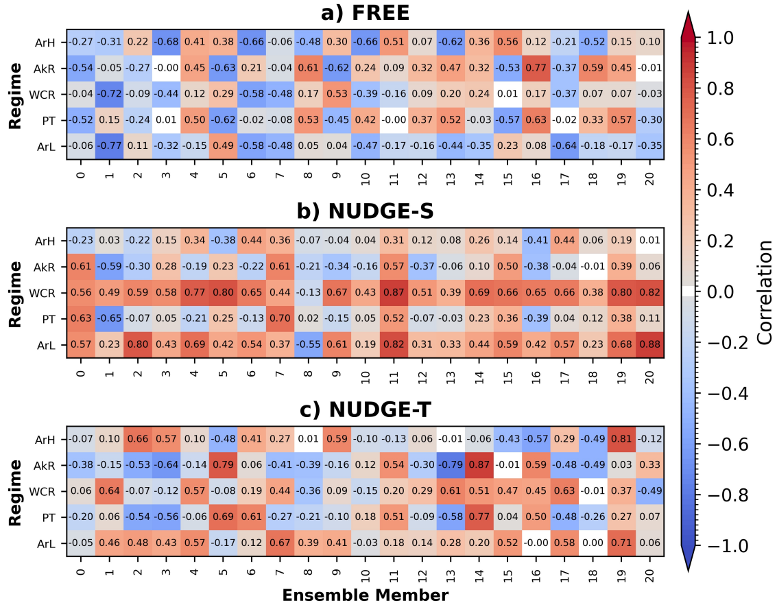
Figure 3.7: The correlation between the MERRA-2 WRIs and the CESM2 CAM6 forecast WRI initialized on 27 November 2017 for the lead time extending from 14 days prior to the CAO to 6 January 2018 (i.e., end of averaging period for NE cold), as a function of ensemble member.
