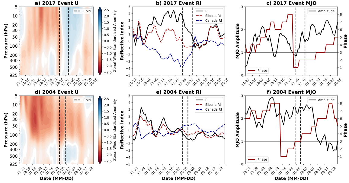
Figure 3.2: The evolution of several key S2S indices for the December 2017 central US CAO event: a) the polar cap (60–90°N) averaged zonal wind standardized anomalies throughout the atmosphere (shading) from MERRA-2, b) the RI (black line) and its Siberian (red dashed line) and Canadian components (blue dashed line) from MERRA-2, and c) the MJO amplitude (black solid line) and phase (red solid line) from the BoM. Panels d)–f) show the same as a)–c), respectively, but for the January 2004 central US CAO. Black dashed lines indicate the start and end of the CAO periods. Anomalies are calculated with respect to the 1999–2020 climatology, where the seasonal cycle is removed from each day.
