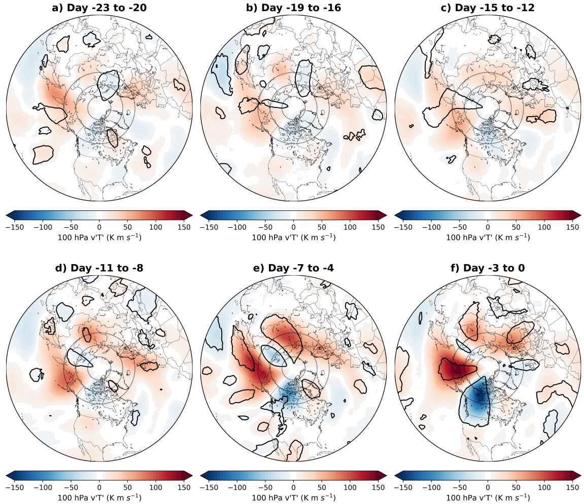
Figure A.3: Lagged composites of the 100 hPa v'T' (K m s -1 , shaded) across the Northern Hemisphere for AkR-CAOs, with respect to CAO onset (Day 0) at 4-day intervals from a) Days -23 to -20 through f) Days -3 to 0. Black contours represent significance at the 95th percentile via a bootstrapping approach of 5000 iterations.
