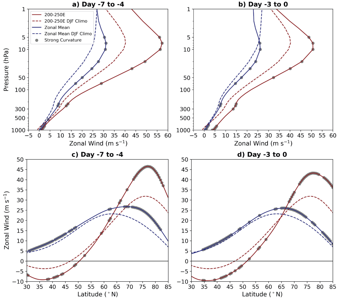
Figure 2.10: Lagged composites of the (a) and (b) vertical profile averaged between 70–80°N, and meridional profile at 30 hPa, (c) and (d), of zonal wind ( \text{m s}^{-1} ) for AkR-CAOs averaged between 200–250°E (red solid line) and in the zonal mean (blue solid line), at 4-day intervals for Days -7 to -4 and Days -3 to 0, respectively, where Day 0 is CAO onset. Red and blue dashed lines represent DJF 1981–2010 climatology of the zonal wind between 200–250°E and in the zonal mean, respectively. Grey dots indicate strong curvature (see Section 2d). Negative lags indicate days prior to CAO onset day (Day 0), and positive lags indicate days after CAO onset.
