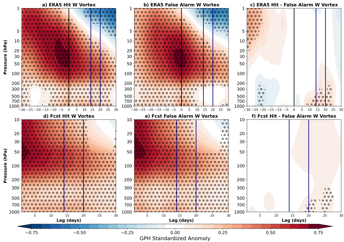
Figure 4.12: As in Fig. 4.5 but for forecasts initialized in weak polar vortex states.
