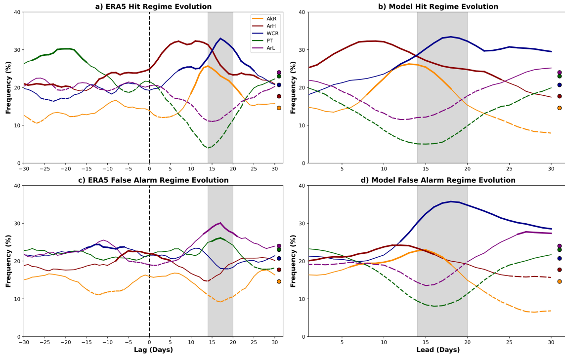
Figure 4.4: Lagged North American winter weather regime frequencies with respect to forecast initialization time (lag 0) for a) the confident hit forecast initializations and c) the confident false alarm forecast initializations in ERA5. Panels b) and d) show the same as panels a) and c) but instead for the model forecasts as a function of lead time. Regime frequencies are calculated relative to the total number of samples in each group and are then smoothed with a 5-day centered filter. Bold and dashed lines represent statistically significant enhanced or suppressed frequencies relative to climatology at the 95 th percentile via 5000-iteration bootstrapping from ERA5 data. Week 3 is shown in gray shading and the colored dots indicate the climatological frequency of the five winter weather regimes.
