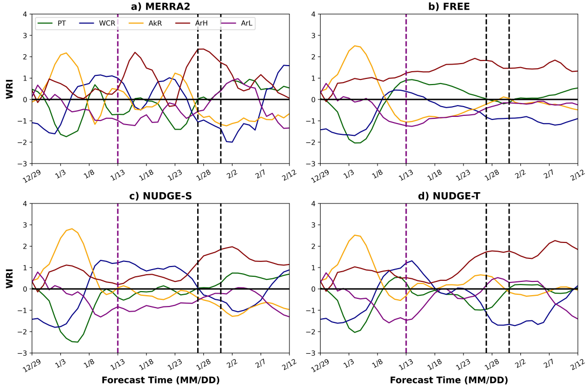
Figure 3.11: The evolution of the ensemble mean weather regime index for the five North American winter weather regimes for the 29 December 2003 CESM2 CAM6 initialization in a) the MERRA-2 evolution, b) the FREE experiment, c) the NUDGE-S experiment, and d) the NUDGE-T experiment. The green line represents the Pacific Trough (PT), the blue line represents the West Coast Ridge (WCR), the orange line represents the Alaskan Ridge (AkR), the red line represents the Arctic High (ArH), and the purple line represents the Arctic Low (ArL). The black dashed lines show the start and end dates of the 2004 CAO during the initialization. The purple dashed line represents the start of the period used for correlation analysis in Fig. 3.12.
