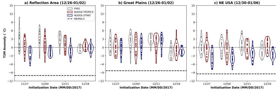
Figure 3.5: Violin plots of the ensemble forecast of area-averaged T2M anomalies ( ^{\circ}\text{C} ) for weekly CESM2 CAM6 initializations from 27 November 2017 to 18 December 2017 for a) the area most prone to cold events due to stratospheric wave reflection ( 40\text{--}55^{\circ}\text{N} , 260\text{--}290^{\circ}\text{E} ) from Messori et al. (2022) averaged between 26 December 2017 to 2 January 2018, b) the Great Plains ( 30\text{--}48^{\circ}\text{N} , 257\text{--}268^{\circ}\text{E} ) averaged between 26 December 2017 to 2 January 2018, and c) the northeast US ( 35\text{--}45^{\circ}\text{N} , 270\text{--}290^{\circ}\text{E} ) averaged between 30 December 2017 to 6 January 2018. The blue, red, and gray distributions represent the NUDGE-S, NUDGE-T, and FREE experiments, respectively. The dashed black lines represents the MERRA-2 values.
