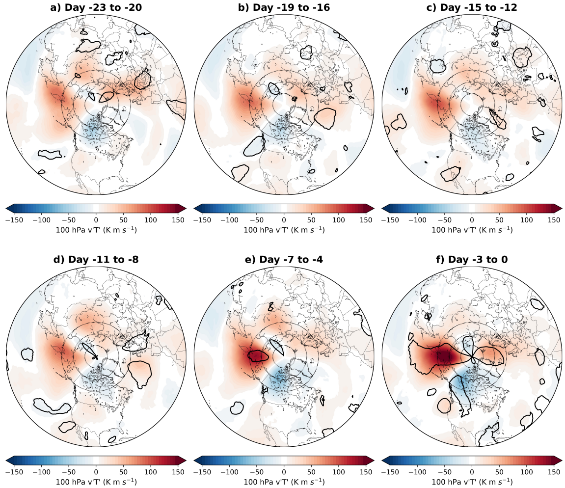
Figure A.2: Lagged composites of the 100 hPa v'T' (K m s -1 , shaded) across the Northern Hemisphere for ArH-CAOs, with respect to CAO onset (Day 0) at 4-day intervals from a) Days -23 to -20 through f) Days -3 to 0. Black contours represent significance at the 95th percentile via a bootstrapping approach of 5000 iterations.
