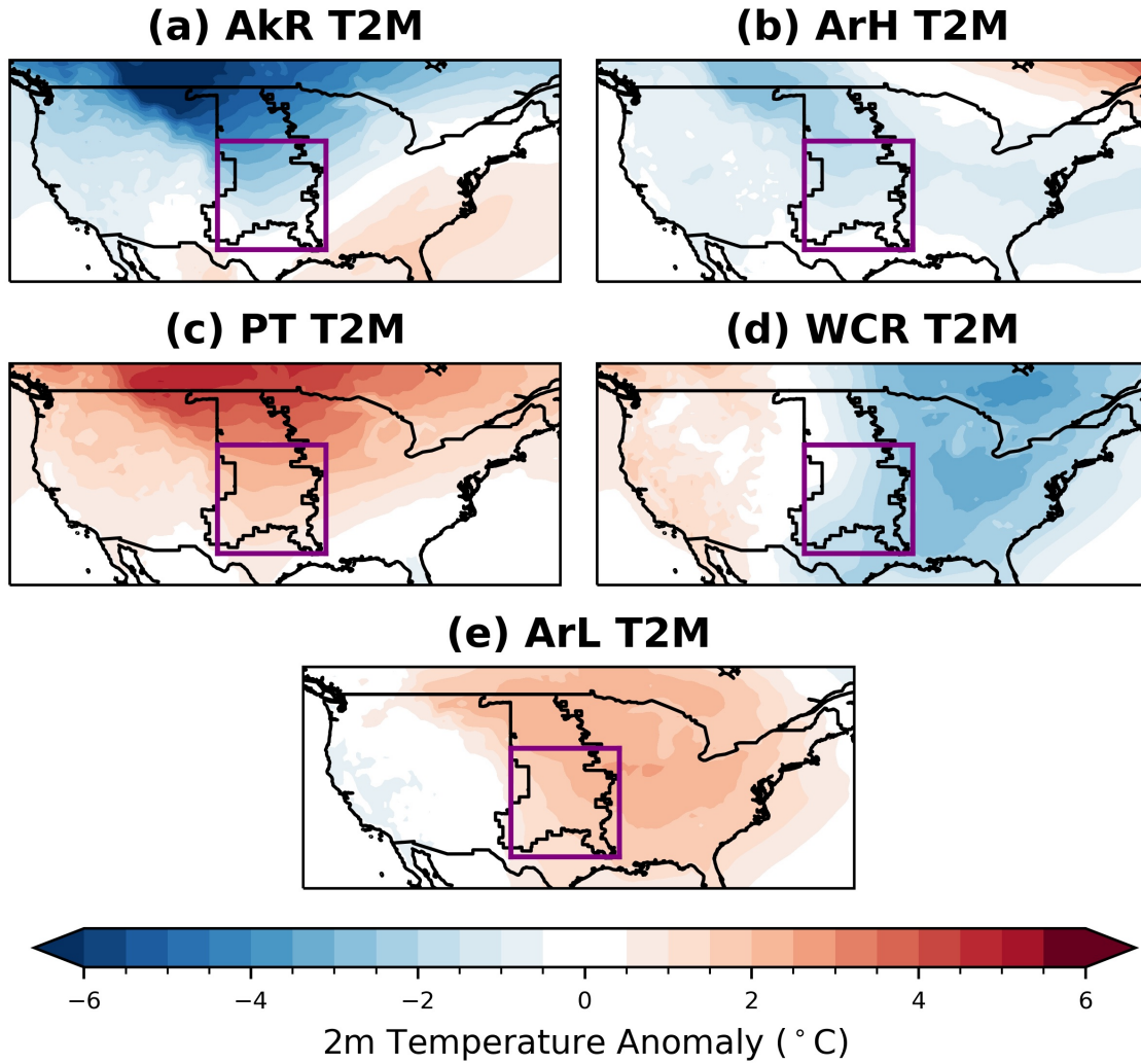
Figure 6.1: As in Fig. A.13 but for ERA5 linearly detrended T2M anomalies (shading, °C). The black lines show the region of the entire Southwest Power Pool (SPP) while the purple box (31-43°N, 256-268°E) represents the region of study for electricity load data in the SPP and the area in which T2M is averaged for Fig. 6.2. A sub-domain of the entire SPP region is used for analysis as it represents the 13 divisions within the SPP that could be consistently matched between load data sources (see methods). Anomalies are with respect to the 1979-2020 climatology also used to calculate the regimes.
