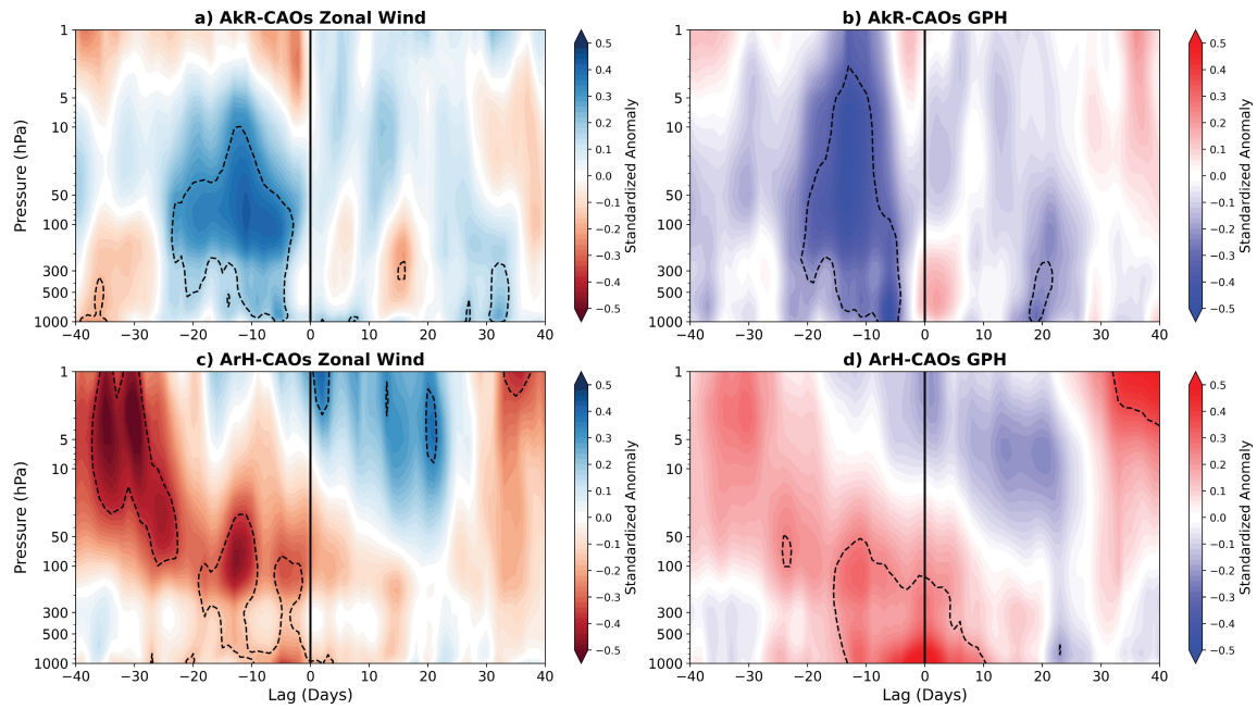
Figure 2.11: Composite pressure-time polar cap (60-90°N) averaged cross-sections of standardized and non-detrended zonal wind anomalies for (a) AkR- and (c) ArH-CAOs, and of linearly-detrended GPH standardized anomalies for (b) AkR- and (d) ArH-CAOs between Days -40 and +40. Dashed lines represent statistical significance at the 95th percentile via bootstrapping of 5000 iterations. Negative lags indicate days prior to CAO onset day (Day 0), and positive lags indicate days after CAO onset.
