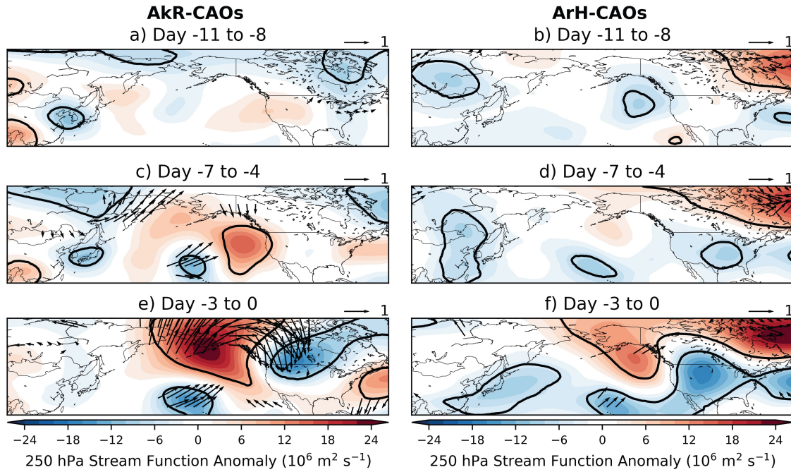
Figure 2.9: Lag composites of the 250 hPa streamfunction anomalies ( 10^6 \text{ m}^2 \text{ s}^{-1} , shaded) and statistically significant ( p < 0.05 ) standardized WAF anomalies (vectors) across the Pacific basin for 4-day intervals of Days -11 to -8 through Days -3 to 0 for (a), (c) and (e) AkR-CAOs, and (b), (d) and (f) ArH-CAOs. Black contours represent statistical significance ( p < 0.05 ) of the streamfunction anomalies via a bootstrapping approach of 5000 iterations without replacement. Statistical significance ( p < 0.05 ) of WAF is computed using the magnitude of the WAF anomalies and 5000-iteration one-tailed bootstrapping without replacement. Negative lags indicate days prior to CAO onset day (Day 0), and positive lags indicate days after CAO onset.
