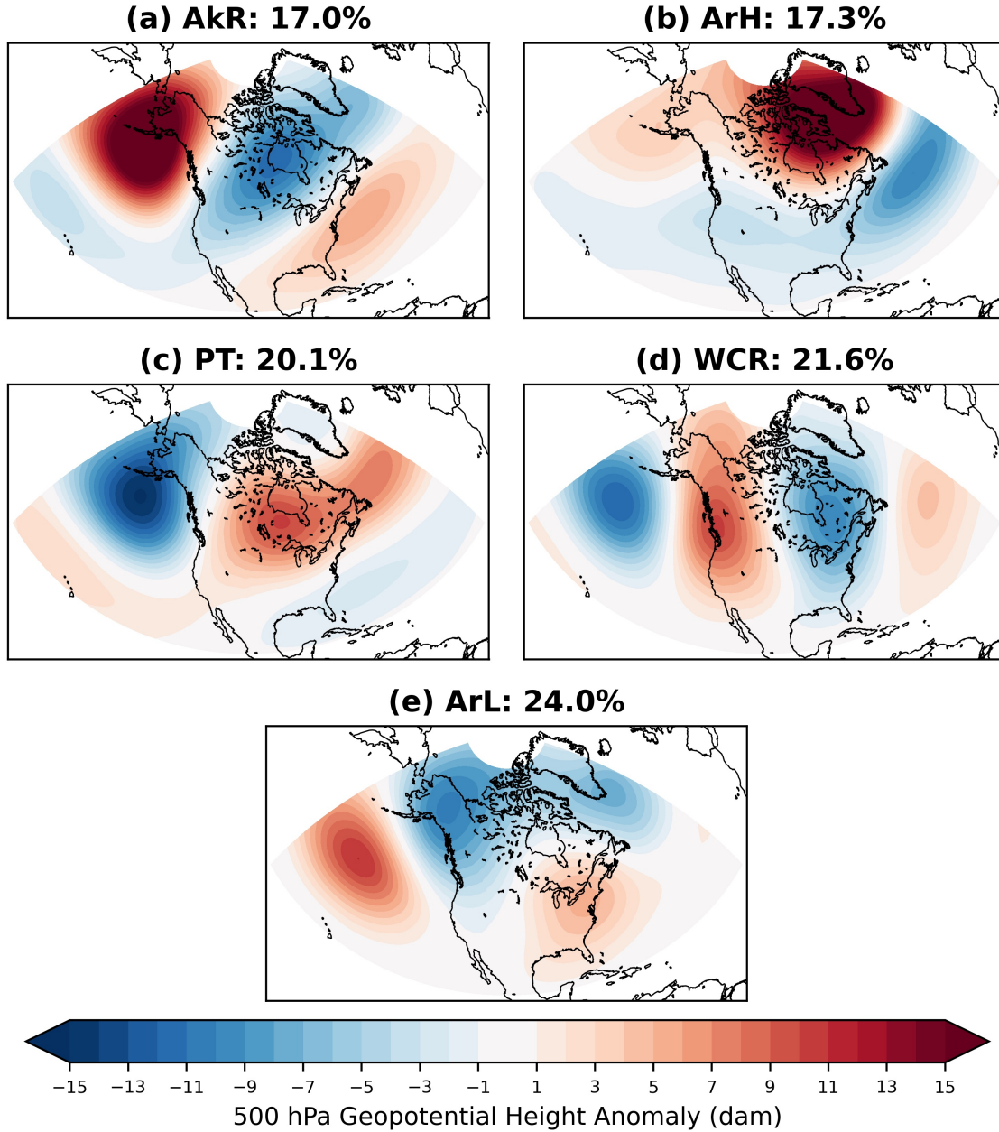
Figure 2.4: Composite 500 hPa linearly-detrended GPH anomalies (dam, shaded), for the five North American weather regimes for NDJFM between 1950 and 2021: (a) Alaskan Ridge (AkR), (b) Arctic High (ArH), (c) Pacific Trough (PT), (d) West Coast Ridge (WCR), and (e) Arctic Low (ArL). Percentages show the frequency of occurrence of a given regime throughout 1950-2021.
