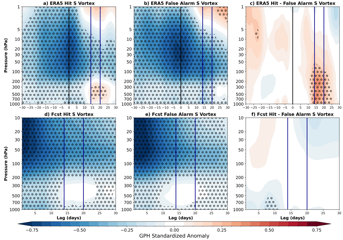
Figure 4.13: As in Fig. 4.5 but for forecasts initialized in strong polar vortex states.
