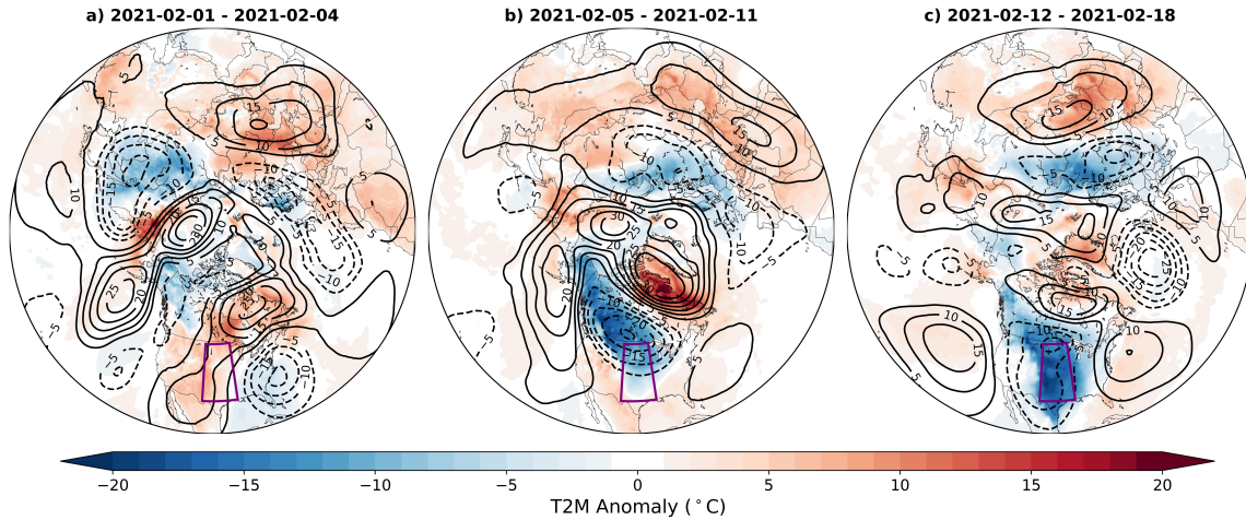
Figure 5.1: ERA5 500 hPa GPH anomalies (dam, contours) and T2M anomalies ( ^{\circ}\text{C} , shaded) averaged between a) 1-4, b) 5-11, and c) 12-18 February 2021. Solid and dashed contours represent positive and negative GPH anomalies, respectively. The purple boxes represent the region defining the Great Plains ( 30\text{--}48^{\circ}\text{N} and 256.5\text{--}268.5^{\circ}\text{E} ).
