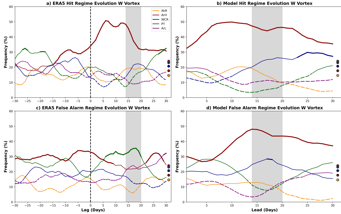
Figure 4.10: As in Fig. 4.4 but for forecasts initialized in weak polar vortex states.
