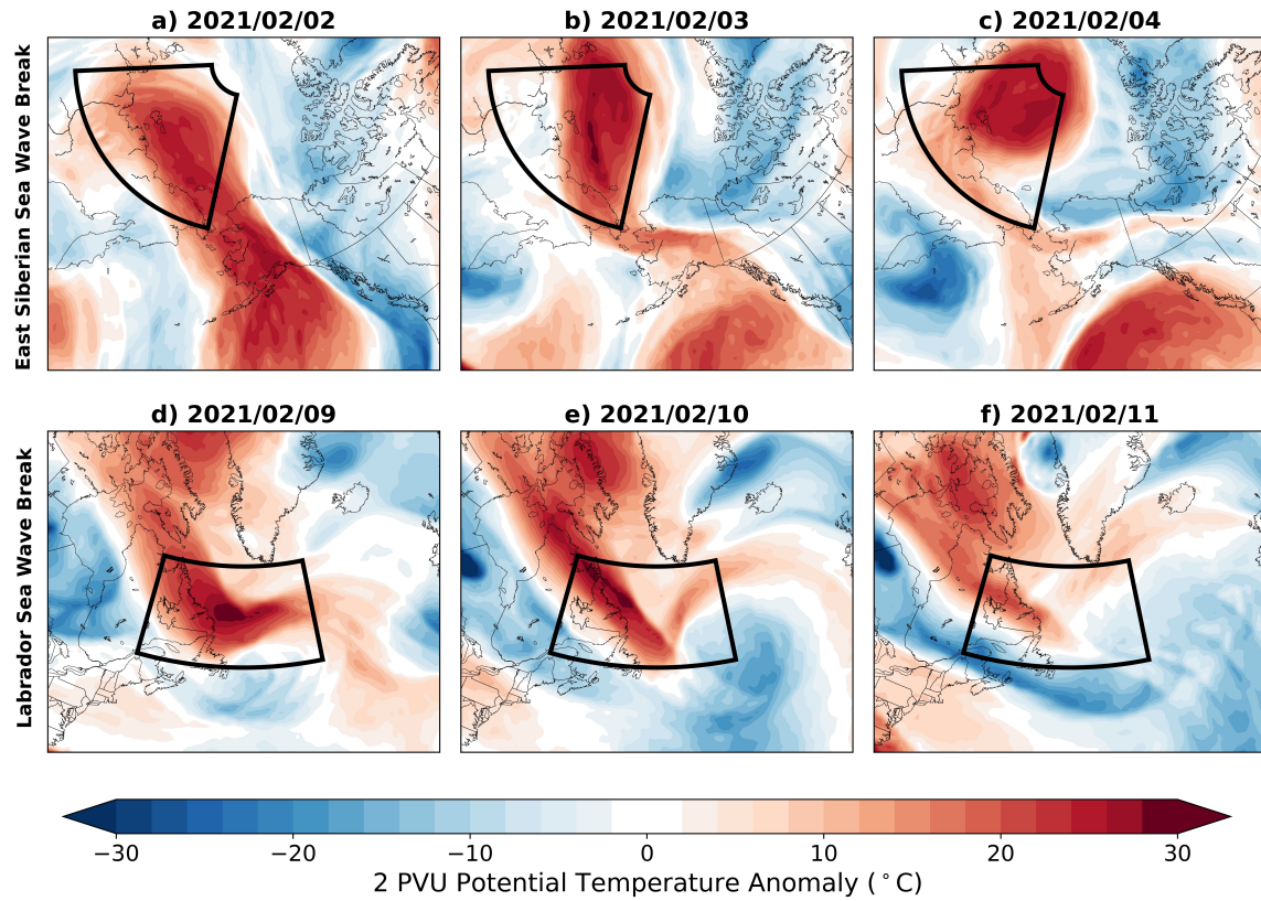
Figure A.10: ERA5 potential temperature anomalies on the 2 PVU surface (°C, shading) for two wave breaks during the evolution of the February 2021 CAO: a) – c) an East Siberian Sea anticyclonic wave break between 2-4 February 2021 and d) – f) a Labrador Sea cyclonic wave break between 9-11 February 2021. Black boxes in a) – c) and d) – f) represent the East Siberian Sea and Labrador Sea wave break regions, respectively.
