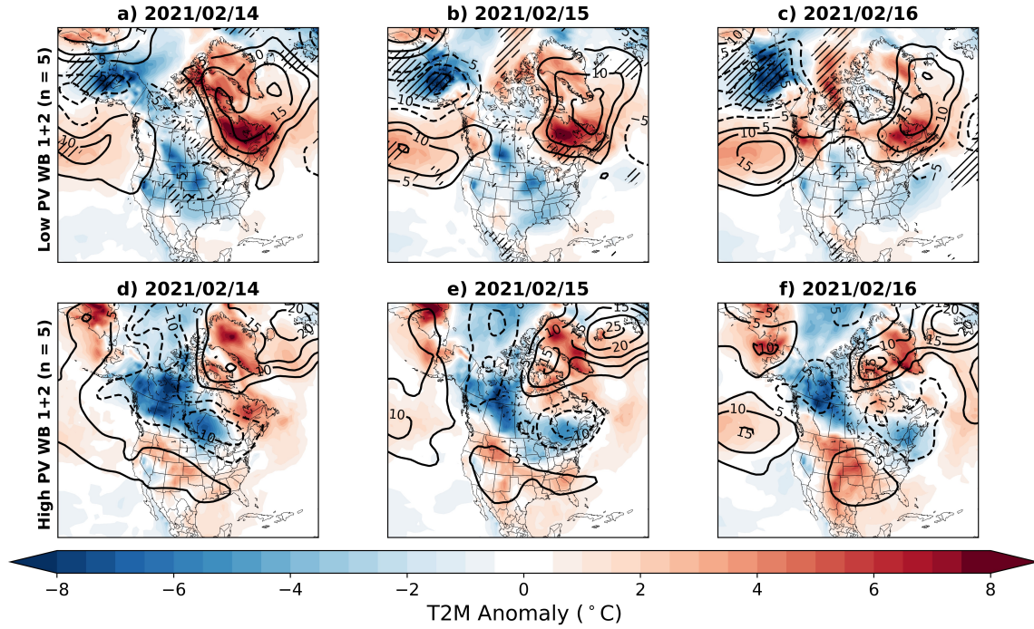
Figure 5.6: 28 January 2021 initialization ECMWF T2M anomaly ( ^{\circ}\text{C} , shading) and 500 hPa geopotential height anomaly (dam, contours) composites between 14-16 February 2021 for ensemble members that a) – c) simulate both the East Siberian Sea and Labrador Sea wave breaks best ( \text{PV} < 25\text{th percentile} ) and for ensemble members that d) – f) simulate both the East Siberian Sea and Labrador Sea wave breaks least effectively ( \text{PV} > 75\text{th percentile} ). Solid contours represent positive anomalies and dashed contours represent negative anomalies. Hatching denotes statistical significance ( p < 0.1 ) in the composite difference (low - high PV) in the T2M field, computed by a 5000-iteration bootstrapping technique, without replacement. Bold dates at the top of panels a) – f) indicate the valid date for the forecasts.
