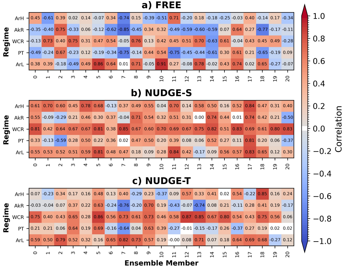
Figure 3.12: The correlation between the MERRA-2 WRI and the CESM2 CAM6 forecast WRI initialized on 29 December 2003 for the lead time extending from 14 days prior to the CAO to 31 January 2004 (i.e., end of the CAO), as a function of ensemble member.
