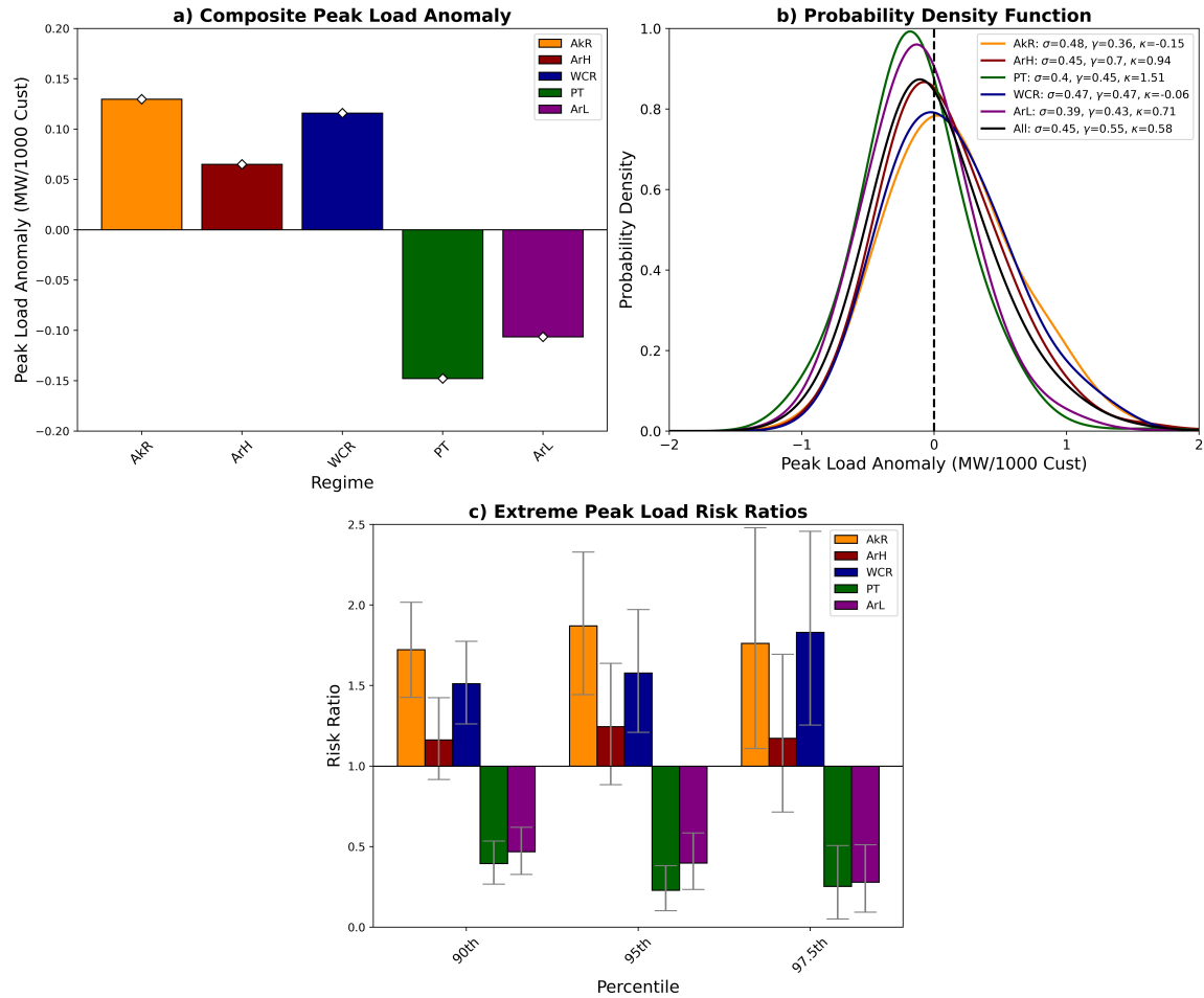
Figure 6.3: (a) The composite mean peak load anomaly (bars, MW/1000 customers) as a function of North American winter weather regime, where white diamonds indicate that the composite value is statistically significant at the 95th percentile via 5000-iteration bootstrapping with replacement. (b) The probability density function for peak load anomaly (lines, MW/1000 customers) as a function of North American winter weather regime via Gaussian kernel density estimation. \sigma , \gamma , and \kappa represent the probability density function standard deviation, skewness, and kurtosis, respectively. (c) The risk ratios of extreme peak load by North American weather regime (bars) for 90th percentile, 95th percentile, and 97.5th percentile extreme thresholds versus that of the entire distribution. Whiskers represent the 95th percentile confidence interval for each risk ratio from 5000-iteration bootstrapping with replacement. For all plots, AkR is orange, ArH is red, WCR is blue, PT is green, and ArL is purple.
