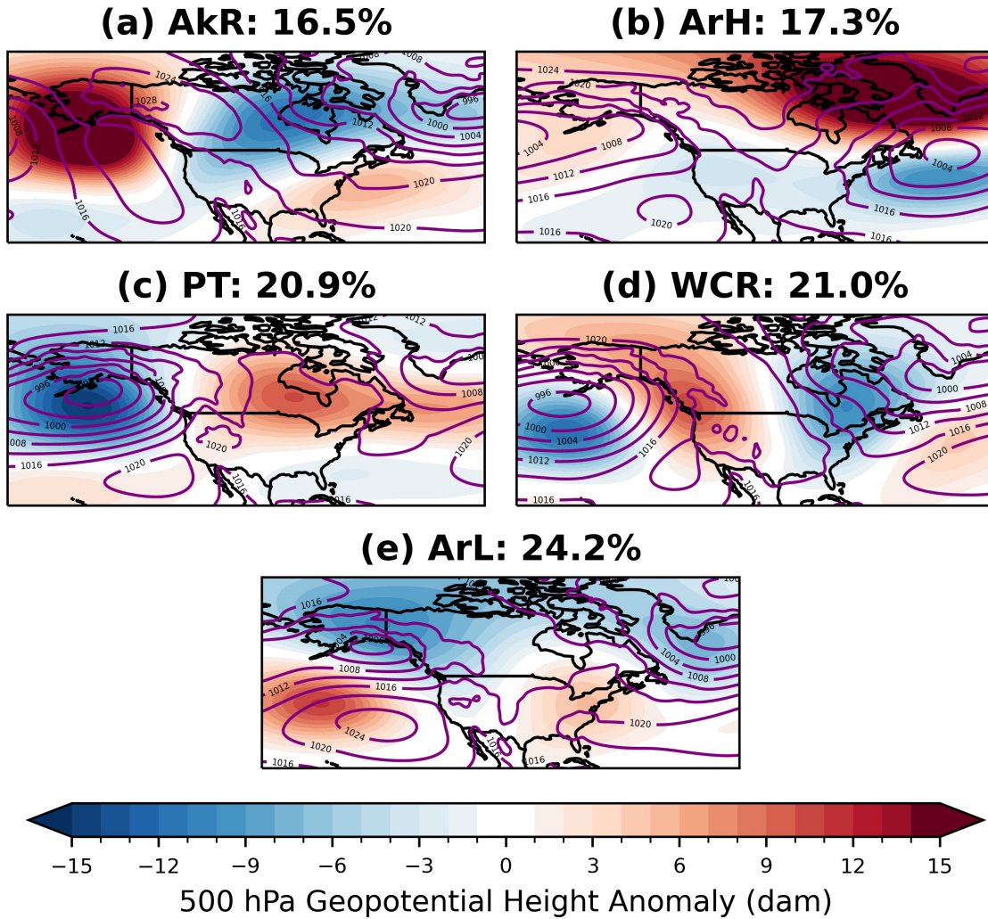
Figure A.13: Composite mean maps of ERA5 linearly detrended 500 hPa GPH anomalies (shading, dam) and full-field MSLP (contours, hPa) for a) the Alaskan Ridge (AkR), b) the Arctic High (ArH), c) the Pacific Trough (PT), d) the West Coast Ridge (WCR), and e) the Arctic Low (ArL), respectively. Percentages on panels represent the frequency of days occupied by a given winter weather regime in the 1950-2023 period. Anomalies are with respect to the 1979-2020 climatology.
