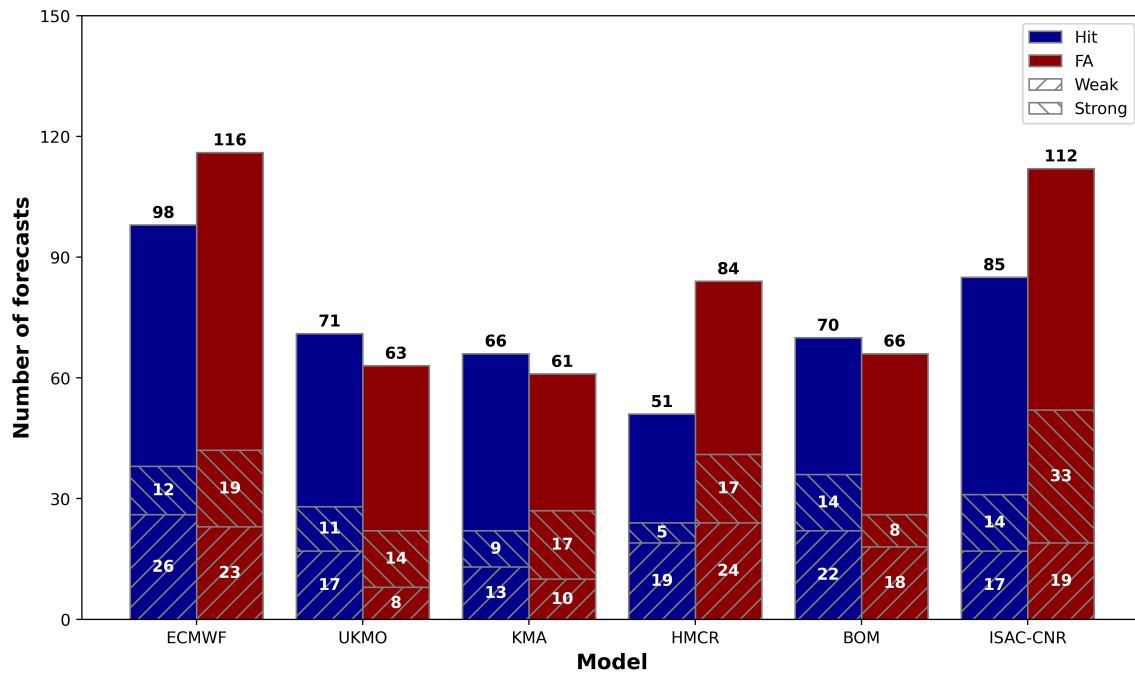
Figure 4.6: The total number of confident hit (blue solid bars) and confident false alarm (red solid bars) forecasts as a function of S2S model for Week 3 cold spells. The left-to-right hatching indicates the proportion of confident hit and false alarm forecasts initialized in a weak SPV state while the right-to-left hatching indicates the proportion of confident hit and false alarm forecasts initialized in a strong SPV state. The bold numbers show the respective counts of these different proportions.
