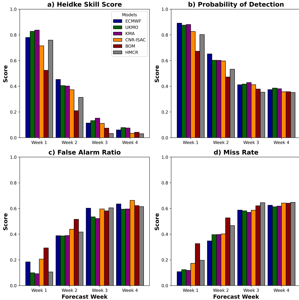
Figure 4.1: The skill of ECMWF (blue bars), UKMO (green bars), KMA (purple bars), CNR-ISAC (orange bars), BOM (red bars), and HMCR (gray bars) models in forecasting cold weeks as a function of forecast week in terms of (a) HSS, (b) POD, (c) FAR, and (d) MR.
