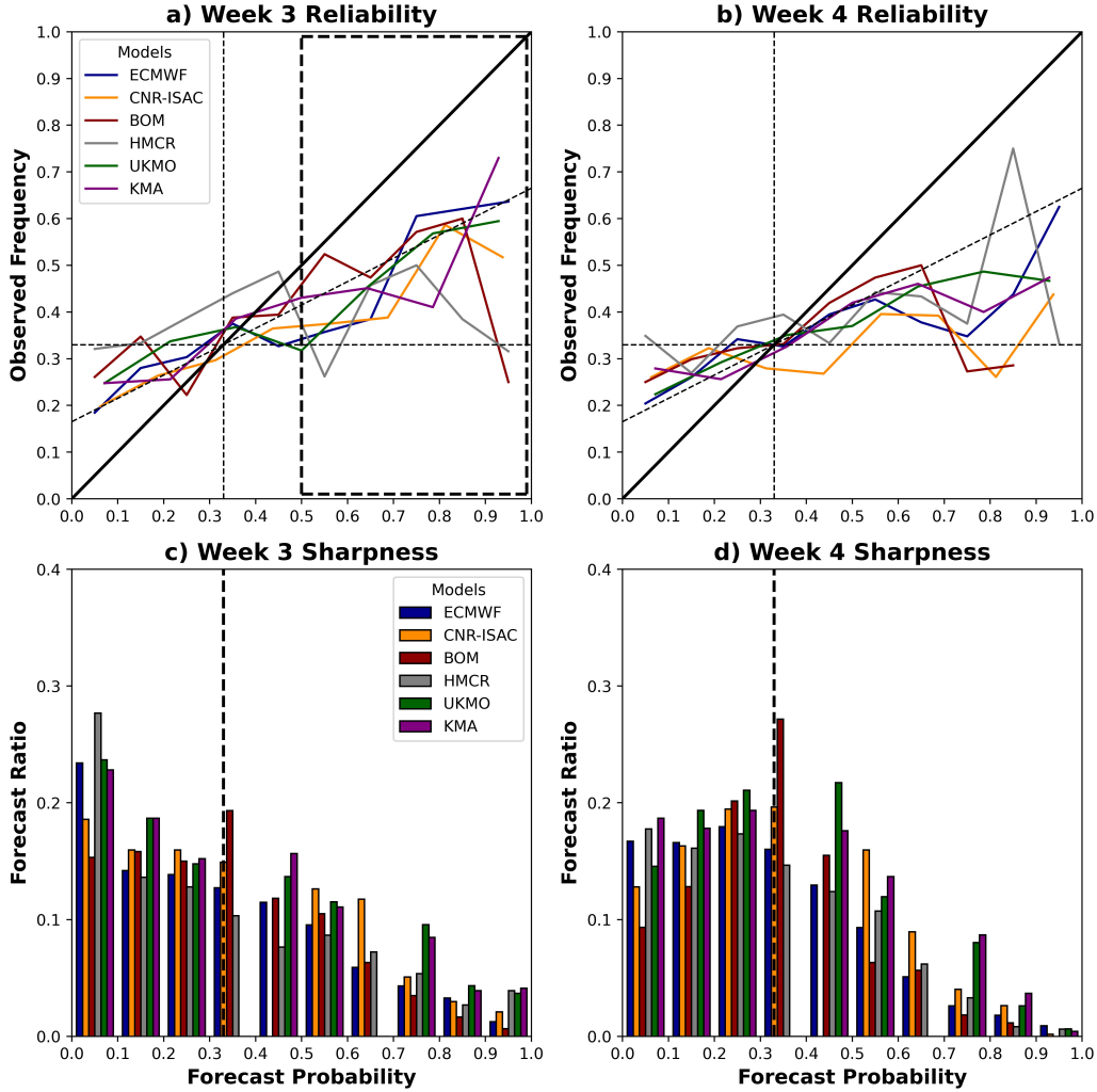
Figure 4.2: Reliability diagrams and sharpness histograms for the S2S models in forecasting (a,c) Week 3 and (b,d) Week 4 cold spells. For the reliability diagrams, the forecast probability is shown in the x -axis and the observed relative frequency is shown on the y -axis, the horizontal and vertical dashed gray lines represent the climatological frequency, the diagonal black line represents the perfect reliability 1:1 line, the diagonal dashed gray line represents the “no-skill” line, and the dashed black box is the region of confident forecasts (i.e., 50%+ forecast probability). The sharpness histograms have forecast probability on the x -axis and forecast ratio on the y -axis, where the vertical dashed black line represents the climatological frequency (i.e., the climatological expected rate of occurrence).
