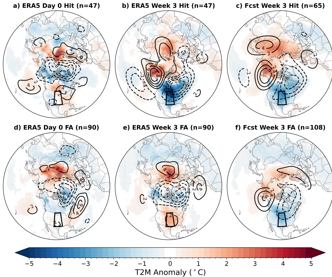
Figure 4.9: As in Fig. 4.3 but for forecasts initialized in strong polar vortex states.
