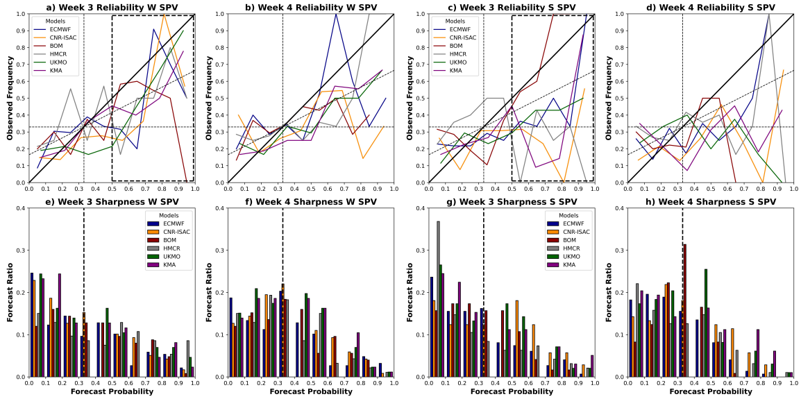
Figure 4.7: As in Fig. 4.2 but the forecast reliability diagrams and sharpness histograms of Week 3 and Week 4 cold spells initialized in (a,b,e,f) weak SPV conditions and (c,d,g,h) strong SPV conditions. Note that here the cumulative number of forecasts used for this analysis is 695 for weak SPV forecasts and 665 for strong SPV forecasts, compared to the total number of 3454 used in Fig. 4.2.
