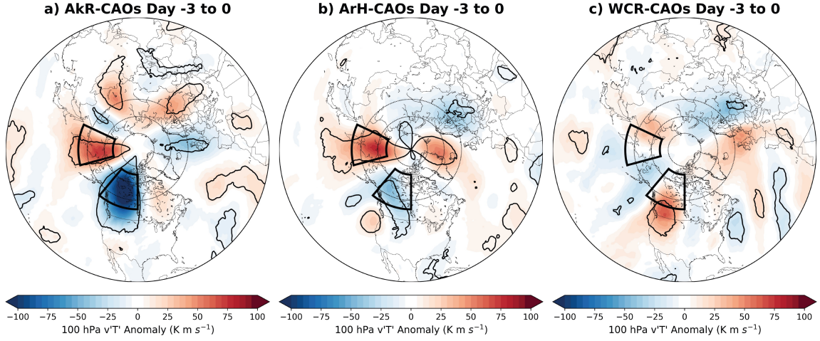
Figure A.4: Composites of the 100 hPa v'T' anomalies ( \text{K m s}^{-1} , shaded) across the Northern Hemisphere for (a) AkR-CAOs, (b) ArH-CAOs, and (c) WCR-CAOs for Days -3 to 0. Black contours represent significance at the 95th percentile via a bootstrapping approach of 5000 iterations.
