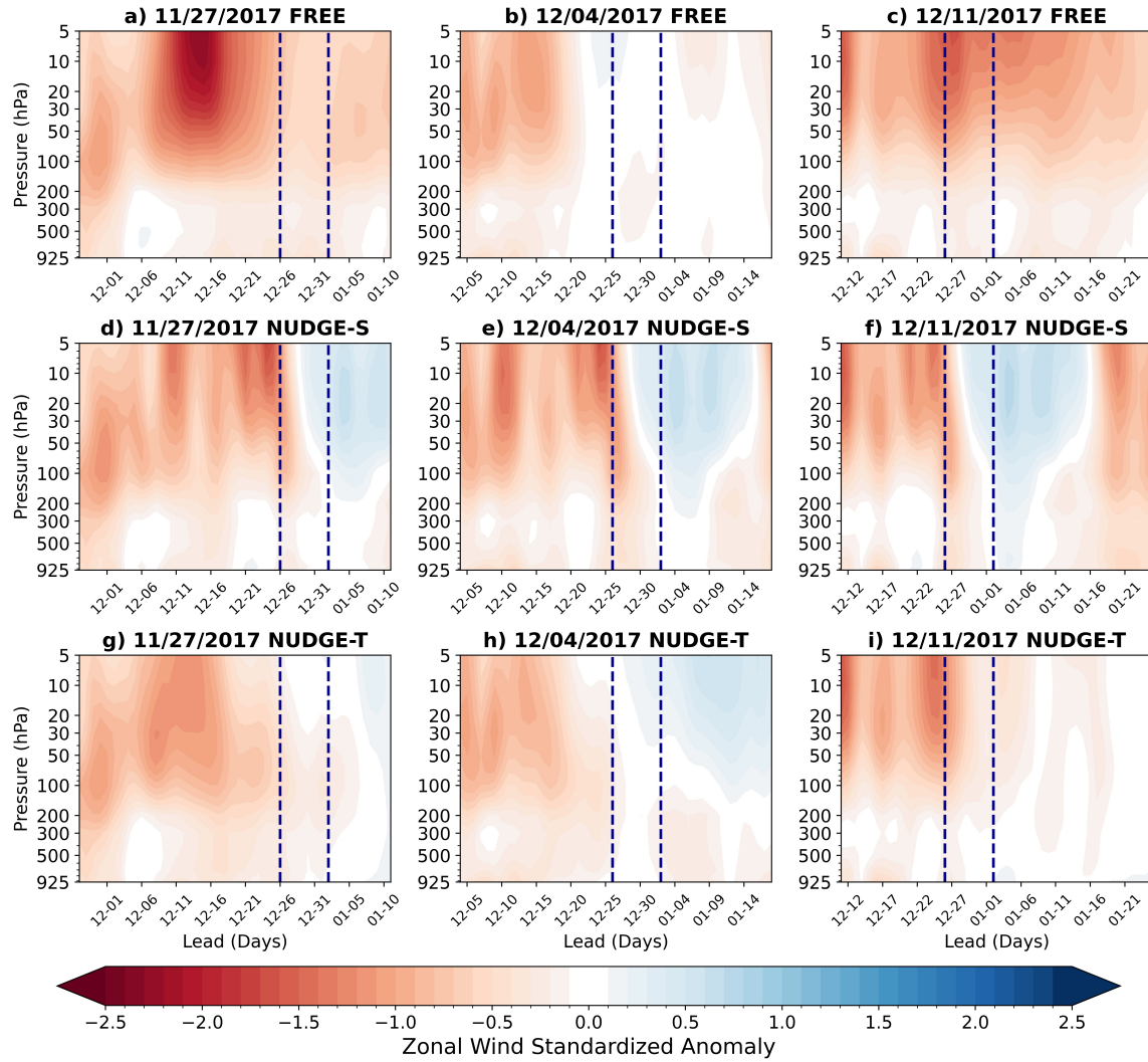
Figure A.6: The evolution of the ensemble mean zonal wind standardized anomaly (shading) averaged over the polar cap (60–90°N for the three subseasonal forecast initializations of 27 November 2017, 4 December 2017, and 11 December 2017 for a)–c) the FREE experiments, d)–f) the NUDGE-S experiments, and g)–i) the NUDGE-T experiments, respectively. The dashed lines show the start and end dates of the central US CAO.
