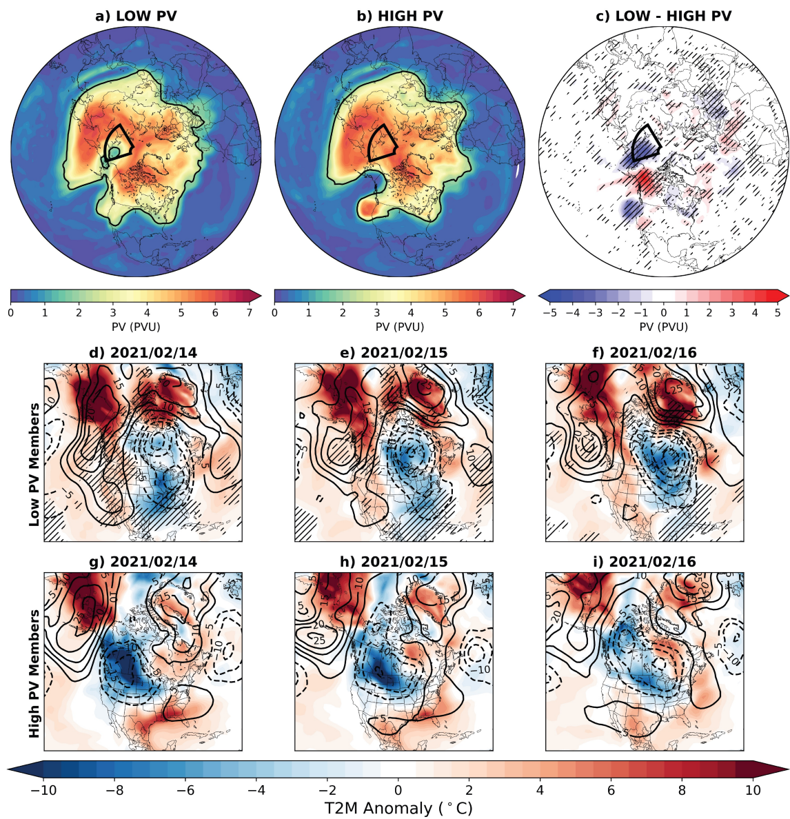
Figure A.11: As in Fig. 5.4 but for the 3 highest and lowest East Siberian Sea 320 K PV ensemble members in the NCEP model.
