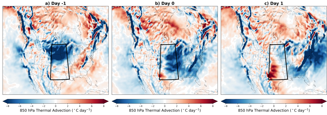
Figure A.1: Lagged composites of the 850 hPa horizontal thermal advection (shaded, ^{\circ}\text{C day}^{-1} ) for all 37 CAOs for a) Day -1, b) Day 0, and c) Day 1. Positive lags represent days after CAO onset day (Day 0) and negative lags represent days prior to CAO onset. The thick, black box represents the region over which the CAOs were defined.
