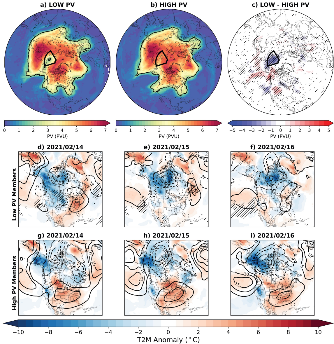
Figure 5.4: 28 January 2021 initialization ECMWF 320 K PV composites (PVU, shaded) for the 5 ensemble members with the a) lowest and b) highest PV in the East Siberian Sea region (black box) averaged over 2-4 February 2021. c) The difference (PVU, shaded) between the low and high PV composites. d) – f) Composites of T2M (°C, shaded) and 500 hPa GPH (dam, line contours) anomalies for the 5 ensemble members with the lowest PV in the East Siberian Sea region. g) – i) As in d) – f) but for the 5 ensemble members with the highest PV in the East Siberian Sea region. Hatching in panels c) – f) denote statistical significance ( p < 0.1 ) in the composite difference (low - high PV) in the PV and T2M fields, computed by a 5000-iteration bootstrapping technique, without replacement. Bold dates at the top of panels d)–i) indicate the valid date for the forecasts.
