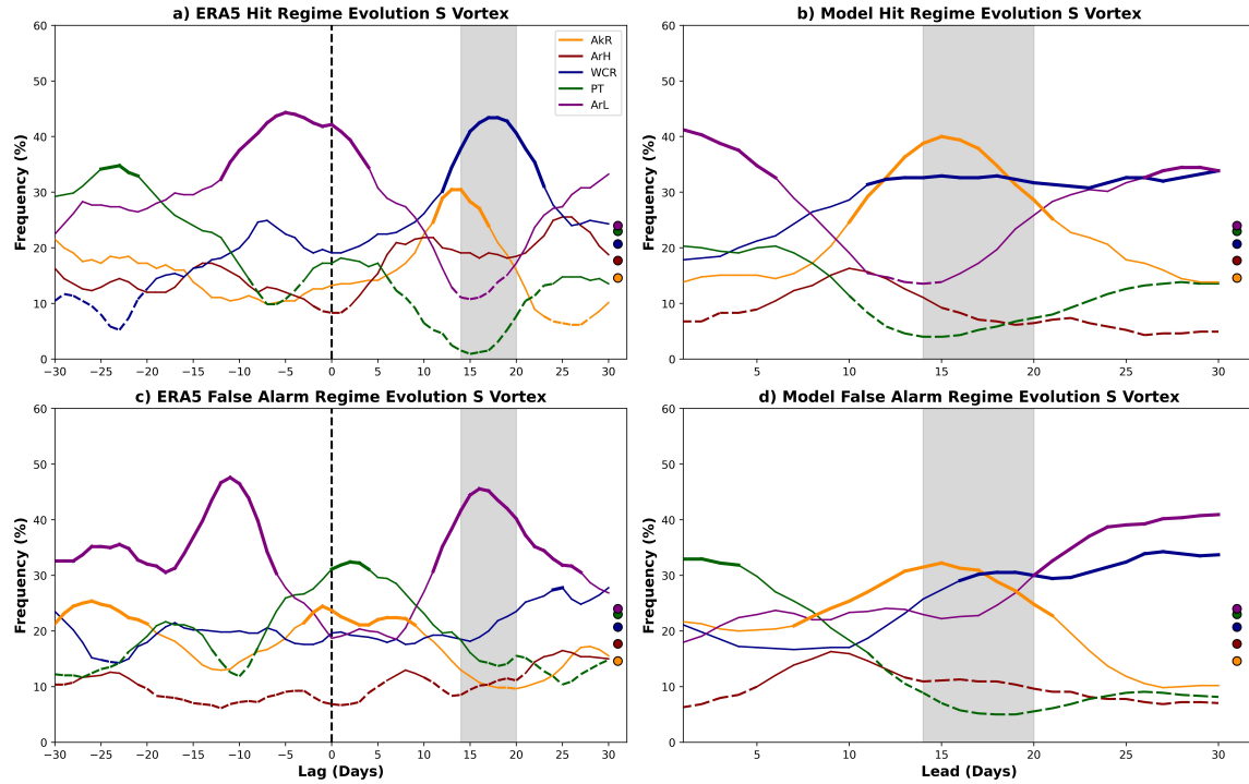
Figure 4.11: As in Fig. 4.4 but for forecasts initialized in strong polar vortex states.
