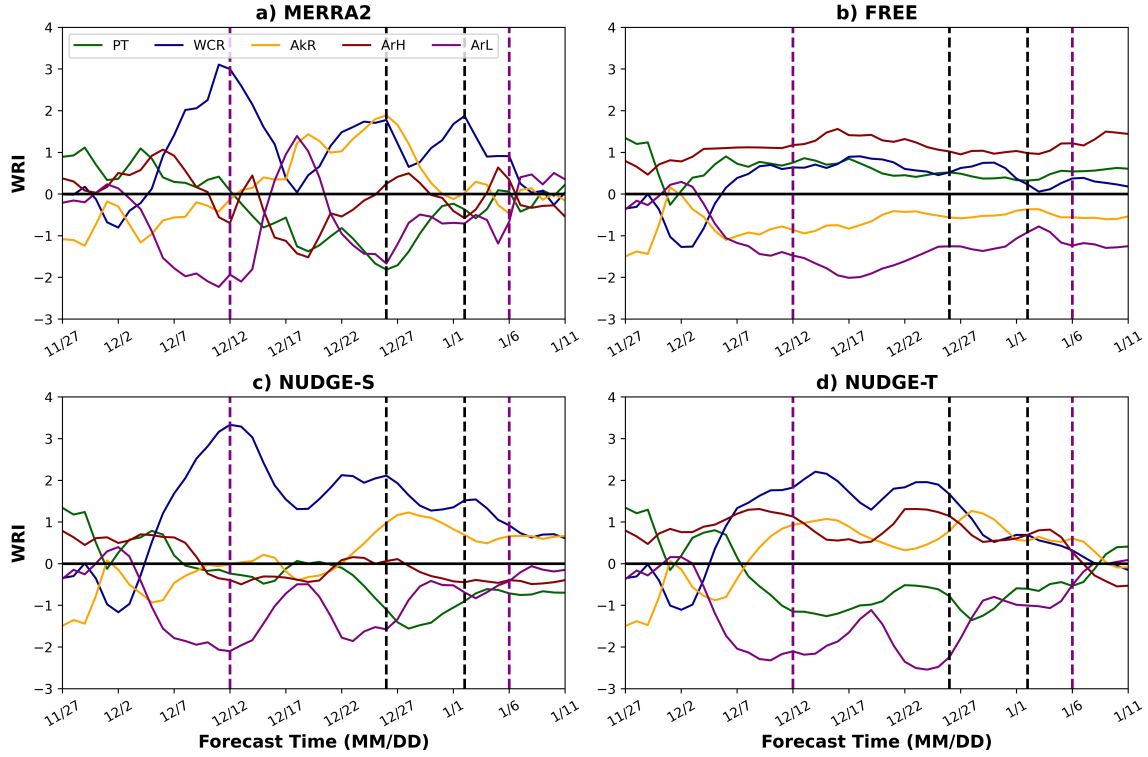
Figure 3.6: The evolution of the ensemble mean WRI for the five North American winter weather regimes for the 27 November 2017 CESM2 CAM6 initialization in a) the MERRA-2 evolution, b) the FREE experiment, c) the NUDGE-S experiment, and d) the NUDGE-T experiment. The green line represents the Pacific Trough (PT), the blue line represents the West Coast Ridge (WCR), the orange line represents the Alaskan Ridge (AkR), the red line represents the Arctic High (ArH), and the purple line represents the Arctic Low (ArL). The black dashed lines show the start and end dates of the 2017/2018 CAO. The purple dashed lines represent the start and end of the period used for correlation analysis in Fig. 3.7.
