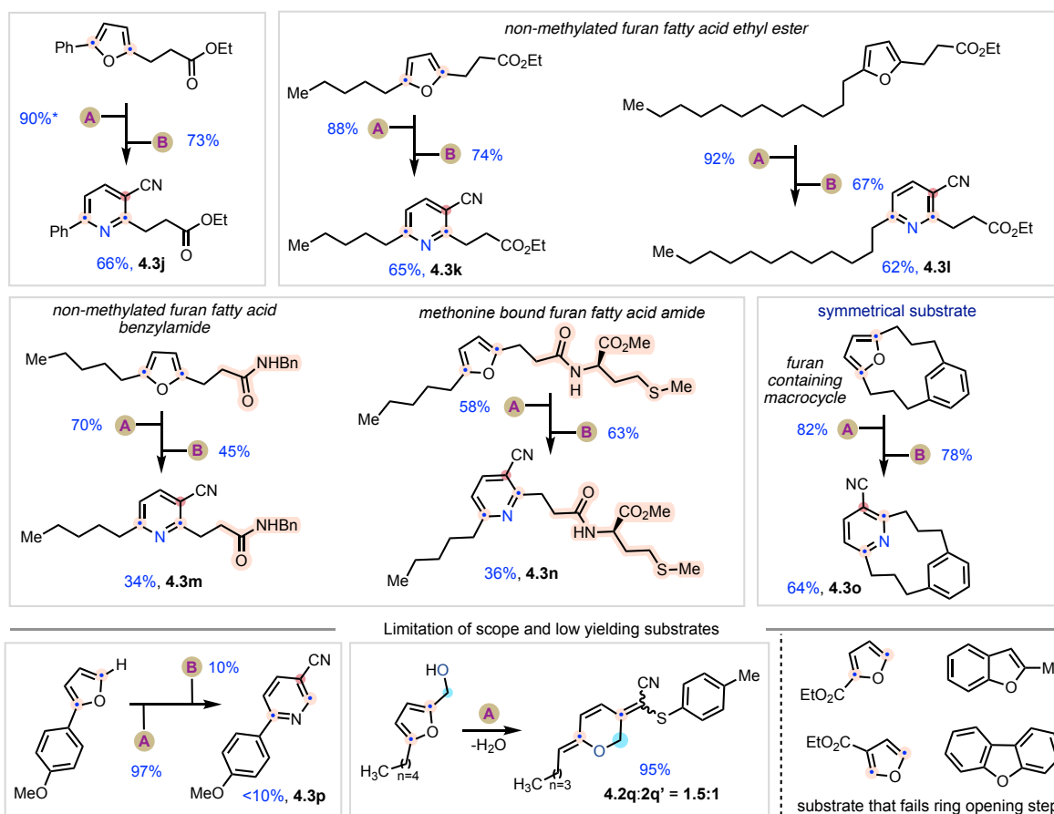
Figure 4.2.4.2: Application to biorelevant furans and limitations of the methodology.
