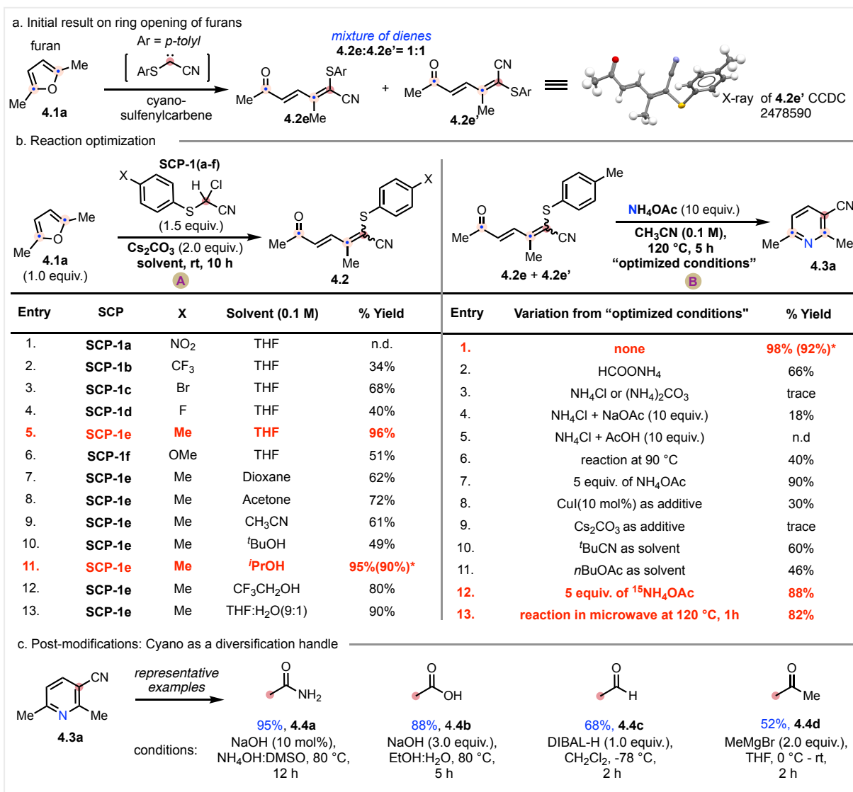
Figure 4.2.1.1: Reaction optimization of furans to 3-cyanopyridines. Conditions A. Reactions were carried out on a 0.5–1.0 mmol scale in a sealed vial. 1a (1.0 equiv.), SCP (1.5 equiv.), base (2.0 equiv.), solvent (0.1 M); Conditions B. Reactions were carried out on a 0.5–1.0 mmol scale in a sealed tube 2 (1.0 equiv.), source of ammonia (10 equiv.), solvent (0.1 M). Yields were determined by 1 H-NMR. Not detected (n.d.). *Isolated yield of reaction in 1 mmol scale.
