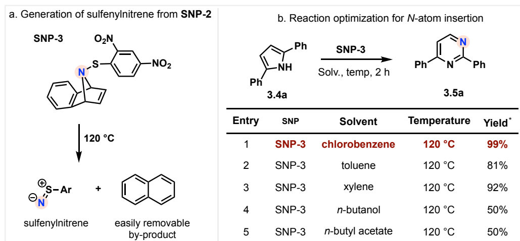
Figure 3.2.2.3: Generation of sulfenylNitrene from SNP-3 and reaction optimization for N -atom insertion.
