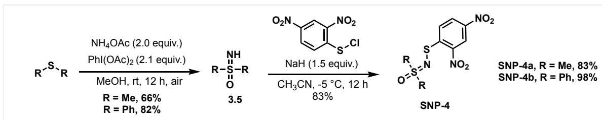
Figure 3.2.1.2.1: Synthesis of sulfoximine-based precursors ( SNP-4a and SNP-4b ).
