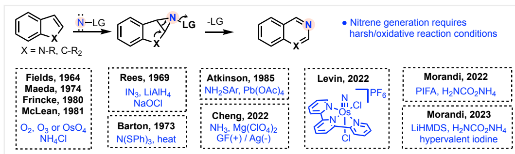
Figure 3.1.2: Concept of nitrogen-atom insertion into arenes.
