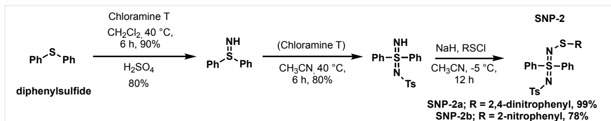
Figure 3.2.1.2.2: Synthesis of sulfodiimide-based precursors ( SNP-2a and SNP-2b ).
