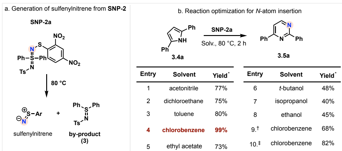
Figure 3.2.2.2: Generation of sulfenylNitrene from SNP-2 and reaction optimization for N -atom insertion. †1 equiv. of SNP-2 was used. ‡1.5 equiv. of SNP-2 was used.
