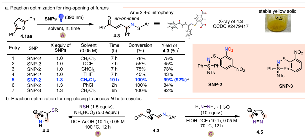
Figure 4.2.3: Reaction optimization of furans to pyrroles and pyridazine. Condition A. Reactions were carried out on a 0.1–1.0 mmol scale in a sealed vial. 4.1aa (1.0 equiv.), SNP-2 (1.3 equiv.), dichloromethane (CH 2 Cl 2 ) (0.1 M) and irradiated at 390 nm. *Yields were determined by 1 H-NMR. a Isolated yield and reaction was done in 1 mmol scale.
