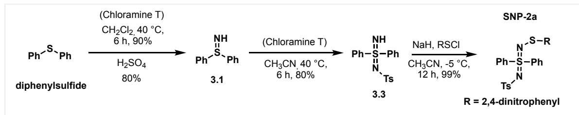
Figure 3.2.1.1.2: Synthesis of a sulfodiimide-based sulfenylNitrene precursor ( SNP-2 ).
