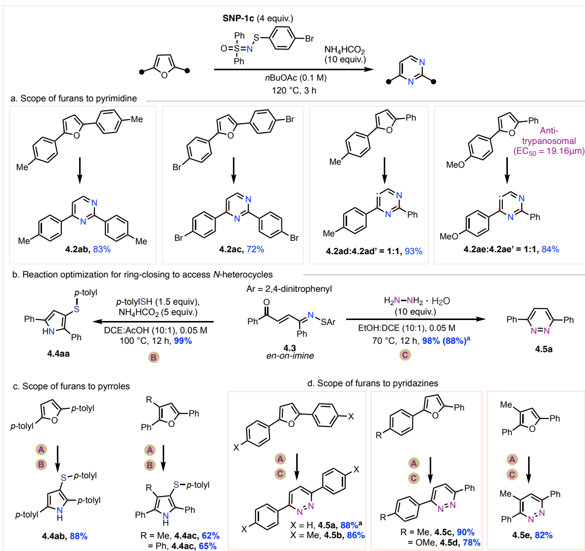
Figure 4.2.5: Scope and regioselectivity of furans to pyrimidines, pyrroles, and pyridazine.
