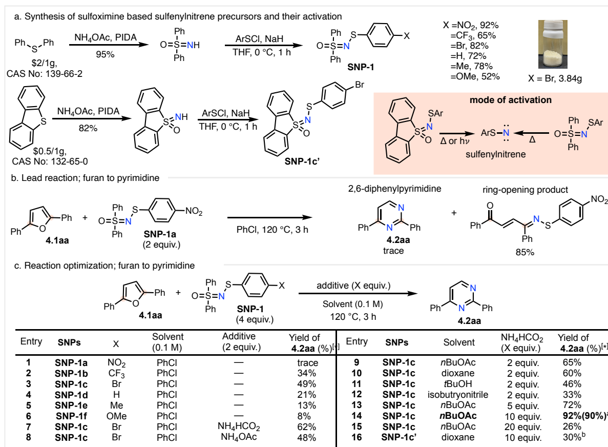
Figure 4.2.2: Reaction optimization of furans to pyrimidine. Conditions: Reactions were carried out on a 0.5–1.0 mmol scale in a sealed vial. 4.1aa (1.0 equiv.), SNP (4.0 equiv.), additive (10.0 equiv.), solvent (0.1 M). *Yields were determined by 1 H-NMR using 1,3,5-trimethoxybenzene as an internal standard. a Isolated yield. b Reaction was done in UV-irradiation (300 nm) at rt for 12 h.
