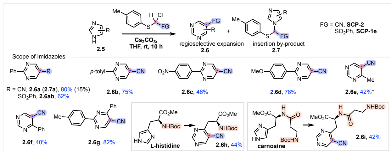
Figure 2.2.3: Scope of imidazoles. *(1:1) mixture of THF:Acetone was used as a solvent.
