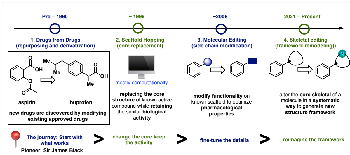
Figure 1.1.3: Conceptual evolution of skeletal editing
