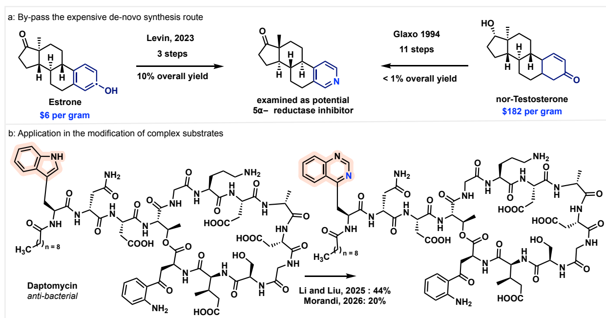
Figure 1.2.2: Skeletal editing bypassing the de-novo synthesis (a) Bypassing the expensive de-novo synthesis route (b) Application in the modification of complex substrates.
