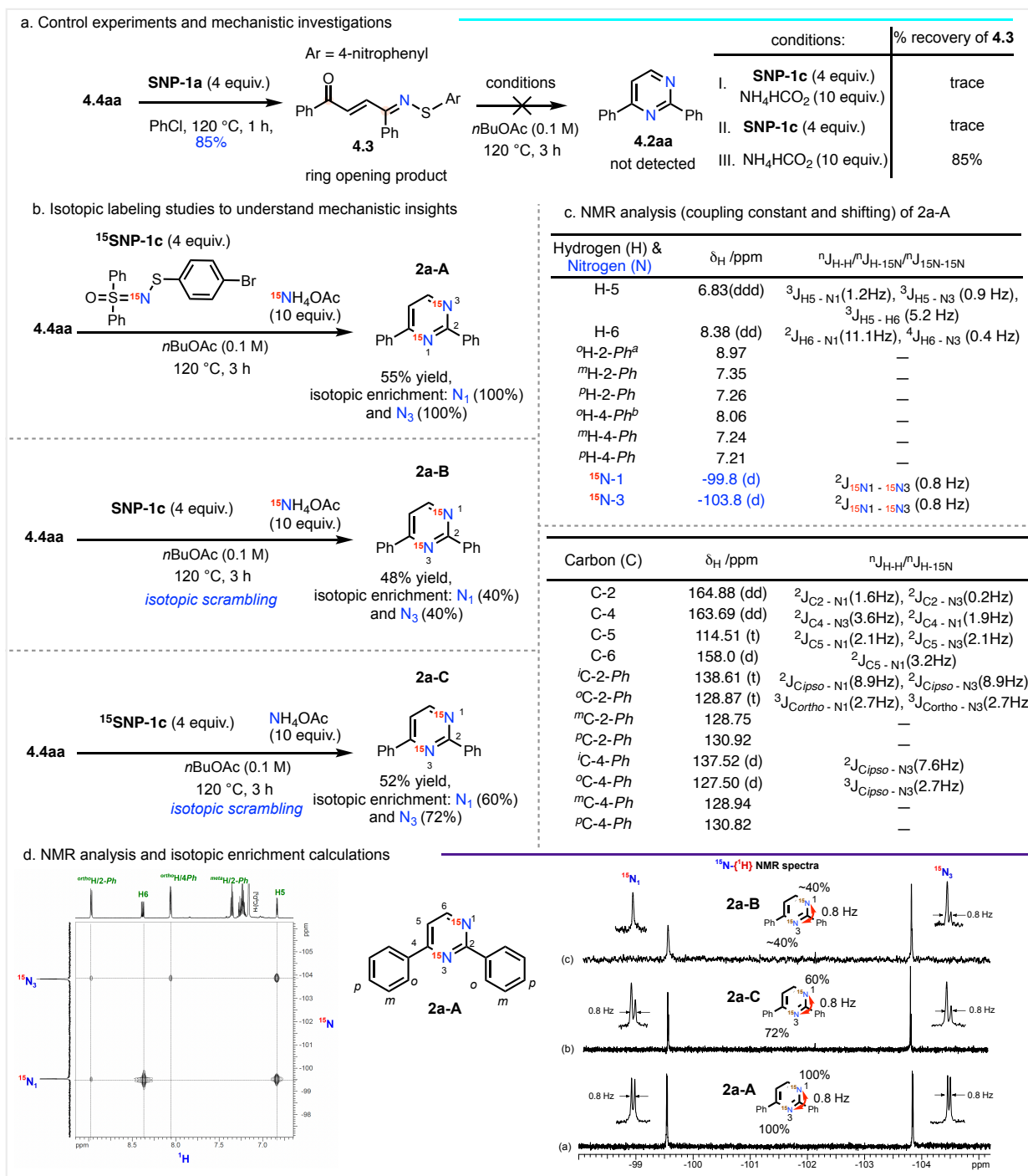
Figure 4.2.6: Control experiment, isotopic labeling, and mechanistic insight.
