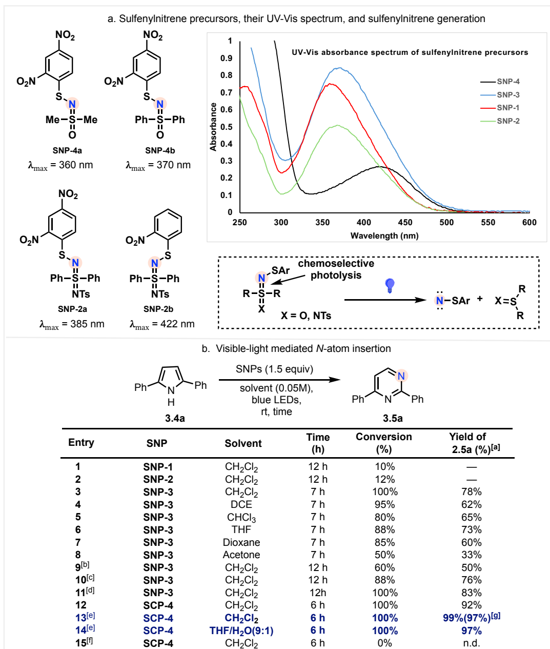
Figure 3.2.2.4: Generation of sulfenylNitrene from SNPs under photolysis conditions and optimization for N-atom insertion. [a] Yields were determined by 1 H-NMR. [b] Irradiation with blue LEDs (390nm, 50% intensity). [c] Irradiation with blue LEDs (390 nm, 75% intensity.) [d] Irradiation with blue LEDs (390 nm, 75% intensity) and 1.8 equiv. of SNP-3. [e] Irradiation with blue LEDs (440nm, 100% intensity). [f] No irradiation. [g] Isolated yield.
