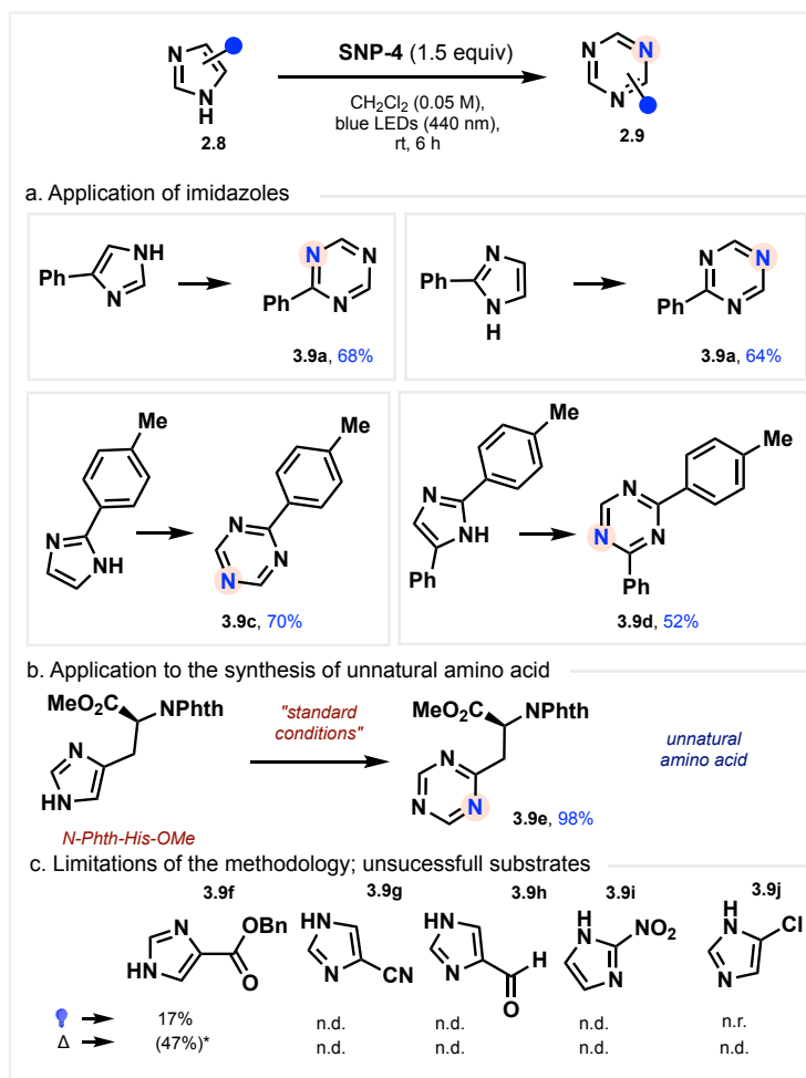
Figure 3.2.2.6.3: Scope of imidazole under photolytic conditions.
