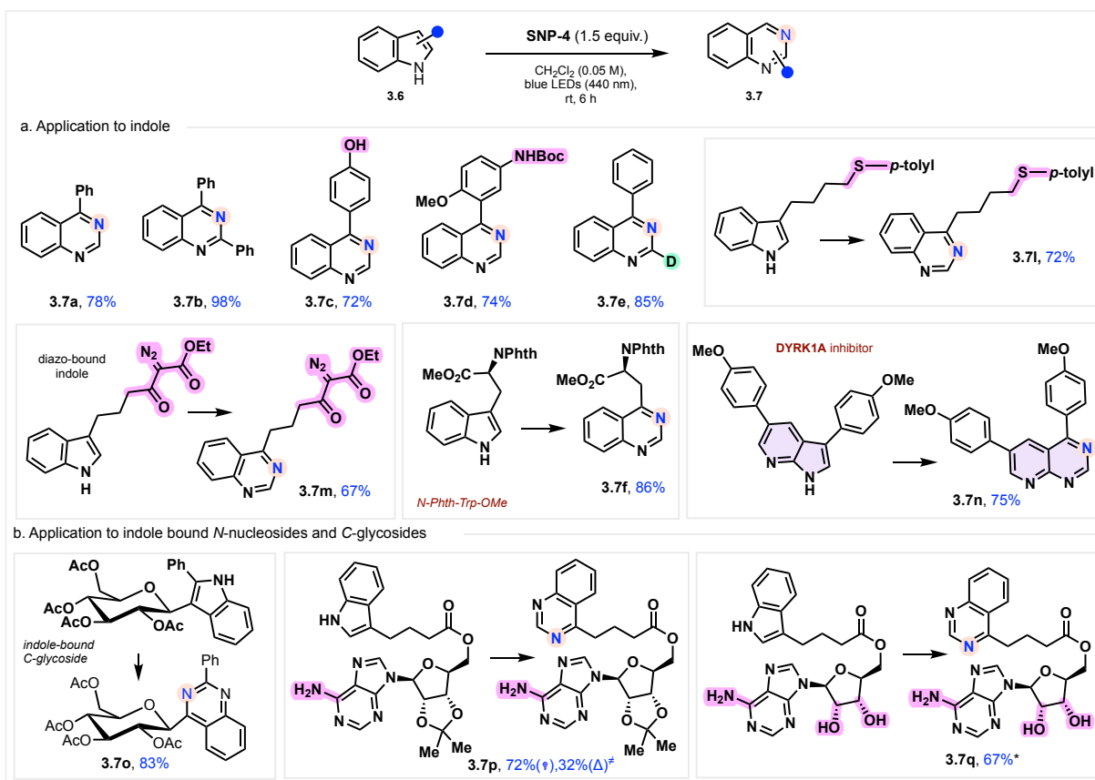
Figure 3.2.2.6.2: Scope of pyrroles under photolytic conditions.
