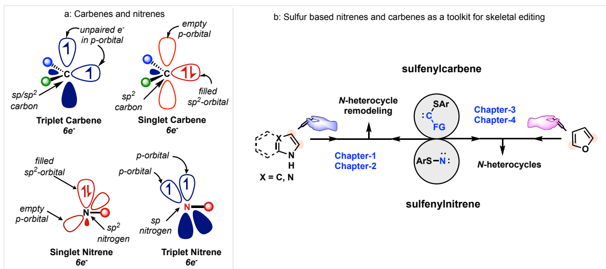
Figure 1.7: Sulfur-based nitrenes and carbenes as a toolkit for skeletal editing.
