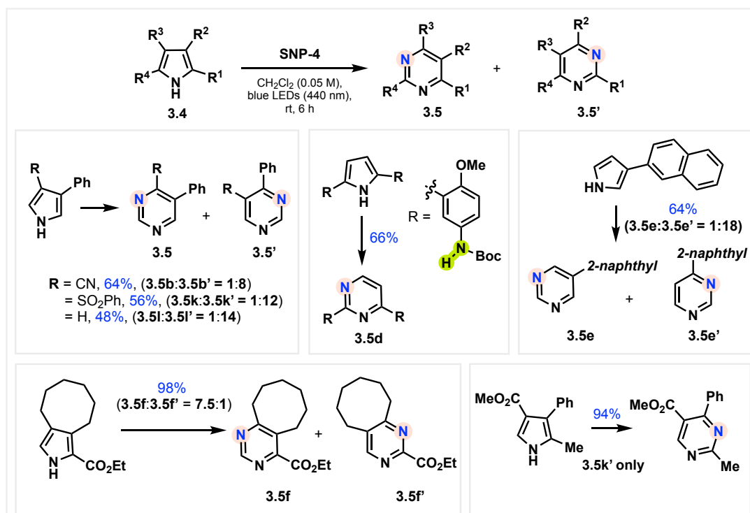
Figure 3.2.2.6.1: Scope of pyrroles under photolytic conditions.
