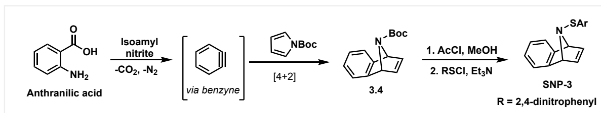
Figure 3.2.1.1.3: Synthesis of naphthalene-based precursor ( SNP-3a ).
