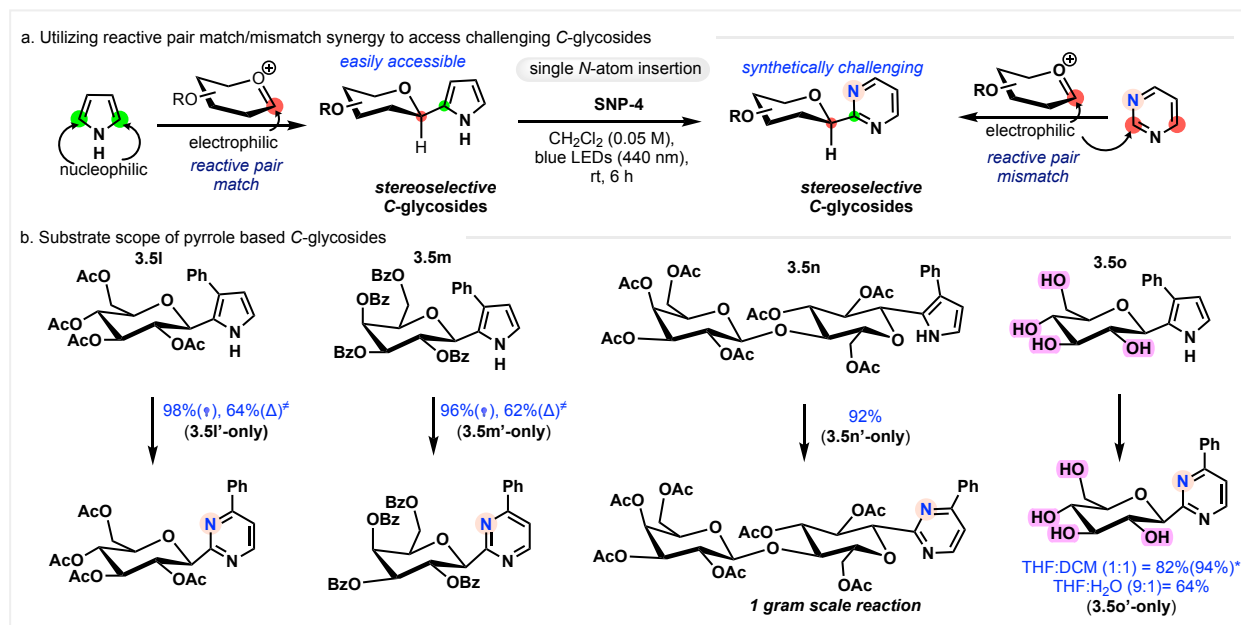
Figure 3.2.2.6.4: Scope of C-glycosides bearing pyrrole.
