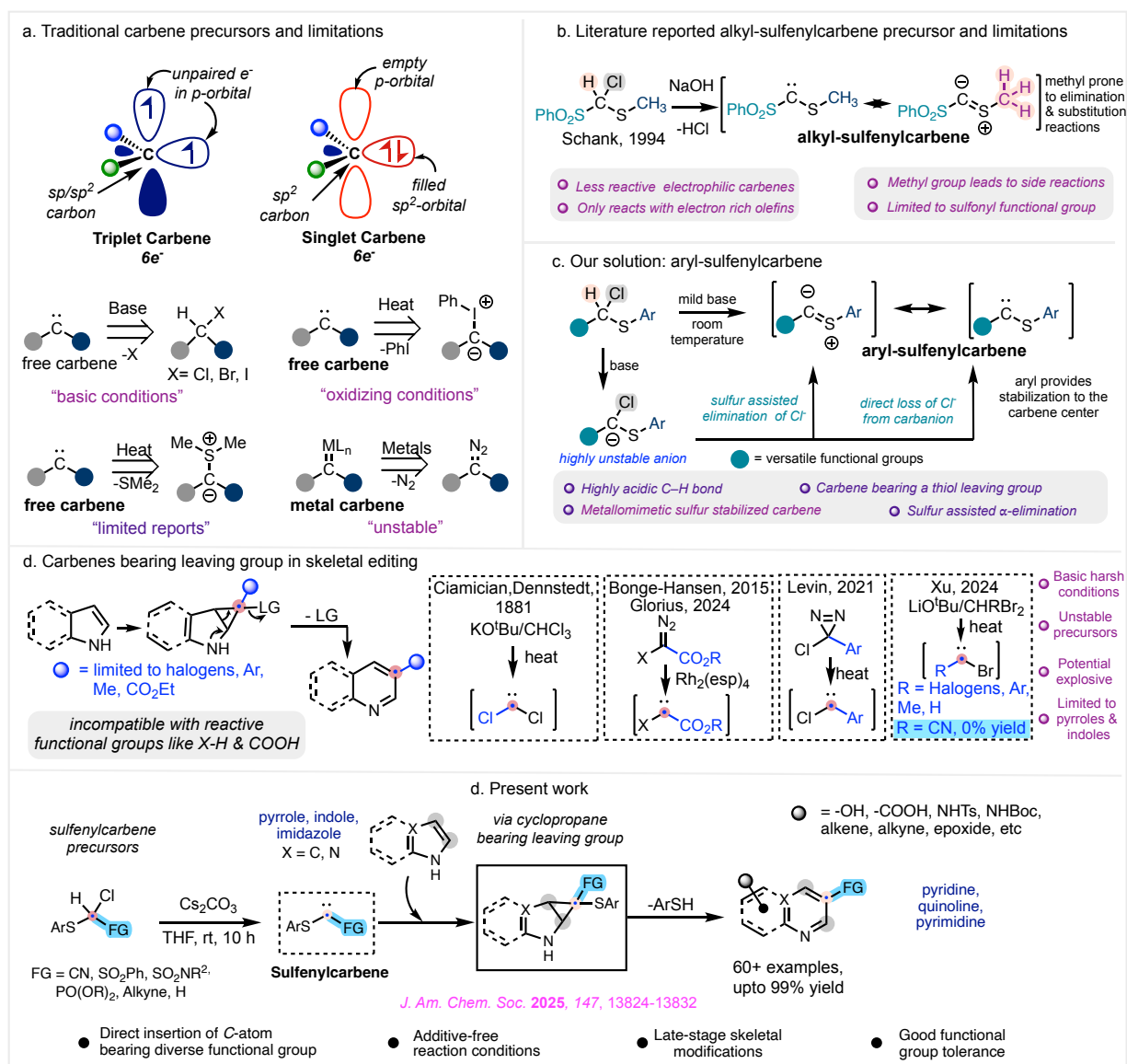
Figure 2.1: State of art for sulfenylcarbene generation. (a) Traditional carbene and their limitations. (b) Literature reported of alkylsulfenylcarbene. (c) Our solution: aryl sulfenylcarbene. (d) Present work.
