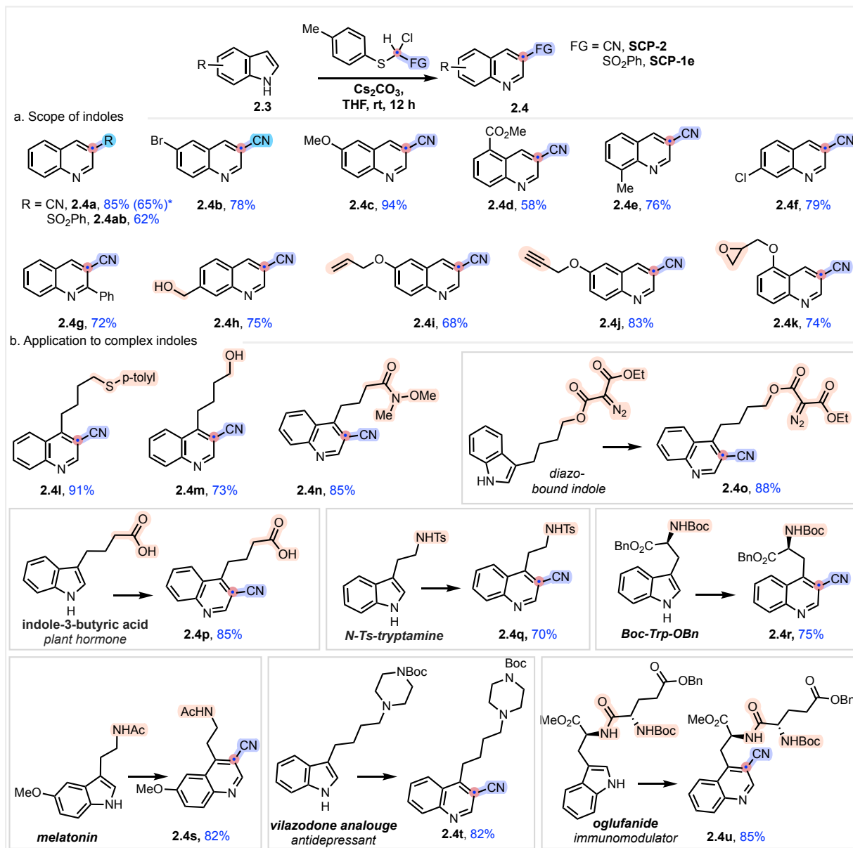
Figure 3.2.3: Scope of indoles. (a) Scope of indoles. (b) Application to complex indoles.
