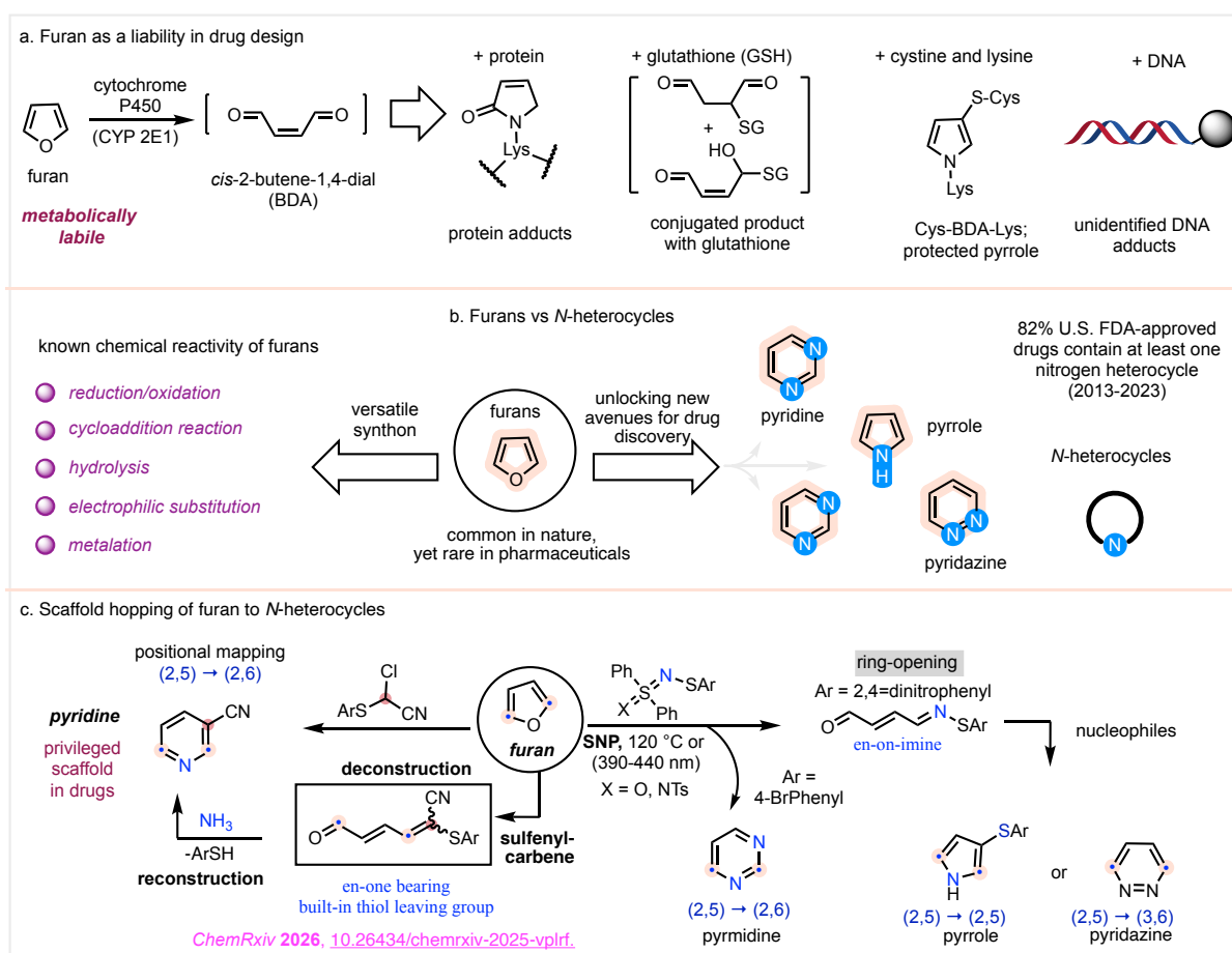
Figure 4.1: Scaffold hopping of furans into N-heterocycles by sulfenylcarbene or sulfenylnitrene.
