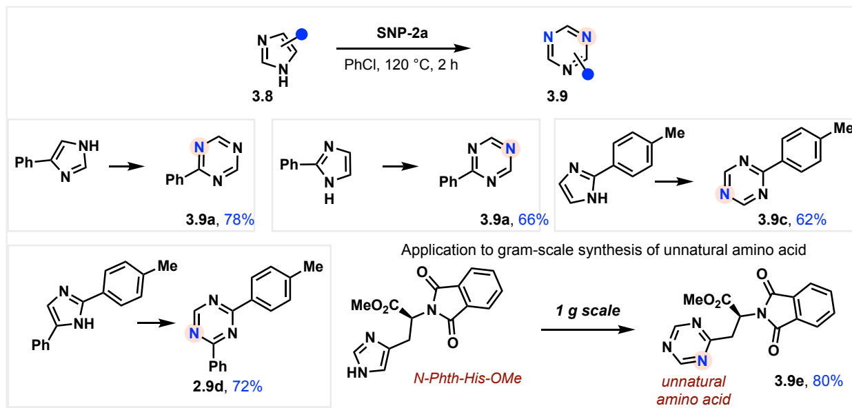
Figure 3.2.2.5.3: Scope of imidazoles under thermal conditions.
