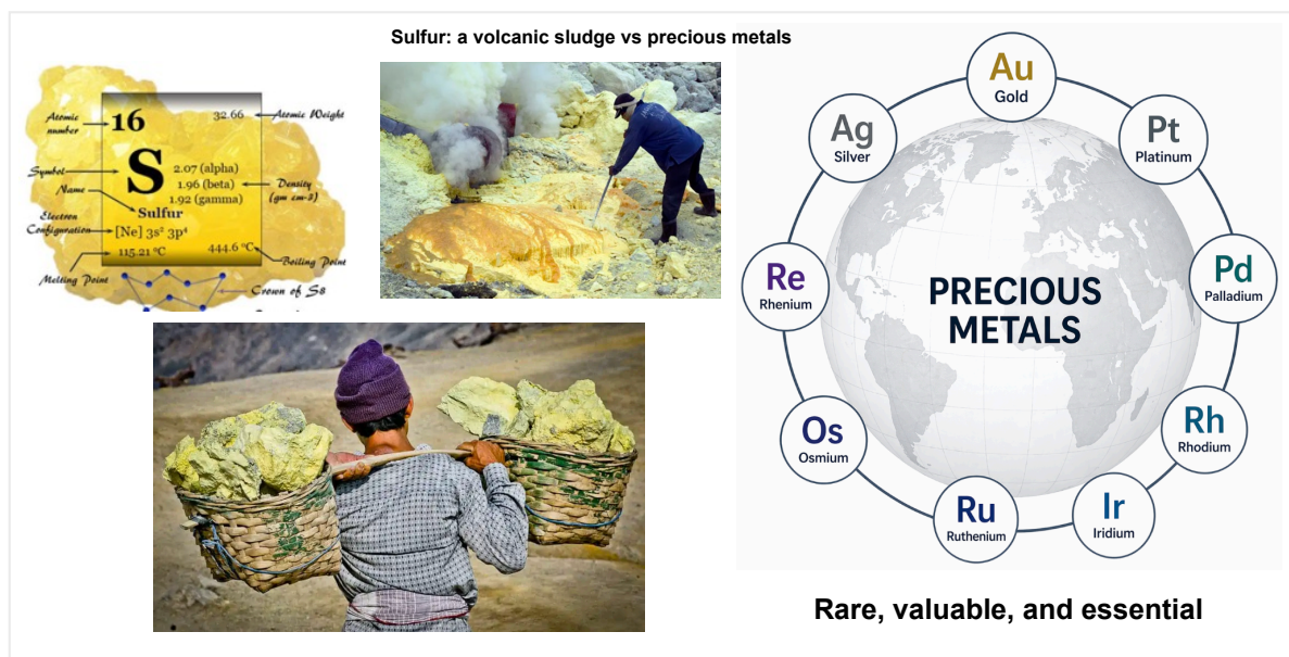
Figure 1.6: Sulfur as an alternative to precious metals.
