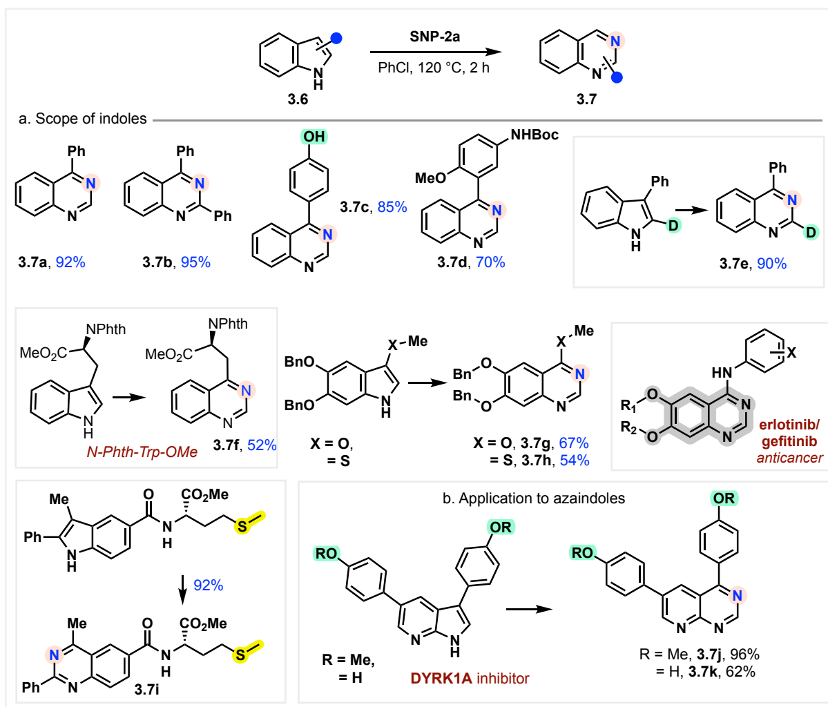
Figure 3.2.2.5.2: Scope of indoles under thermal conditions.
