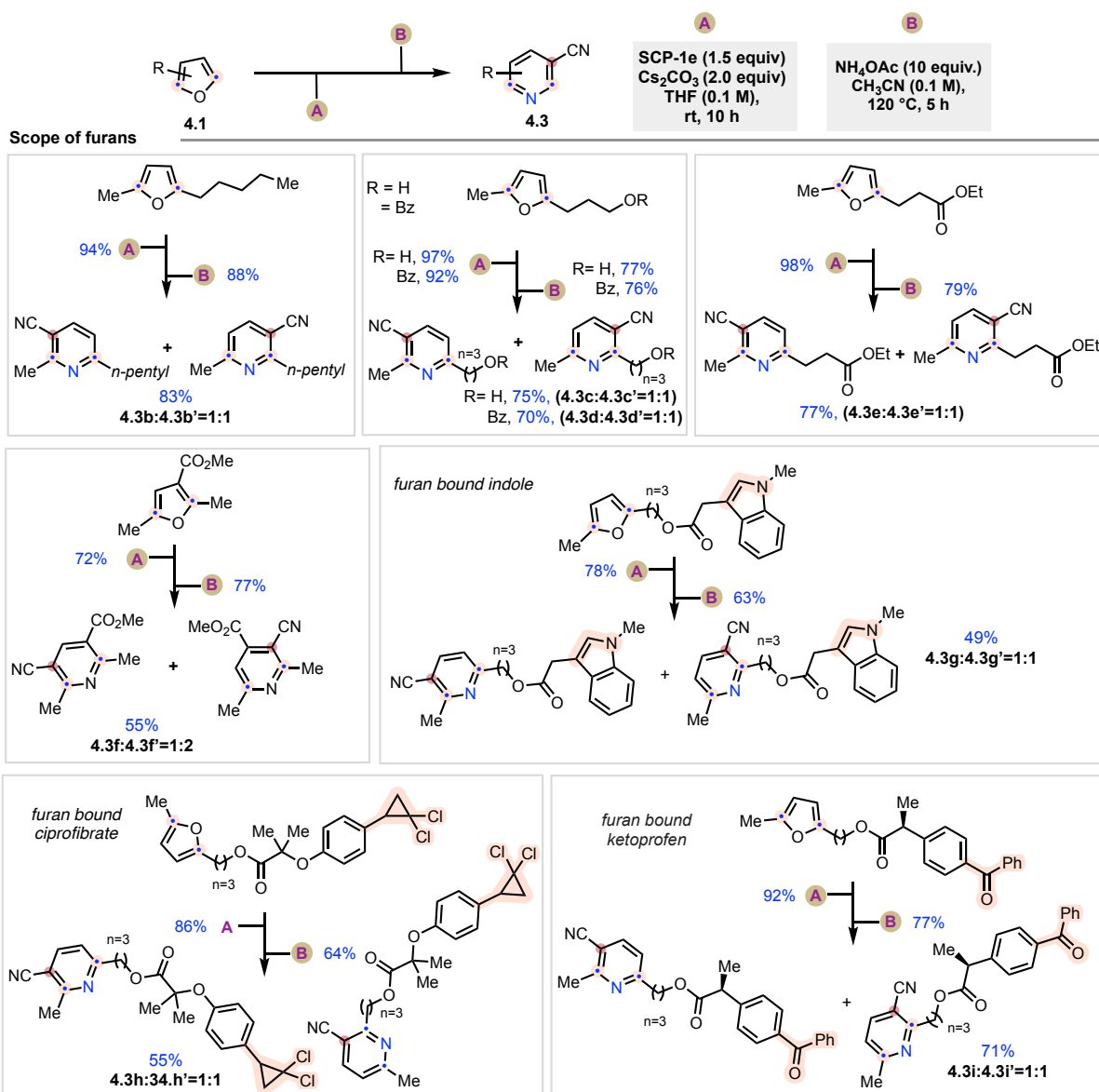
Figure 4.2.4.1: Scope and regioselectivity of furans.
