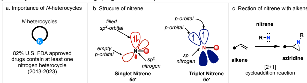
Figure 3.1.1: N -Heterocycles and nitrenes (a) Importance of N -heterocycles (b) Structure of nitrene (c) Reaction of nitrene with alkene.
