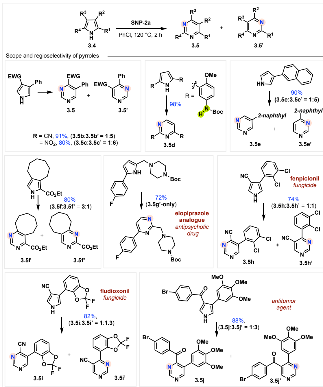
Figure 3.2.2.5.1: Substrate scope of pyrroles under thermal conditions.
