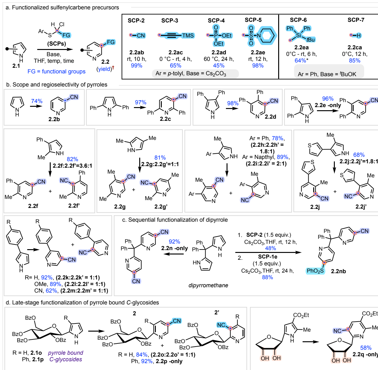
Figure 2.2.2: Scope of sulfenylcarbene and pyrroles. (a) Functionalized sulfenylcarbene precursors. (b) Scope and regioselectivity of pyrroles. (c) Sequential functionalization of di-pyrrole. (d) Late-stage functionalization of pyrrole bound C-glycosides. Reaction conditions: 2.1 (1.0 equiv.), SCP (1.5 equiv.), base (3.0 equiv.), and tetrahydrofuran (0.1 M). Reactions were carried out on 0.5–1.0 mmol scale. All the reported yields are isolated, and the regioisomeric ratio was determined by 1 H-NMR using 1,3,5-trimethoxybenzene as an internal standard. *5.0 equiv. of base was used.
