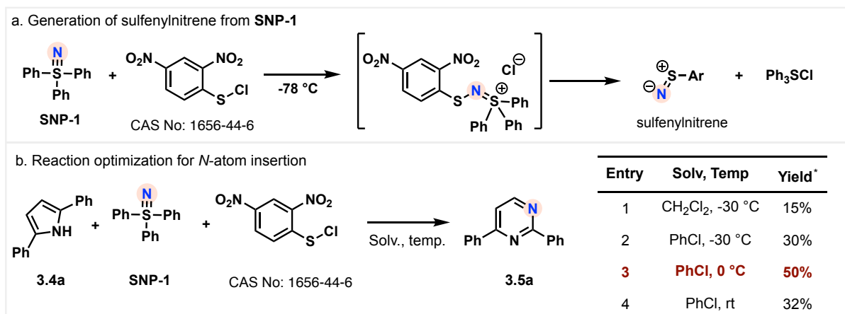
Figure 3.2.2.1: Generation of sulfenylNitrene from SNP-1 and reaction optimization for N -atom insertion.
