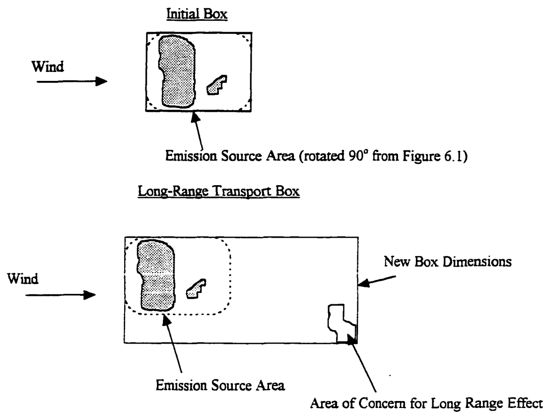
Figure 6.5: Long Range Pollutant Transport Analysis
