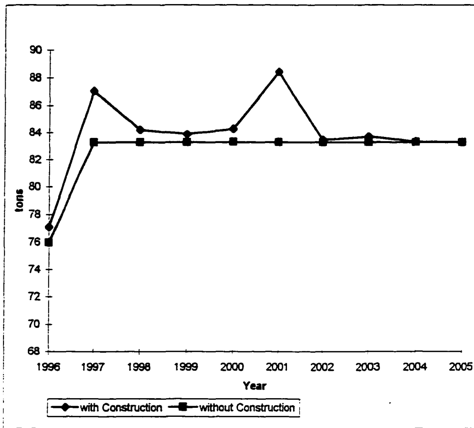
Figure D.9: AFB SO x Emission Comparisons
