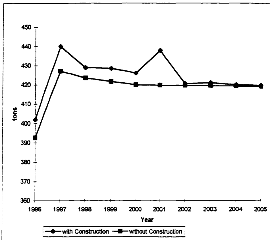
Figure D.5: AFB VOC Emission Comparisons
