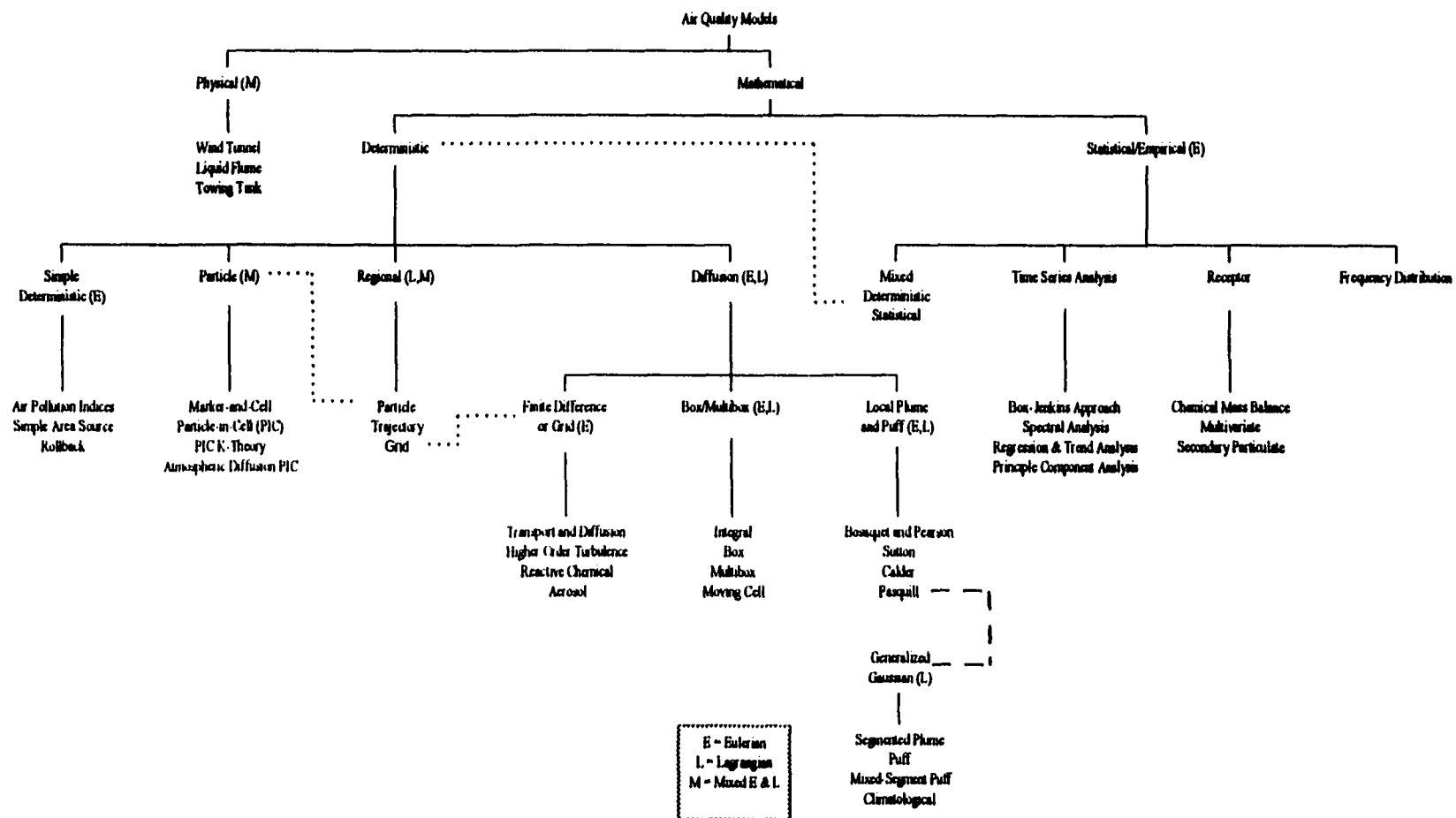
Figure A.1: Air Quality Model Classification
