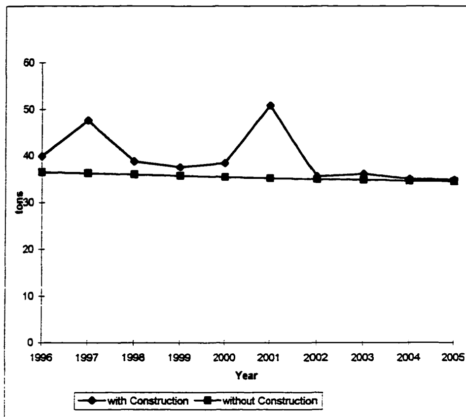
Figure D.11: AFB PM10 Emissions Comparisons
