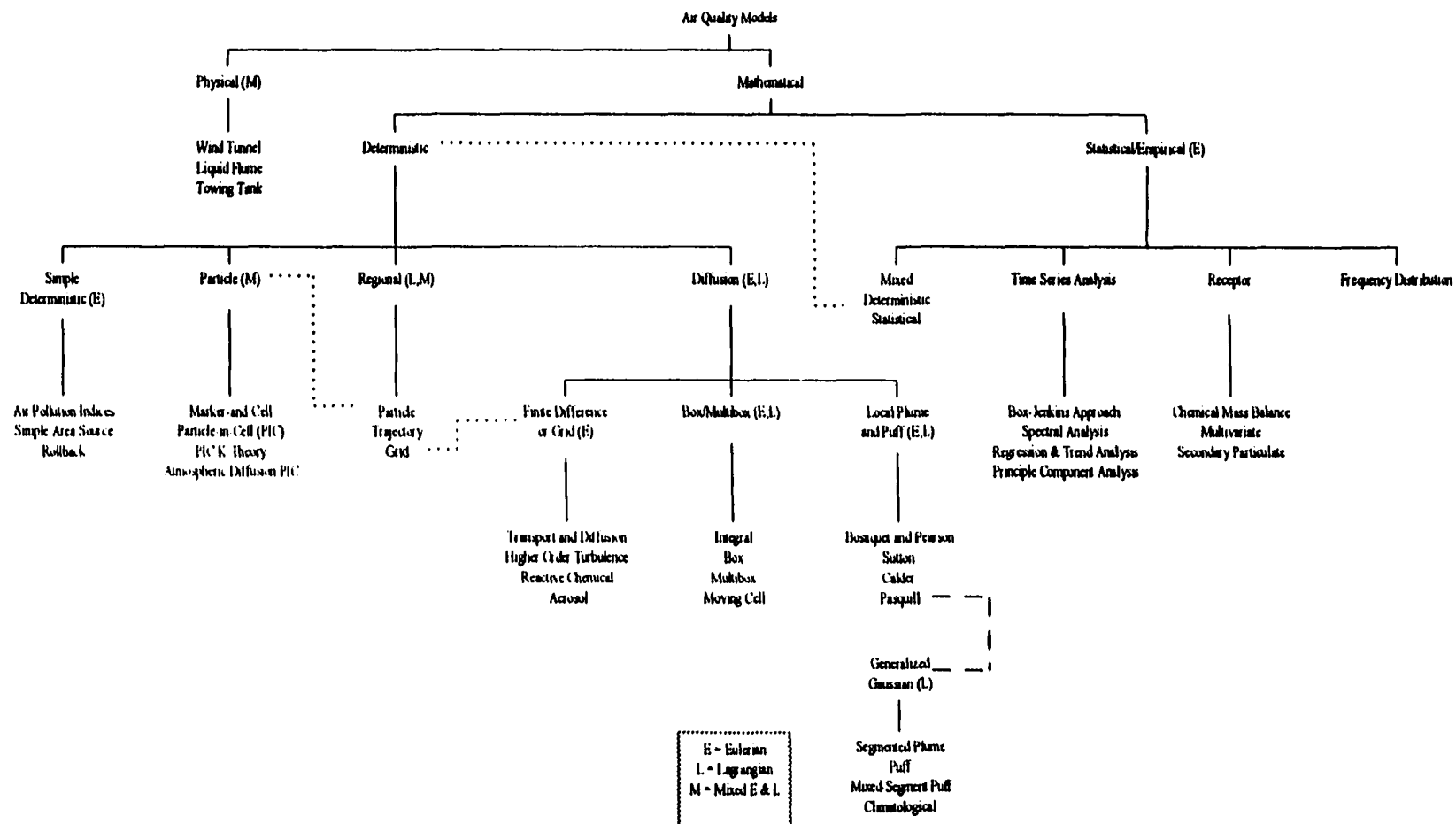
Figure 4.1: Air Quality Model Classification
