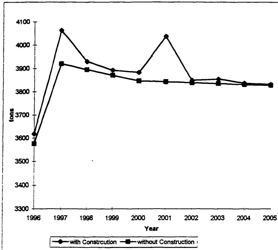
Figure D.3: AFB CO Comparisons
