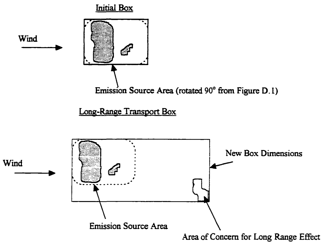
Figure D.13: Long Range Pollutant Transport Analysis
