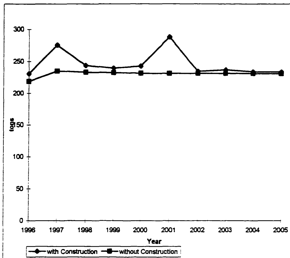
Figure D.7: AFB NOx Emission Comparisons
