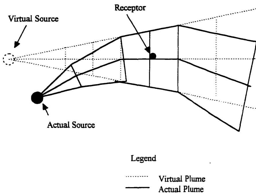
Figure A.7: The Segmented Plume Method (from Zannetti, 1990)
