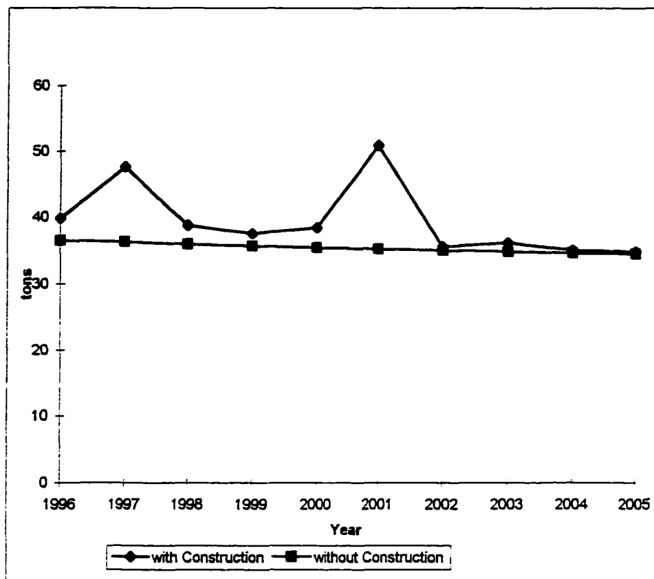
Figure 6.3: AFB PM10 Emissions Comparisons
