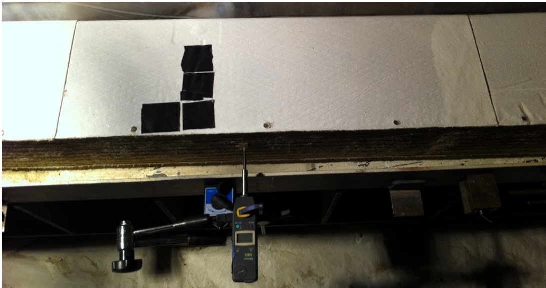
Figure 5.5 Plan view of the test setup showing the holes covered by tape, deflection gauge secured to the beam, and demec points glued on the surface of the concrete
