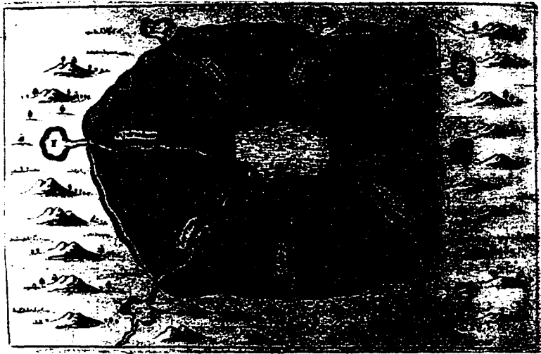
FIGURE 132. Growth of minerals beneath the ground. Kircher, Mundus subterraneus , 1664, 258. HSCI.
