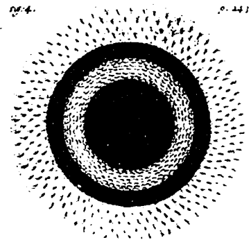
FIGURE 161. Whiston's fourth geogonic section. (Days 2 and 3.)
