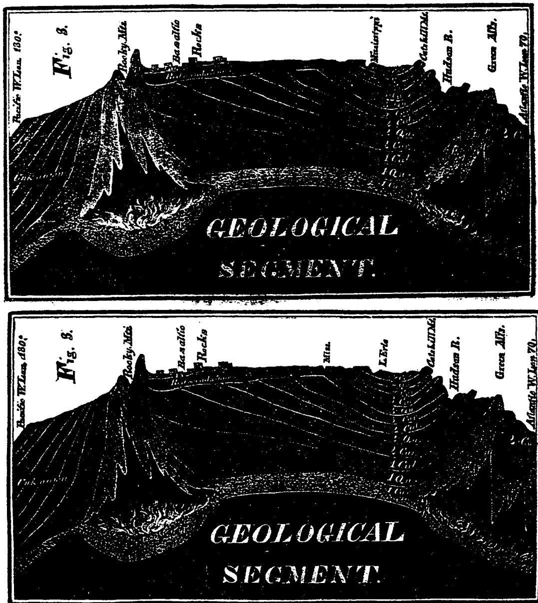
FIGURE 225. Amos Eaton, 1830 (top) and 1832 (below); Figure 3 . HSCI.
