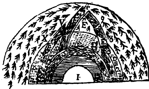
FIGURE 153. Gadroys, Systeme du Monde (1675), global hemisection. HSCI.
