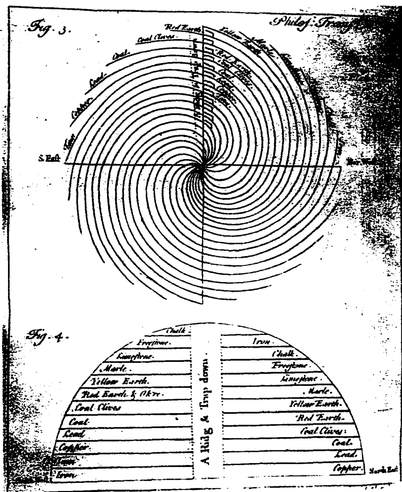
FIGURE 201. Strachey global section.
