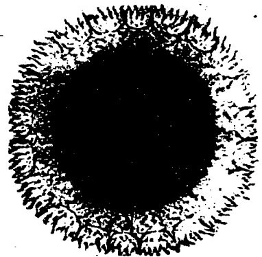
FIGURE 183. Fludd, I. II, 66. Extraction of earth. HSCI.
