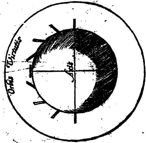
FIGURE 46. Dip or “verticity” of a terrella 45 depicted by William Gilbert, De magnete , 1600, Book V, chapter II. Image rotated to make axis vertical. HSCI.
