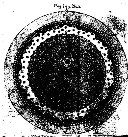
FIGURE 73. Beati, Tychonic positions, LH
