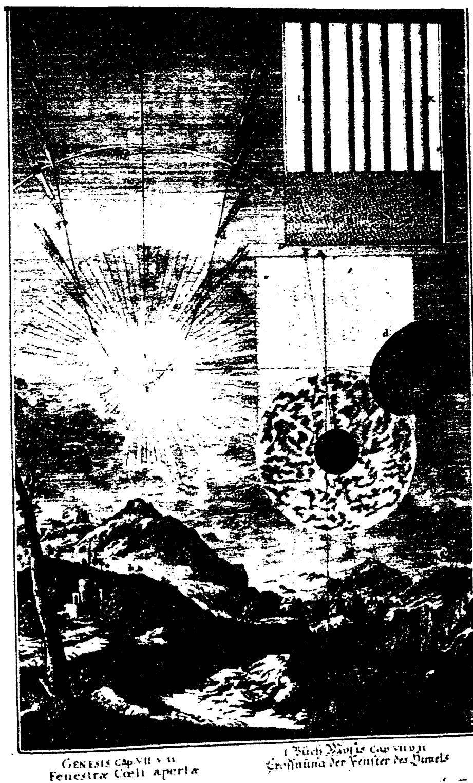
FIGURE 167. Scheuchzer's Deluge, Physica Sacra .
