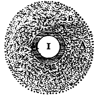
FIGURE 88. René Descartes, Principia philosophiae (1644), star-to-comet cosmogonic section. Later Plate XVI . LH.
