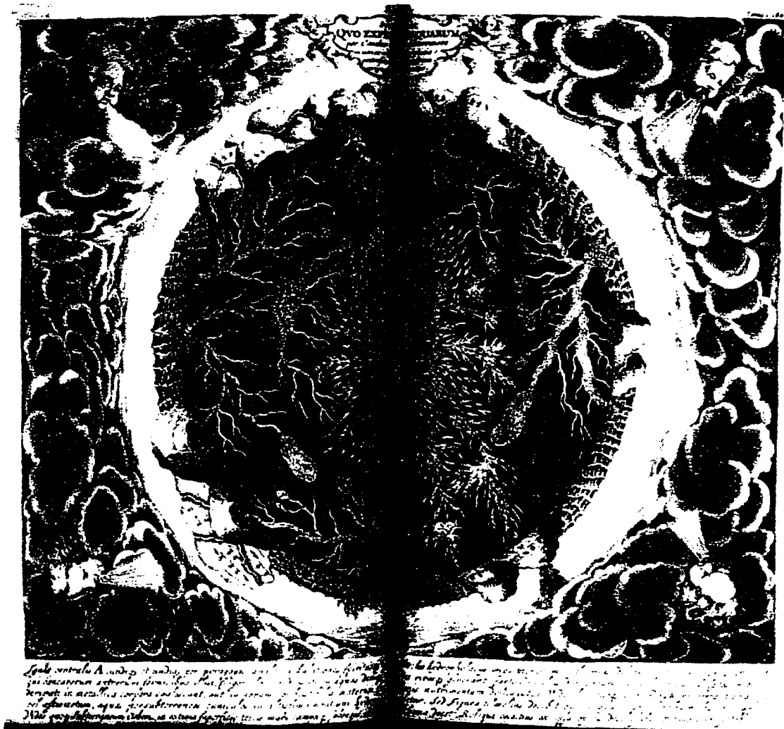
FIGURE 140. Global hydrophylacia , or circulation of water. Kircher, Mundus subterraneus , 1664, before p. 175. HSCI.
