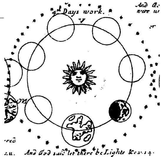
FIGURE 120. Nicholls, Figure V , "4th Days work. And God said let there be Lights &c. v. 14." LH.
