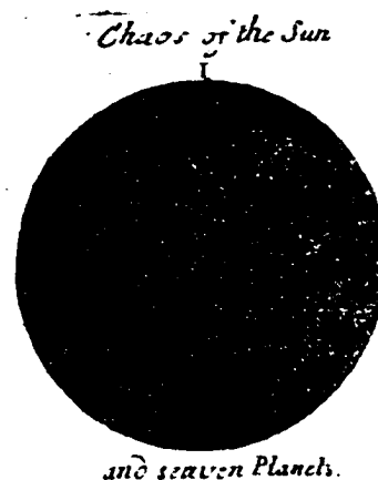
FIGURE 116. Nicholls, Figure I , "Chaos of the Sun and seaven Planets." A solar system cosmogonic section. LH.
