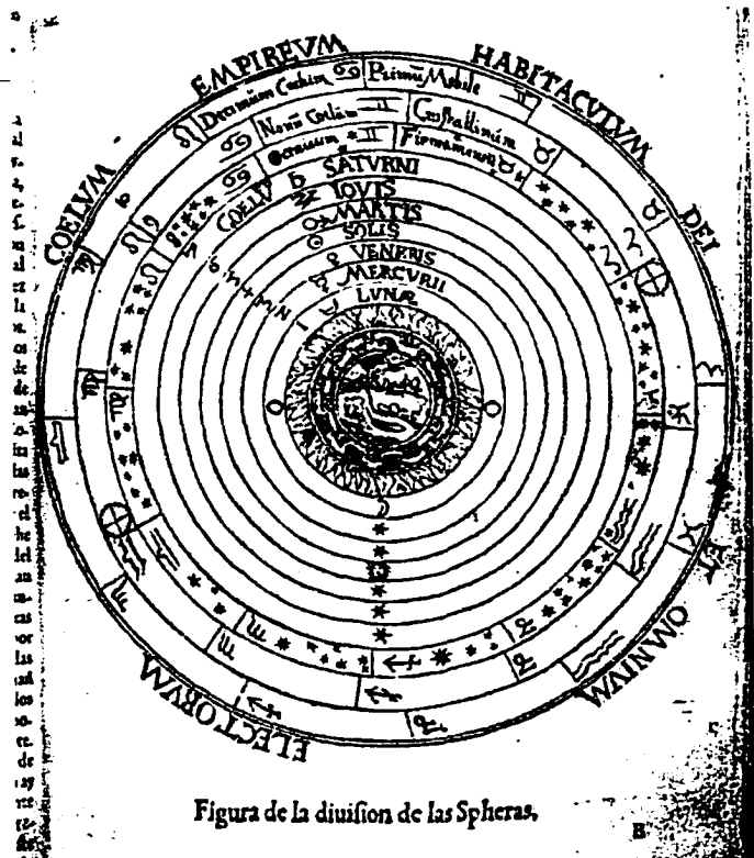
FIGURE 57. Peter Apian, Cosmographia (1548). LH.
