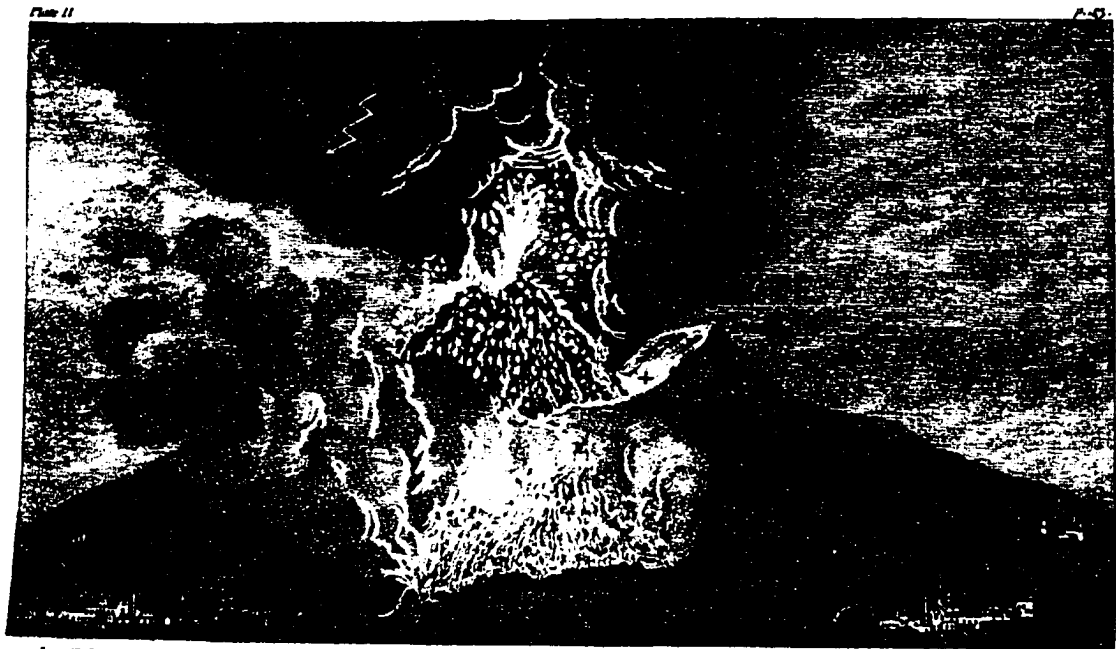
View of the GREAT ERUPTION of VESUVIUS 1767, from Torre dell'Annunziata
