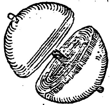
FIGURE 189. Kepler, Epitome of Copernican Astronomy , p. 121. The Earth as a spinning top.
