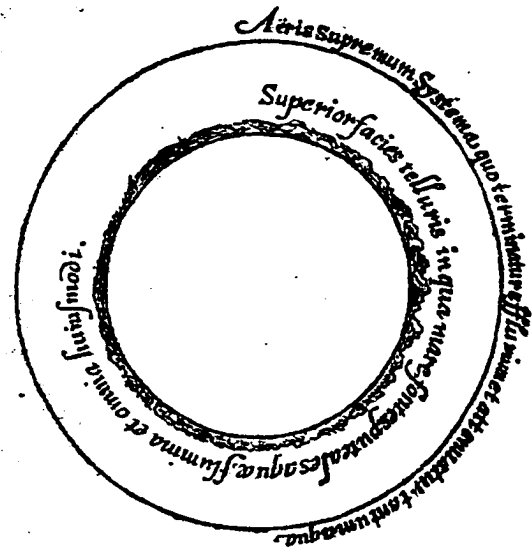
FIGURE 190. William Gilbert, De mundo (1651). HSCI. Partial meteorological section.
