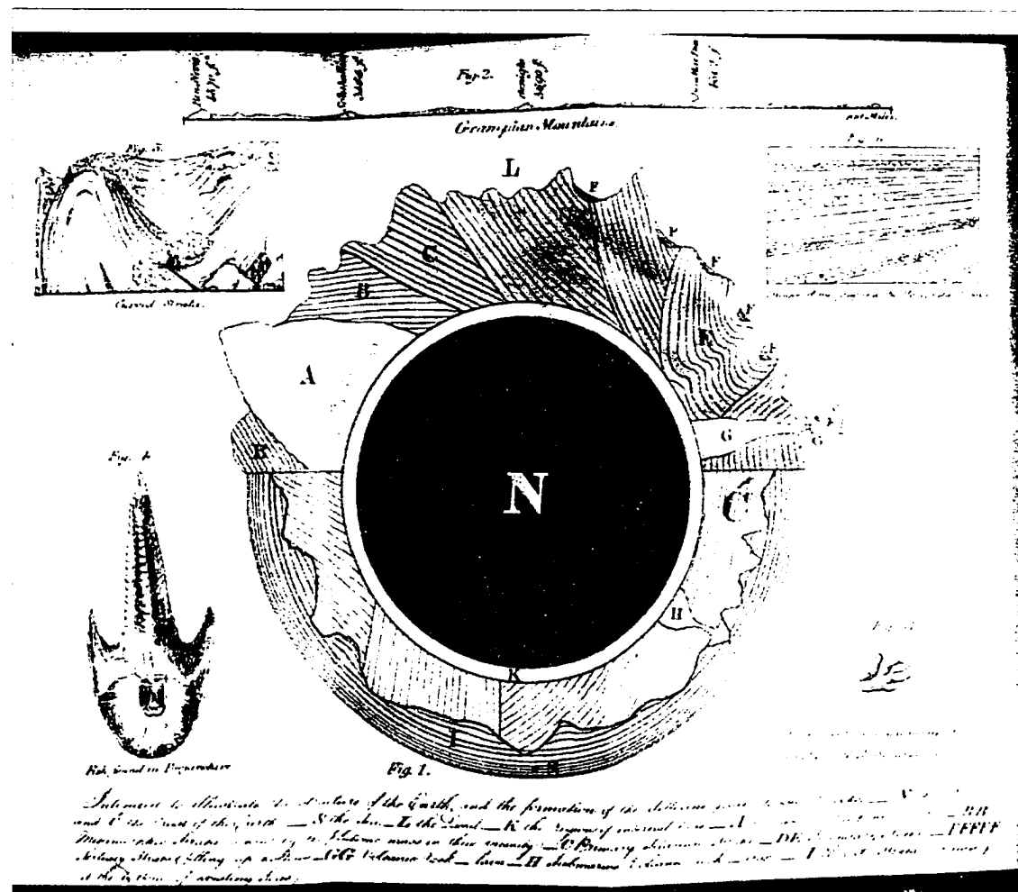
FIGURE 228. Mackintosh, Fig. 1 : Huttonian colored global section "Intended to illustrate the structure of the Earth, and the formation of the different great classes of rocks."
