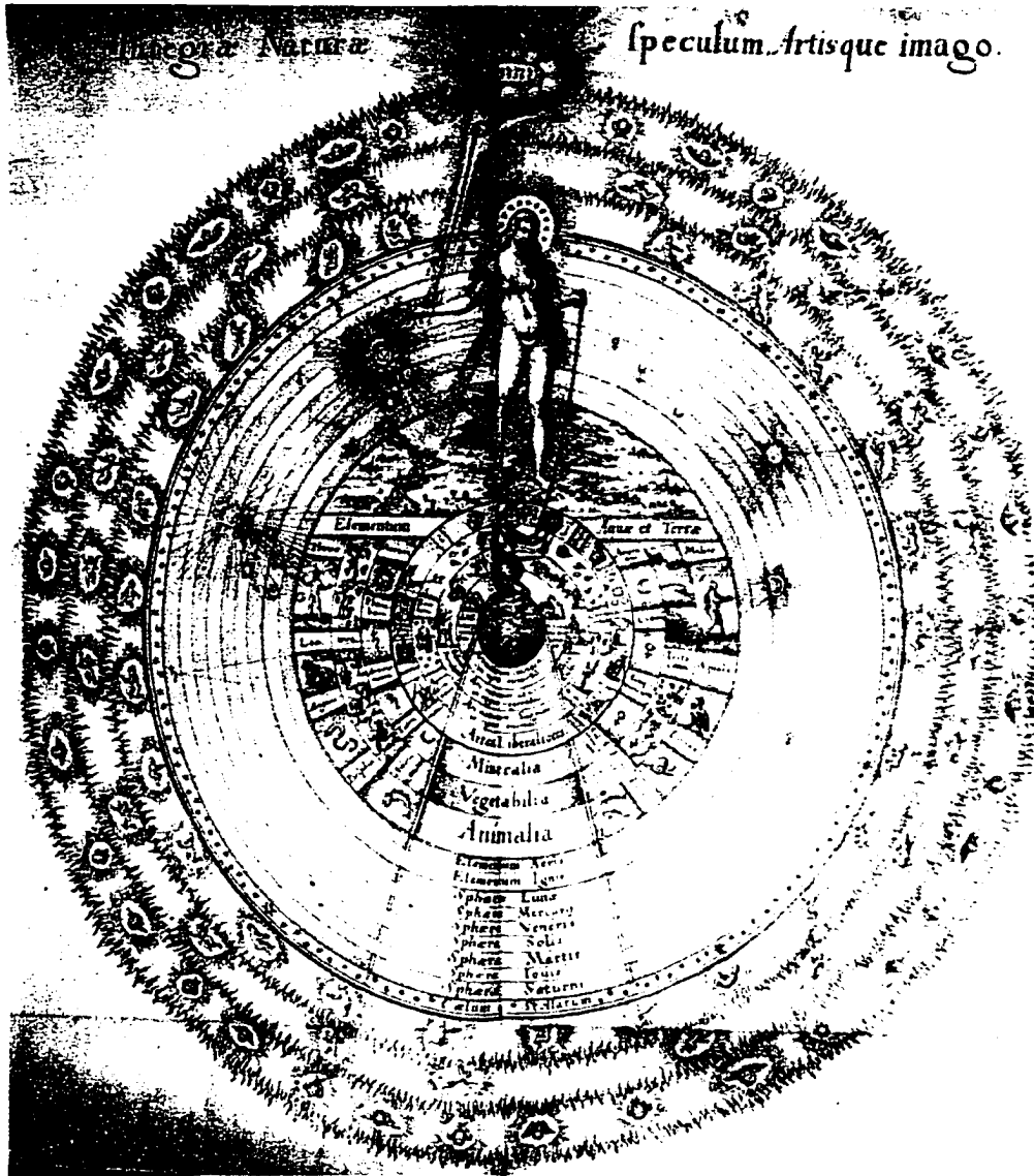
FIGURE 75. Robert Fludd, Integrae naturae . 1617. LH.
