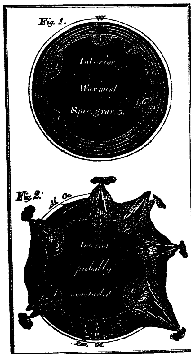
FIGURE 224. Amos Eaton, Geological Text-Book (1830), Figures 1 and 2 . HSCI.
