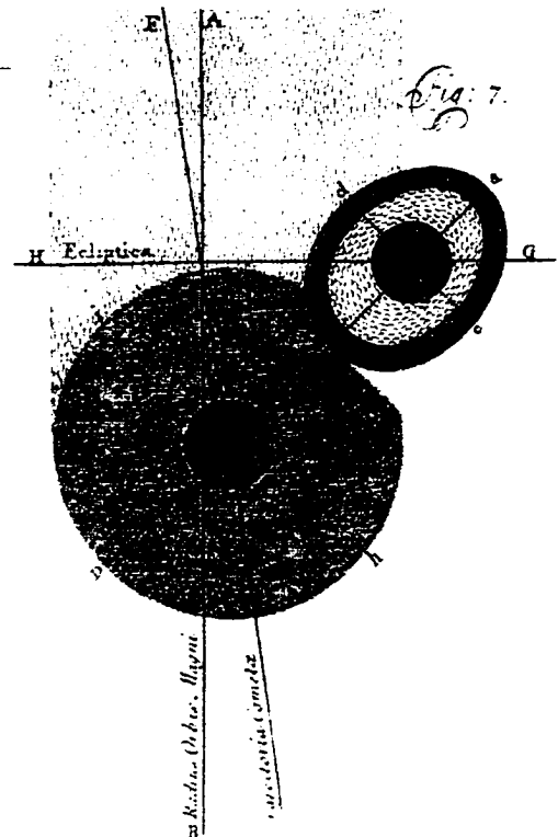
FIGURE 165. Whiston's Figure 7 . First day of the deluge.
