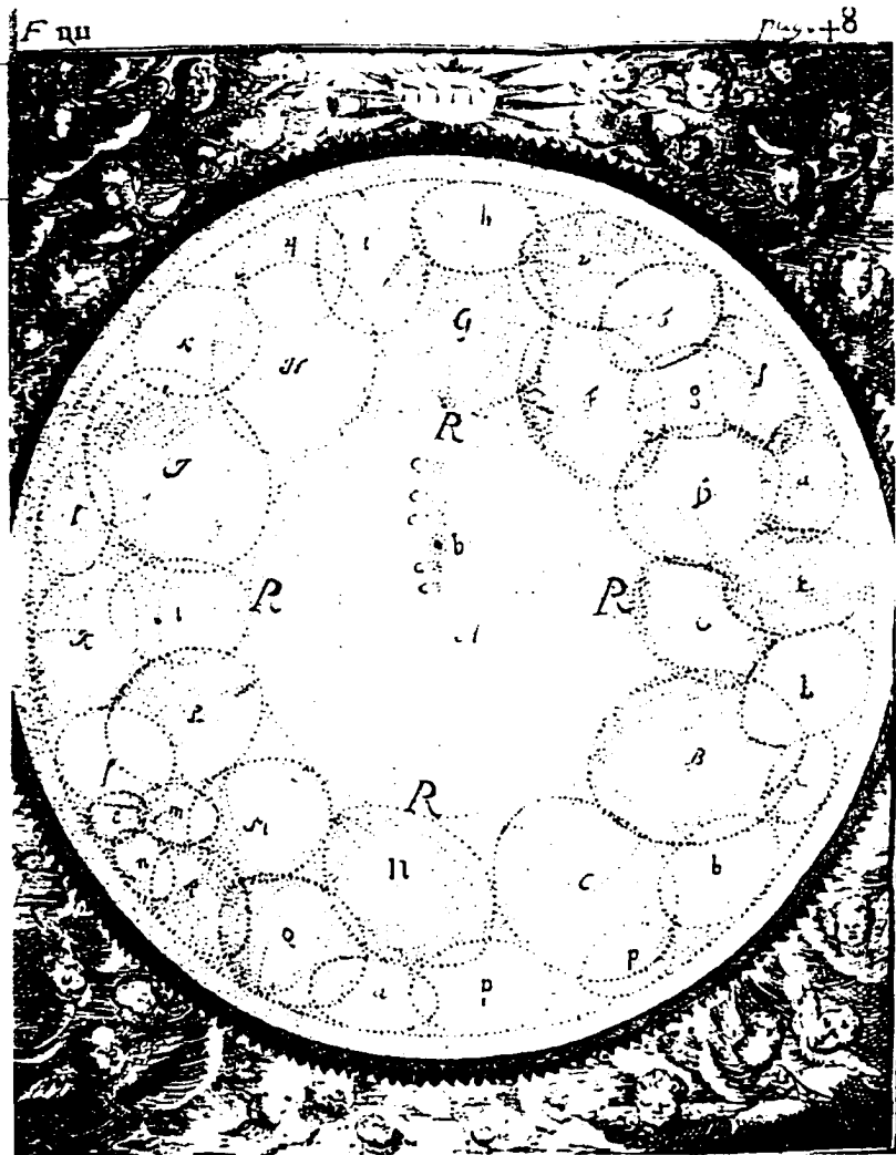
FIGURE 145. Barin Fig. IIII , p. 48; Second day. LH.
