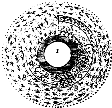
FIGURE 152. Gadroys, Systeme du Monde (1675), wheel of time. HSCI.
