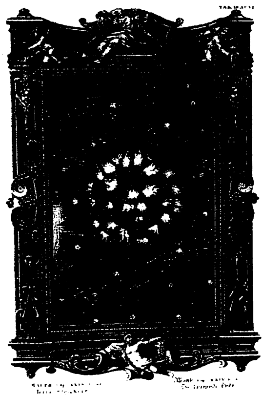
FIGURE 173. Scheuchzer, Revelation. LH.
