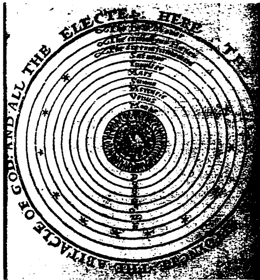
FIGURE 69. Leonard Digges, Ptolemaic Section a
