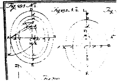
FIGURE 47. Maclaurin, Fluxions (1742), Hollow Earth. LH. 49
