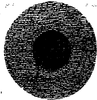
FIGURE 158. Whiston's first geogonic section. (Before day 1.)
