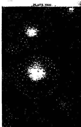
FIGURE 54. Wright, Plate XXXI. HSCI
