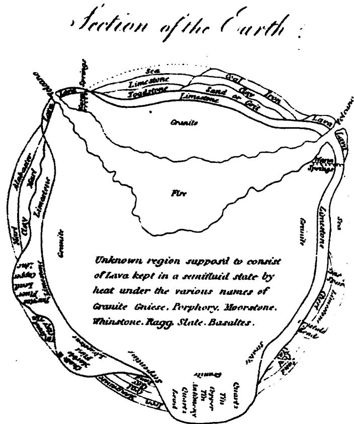
FIGURE 211. Erasmus Darwin, Botanic Garden (Dublin, 1799). "Section of the Earth" HSCI.
