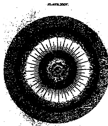
FIGURE 51. Wright, Plate XXV. HSCI
