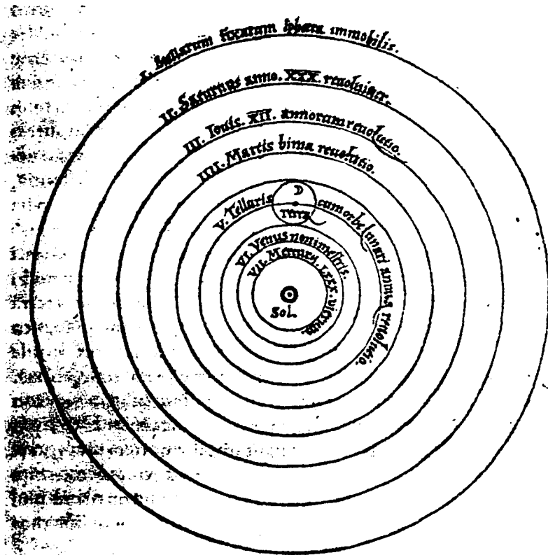
FIGURE 82. Nicolaus Copernicus, De revolutionibus orbium coelestium (1543). Book I, chapter 10. HSCI.
