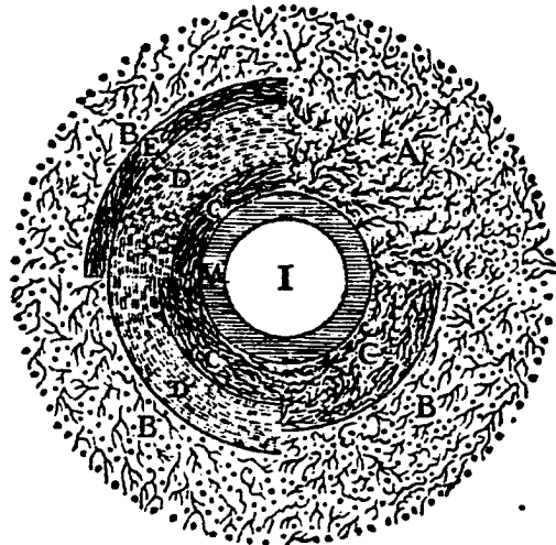
FIGURE 89. René Descartes, Principia philosophiae (1644), comet-to-planet cosmogonic section. LH.
