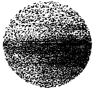
FIGURE 85. Burnet's geogonic series, Chaos section. Telluris Theoria Sacra (1681), Book I, ch. 5, p. 35. HSCI.
