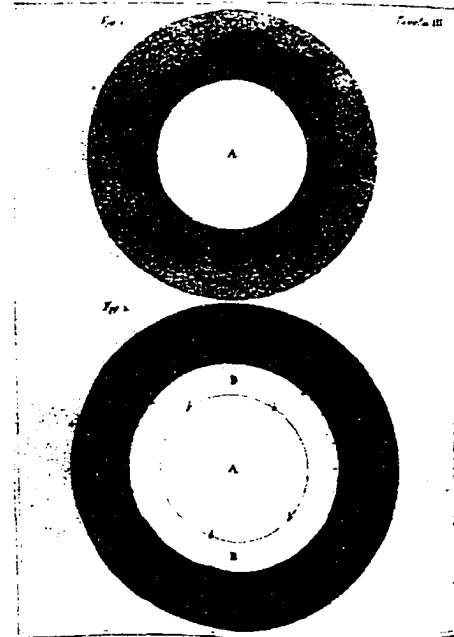
FIGURE 206. Moro, Tavola III
