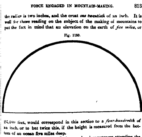
FIGURE 227. Dana, Manual of Geology .
