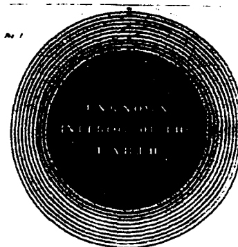
FIGURE 221. Amos Eaton, Index , 1820, Plate 1 , figure 1 (Day 2). LH and HSCI. 144
