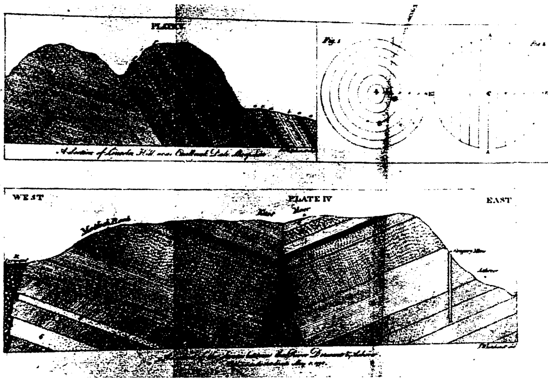
FIGURE 209. Whitehurst, Plates IV and V . HSCI.
