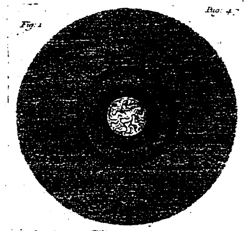
FIGURE 168. Warren's Figure 1 . Summary of Burnet's geogonic series.
