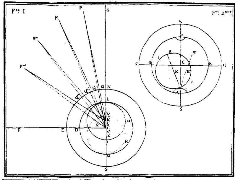
FIGURE 30. Louis Bertrand, Figures 1 and 2
