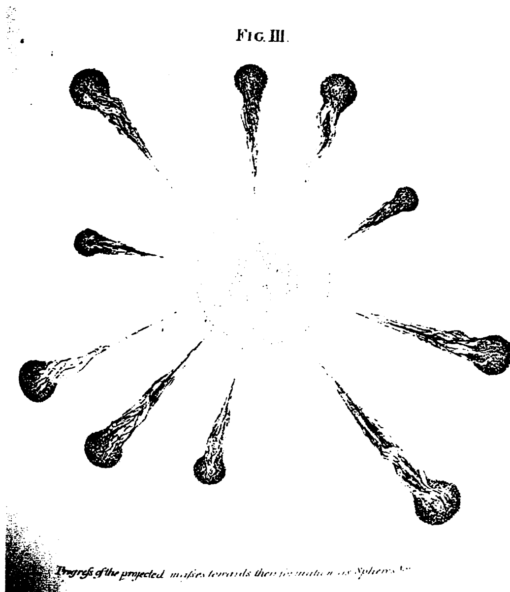
FIGURE 11. John Hay. Fig. III, New Theory of the Earth (Edinburgh, 1824), LH.
