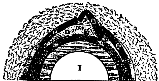
FIGURE 102. Second global hemisection. Descartes, Principia philosophiae , 1644. LH.
