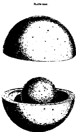
FIGURE 52. Wright, Plate XXVI. HSCI
