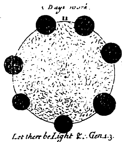
FIGURE 117. Nicholls, Figure II , "1. Days work. Let there be Light &c. Gen. 1.3" LH.
