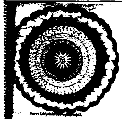
FIGURE 187. Fludd, I. I, 43. Extraction of aetherial bodies. HSCI.
