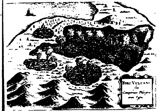
FIGURE 129. Camporum phlegra , from Kircher, Mundus subterraneus , 1664, 179. HSCI.
