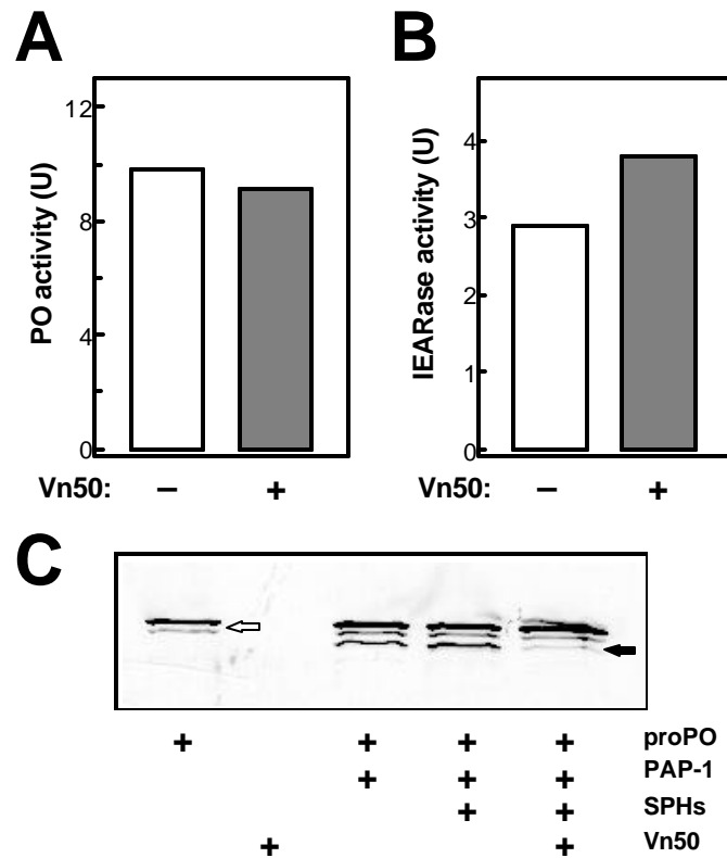
Fig. 6 Mechanistic analysis of the proPO activation regulation by Vn50
