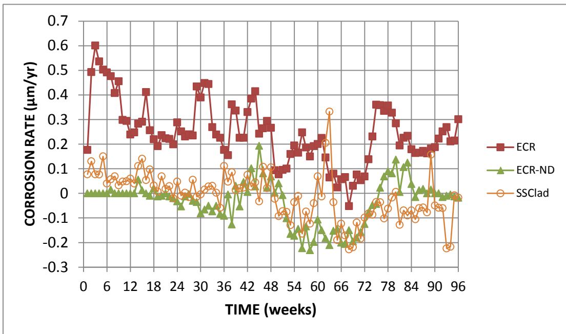
Figure 75b: Average corrosion rate of cracked beam specimens containing conventional reinforcement, epoxy coated reinforcement, undamaged epoxy coated reinforcement, and undamaged stainless steel clad reinforcement (different scale)
