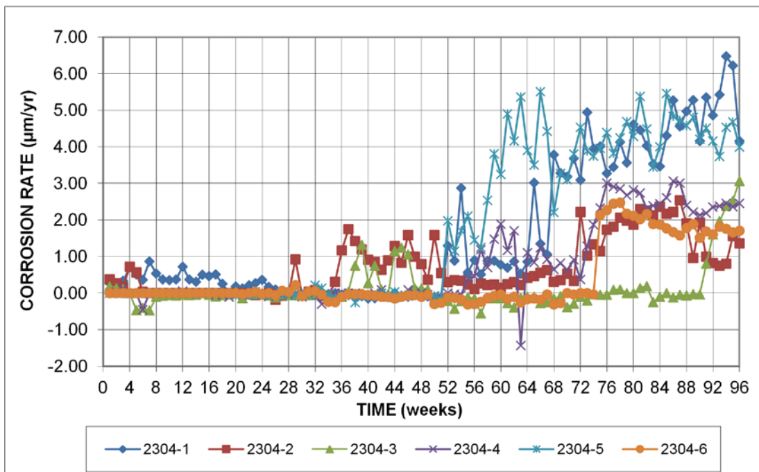
Figure 67: Individual corrosion rates ( \mu\text{m}/\text{yr} ) based on total area for cracked beam specimens with 2304 reinforcement
