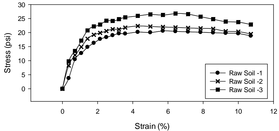
Figure 67: Raw Soil Untreated 28-Day Curing
