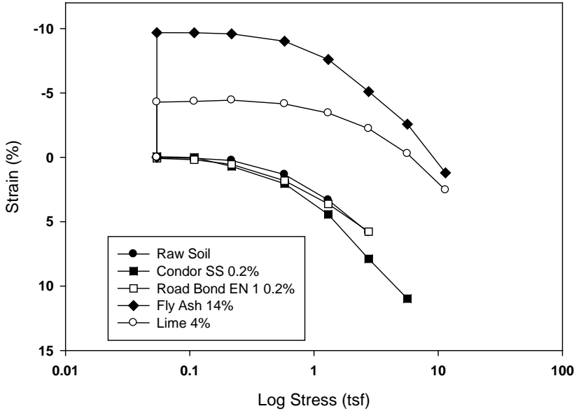
Figure 30: Vernon Soil Free Swell Oedometer
