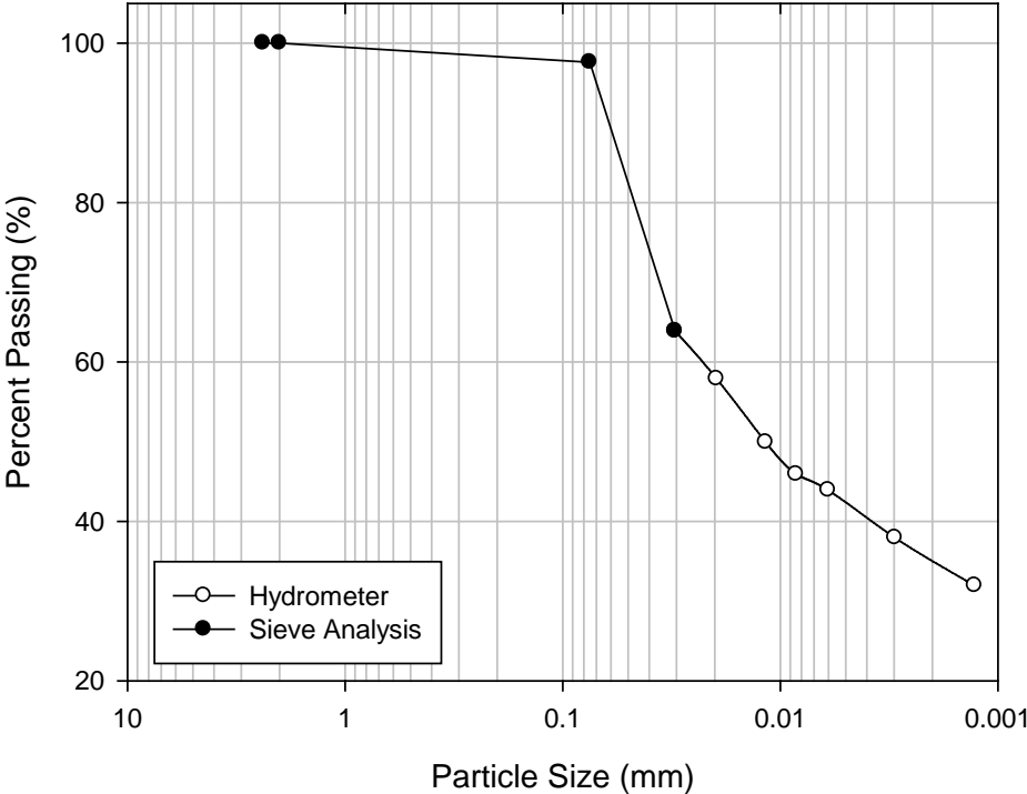
Figure 14: Renfrow Clay Grain Size Distribution
