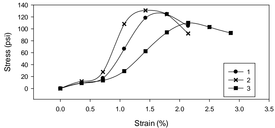
Figure 70: Renfrow Clay with Lime 6% 14-Day Curing
