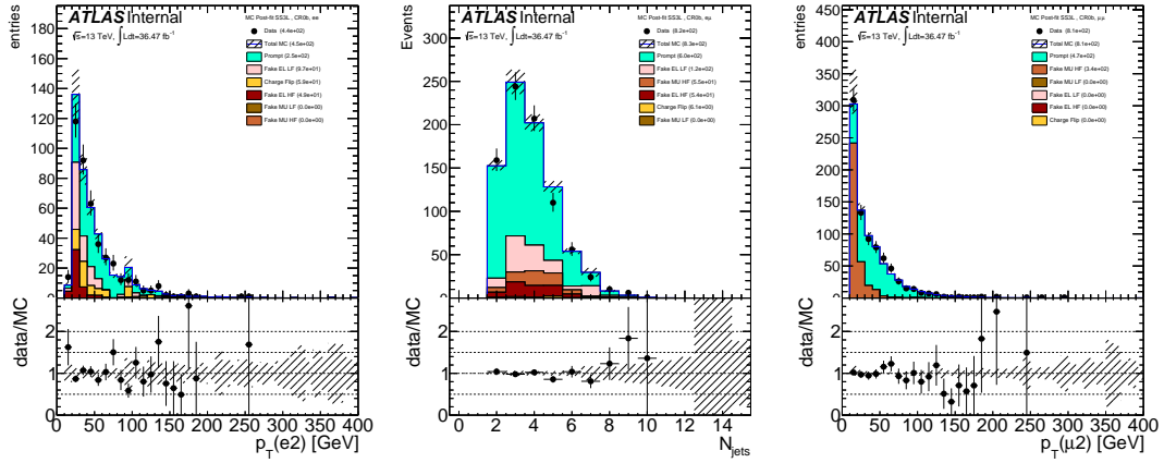
Figure 6.3: Post-fit distributions for ee channel (left), for e\mu channel (middle), and for \mu\mu channel (right) from CR0b that were used in the fit to extract the FNP lepton and charge flip multipliers. The generator used in these plots is POWHEG-BOX +Pythia . The hashed band represents the sum of systematic uncertainties on the predictions.
