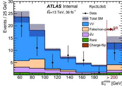
(c) Rpc3L0bS before the E_T^{\text{miss}} requirement re- (d) Rpc3L1bS before the E_T^{\text{miss}} requirement
