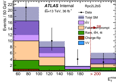
(a) Rpc2L2bS before the E_T^{\text{miss}} requirement re- (b) Rpc2Lsoft2b before the E_T^{\text{miss}} requirement
