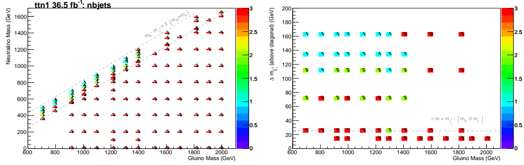
Figure 5.16: Optimal cut on the number of b -jets leading to the best discovery significance.
