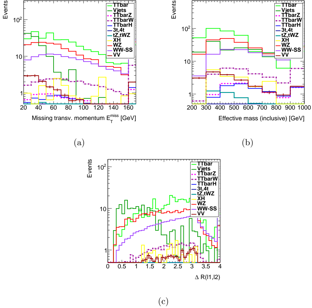
Figure 7.2: (a) E_T^{\text{miss}} , (b) m_{\text{eff}} , and (c) \min \Delta R(\ell_1, \ell_2) after lepton and jet selection of the W^\pm W^\pm -VR (and no additional requirements). Signal regions are vetoed. All MC samples are normalized to a luminosity of 36.1 \text{ fb}^{-1} . The last bin includes overflow.
