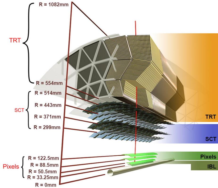
Figure 3.7: Drawing showing the detector elements crossed by a charged particle with 10 \text{ GeV } p_T in the barrel of the Inner Detector. The particle emerges from the interaction point and traverses the beam-pipe, one IBL layer, three pixel layers, four double layers of SCT sensors, and around 35 TRT straws.
