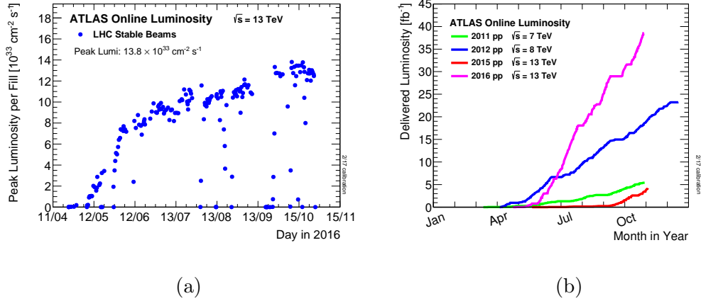
Figure 3.2: (a) The peak instantaneous luminosity delivered to ATLAS in 2016 and (b) the cumulative luminosity delivered to ATLAS between 2011 and 2016, during stable beams for pp collisions
