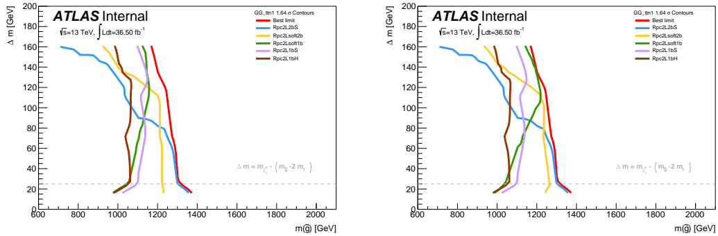
Figure 5.17: Comparison of significance contours at 1.64\sigma for 36.5 \text{ fb}^{-1} between Rpc2Lsoft2b and Rpc2Lsoft1b and other signal regions in the off-diagonal region (left) without and (right) with an upper cut on the leading lepton p_T .
