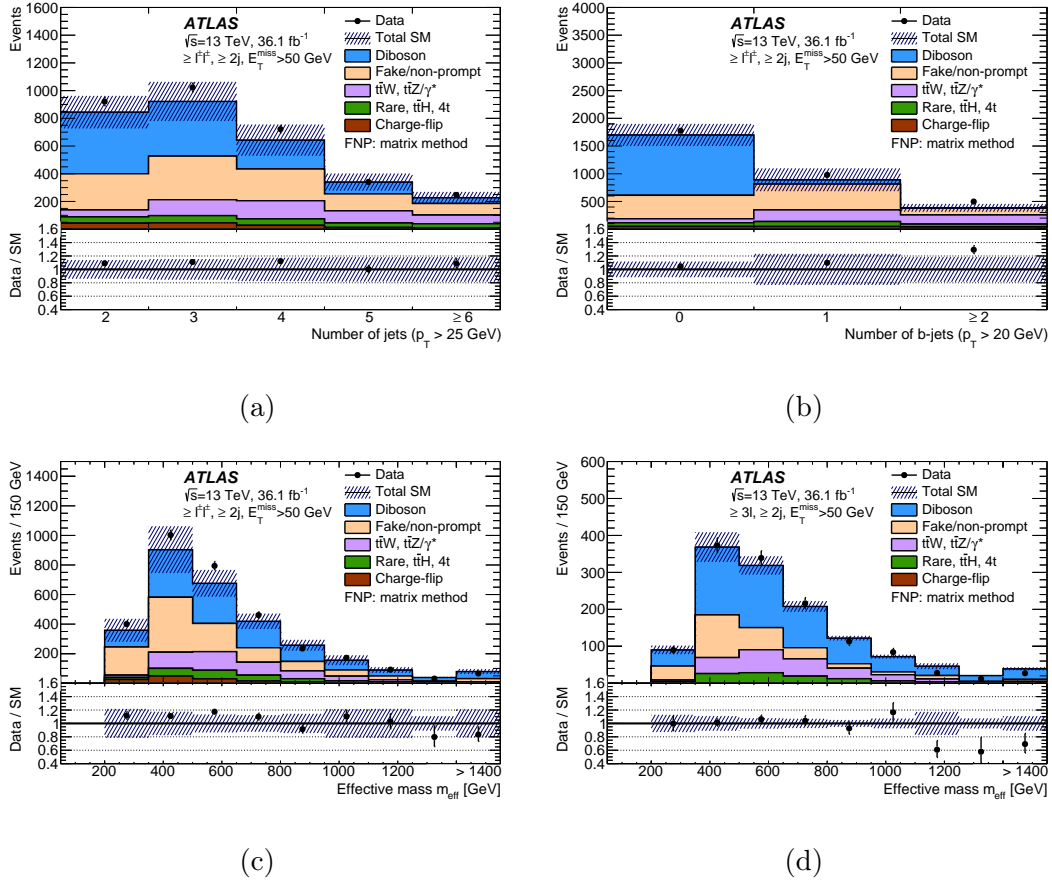
Figure 7.19: Distributions of (a) the number of jets, (b) the number of b -tagged jets and (c), (d) the effective mass. The distributions are made after requiring at least two jets ( p_T > 40 \text{ GeV} ) and E_T^{\text{miss}} > 50 \text{ GeV} , as well as at least two same-sign leptons ((a), (b), (c)) or three leptons (d). The uncertainty bands include the statistical uncertainties for the background prediction as well as the systematic uncertainties for fake- or non-prompt-lepton backgrounds (using the matrix method) and charge-flip electrons. Not included are theoretical uncertainties in the irreducible background contributions. The rare category is defined in the text.
