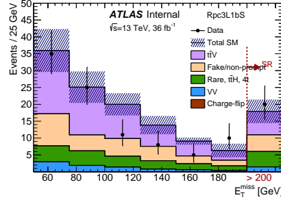
(c) Rpc3L0bS before the E_T^{\text{miss}} requirement re- (d) Rpc3L1bS before the E_T^{\text{miss}} requirement
