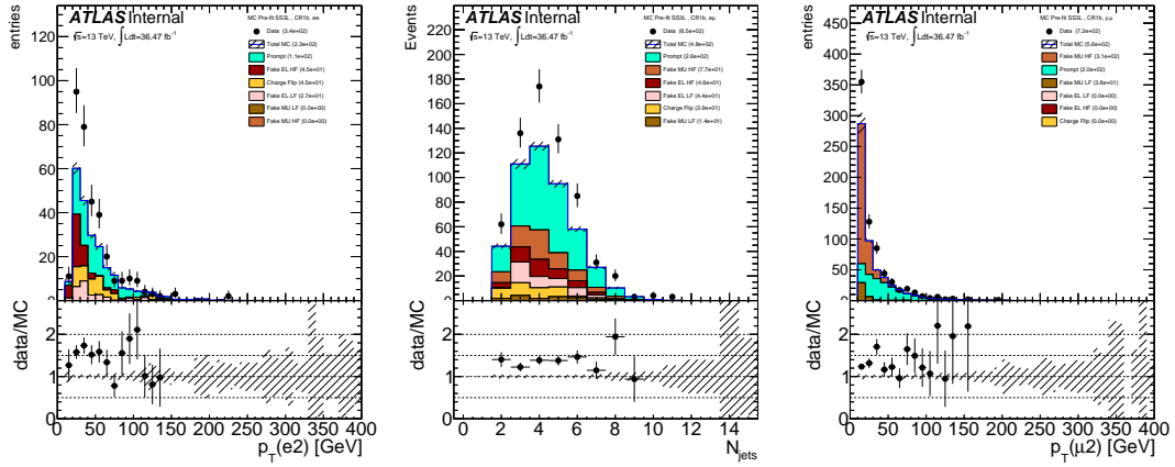
Figure 6.4: Pre-fit distributions for ee channel (left), for e\mu channel (middle), and for \mu\mu channel (right) from CR1b that were used in the fit to extract the FNP lepton and charge flip multipliers. The generator used in these plots is POWHEG-BOX +Pythia. The hashed band represents the sum of systematic uncertainties on the predictions.
