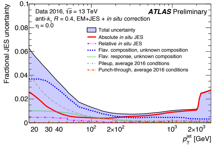
Figure 3.21: Fractional jet energy scale systematic uncertainty components as a function of p_T for anti- k_t jets at \eta = 0.0 with distance parameter of R = 0.4 after calibration. The total uncertainty (all components summed in quadrature) is shown as a filled blue region topped by a solid black line.
