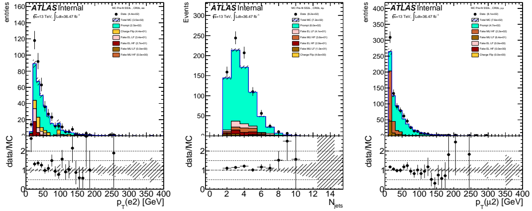
Figure 6.2: Pre-fit distributions for ee channel (left), for e\mu channel (middle), and for \mu\mu channel (right) from CR0b that were used in the fit to extract the FNP lepton and charge flip multipliers. The generator used in these plots is POWHEG-BOX +Pythia. The hashed band represents the sum of systematic uncertainties on the predictions.
