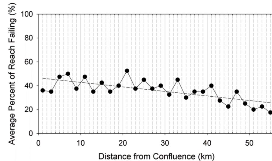
Figure 3. Percentage of streambanks eroding and failing in the Barren Fork Creek watershed in Oklahoma from a helicopter video survey. The x-axis is the distance from the confluence with the Illinois River in Oklahoma. Source: Miller et al. (2014).
